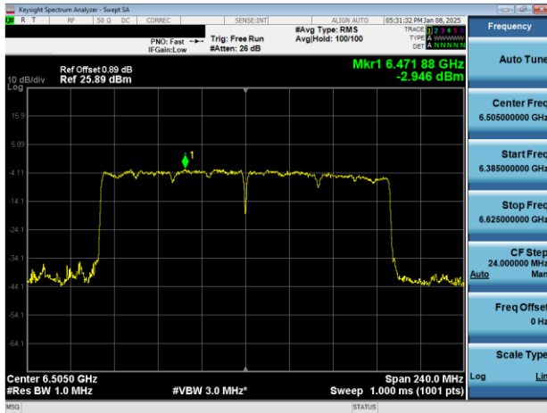
Plot 7-479. PSD Plot CDD Diversity Antenna 5T (160MHz 802.11ax RU996x2 (UNII Band 6) – Ch. 111)
