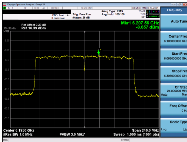
Plot 7-512. PSD Plot SDM Diversity Antenna 1b (160MHz 802.11ax RU996x2 (UNII Band 5) - Ch. 47)
