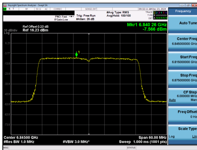
Plot 7-427. PSD Plot SDM Primary Antenna 5T (40MHz 802.11ax RU484 (UNII Band 7) – Ch. 179)
