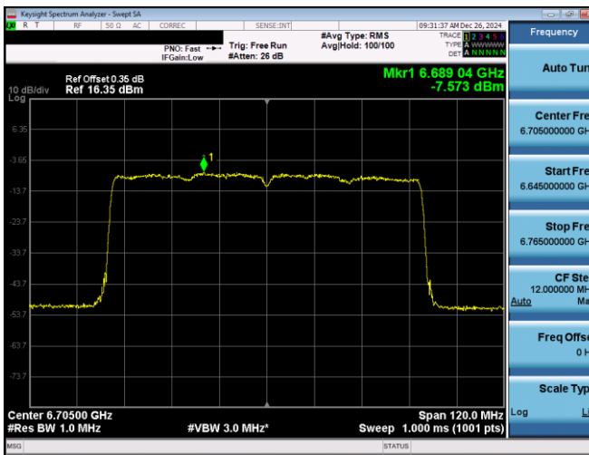
Plot 7-430. PSD Plot SDM Primary Antenna 3b (80MHz 802.11ax RU996 (UNII Band 7) – Ch. 151)
