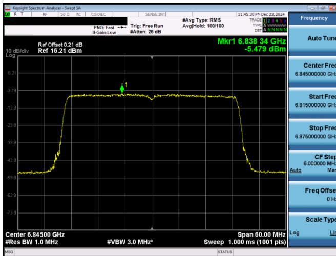
Plot 7-270. PSD Plot Antenna 3b (40MHz 802.11ax RU484 (UNII Band 7) – Ch. 179)
