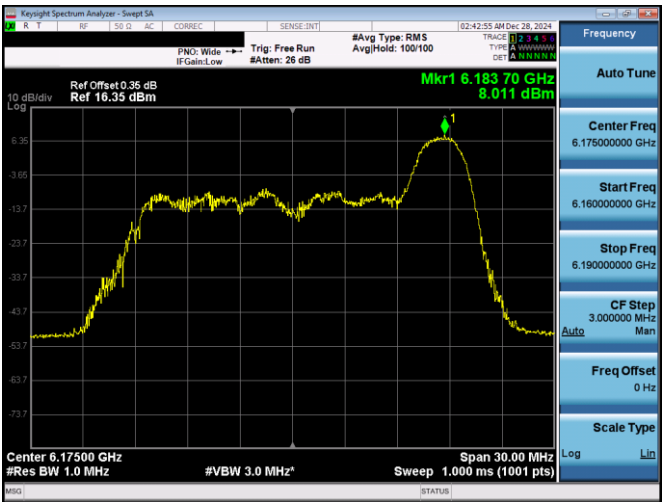
Plot 7-225. PSD Plot Antenna 3b (20MHz 802.11ax RU26 (UNII Band 5) – Ch. 45)
