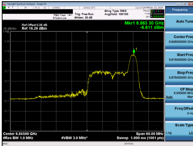
Plot 7-266. PSD Plot Antenna 3b (40MHz 802.11ax RU26 (UNII Band 7) – Ch. 179)
