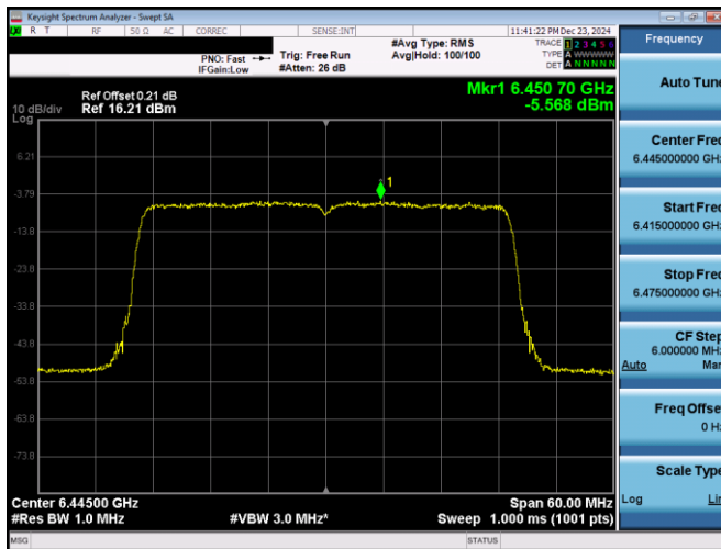
Plot 7-262. PSD Plot Antenna 3b (40MHz 802.11ax RU484 (UNII Band 6) – Ch. 99)
