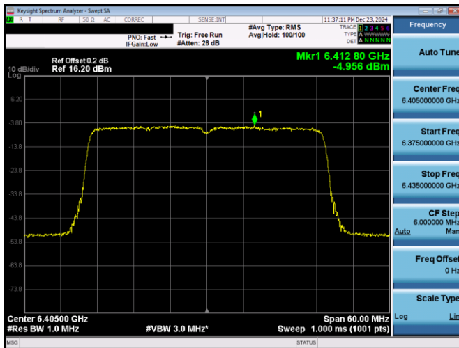
Plot 7-254. PSD Plot Antenna 3b (40MHz 802.11ax RU484 (UNII Band 5) – Ch. 91)
