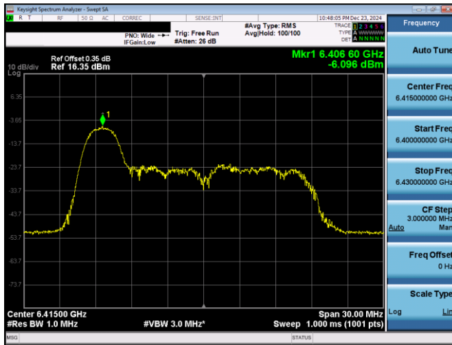
Plot 7-249. PSD Plot Antenna 3b (20MHz 802.11ax RU26 (UNII Band 5) – Ch. 93)
