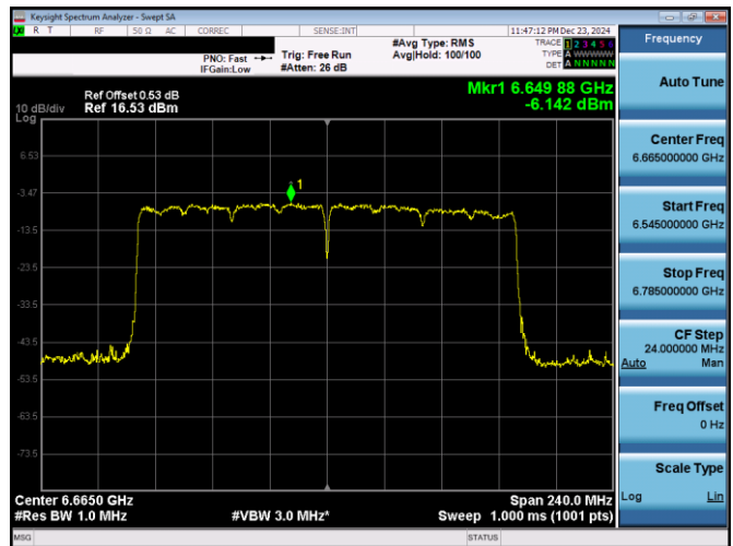
Plot 7-272. PSD Plot Antenna 3b (160MHz 802.11ax RU26 (UNII Band 7) – Ch. 143)
