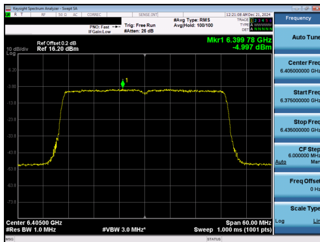
Plot 7-198. PSD Plot Antenna 5T (40MHz 802.11ax RU484 (UNII Band 5) – Ch. 91)
