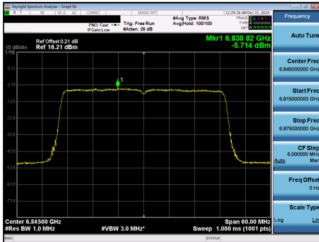
Plot 7-214. PSD Plot Antenna 5T (40MHz 802.11ax RU484 (UNII Band 7) – Ch. 179)
