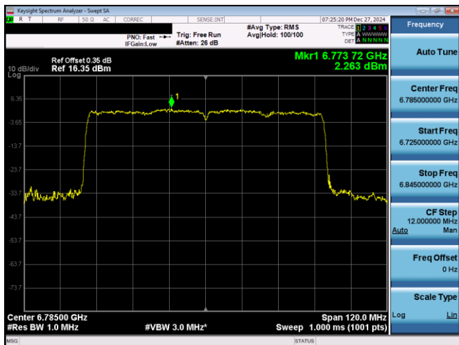
Plot 7-191. PSD Plot Antenna 5T (80MHz 802.11ax RU996 (UNII Band 7) – Ch. 167)
