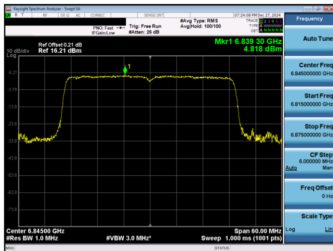
Plot 7-190. PSD Plot Antenna 5T (40MHz 802.11ax RU484 (UNII Band 7) – Ch. 179)
