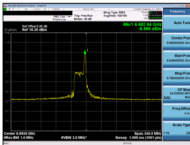
Plot 7-212. PSD Plot Antenna 5T (160MHz 802.11ax RU26 (UNII Band 7) – Ch. 143)
