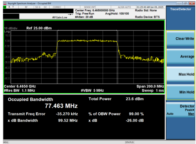
Plot 7-127. 26dB & 99% Bandwidth Plot Antenna 1b (80MHz 802.11ax RU996 (UNII Band 6) – Ch. 103)
