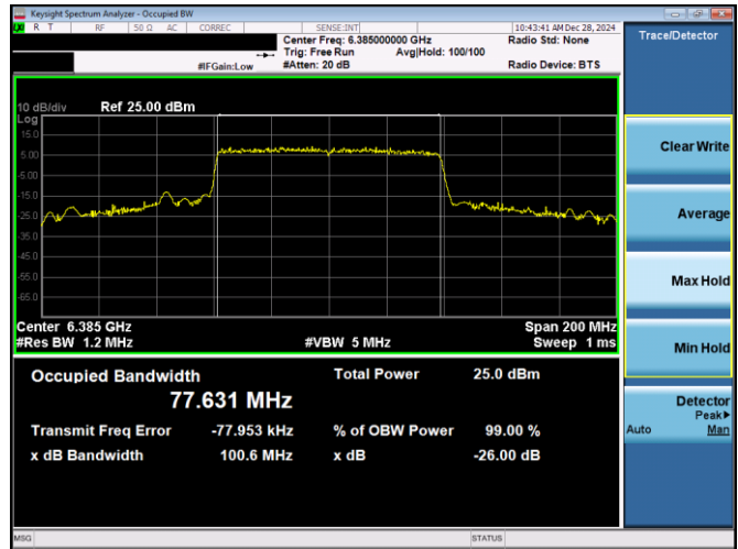
Plot 7-119. 26dB & 99% Bandwidth Plot Antenna 1b (80MHz 802.11ax RU996 (UNII Band 5) - Ch. 87)
