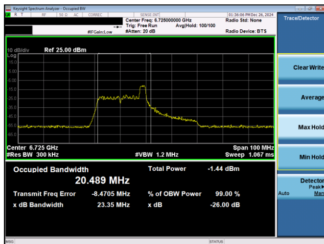
Plot 7-154. 26dB & 99% Bandwidth Plot Antenna 1b (40MHz 802.11ax RU26 (UNII Band 7) – Ch. 155)
