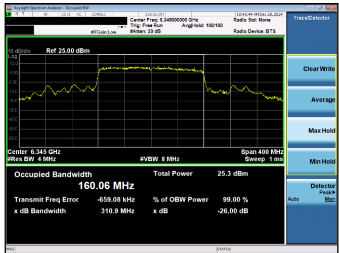
Plot 7-120. 26dB & 99% Bandwidth Plot Antenna 1b (160MHz 802.11ax RU996x2 (UNII Band 5) - Ch. 79)
