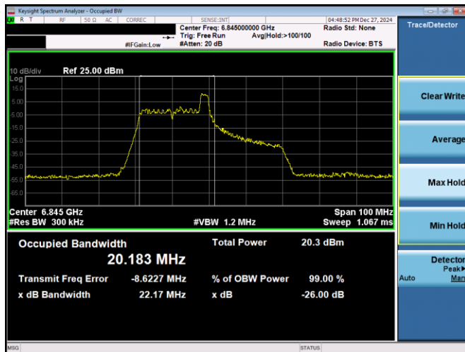
Plot 7-18. 26dB & 99% Bandwidth Plot Antenna 5T (40MHz 802.11ax RU26 (UNII Band 7) – Ch. 179)
