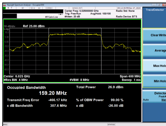
Plot 7-8. 26dB & 99% Bandwidth Plot Antenna WF8 (160MHz 802.11ax RU996x2 (UNII Band 5) – Ch. 15)
