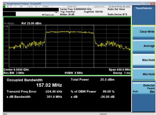
Plot 7-16. 26dB & 99% Bandwidth Plot Antenna WF8 (160MHz 802.11ax RU996x2 (UNII Band 6) – Ch. 111)
