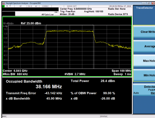
Plot 7-22. 26dB & 99% Bandwidth Plot Antenna 5T (40MHz 802.11ax RU484 (UNII Band 7) – Ch. 179)
