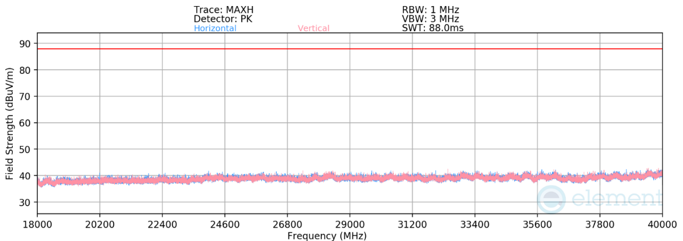
Plot 7-552. Radiated Spurious Emissions 18-40GHz CDD Diversity (802.11ax – Ch. 45)
