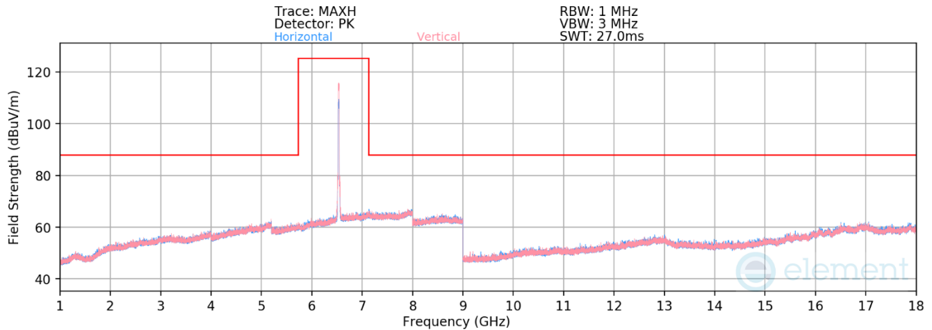
Plot 7-558. Radiated Spurious Emissions above 1GHz SDM Diversity (802.11ax – Ch. 117)
