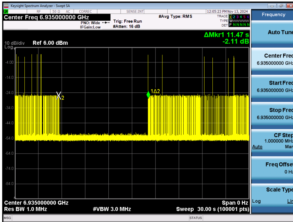
Plot 7-526. Contention Based Protocol Timing Plot – UNII 8 – 20MHz Channel 197
