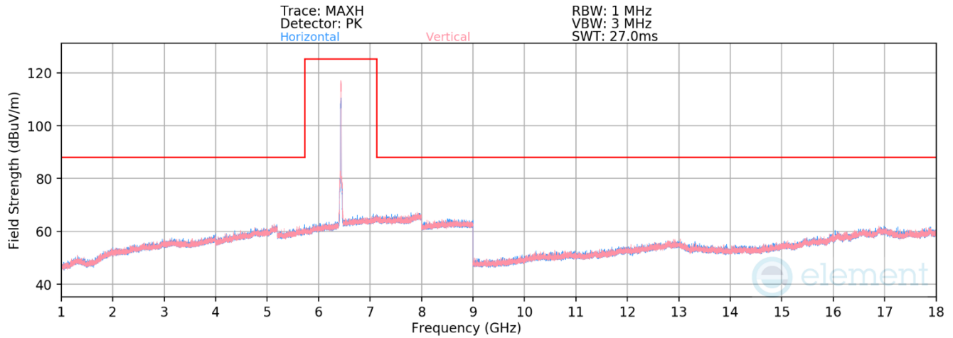
Plot 7-538. Radiated Spurious Emissions above 1GHz CDD Primary (802.11ax – Ch. 97)
