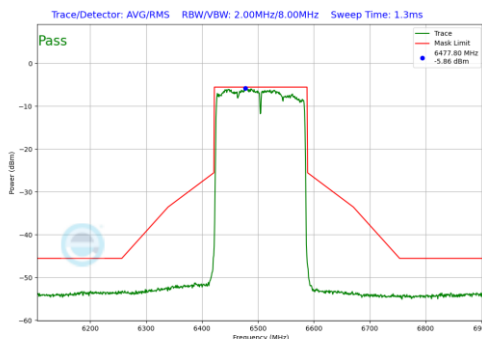
Plot 7-480. In-Band Emission Plot SDM Diversity Antenna 5T (160MHz 802.11ax (UNII Band 6) – Ch. 111)
