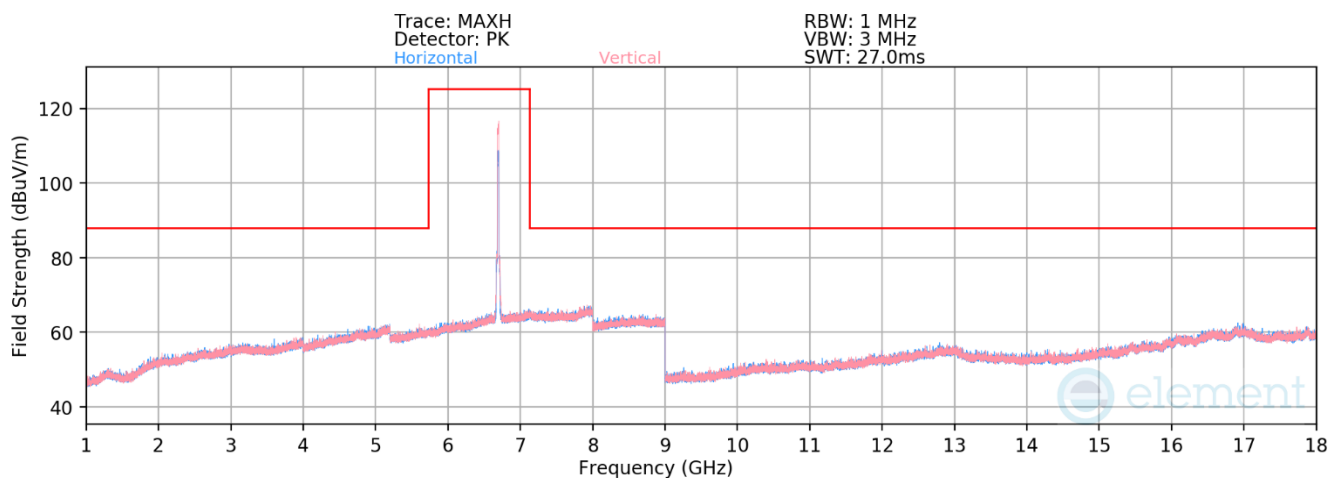
Plot 7-543. Radiated Spurious Emissions above 1GHz CDD Primary (802.11ax – Ch. 149)
