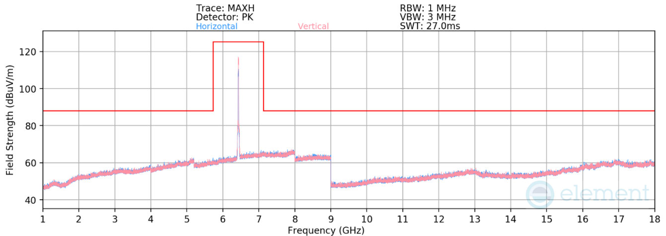
Plot 7-540. Radiated Spurious Emissions above 1GHz CDD Primary (802.11ax – Ch. 113)
