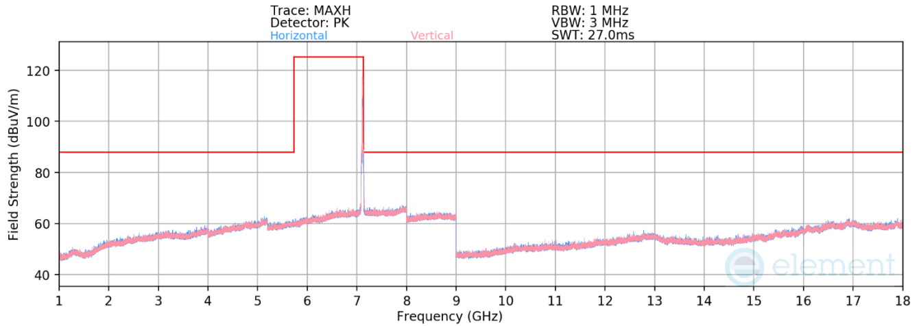
Plot 7-549. Radiated Spurious Emissions above 1GHz CDD Primary (802.11ax – Ch. 233)
