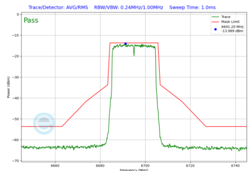
Plot 7-482. In-Band Emission Plot SDM Diversity Antenna 5T (20MHz 802.11ax (UNII Band 7) – Ch. 149)
