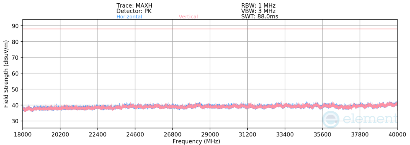
Plot 7-535. Radiated Spurious Emissions 18-40GHz SDM (802.11ax – Ch. 1)
