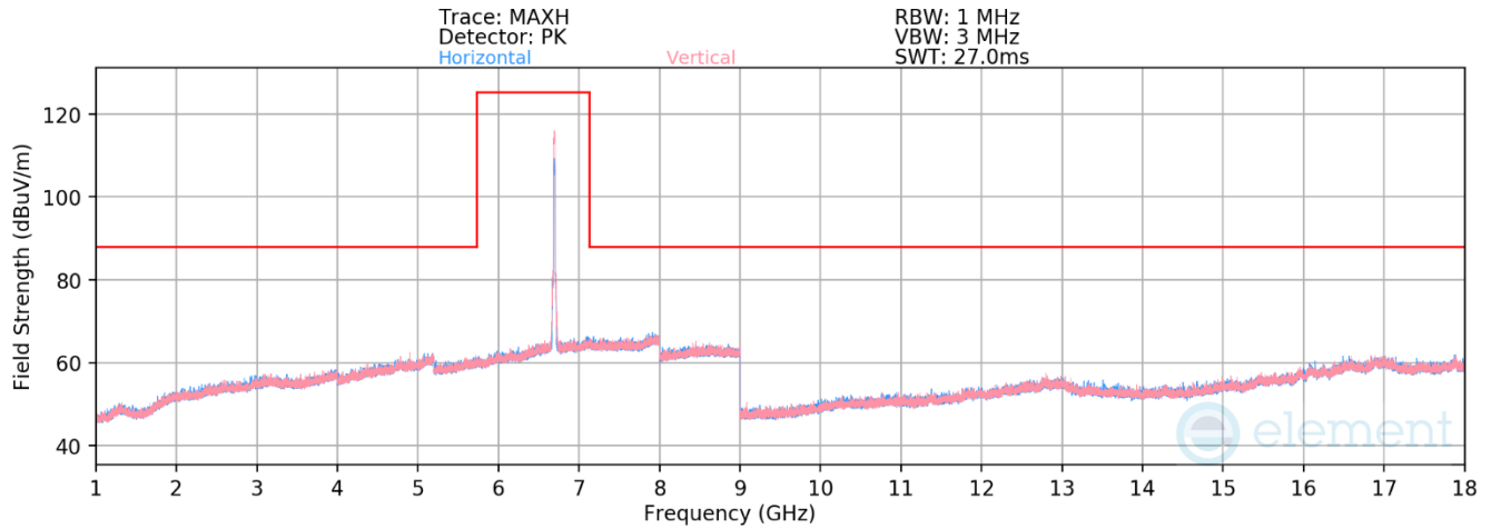
Plot 7-559. Radiated Spurious Emissions above 1GHz SDM Diversity (802.11ax – Ch. 149)
