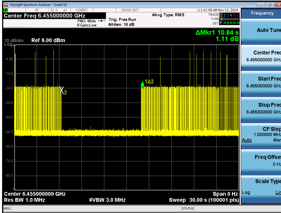
Plot 7-518. Contention Based Protocol Timing Plot – UNII 6 – 20MHz Channel 101
