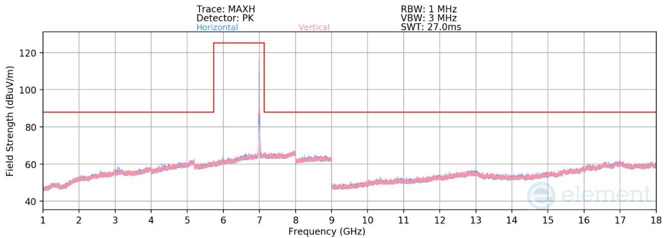
Plot 7-548. Radiated Spurious Emissions above 1GHz CDD Primary (802.11ax – Ch. 209)
