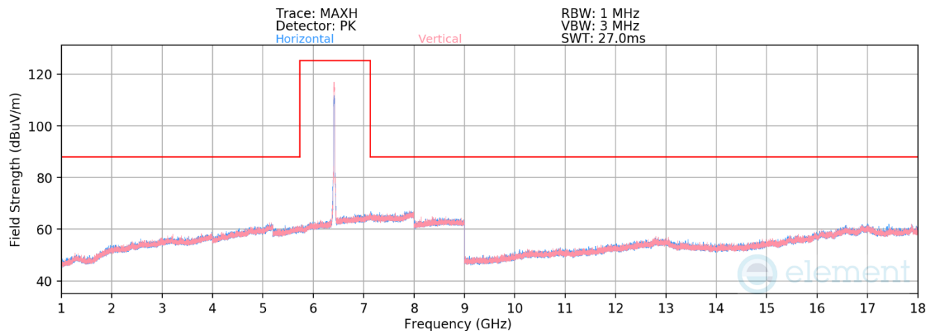
Plot 7-553. Radiated Spurious Emissions above 1GHz SDM Diversity (802.11ax – Ch. 93)
