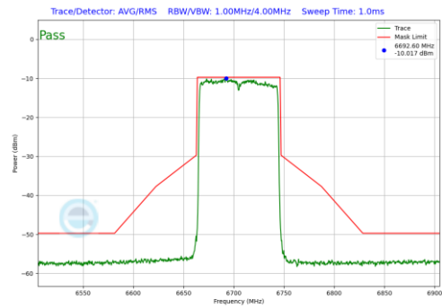
Plot 7-487. In-Band Emission Plot SDM Diversity Antenna 1b (80MHz 802.11ax (UNII Band 7) – Ch. 151)
