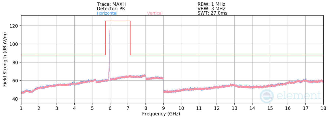
Plot 7-534. Radiated Spurious Emissions above 1GHz SDM (802.11ax – Ch. 1)
