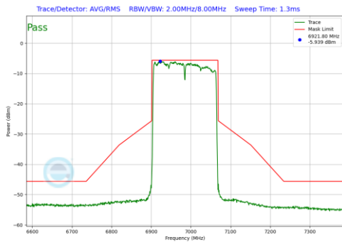
Plot 7-496. In-Band Emission Plot SDM Diversity Antenna 5T (160MHz 802.11ax (UNII Band 8) – Ch. 207)
