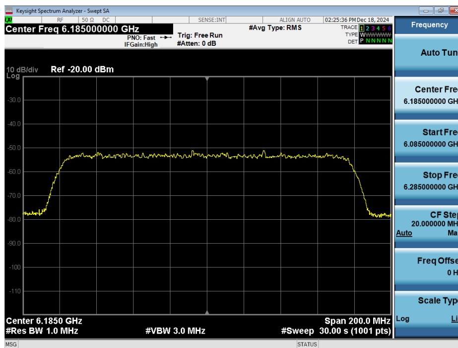
Plot 7-530. 160MHz Bandwidth, Before AWGN Signal Injected – Channel 47
