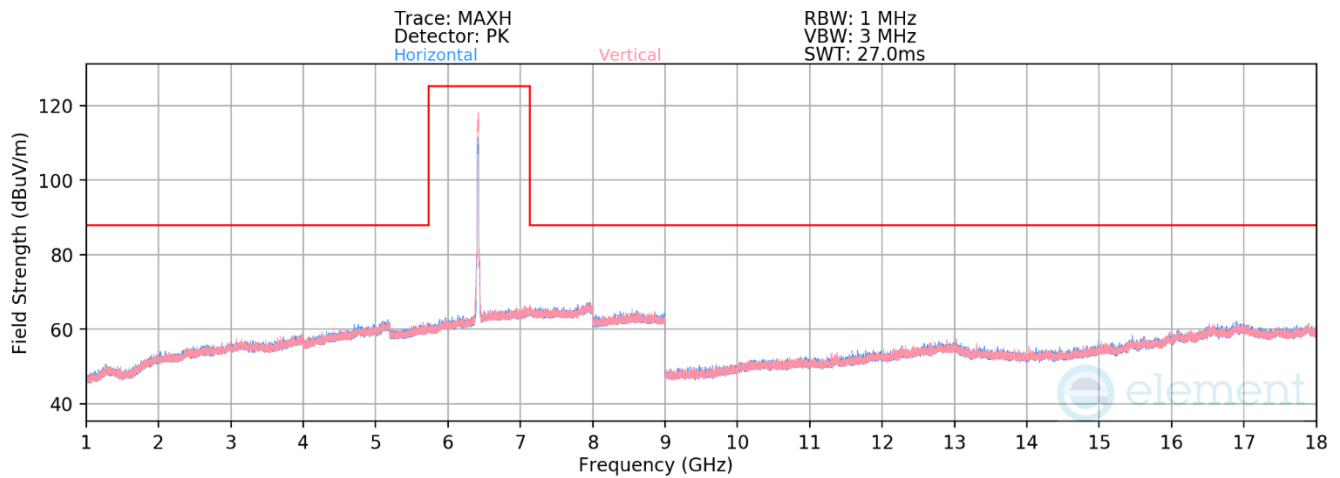
Plot 7-537. Radiated Spurious Emissions above 1GHz CDD Primary (802.11ax – Ch. 93)
