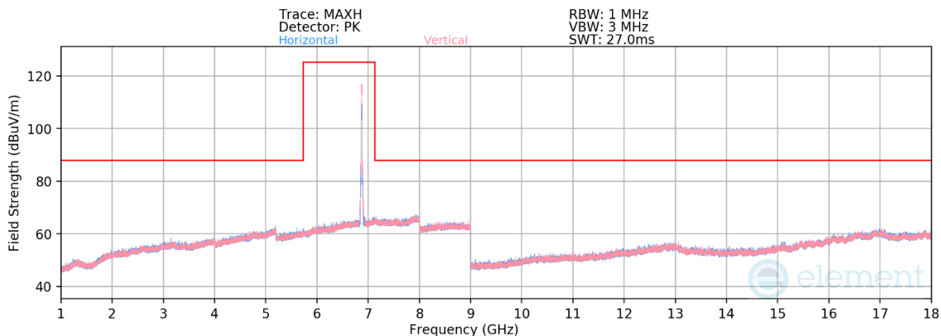
Plot 7-544. Radiated Spurious Emissions above 1GHz CDD Primary (802.11ax – Ch. 185)
