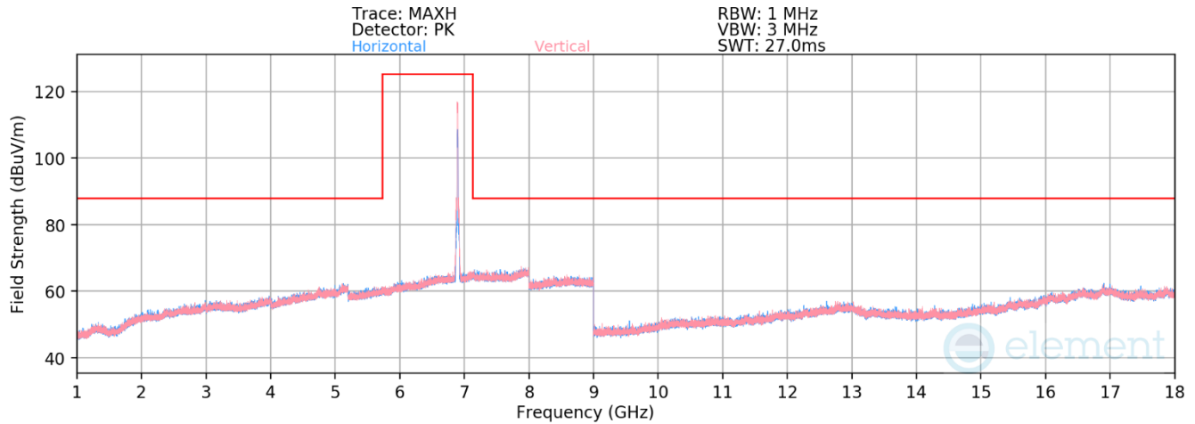
Plot 7-546. Radiated Spurious Emissions above 1GHz CDD Primary (802.11ax – Ch. 189)
