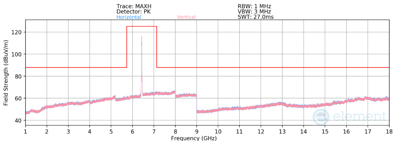
Plot 7-555. Radiated Spurious Emissions above 1GHz SDM Diversity (802.11ax – Ch. 105)
