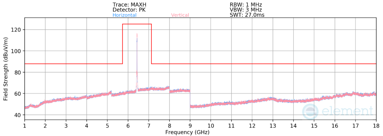
Plot 7-554. Radiated Spurious Emissions above 1GHz SDM Diversity (802.11ax – Ch. 97)
