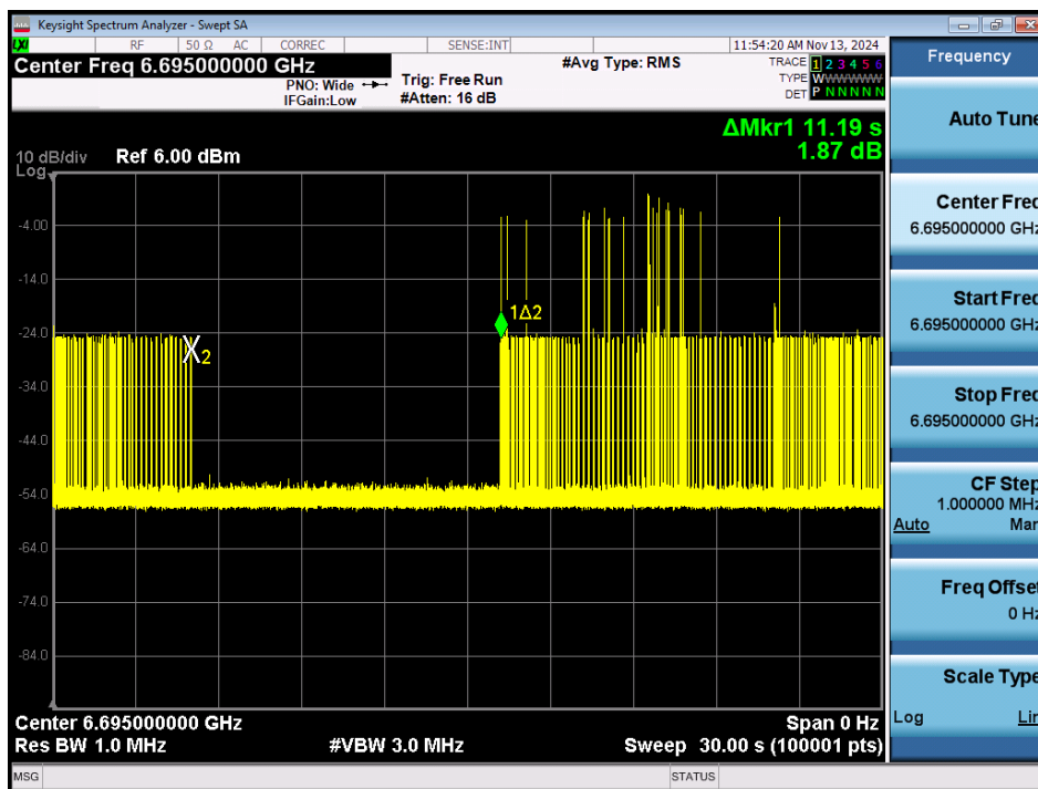
Plot 7-522. Contention Based Protocol Timing Plot – UNII 7 – 20MHz Channel 149
