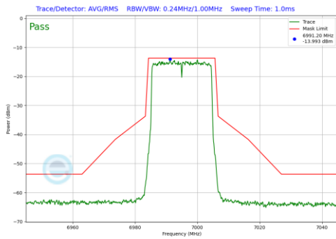
Plot 7-490. In-Band Emission Plot SDM Diversity Antenna 5T (20MHz 802.11ax (UNII Band 8) – Ch. 209)
