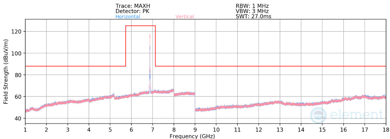
Plot 7-560. Radiated Spurious Emissions above 1GHz SDM Diversity (802.11ax – Ch. 185)
