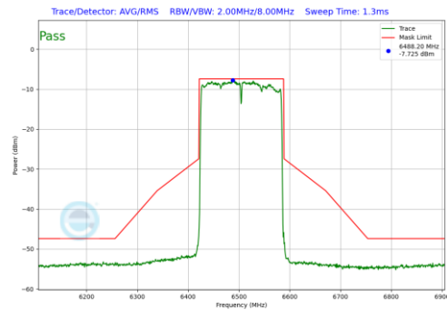
Plot 7-481. In-Band Emission Plot SDM Diversity Antenna 1b (160MHz 802.11ax (UNII Band 6) – Ch. 111)
