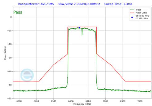
Plot 7-489. In-Band Emission Plot SDM Diversity Antenna 1b (160MHz 802.11ax (UNII Band 7) – Ch. 143)
