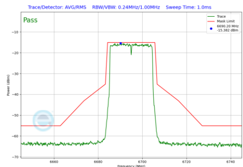
Plot 7-483. In-Band Emission Plot SDM Diversity Antenna 1b (20MHz 802.11ax (UNII Band 7) – Ch. 149)
