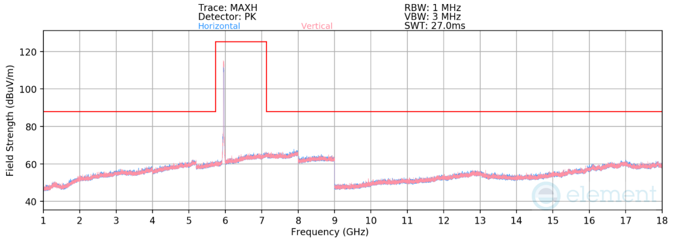
Plot 7-550. Radiated Spurious Emissions above 1GHz SDM Diversity (802.11ax – Ch. 1)
