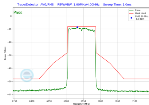
Plot 7-494. In-Band Emission Plot SDM Diversity Antenna 5T (80MHz 802.11ax (UNII Band 8) – Ch. 199)
