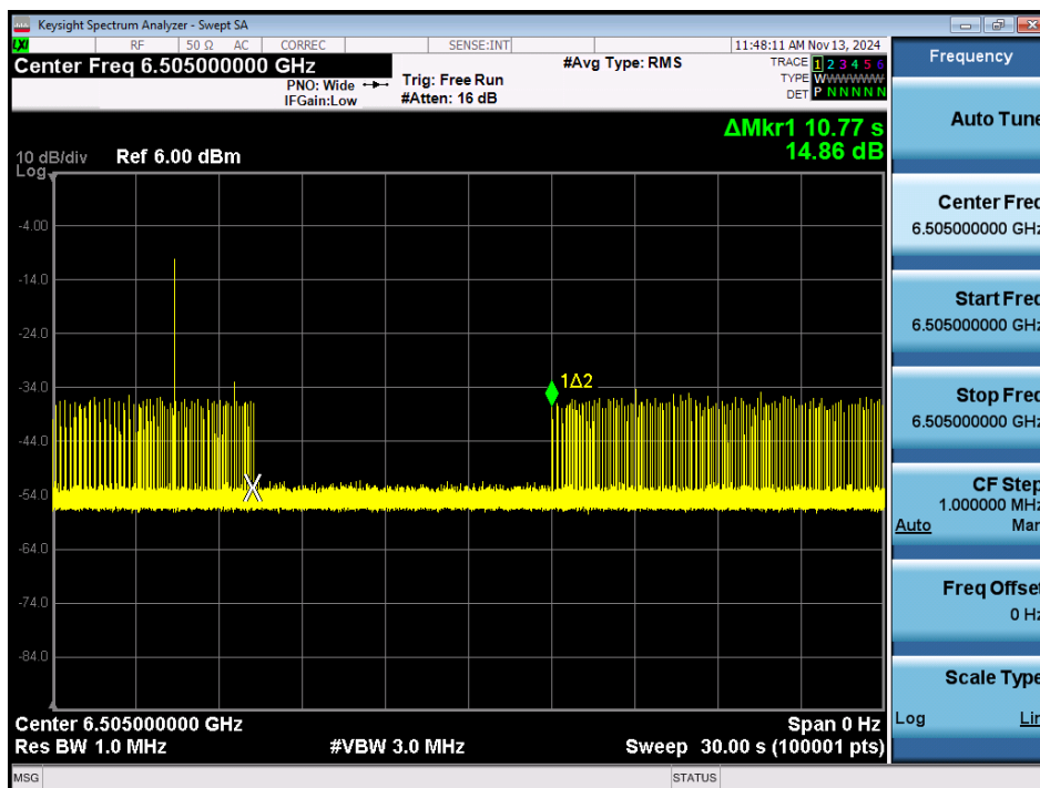
Plot 7-520. Contention Based Protocol Timing Plot – UNII 6 – 160MHz Channel 111 – Mid
