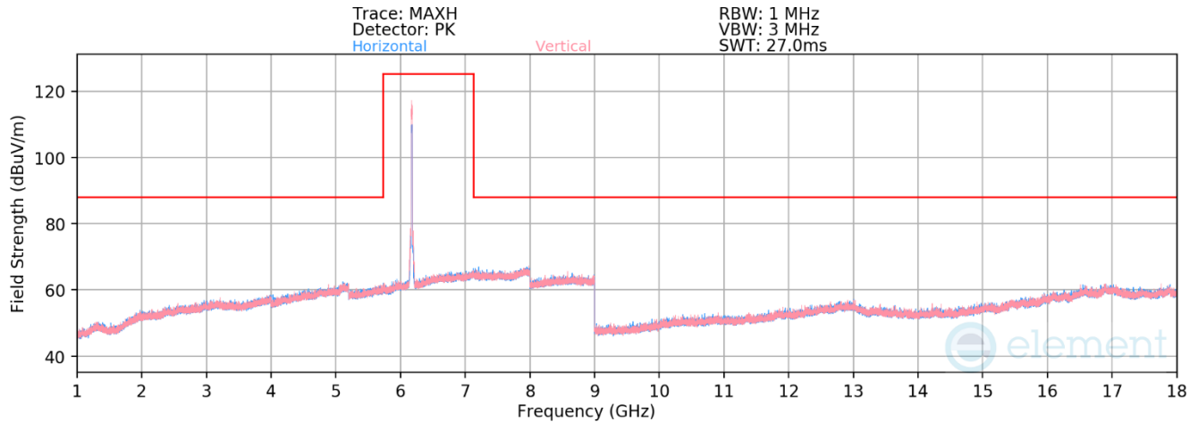
Plot 7-536. Radiated Spurious Emissions above 1GHz CDD Primary (802.11ax – Ch. 45)
