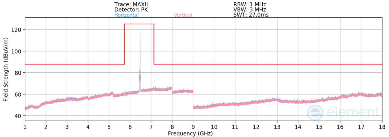
Plot 7-539. Radiated Spurious Emissions above 1GHz CDD Primary (802.11ax – Ch. 105)
