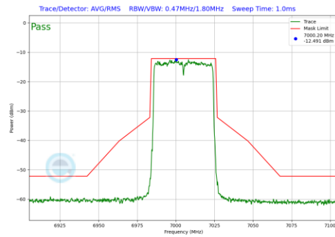
Plot 7-493. In-Band Emission Plot SDM Diversity Antenna 1b (40MHz 802.11ax (UNII Band 8) – Ch. 211)
