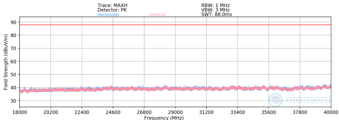
Plot 7-562. Radiated Spurious Emissions 18-40GHz CDD Diversity (802.11ax – Ch. 189)
