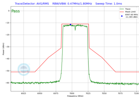
Plot 7-492. In-Band Emission Plot SDM Diversity Antenna 5T (40MHz 802.11ax (UNII Band 8) – Ch. 211)
