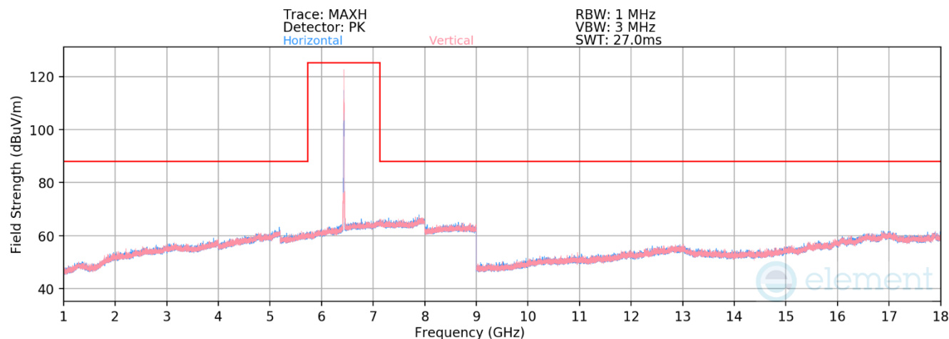
Plot 7-542. Radiated Spurious Emissions above 1GHz CDD Primary (802.11ax – Ch. 117)
