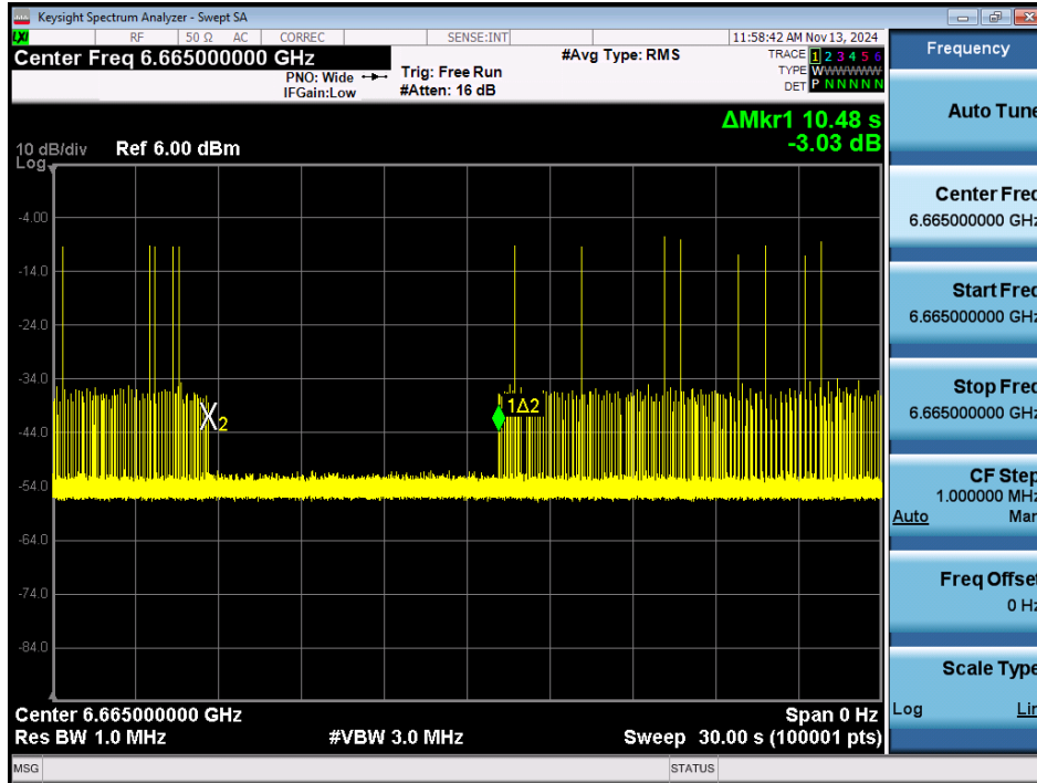
Plot 7-524. Contention Based Protocol Timing Plot – UNII 7 – 160MHz Channel 143 – Mid
