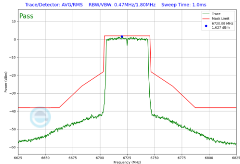
Plot 7-460. In-Band Emission Plot CDD Diversity Antenna 5T (40MHz 802.11ax (UNII Band 7) – Ch. 155)
