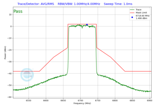
Plot 7-462. In-Band Emission Plot CDD Diversity Antenna 5T (80MHz 802.11ax (UNII Band 7) – Ch. 151)
