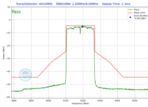
Plot 7-416. In-Band Emission Plot SDM Primary Antenna 5T (160MHz 802.11ax (UNII Band 5) – Ch. 47)
