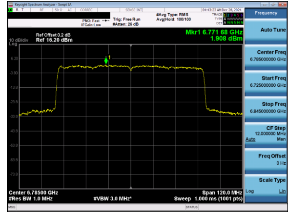
Plot 7-190. Power Spectral Density Plot CDD Primary Antenna 3b (80MHz 802.11ax (UNII Band 7) – Ch. 167)
