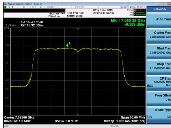
Plot 7-110. Power Spectral Density Plot Antenna 5T (40MHz 802.11ax (UNII Band 8) – Ch. 227)
