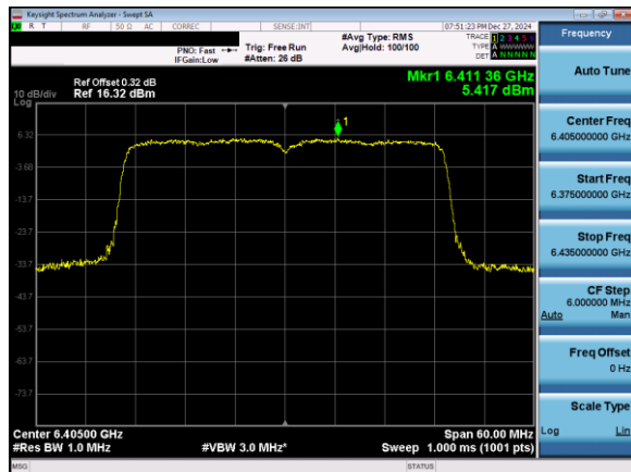
Plot 7-86. Power Spectral Density Plot Antenna 5T (40MHz 802.11ax (UNII Band 5) – Ch. 91)
