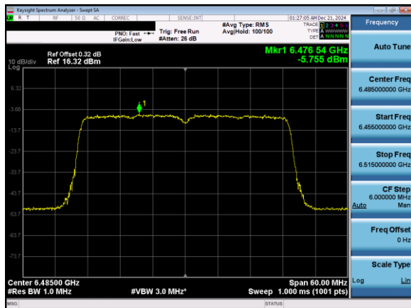
Plot 7-102. Power Spectral Density Plot Antenna 5T (40MHz 802.11ax (UNII Band 6) – Ch. 107)
