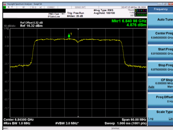
Plot 7-122. Power Spectral Density Plot Antenna 3b (40MHz 802.11ax (UNII Band 7) – Ch. 179)
