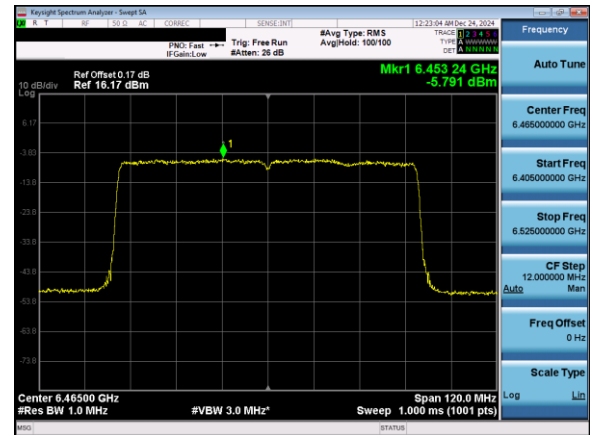
Plot 7-131. Power Spectral Density Plot Antenna 3b (80MHz 802.11ax (UNII Band 6) – Ch. 103)
