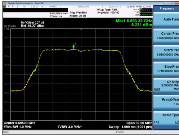
Plot 7-105. Power Spectral Density Plot Antenna 5T (20MHz 802.11a (UNII Band 7) – Ch. 149)
