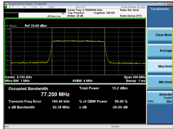
Plot 7-79. 26dB & 99% Bandwidth Plot Antenna 1b (80MHz 802.11ax (UNII Band 7) – Ch. 151)
