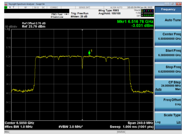
Plot 7-92. Power Spectral Density Plot Antenna 5T (160MHz 802.11ax (UNII Band 6) – Ch. 111)
