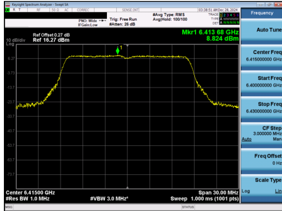
Plot 7-113. Power Spectral Density Plot Antenna 3b (20MHz 802.11a (UNII Band 5) – Ch. 93)
