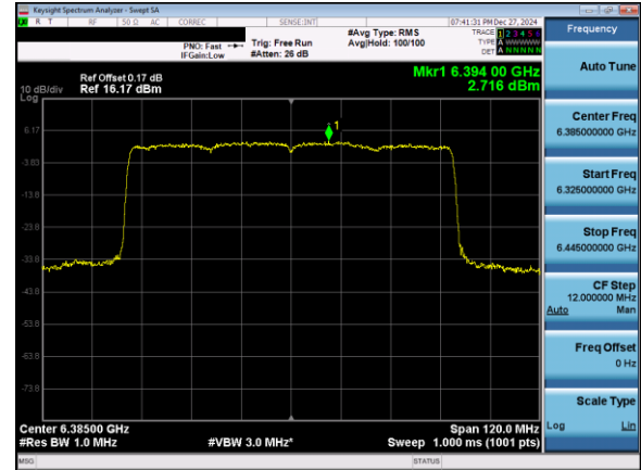
Plot 7-87. Power Spectral Density Plot Antenna 5T (80MHz 802.11ax (UNII Band 5) – Ch. 87)
