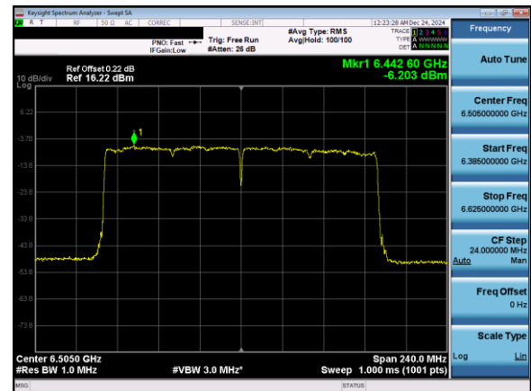
Plot 7-132. Power Spectral Density Plot Antenna 3b (160MHz 802.11ax (UNII Band 6) – Ch. 111)
