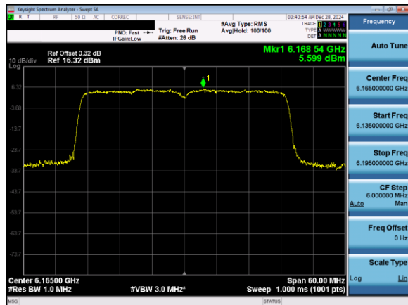
Plot 7-114. Power Spectral Density Plot Antenna 3b (40MHz 802.11ax (UNII Band 5) – Ch. 43)
