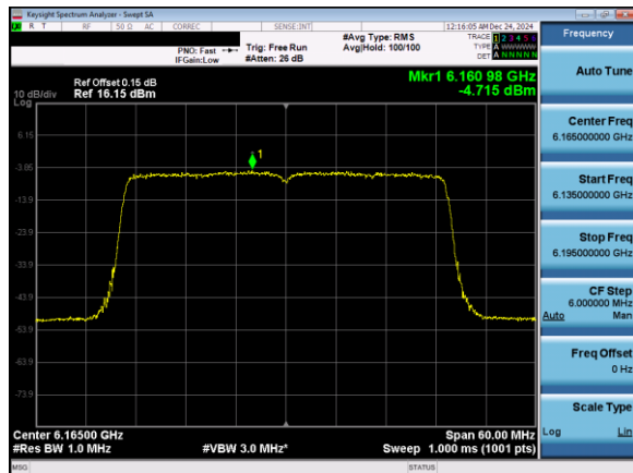
Plot 7-126. Power Spectral Density Plot Antenna 3b (40MHz 802.11ax (UNII Band 5) – Ch. 43)
