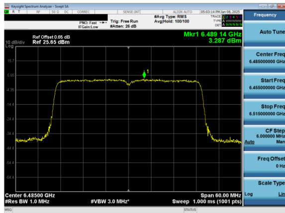
Plot 7-90. Power Spectral Density Plot Antenna 5T (40MHz 802.11ax (UNII Band 6) – Ch. 107)
