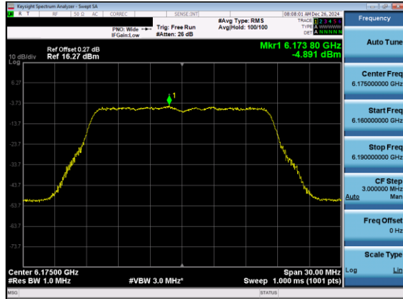
Plot 7-125. Power Spectral Density Plot Antenna 3b (20MHz 802.11a (UNII Band 5) – Ch. 45)
