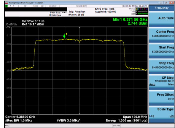
Plot 7-115. Power Spectral Density Plot Antenna 3b (80MHz 802.11ax (UNII Band 5) – Ch. 87)
