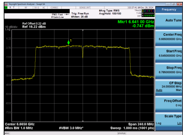
Plot 7-124. Power Spectral Density Plot Antenna 3b (160MHz 802.11ax (UNII Band 7) – Ch. 143)
