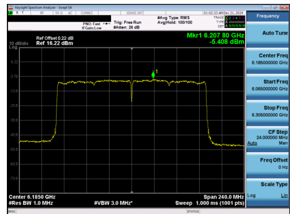
Plot 7-100. Power Spectral Density Plot Antenna 5T (160MHz) 802.11ax (UNII Band 5) – Ch. 47)
