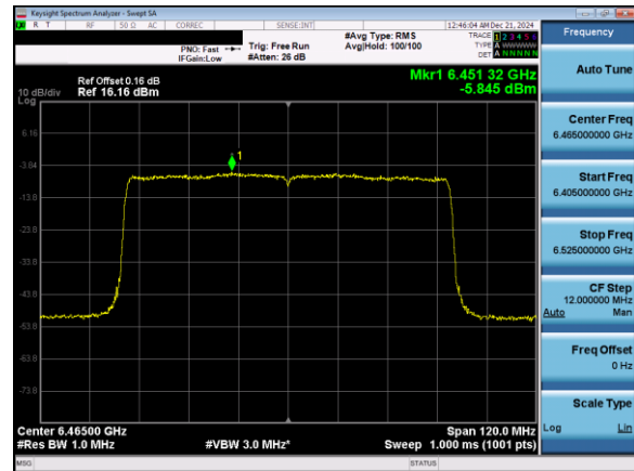
Plot 7-103. Power Spectral Density Plot Antenna 5T (80MHz 802.11ax (UNII Band 6) – Ch. 103)
