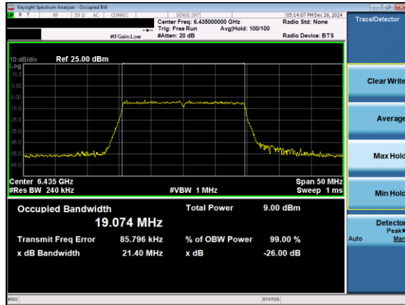
Plot 7-73. 26dB & 99% Bandwidth Plot Antenna 1b (20MHz 802.11ax (UNII Band 6) – Ch. 97)
