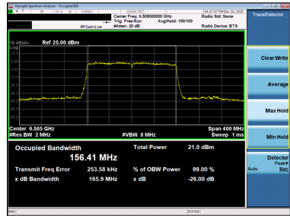
Plot 7-76. 26dB & 99% Bandwidth Plot Antenna 1b (160MHz 802.11ax (UNII Band 6) – Ch. 111)
