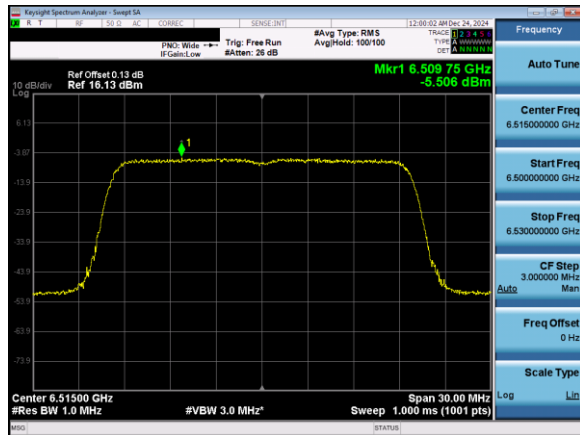
Plot 7-129. Power Spectral Density Plot Antenna 3b (20MHz 802.11ax (UNII Band 6) – Ch. 113)
