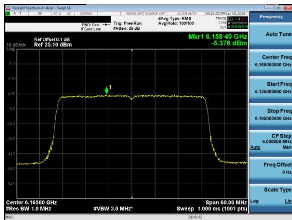
Plot 7-98. Power Spectral Density Plot Antenna 5T (40MHz) 802.11ax (UNII Band 5) – Ch. 43)
