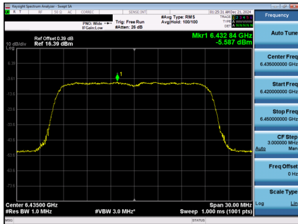
Plot 7-101. Power Spectral Density Plot Antenna 5T (20MHz 802.11ax (UNII Band 6) – Ch. 97)
