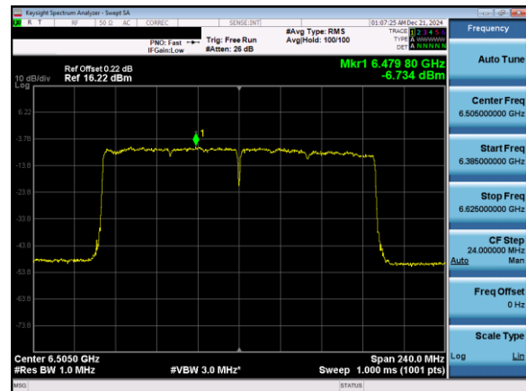
Plot 7-104. Power Spectral Density Plot Antenna 5T (160MHz 802.11ax (UNII Band 6) – Ch. 111)
