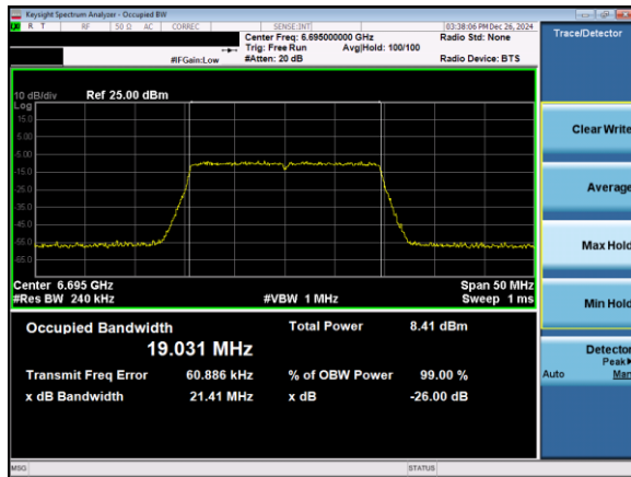
Plot 7-77. 26dB & 99% Bandwidth Plot Antenna 1b (20MHz 802.11ax (UNII Band 7) – Ch. 149)
