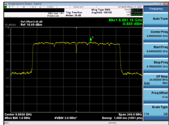
Plot 7-96. Power Spectral Density Plot Antenna 5T (160MHz 802.11ax (UNII Band 7) – Ch. 143)
