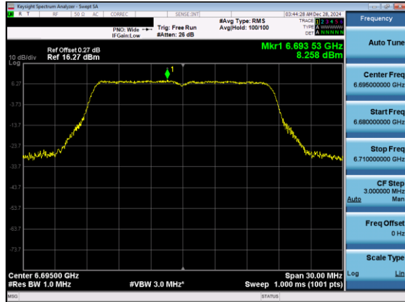
Plot 7-121. Power Spectral Density Plot Antenna 3b (20MHz 802.11a (UNII Band 7) – Ch. 149)
