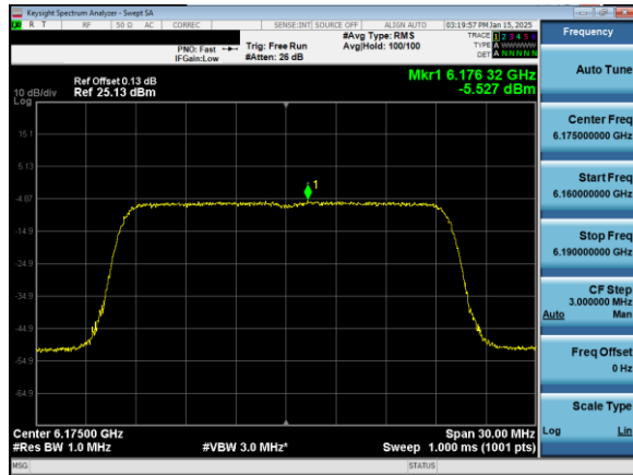
Plot 7-97. Power Spectral Density Plot Antenna 5T (20MHz) 802.11ax (UNII Band 5) – Ch. 45)
