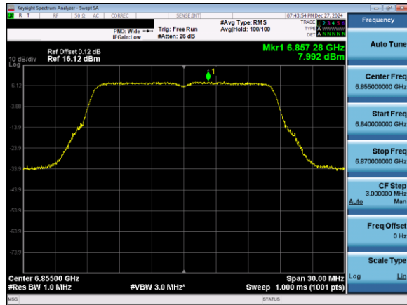
Plot 7-93. Power Spectral Density Plot Antenna 5T (20MHz 802.11a (UNII Band 7) – Ch. 181)
