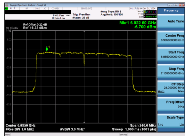
Plot 7-112. Power Spectral Density Plot Antenna 5T (160MHz 802.11ax (UNII Band 8) – Ch. 207)
