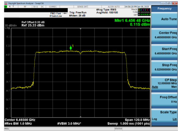
Plot 7-91. Power Spectral Density Plot Antenna 5T (80MHz 802.11ax (UNII Band 6) – Ch. 103)
