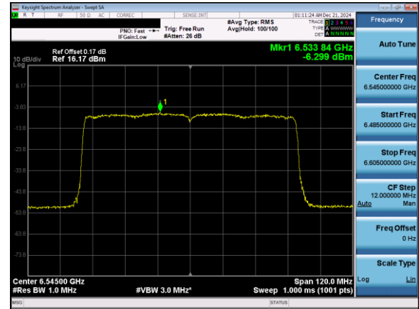
Plot 7-107. Power Spectral Density Plot Antenna 5T (80MHz 802.11ax (UNII Band 7) – Ch. 119)
