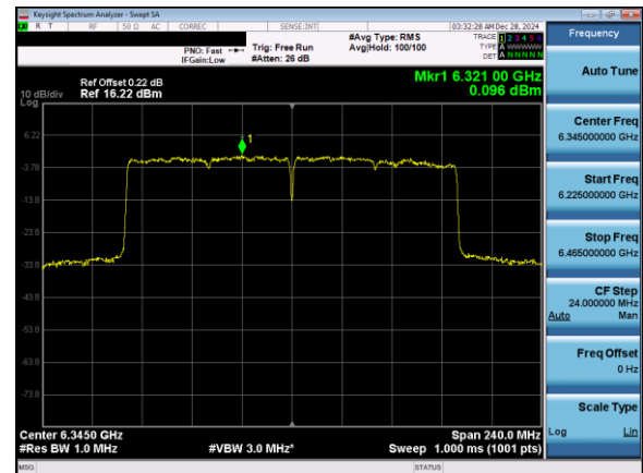
Plot 7-116. Power Spectral Density Plot Antenna 3b (160MHz 802.11ax (UNII Band 5) – Ch. 79)
