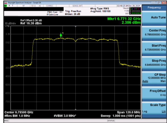
Plot 7-123. Power Spectral Density Plot Antenna 3b (80MHz 802.11ax (UNII Band 7) – Ch. 167)
