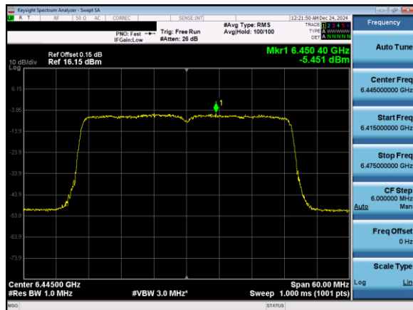
Plot 7-130. Power Spectral Density Plot Antenna 3b (40MHz 802.11ax (UNII Band 6) –Ch. 99)
