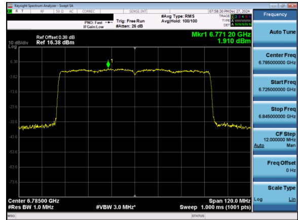
Plot 7-95. Power Spectral Density Plot Antenna 5T (80MHz 802.11ax (UNII Band 7) – Ch. 167)
