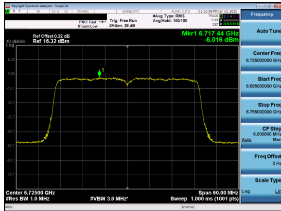
Plot 7-106. Power Spectral Density Plot Antenna 5T (40MHz 802.11ax (UNII Band 7) – Ch. 155)
