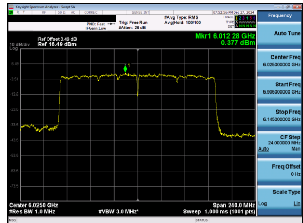
Plot 7-88. Power Spectral Density Plot Antenna 5T (160MHz 802.11ax (UNII Band 5) – Ch. 15)
