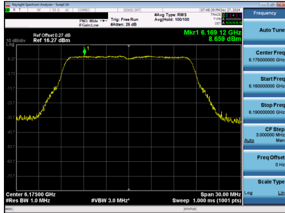
Plot 7-85. Power Spectral Density Plot Antenna 5T (20MHz 802.11a (UNII Band 5) – Ch. 45)
