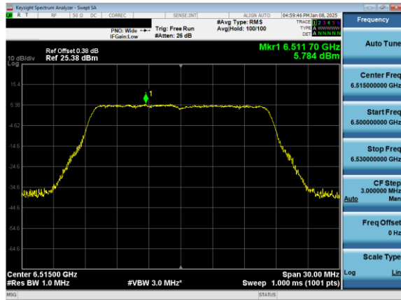
Plot 7-89. Power Spectral Density Plot Antenna 5T (20MHz 802.11a (UNII Band 6) – Ch. 113)
