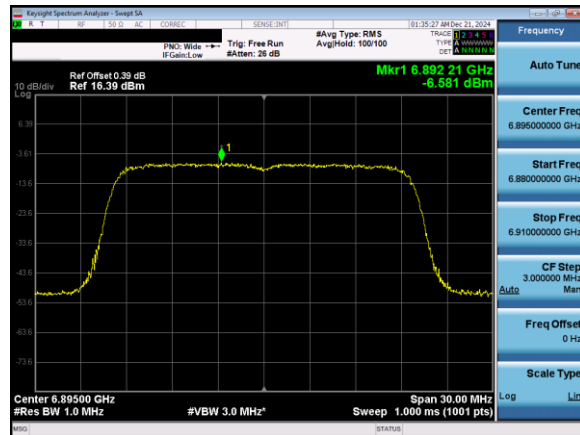
Plot 7-109. Power Spectral Density Plot Antenna 5T (20MHz 802.11ax (UNII Band 8) – Ch. 189)
