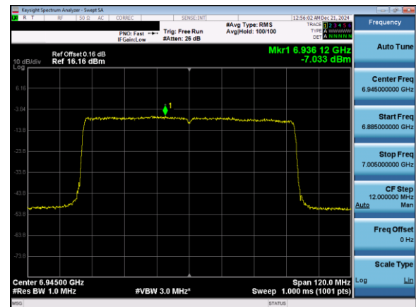
Plot 7-111. Power Spectral Density Plot Antenna 5T (80MHz 802.11ax (UNII Band 8) – Ch. 199)
