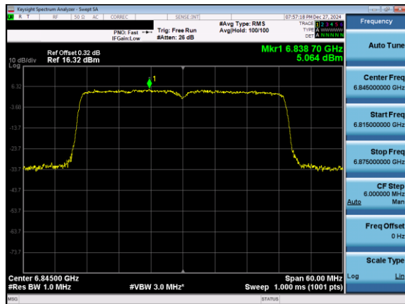
Plot 7-94. Power Spectral Density Plot Antenna 5T (40MHz 802.11ax (UNII Band 7) – Ch. 179)
