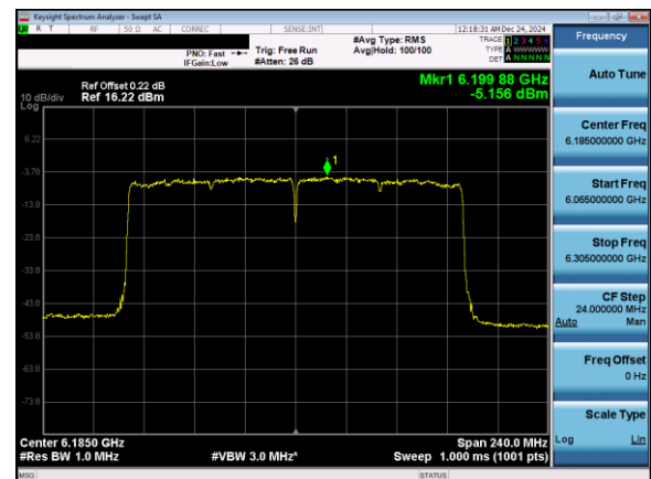
Plot 7-128. Power Spectral Density Plot Antenna 3b (160MHz 802.11ax (UNII Band 5) – Ch. 47)
