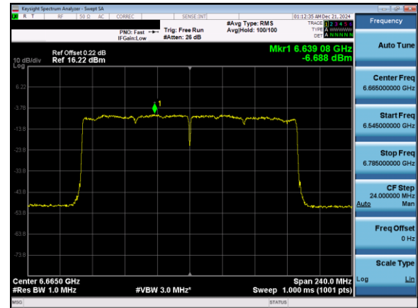
Plot 7-108. Power Spectral Density Plot Antenna 5T (160MHz 802.11ax (UNII Band 7) – Ch. 143)
