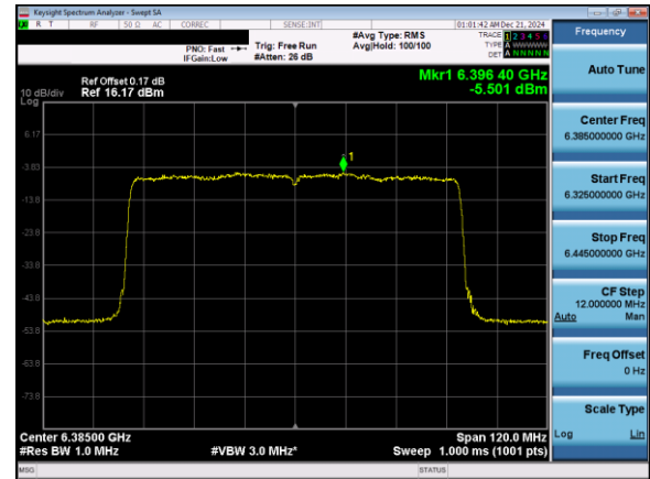
Plot 7-99. Power Spectral Density Plot Antenna 5T (80MHz) 802.11ax (UNII Band 5) – Ch. 87)
