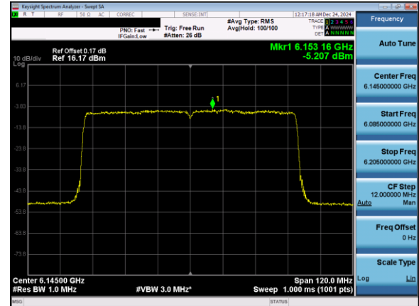
Plot 7-127. Power Spectral Density Plot Antenna 3b (80MHz 802.11ax (UNII Band 5) – Ch. 39)
