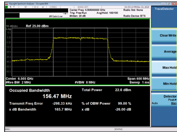
Plot 7-20. 26dB & 99% Bandwidth Plot Antenna 5T (160MHz 802.11ax (UNII Band 6) – Ch. 111)
