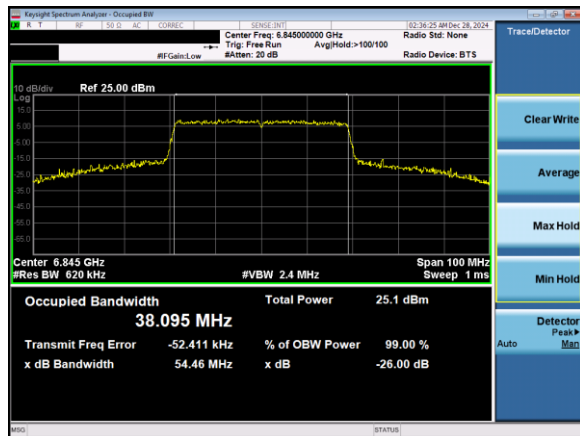
Plot 7-38. 26dB & 99% Bandwidth Plot Antenna 3b (40MHz 802.11ax (UNII Band 7) – Ch. 179)
