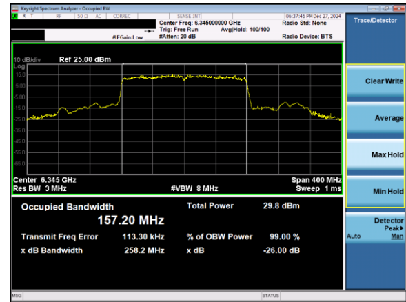
Plot 7-4. 26dB & 99% Bandwidth Plot Antenna 5T (160MHz 802.11ax (UNII Band 5) – Ch. 79)
