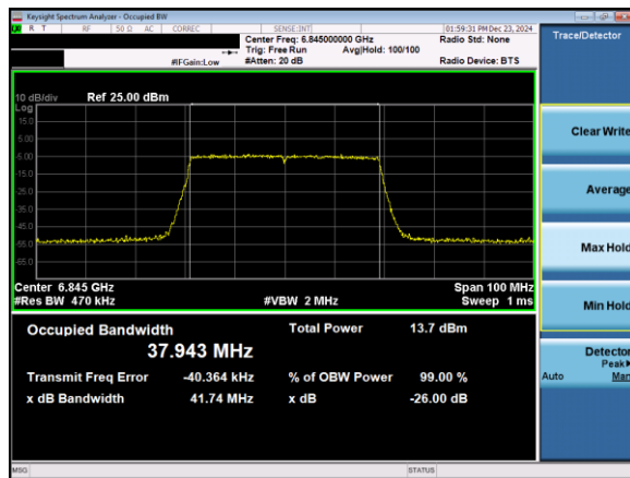
Plot 7-22. 26dB & 99% Bandwidth Plot Antenna 5T (40MHz 802.11ax (UNII Band 7) – Ch. 179)
