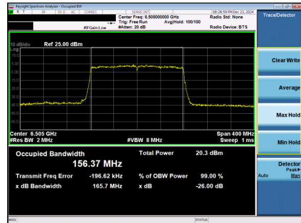
Plot 7-48. 26dB & 99% Bandwidth Plot Antenna 3b (160MHz 802.11ax (UNII Band 6) – Ch. 111)
