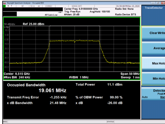
Plot 7-17. 26dB & 99% Bandwidth Plot Antenna 5T (20MHz 802.11ax (UNII Band 6) – Ch. 113)
