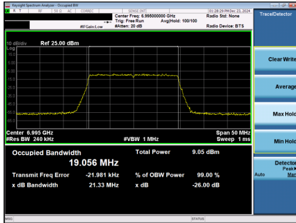
Plot 7-25. 26dB & 99% Bandwidth Plot Antenna 5T (20MHz 802.11ax (UNII Band 8) – Ch. 209)
