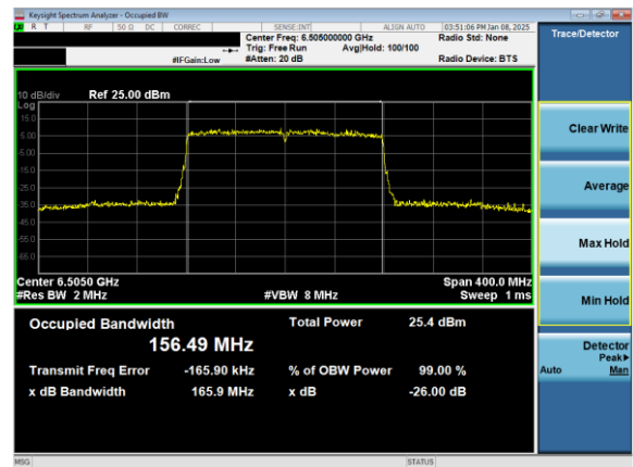
Plot 7-8. 26dB & 99% Bandwidth Plot Antenna 5T (160MHz) 802.11ax (UNII Band 6) – Ch. 111)
