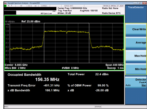
Plot 7-28. 26dB & 99% Bandwidth Plot Antenna 5T (160MHz 802.11ax (UNII Band 8) – Ch. 207)
