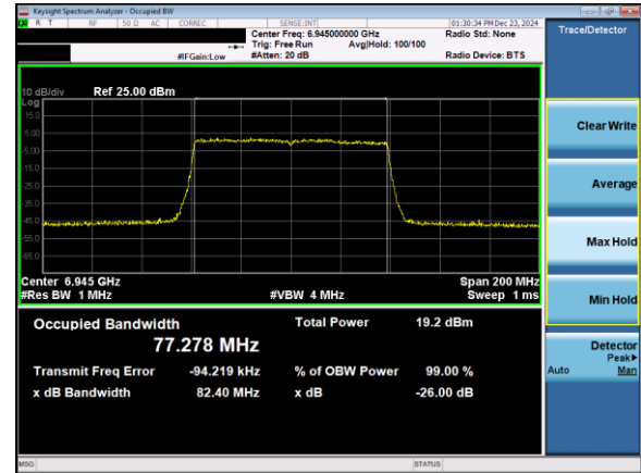
Plot 7-27. 26dB & 99% Bandwidth Plot Antenna 5T (80MHz 802.11ax (UNII Band 8) – Ch. 199)
