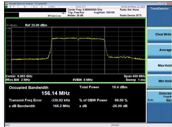
Plot 7-56. 26dB & 99% Bandwidth Plot Antenna 3b (160MHz 802.11ax (UNII Band 8) – Ch. 207)
