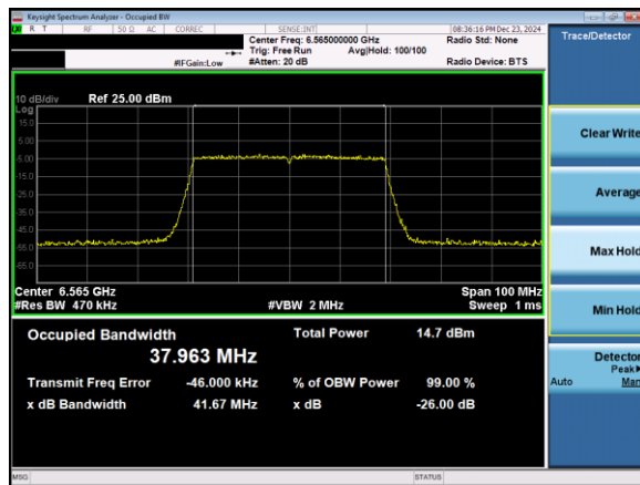
Plot 7-50. 26dB & 99% Bandwidth Plot Antenna 3b (40MHz 802.11ax (UNII Band 7) – Ch. 123)
