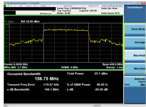
Plot 7-36. 26dB & 99% Bandwidth Plot Antenna 3b (160MHz 802.11ax (UNII Band 6) – Ch. 111)
