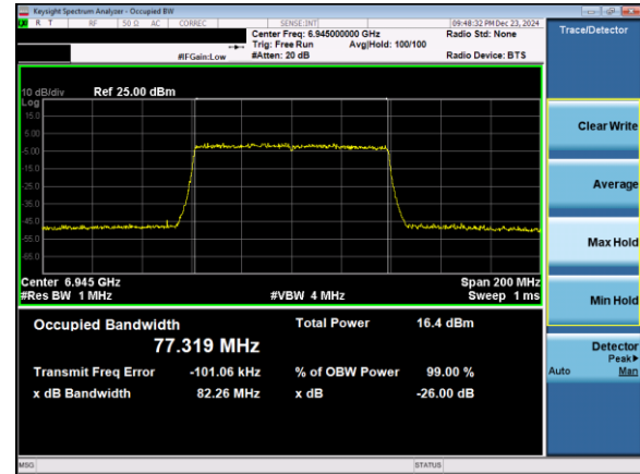
Plot 7-55. 26dB & 99% Bandwidth Plot Antenna 3b (80MHz 802.11ax (UNII Band 8) – Ch. 199)
