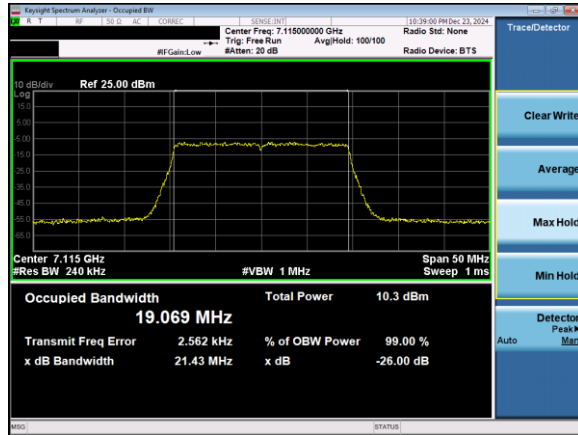
Plot 7-53. 26dB & 99% Bandwidth Plot Antenna 3b (20MHz 802.11ax (UNII Band 8) – Ch. 233)
