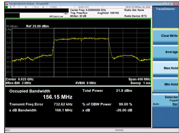
Plot 7-72. 26dB & 99% Bandwidth Plot Antenna 1b (160MHz 802.11ax (UNII Band 5) – Ch. 15)
