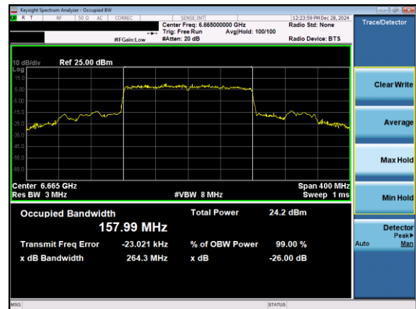
Plot 7-68. 26dB & 99% Bandwidth Plot Antenna 1b (160MHz 802.11ax (UNII Band 7) – Ch. 143)
