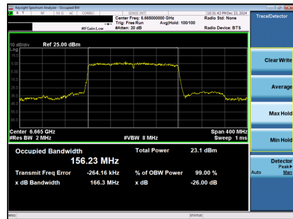
Plot 7-52. 26dB & 99% Bandwidth Plot Antenna 3b (160MHz 802.11ax (UNII Band 7) – Ch. 143)
