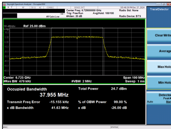
Plot 7-10. 26dB & 99% Bandwidth Plot Antenna 5T (40MHz 802.11ax (UNII Band 7) – Ch. 155)
