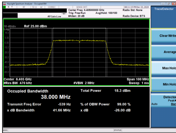
Plot 7-42. 26dB & 99% Bandwidth Plot Antenna 3b (40MHz 802.11ax (UNII Band 5) – Ch. 91)
