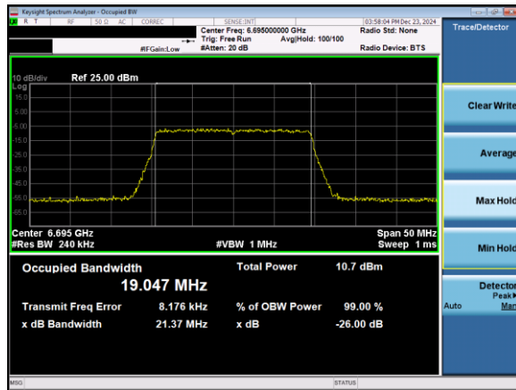
Plot 7-21. 26dB & 99% Bandwidth Plot Antenna 5T (20MHz 802.11ax (UNII Band 7) – Ch. 149)
