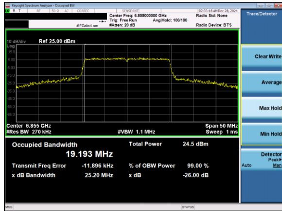
Plot 7-37. 26dB & 99% Bandwidth Plot Antenna 3b (20MHz 802.11ax (UNII Band 7) – Ch. 181)
