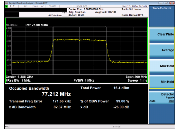
Plot 7-71. 26dB & 99% Bandwidth Plot Antenna 1b (80MHz 802.11ax (UNII Band 5) – Ch. 87)
