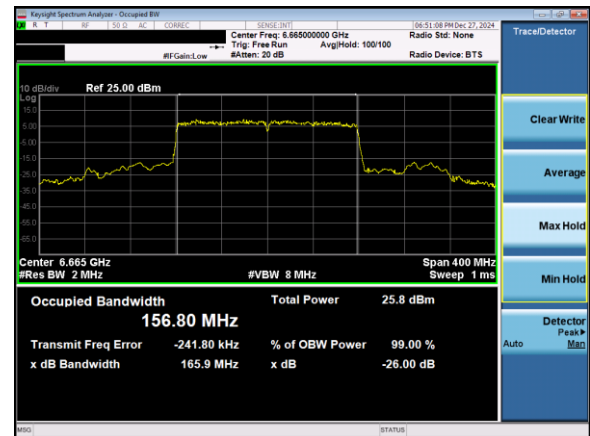
Plot 7-12. 26dB & 99% Bandwidth Plot Antenna 5T (160MHz 802.11ax (UNII Band 7) – Ch. 143)
