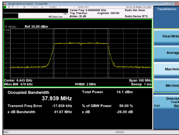
Plot 7-18. 26dB & 99% Bandwidth Plot Antenna 5T (40MHz 802.11ax (UNII Band 6) – Ch. 99)
