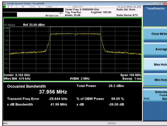
Plot 7-30. 26dB & 99% Bandwidth Plot Antenna 3b (40MHz 802.11ax (UNII Band 5) – Ch. 43)
