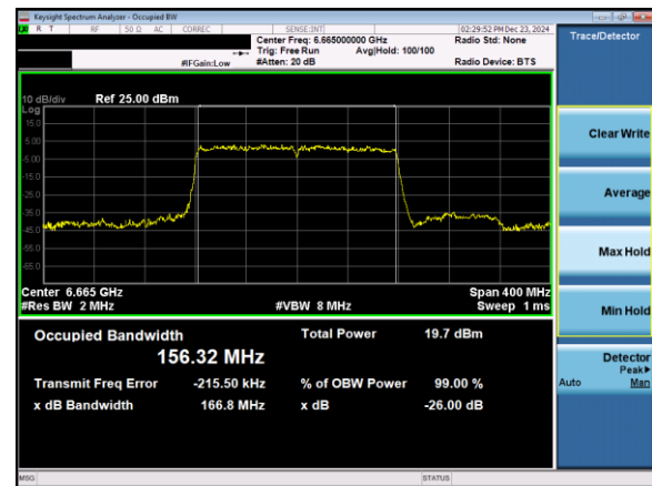
Plot 7-24. 26dB & 99% Bandwidth Plot Antenna 5T (160MHz 802.11ax (UNII Band 7) – Ch. 143)
