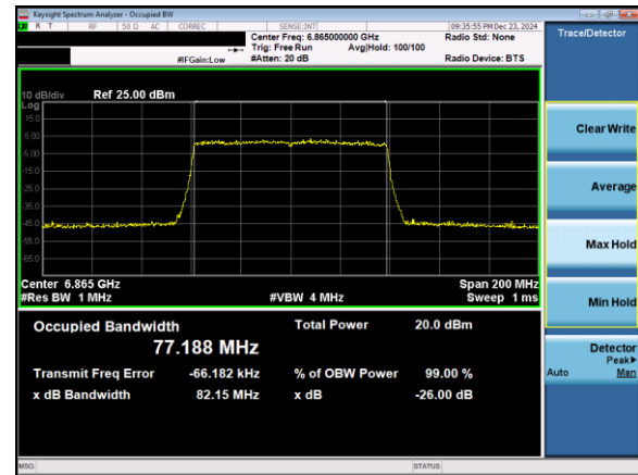
Plot 7-51. 26dB & 99% Bandwidth Plot Antenna 3b (80MHz 802.11ax (UNII Band 7) – Ch. 183)
