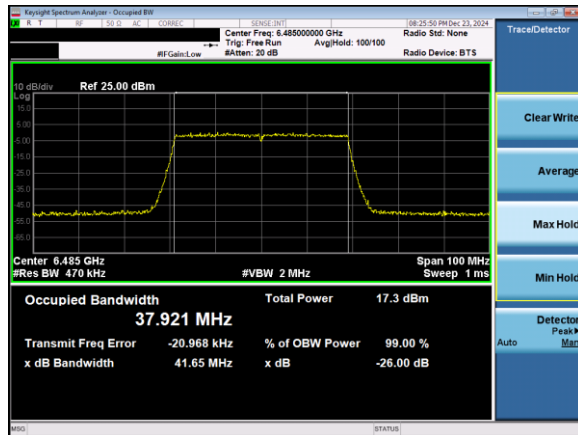
Plot 7-46. 26dB & 99% Bandwidth Plot Antenna 3b (40MHz 802.11ax (UNII Band 6) – Ch. 107)
