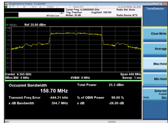
Plot 7-60. 26dB & 99% Bandwidth Plot Antenna 1b (160MHz 802.11ax (UNII Band 5) – Ch. 79)
