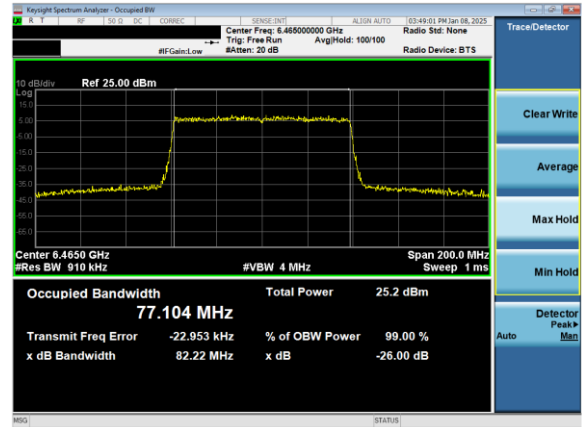
Plot 7-7. 26dB & 99% Bandwidth Plot Antenna 5T (80MHz) 802.11ax (UNII Band 6) – Ch. 103)
