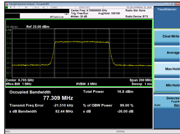
Plot 7-23. 26dB & 99% Bandwidth Plot Antenna 5T (80MHz 802.11ax (UNII Band 7) – Ch. 151)
