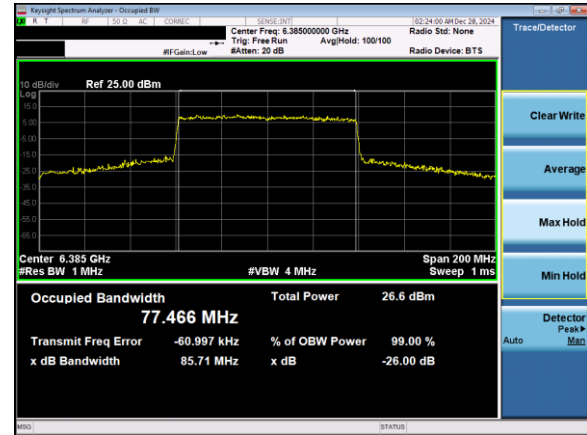
Plot 7-31. 26dB & 99% Bandwidth Plot Antenna 3b (80MHz 802.11ax (UNII Band 5) – Ch. 87)
