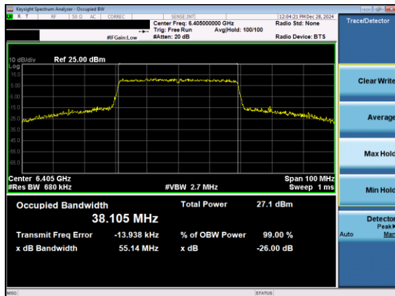
Plot 7-58. 26dB & 99% Bandwidth Plot Antenna 1b (40MHz 802.11ax (UNII Band 5) – Ch. 91)
