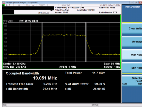
Plot 7-41. 26dB & 99% Bandwidth Plot Antenna 3b (20MHz 802.11ax (UNII Band 5) – Ch. 93)
