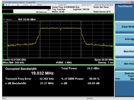
Plot 7-5. 26dB & 99% Bandwidth Plot Antenna 5T (20MHz) 802.11ax (UNII Band 6) – Ch. 113)
