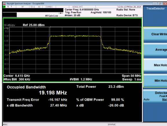
Plot 7-57. 26dB & 99% Bandwidth Plot 1b (20MHz 802.11ax (UNII Band 5) – Ch. 93)
