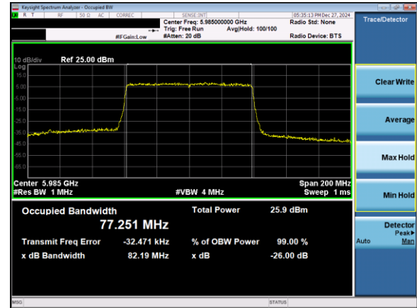
Plot 7-3. 26dB & 99% Bandwidth Plot Antenna 5T (80MHz 802.11ax (UNII Band 5) – Ch. 7)
