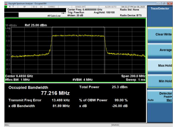
Plot 7-35. 26dB & 99% Bandwidth Plot Antenna 3b (80MHz 802.11ax (UNII Band 6) – Ch. 103)
