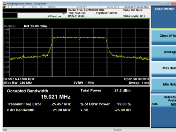
Plot 7-33. 26dB & 99% Bandwidth Plot Antenna 3b (20MHz 802.11ax (UNII Band 6) – Ch. 105)
