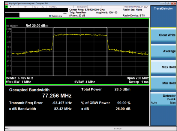
Plot 7-11. 26dB & 99% Bandwidth Plot Antenna 5T (80MHz 802.11ax (UNII Band 7) – Ch. 167)
