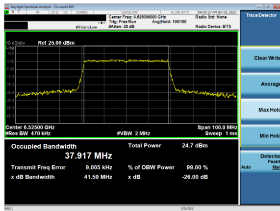
Plot 7-6. 26dB & 99% Bandwidth Plot Antenna 5T (40MHz) 802.11ax (UNII Band 6) – Ch. 115)
