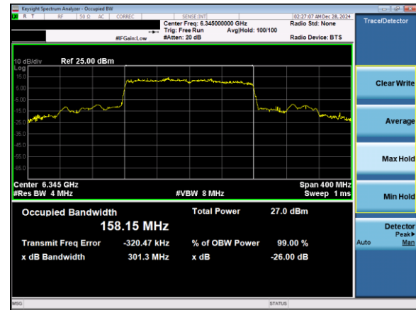
Plot 7-32. 26dB & 99% Bandwidth Plot Antenna 3b (160MHz 802.11ax (UNII Band 5) – Ch. 79)
