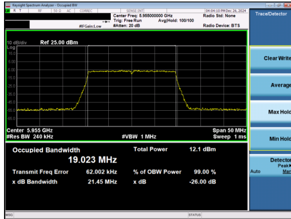
Plot 7-69. 26dB & 99% Bandwidth Plot Antenna 1b (20MHz 802.11ax (UNII Band 5) – Ch. 1)
