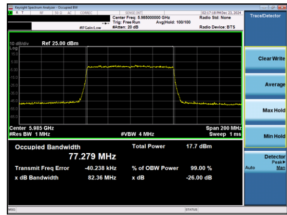
Plot 7-15. 26dB & 99% Bandwidth Plot Antenna 5T (80MHz 802.11ax (UNII Band 5) – Ch. 7)
