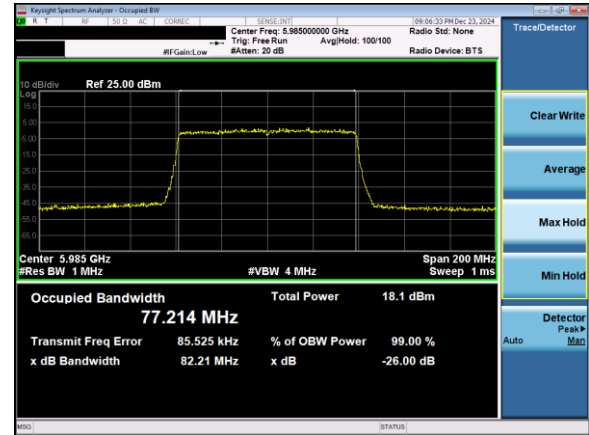
Plot 7-43. 26dB & 99% Bandwidth Plot Antenna 3b (80MHz 802.11ax (UNII Band 5) – Ch. 7)
