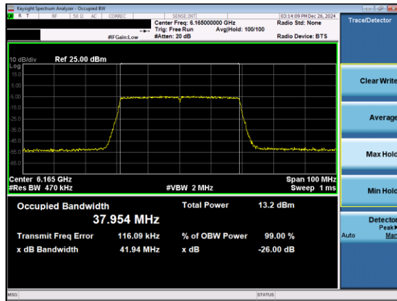
Plot 7-70. 26dB & 99% Bandwidth Plot Antenna 1b (40MHz 802.11ax (UNII Band 5) – Ch. 43)
