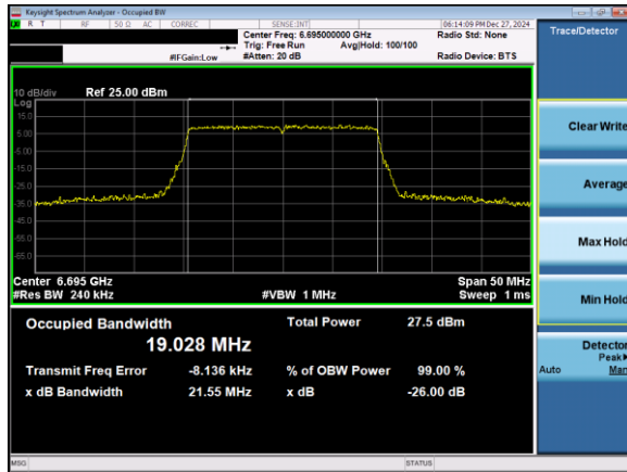
Plot 7-9. 26dB & 99% Bandwidth Plot Antenna 5T (20MHz 802.11ax (UNII Band 7) – Ch. 149)
