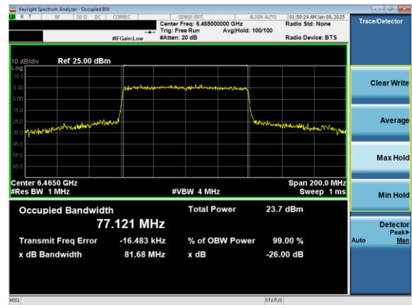
Plot 7-63. 26dB & 99% Bandwidth Plot Antenna 1b (80MHz 802.11ax (UNII Band 6) – Ch. 103)
