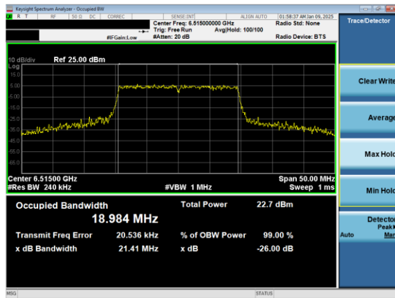
Plot 7-61. 26dB & 99% Bandwidth Plot Antenna 1b (20MHz 802.11ax (UNII Band 6) – Ch. 113)
