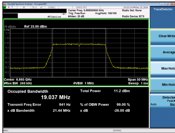
Plot 7-49. 26dB & 99% Bandwidth Plot Antenna 3b (20MHz 802.11ax (UNII Band 7) – Ch. 149)
