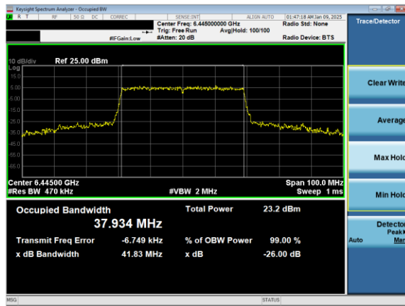
Plot 7-62. 26dB & 99% Bandwidth Plot Antenna 1b (40MHz 802.11ax (UNII Band 6) – Ch. 99)
