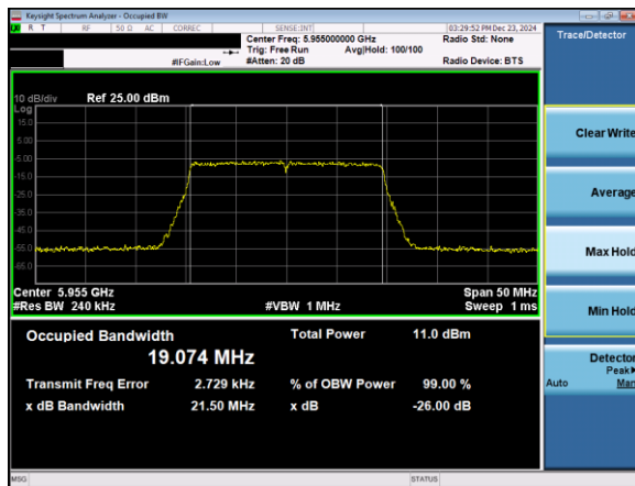
Plot 7-13. 26dB & 99% Bandwidth Plot Antenna 5T (20MHz 802.11ax (UNII Band 5) – Ch. 1)
