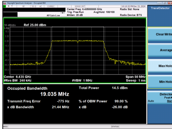
Plot 7-45. 26dB & 99% Bandwidth Plot Antenna 3b (20MHz 802.11ax (UNII Band 6) – Ch. 97)
