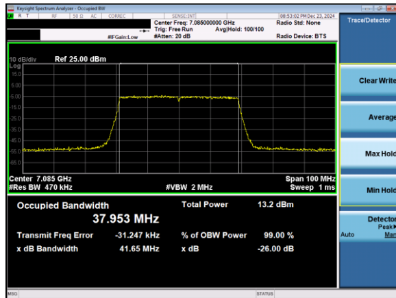
Plot 7-54. 26dB & 99% Bandwidth Plot Antenna 3b (40MHz 802.11ax (UNII Band 8) – Ch. 227)
