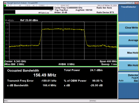
Plot 7-44. 26dB & 99% Bandwidth Plot Antenna 3b (160MHz 802.11ax (UNII Band 5) – Ch. 79)
