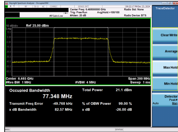
Plot 7-47. 26dB & 99% Bandwidth Plot Antenna 3b (80MHz 802.11ax (UNII Band 6) – Ch. 103)
