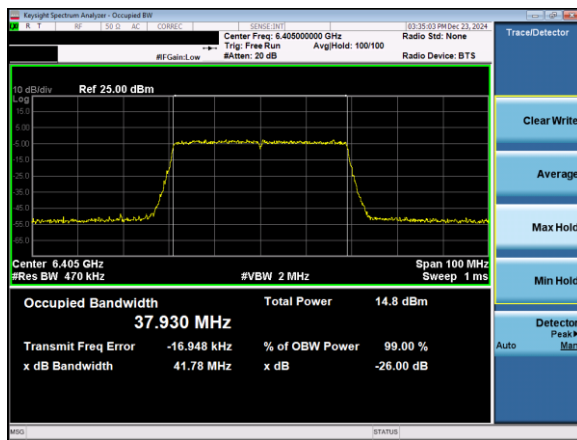
Plot 7-14. 26dB & 99% Bandwidth Plot Antenna 5T (40MHz 802.11ax (UNII Band 5) – Ch. 91)
