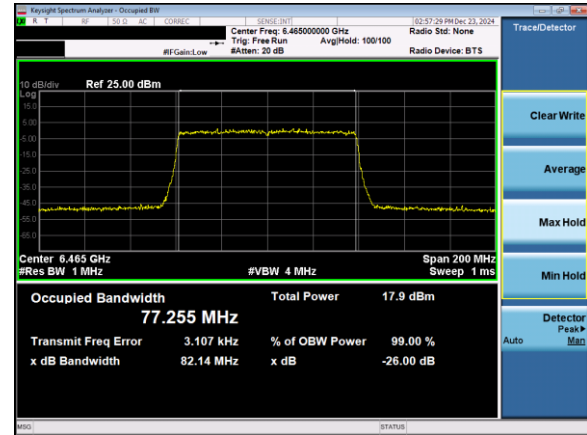
Plot 7-19. 26dB & 99% Bandwidth Plot Antenna 5T (80MHz 802.11ax (UNII Band 6) – Ch. 103)
