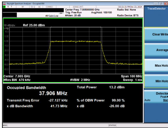
Plot 7-26. 26dB & 99% Bandwidth Plot Antenna 5T (40MHz 802.11ax (UNII Band 8) – Ch. 211)
