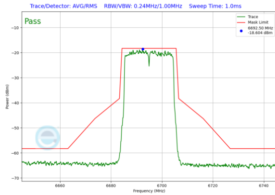
Plot 7-188. In-Band Emission Plot Antenna 1b (20MHz 802.11ax RU242 (UNII Band 7) – Ch. 149)
