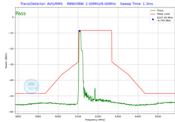
Plot 7-165. In-Band Emission Plot Antenna 3b (160MHz 802.11ax RU106 (UNII Band 5) – Ch. 47)
