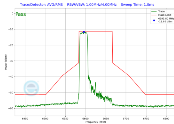
Plot 7-171. In-Band Emission Plot Antenna 3b (80MHz 802.11ax RU242 (UNII Band 7) – Ch. 135)
