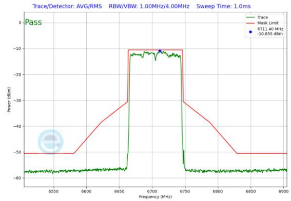
Plot 7-160. In-Band Emission Plot Antenna 5T (80MHz 802.11ax RU996 (UNII Band 7) – Ch. 151)
