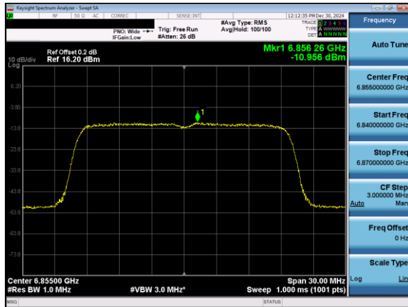
Plot 7-139. PSD Plot Antenna 5T (20MHz 802.11ax RU242 (UNII Band 7) – Ch. 181)
