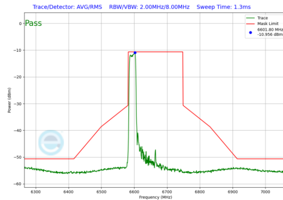
Plot 7-187. In-Band Emission Plot Antenna 1b (160MHz 802.11ax RU242 (UNII Band 7) – Ch. 143)
