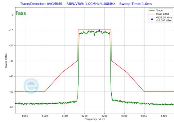
Plot 7-153. In-Band Emission Plot Antenna 5T (80MHz 802.11ax RU996 (UNII Band 5) – Ch. 55)
