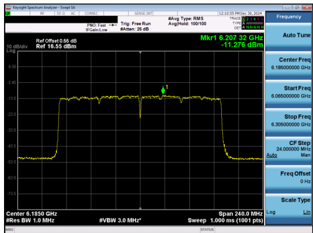
Plot 7-131. PSD Plot Antenna 5T (160MHz 802.11ax RU996x2 (UNII Band 5) – Ch. 47)
