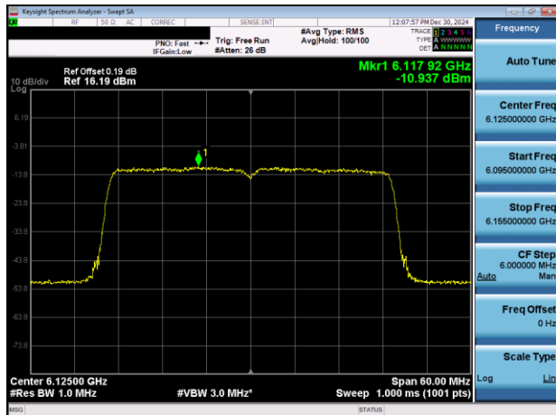
Plot 7-127. PSD Plot Antenna 5T (40MHz 802.11ax RU484 (UNII Band 5) – Ch. 35)
