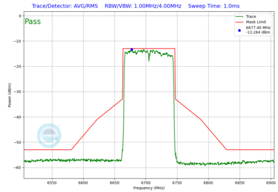
Plot 7-190. In-Band Emission Plot Antenna 1b (80MHz 802.11ax RU996 (UNII Band 7) – Ch. 151)
