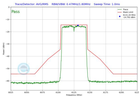
Plot 7-228. In-Band Emission Plot Antenna 5T (40MHz 802.11ax RU484 (UNII Band 5) – Ch. 35)
