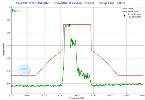
Plot 7-163. In-Band Emission Plot Antenna 3b (40MHz 802.11ax RU106 (UNII Band 5) – Ch. 35)
