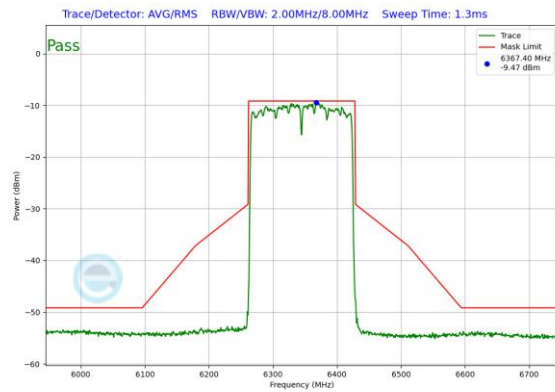
Plot 7-232. In-Band Emission Plot Antenna 5T (160MHz 802.11ax RU996x2 (UNII Band 5) – Ch. 79)
