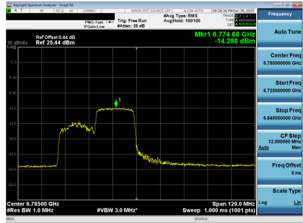
Plot 7-136. PSD Plot Antenna 1b (80MHz 802.11ax RU242 (UNII Band 7) – Ch. 167)
