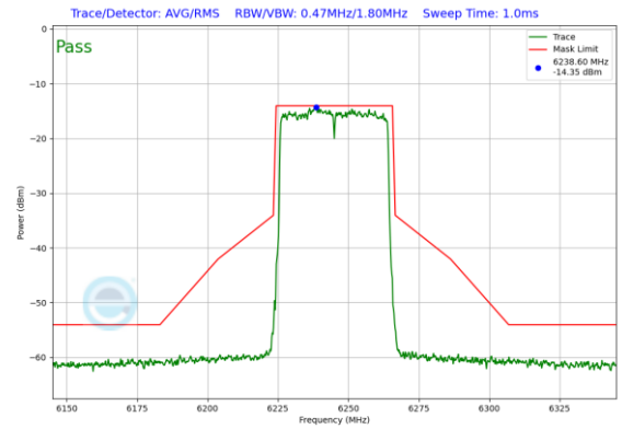
Plot 7-201. In-Band Emission Plot Antenna 3b (40MHz 802.11ax RU484 (UNII Band 5) – Ch. 59)
