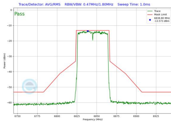
Plot 7-159. In-Band Emission Plot Antenna 5T (40MHz 802.11ax RU484 (UNII Band 7) – Ch. 179)
