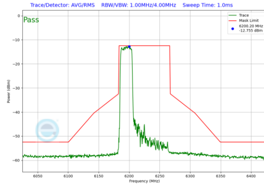
Plot 7-195. In-Band Emission Plot Antenna 3b (80MHz 802.11ax RU242 (UNII Band 5) – Ch. 55)
