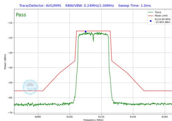
Plot 7-166. In-Band Emission Plot Antenna 3b (20MHz 802.11ax RU242 (UNII Band 5) – Ch. 33)
