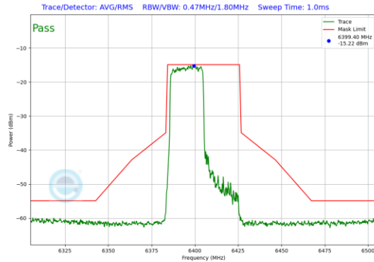
Plot 7-192. In-Band Emission Plot Antenna 5T (40MHz 802.11ax RU242 (UNII Band 5) – Ch. 91)
