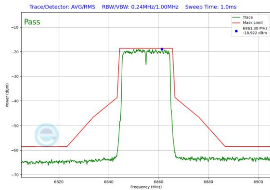
Plot 7-213. In-Band Emission Plot Antenna 3b (20MHz 802.11ax RU242 (UNII Band 7) – Ch. 181)
