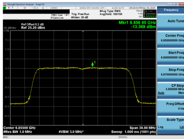
Plot 7-140. PSD Plot Antenna 1b (20MHz 802.11ax RU242 (UNII Band 7) – Ch. 181)
