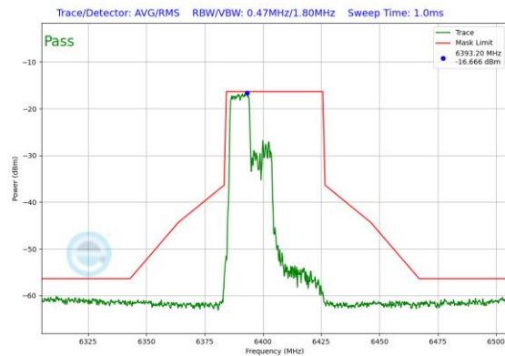
Plot 7-178. In-Band Emission Plot Antenna 1b (40MHz 802.11ax RU106 (UNII Band 5) – Ch. 91)
