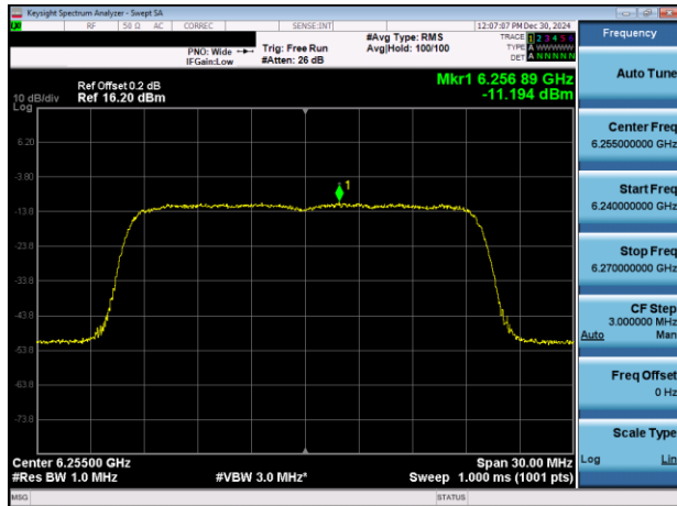
Plot 7-125. PSD Plot Antenna 5T (20MHz 802.11ax RU242 (UNII Band 5) – Ch. 61)
