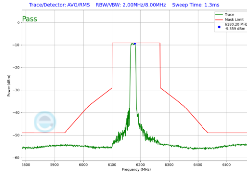
Plot 7-224. In-Band Emission Plot Antenna 5T (160MHz 802.11ax RU242 (UNII Band 5) – Ch. 47)
