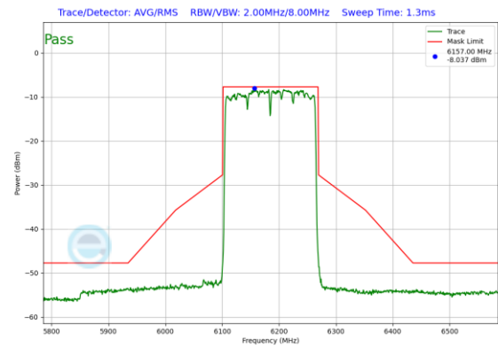
Plot 7-154. In-Band Emission Plot Antenna 5T (160MHz 802.11ax RU996x2 (UNII Band 5) – Ch. 47)
