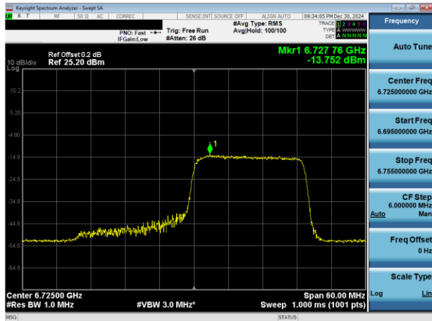
Plot 7-134. PSD Plot Antenna 1b (40MHz 802.11ax RU242 (UNII Band 7) – Ch. 155)
