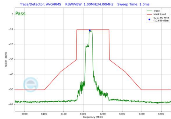
Plot 7-149. In-Band Emission Plot Antenna 5T (80MHz 802.11ax RU106 (UNII Band 5) – Ch. 55)
