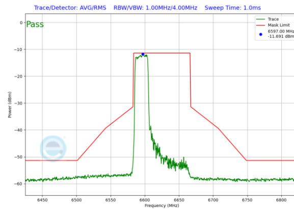
Plot 7-156. In-Band Emission Plot Antenna 5T (80MHz 802.11ax RU242 (UNII Band 7) – Ch. 135)
