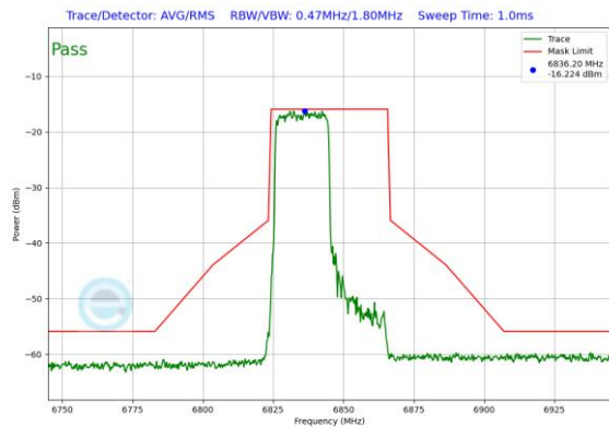
Plot 7-207. In-Band Emission Plot Antenna 3b (40MHz 802.11ax RU242 (UNII Band 7) – Ch. 179)
