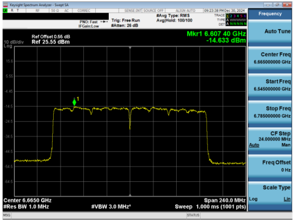
Plot 7-146. PSD Plot Antenna 1b (160MHz 802.11ax RU996x2 (UNII Band 7) – Ch. 143)
