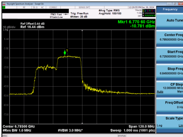
Plot 7-135. PSD Plot Antenna 5T (80MHz 802.11ax RU242 (UNII Band 7) – Ch. 167)
