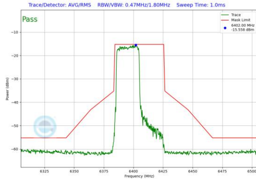
Plot 7-193. In-Band Emission Plot Antenna 3b (40MHz 802.11ax RU242 (UNII Band 5) – Ch. 91)
