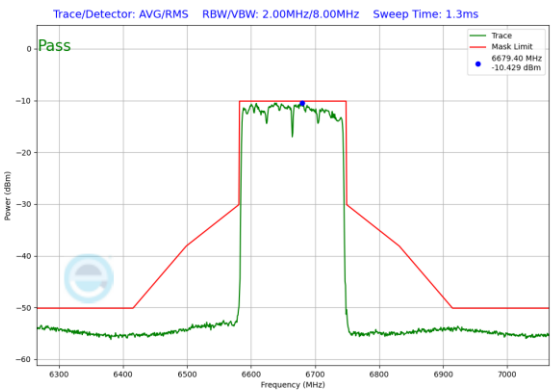
Plot 7-219. In-Band Emission Plot Antenna 3b (160MHz 802.11ax RU996x2 (UNII Band 7) – Ch. 143)
