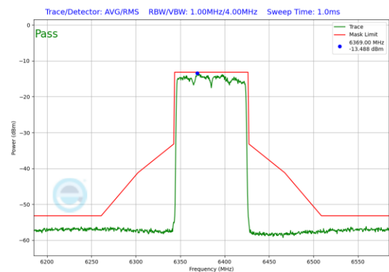
Plot 7-231. In-Band Emission Plot Antenna 1b (80MHz 802.11ax RU996 (UNII Band 5) – Ch. 87)
