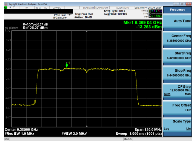
Plot 7-130. PSD Plot Antenna 1b (80MHz 802.11ax RU996 (UNII Band 5) – Ch. 87)
