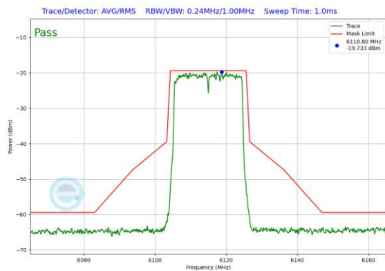
Plot 7-227. In-Band Emission Plot Antenna 1b (20MHz 802.11ax RU242 (UNII Band 5) – Ch. 33)
