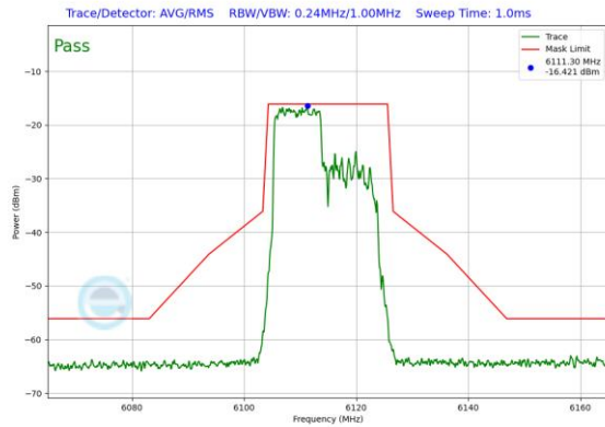
Plot 7-162. In-Band Emission Plot Antenna 3b (20MHz 802.11ax RU106 (UNII Band 5) – Ch. 33)
