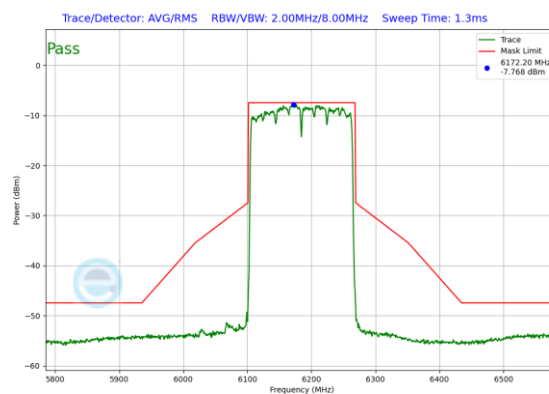
Plot 7-169. In-Band Emission Plot Antenna 3b (160MHz 802.11ax RU996x2 (UNII Band 5) – Ch. 47)
