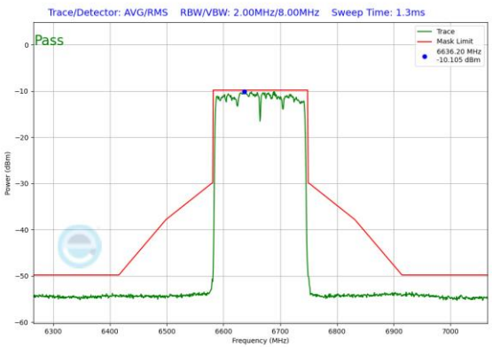
Plot 7-218. In-Band Emission Plot Antenna 5T (160MHz 802.11ax RU996x2 (UNII Band 7) – Ch. 143)
