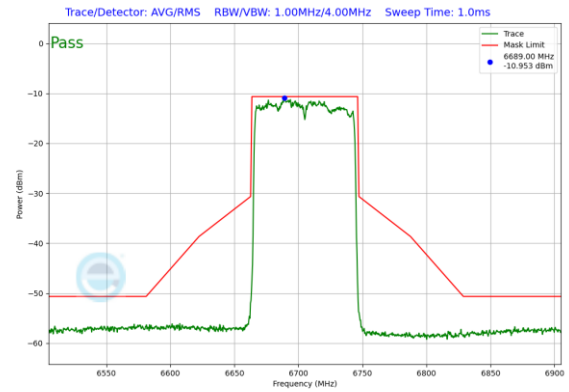
Plot 7-175. In-Band Emission Plot Antenna 3b (80MHz 802.11ax RU996 (UNII Band 7) – Ch. 151)
