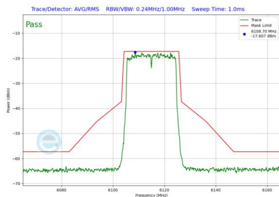
Plot 7-181. In-Band Emission Plot Antenna 1b (20MHz 802.11ax RU242 (UNII Band 5) – Ch. 33)
