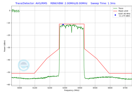
Plot 7-233. In-Band Emission Plot Antenna 1b (160MHz 802.11ax RU996x2 (UNII Band 5) – Ch. 79)
