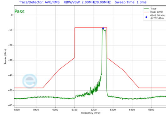
Plot 7-196. In-Band Emission Plot Antenna 5T (160MHz 802.11ax RU242 (UNII Band 5) – Ch. 47)
