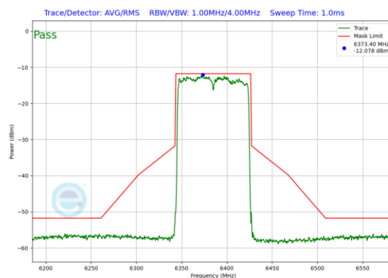
Plot 7-183. In-Band Emission Plot Antenna 1b (80MHz 802.11ax RU996 (UNII Band 5) – Ch. 87)
