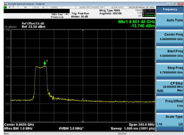
Plot 7-138. PSD Plot Antenna 1b (160MHz 802.11ax RU242 (UNII Band 7) – Ch. 143)
