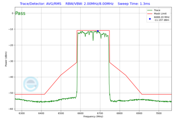
Plot 7-191. In-Band Emission Plot Antenna 1b (160MHz 802.11ax RU996x2 (UNII Band 7) – Ch. 143)
