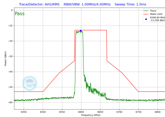
Plot 7-186. In-Band Emission Plot Antenna 1b (80MHz 802.11ax RU242 (UNII Band 7) – Ch. 135)
