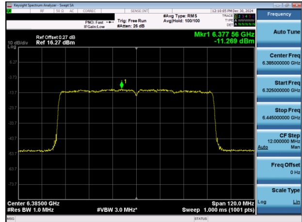
Plot 7-129. PSD Plot Antenna 5T (80MHz 802.11ax RU996 (UNII Band 5) – Ch. 87)
