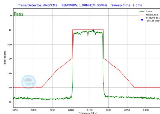
Plot 7-168. In-Band Emission Plot Antenna 3b (80MHz 802.11ax RU996 (UNII Band 5) – Ch. 39)
