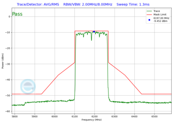
Plot 7-204. In-Band Emission Plot Antenna 5T (160MHz 802.11ax RU996x2 (UNII Band 5) – Ch. 47)
