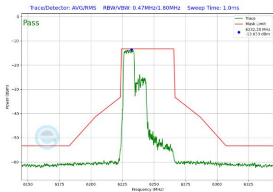
Plot 7-148. In-Band Emission Plot Antenna 5T (40MHz 802.11ax RU106 (UNII Band 5) – Ch. 59)
