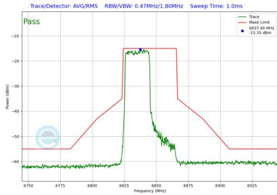
Plot 7-206. In-Band Emission Plot Antenna 5T (40MHz 802.11ax RU242 (UNII Band 7) – Ch. 179)
