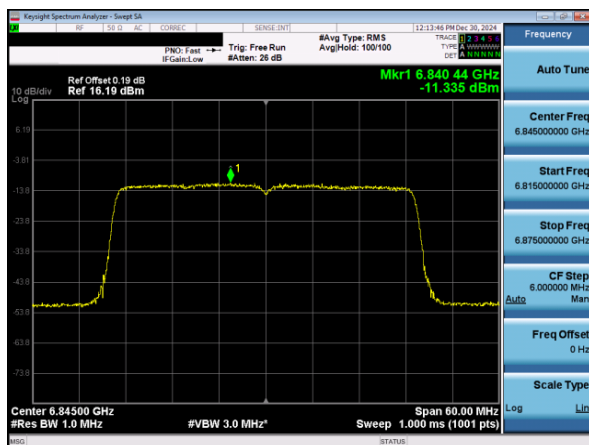
Plot 7-141. PSD Plot Antenna 5T (40MHz 802.11ax RU484 (UNII Band 7) – Ch. 179)
