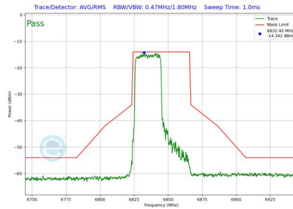
Plot 7-155. In-Band Emission Plot Antenna 5T (40MHz 802.11ax RU242 (UNII Band 7) – Ch. 179)
