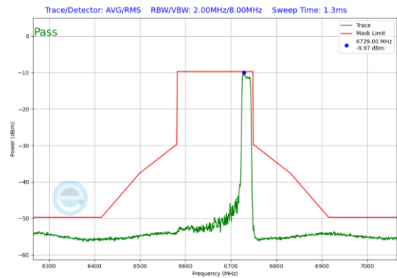
Plot 7-210. In-Band Emission Plot Antenna 5T (160MHz 802.11ax RU242 (UNII Band 7) – Ch. 143)
