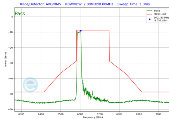
Plot 7-172. In-Band Emission Plot Antenna 3b (160MHz 802.11ax RU242 (UNII Band 7) – Ch. 143)
