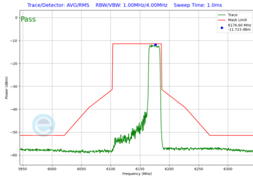
Plot 7-222. In-Band Emission Plot Antenna 5T (80MHz 802.11ax RU242 (UNII Band 5) – Ch. 39)
