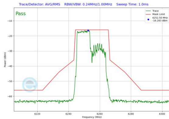
Plot 7-147. In-Band Emission Plot Antenna 5T (20MHz 802.11ax RU106 (UNII Band 5) – Ch. 61)
