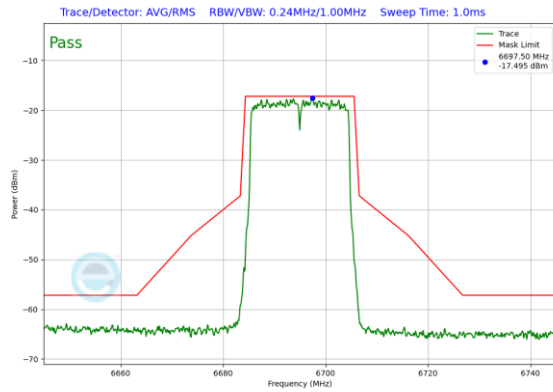
Plot 7-173. In-Band Emission Plot Antenna 3b (20MHz 802.11ax RU242 (UNII Band 7) – Ch. 149)
