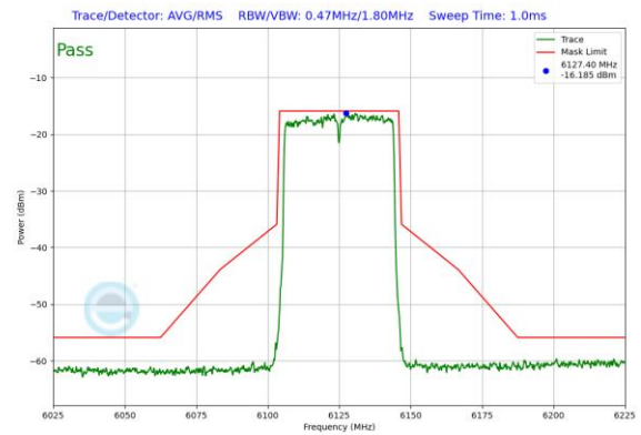
Plot 7-229. In-Band Emission Plot Antenna 1b (40MHz 802.11ax RU484 (UNII Band 5) – Ch. 35)
