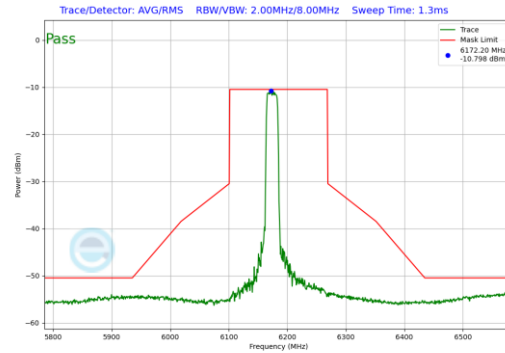
Plot 7-225. In-Band Emission Plot Antenna 1b (160MHz 802.11ax RU242 (UNII Band 5) – Ch. 47)
