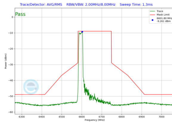
Plot 7-157. In-Band Emission Plot Antenna 5T (160MHz 802.11ax RU242 (UNII Band 7) – Ch. 143)
