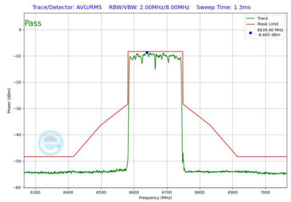
Plot 7-161. In-Band Emission Plot Antenna 5T (160MHz 802.11ax RU996x2 (UNII Band 7) – Ch. 143)
