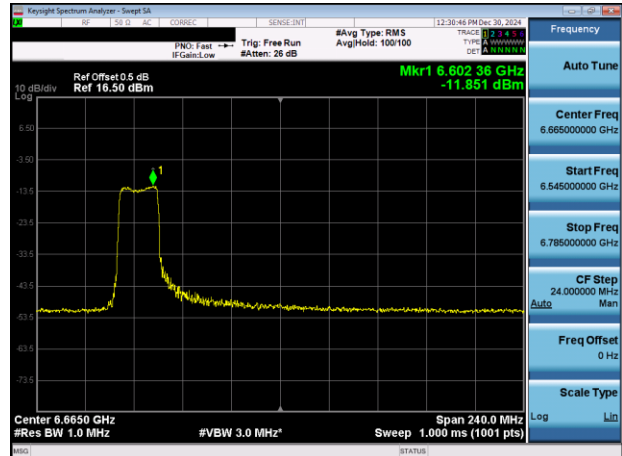
Plot 7-137. PSD Plot Antenna 5T (160MHz 802.11ax RU242 (UNII Band 7) – Ch. 143)
