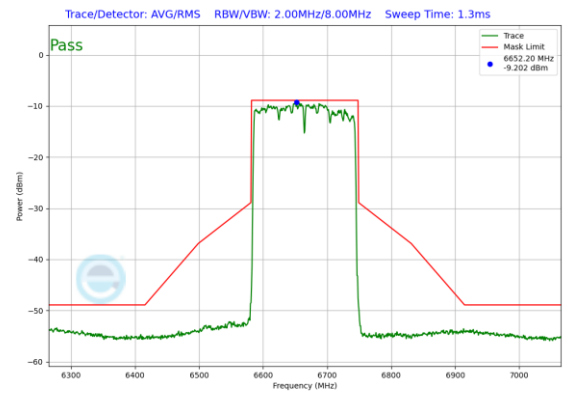
Plot 7-176. In-Band Emission Plot Antenna 3b (160MHz 802.11ax RU996x2 (UNII Band 7) – Ch. 143)
