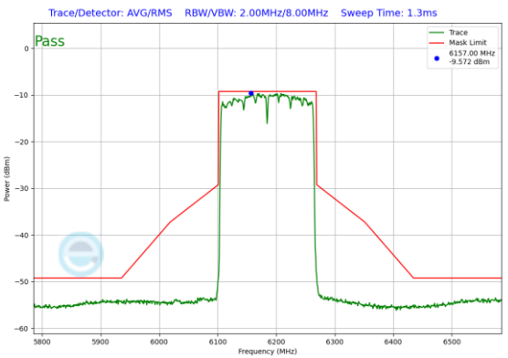
Plot 7-205. In-Band Emission Plot Antenna 3b (160MHz 802.11ax RU996x2 (UNII Band 5) – Ch. 47)
