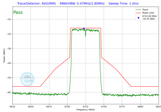
Plot 7-189. In-Band Emission Plot Antenna 1b (40MHz 802.11ax RU484 (UNII Band 7) – Ch. 155)
