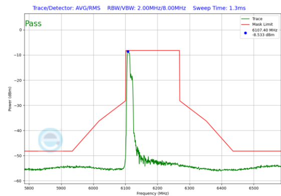
Plot 7-150. In-Band Emission Plot Antenna 5T (160MHz 802.11ax RU106 (UNII Band 5) – Ch. 47)
