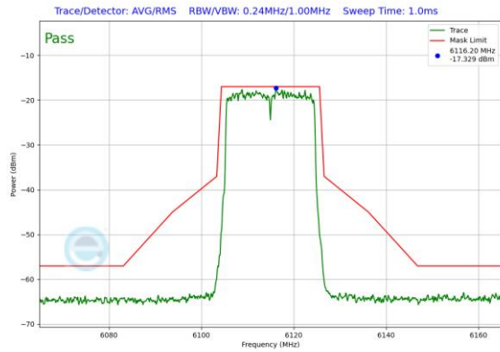
Plot 7-198. In-Band Emission Plot Antenna 5T (20MHz 802.11ax RU242 (UNII Band 5) – Ch. 33)
