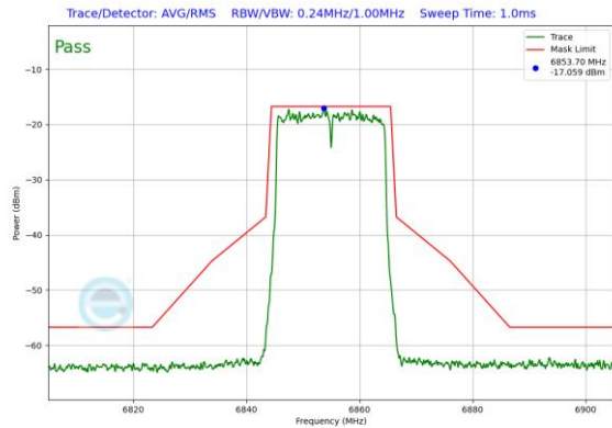
Plot 7-212. In-Band Emission Plot Antenna 5T (20MHz 802.11ax RU242 (UNII Band 7) – Ch. 181)
