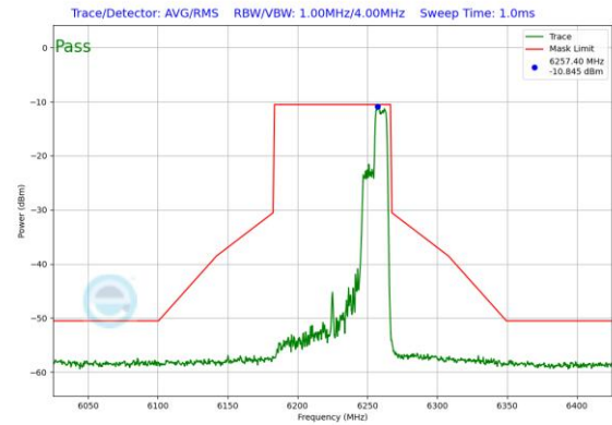
Plot 7-164. In-Band Emission Plot Antenna 3b (80MHz 802.11ax RU106 (UNII Band 5) – Ch. 55)
