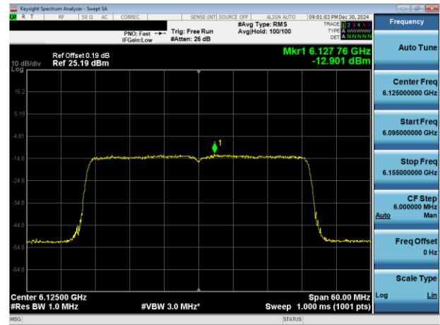
Plot 7-128. PSD Plot Antenna 1b (40MHz 802.11ax RU484 (UNII Band 5) – Ch. 35)
