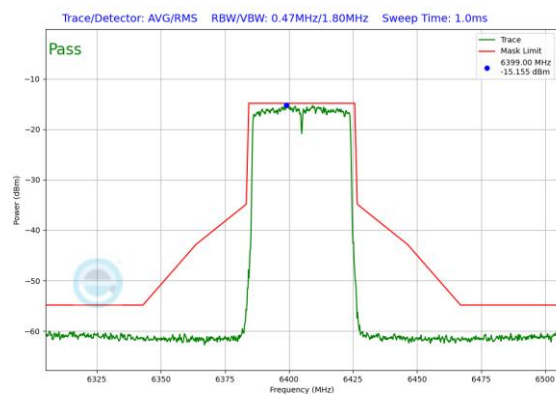
Plot 7-182. In-Band Emission Plot Antenna 1b (40MHz 802.11ax RU484 (UNII Band 5) – Ch. 91)
