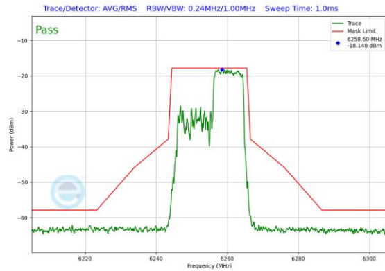
Plot 7-177. In-Band Emission Plot Antenna 1b (20MHz 802.11ax RU106 (UNII Band 5) – Ch. 61)
