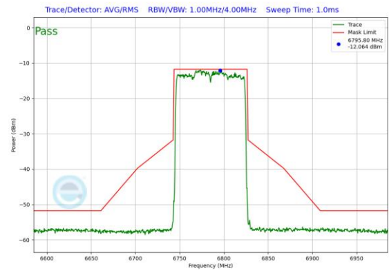
Plot 7-216. In-Band Emission Plot Antenna 5T (80MHz 802.11ax RU996 (UNII Band 7) – Ch. 167)
