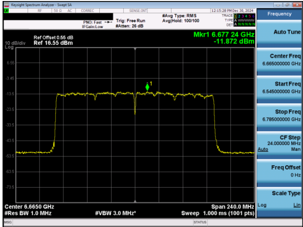
Plot 7-145. PSD Plot Antenna 5T (160MHz 802.11ax RU996x2 (UNII Band 7) – Ch. 143)
