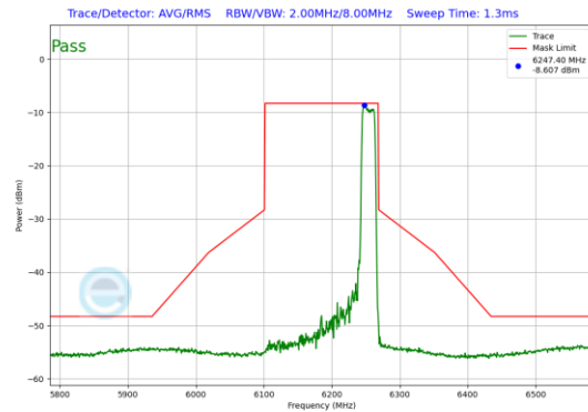
Plot 7-197. In-Band Emission Plot Antenna 3b (160MHz 802.11ax RU242 (UNII Band 5) – Ch. 47)
