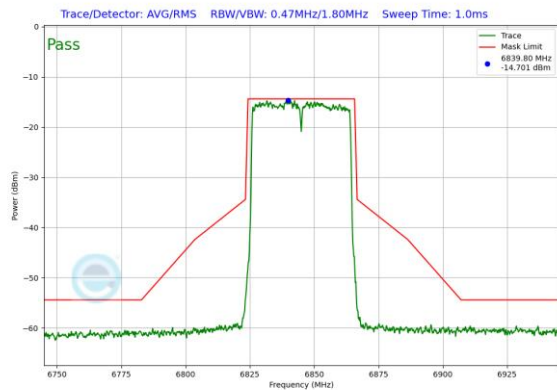
Plot 7-214. In-Band Emission Plot Antenna 5T (40MHz 802.11ax RU484 (UNII Band 7) – Ch. 179)
