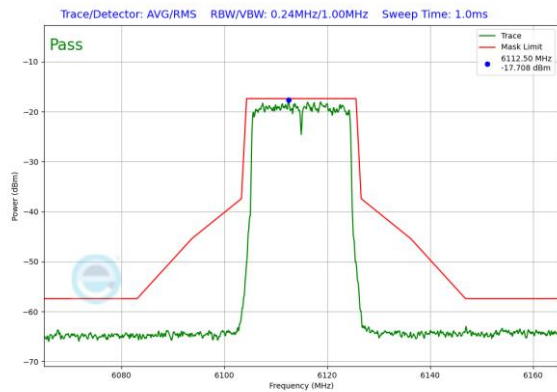
Plot 7-199. In-Band Emission Plot Antenna 3b (20MHz 802.11ax RU242 (UNII Band 5) – Ch. 33)
