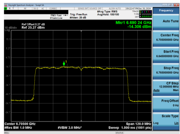
Plot 7-144. PSD Plot Antenna 1b (80MHz 802.11ax RU996 (UNII Band 7) – Ch. 151)
