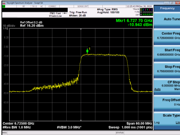
Plot 7-133. PSD Plot Antenna 5T (40MHz 802.11ax RU242 (UNII Band 7) – Ch. 155)
