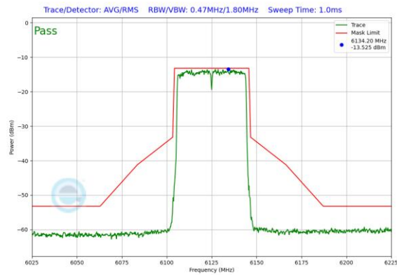
Plot 7-152. In-Band Emission Plot Antenna 5T (40MHz 802.11ax RU484 (UNII Band 5) – Ch. 35)
