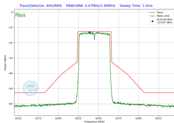
Plot 7-167. In-Band Emission Plot Antenna 3b (40MHz 802.11ax RU484 (UNII Band 5) – Ch. 59)
