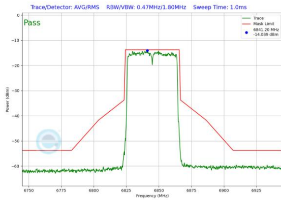
Plot 7-174. In-Band Emission Plot Antenna 3b (40MHz 802.11ax RU484 (UNII Band 7) – Ch. 179)
