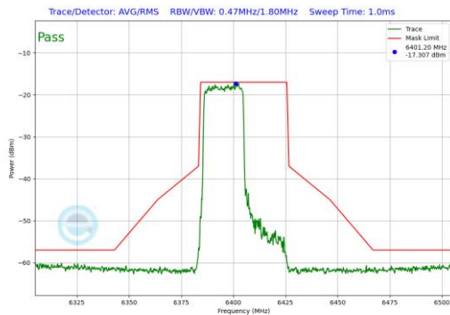
Plot 7-221. In-Band Emission Plot Antenna 1b (40MHz 802.11ax RU242 (UNII Band 5) – Ch. 91)
