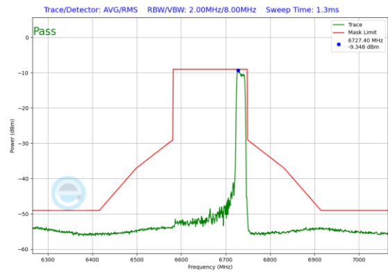
Plot 7-211. In-Band Emission Plot Antenna 3b (160MHz 802.11ax RU242 (UNII Band 7) – Ch. 143)
