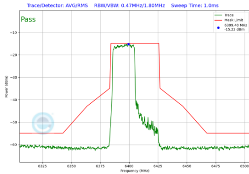
Plot 7-220. In-Band Emission Plot Antenna 5T (40MHz 802.11ax RU242 (UNII Band 5) – Ch. 91)
