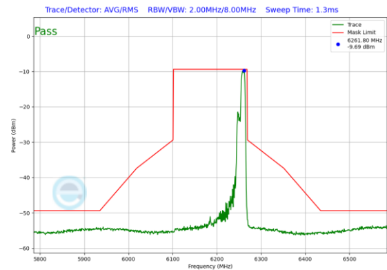
Plot 7-180. In-Band Emission Plot Antenna 1b (160MHz 802.11ax RU106 (UNII Band 5) – Ch. 47)
