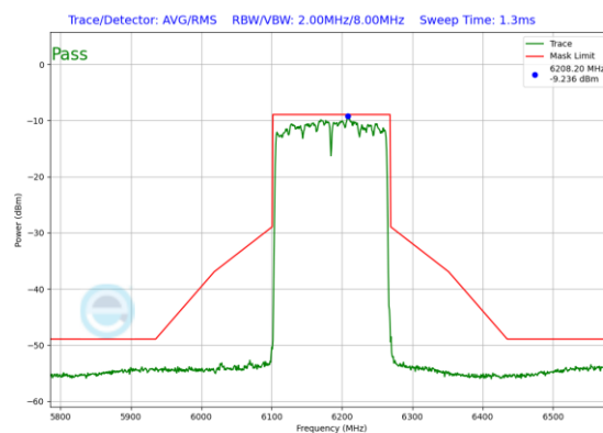
Plot 7-184. In-Band Emission Plot Antenna 1b (160MHz 802.11ax RU996x2 (UNII Band 5) – Ch. 47)
