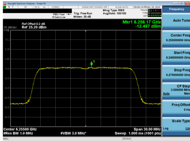
Plot 7-126. PSD Plot Antenna 1b (20MHz 802.11ax RU242 (UNII Band 5) – Ch. 61)
