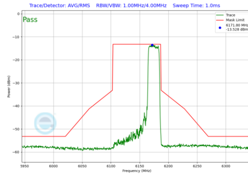
Plot 7-223. In-Band Emission Plot Antenna 1b (80MHz 802.11ax RU242 (UNII Band 5) – Ch. 39)
