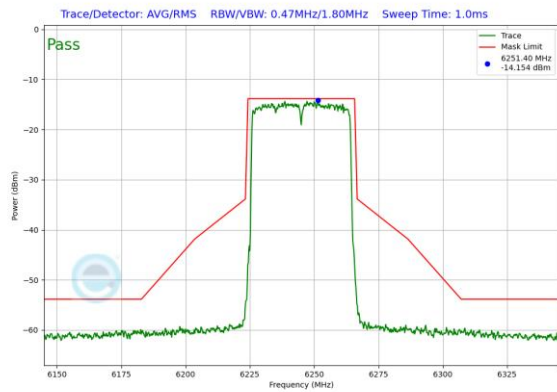
Plot 7-200. In-Band Emission Plot Antenna 5T (40MHz 802.11ax RU484 (UNII Band 5) – Ch. 59)
