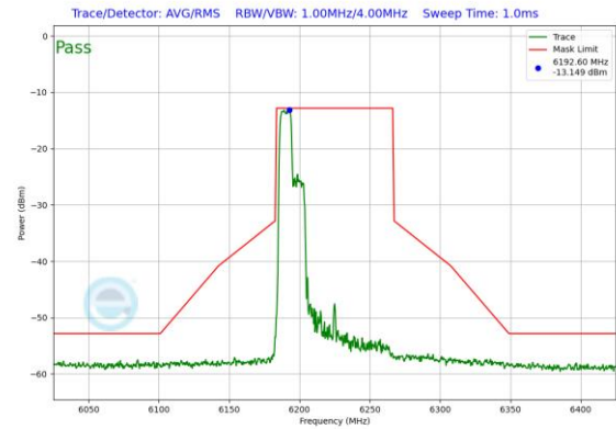
Plot 7-179. In-Band Emission Plot Antenna 1b (80MHz 802.11ax RU106 (UNII Band 5) – Ch. 55)
