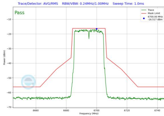
Plot 7-158. In-Band Emission Plot Antenna 5T (20MHz 802.11ax RU242 (UNII Band 7) – Ch. 149)
