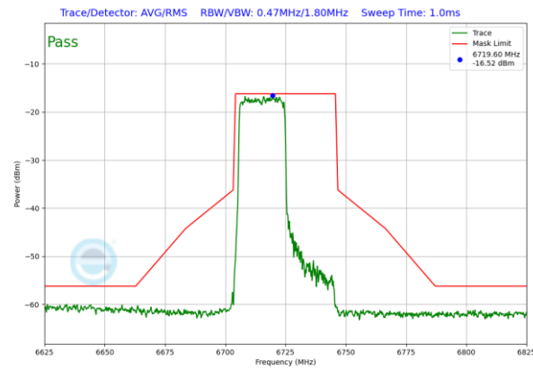
Plot 7-185. In-Band Emission Plot Antenna 1b (40MHz 802.11ax RU242 (UNII Band 7) – Ch. 155)
