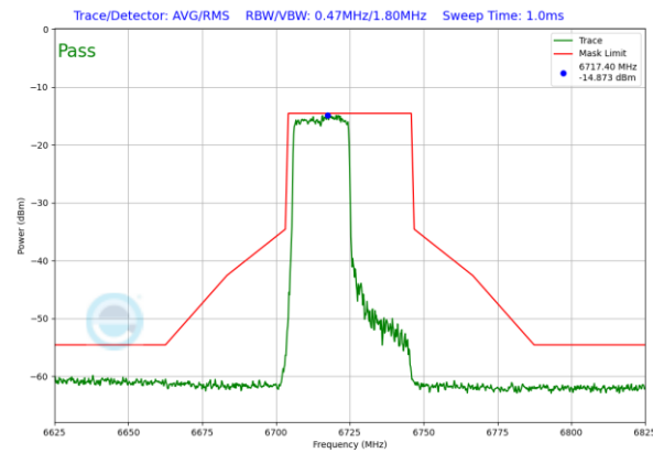
Plot 7-170. In-Band Emission Plot Antenna 3b (40MHz 802.11ax RU242 (UNII Band 7) – Ch. 155)
