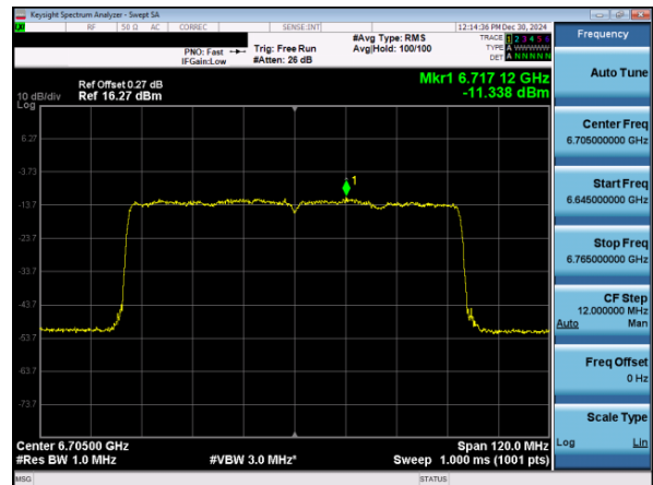
Plot 7-143. PSD Plot Antenna 5T (80MHz 802.11ax RU996 (UNII Band 7) – Ch. 151)
