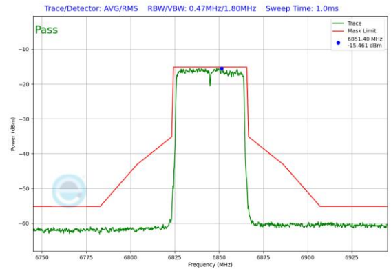
Plot 7-215. In-Band Emission Plot Antenna 3b (40MHz 802.11ax RU484 (UNII Band 7) – Ch. 179)
