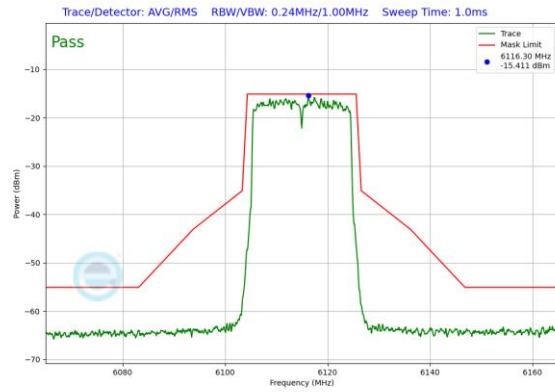
Plot 7-151. In-Band Emission Plot Antenna 5T (20MHz 802.11ax RU242 (UNII Band 5) – Ch. 33)
