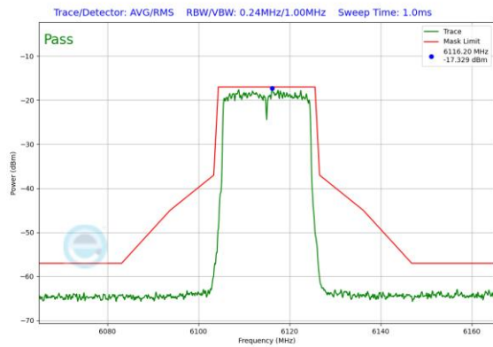
Plot 7-226. In-Band Emission Plot Antenna 5T (20MHz 802.11ax RU242 (UNII Band 5) – Ch. 33)
