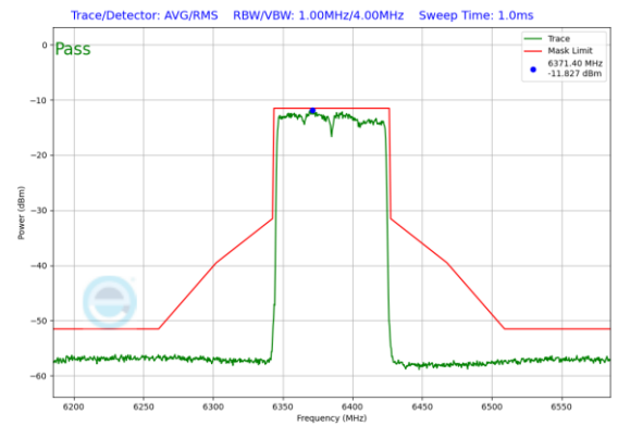
Plot 7-203. In-Band Emission Plot Antenna 3b (80MHz 802.11ax RU996 (UNII Band 5) – Ch. 87)
