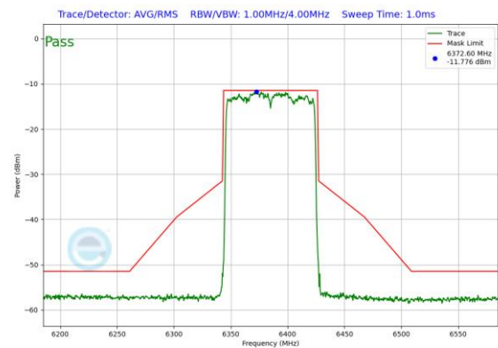
Plot 7-230. In-Band Emission Plot Antenna 5T (80MHz 802.11ax RU996 (UNII Band 5) – Ch. 87)
