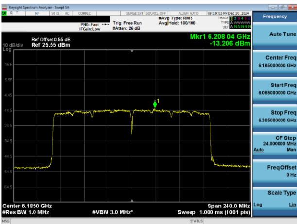
Plot 7-132. PSD Plot Antenna 1b (160MHz 802.11ax RU996x2 (UNII Band 5) – Ch. 47)
