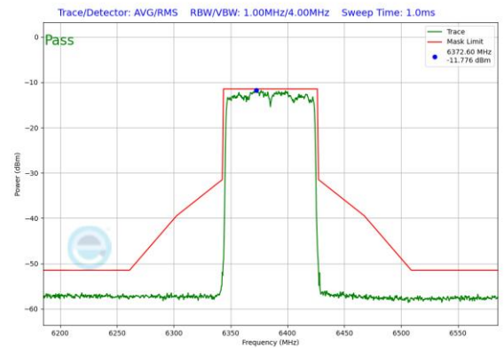
Plot 7-202. In-Band Emission Plot Antenna 5T (80MHz 802.11ax RU996 (UNII Band 5) – Ch. 87)
