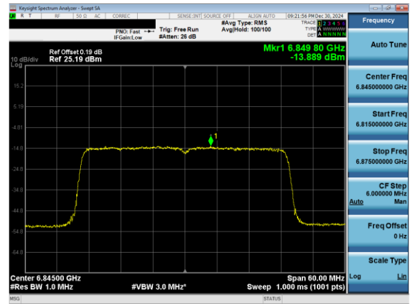
Plot 7-142. PSD Plot Antenna 1b (40MHz 802.11ax RU484 (UNII Band 7) – Ch. 179)
