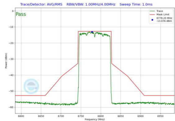
Plot 7-217. In-Band Emission Plot Antenna 3b (80MHz 802.11ax RU996 (UNII Band 7) – Ch. 167)
