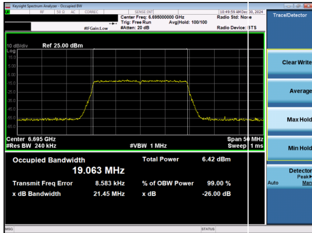
Plot 7-12. 26dB & 99% Bandwidth Plot Antenna 5T (20MHz 802.11ax RU242 (UNII Band 7) – Ch. 149)
