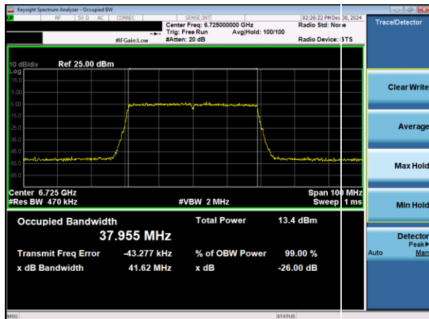
Plot 7-28. 26dB & 99% Bandwidth Plot Antenna 3b (40MHz 802.11ax RU484 (UNII Band 7) – Ch. 155)
