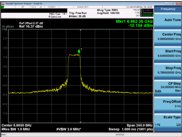
Plot 7-56. PSD Plot Antenna 5T (160MHz 802.11ax RU106 (UNII Band 7) – Ch. 143)
