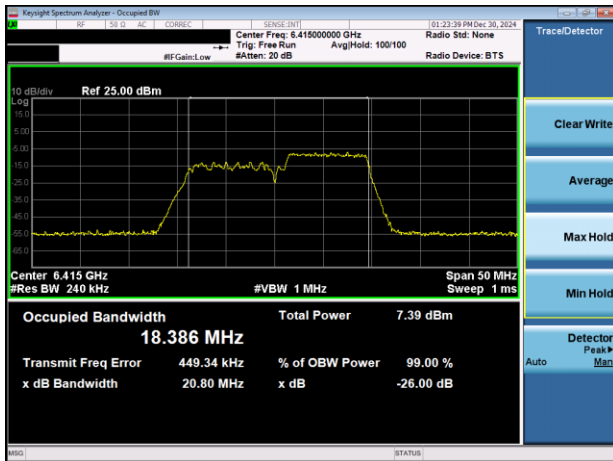
Plot 7-16. 26dB & 99% Bandwidth Plot Antenna 3b (20MHz 802.11ax RU106 (UNII Band 5) – Ch. 93)
