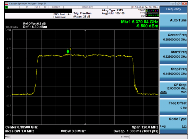
Plot 7-52. PSD Plot Antenna 5T (80MHz 802.11ax RU996 (UNII Band 5) – Ch. 87)
