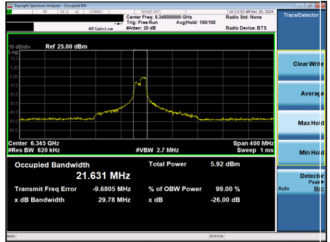
Plot 7-4. 26dB & 99% Bandwidth Plot Antenna 5T (160MHz 802.11ax RU106 (UNII Band 5) – Ch. 79)
