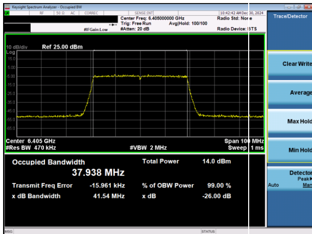
Plot 7-6. 26dB & 99% Bandwidth Plot Antenna 5T (40MHz 802.11ax RU484 (UNII Band 5) – Ch. 91)
