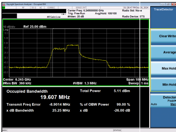
Plot 7-17. 26dB & 99% Bandwidth Plot Antenna 3b (40MHz 802.11ax RU106 (UNII Band 5) – Ch. 59)
