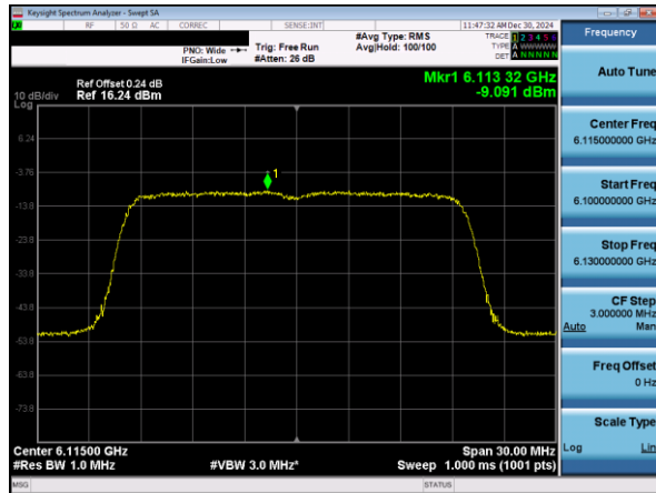
Plot 7-50. PSD Plot Antenna 5T (20MHz 802.11ax RU242 (UNII Band 5) – Ch. 33)
