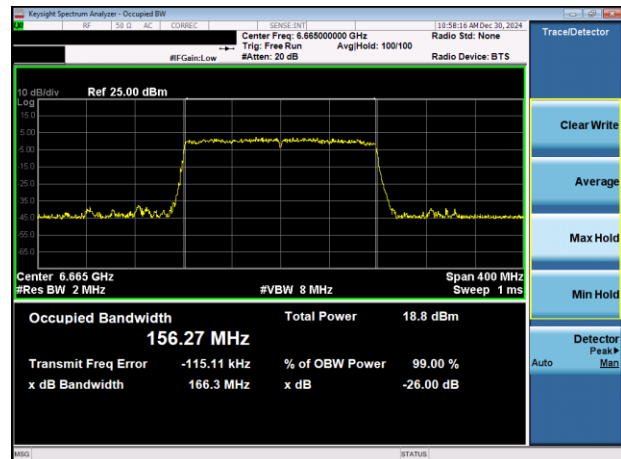
Plot 7-15. 26dB & 99% Bandwidth Plot Antenna 5T (160MHz 802.11ax RU996x2 (UNII Band 7) – Ch. 143)
