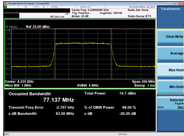
Plot 7-22. 26dB & 99% Bandwidth Plot Antenna 3b (80MHz 802.11ax RU996 (UNII Band 5) – Ch. 55)
