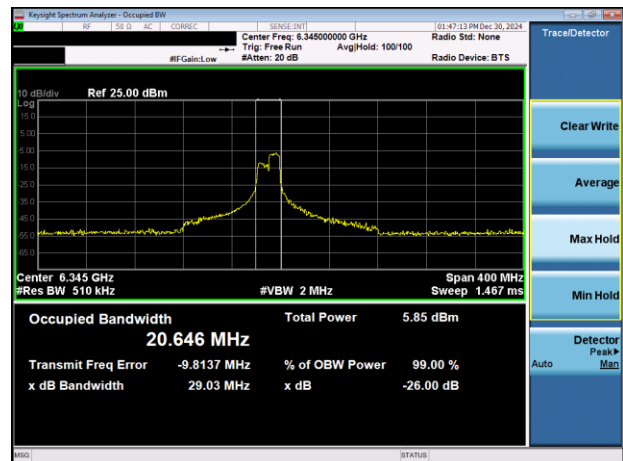
Plot 7-19. 26dB & 99% Bandwidth Plot Antenna 3b (160MHz 802.11ax RU106 (UNII Band 5) – Ch. 79)
