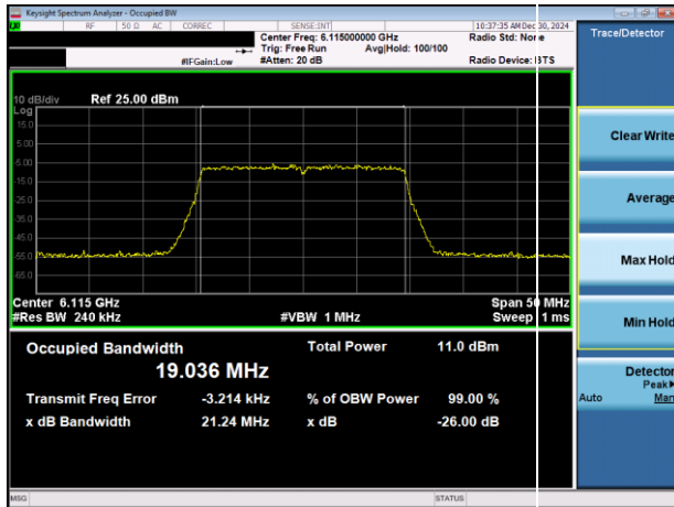
Plot 7-5. 26dB & 99% Bandwidth Plot Antenna 5T (20MHz 802.11ax RU242 (UNII Band 5) – Ch. 33)
