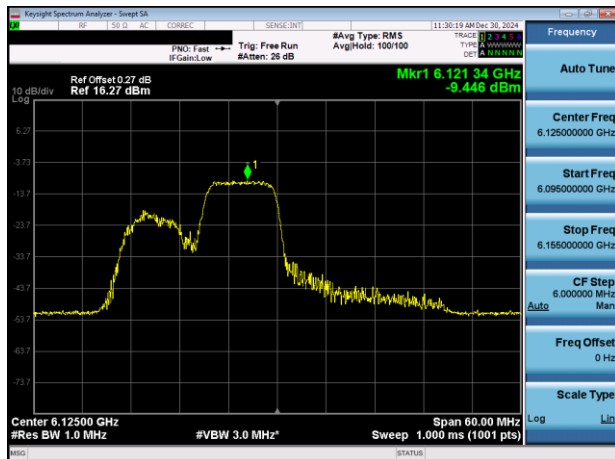
Plot 7-47. PSD Plot Antenna 5T (40MHz 802.11ax RU106 (UNII Band 5) – Ch. 35)
