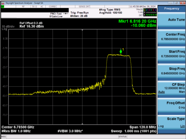
Plot 7-55. PSD Plot Antenna 5T (80MHz 802.11ax RU242 (UNII Band 7) – Ch. 167)
