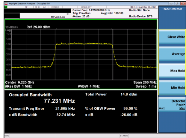
Plot 7-7. 26dB & 99% Bandwidth Plot Antenna 5T (80MHz 802.11ax RU996 (UNII Band 5) – Ch. 55)
