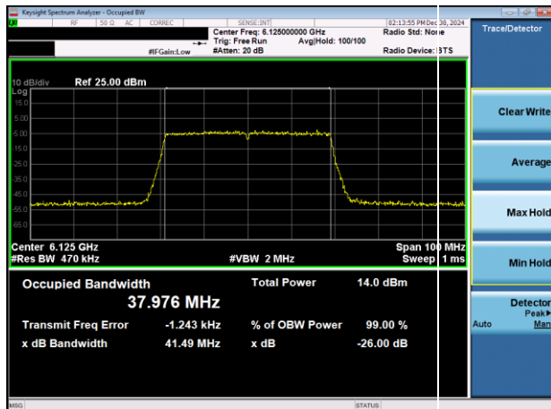
Plot 7-21. 26dB & 99% Bandwidth Plot Antenna 3b (40MHz 802.11ax RU484 (UNII Band 5) – Ch. 35)
