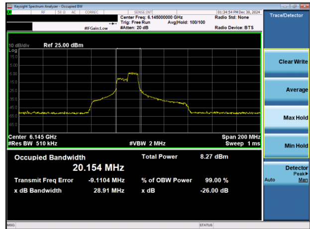
Plot 7-18. 26dB & 99% Bandwidth Plot Antenna 3b (80MHz 802.11ax RU106 (UNII Band 5) – Ch. 39)
