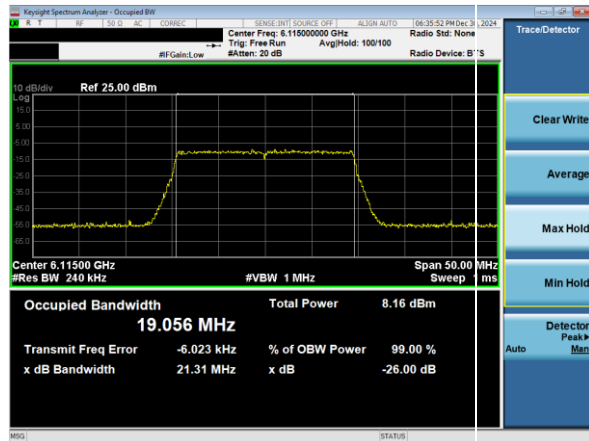
Plot 7-35. 26dB & 99% Bandwidth Plot Antenna 1b (20MHz 802.11ax RU242 (UNII Band 5) – Ch. 33)
