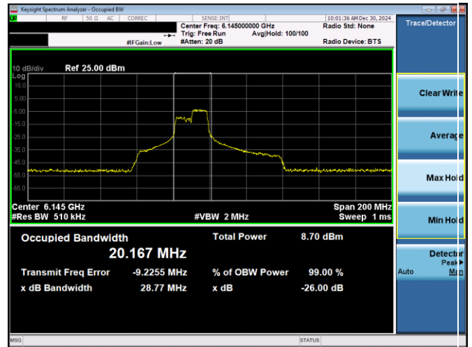
Plot 7-3. 26dB & 99% Bandwidth Plot Antenna 5T (80MHz 802.11ax RU106 (UNII Band 5) – Ch. 39)
