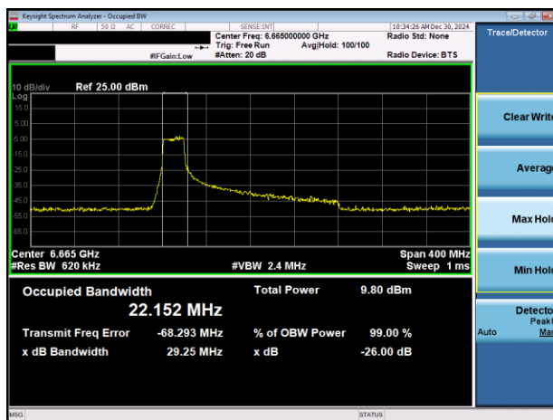
Plot 7-11. 26dB & 99% Bandwidth Plot Antenna 5T (160MHz 802.11ax RU242 (UNII Band 7) – Ch. 143)
