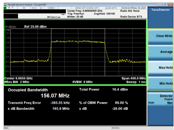
Plot 7-45. 26dB & 99% Bandwidth Plot Antenna 1b (160MHz 802.11ax RU996x2 (UNII Band 7) – Ch. 143)
