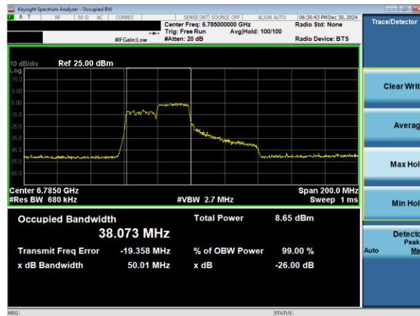
Plot 7-40. 26dB & 99% Bandwidth Plot Antenna 1b (80MHz 802.11ax RU242 (UNII Band 7) – Ch. 167)
