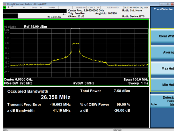
Plot 7-41. 26dB & 99% Bandwidth Plot Antenna 1b (160MHz 802.11ax RU242 (UNII Band 7) – Ch. 143)
