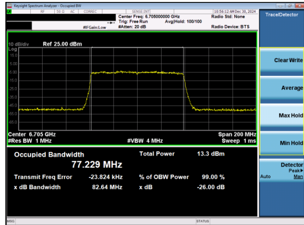
Plot 7-14. 26dB & 99% Bandwidth Plot Antenna 5T (80MHz 802.11ax RU996 (UNII Band 7) – Ch. 151)
