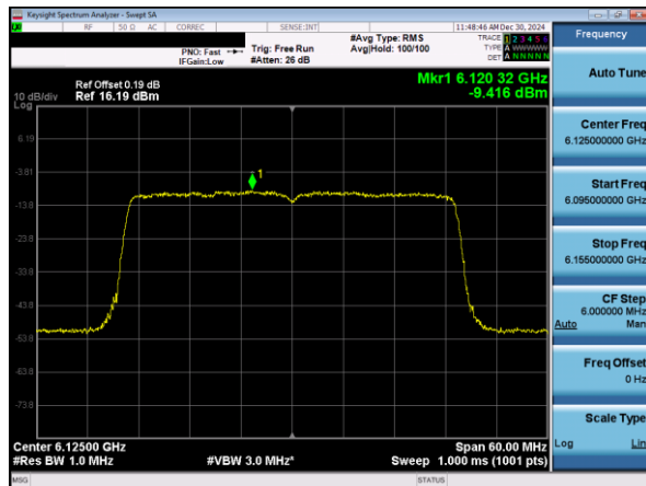
Plot 7-51. PSD Plot Antenna 5T (40MHz 802.11ax RU484 (UNII Band 5) – Ch. 35)
