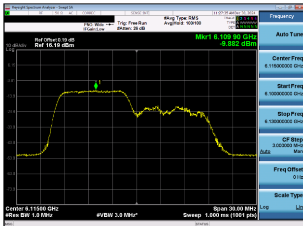
Plot 7-46. PSD Plot Antenna 5T (20MHz 802.11ax RU106 (UNII Band 5) – Ch. 33)
