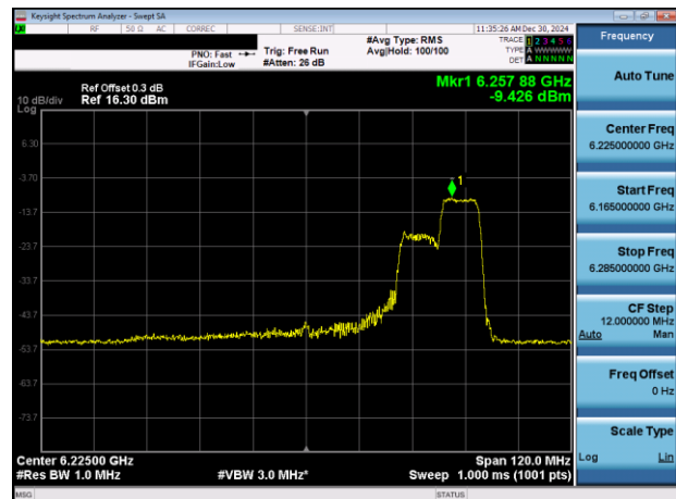
Plot 7-48. PSD Plot Antenna 5T (80MHz 802.11ax RU106 (UNII Band 5) – Ch. 55)
