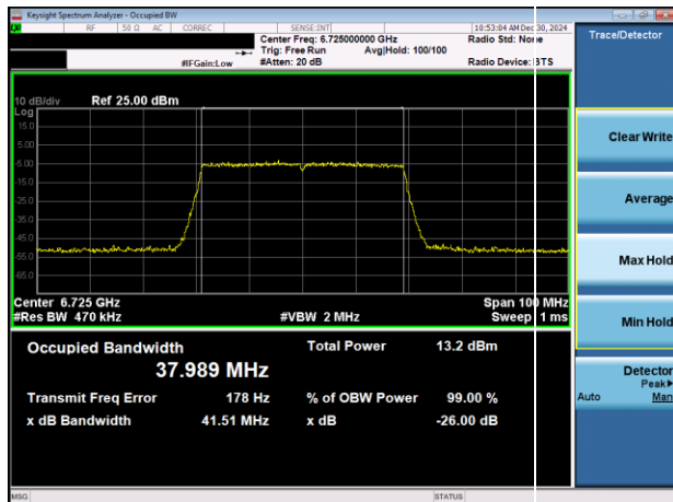
Plot 7-13. 26dB & 99% Bandwidth Plot Antenna 5T (40MHz 802.11ax RU484 (UNII Band 7) – Ch. 155)
