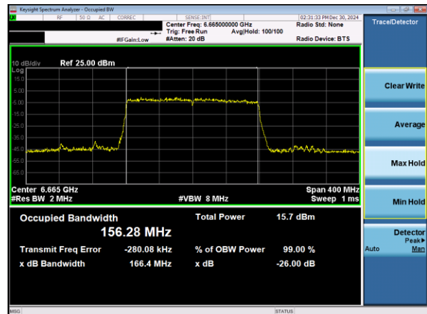
Plot 7-30. 26dB & 99% Bandwidth Plot Antenna 3b (160MHz 802.11ax RU996x2 (UNII Band 7) – Ch. 143)
