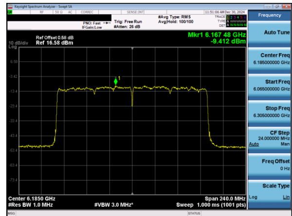
Plot 7-53. PSD Plot Antenna 5T (160MHz 802.11ax RU996x2 (UNII Band 5) – Ch. 47)
