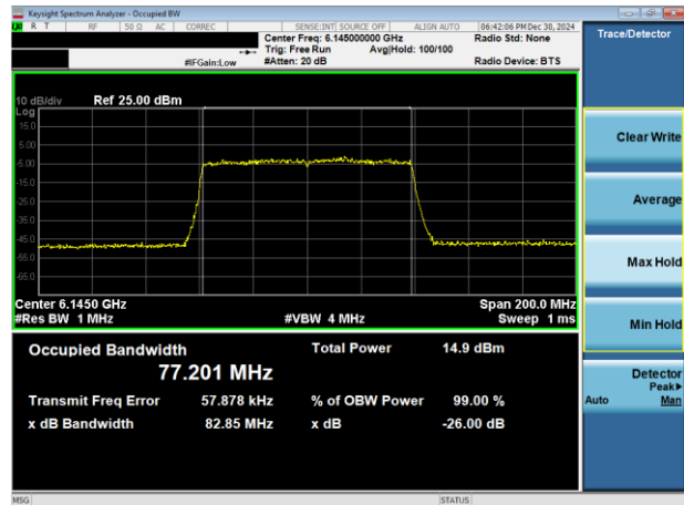
Plot 7-37. 26dB & 99% Bandwidth Plot Antenna 1b (80MHz 802.11ax RU996 (UNII Band 5) – Ch. 39)
