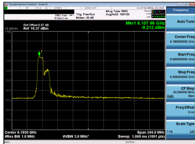
Plot 7-49. PSD Plot Antenna 5T (160MHz 802.11ax RU106 (UNII Band 5) – Ch. 47)
