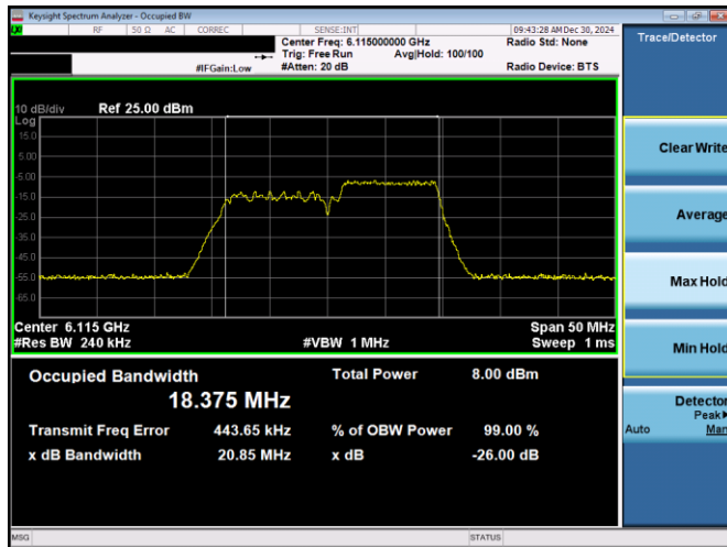
Plot 7-1. 26dB & 99% Bandwidth Plot Antenna 5T (20MHz 802.11ax RU106 (UNII Band 5) – Ch. 33)
