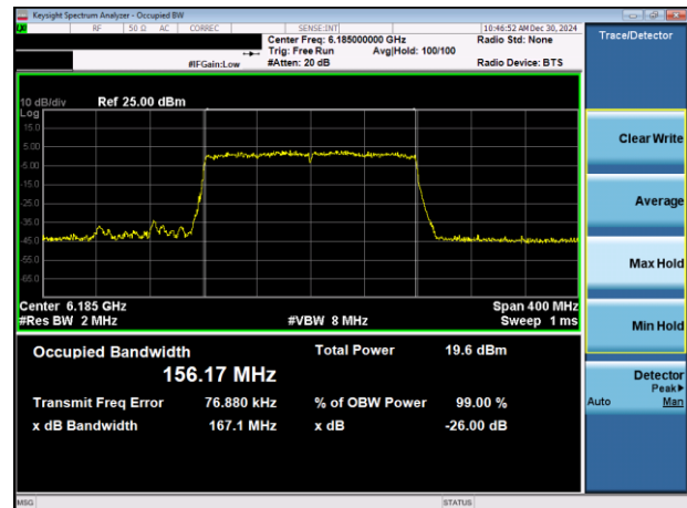
Plot 7-8. 26dB & 99% Bandwidth Plot Antenna 5T (160MHz 802.11ax RU996x2 (UNII Band 5) – Ch. 47)
