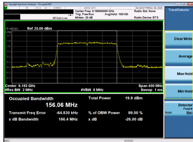
Plot 7-23. 26dB & 99% Bandwidth Plot Antenna 3b (160MHz 802.11ax RU996x2 (UNII Band 5) – Ch. 47)
