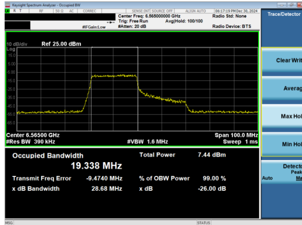
Plot 7-39. 26dB & 99% Bandwidth Plot Antenna 1b (40MHz 802.11ax RU242 (UNII Band 7) – Ch. 123)
