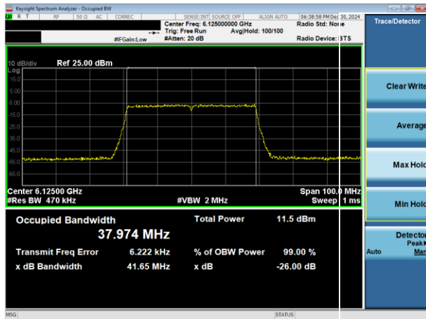
Plot 7-36. 26dB & 99% Bandwidth Plot Antenna 1b (40MHz 802.11ax RU484 (UNII Band 5) – Ch. 35)
