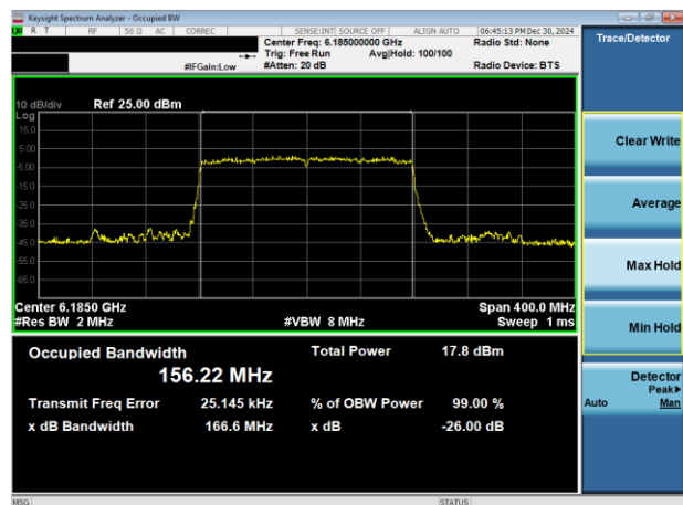
Plot 7-38. 26dB & 99% Bandwidth Plot Antenna 1b (160MHz 802.11ax RU996x2 (UNII Band 5) – Ch. 47)
