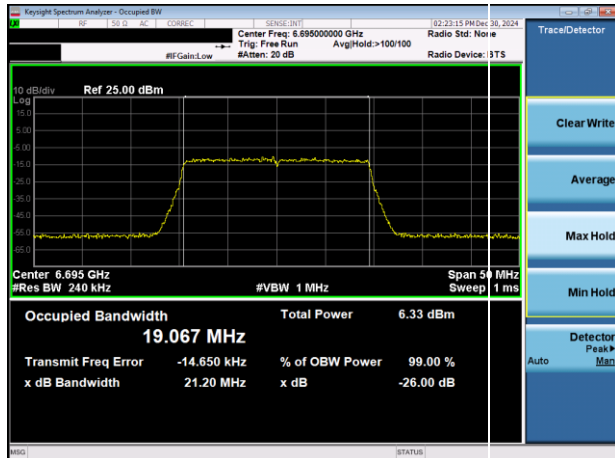
Plot 7-27. 26dB & 99% Bandwidth Plot Antenna 3b (20MHz 802.11ax RU242 (UNII Band 7) – Ch. 149)
