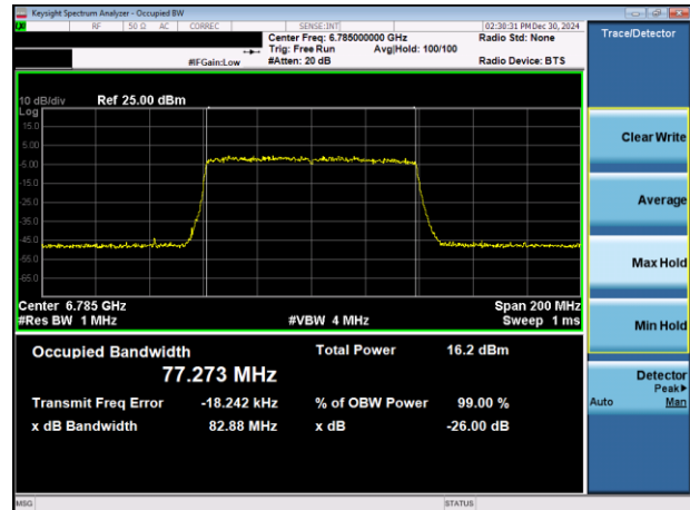
Plot 7-29. 26dB & 99% Bandwidth Plot Antenna 3b (80MHz 802.11ax RU996 (UNII Band 7) – Ch. 167)
