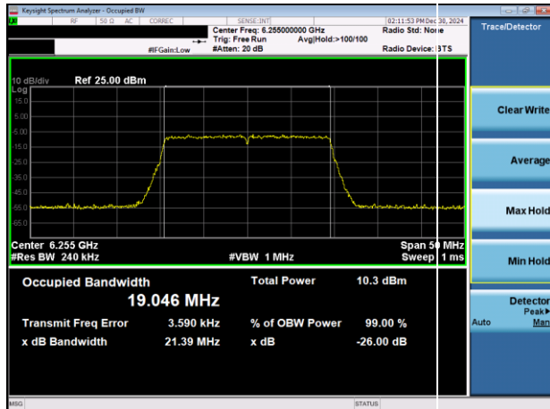
Plot 7-20. 26dB & 99% Bandwidth Plot Antenna 3b (20MHz 802.11ax RU242 (UNII Band 5) – Ch. 61)
