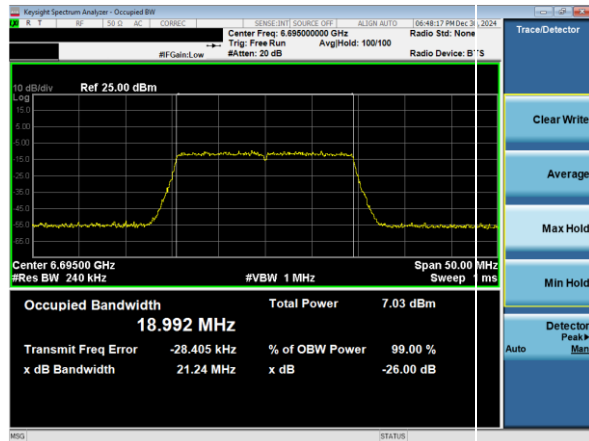
Plot 7-42. 26dB & 99% Bandwidth Plot Antenna 1b (20MHz 802.11ax RU242 (UNII Band 7) – Ch. 149)
