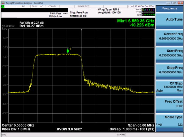
Plot 7-54. PSD Plot Antenna 5T (40MHz 802.11ax RU242 (UNII Band 7) – Ch. 123)
