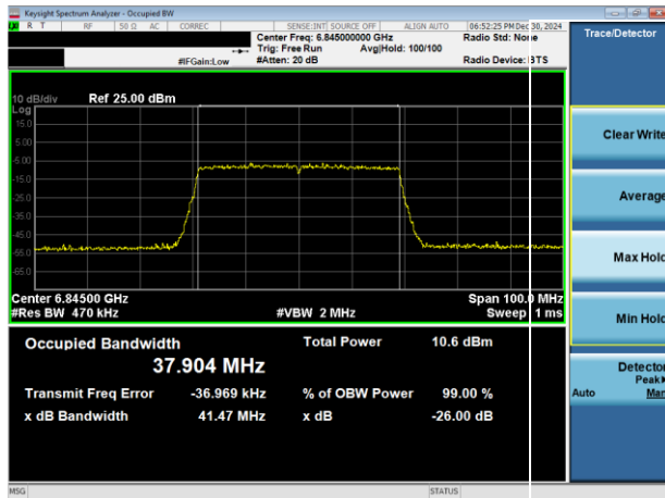
Plot 7-43. 26dB & 99% Bandwidth Plot Antenna 1b (40MHz 802.11ax RU484 (UNII Band 7) – Ch. 179)
