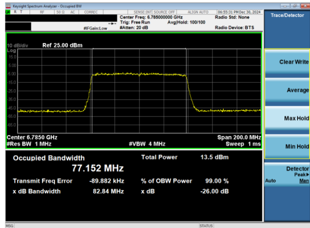
Plot 7-44. 26dB & 99% Bandwidth Plot Antenna 1b (80MHz 802.11ax RU996 (UNII Band 7) – Ch. 167)
