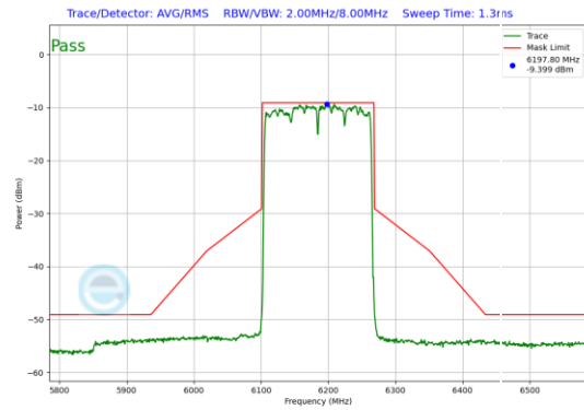
Plot 7-133. In-Band Emission Plot SDM Diversity Antenna 5T (160MHz 802.11ax (UNII Band 5) – Ch. 47)
