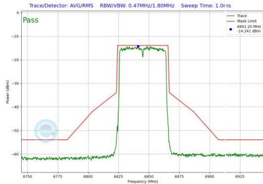
Plot 7-98. In-Band Emission Plot Antenna 3b (40MHz 802.11ax (UNII Band 7) – Ch. 179)
