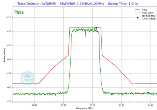
Plot 7-111. In-Band Emission Plot SDM Primary Antenna 5T (20MHz 802.11ax (UNII Band 5) – Ch. 33)
