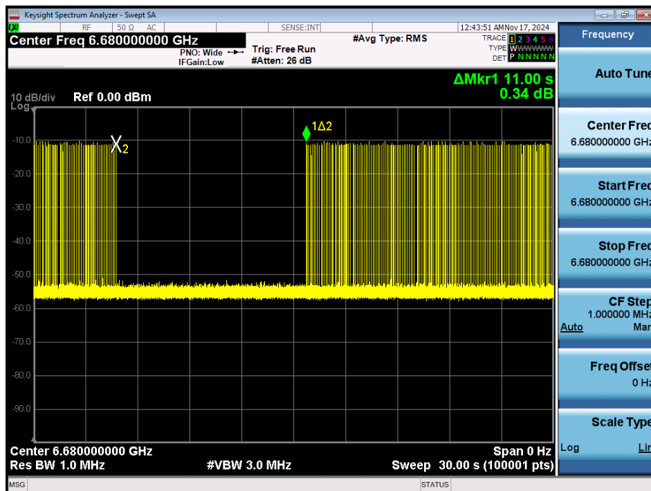
Plot 7-158. Contention Based Protocol Timing Plot – UNII 7 – 160MHz Channel 143 – High
