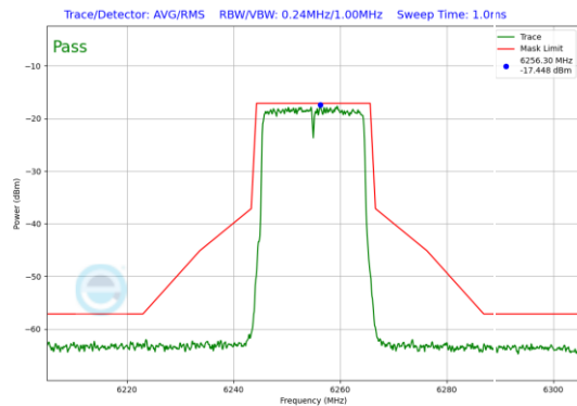
Plot 7-102. In-Band Emission Plot Antenna 1b (20MHz 802.11ax (UNII Band 5) – Ch. 61)
