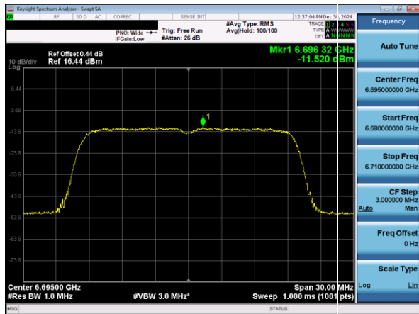
Plot 7-73. Power Spectral Density Plot SDM Diversity Antenna 5T (20MHz 802.11ax (UNII Band 7) – Ch. 149)
