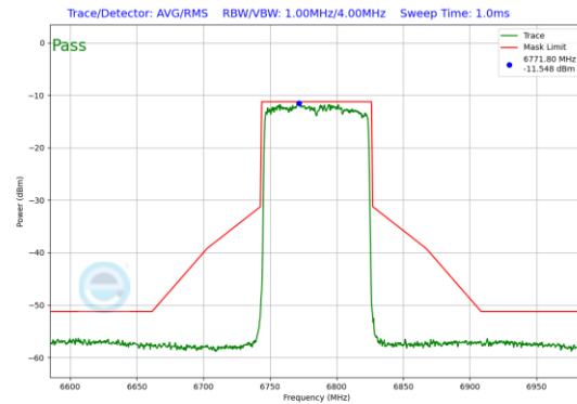
Plot 7-89. In-Band Emission Plot Antenna 5T (80MHz 802.11ax (UNII Band 7) – Ch. 167)
