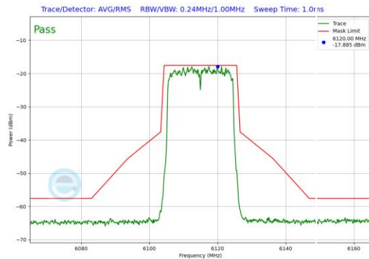
Plot 7-112. In-Band Emission Plot SDM Primary Antenna 3b (20MHz 802.11ax (UNII Band 5) – Ch. 33)
