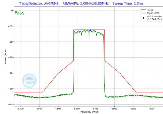
Plot 7-142. In-Band Emission Plot SDM Diversity Antenna 1b (160MHz 802.11ax (UNII Band 7) – Ch. 143)
