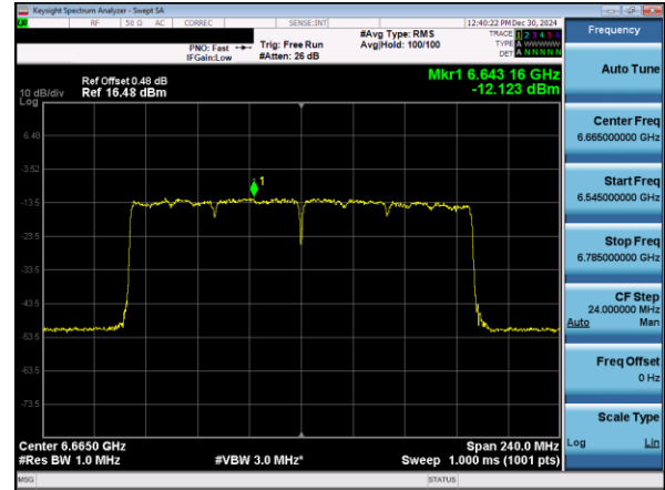
Plot 7-79. Power Spectral Density Plot SDM Diversity Antenna 5T (160MHz 802.11ax (UNII Band 7) – Ch. 143)
