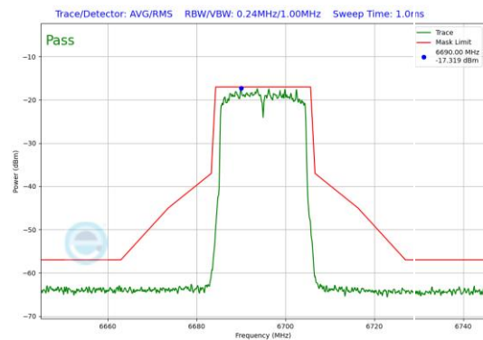
Plot 7-135. In-Band Emission Plot SDM Diversity Antenna 5T (20MHz 802.11ax (UNII Band 7) – Ch. 149)
