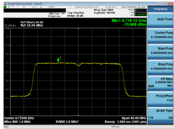
Plot 7-76. Power Spectral Density Plot SDM Diversity Antenna 1b (40MHz 802.11ax (UNII Band 7) – Ch. 155)
