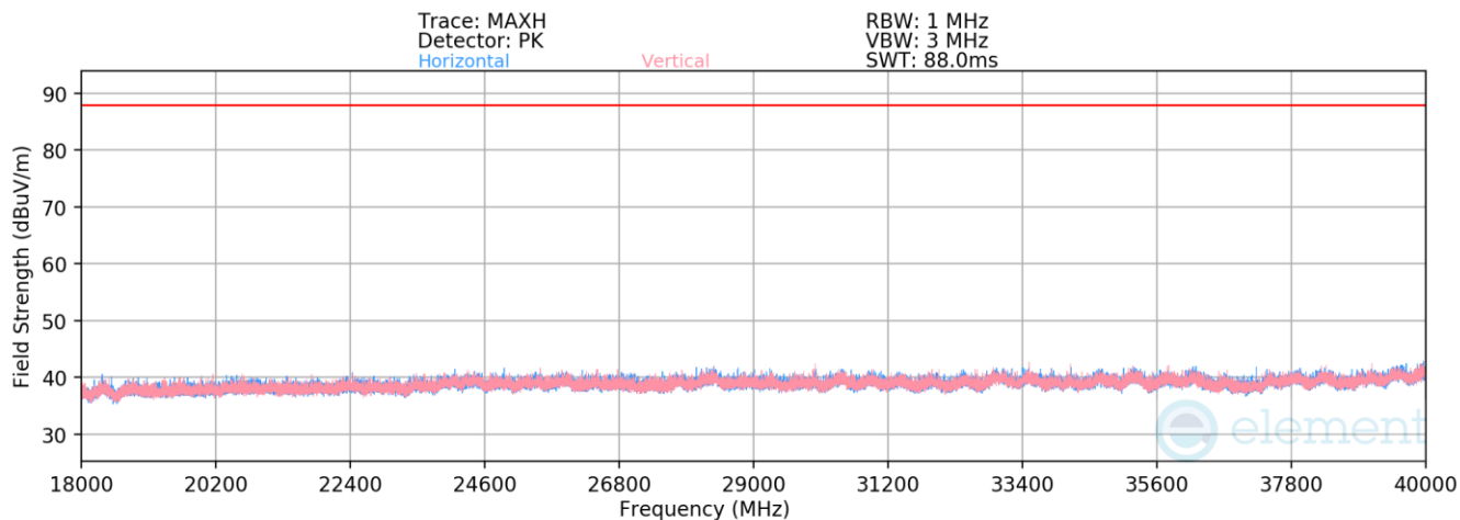
Plot 7-166. Radiated Spurious Emissions 18-40GHz SDM Primary (802.11ax – Ch. 33)
