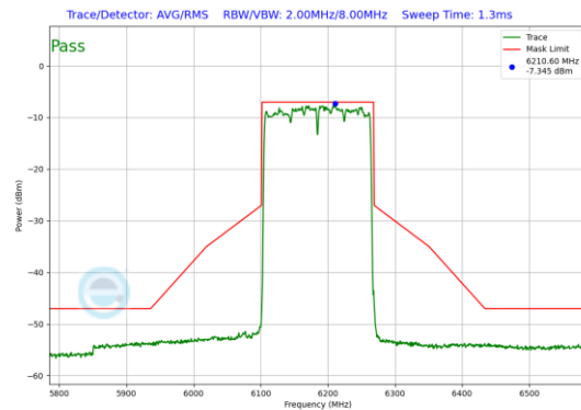
Plot 7-85. In-Band Emission Plot Antenna 5T (160MHz 802.11ax (UNII Band 5) – Ch. 47)
