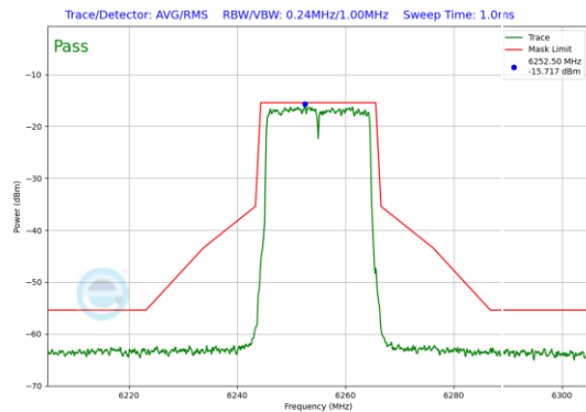
Plot 7-92. In-Band Emission Plot Antenna 3b (20MHz 802.11ax (UNII Band 5) – Ch. 61)
