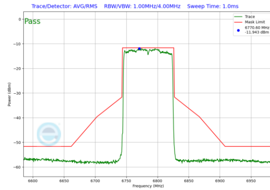
Plot 7-99. In-Band Emission Plot Antenna 3b (80MHz 802.11ax (UNII Band 7) – Ch. 167)
