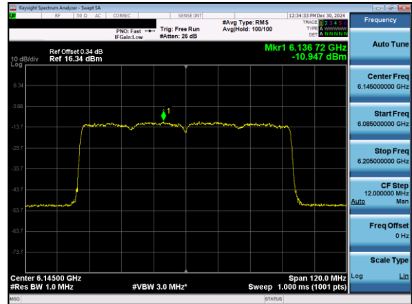
Plot 7-69. Power Spectral Density Plot SDM Diversity Antenna 5T (80MHz 802.11ax (UNII Band 5) – Ch. 39)
