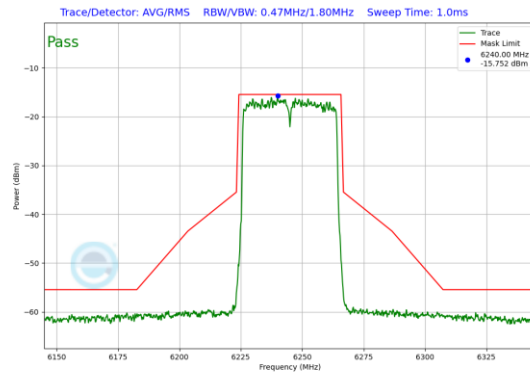
Plot 7-130. In-Band Emission Plot SDM Diversity Antenna 1b (40MHz 802.11ax (UNII Band 5) – Ch. 59)
