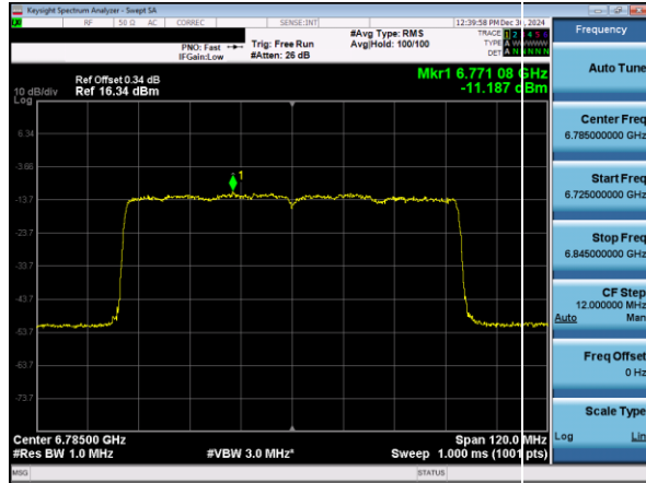
Plot 7-77. Power Spectral Density Plot SDM Diversity Antenna 5T (80MHz 802.11ax (UNII Band 7) – Ch. 167)
