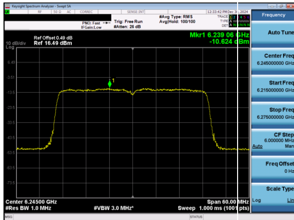
Plot 7-67. Power Spectral Density Plot SDM Diversity Antenna 5T (40MHz 802.11ax (UNII Band 5) – Ch. 59)
