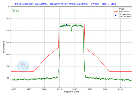
Plot 7-113. In-Band Emission Plot SDM Primary Antenna 5T (40MHz 802.11ax (UNII Band 5) – Ch. 59)
