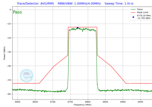
Plot 7-123. In-Band Emission Plot SDM Primary Antenna 5T (80MHz 802.11ax (UNII Band 7) – Ch. 167)
