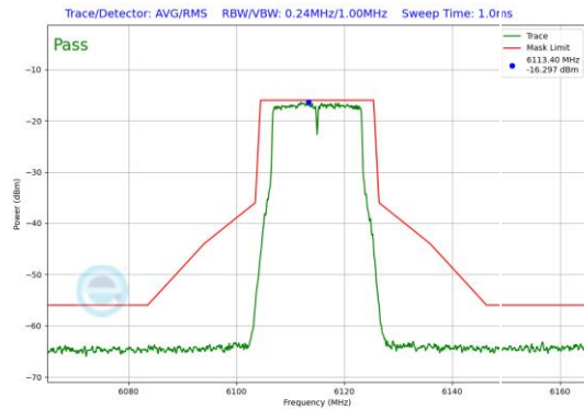
Plot 7-91. In-Band Emission Plot Antenna 3b (20MHz 802.11a (UNII Band 5) – Ch. 33)
