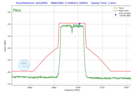
Plot 7-136. In-Band Emission Plot SDM Diversity Antenna 1b (20MHz 802.11ax (UNII Band 7) – Ch. 149)
