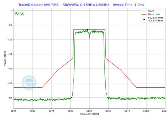
Plot 7-83. In-Band Emission Plot Antenna 5T (40MHz 802.11ax (UNII Band 5) – Ch. 35)
