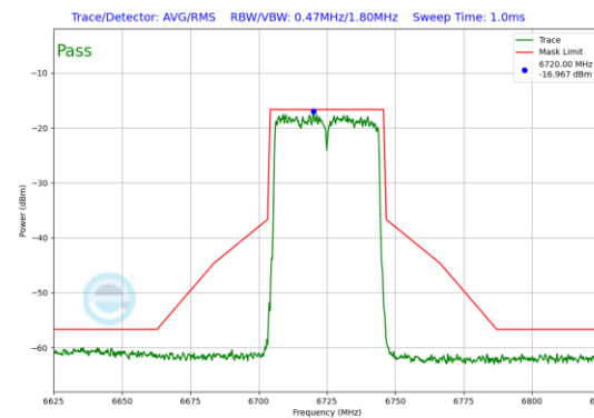
Plot 7-138. In-Band Emission Plot SDM Diversity Antenna 1b (40MHz 802.11ax (UNII Band 7) – Ch. 155)
