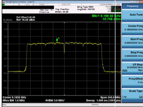
Plot 7-71. Power Spectral Density Plot SDM Diversity Antenna 5T (160MHz 802.11ax (UNII Band 5) – Ch. 47)
