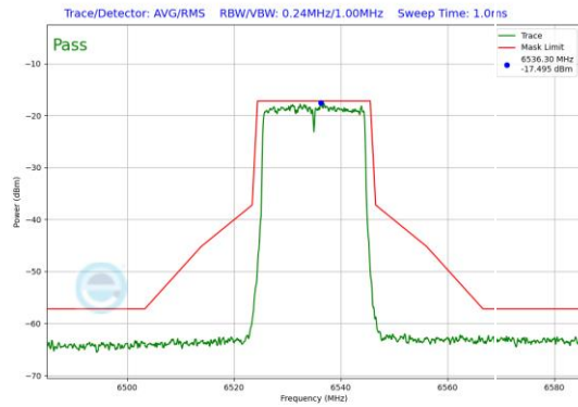
Plot 7-97. In-Band Emission Plot Antenna 3b (20MHz 802.11ax (UNII Band 7) – Ch. 117)
