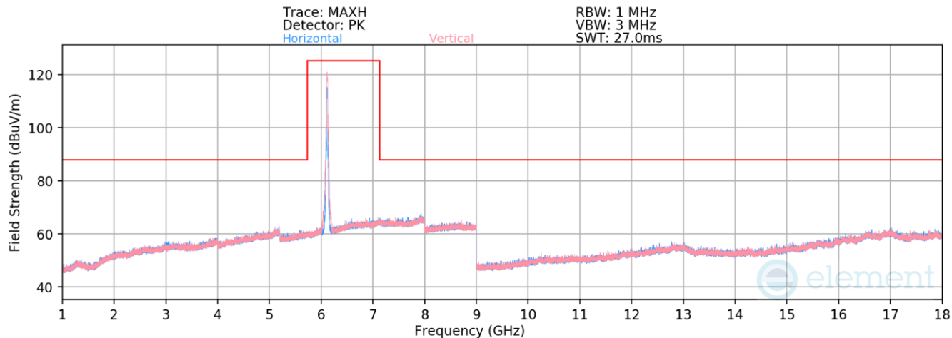
Plot 7-165. Radiated Spurious Emissions 1-18GHz SDM Primary (802.11ax – Ch. 33)
