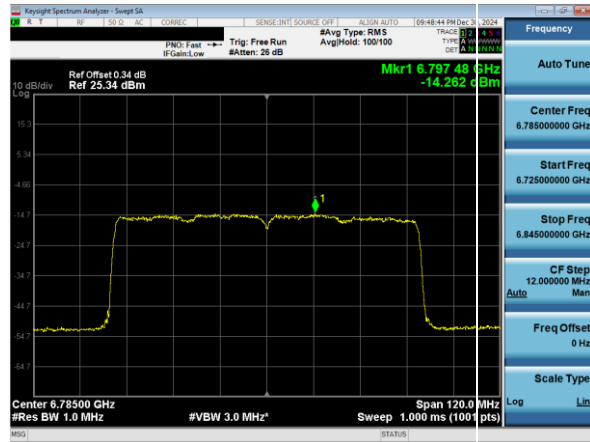
Plot 7-78. Power Spectral Density Plot SDM Diversity Antenna 1b (80MHz 802.11ax (UNII Band 7) – Ch. 167)
