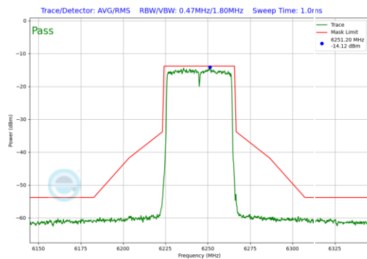
Plot 7-103. In-Band Emission Plot Antenna 1b (40MHz 802.11ax (UNII Band 5) – Ch. 59)
