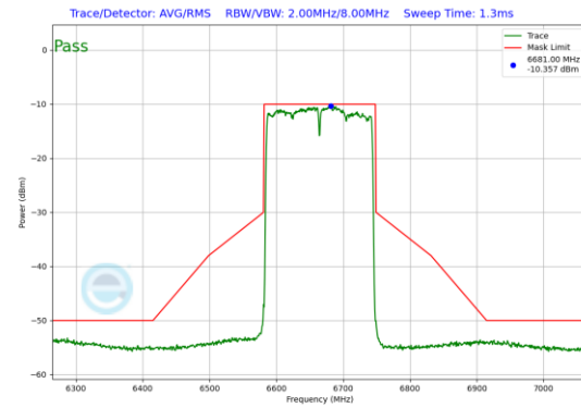
Plot 7-125. In-Band Emission Plot SDM Primary Antenna 5T (160MHz 802.11ax (UNII Band 7) – Ch. 143)
