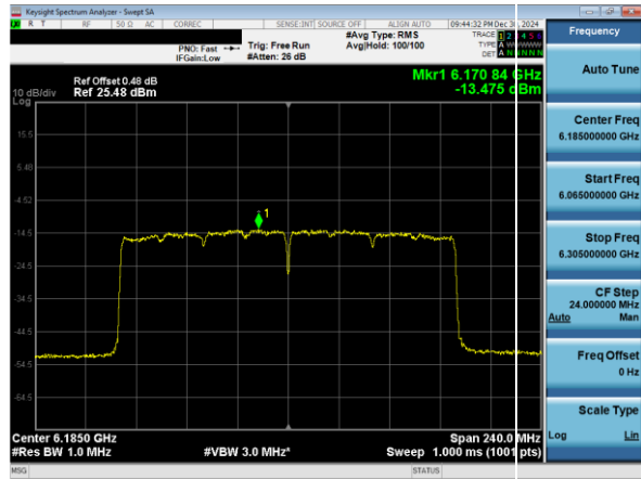
Plot 7-72. Power Spectral Density Plot SDM Diversity Antenna 1b (160MHz 802.11ax (UNII Band 5) – Ch. 47)
