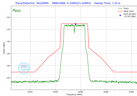
Plot 7-81. In-Band Emission Plot Antenna 5T (20MHz 802.11a (UNII Band 5) – Ch. 61)
