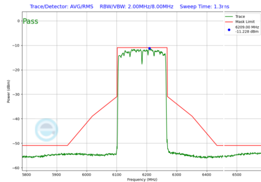
Plot 7-134. In-Band Emission Plot SDM Diversity Antenna 1b (160MHz 802.11ax (UNII Band 5) – Ch. 47)
