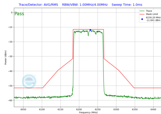
Plot 7-116. In-Band Emission Plot SDM Primary Antenna 3b (80MHz 802.11ax (UNII Band 5) – Ch. 55)
