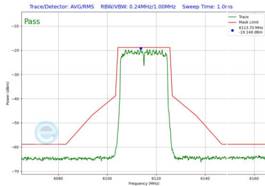
Plot 7-128. In-Band Emission Plot SDM Diversity Antenna 1b (20MHz 802.11ax (UNII Band 5) – Ch. 33)
