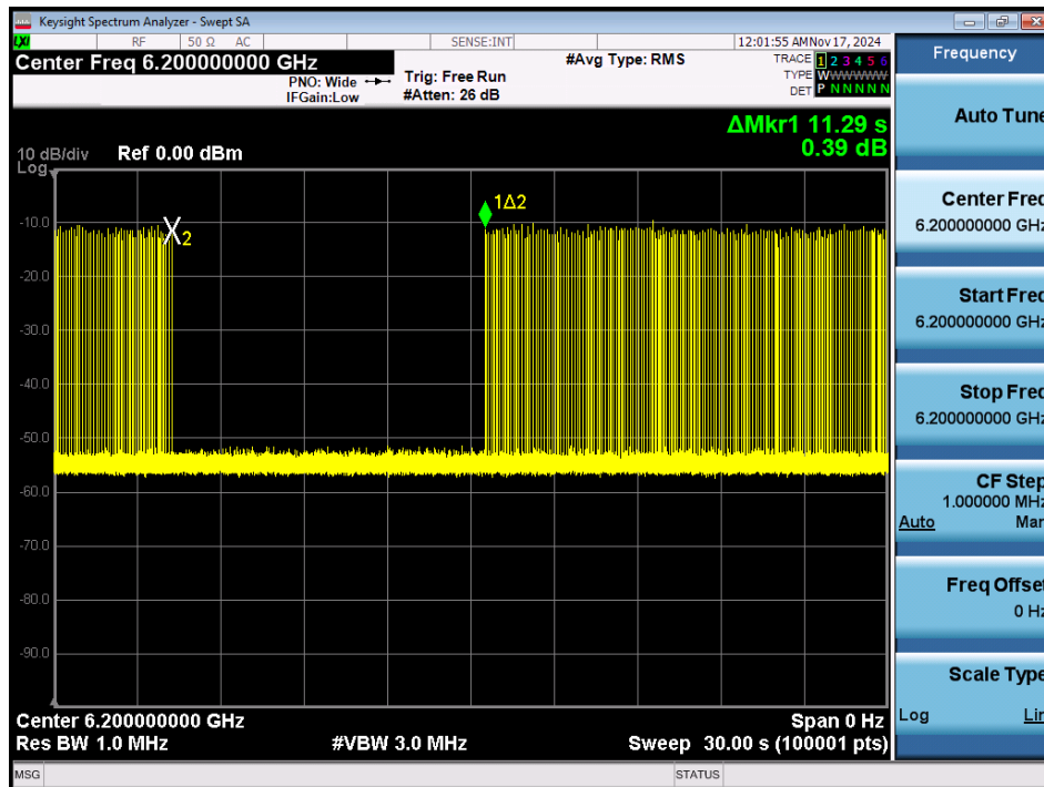
Plot 7-154. Contention Based Protocol Timing Plot – UNII 5 – 160MHz Channel 47 – High
