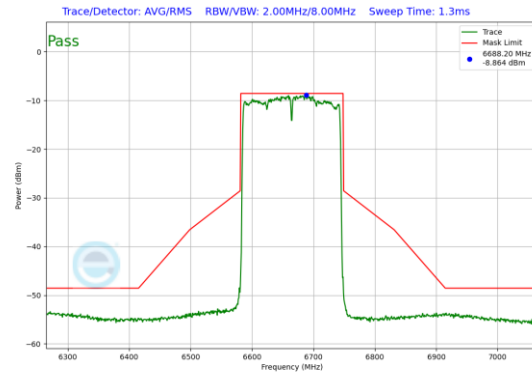
Plot 7-90. In-Band Emission Plot Antenna 5T (160MHz 802.11ax (UNII Band 7) – Ch. 143)
