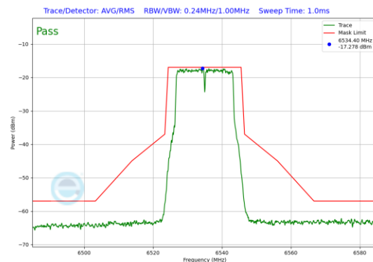
Plot 7-96. In-Band Emission Plot Antenna 3b (20MHz 802.11a (UNII Band 7) – Ch. 117)
