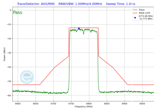
Plot 7-124. In-Band Emission Plot SDM Primary Antenna 3b (80MHz 802.11ax (UNII Band 7) – Ch. 167)
