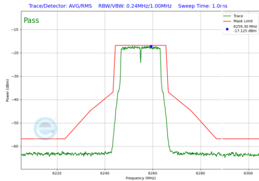
Plot 7-101. In-Band Emission Plot Antenna 1b (20MHz 802.11a (UNII Band 5) – Ch. 61)
