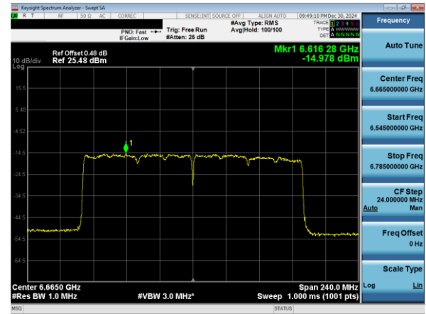
Plot 7-80. Power Spectral Density Plot SDM Diversity Antenna 1b (160MHz 802.11ax (UNII Band 7) – Ch. 143)
