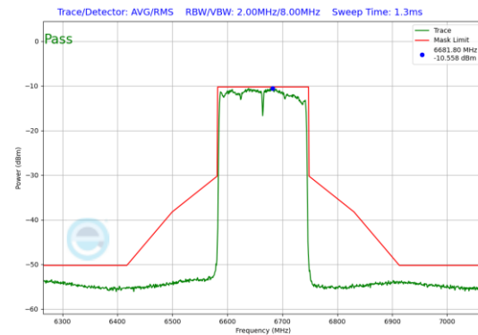
Plot 7-126. In-Band Emission Plot SDM Primary Antenna 3b (160MHz 802.11ax (UNII Band 7) – Ch. 143)
