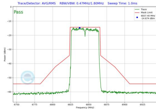
Plot 7-121. In-Band Emission Plot SDM Primary Antenna 5T (40MHz 802.11ax (UNII Band 7) – Ch. 179)
