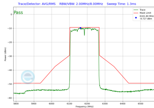
Plot 7-105. In-Band Emission Plot Antenna 1b (160MHz 802.11ax (UNII Band 5) – Ch. 47)
