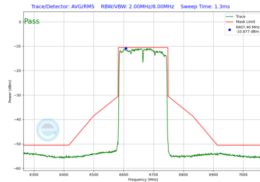
Plot 7-110. In-Band Emission Plot Antenna 1b (160MHz 802.11ax (UNII Band 7) – Ch. 143)
