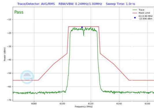
Plot 7-82. In-Band Emission Plot Antenna 5T (20MHz 802.11ax (UNII Band 5) – Ch. 33)
