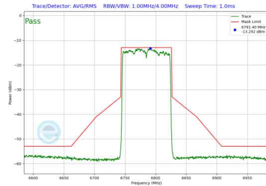
Plot 7-109. In-Band Emission Plot Antenna 1b (80MHz 802.11ax (UNII Band 7) – Ch. 167)
