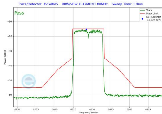
Plot 7-122. In-Band Emission Plot SDM Primary Antenna 3b (40MHz 802.11ax (UNII Band 7) – Ch. 179)
