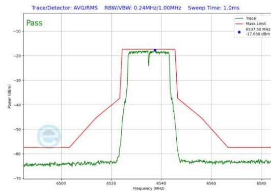
Plot 7-106. In-Band Emission Plot Antenna 1b (20MHz 802.11a (UNII Band 7) – Ch. 117)
