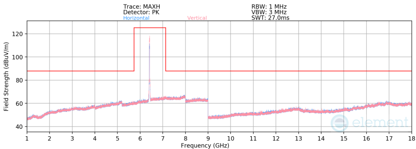
Plot 7-168. Radiated Spurious Emissions 1-18GHz SDM Primary (802.11ax – Ch. 93)
