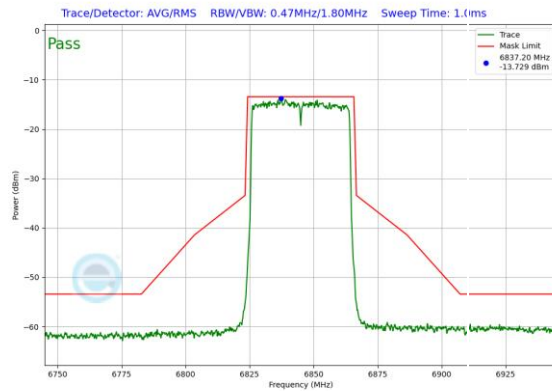
Plot 7-88. In-Band Emission Plot Antenna 5T (40MHz 802.11ax (UNII Band 7) – Ch. 179)
