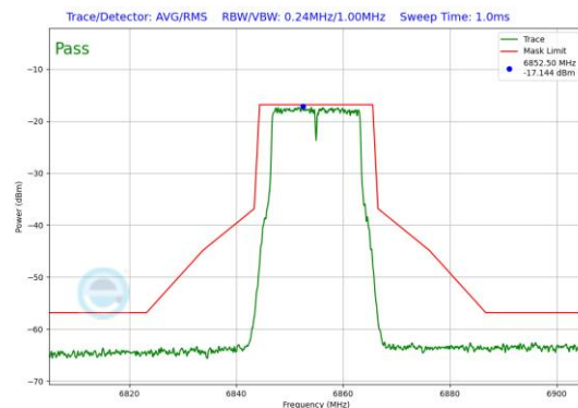
Plot 7-86. In-Band Emission Plot Antenna 5T (20MHz 802.11a (UNII Band 7) – Ch. 181)
