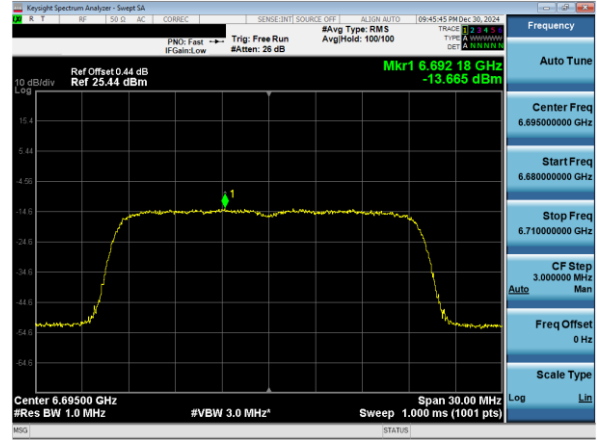
Plot 7-74. Power Spectral Density Plot SDM Diversity Antenna 1b (20MHz 802.11ax (UNII Band 7) – Ch. 149)
