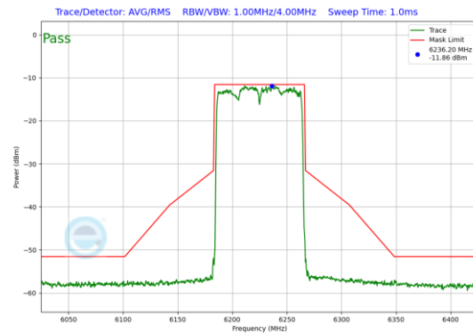
Plot 7-115. In-Band Emission Plot SDM Primary Antenna 5T (80MHz 802.11ax (UNII Band 5) – Ch. 55)
