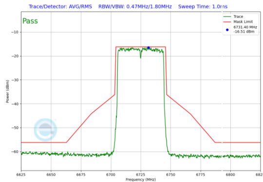
Plot 7-108. In-Band Emission Plot Antenna 1b (40MHz 802.11ax (UNII Band 7) – Ch. 155)
