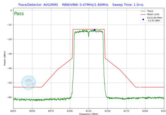
Plot 7-93. In-Band Emission Plot Antenna 3b (40MHz 802.11ax (UNII Band 5) – Ch. 35)
