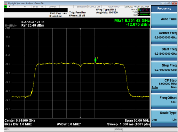
Plot 7-68. Power Spectral Density Plot SDM Diversity Antenna 1b (40MHz 802.11ax (UNII Band 5) – Ch. 59)
