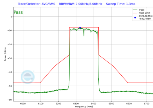
Plot 7-95. In-Band Emission Plot Antenna 3b (160MHz 802.11ax (UNII Band 5) – Ch. 79)
