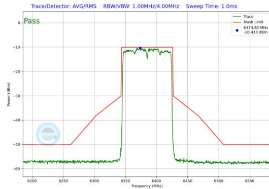
Plot 7-84. In-Band Emission Plot Antenna 5T (80MHz 802.11ax (UNII Band 5) – Ch. 87)
