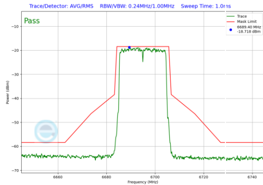
Plot 7-107. In-Band Emission Plot Antenna 1b (20MHz 802.11ax (UNII Band 7) – Ch. 149)
