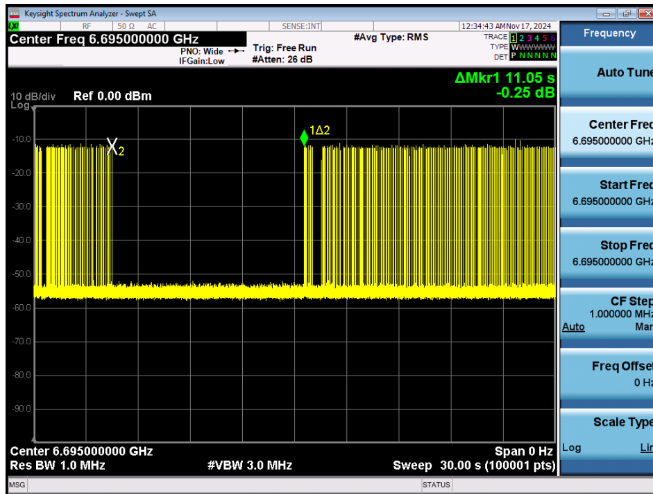
Plot 7-155. Contention Based Protocol Timing Plot – UNII 7 – 20MHz Channel 149
