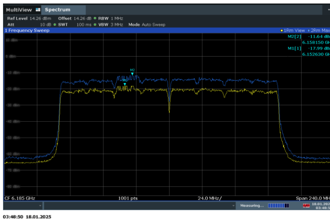
Plot 7-163. 160MHz Bandwidth – 6185MHz Antenna 5T
