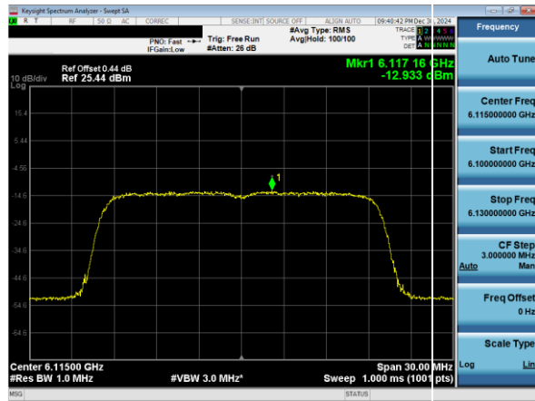
Plot 7-66. Power Spectral Density Plot SDM Diversity Antenna 1b (20MHz 802.11ax (UNII Band 5) – Ch. 33)
