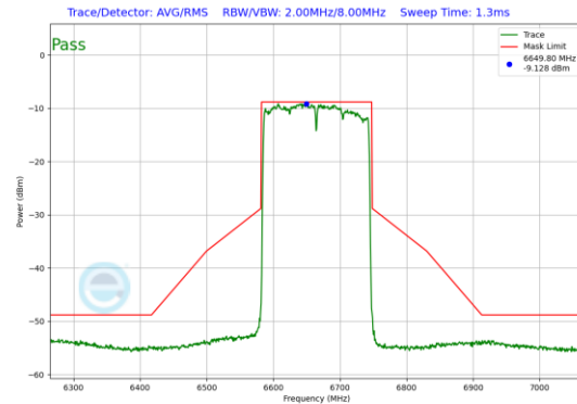
Plot 7-100. In-Band Emission Plot Antenna 3b (160MHz 802.11ax (UNII Band 7) – Ch. 143)
