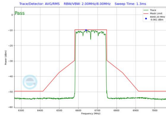
Plot 7-141. In-Band Emission Plot SDM Diversity Antenna 5T (160MHz 802.11ax (UNII Band 7) – Ch. 143)
