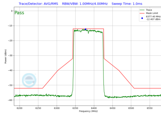
Plot 7-104. In-Band Emission Plot Antenna 1b (80MHz 802.11ax (UNII Band 5) – Ch. 87)
