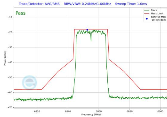
Plot 7-120. In-Band Emission Plot SDM Primary Antenna 3b (20MHz 802.11ax (UNII Band 7) – Ch. 181)
