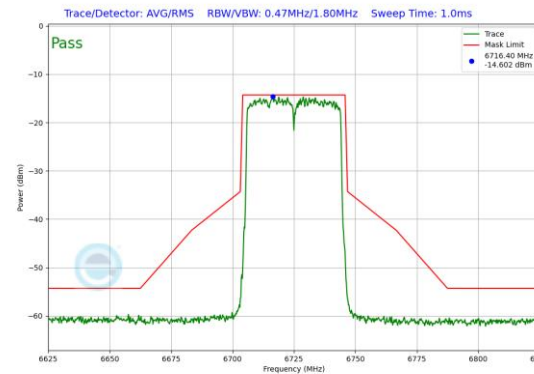
Plot 7-137. In-Band Emission Plot SDM Diversity Antenna 5T (40MHz 802.11ax (UNII Band 7) – Ch. 155)
