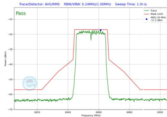
Plot 7-119. In-Band Emission Plot SDM Primary Antenna 5T (20MHz 802.11ax (UNII Band 7) – Ch. 181)
