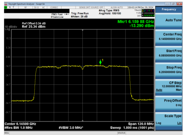
Plot 7-70. Power Spectral Density Plot SDM Diversity Antenna 1b (80MHz 802.11ax (UNII Band 5) – Ch. 39)
