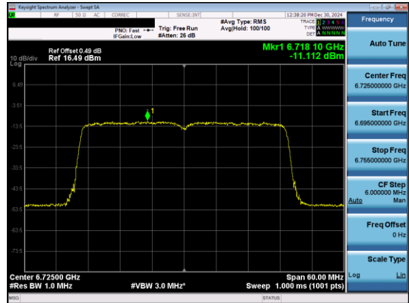
Plot 7-75. Power Spectral Density Plot SDM Diversity Antenna 5T (40MHz 802.11ax (UNII Band 7) – Ch. 155)
