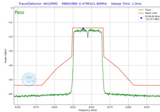
Plot 7-114. In-Band Emission Plot SDM Primary Antenna 3b (40MHz 802.11ax (UNII Band 5) – Ch. 59)
