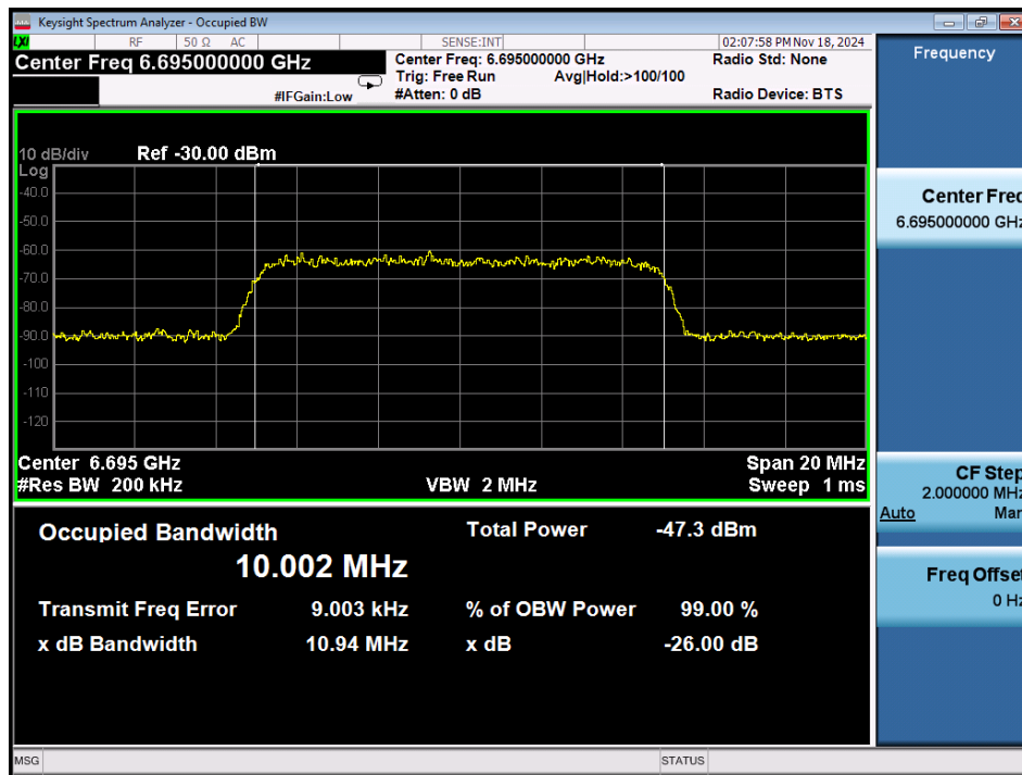
Plot 7-147. AWGN Signal – UNII 7 – 20MHz
