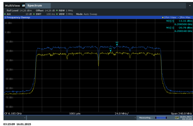
Plot 7-164. 160MHz Bandwidth – 6185MHz Antenna 3b
