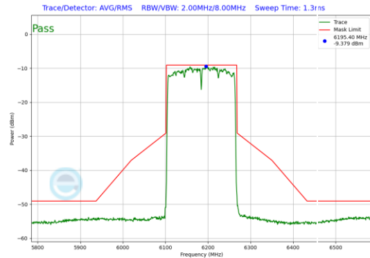
Plot 7-118. In-Band Emission Plot SDM Primary Antenna 3b (160MHz 802.11ax (UNII Band 5) – Ch. 47)
