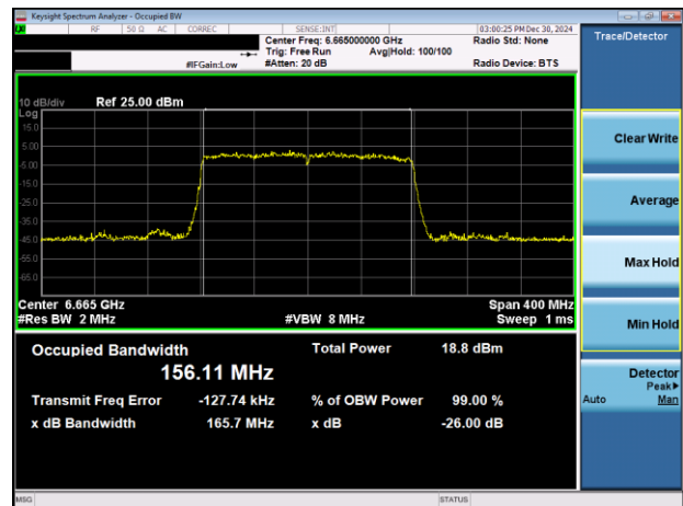
Plot 7-16. 26dB & 99% Bandwidth Plot Antenna 3b (160MHz) 802.11ax (UNII Band 7) – Ch. 143)
