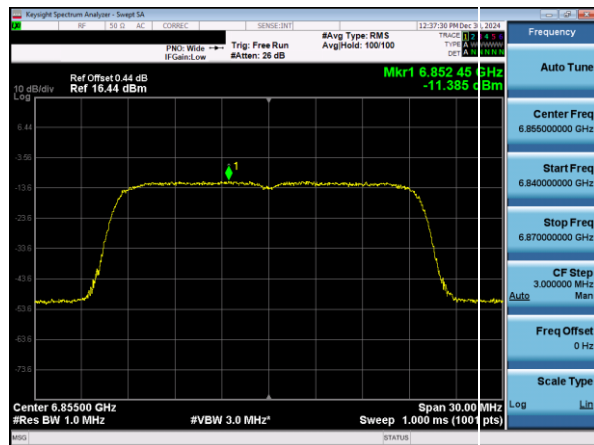
Plot 7-57. Power Spectral Density Plot SDM Primary Antenna 5T (20MHz 802.11ax (UNII Band 7) – Ch. 181)
