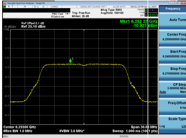
Plot 7-41. PSD Plot Antenna 1b (20MHz 802.11a (UNII Band 5) – Ch. 61)
