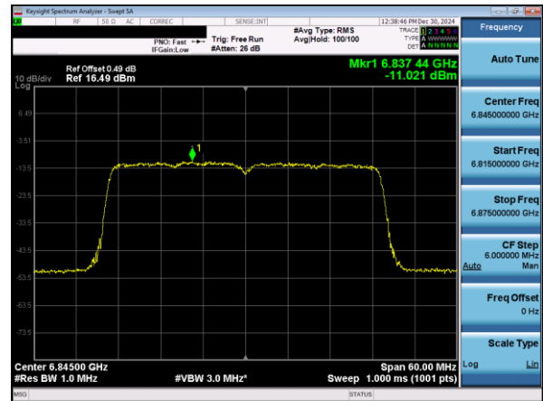
Plot 7-59. Power Spectral Density Plot SDM Primary Antenna 5T (40MHz 802.11ax (UNII Band 7) – Ch. 179)
