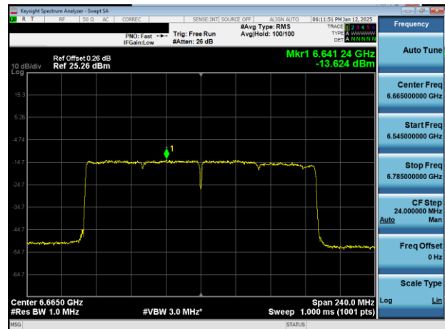
Plot 7-48. PSD Plot Antenna 1b (160MHz 802.11ax (UNII Band 7) – Ch. 143)
