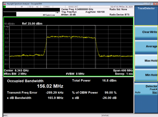
Plot 7-12. 26dB & 99% Bandwidth Plot Antenna 3b (160MHz 802.11ax (UNII Band 5) – Ch. 79)
