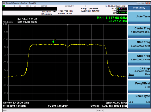
Plot 7-26. PSD Plot Antenna 5T (40MHz 802.11ax (UNII Band 5) – Ch. 35)
