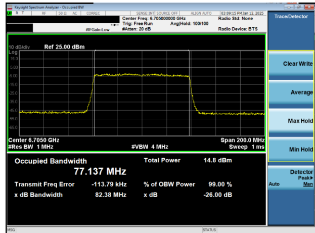
Plot 7-15. 26dB & 99% Bandwidth Plot Antenna 3b (80MHz) 802.11ax (UNII Band 7) – Ch. 151)
