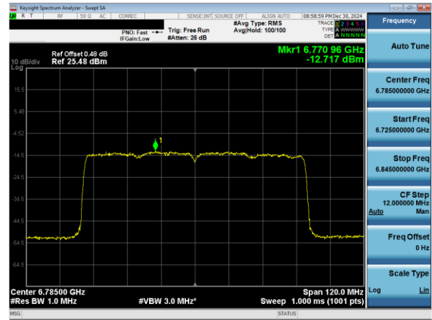
Plot 7-47. PSD Plot Antenna 1b (80MHz 802.11ax (UNII Band 7) – Ch. 167)
