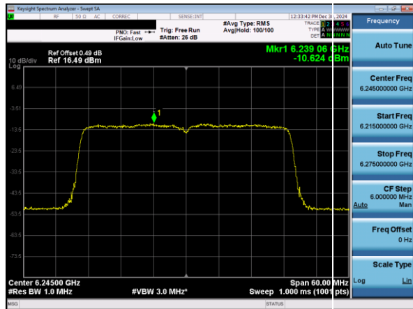
Plot 7-51. Power Spectral Density Plot SDM Primary Antenna 5T (40MHz 802.11ax (UNII Band 5) – Ch. 59)
