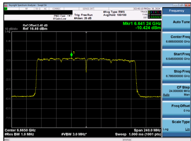
Plot 7-40. PSD Plot Antenna 3b (160MHz 802.11ax (UNII Band 7) - Ch. 143)
