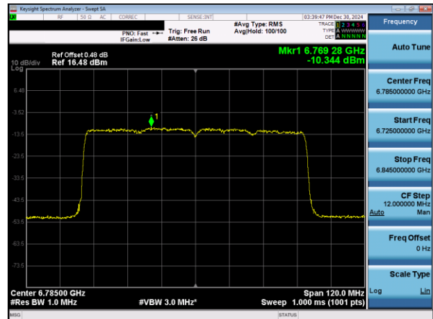
Plot 7-39. PSD Plot Antenna 3b (80MHz 802.11ax (UNII Band 7) - Ch. 167)
