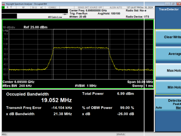
Plot 7-21. 26dB & 99% Bandwidth Plot Antenna 1b (20MHz 802.11ax (UNII Band 7) – Ch. 149)
