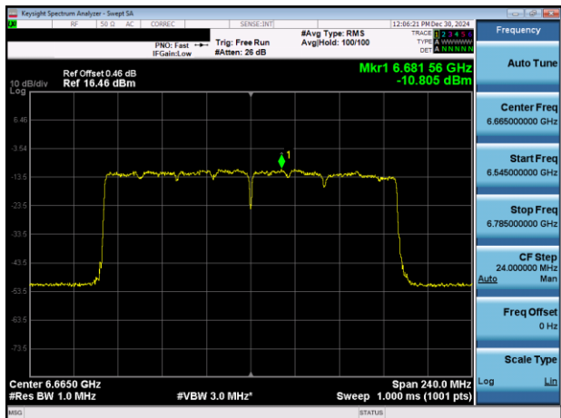
Plot 7-32. PSD Plot Antenna 5T (160MHz 802.11ax (UNII Band 7) – Ch. 143)
