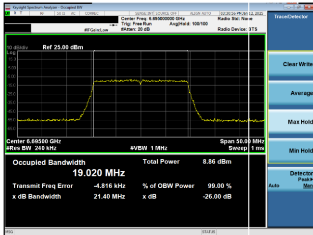
Plot 7-13. 26dB & 99% Bandwidth Plot Antenna 3b (20MHz) 802.11ax (UNII Band 7) – Ch. 149)
