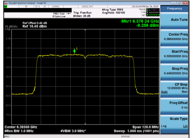
Plot 7-35. PSD Plot Antenna 3b (80MHz 802.11ax (UNII Band 5) – Ch. 87)
