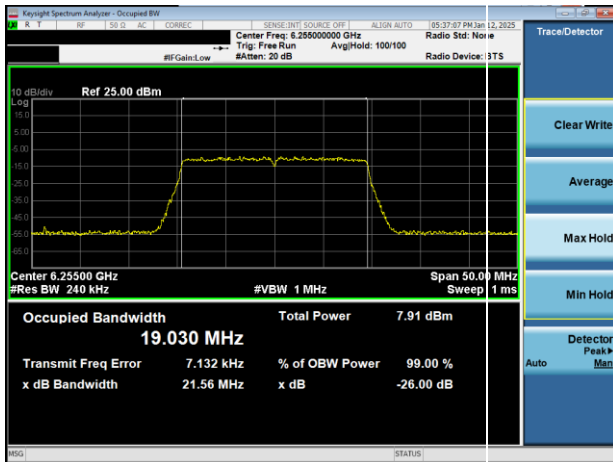
Plot 7-17. 26dB & 99% Bandwidth Plot Antenna 1b (20MHz 802.11ax (UNII Band 5) – Ch. 61)
