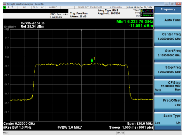
Plot 7-54. Power Spectral Density Plot SDM Primary Antenna 3b (80MHz 802.11ax (UNII Band 5) – Ch. 55)
