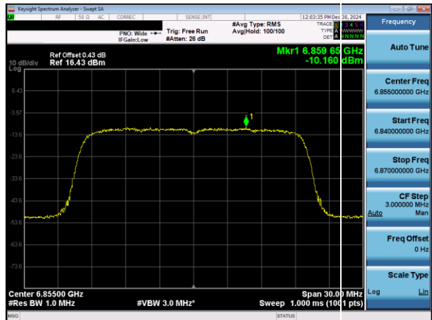
Plot 7-29. PSD Plot Antenna 5T (20MHz 802.11a (UNII Band 7) – Ch. 181)– Ch. 181)
