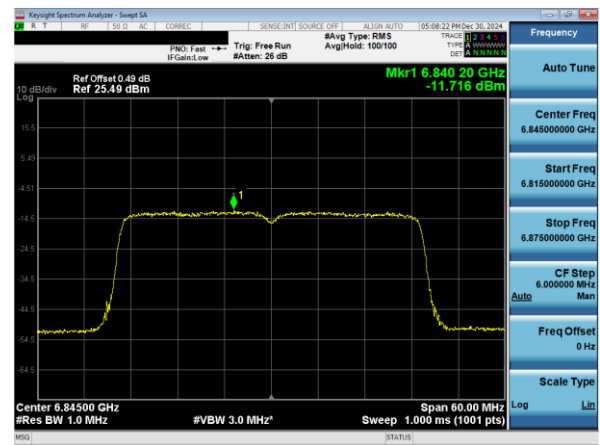
Plot 7-60. Power Spectral Density Plot SDM Primary Antenna 3b (40MHz 802.11ax (UNII Band 7) – Ch. 179)
