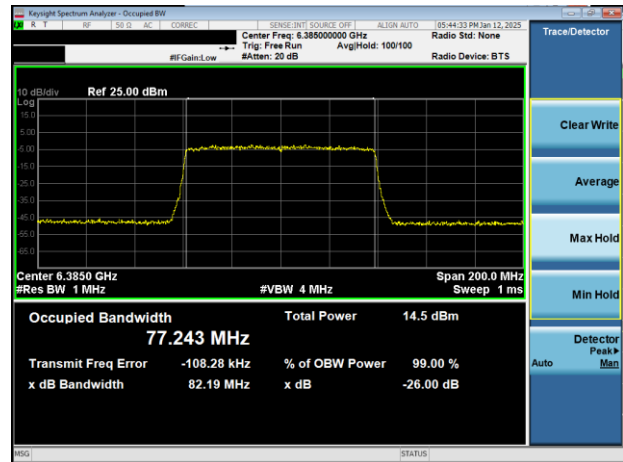
Plot 7-19. 26dB & 99% Bandwidth Plot Antenna 1b (80MHz 802.11ax (UNII Band 5) – Ch. 87)
