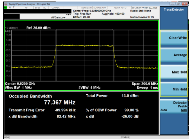
Plot 7-23. 26dB & 99% Bandwidth Plot Antenna 1b (80MHz 802.11ax (UNII Band 7) – Ch. 135)
