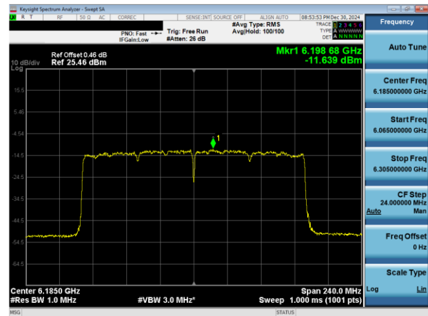
Plot 7-44. PSD Plot Antenna 1b (160MHz 802.11ax (UNII Band 5) Ch. 47)
