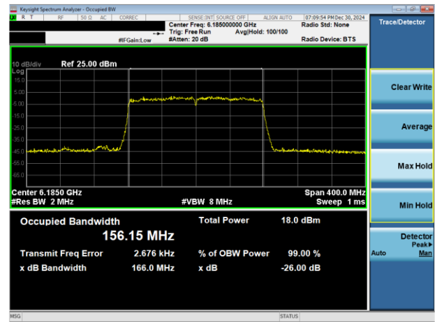
Plot 7-20. 26dB & 99% Bandwidth Plot Antenna 1b (160MHz 802.11ax (UNII Band 5) – Ch. 47)
