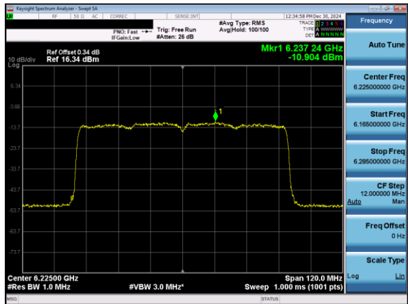
Plot 7-53. Power Spectral Density Plot SDM Primary Antenna 5T (80MHz 802.11ax (UNII Band 5) – Ch. 55)
