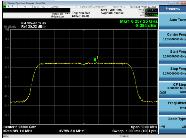
Plot 7-33. PSD Plot Antenna 3b (20MHz 802.11a (UNII Band 5) – Ch. 61)
