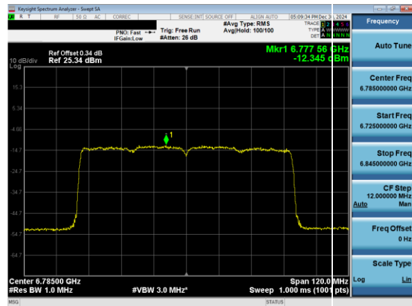
Plot 7-62. Power Spectral Density Plot SDM Primary Antenna 3b (80MHz 802.11ax (UNII Band 7) – Ch. 167)
