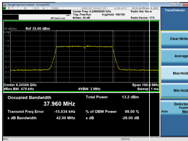
Plot 7-10. 26dB & 99% Bandwidth Plot Antenna 3b (40MHz 802.11ax (UNII Band 5) – Ch. 59)
