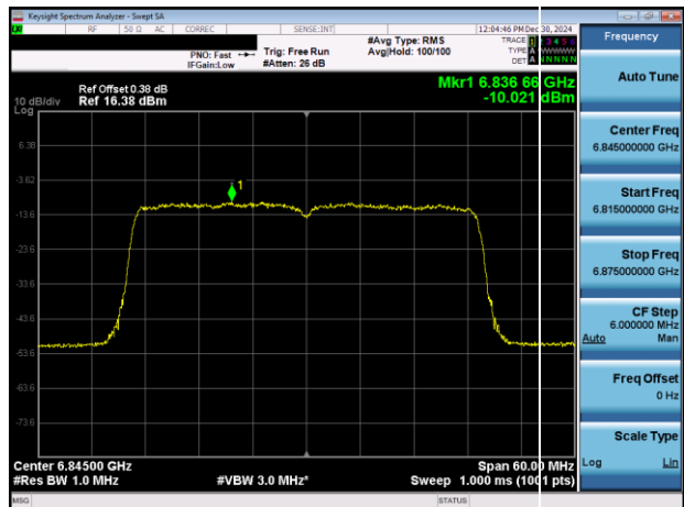
Plot 7-30. PSD Plot Antenna 5T (40MHz 802.11ax (UNII Band 7) – Ch. 179)
