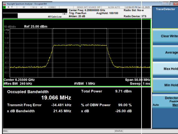
Plot 7-1. 26dB & 99% Bandwidth Plot Antenna 5T (20MHz 802.11ax (UNII Band 5) – Ch. 61)
