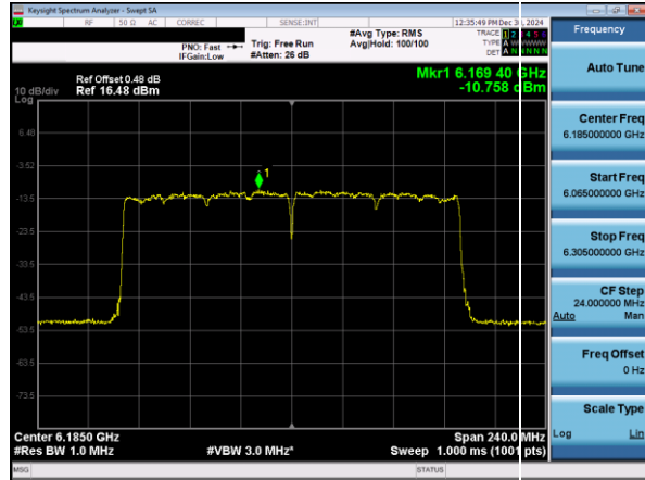
Plot 7-55. Power Spectral Density Plot SDM Primary Antenna 5T (160MHz 802.11ax (UNII Band 5) – Ch. 47)
