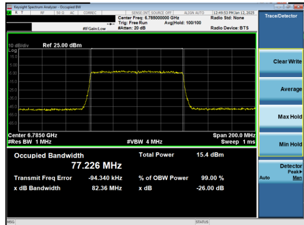
Plot 7-7. 26dB & 99% Bandwidth Plot Antenna 5T (80MHz 802.11ax (UNII Band 7) – Ch. 167)
