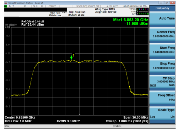
Plot 7-58. Power Spectral Density Plot SDM Primary Antenna 3b (20MHz 802.11ax (UNII Band 7) – Ch. 181)
