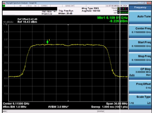
Plot 7-25. PSD Plot Antenna 5T (20MHz 802.11ax (UNII Band 5) – Ch. 33)
