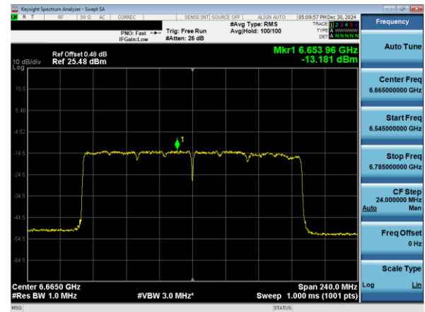
Plot 7-64. Power Spectral Density Plot SDM Primary Antenna 3b (160MHz 802.11ax (UNII Band 7) – Ch. 143)
