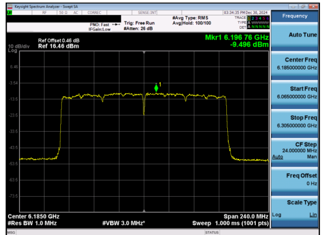
Plot 7-36. PSD Plot Antenna 3b (160MHz 802.11ax (UNII Band 5) – Ch. 47)
