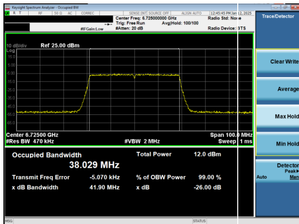
Plot 7-6. 26dB & 99% Bandwidth Plot Antenna 5T (40MHz 802.11ax (UNII Band 7) – Ch. 155)
