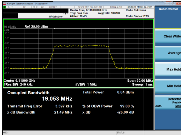
Plot 7-9. 26dB & 99% Bandwidth Plot Antenna 3b (20MHz 802.11ax (UNII Band 5) – Ch. 33)
