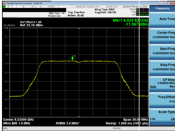
Plot 7-45. PSD Plot Antenna 1b (20MHz 802.11ax (UNII Band 7) – Ch. 117)
