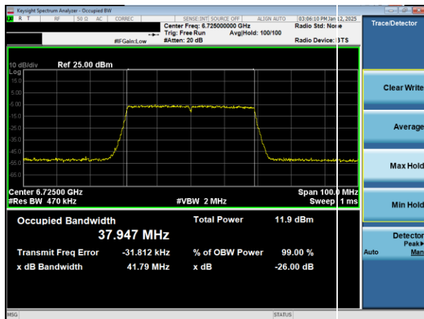
Plot 7-14. 26dB & 99% Bandwidth Plot Antenna 3b (40MHz) 802.11ax (UNII Band 7) – Ch. 155)
