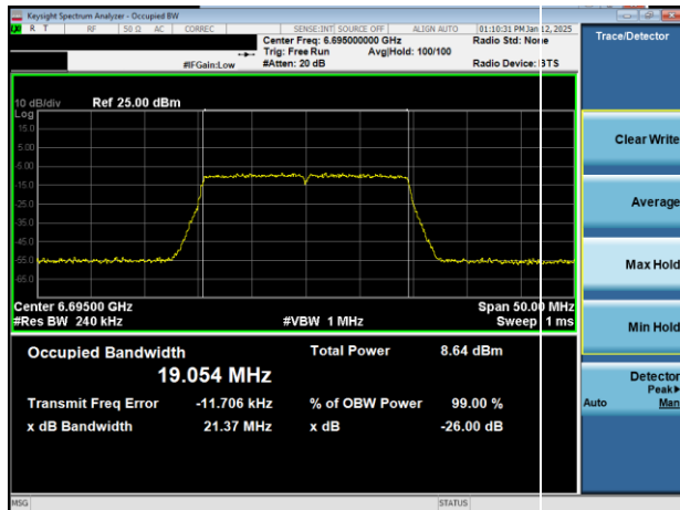
Plot 7-5. 26dB & 99% Bandwidth Plot Antenna 5T (20MHz 802.11ax (UNII Band 7) – Ch. 149)
