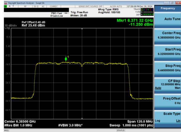
Plot 7-43. PSD Plot Antenna 1b (80MHz 802.11ax (UNII Band 5) – Ch. 87)
