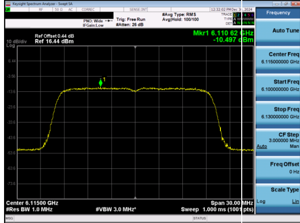
Plot 7-49. Power Spectral Density Plot SDM Primary Antenna 5T (20MHz 802.11ax (UNII Band 5) – Ch.33)
