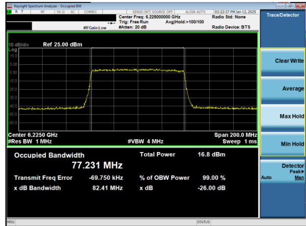
Plot 7-11. 26dB & 99% Bandwidth Plot Antenna 3b (80MHz 802.11ax (UNII Band 5) – Ch. 55)
