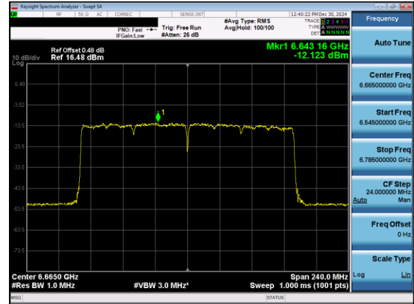
Plot 7-63. Power Spectral Density Plot SDM Primary Antenna 5T (160MHz 802.11ax (UNII Band 7) – Ch. 143)
