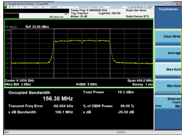
Plot 7-4. 26dB & 99% Bandwidth Plot Antenna 5T (160MHz 802.11ax (UNII Band 5) – Ch. 47)
