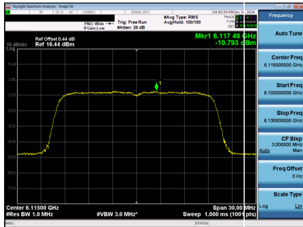
Plot 7-50. Power Spectral Density Plot SDM Primary Antenna 3b (20MHz 802.11ax (UNII Band 5) – Ch.33)
