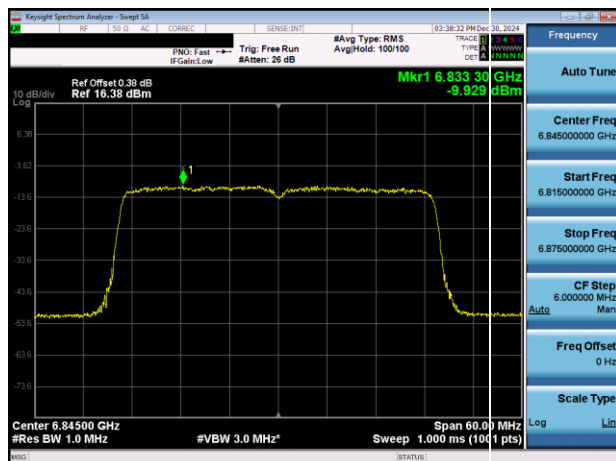
Plot 7-38. PSD Plot Antenna 3b (40MHz 802.11ax (UNII Band 7) - Ch. 179)
