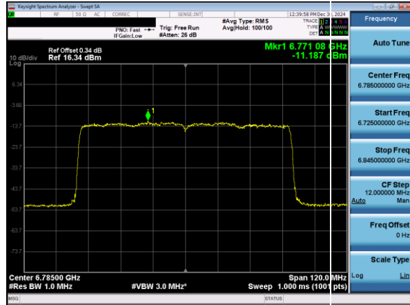
Plot 7-61. Power Spectral Density Plot SDM Primary Antenna 5T (80MHz 802.11ax (UNII Band 7) – Ch. 167)
