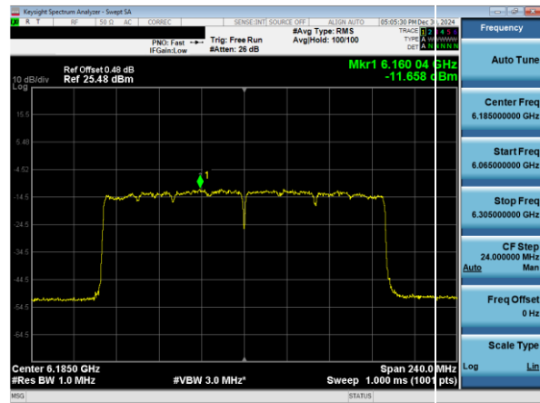
Plot 7-56. Power Spectral Density Plot SDM Primary Antenna 3b (160MHz 802.11ax (UNII Band 5) – Ch. 47)
