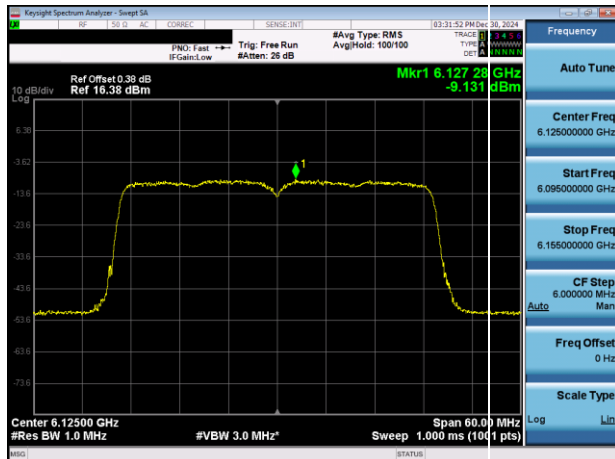
Plot 7-34. PSD Plot Antenna 3b (40MHz 802.11ax (UNII Band 5) – Ch. 35)
