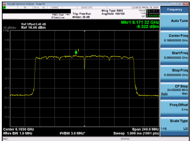
Plot 7-28. PSD Plot Antenna 5T (160MHz 802.11ax (UNII Band 5) – Ch. 47)
