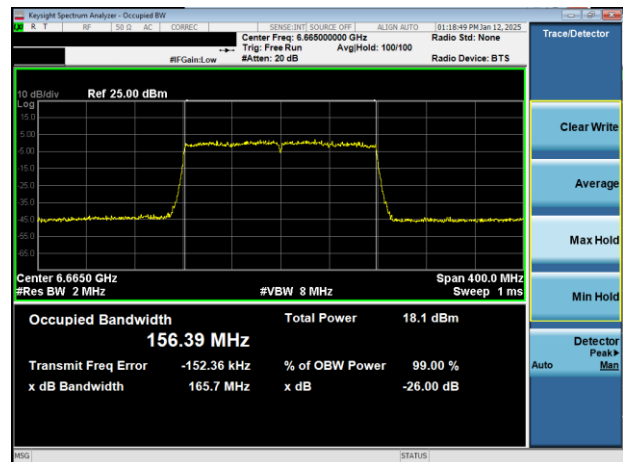
Plot 7-8. 26dB & 99% Bandwidth Plot Antenna 5T (160MHz 802.11ax (UNII Band 7) – Ch. 143)
