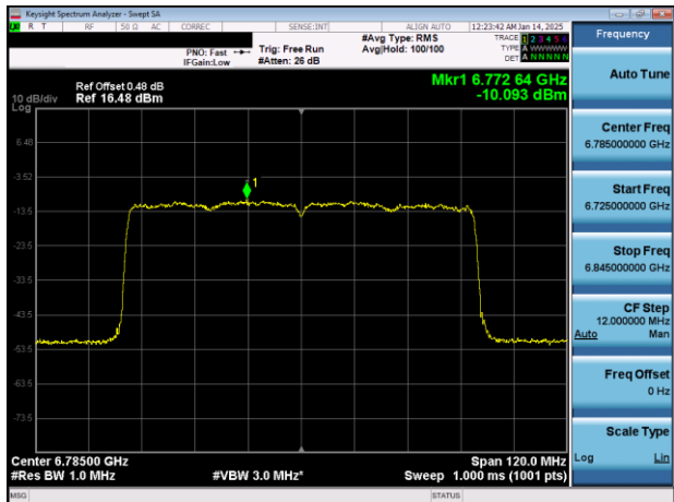
Plot 7-31. PSD Plot Antenna 5T (80MHz 802.11ax (UNII Band 7) – Ch. 167)
