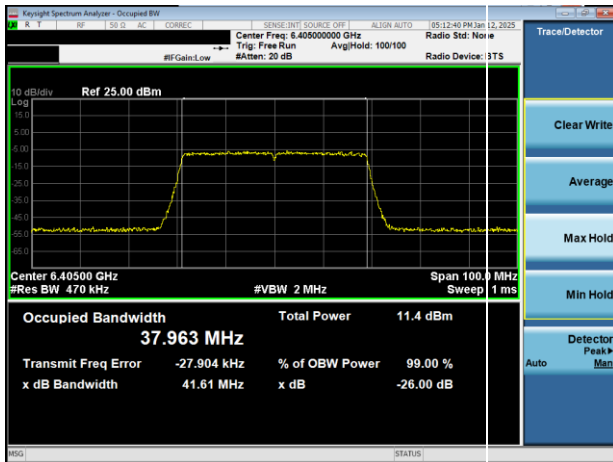
Plot 7-18. 26dB & 99% Bandwidth Plot Antenna 1b (40MHz 802.11ax (UNII Band 5) – Ch. 91)
