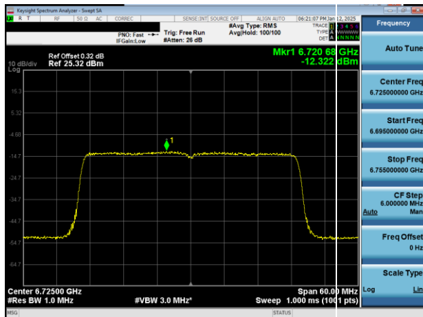
Plot 7-46. PSD Plot Antenna 1b (40MHz 802.11ax (UNII Band 7) – Ch. 155)
