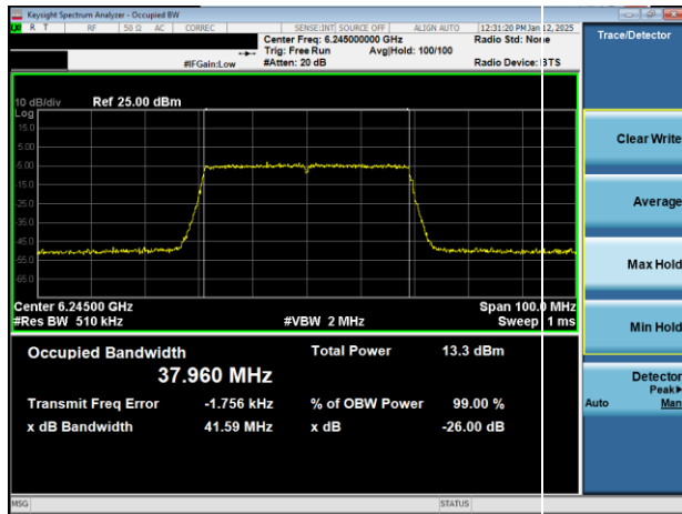
Plot 7-2. 26dB & 99% Bandwidth Plot Antenna 5T (40MHz 802.11ax (UNII Band 5) – Ch. 59)
