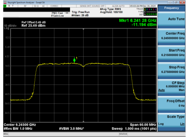
Plot 7-52. Power Spectral Density Plot SDM Primary Antenna 3b (40MHz 802.11ax (UNII Band 5) – Ch. 59)
