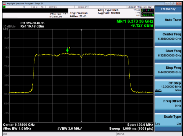
Plot 7-27. PSD Plot Antenna 5T (80MHz 802.11ax (UNII Band 5) – Ch. 87)
