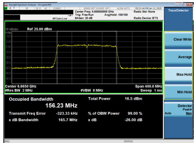
Plot 7-24. 26dB & 99% Bandwidth Plot Antenna 1b (160MHz 802.11ax (UNII Band 7) – Ch. 143)
