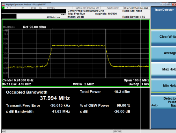
Plot 7-22. 26dB & 99% Bandwidth Plot Antenna 1b (40MHz 802.11ax (UNII Band 7) – Ch. 179)
