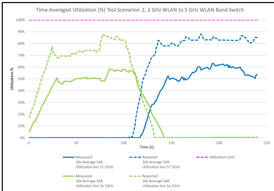
Figure K-5 30s Average Utilization vs. Time during Band Switch
