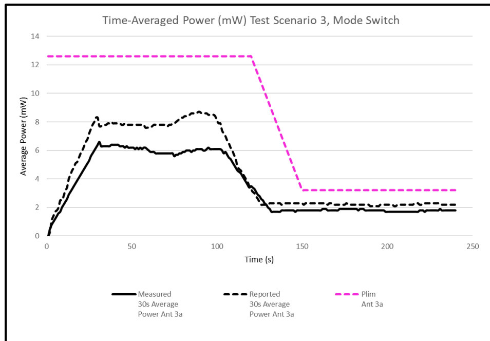
Figure K-8 30s Average Power vs. Time during Mode Switch
