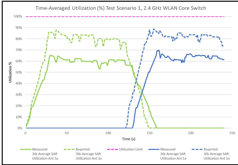
Figure K-1 30s Average SAR Utilization vs. Time, 2.4 GHz
