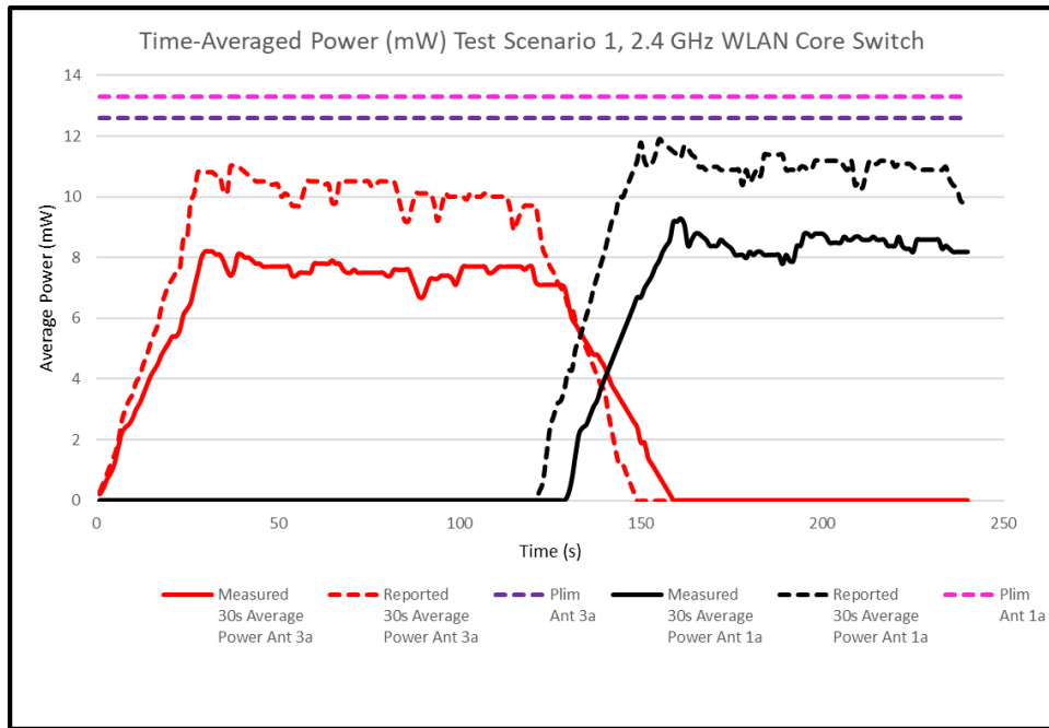
Figure K-2 30s Average Power vs. Time, 2.4 GHz
