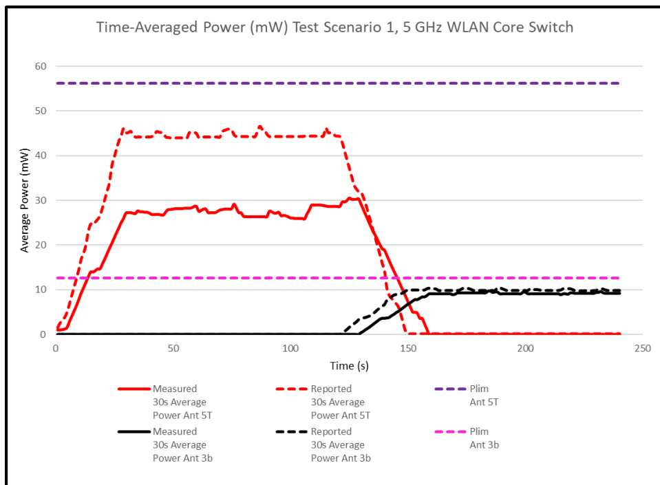
Figure K-4 30s Average Power vs. Time, 5 GHz
