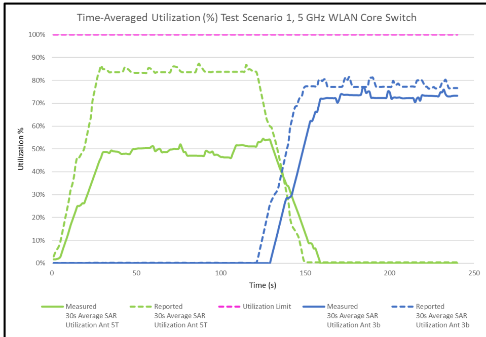
Figure K-3 30s Average SAR Utilization vs. Time, 5 GHz
