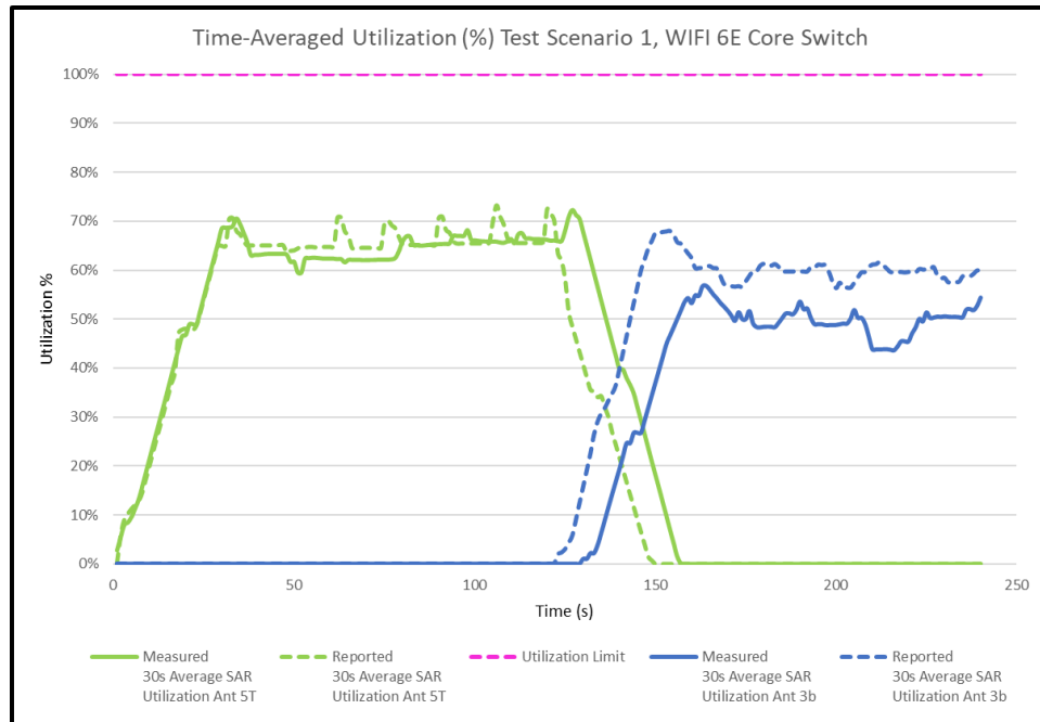
Figure K-5 30s Average SAR Utilization vs. Time, 6 GHz
