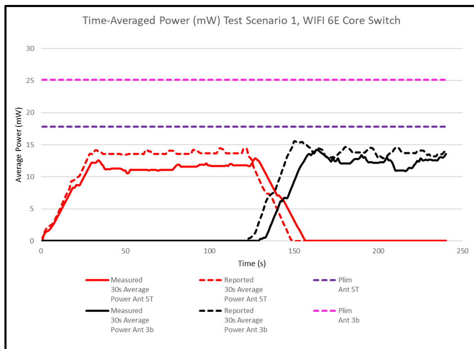
Figure K-6 30s Average Power vs. Time, 6 GHz
