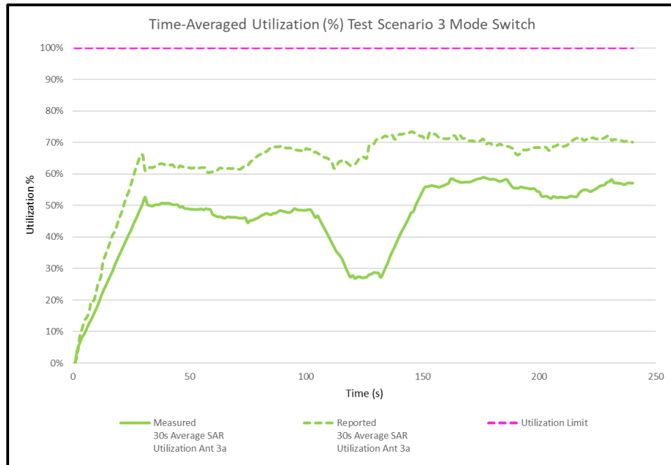
Figure K-7 30s Average Utilization vs. Time during Mode Switch
