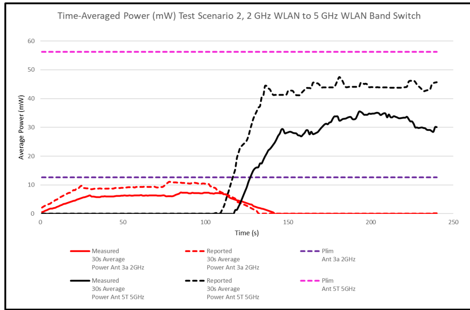
Figure K-6 30s Average Power vs. Time during Band Switch
