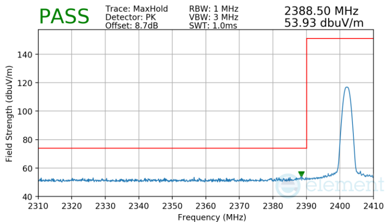
Plot 7-69. Radiated Restricted Lower Band Edge Measurement TxBF
