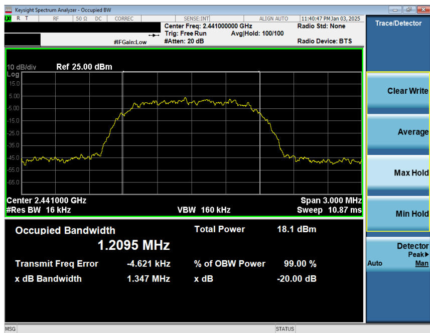
Plot 7-11. 20dB BW and 99% OBW Plot Antenna 1a (Bluetooth, 8DPSK, ePA – Ch. 39)
