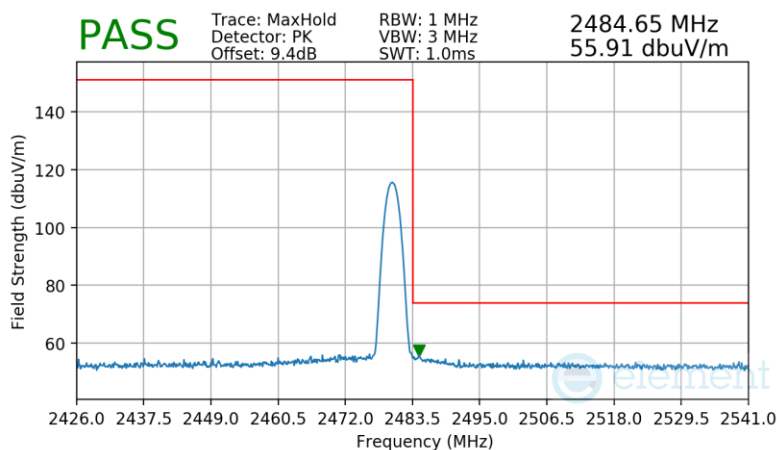
Plot 7-64. Radiated Restricted Upper Band Edge Measurement Antenna 3a
