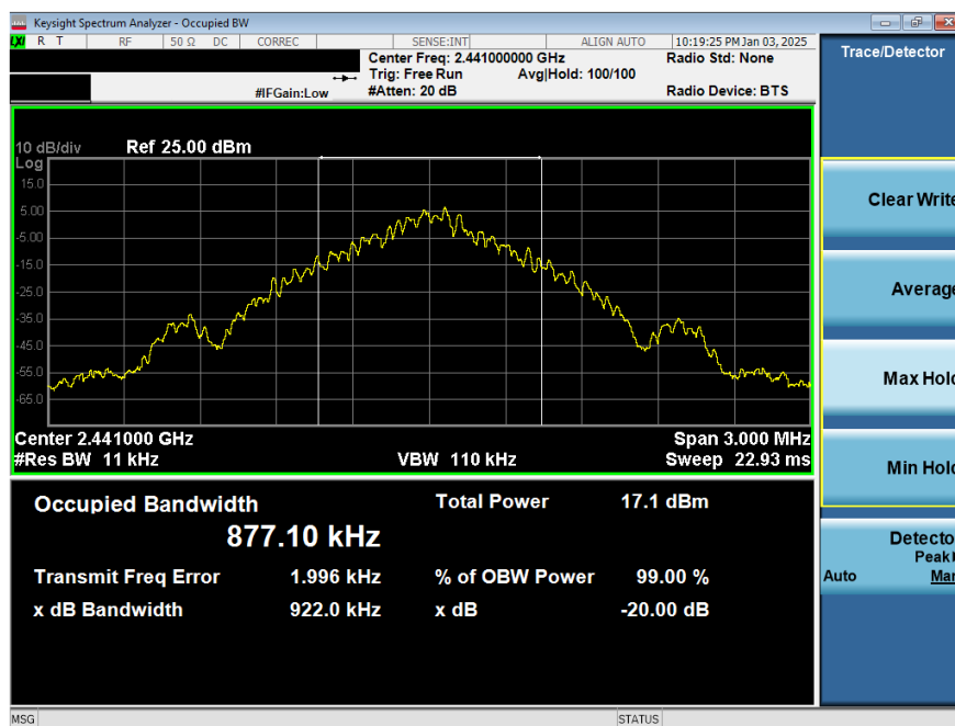
Plot 7-2. 20dB BW and 99% OBW Plot Antenna 3a (Bluetooth, GFSK, ePA – Ch. 39)
