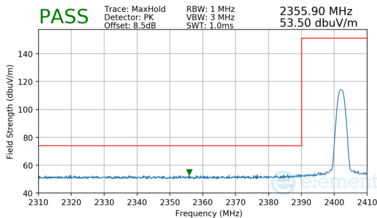
Plot 7-61. Radiated Restricted Lower Band Edge Measurement Antenna 3a
