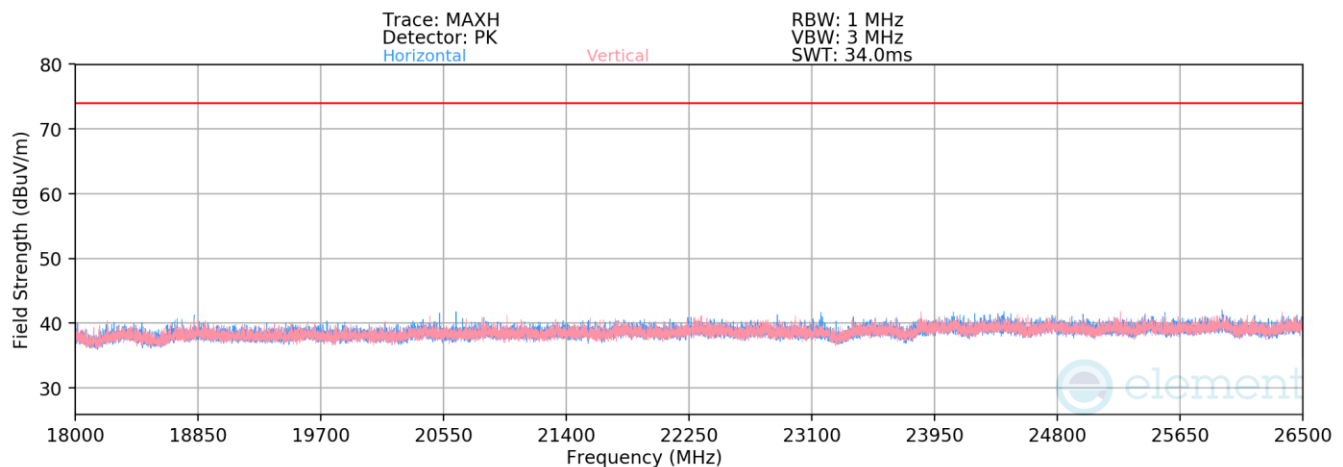
Plot 7-59. Radiated Spurious Emissions above 18GHz TxBF (BT GFSK ePA – Ch. 39)
