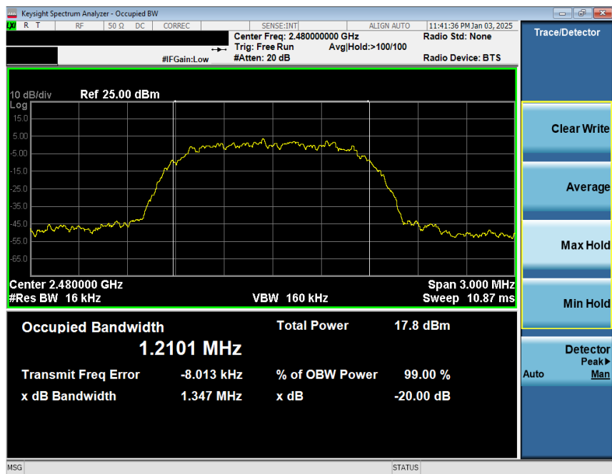
Plot 7-12. 20dB BW and 99% OBW Plot Antenna 1a (Bluetooth, 8DPSK, ePA – Ch. 78)
