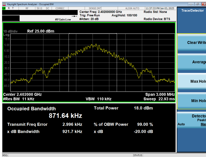
Plot 7-7. 20dB BW and 99% OBW Plot Antenna 1a (Bluetooth, GFSK, ePA – Ch. 0)
