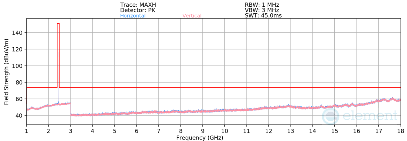
Plot 7-58. Radiated Spurious Emissions above 1GHz TxBF (BT GFSK ePA – Ch. 39)
