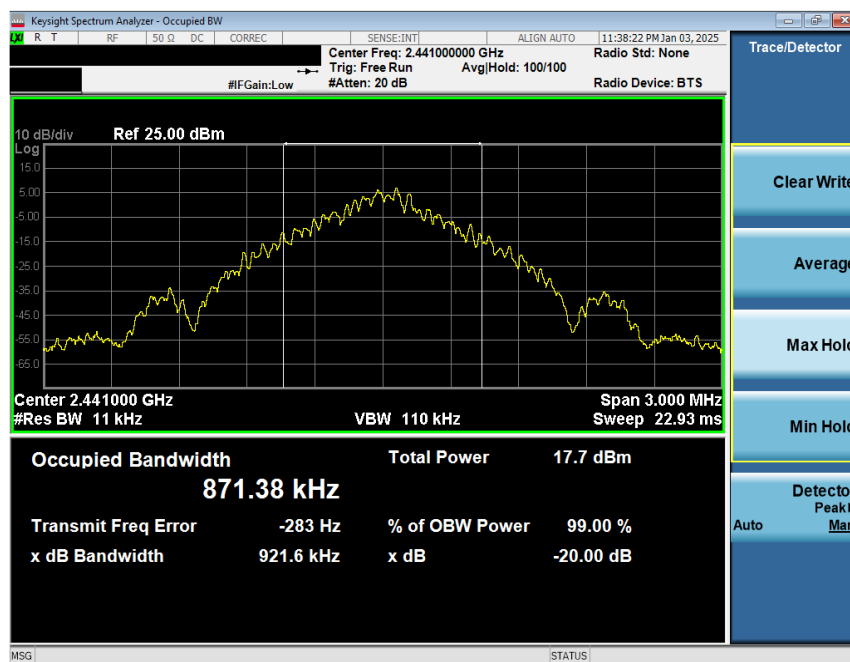
Plot 7-8. 20dB BW and 99% OBW Plot Antenna 1a (Bluetooth, GFSK, ePA – Ch. 39)
