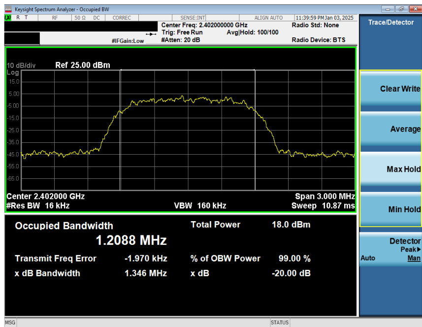
Plot 7-10. 20dB BW and 99% OBW Plot Antenna 1a (Bluetooth, 8DPSK, ePA – Ch. 0)
