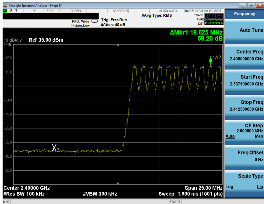
Plot 7-23. Band Edge Plot Antenna 1a (Bluetooth with Hopping Enabled, GFSK, ePA)
