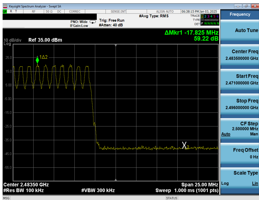
Plot 7-24. Band Edge Plot Antenna 1a (Bluetooth with Hopping Enabled, GFSK, ePA)
