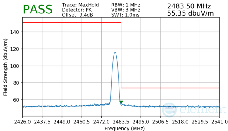
Plot 7-72. Radiated Restricted Upper Band Edge Measurement TxBF
