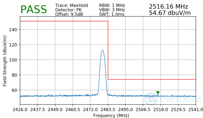
Plot 7-68. Radiated Restricted Upper Band Edge Measurement Antenna 1a
