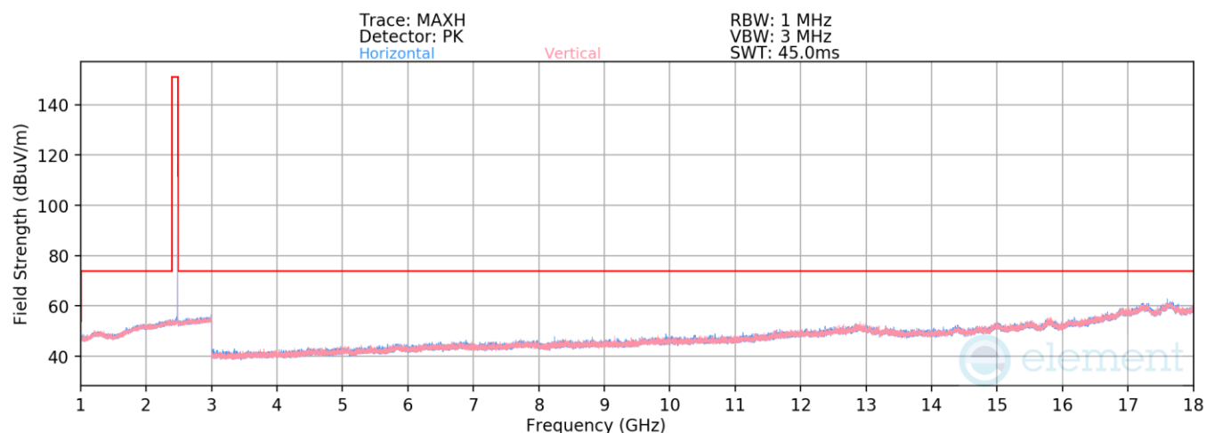
Plot 7-60. Radiated Spurious Emissions above 1GHz TxBF (BT GFSK ePA – Ch. 78)
