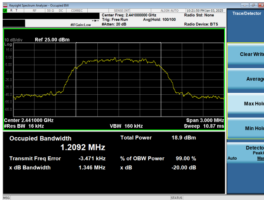
Plot 7-5. 20dB BW and 99% OBW Plot Antenna 3a (Bluetooth, 8DPSK, ePA – Ch. 39)
