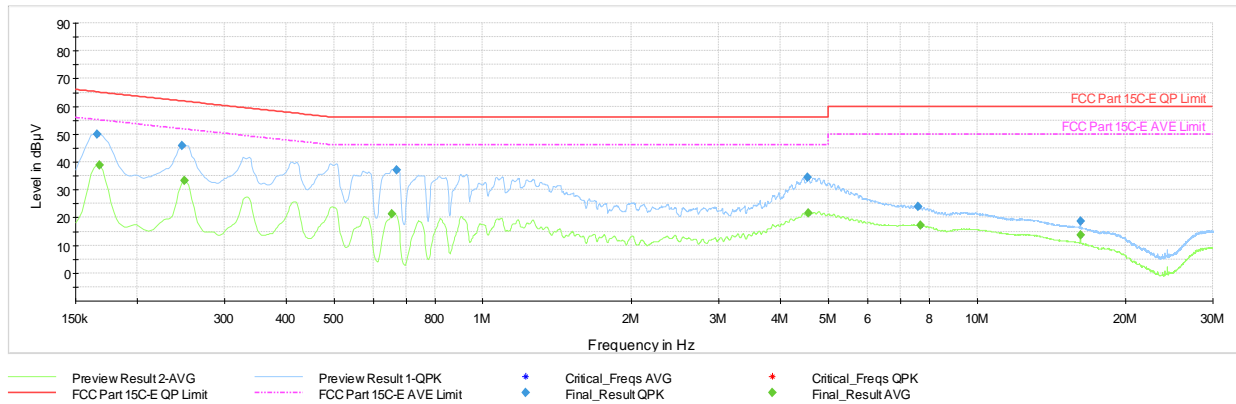
Plot 7-74. AC Line-Conducted Test Plot TxBF (L1, GFSK ePA – Ch.39, with AC/DC Adapter)
