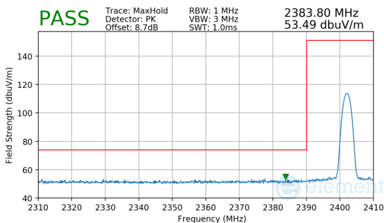
Plot 7-66. Radiated Restricted Lower Band Edge Measurement Antenna 1a
