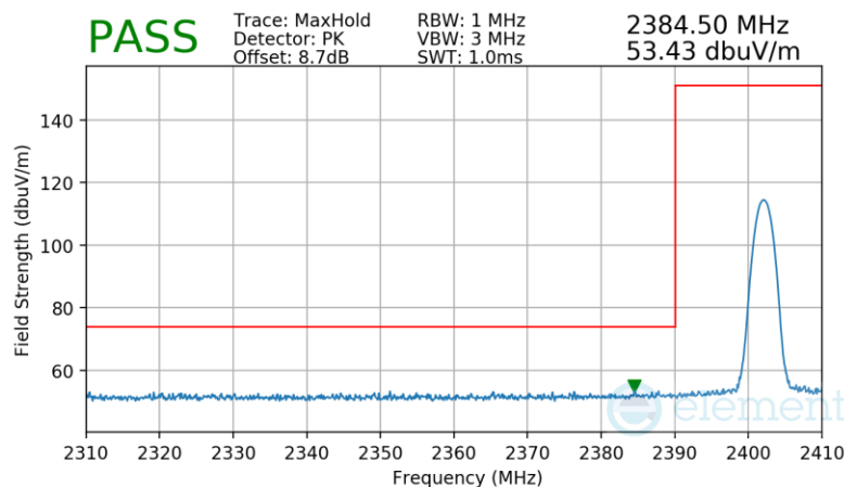
Plot 7-62. Radiated Restricted Lower Band Edge Measurement Antenna 3a
