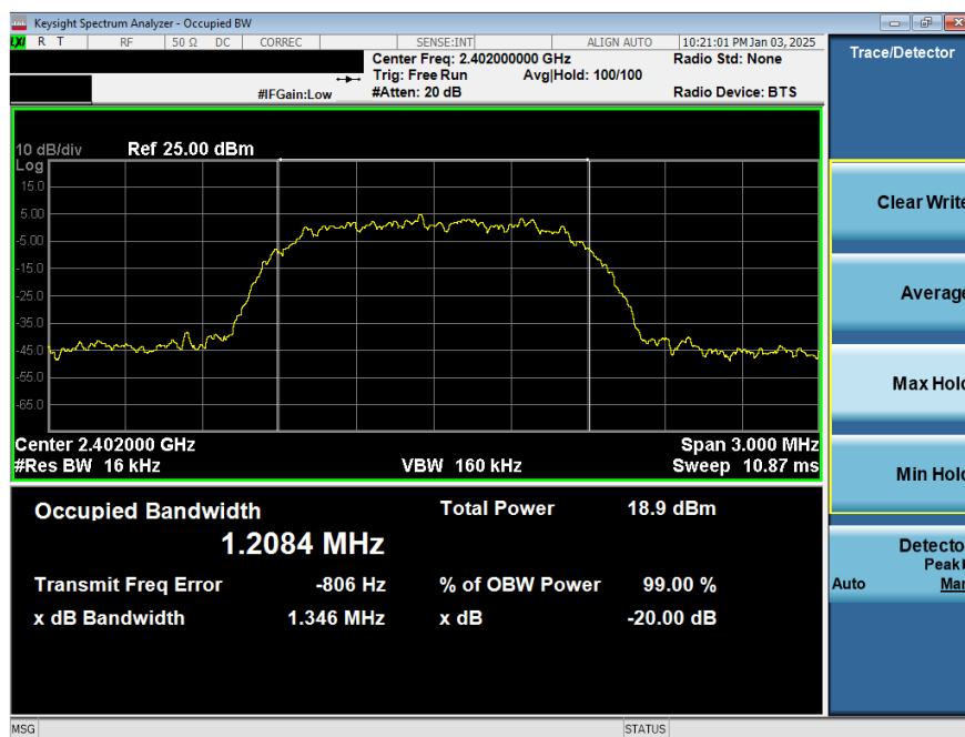
Plot 7-4. 20dB BW and 99% OBW Plot Antenna 3a (Bluetooth, 8DPSK, ePA – Ch. 0)
