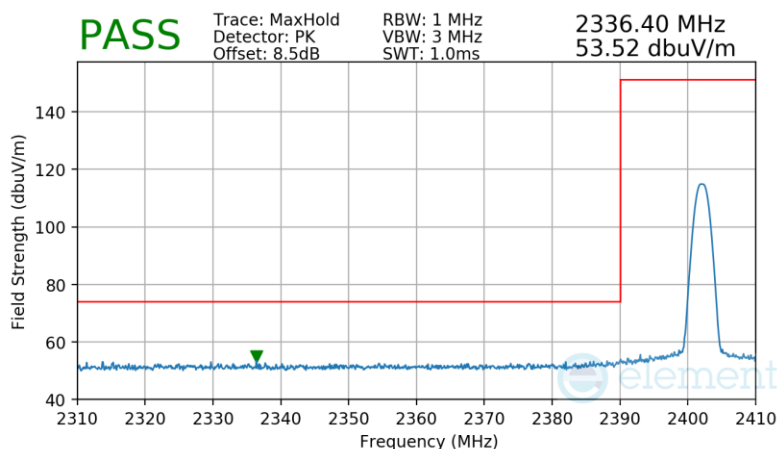
Plot 7-65. Radiated Restricted Lower Band Edge Measurement Antenna 1a
