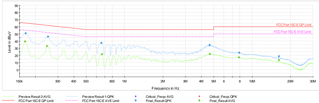
Plot 7-75. AC Line-Conducted Test Plot TxBF (N, GFSK ePA – Ch.39, with AC/DC Adapter)
