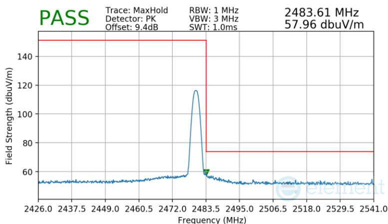
Plot 7-63. Radiated Restricted Upper Band Edge Measurement Antenna 3a
