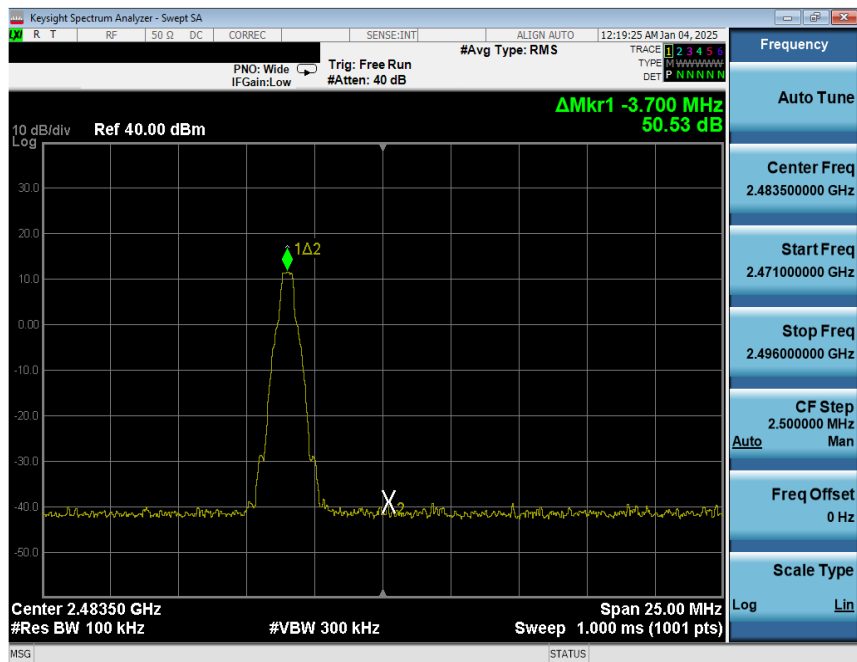
Plot 7-22. Band Edge Plot Antenna 1a (Bluetooth with Hopping Disabled, GFSK, ePA – Ch. 78)
