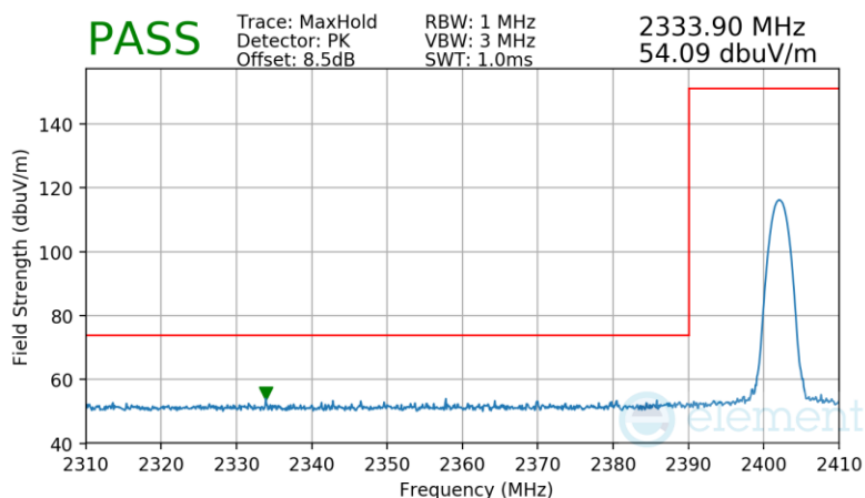
Plot 7-70. Radiated Restricted Lower Band Edge Measurement TxBF
