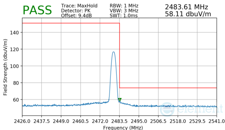
Plot 7-71. Radiated Restricted Upper Band Edge Measurement TxBF
