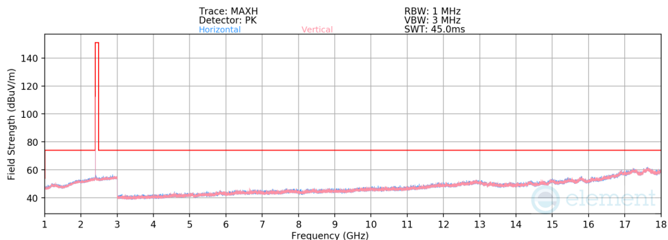
Plot 7-57. Radiated Spurious Emissions above 1GHz TxBF (BT GFSK ePA – Ch. 0)
