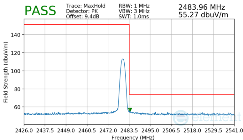
Plot 7-67. Radiated Restricted Upper Band Edge Measurement Antenna 1a
