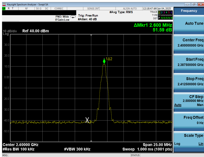
Plot 7-21. Band Edge Plot Antenna 1a (Bluetooth with Hopping Disabled, GFSK, ePA – Ch. 0)
