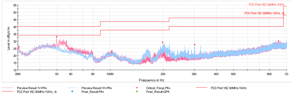
Plot 7-73. Radiated Spurious Emissions Below 1GHz TxBF (GFSK ePA – Ch.39, with AC/DC Adapter)
