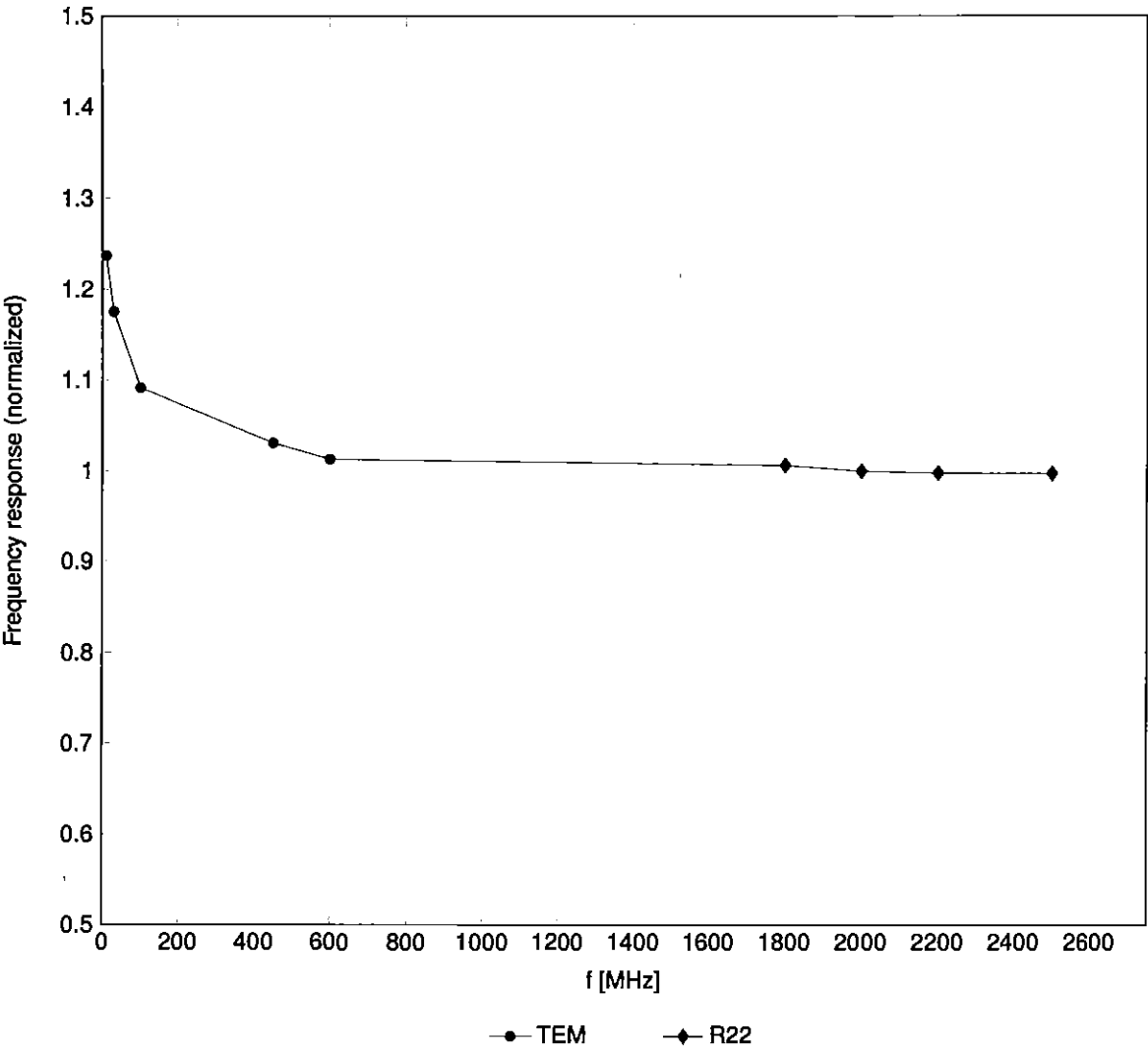
Frequency Response of E-Field (TEM-Cell:if110 EXX, Waveguide:R22)
