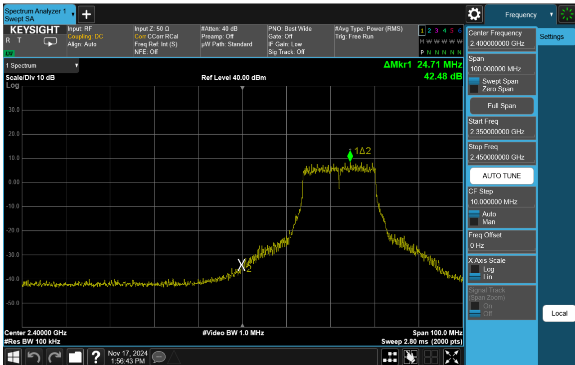
Plot 7-69. Band Edge Plot Antenna 1a (802.11g – Ch. 4)
