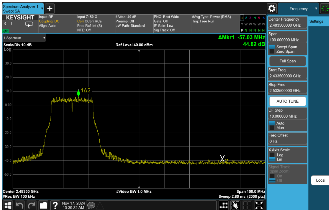
Plot 7-35. Band Edge Plot Antenna 3a (802.11g – Ch. 10)
