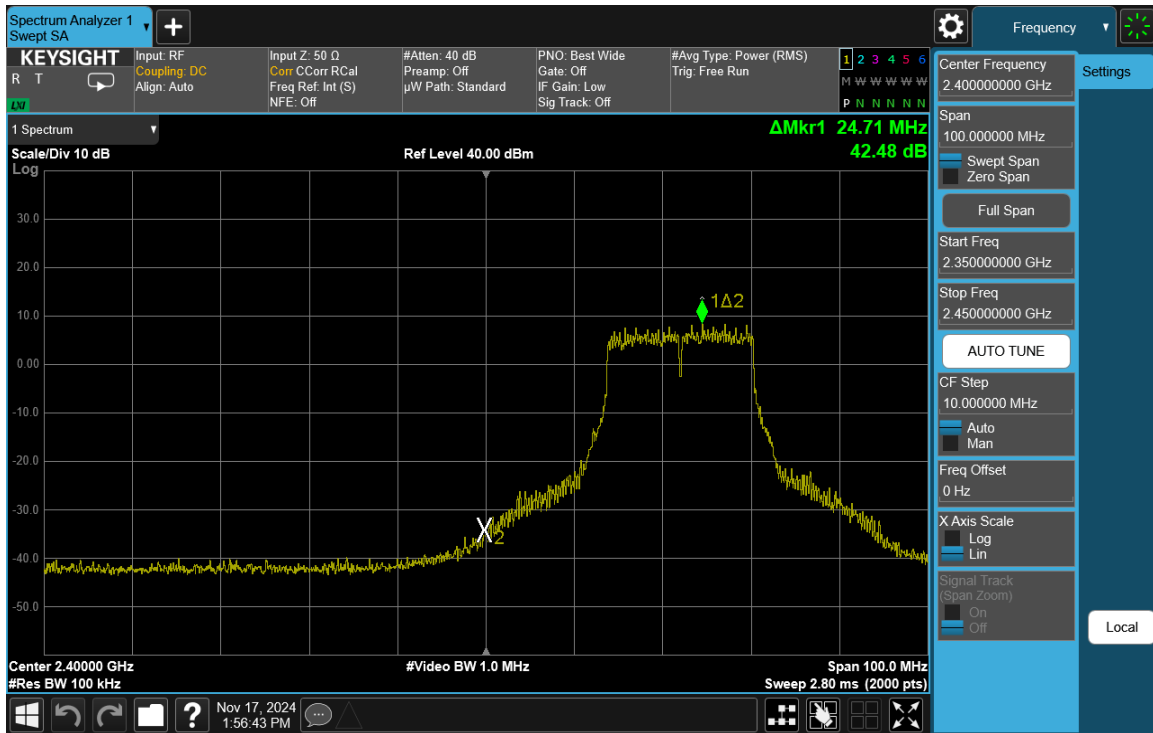
Plot 7-68. Band Edge Plot Antenna 1a (802.11g – Ch. 3)
