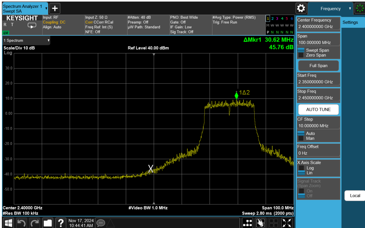
Plot 7-42. Band Edge Plot Antenna 3a (802.11n – Ch. 4)
