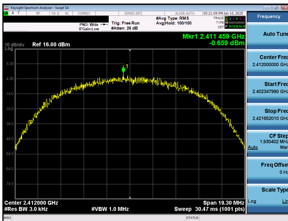
Plot 7-9. Power Spectral Density Plot Antenna 3a (802.11b – Ch. 1)
