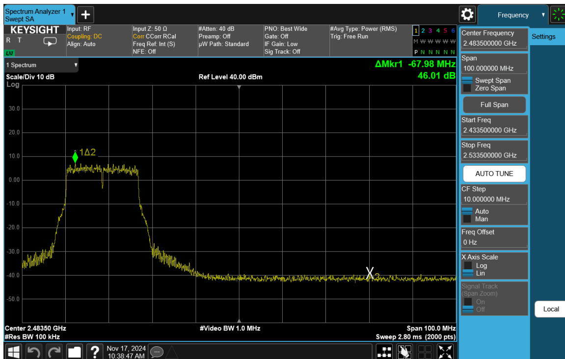
Plot 7-34. Band Edge Plot Antenna 3a (802.11g – Ch. 9)
