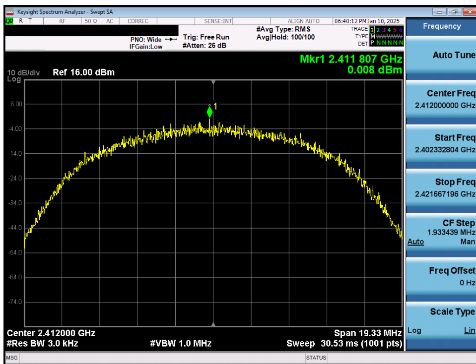
Plot 7-13. Power Spectral Density Plot Antenna 3a (802.11b – Ch. 1)
