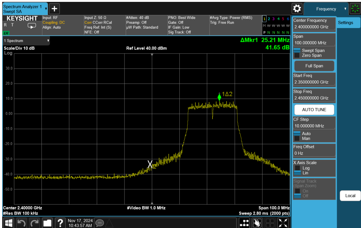
Plot 7-41. Band Edge Plot Antenna 3a (802.11n (2.4GHz) – Ch. 3)
