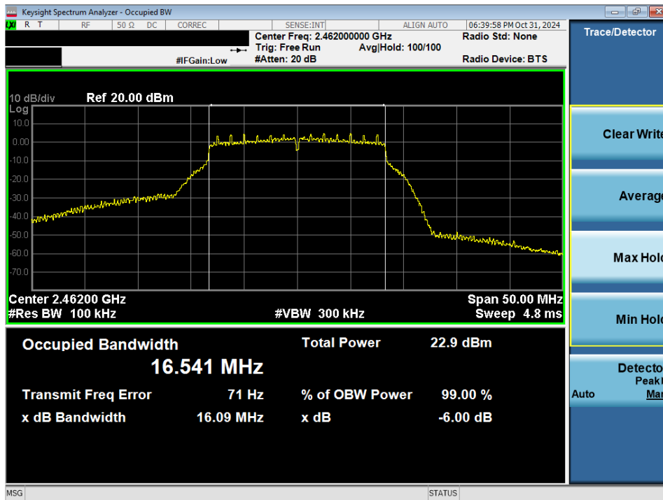
Plot 7-6. 6 dB BW and 99% OBW Plot Antenna 1a (802.11g – Ch. 11)
