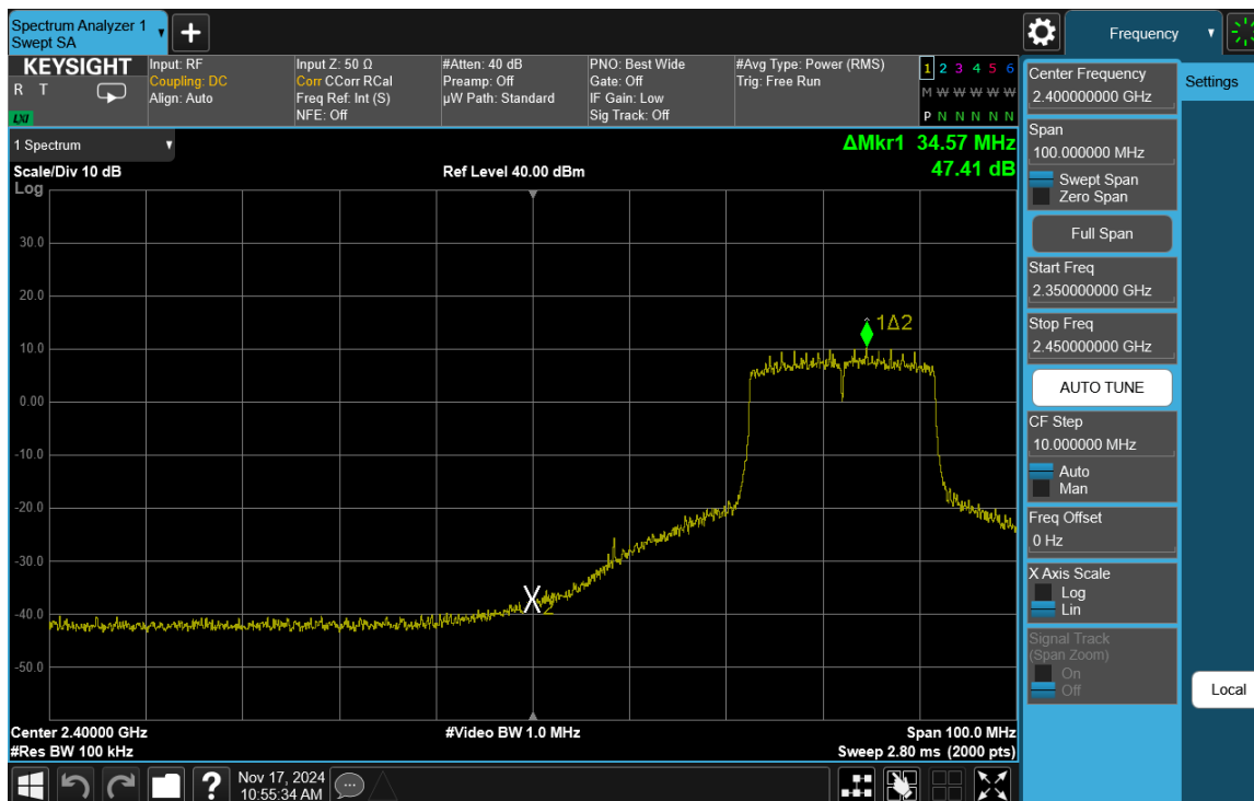
Plot 7-55. Band Edge Plot Antenna 3a (802.11ax (SU - 2.4GHz) – Ch. 5)
