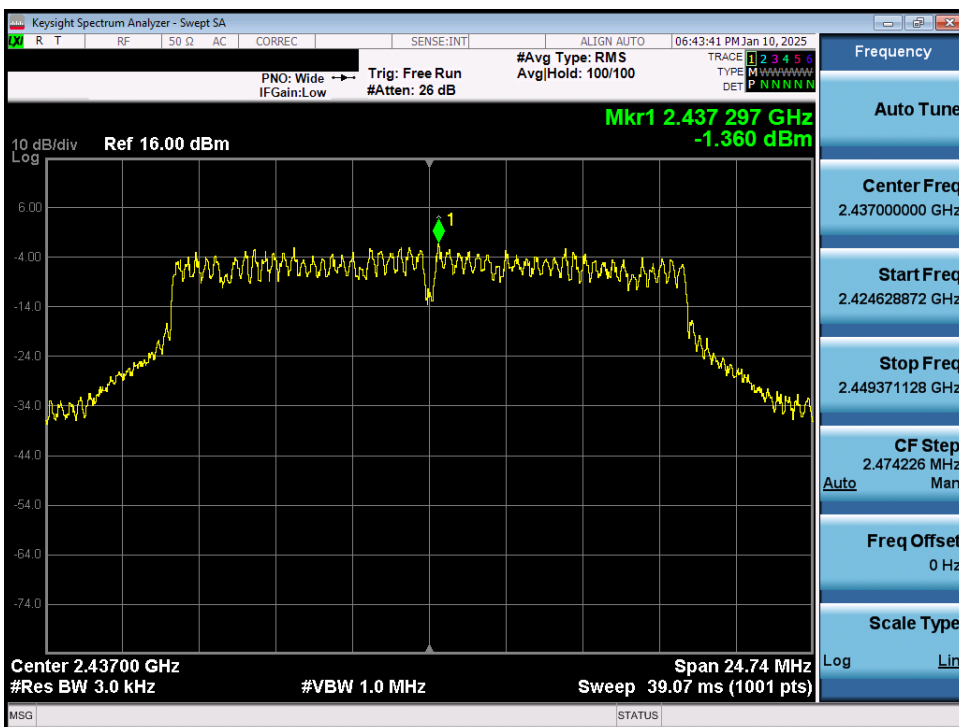
Plot 7-14. Power Spectral Density Plot Antenna 3a (802.11g – Ch. 6)
