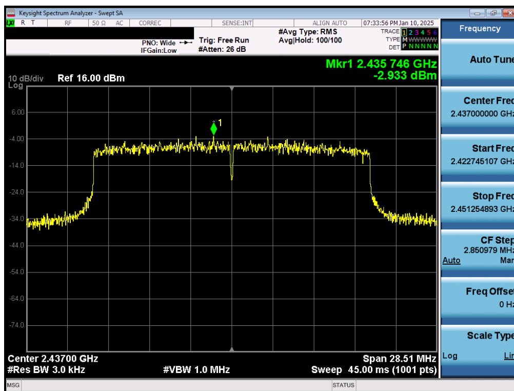
Plot 7-22. Power Spectral Density Plot CDD Antenna 1a (802.11 ax (SU) – Ch. 6)
