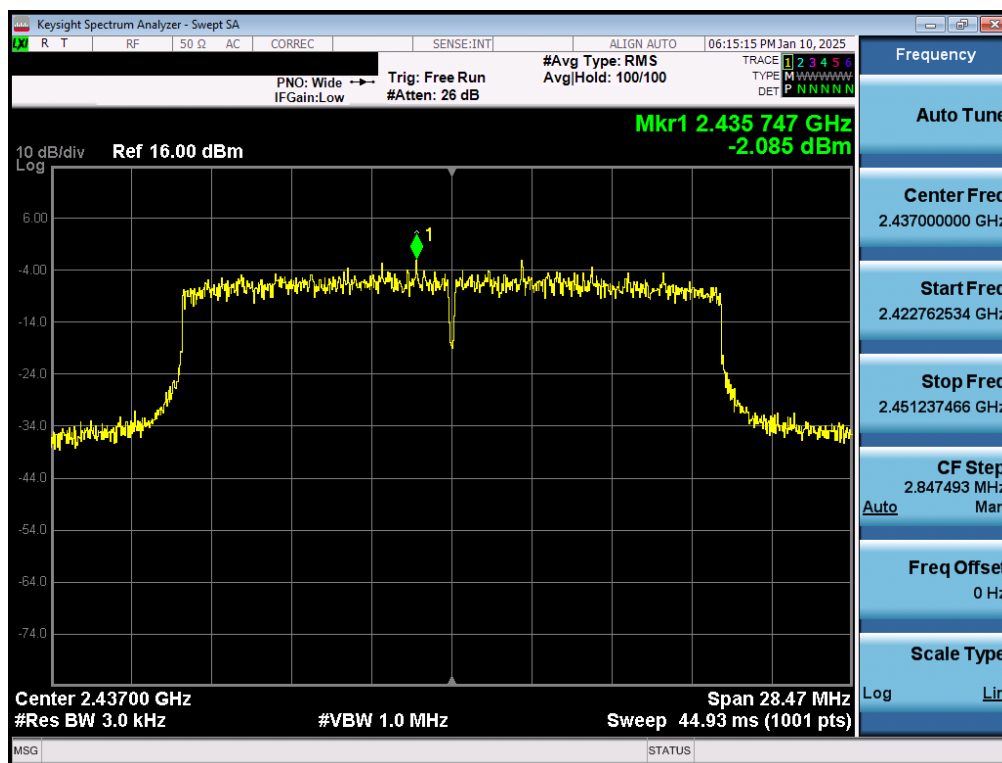
Plot 7-21. Power Spectral Density Plot CDD Antenna 3a (802.11ax (SU) – Ch. 6)
