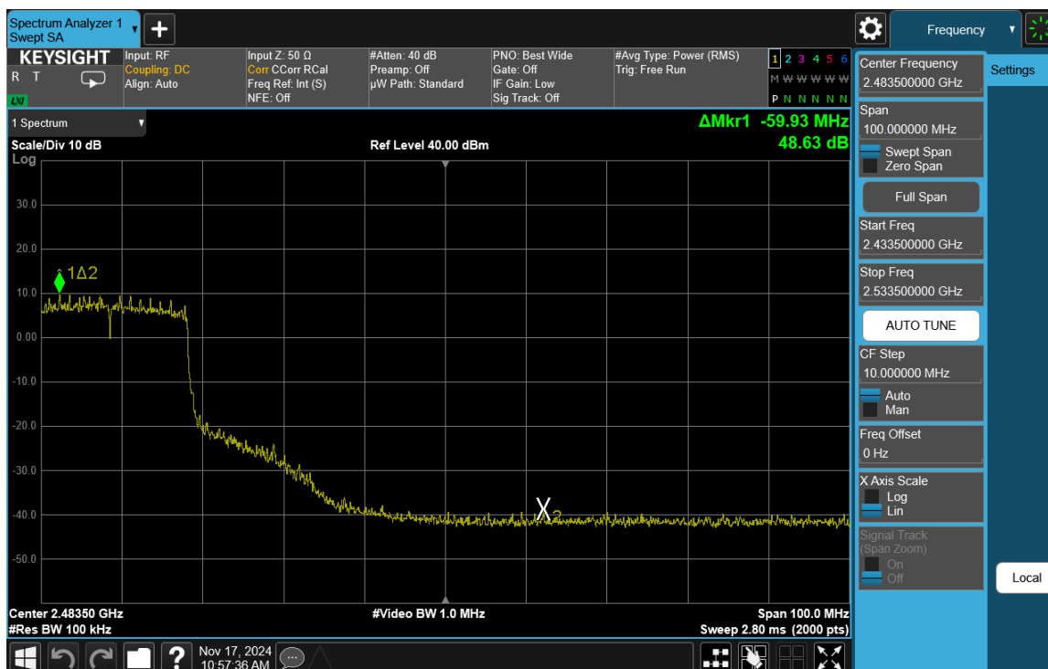
Plot 7-56. Band Edge Plot Antenna 3a (802.11ax (SU - 2.4GHz) – Ch. 7)
