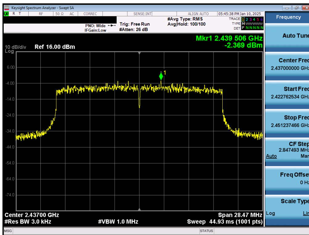
Plot 7-12. Power Spectral Density Plot Antenna 3a (802.11ax(SU) – Ch. 6)
