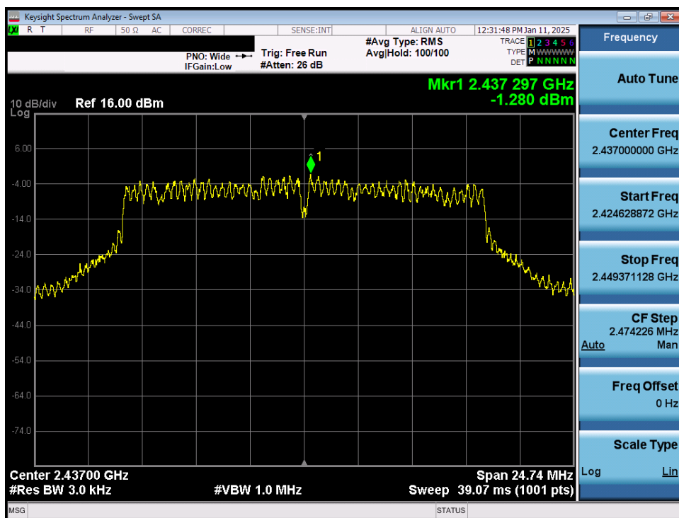
Plot 7-18. Power Spectral Density Plot CDD Antenna 1a (802.11g – Ch. 6)
