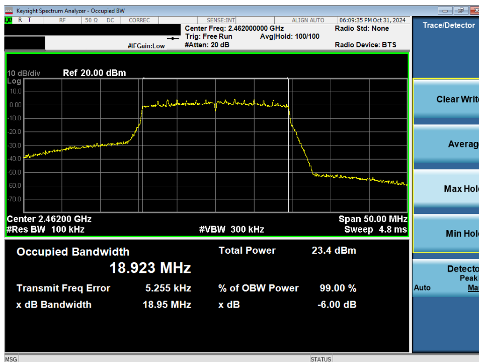
Plot 7-4. 6 dB BW and 99% OBW Plot Antenna 3a (802.11ax(SU) – Ch. 11)
