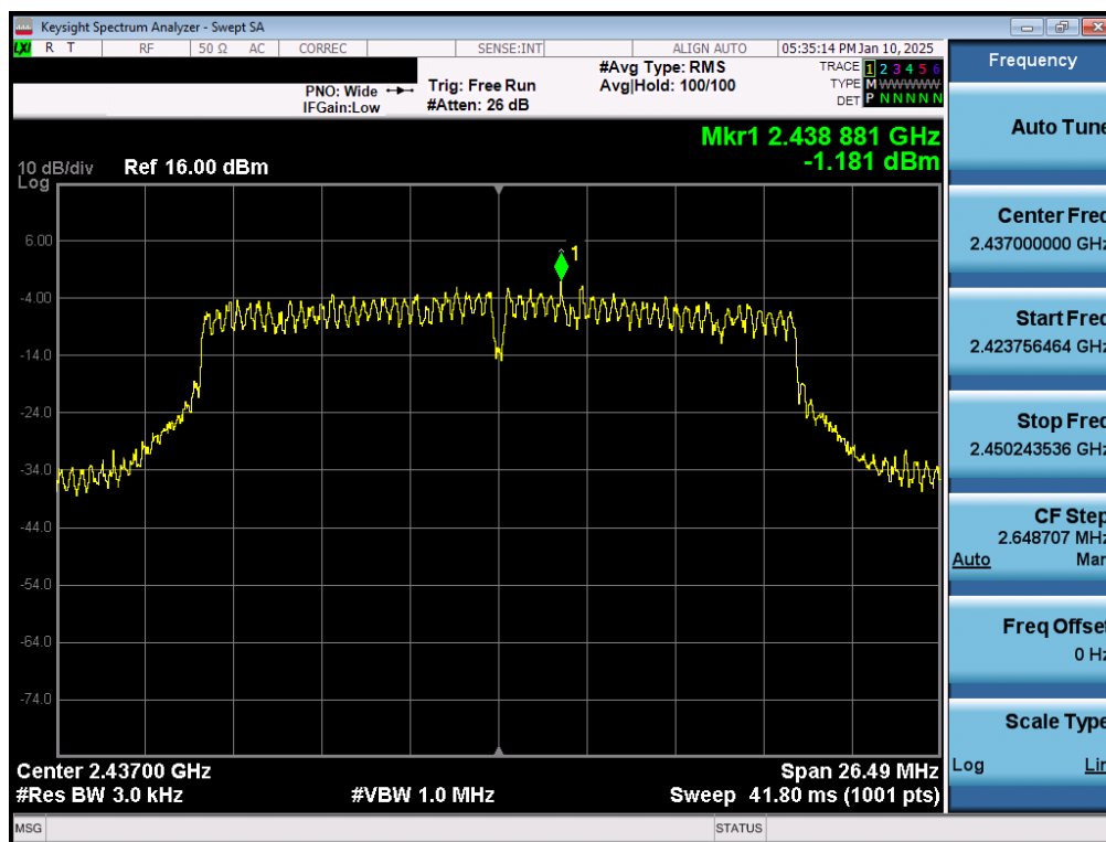
Plot 7-11. Power Spectral Density Plot Antenna 3a (802.11n – Ch. 6)
