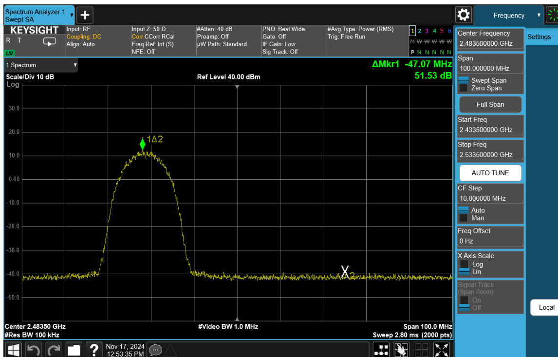
Plot 7-63. Band Edge Plot Antenna 1a (802.11b – Ch. 11)
