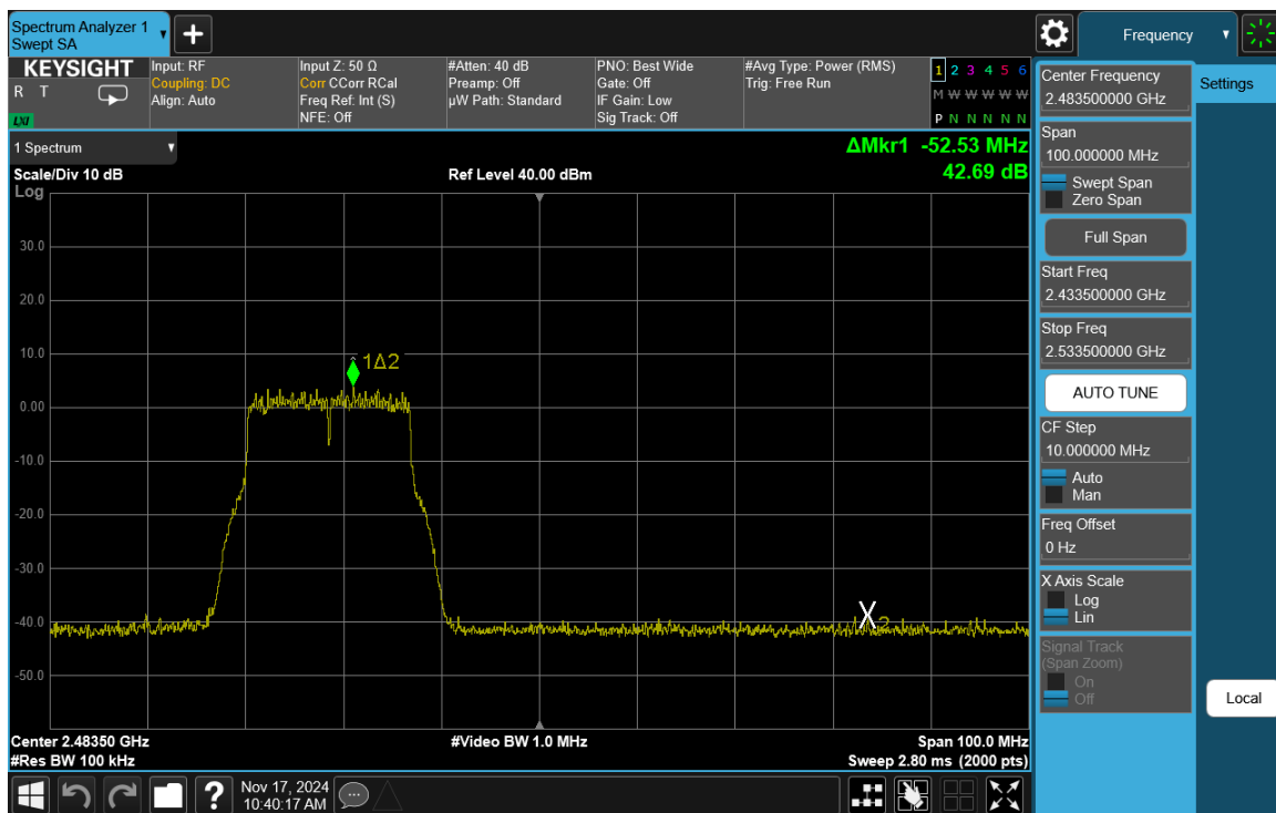
Plot 7-36. Band Edge Plot Antenna 3a (802.11g – Ch. 11)
