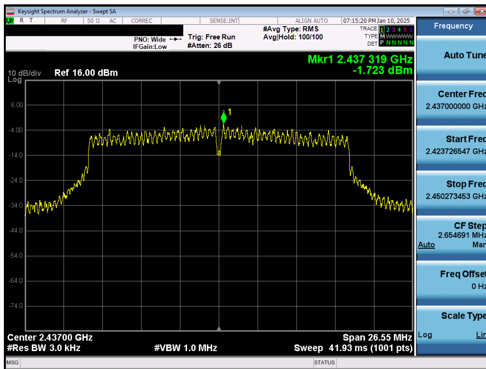
Plot 7-20. Power Spectral Density Plot CDD Antenna 1a (802.11n – Ch. 6)
