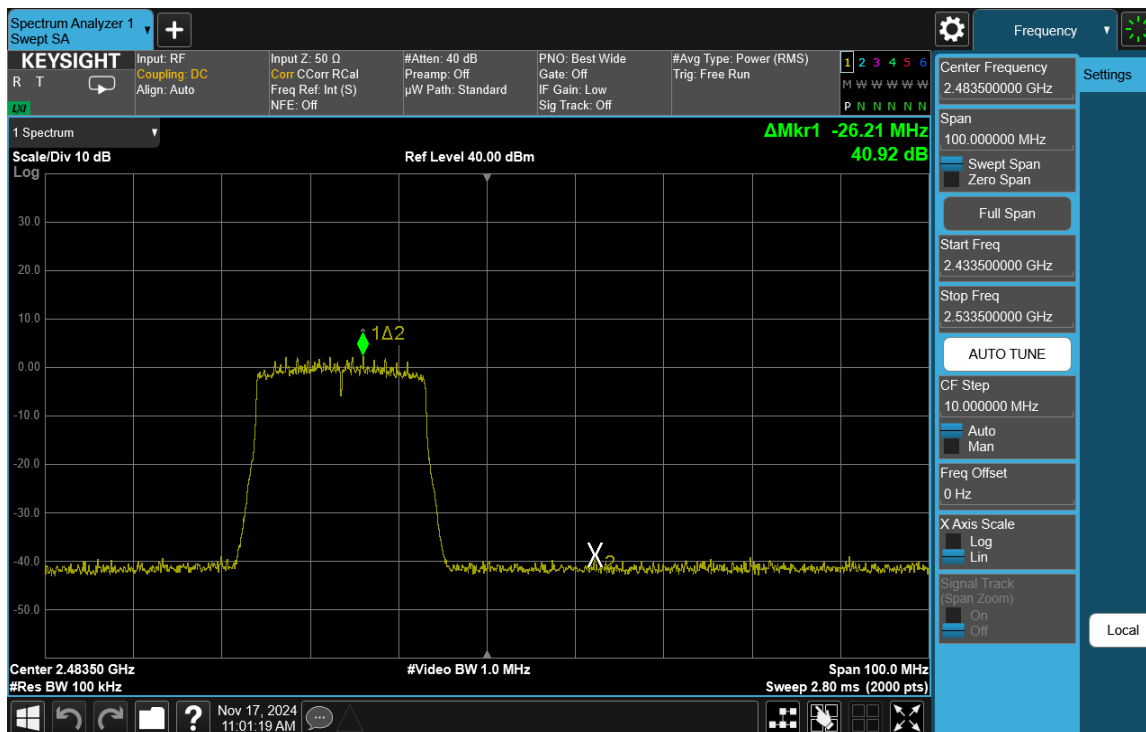
Plot 7-61. Band Edge Plot Antenna 3a (802.11ax (SU - 2.4GHz) – Ch. 12)
