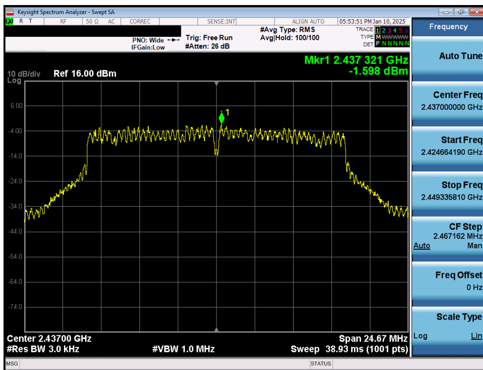
Plot 7-17. Power Spectral Density Plot CDD Antenna 3a (802.11g – Ch. 6)
