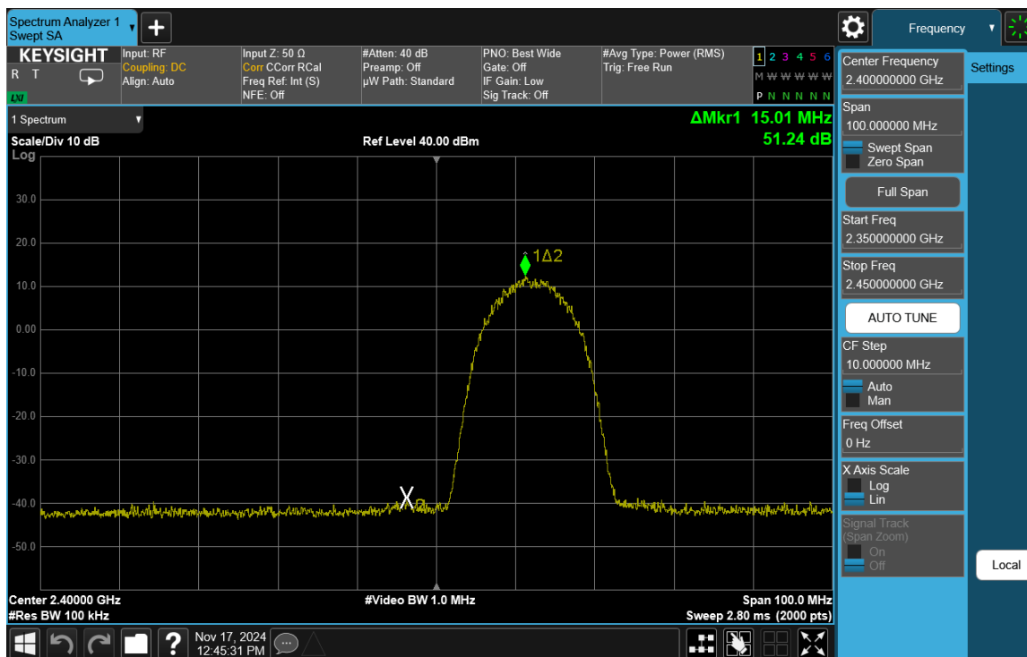
Plot 7-62. Band Edge Plot Antenna 1a (802.11b – Ch. 1)
