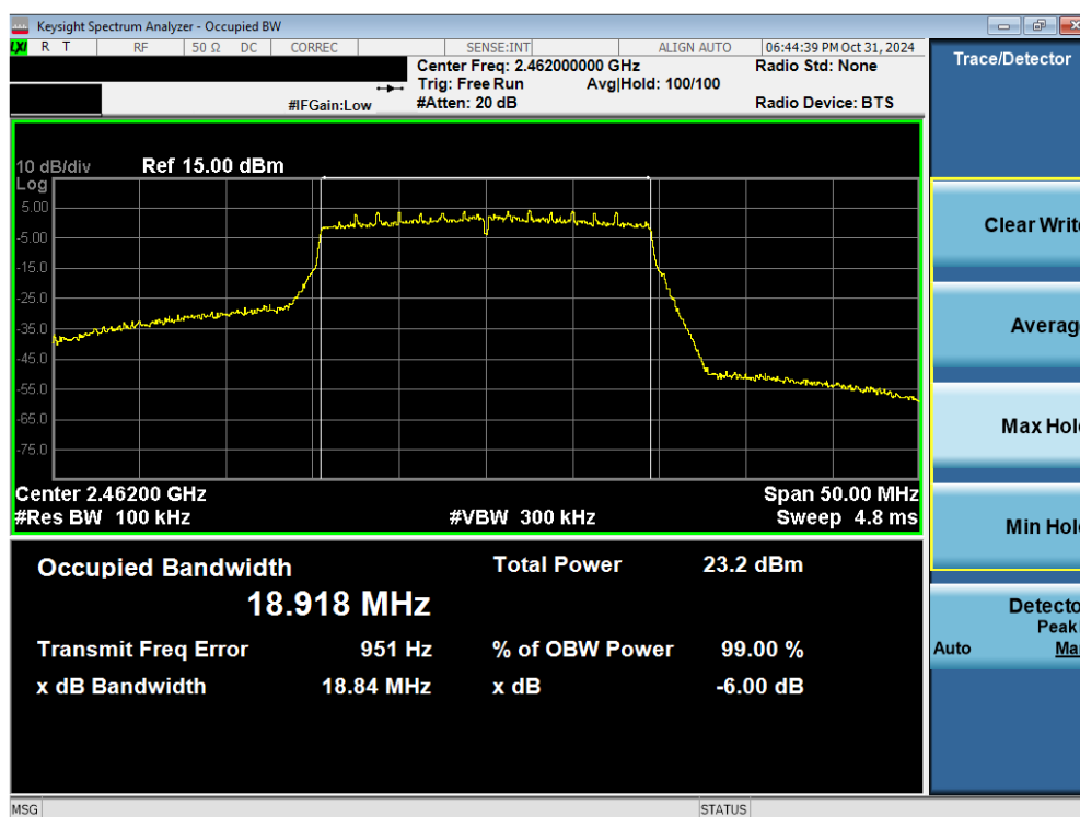
Plot 7-8. 6 dB BW and 99% OBW Plot Antenna 1a (802.11ax (SU) – Ch. 11)
