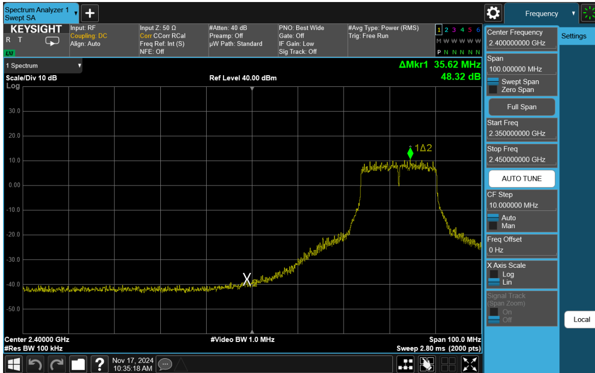
Plot 7-31. Band Edge Plot Antenna 3a (802.11g – Ch. 5)
