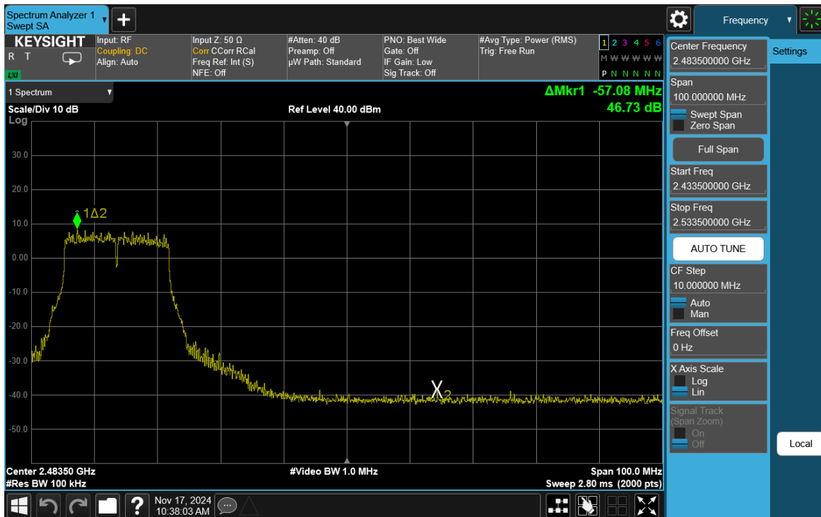
Plot 7-33. Band Edge Plot Antenna 3a (802.11g – Ch. 8)
