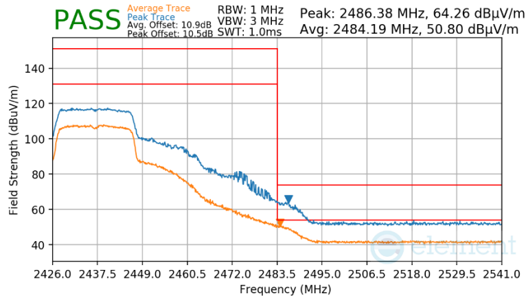
Plot 7-102 Radiated Restricted Upper Band Edge Measurement Antenna 1a (Peak & Average – RU242)
