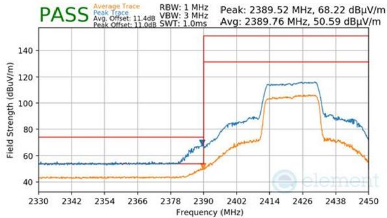
Plot 7-81 Radiated Restricted Lower Band Edge Measurement Antenna 3a (Peak & Average – RU242)
