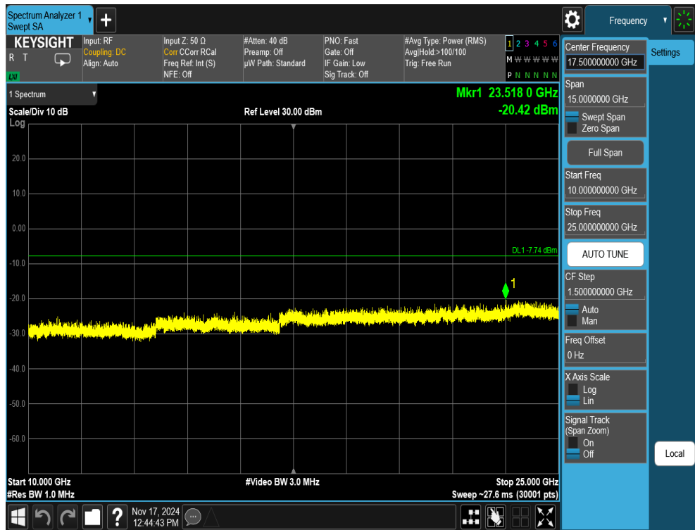
Plot 7-66. Conducted Spurious Plot Antenna 1a (802.11ax OFDMA – RU242 – Ch. 11)
