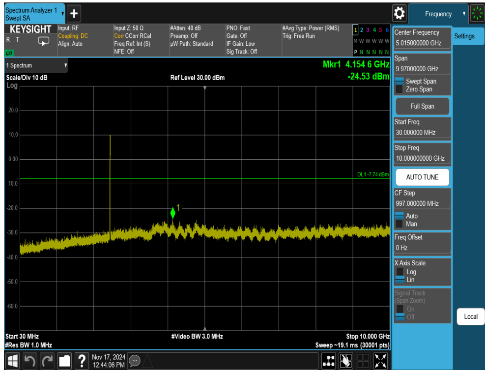
Plot 7-65. Conducted Spurious Plot Antenna 1a (802.11ax OFDMA – RU242 – Ch. 11)
