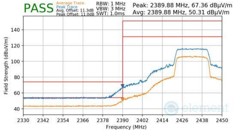
Plot 7-83 Radiated Restricted Lower Band Edge Measurement Antenna 3a (Peak & Average – RU242)
