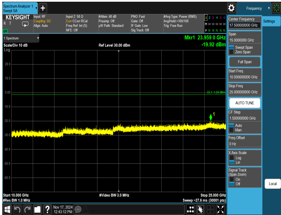
Plot 7-64. Conducted Spurious Plot Antenna 1a (802.11ax OFDMA – RU242 – Ch. 6)
