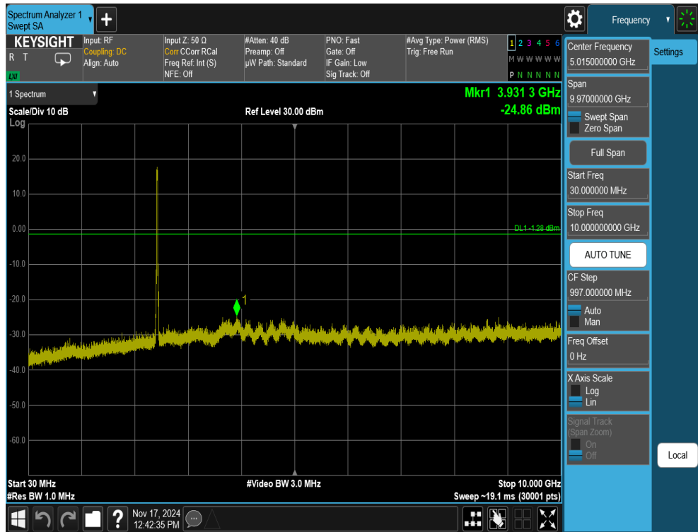
Plot 7-63. Conducted Spurious Plot Antenna 1a (802.11ax OFDMA – RU242 – Ch. 6)
