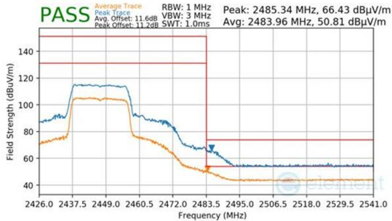
Plot 7-104 Radiated Restricted Upper Band Edge Measurement Antenna 1a (Peak & Average – RU242)
