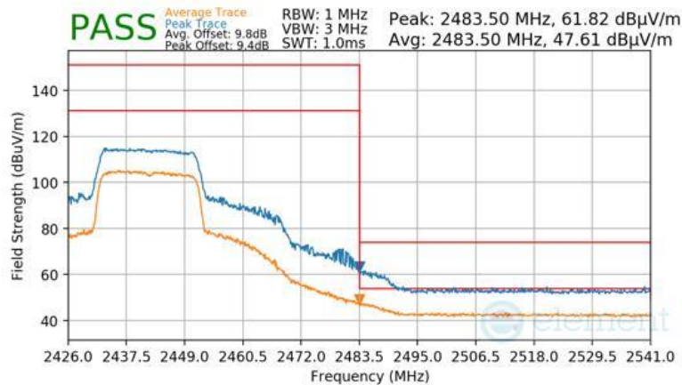
Plot 7-86 Radiated Restricted Upper Band Edge Measurement Antenna 3a (Peak & Average – RU242)
