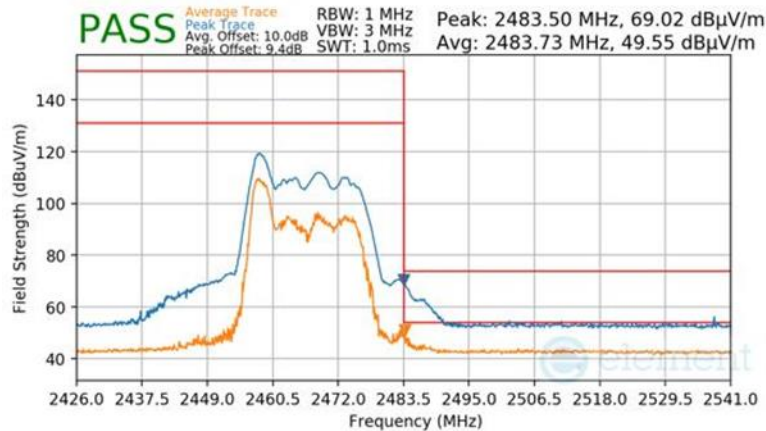
Plot 7-111 Radiated Restricted Upper Band Edge Measurement CDD (Peak & Average – RU26)
