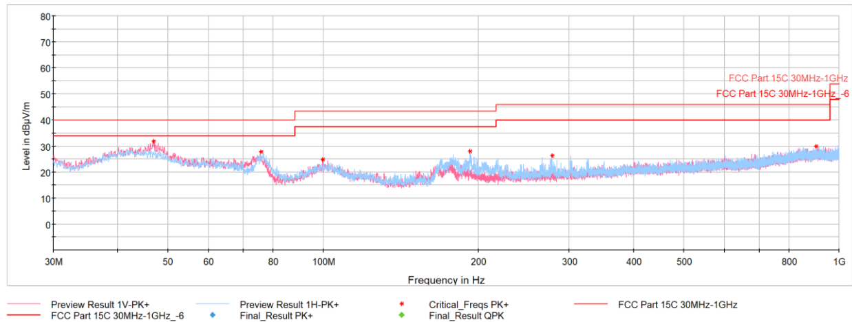
Plot 7-126. Radiated Spurious Emissions below 1GHz CDD Ch.6 (RU26), with AC/DC Adapter
