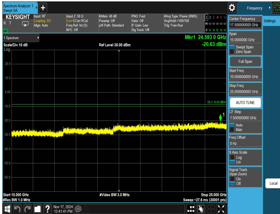
Plot 7-62. Conducted Spurious Plot Antenna 1a (802.11ax OFDMA – RU242 – Ch. 1)
