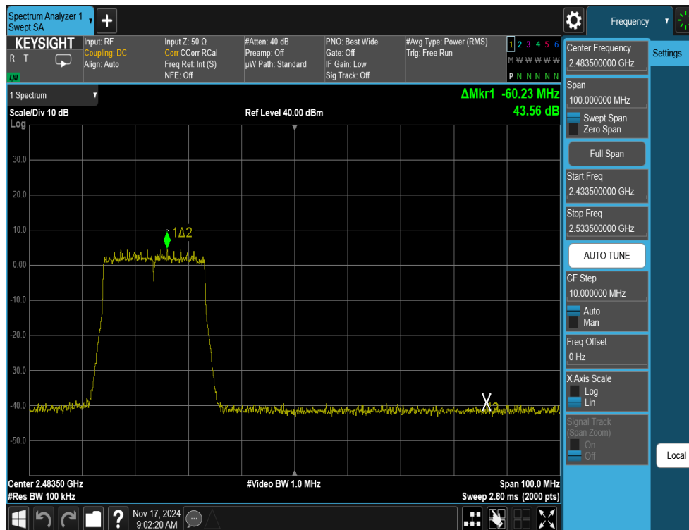
Plot 7-25. Band Edge Antenna 3a (802.11ax OFDMA – RU242 – Ch. 10)
