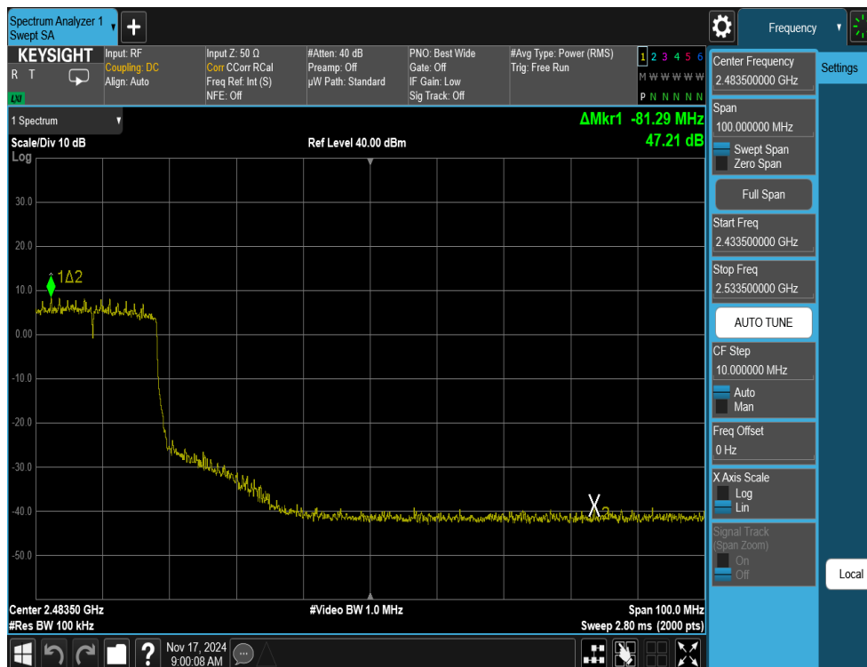
Plot 7-22. Band Edge Antenna 3a (802.11ax OFDMA – RU242 – Ch. 7)
