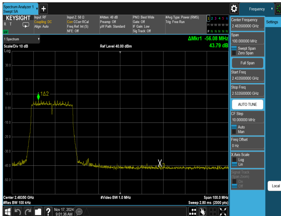
Plot 7-24. Band Edge Antenna 3a (802.11ax OFDMA – RU242 – Ch. 9)
