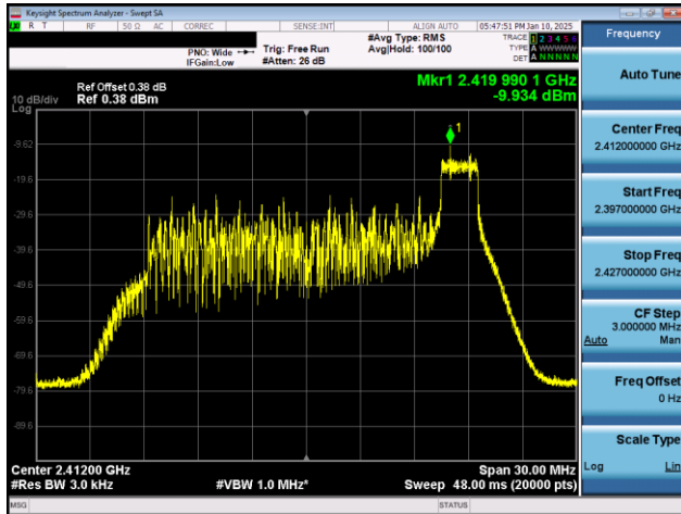
Plot 7-9. Power Spectral Density Plot Antenna 3a (802.11ax OFDMA – RU26 Index 8 – Ch. 1)
