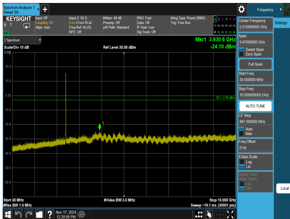
Plot 7-55. Conducted Spurious Plot Antenna 1a (802.11ax OFDMA – RU26 – Ch. 1)
