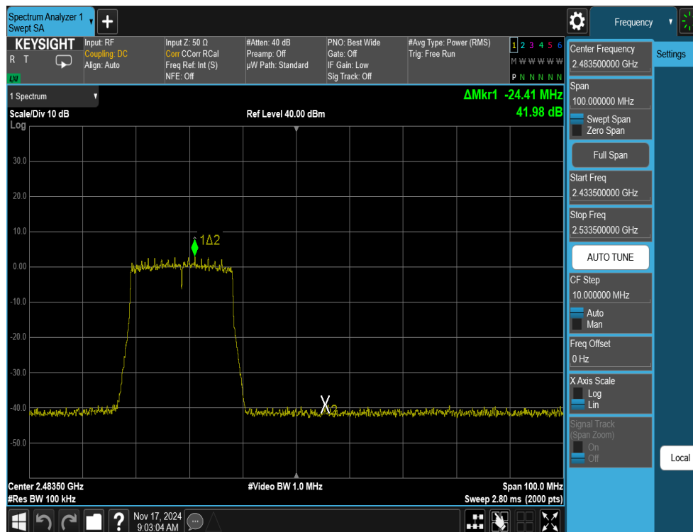
Plot 7-26. Band Edge Antenna 3a (802.11ax OFDMA – RU242 – Ch. 11)
