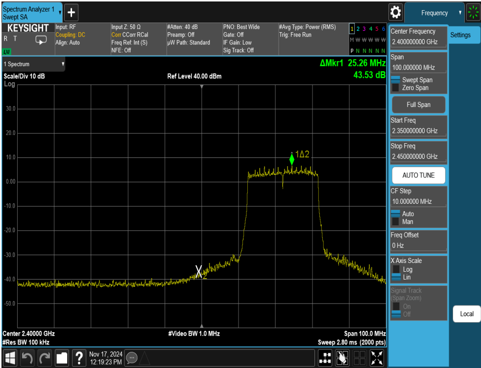
Plot 7-32. Band Edge Antenna 1a (802.11ax OFDMA – RU242 – Ch. 3)
