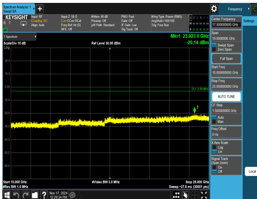
Plot 7-56. Conducted Spurious Plot Antenna 1a (802.11ax OFDMA – RU26 – Ch. 1)
