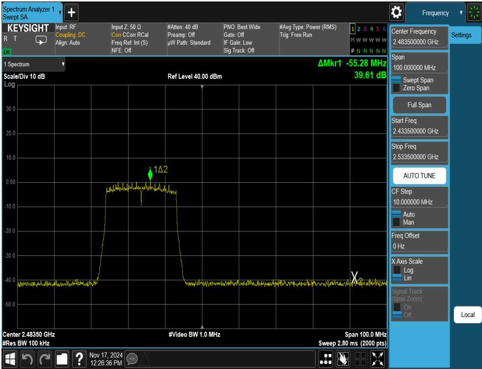
Plot 7-42. Band Edge Antenna 1a (802.11ax OFDMA – RU242 – Ch. 12)
