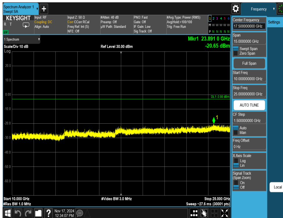
Plot 7-58. Conducted Spurious Plot Antenna 1a (802.11ax OFDMA – RU26 – Ch. 6)
