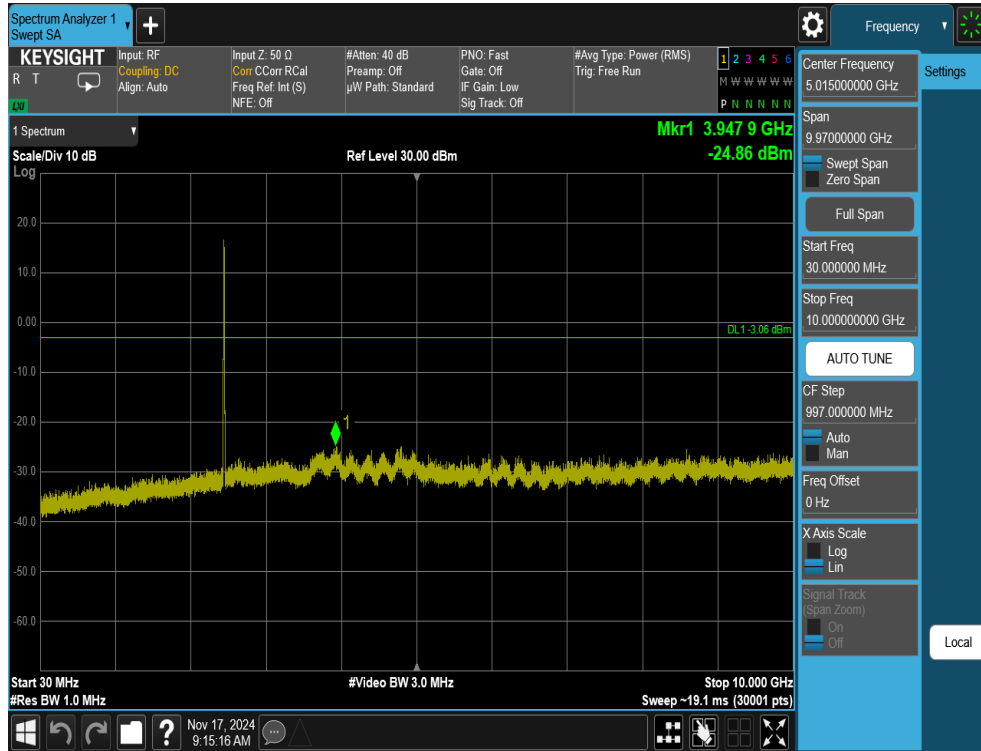
Plot 7-47. Conducted Spurious Plot Antenna 3a (802.11ax OFDMA – RU26 – Ch. 11)
