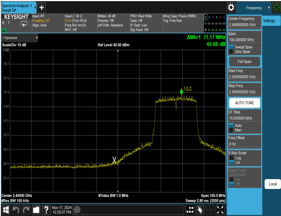
Plot 7-33. Band Edge Antenna 1a (802.11ax OFDMA – RU242 – Ch. 4)
