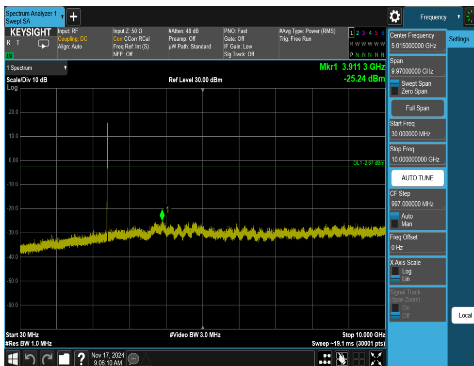
Plot 7-43. Conducted Spurious Plot Antenna 3a (802.11ax OFDMA – RU26 – Ch. 1)
