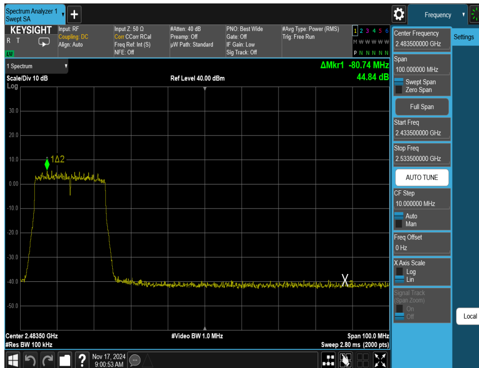
Plot 7-23. Band Edge Antenna 3a (802.11ax OFDMA – RU242 – Ch. 8)
