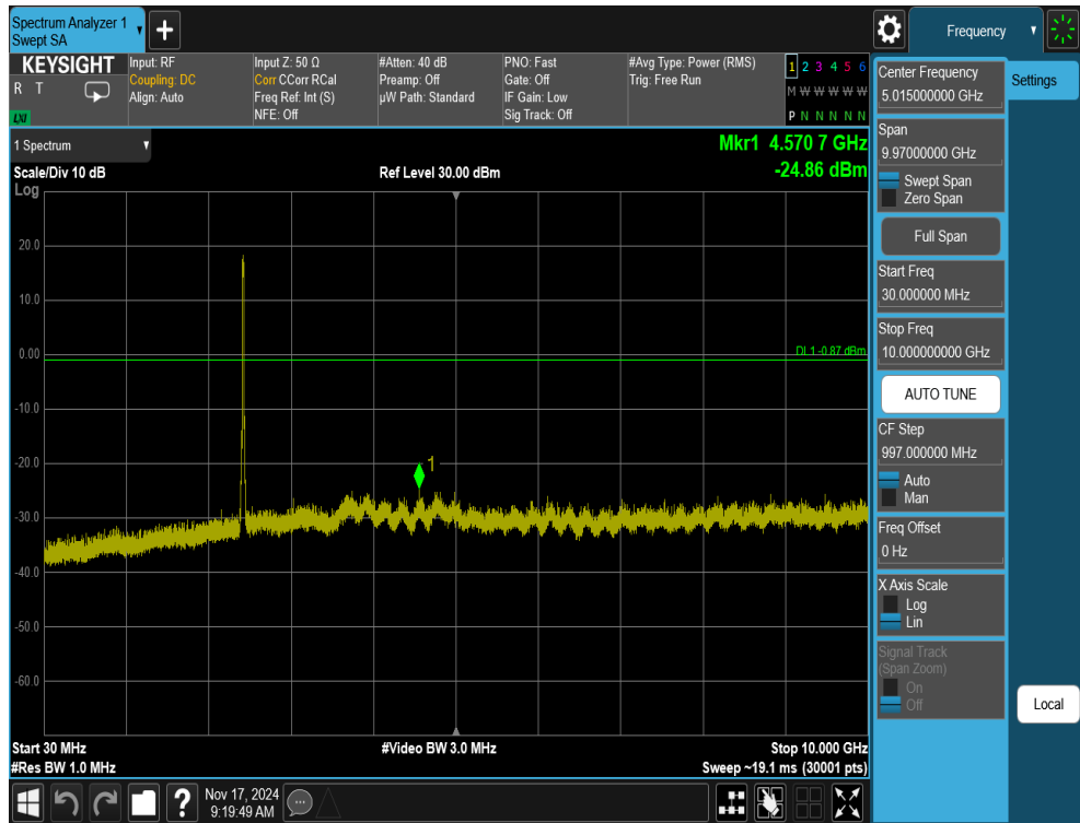
Plot 7-51. Conducted Spurious Plot Antenna 3a (802.11ax OFDMA – RU242 – Ch. 6)
