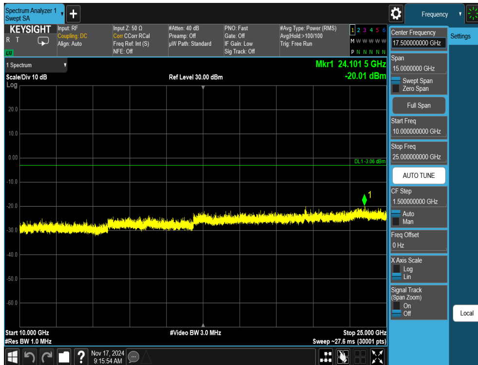
Plot 7-48. Conducted Spurious Plot Antenna 3a (802.11ax OFDMA – RU26 – Ch. 11)
