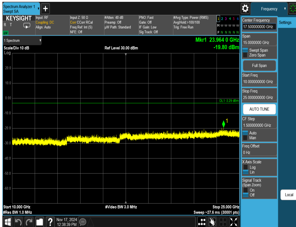
Plot 7-60. Conducted Spurious Plot Antenna 1a (802.11ax OFDMA – RU26 – Ch. 11)
