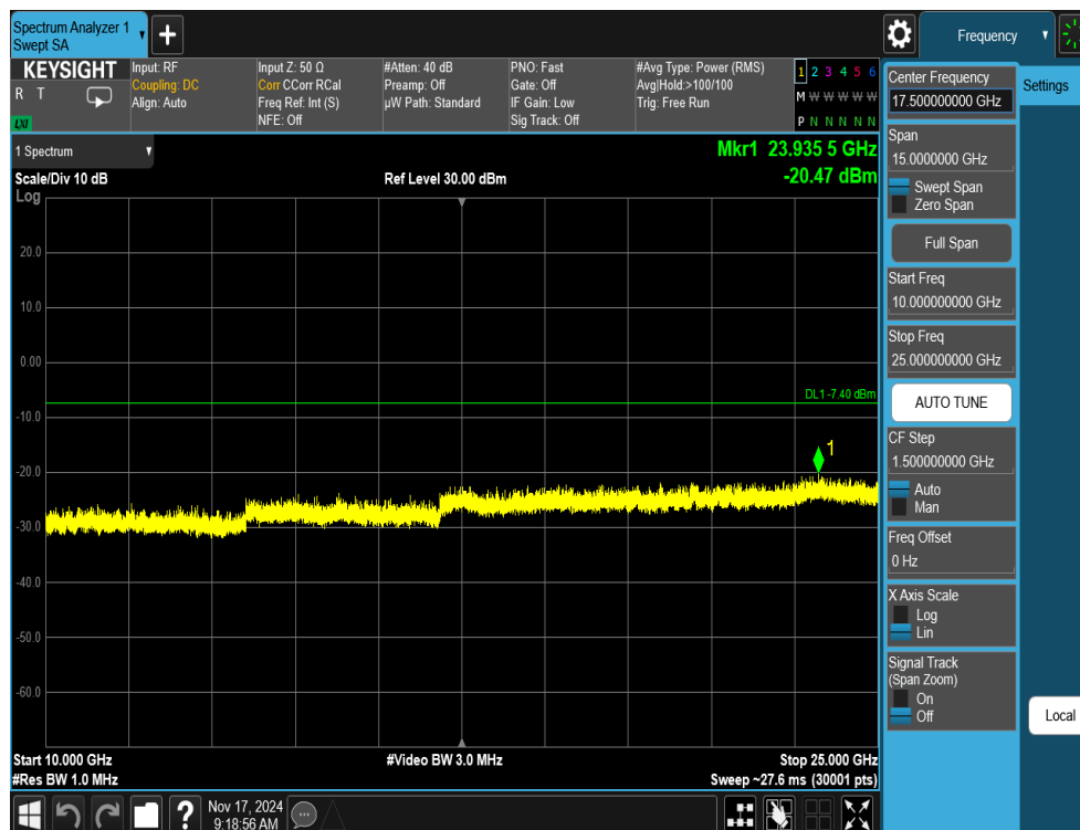
Plot 7-50. Conducted Spurious Plot Antenna 3a (802.11ax OFDMA – RU242 – Ch. 1)
