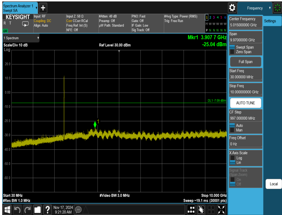
Plot 7-53. Conducted Spurious Plot Antenna 3a (802.11ax OFDMA – RU242 – Ch. 11)
