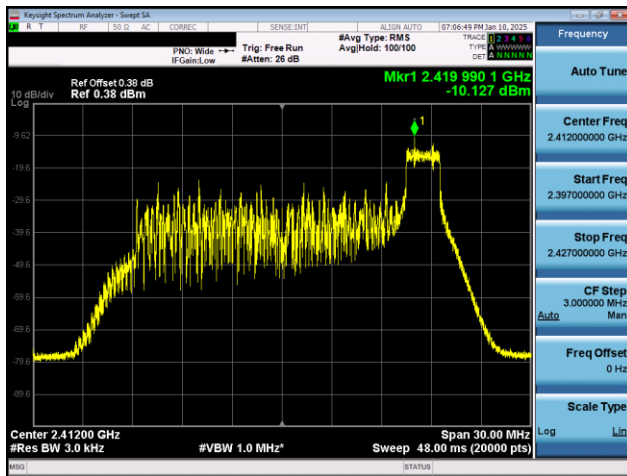
Plot 7-10. Power Spectral Density Plot Antenna 1a (802.11ax OFDMA – RU26 Index 8 – Ch. 1)
