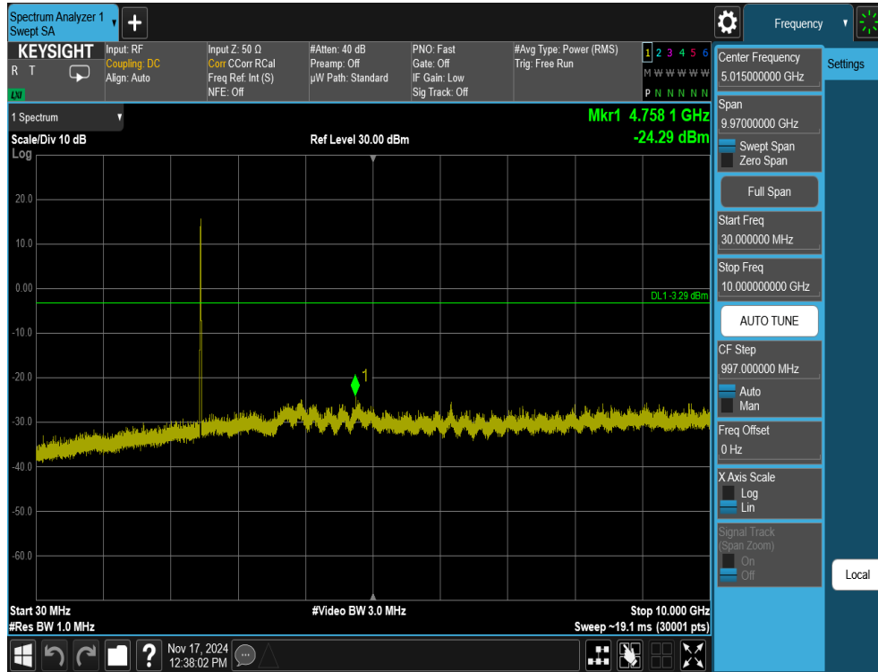
Plot 7-59. Conducted Spurious Plot Antenna 1a (802.11ax OFDMA – RU26 – Ch. 11)
