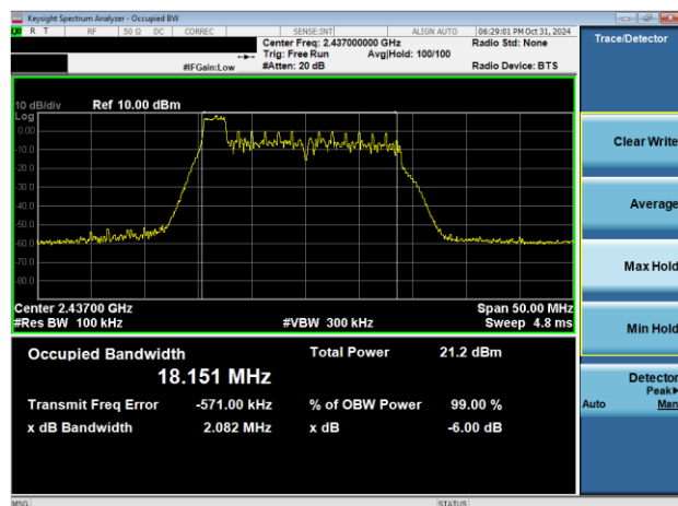
Plot 7-3. 6dB BW & 99% OBW Antenna 1a (802.11ax OFDMA – RU26 Index 0 – Ch. 6)
