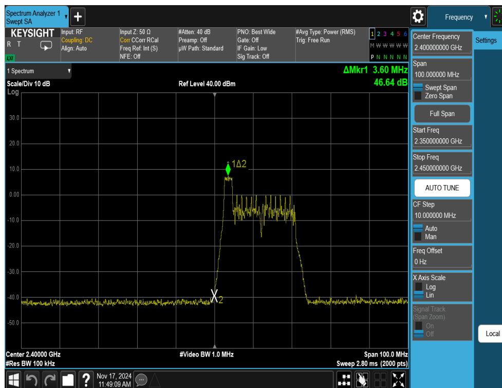
Plot 7-28. Band Edge Antenna 1a (802.11ax OFDMA – RU26 Index 0 – Ch. 1)
