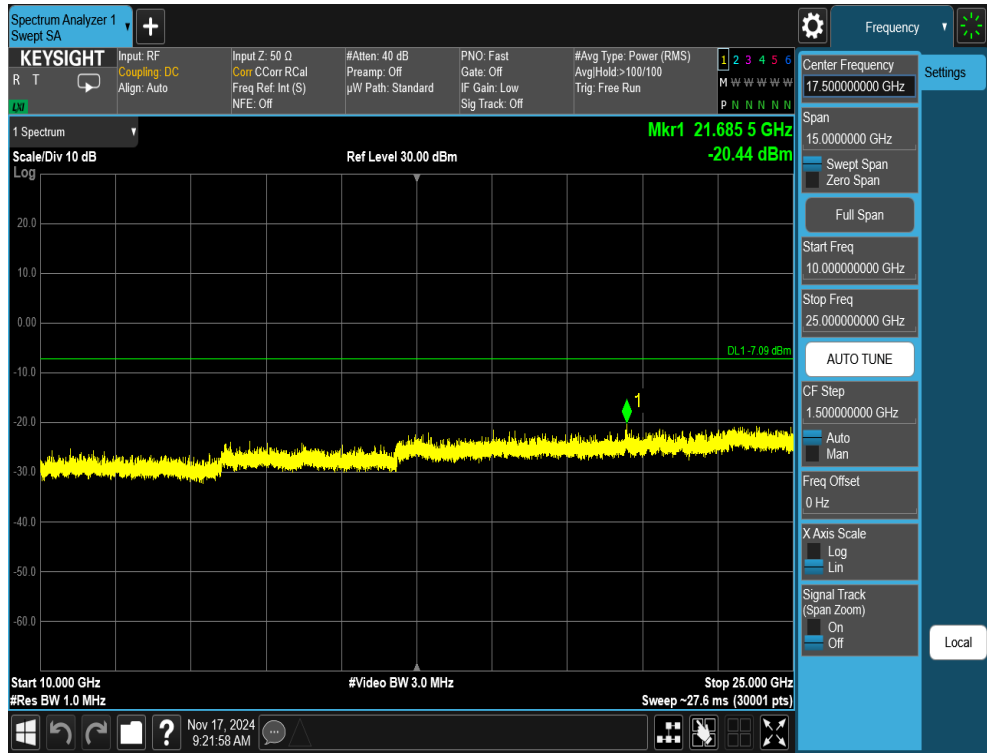
Plot 7-54. Conducted Spurious Plot Antenna 3a (802.11ax OFDMA – RU242 – Ch. 11)
