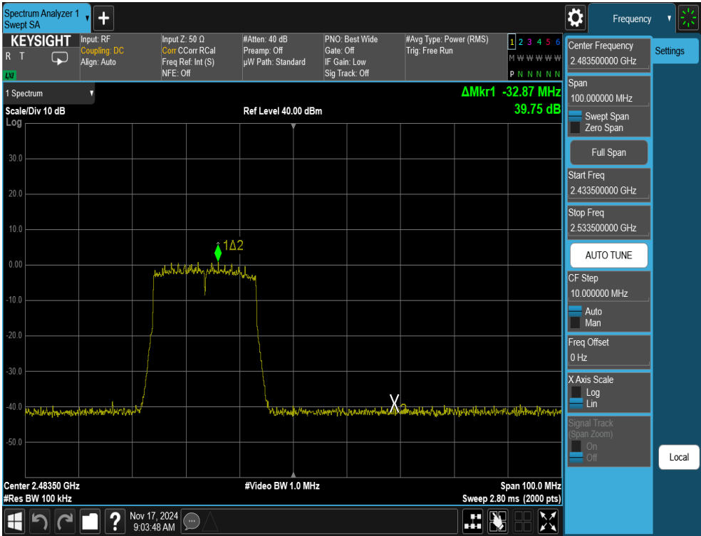
Plot 7-27. Band Edge Antenna 3a (802.11ax OFDMA – RU242 – Ch. 12)
