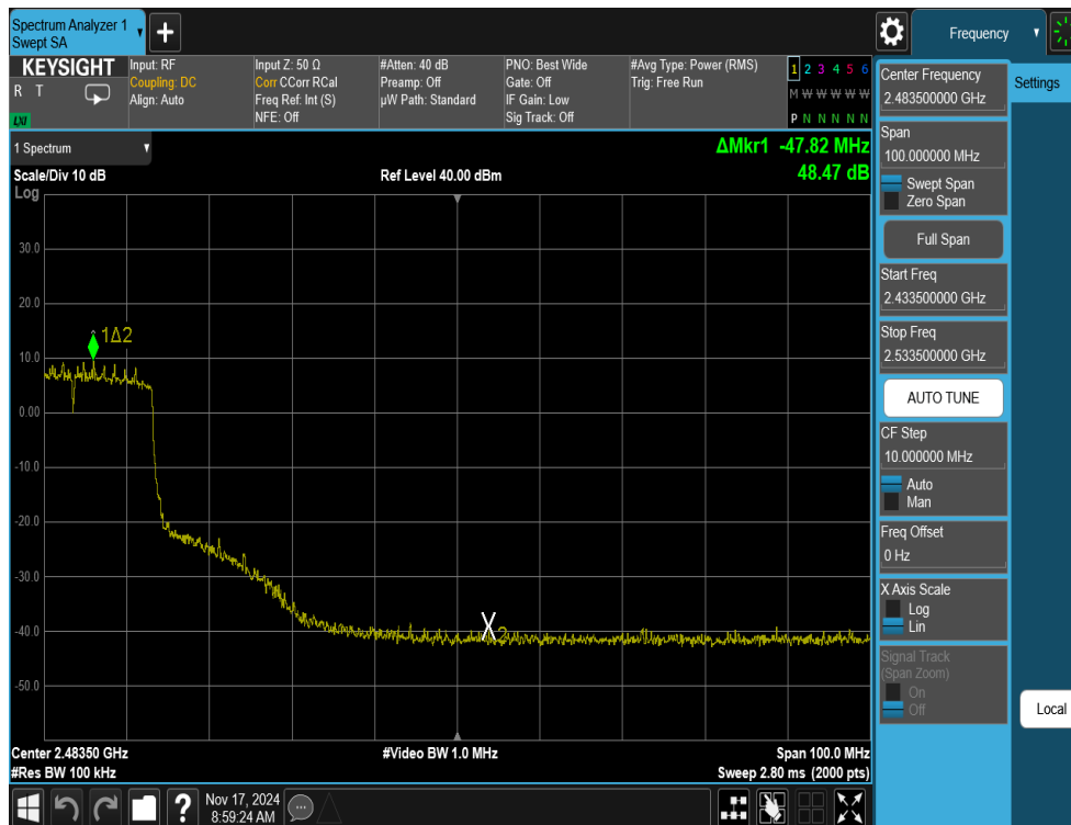
Plot 7-21. Band Edge Antenna 3a (802.11ax OFDMA – RU242 – Ch. 6(High Channel))
