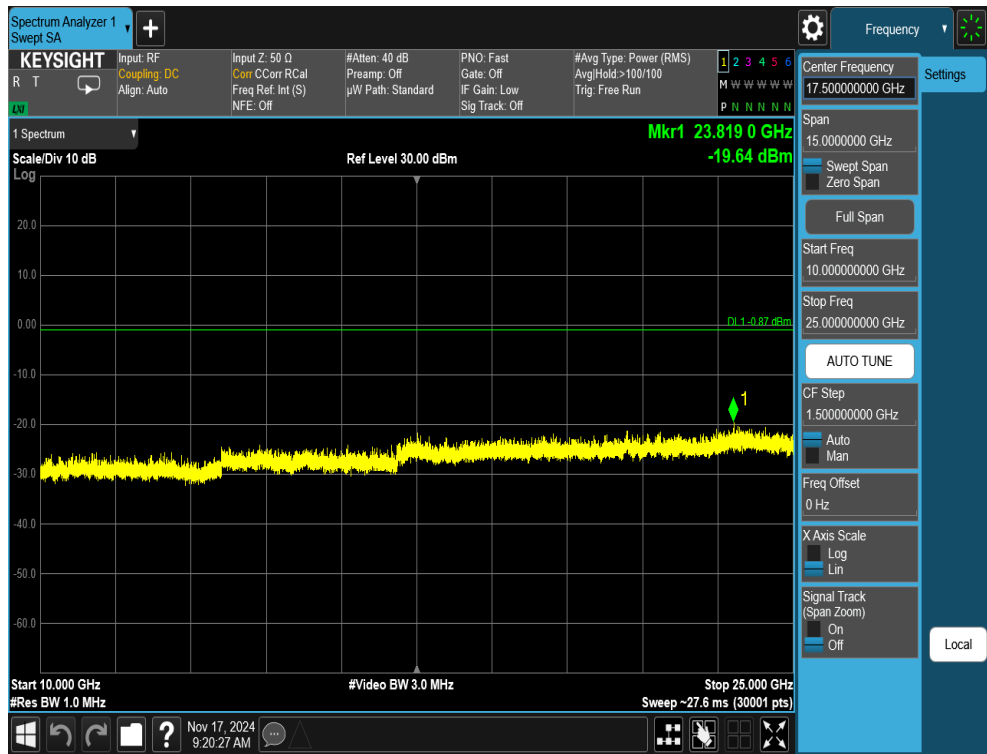
Plot 7-52. Conducted Spurious Plot Antenna 3a (802.11ax OFDMA – RU242 – Ch. 6)
