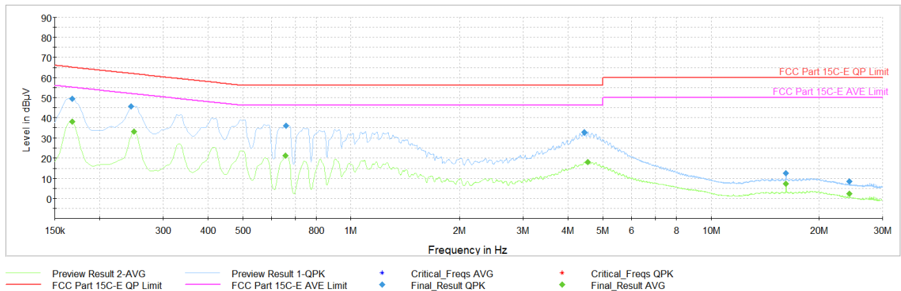
Plot 7-99. AC Line Conducted Plot with Bluetooth LE Tx BF (N, 1Mbps ePA – Ch.19, with AC/DC Adapter)
