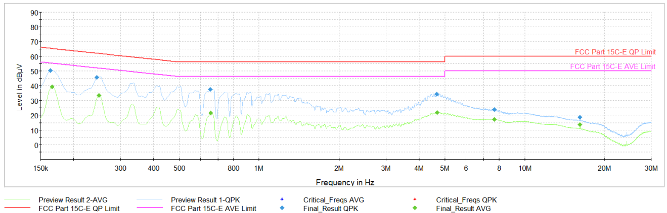
Plot 7-98. AC Line Conducted Plot with Bluetooth LE Tx BF (L1, 1Mbps ePA – Ch.19 with AC/DC Adapter)
