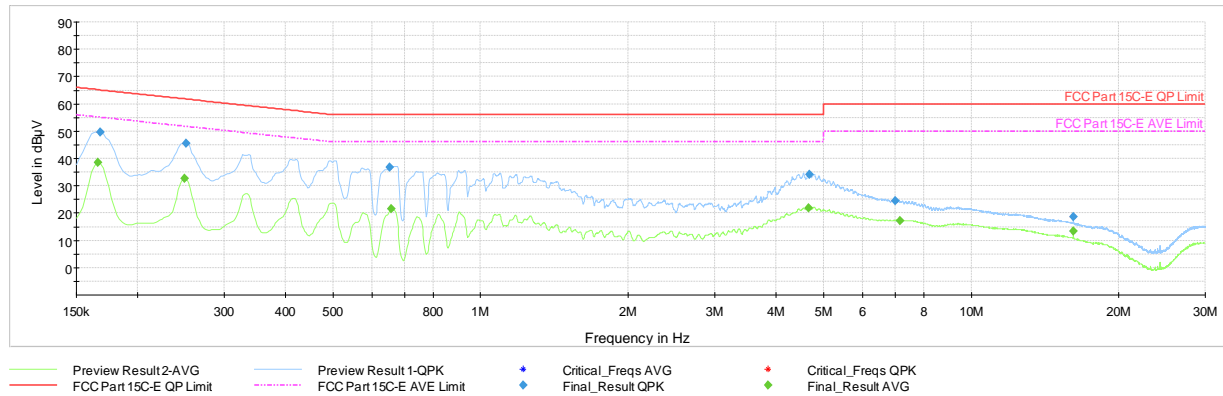
Plot 7-98. AC Line Conducted Plot with Bluetooth HDR Tx BF (L1, 4Mbps ePA - Ch.38 with AC/DC Adapter via USB-C cable with wire charger)
