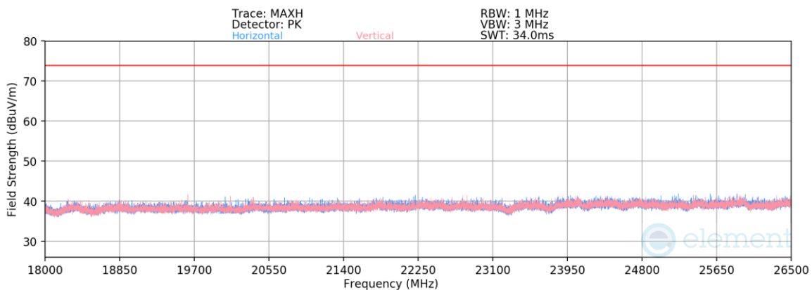
Plot 7-83. Radiated Spurious Emissions Above 18GHz TxBF (4Mbps, HDR4, ePA – Ch. 38)
