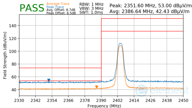
Plot 7-93. Radiated Restricted Lower Band Edge Measurement TxBF
