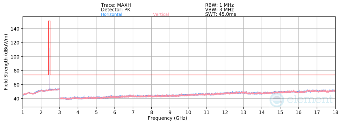
Plot 7-82. Radiated Spurious Emissions 1-18GHz TxBF (4Mbps, HDR4, ePA – Ch. 38)
