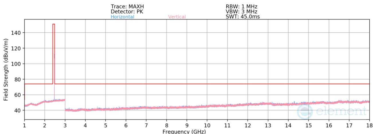
Plot 7-84. Radiated Spurious Emissions 1-18GHz TxBF (4Mbps, HDR4, ePA – Ch. 73)
