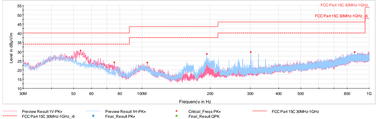
Plot 7-97. Radiated Spurious Emissions Below 1GHz TxBF (4Mbps, ePA – Ch.38 with AC/DC Adapter via USB-C cable with wire charger)
