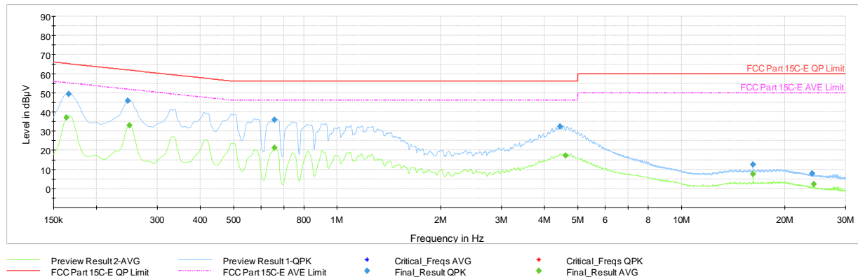
Plot 7-99. AC Line Conducted Plot with Bluetooth HDR (N, 4Mbps ePA - Ch.38 with AC/DC Adapter via USB-C cable with wire charger)
