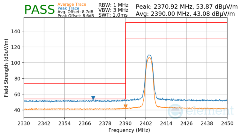
Plot 7-89. Radiated Restricted Lower Band Edge Measurement Antenna 1a
