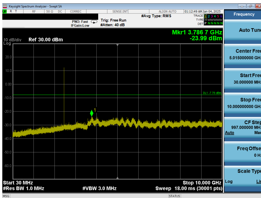
Plot 7-27. Conducted Spurious Antenna 3a (802.15.4, ePA – Ch. 25)
