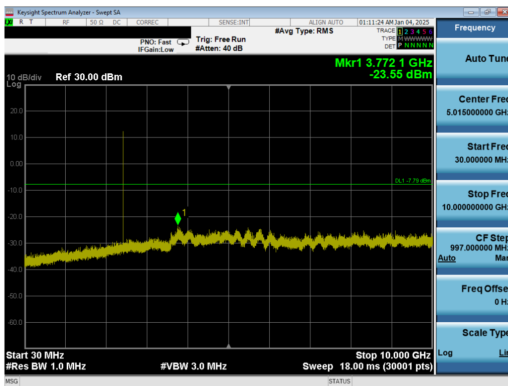
Plot 7-25. Conducted Spurious Antenna 3a (802.15.4, ePA – Ch. 18)
