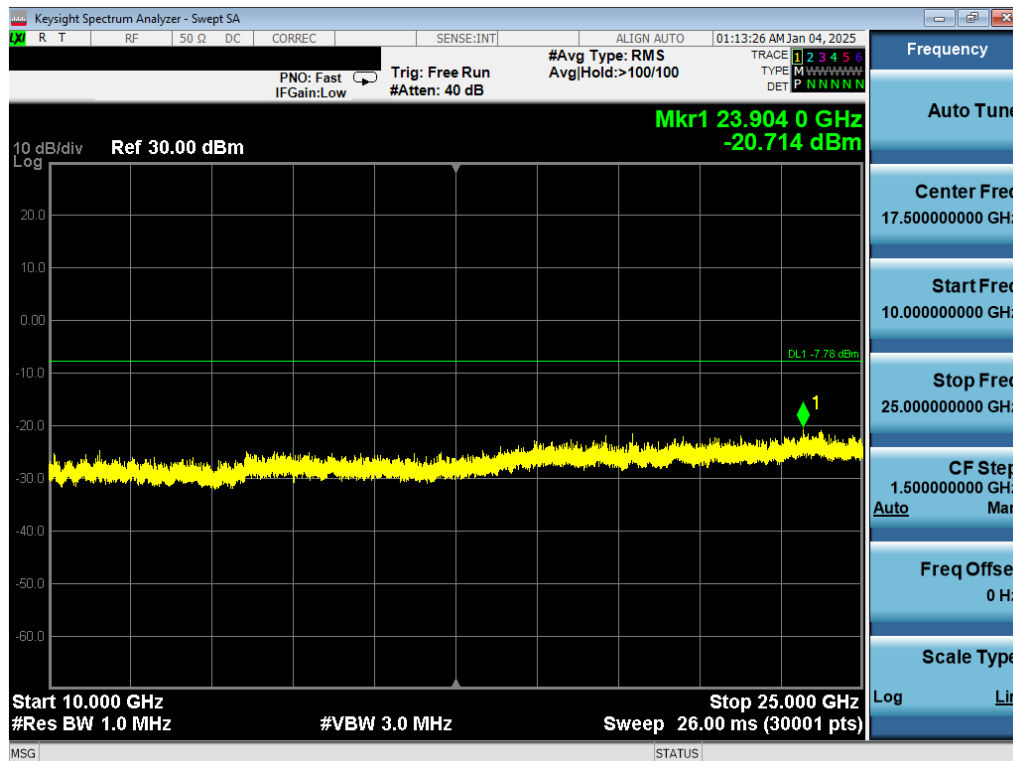
Plot 7-28. Conducted Spurious Antenna 3a (802.15.4, ePA – Ch. 25)
