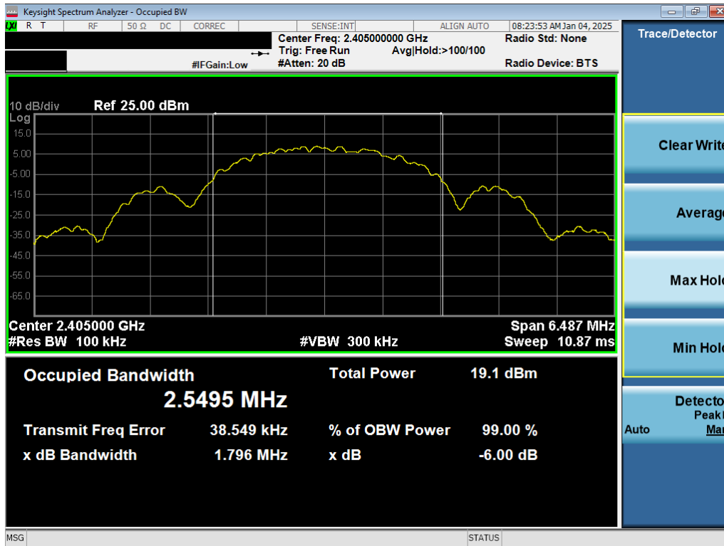
Plot 7-4. 6dB BW & 99% OBW Antenna 1a (802.15.4, Ch. 11)
