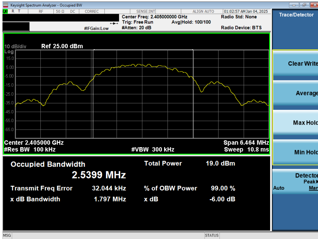
Plot 7-1. 6dB BW & 99% OBW Antenna 3a (802.15.4, Ch. 11)
