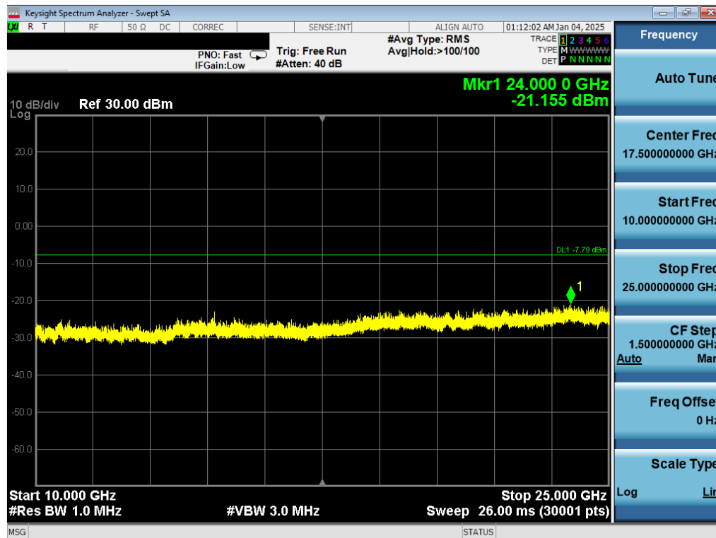
Plot 7-26. Conducted Spurious Antenna 3a (802.15.4, ePA – Ch. 18)
