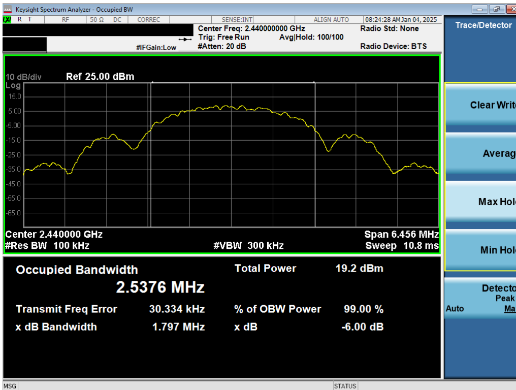
Plot 7-5. 6dB BW & 99% OBW Antenna 1a (802.15.4, Ch. 18)
