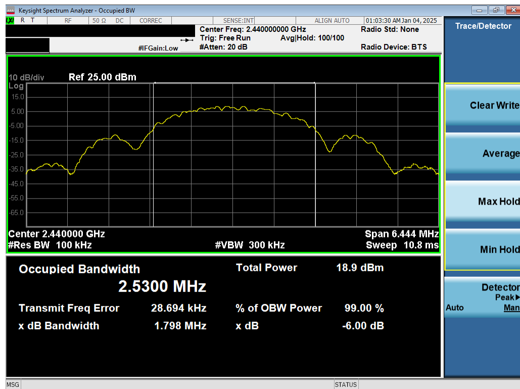
Plot 7-2. 6dB BW & 99% OBW Antenna 3a (802.15.4, Ch. 18)
