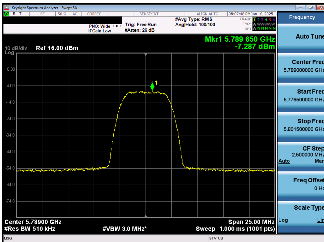
Plot 7-30. PSD Antenna 5T (NB UNII HDR8, iPA – 5789MHz)
