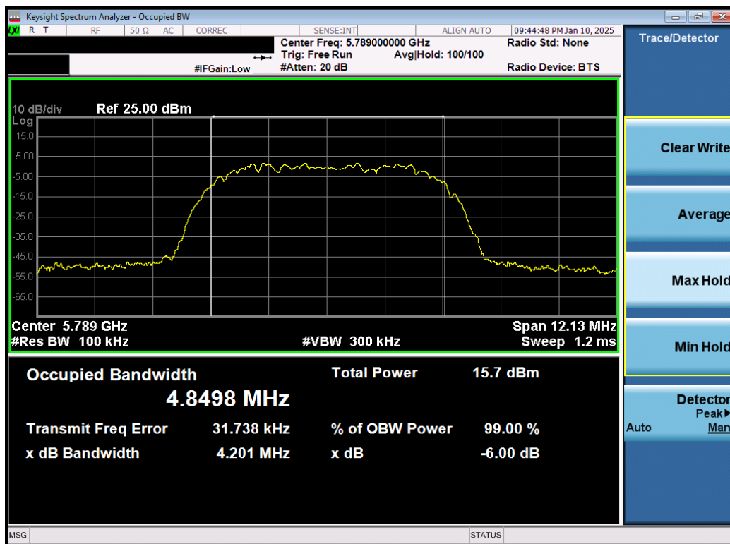
Plot 7-15. 6dB BW & 99% OBW Antenna 3b (NB UNII HDR8, 5789MHz)
