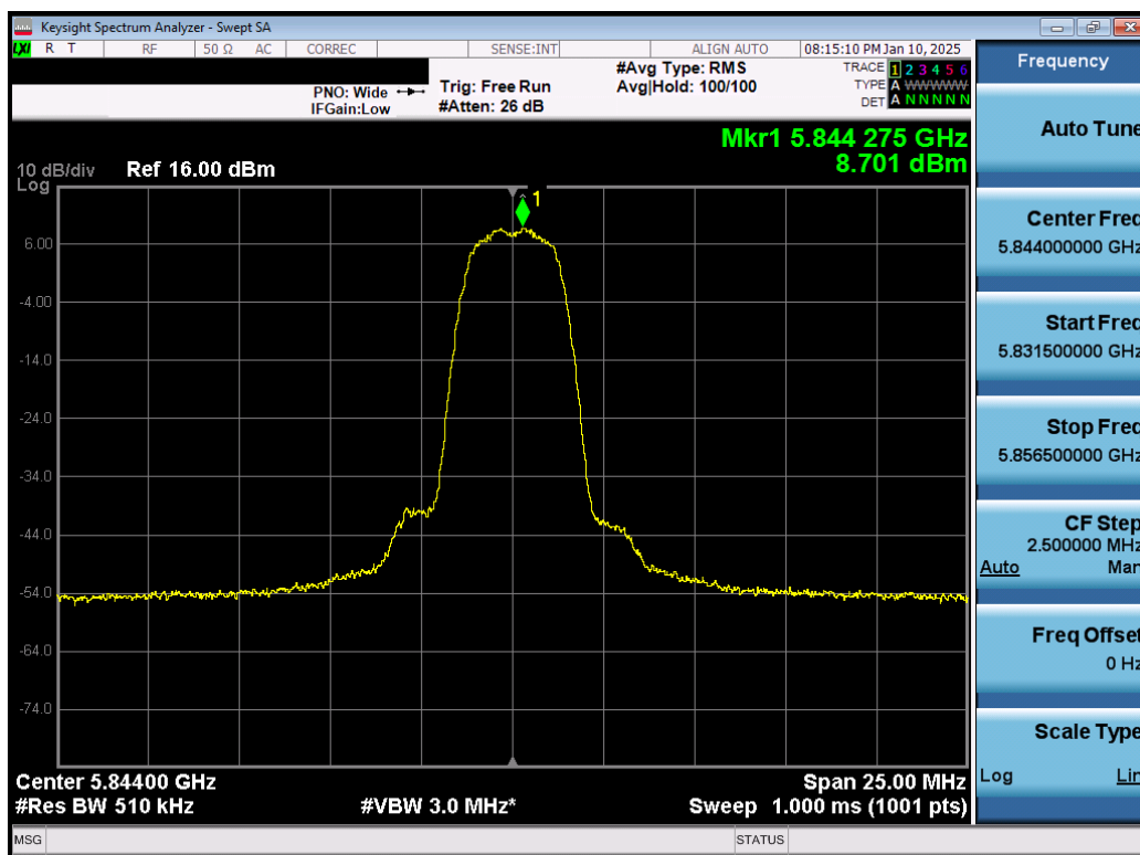
Plot 7-71. PSD TxBF Antenna 5T (NB UNII HDR4, ePA – 5844MHz)
