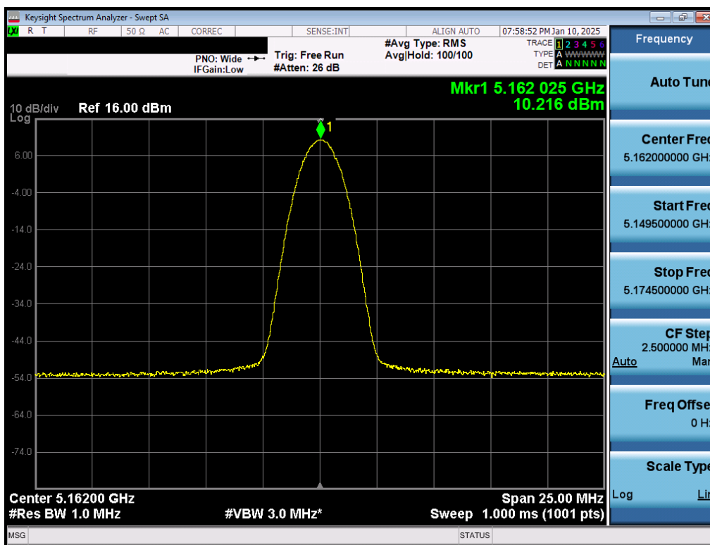
Plot 7-19. PSD Antenna 5T (NB UNII BDR, ePA – 5162MHz)
