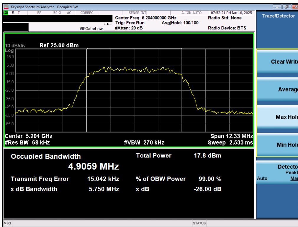
Plot 7-3. 26dB BW & 99% OBW Antenna 5T (NB UNII HDR8, ePA- 5204MHz)
