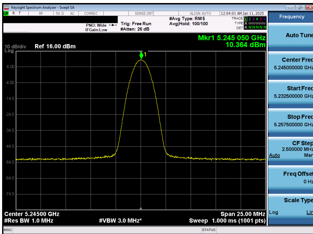
Plot 7-43. PSD Antenna 1b (NB UNII BDR, ePA – 5245MHz)
