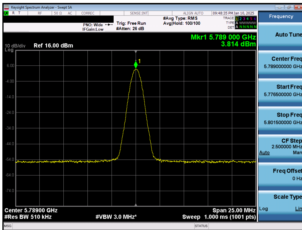
Plot 7-38. PSD Antenna 3b (NB UNII BDR, iPA – 5789MHz)
