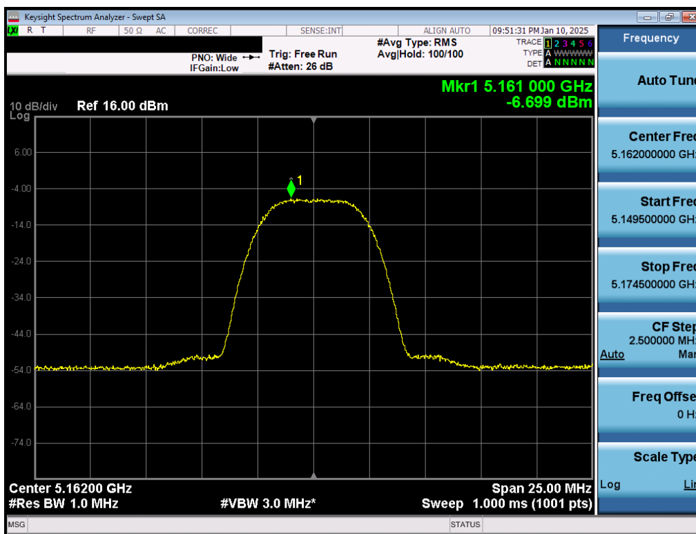
Plot 7-36. PSD Antenna 3b (NB UNII HDR8, iPA – 5162MHz)
