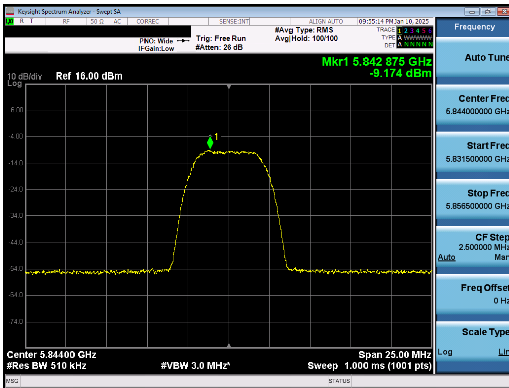
Plot 7-42. PSD Antenna 3b (NB UNII HDR8, iPA – 5844MHz)
