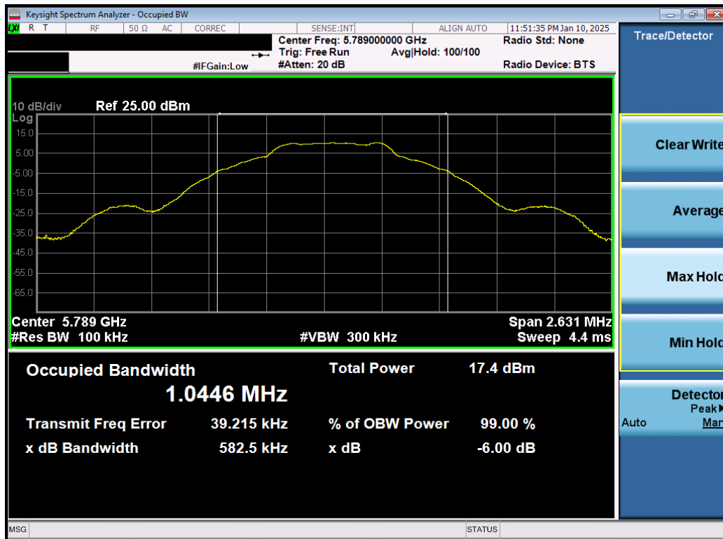
Plot 7-16. 6dB BW & 99% OBW Antenna 1b (NB UNII BDR, 5789MHz)
