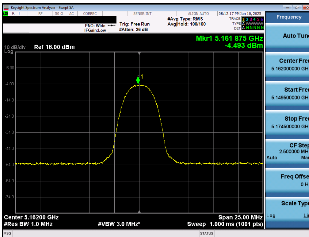
Plot 7-61. PSD TxBF Antenna 5T (NB UNII HDR4, iPA - 5162MHz)
