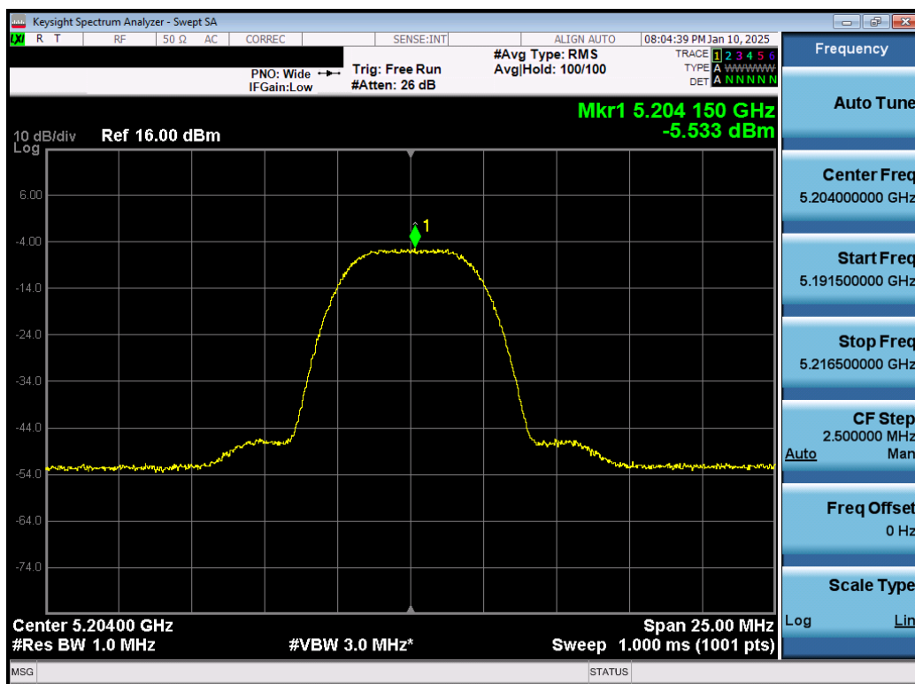
Plot 7-24. PSD Antenna 5T (NB UNII HDR8, iPA – 5204MHz)
