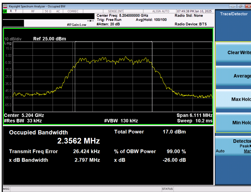
Plot 7-2. 26dB BW & 99% OBW Antenna 5T (NB UNII HDR4, ePA- 5204MHz)
