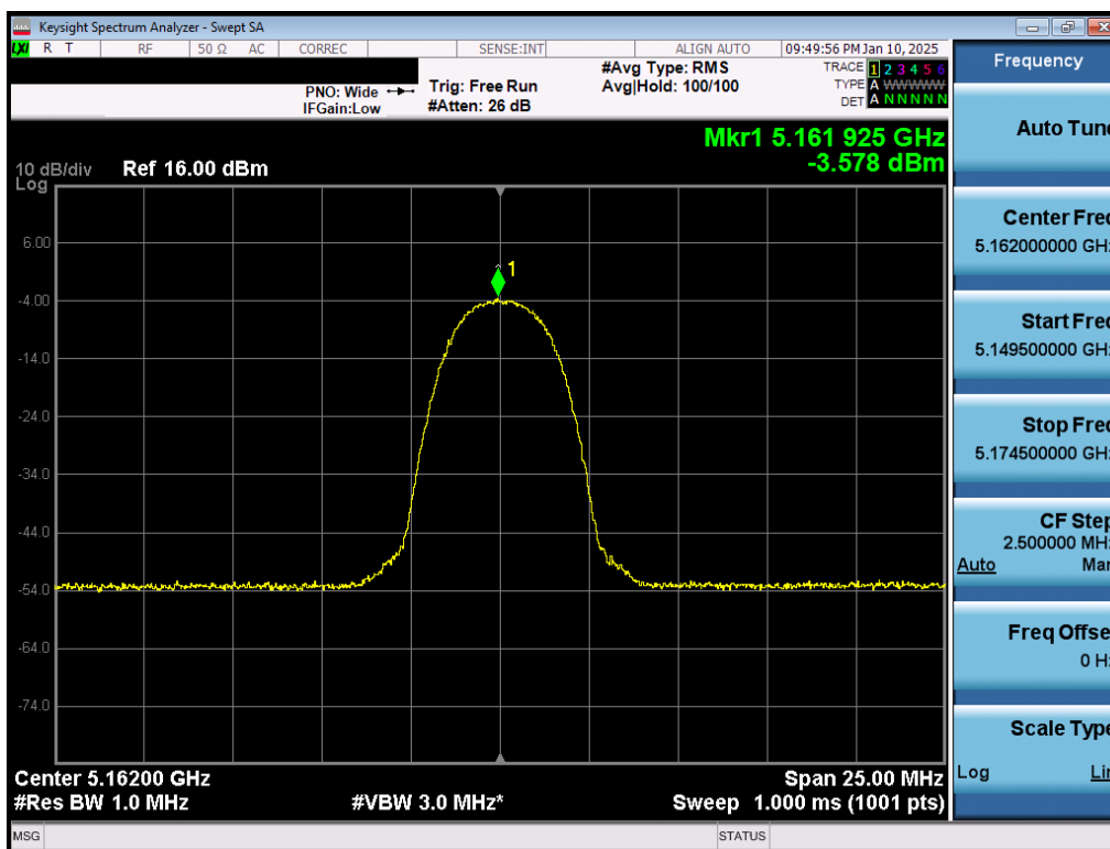
Plot 7-34. PSD Antenna 3b (NB UNII HDR4, iPA – 5162MHz)
