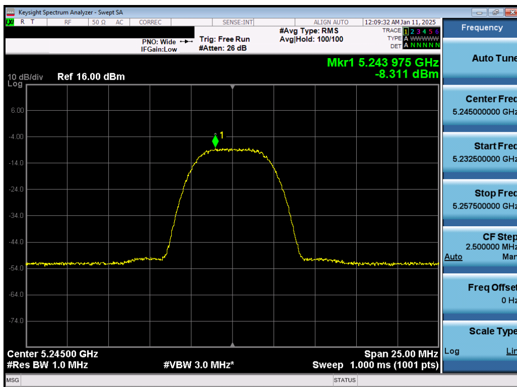
Plot 7-48. PSD Antenna 1b (NB UNII HDR8, iPA – 5245MHz)
