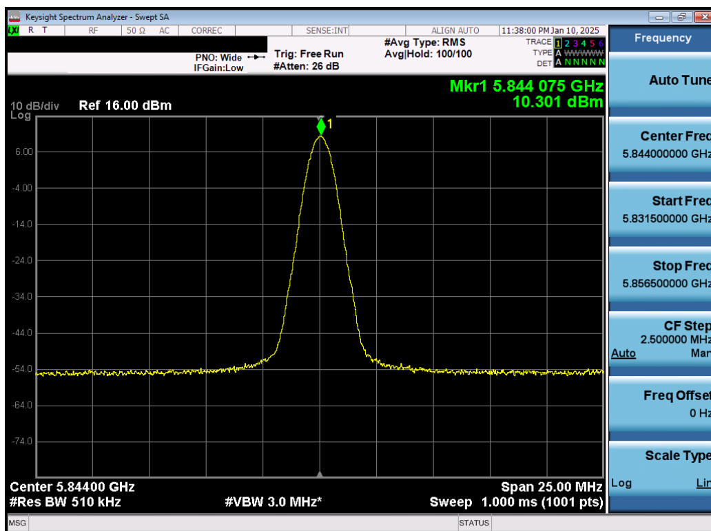
Plot 7-68. PSD TxBF Antenna 3b (NB UNII BDR, ePA – 5844MHz)
