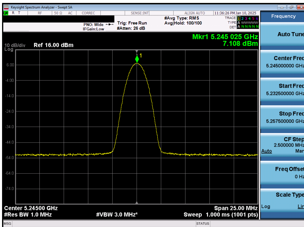
Plot 7-56. PSD TxBF Antenna 3b (NB UNII BDR, ePA – 5245MHz)
