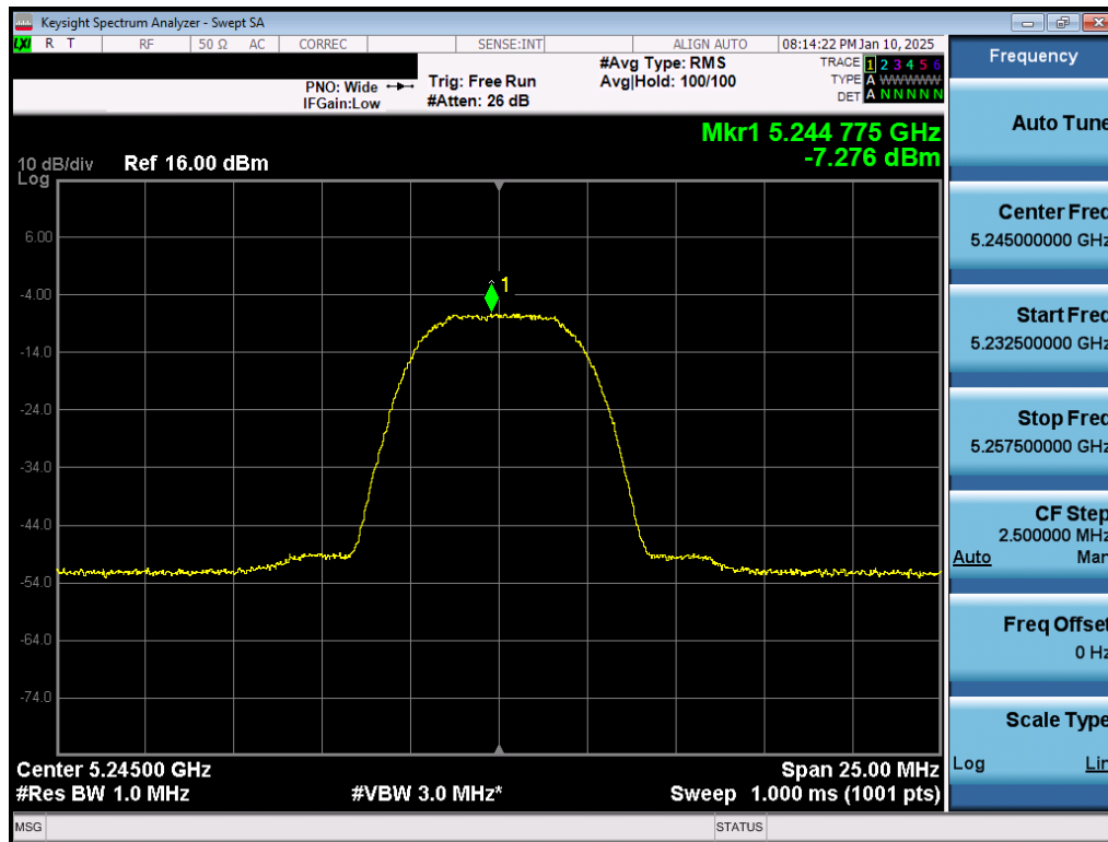
Plot 7-65. PSD Tx BF Antenna 5T (NB UNII HDR8, iPA – 5245MHz)
