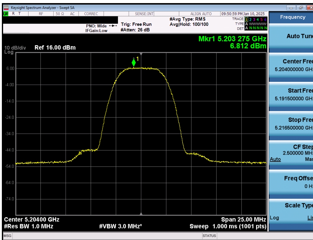
Plot 7-35. PSD Antenna 3b (NB UNII HDR8, ePA – 5204MHz)
