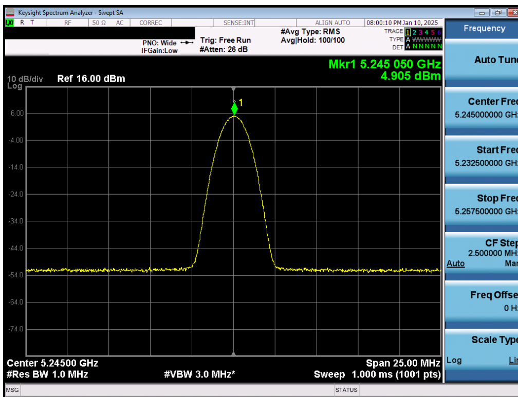
Plot 7-20. PSD Antenna 5T (NB UNII BDR, iPA – 5245MHz)
