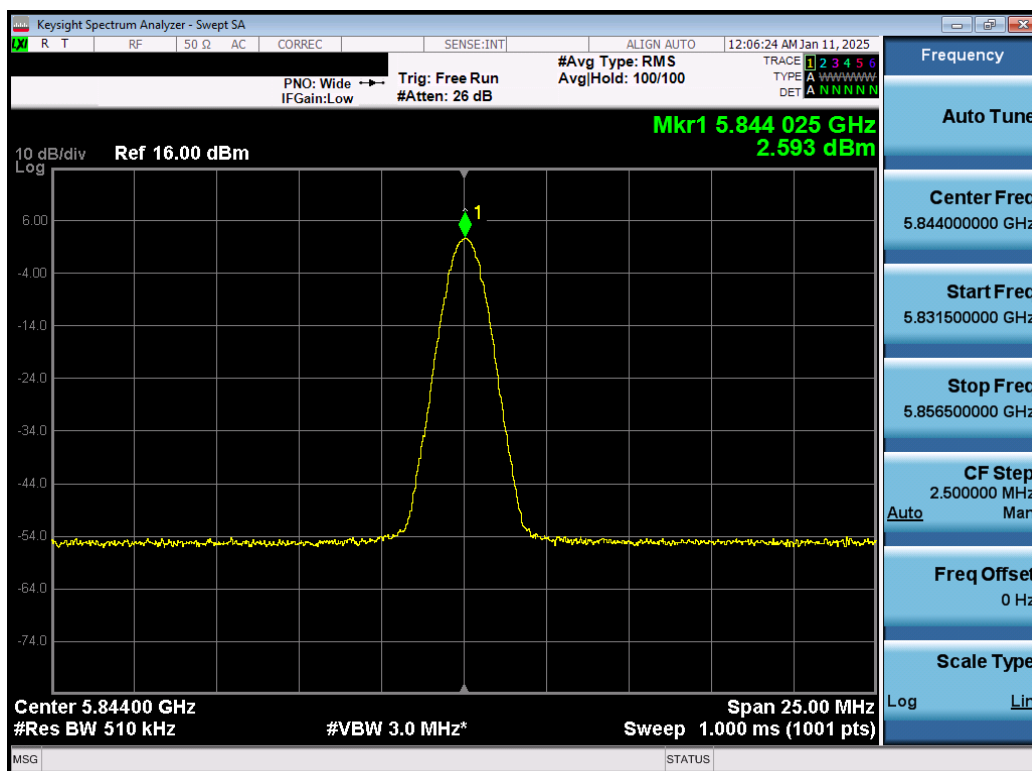
Plot 7-50. PSD Antenna 1b (NB UNII BDR, iPA – 5844MHz)
