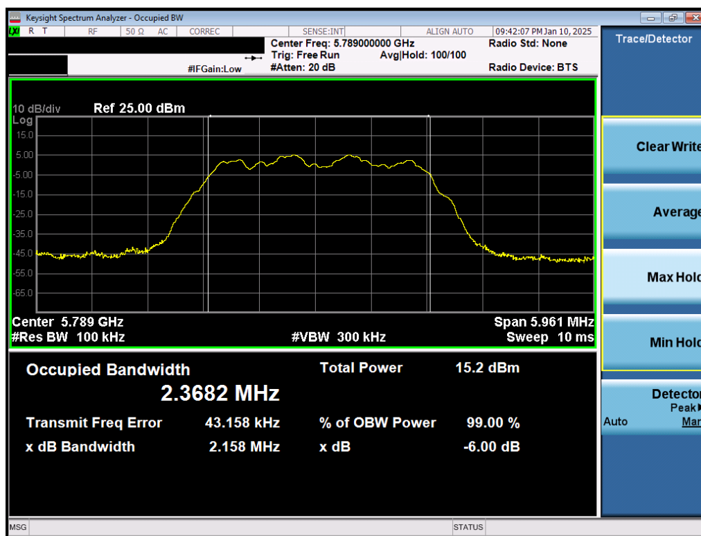
Plot 7-14. 6dB BW & 99% OBW Antenna 3b (NB UNII HDR4, 5789MHz)
