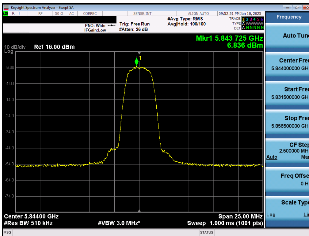
Plot 7-39. PSD Antenna 3b (NB UNII HDR4, ePA – 5844MHz)
