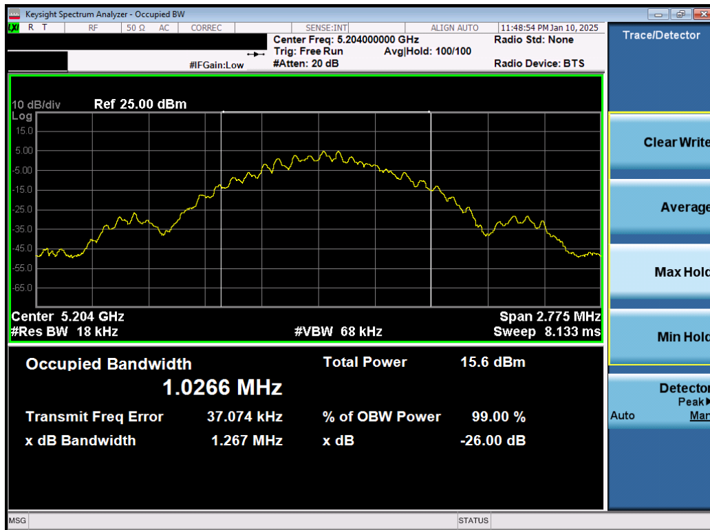
Plot 7-7. 26dB BW & 99% OBW Antenna 1b (BDR GFSK, ePA- 5204MHz)
