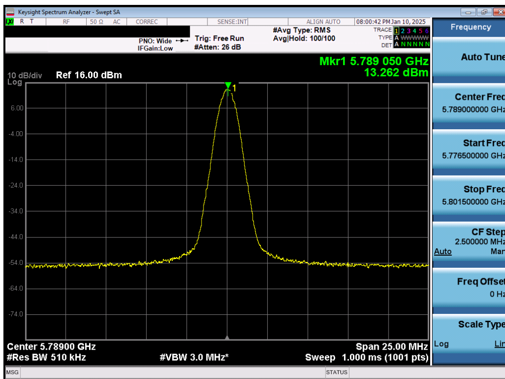
Plot 7-25. PSD Antenna 5T (NB UNII BDR, ePA – 5789MHz)
