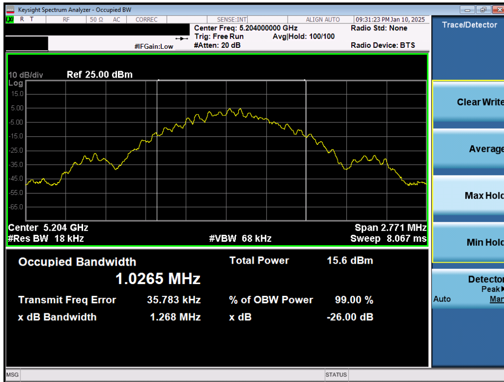
Plot 7-4. 26dB BW & 99% OBW Antenna 3b (BDR GFSK, ePA- 5204MHz)
