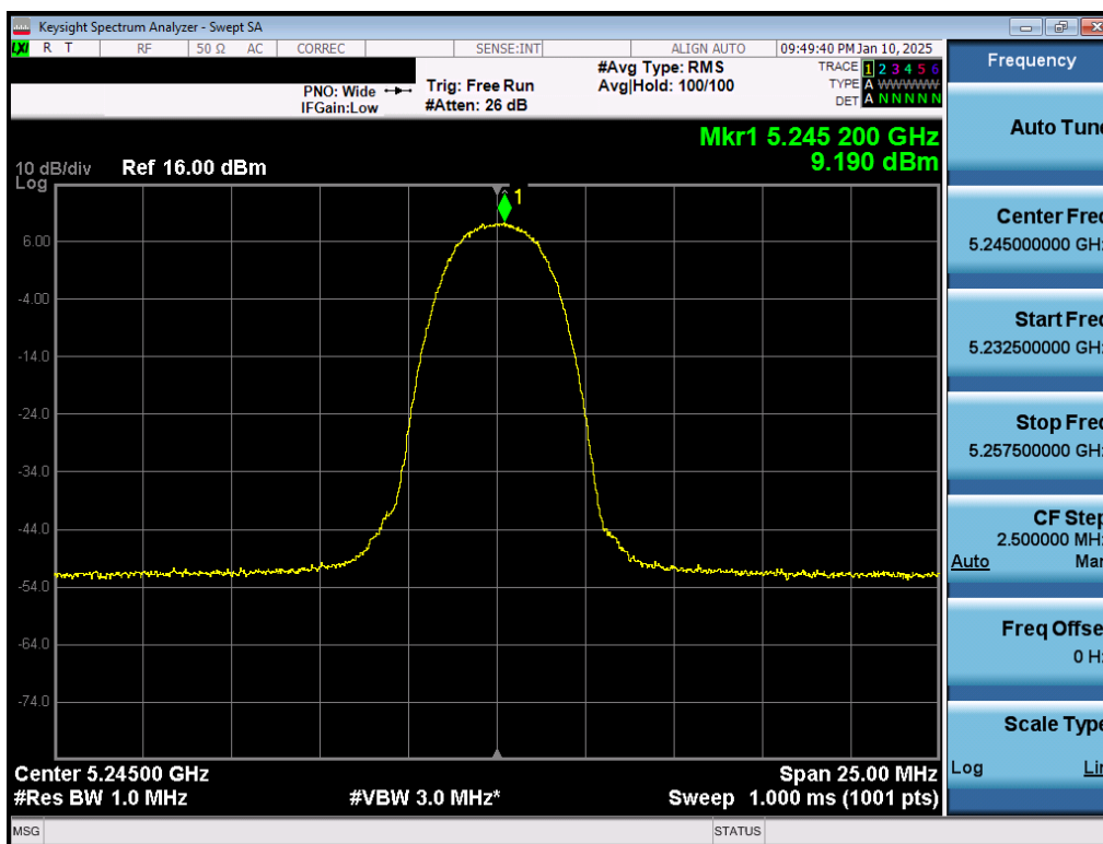
Plot 7-33. PSD Antenna 3b (NB UNII HDR4, ePA – 5245MHz)
