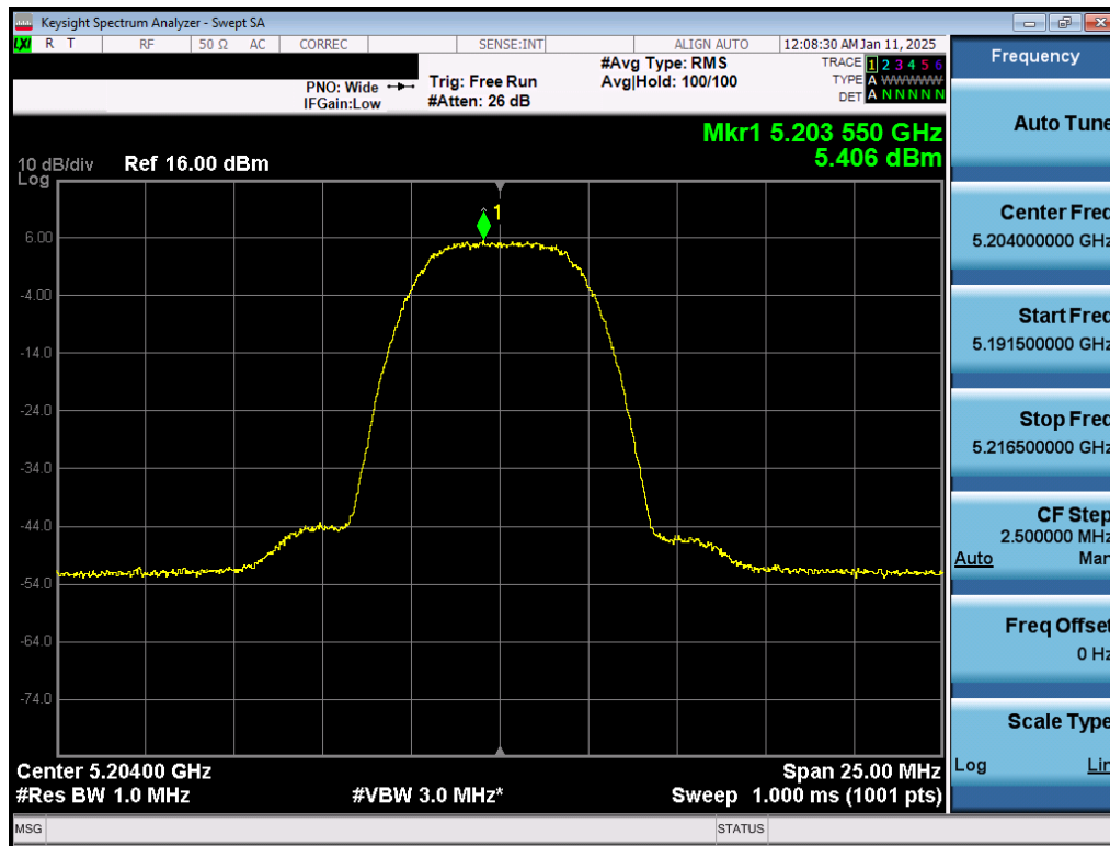
Plot 7-47. PSD Antenna 1b (NB UNII HDR8, ePA – 5204MHz)
