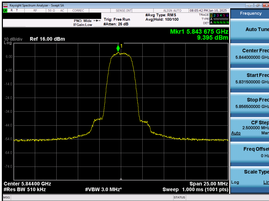
Plot 7-27. PSD Antenna 5T (NB UNII HDR4, ePA – 5844MHz)
