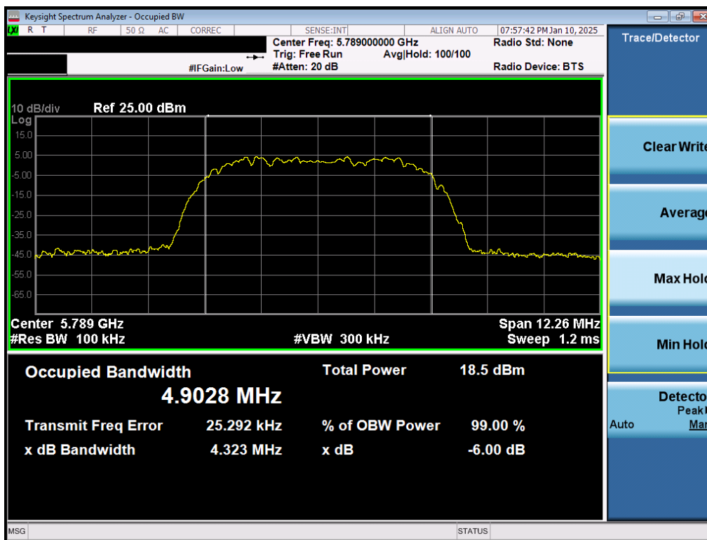
Plot 7-12. 6dB BW & 99% OBW Antenna 5T (NB UNII HDR8, 5789MHz)
