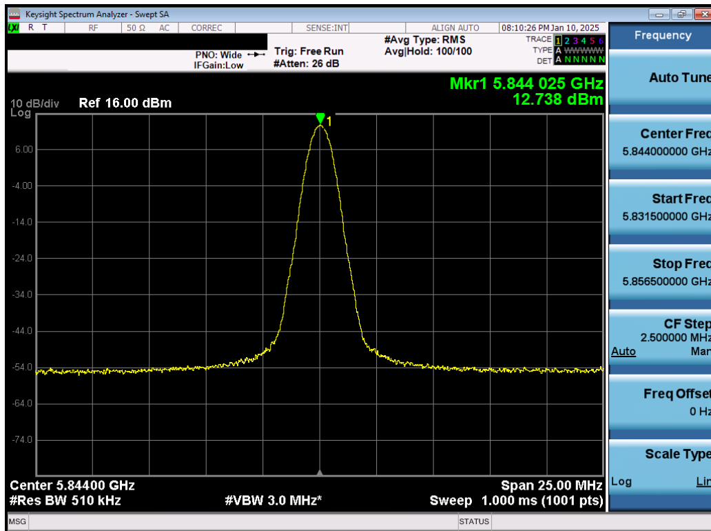
Plot 7-67. PSD TxBF Antenna 5T (NB UNII BDR, ePA – 5844MHz)
