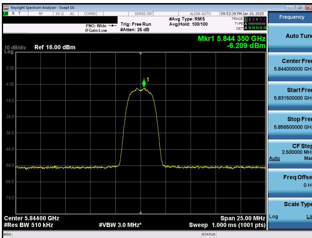
Plot 7-40. PSD Antenna 3b (NB UNII HDR4, iPA – 5844MHz)
