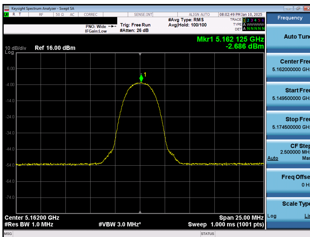
Plot 7-22. PSD Antenna 5T (NB UNII HDR4, iPA – 5162MHz)
