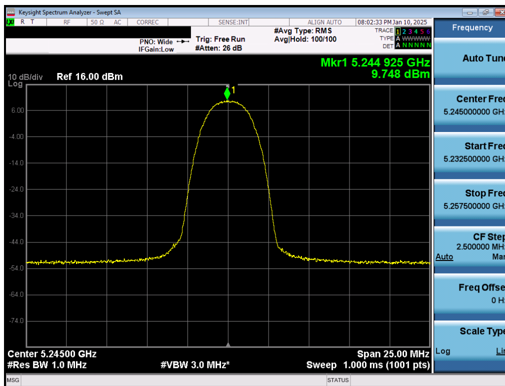
Plot 7-21. PSD Antenna 5T (NB UNII HDR4, ePA – 5245MHz)
