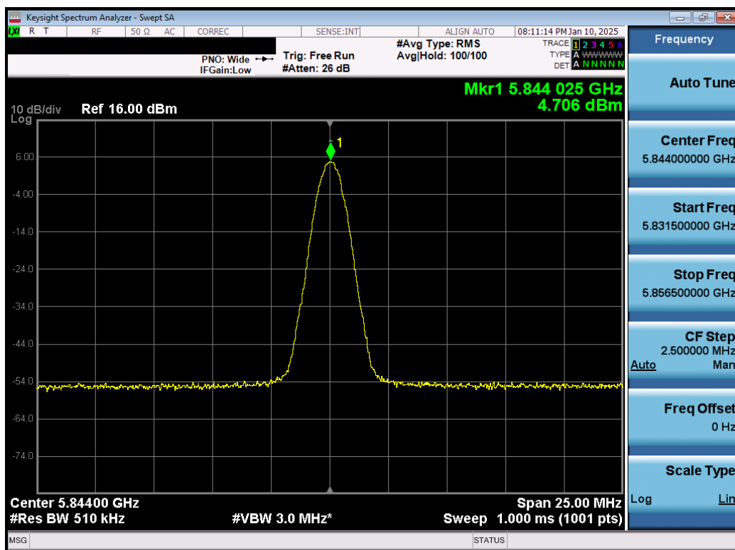
Plot 7-69. PSD TxBF Antenna 5T (NB UNII BDR, iPA - 5844MHz)
