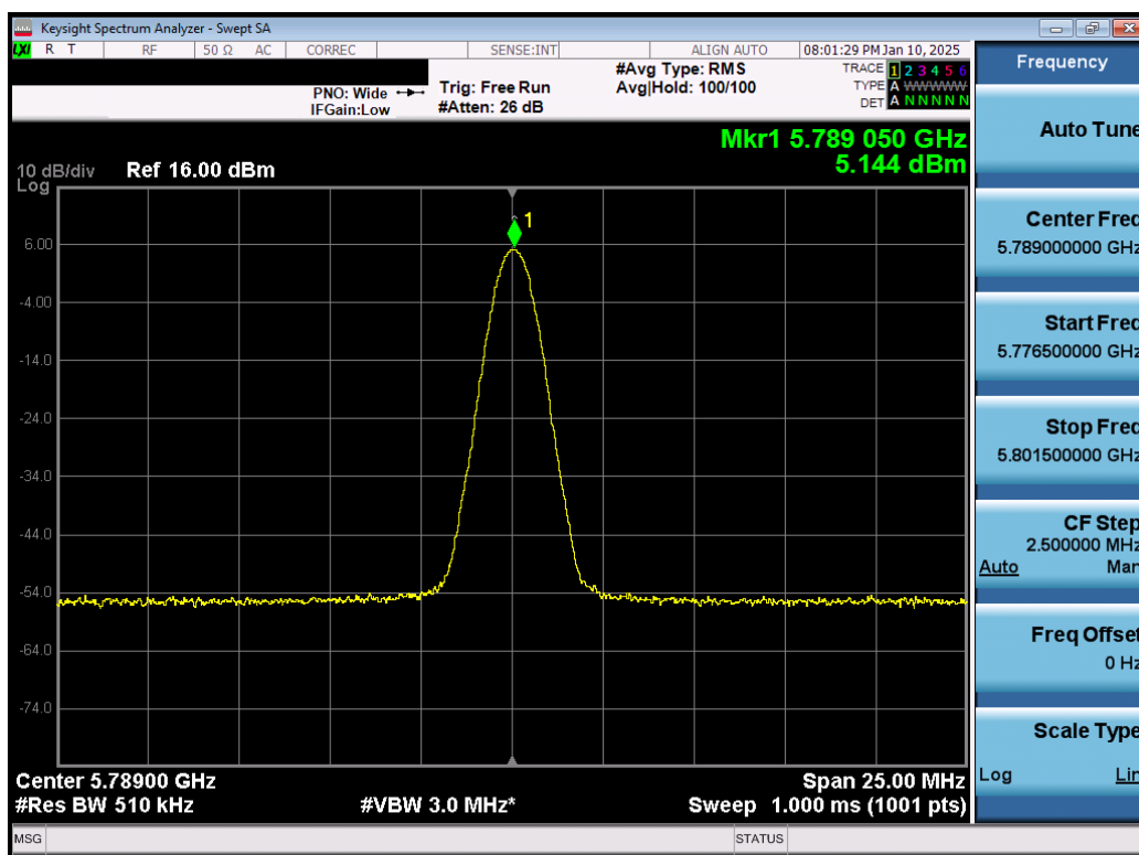
Plot 7-26. PSD Antenna 5T (NB UNII BDR, iPA – 5789MHz)
