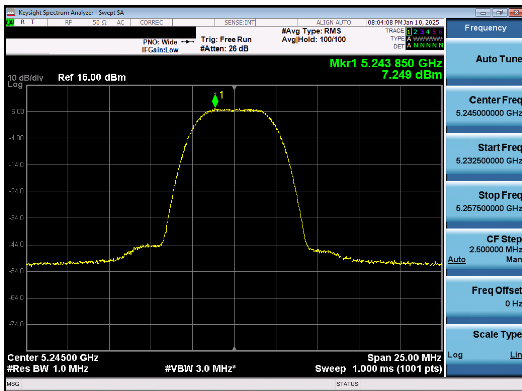
Plot 7-23. PSD Antenna 5T (NB UNII HDR8, ePA – 5245MHz)
