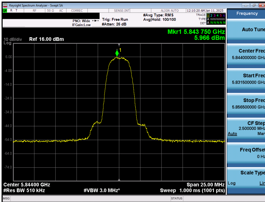
Plot 7-51. PSD Antenna 1b (NB UNII HDR4, ePA - 5844MHz)
