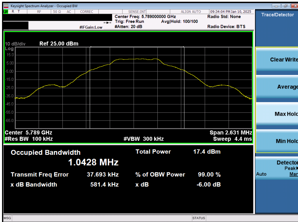
Plot 7-13. 6dB BW & 99% OBW Antenna 3b (NB UNII BDR, 5789MHz)
