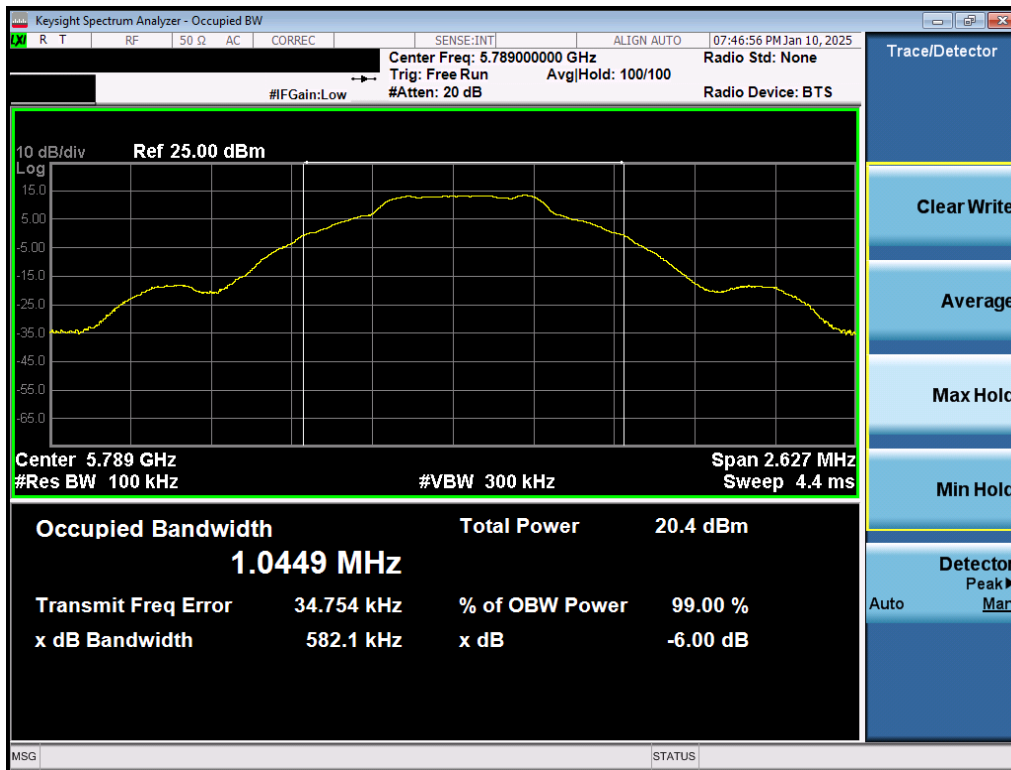
Plot 7-10. 6dB BW & 99% OBW Antenna 5T (NB UNII BDR, 5789MHz)
