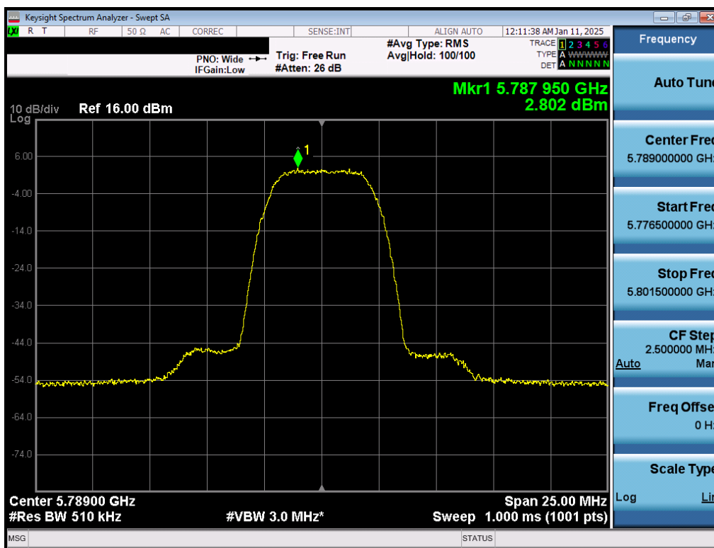
Plot 7-53. PSD Antenna 1b (NB UNII HDR8, ePA – 5789MHz)
