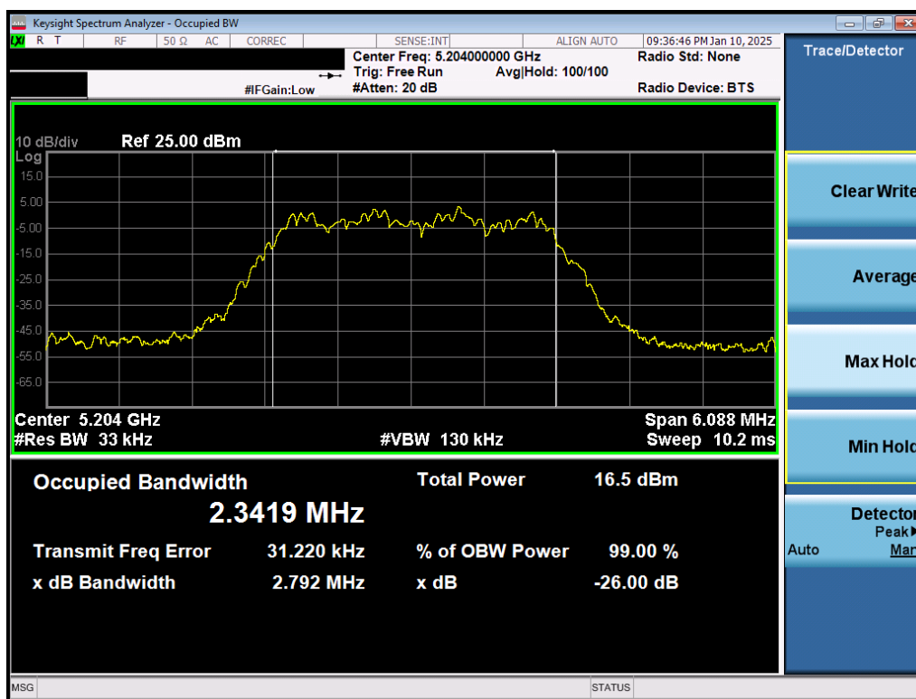
Plot 7-5. 26dB BW & 99% OBW Antenna 3b (NB UNII HDR4, ePA- 5204MHz)
