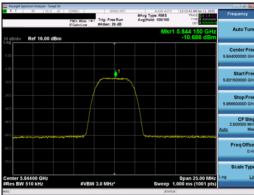
Plot 7-54. PSD Antenna 1b (NB UNII HDR8, iPA – 5844MHz)
