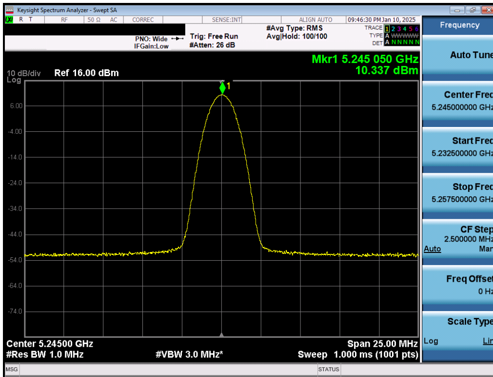
Plot 7-31. PSD Antenna 3b (NB UNII BDR, ePA – 5245MHz)
