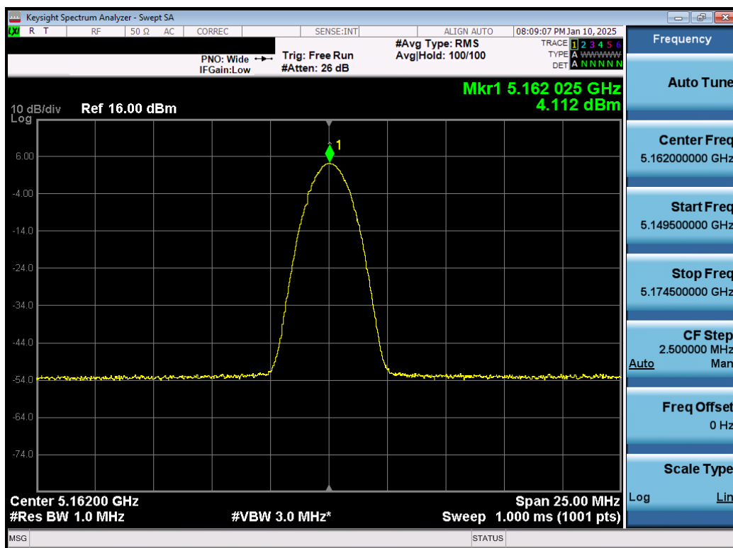
Plot 7-57. PSD TxBF Antenna 5T (NB UNII BDR, iPA – 5162MHz)
