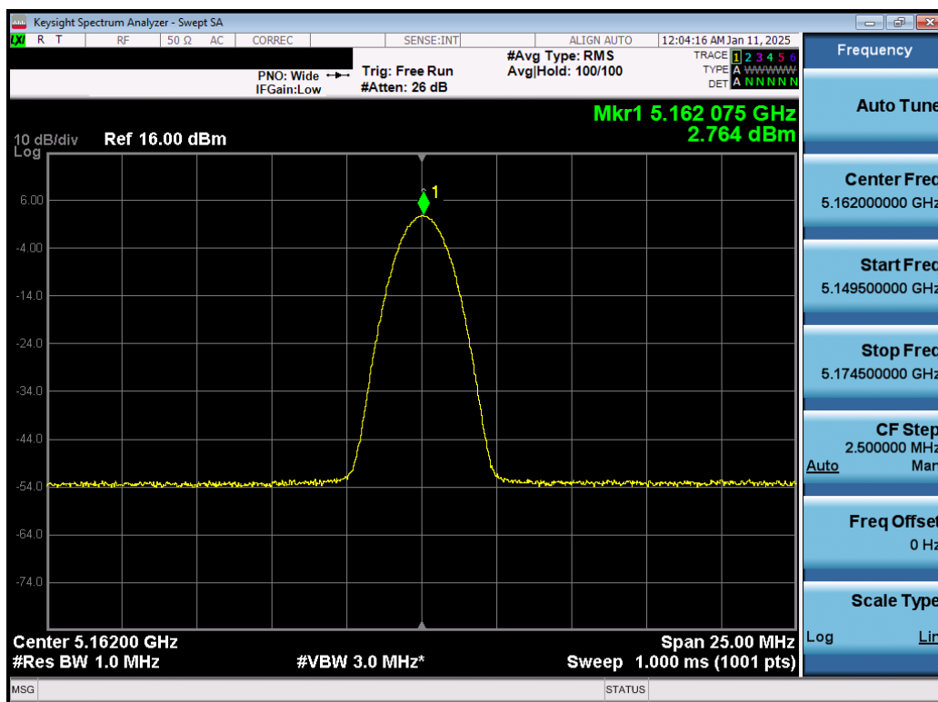
Plot 7-44. PSD Antenna 1b (NB UNII BDR, iPA – 5162MHz)
