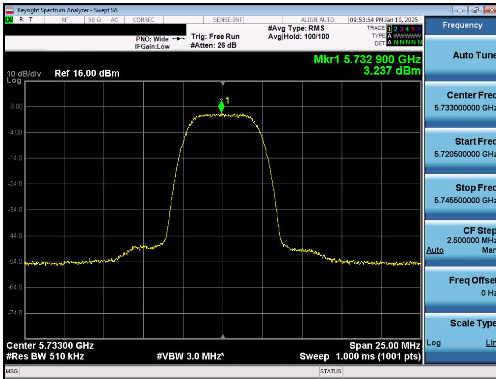
Plot 7-41. PSD Antenna 3b (NB UNII HDR8, ePA – 5733MHz)
