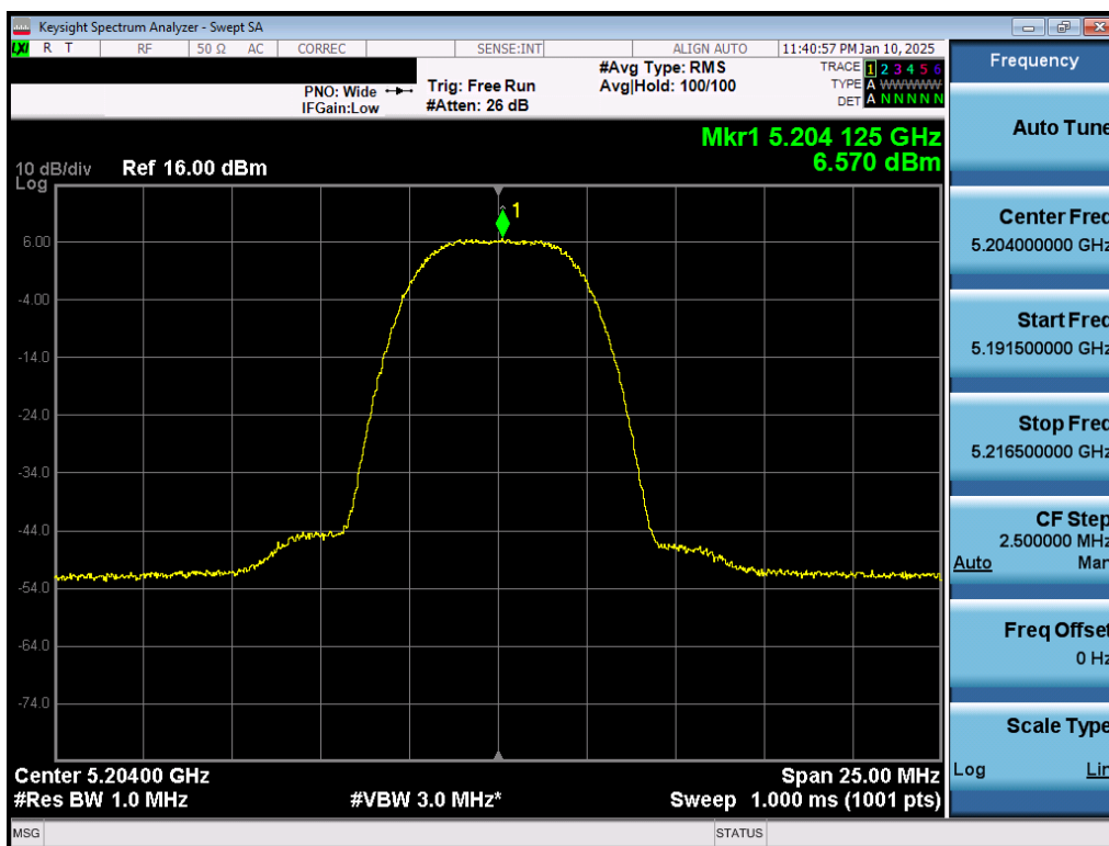
Plot 7-64. PSD Tx BF Antenna 3b (NB UNII HDR8, ePA – 5204MHz)
