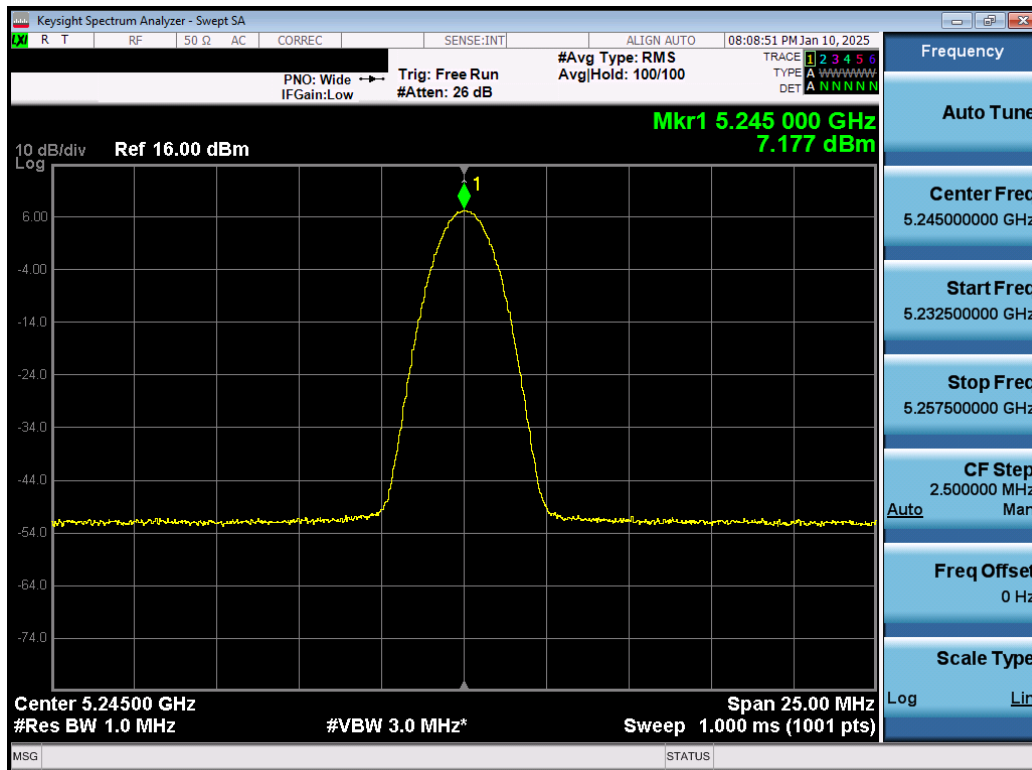
Plot 7-55. PSD TxBF Antenna 5T (NB UNII BDR, ePA – 5245MHz)
