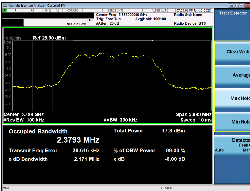
Plot 7-11. 6dB BW & 99% OBW Antenna 5T (NB UNII HDR4, 5789MHz)
