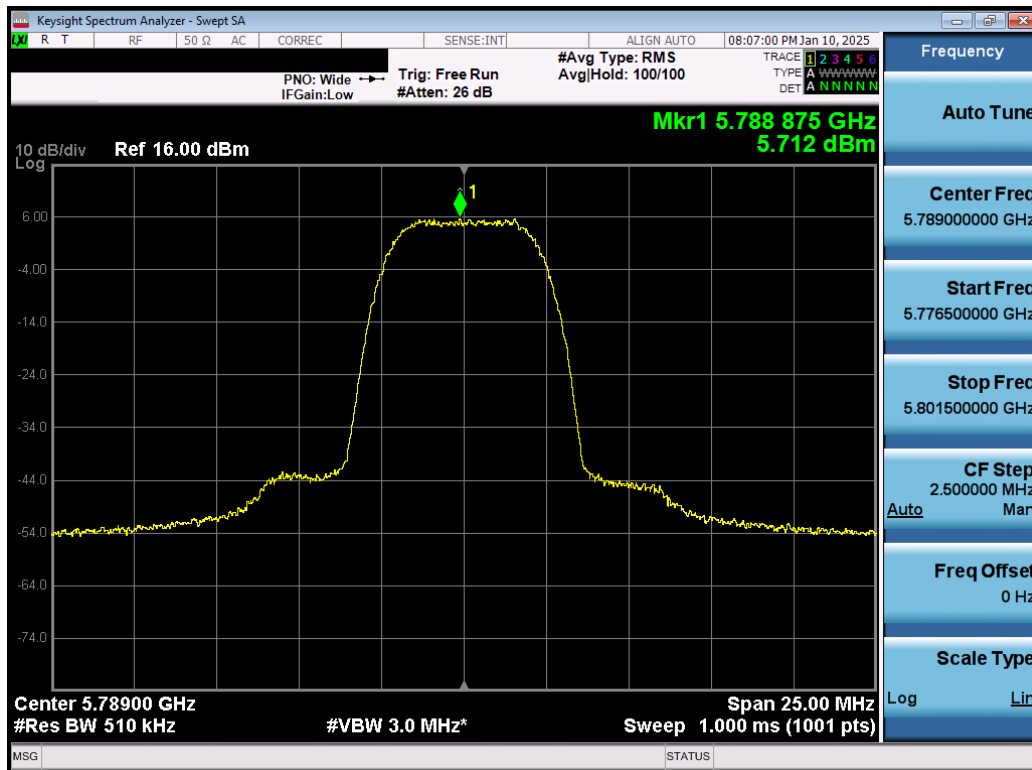
Plot 7-29. PSD Antenna 5T (NB UNII HDR8, ePA – 5789MHz)
