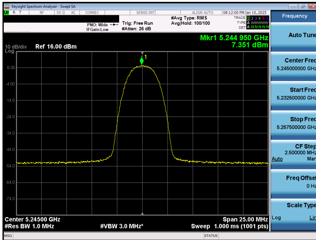
Plot 7-59. PSD TxBF Antenna 5T (NB UNII HDR4, ePA - 5245MHz)
