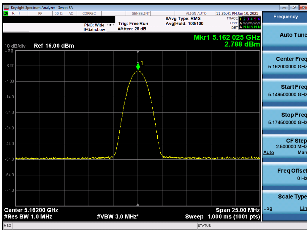
Plot 7-58. PSD TxBF Antenna 3b (NB UNII BDR, iPA – 5162MHz)
