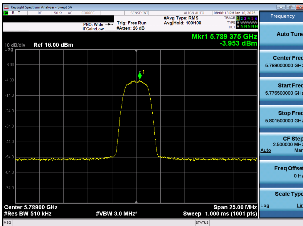
Plot 7-28. PSD Antenna 5T (NB UNII HDR4, iPA – 5789MHz)
