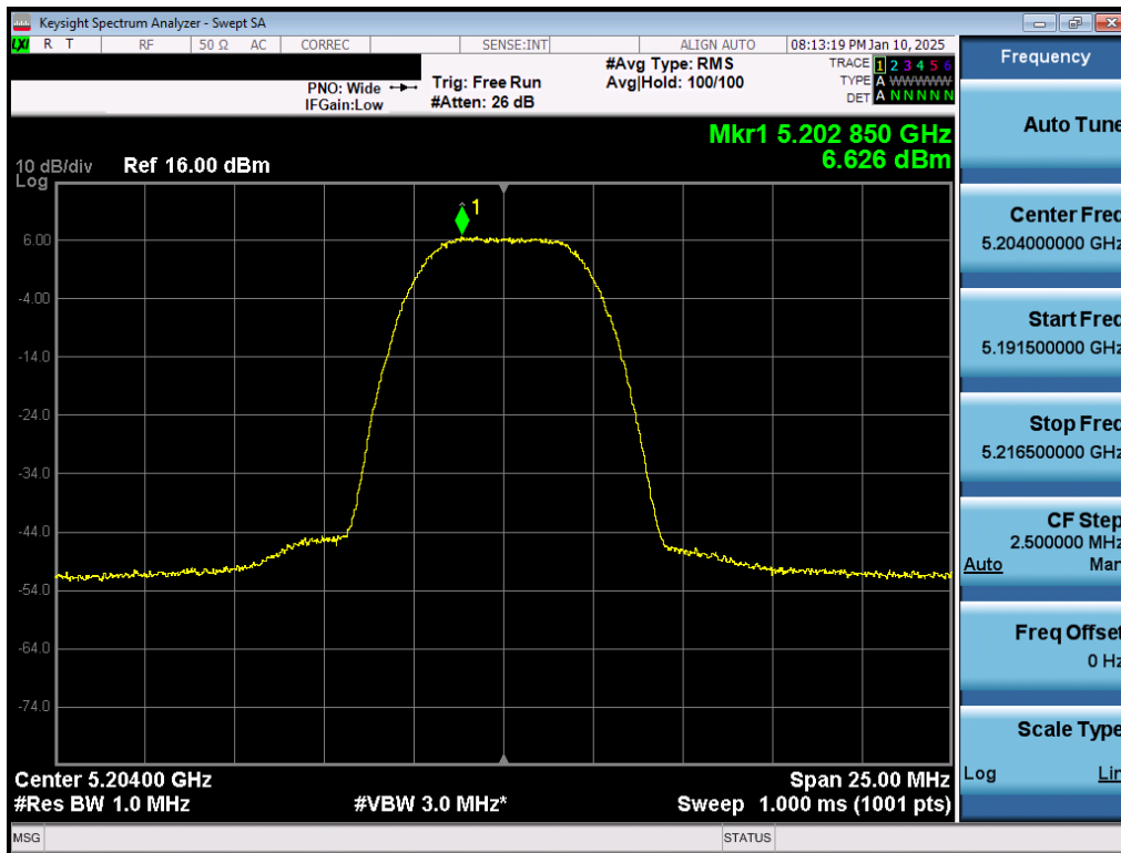
Plot 7-63. PSD Tx BF Antenna 5T (NB UNII HDR8, ePA – 5204MHz)
