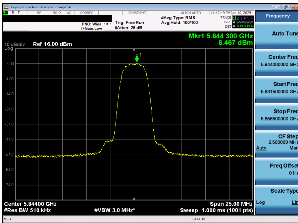
Plot 7-72. PSD TxBF Antenna 3b (NB UNII HDR4, ePA – 5844MHz)
