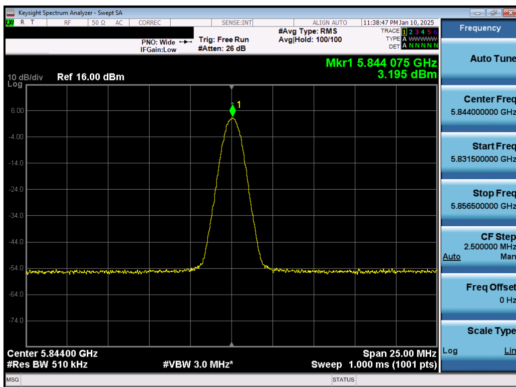
Plot 7-70. PSD TxBF Antenna 3b (NB UNII BDR, iPA - 5844MHz)
