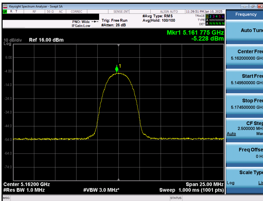
Plot 7-62. PSD TxBF Antenna 3b (NB UNII HDR4, iPA - 5162MHz)
