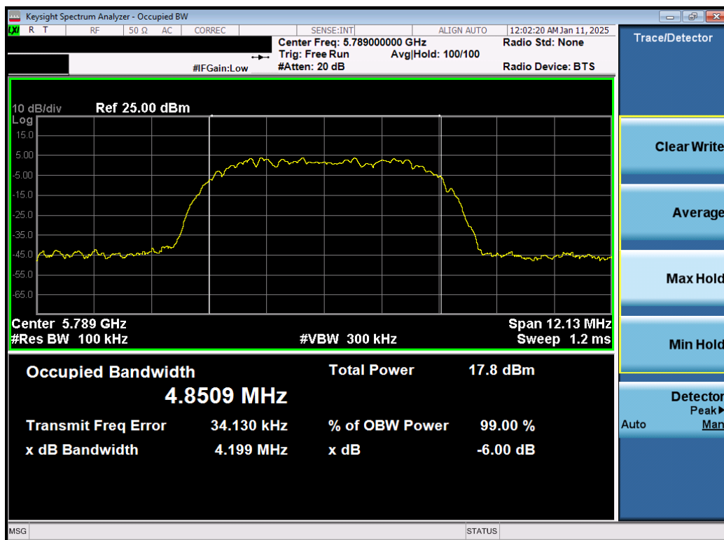
Plot 7-18. 6dB BW & 99% OBW Antenna 1b (NB UNII HDR8, 5789MHz)
