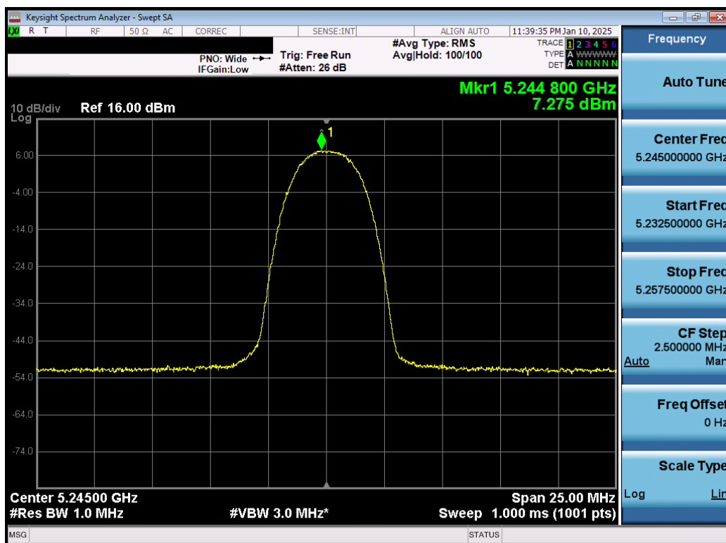
Plot 7-60. PSD TxBF Antenna 3b (NB UNII HDR4, ePA - 5245MHz)
