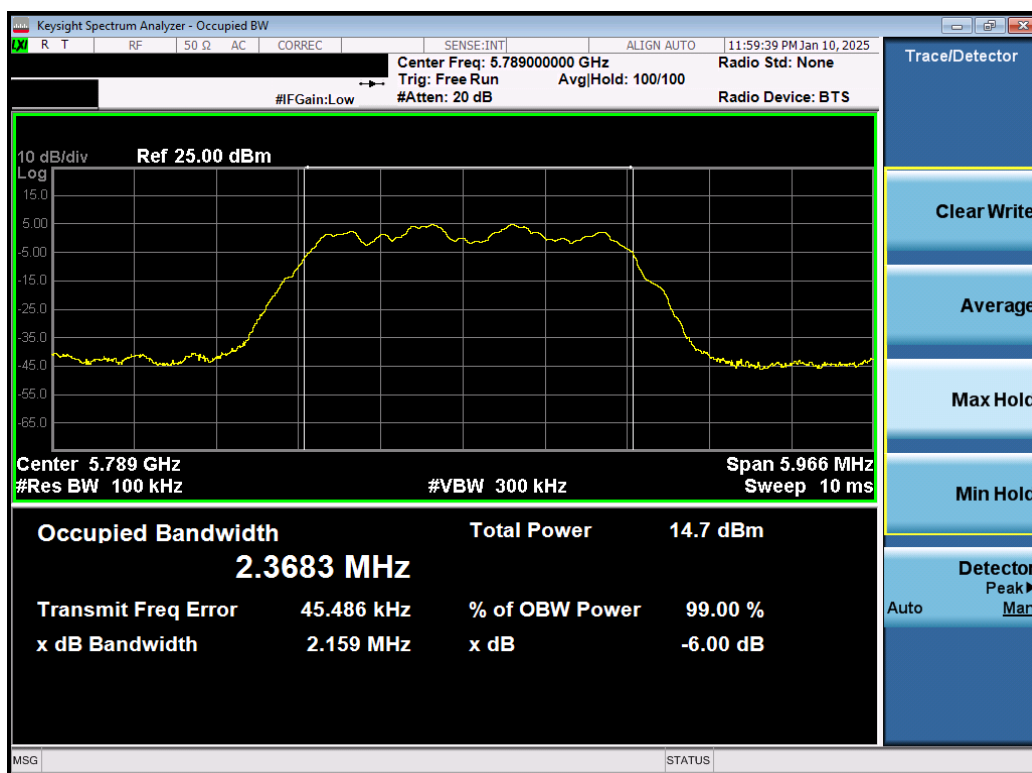
Plot 7-17. 6dB BW & 99% OBW Antenna 1b (NB UNII HDR4, 5789MHz)
