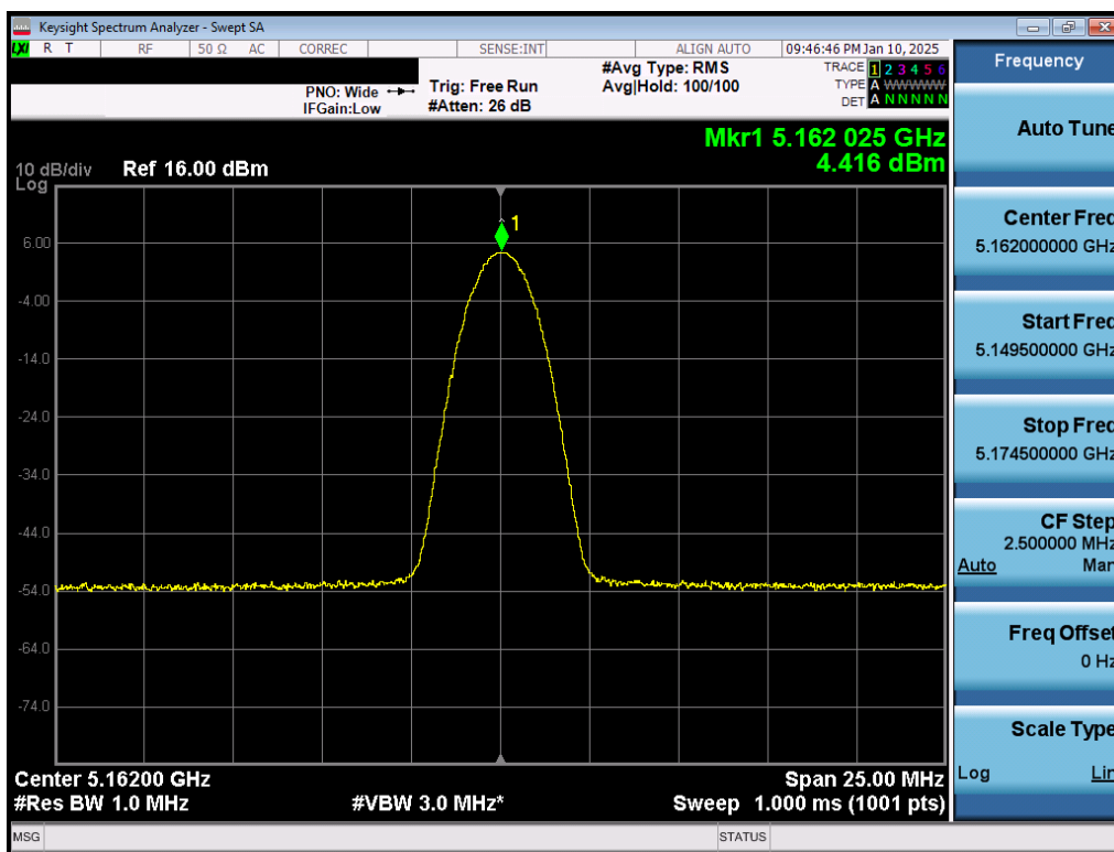
Plot 7-32. PSD Antenna 3b (NB UNII BDR, iPA – 5162MHz)
