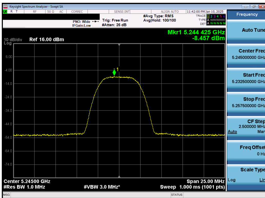
Plot 7-66. PSD Tx BF Antenna 3b (NB UNII HDR8, iPA – 5245MHz)
