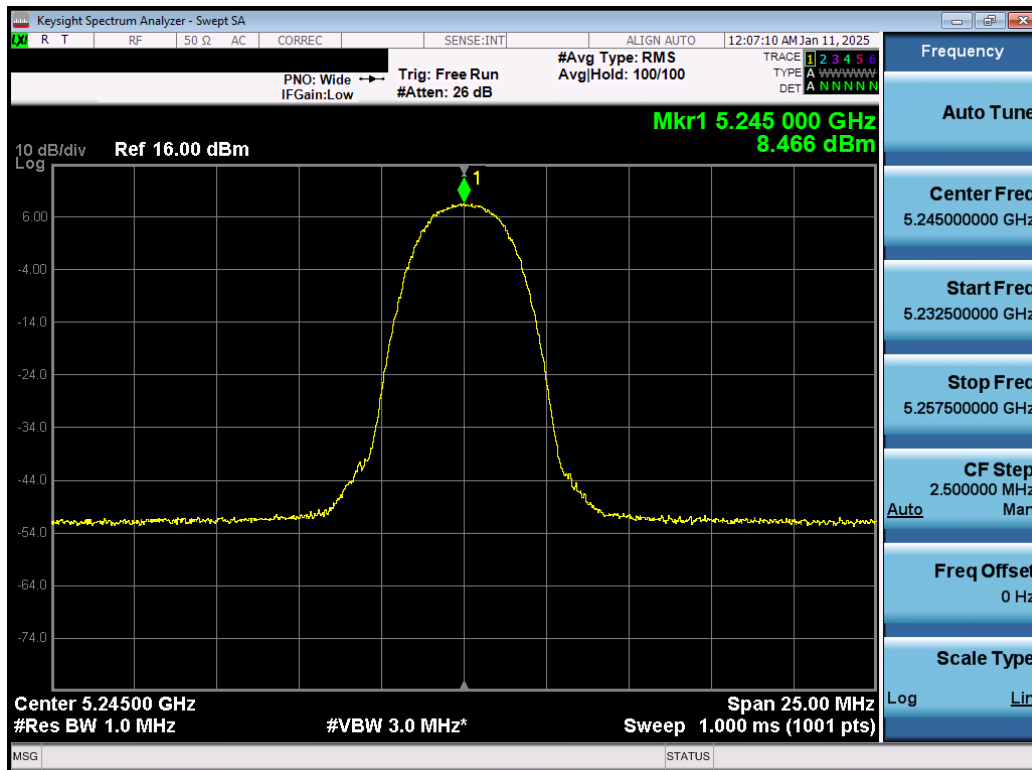
Plot 7-45. PSD Antenna 1b (NB UNII HDR4, ePA – 5245MHz)
