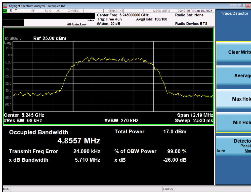
Plot 7-6. 26dB BW & 99% OBW Antenna 3b (NB UNII HDR8, ePA- 5245MHz)
