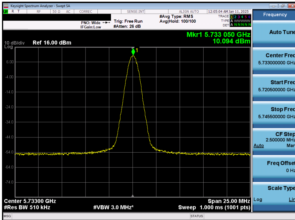
Plot 7-49. PSD Antenna 1b (NB UNII BDR, ePA – 5733MHz)
