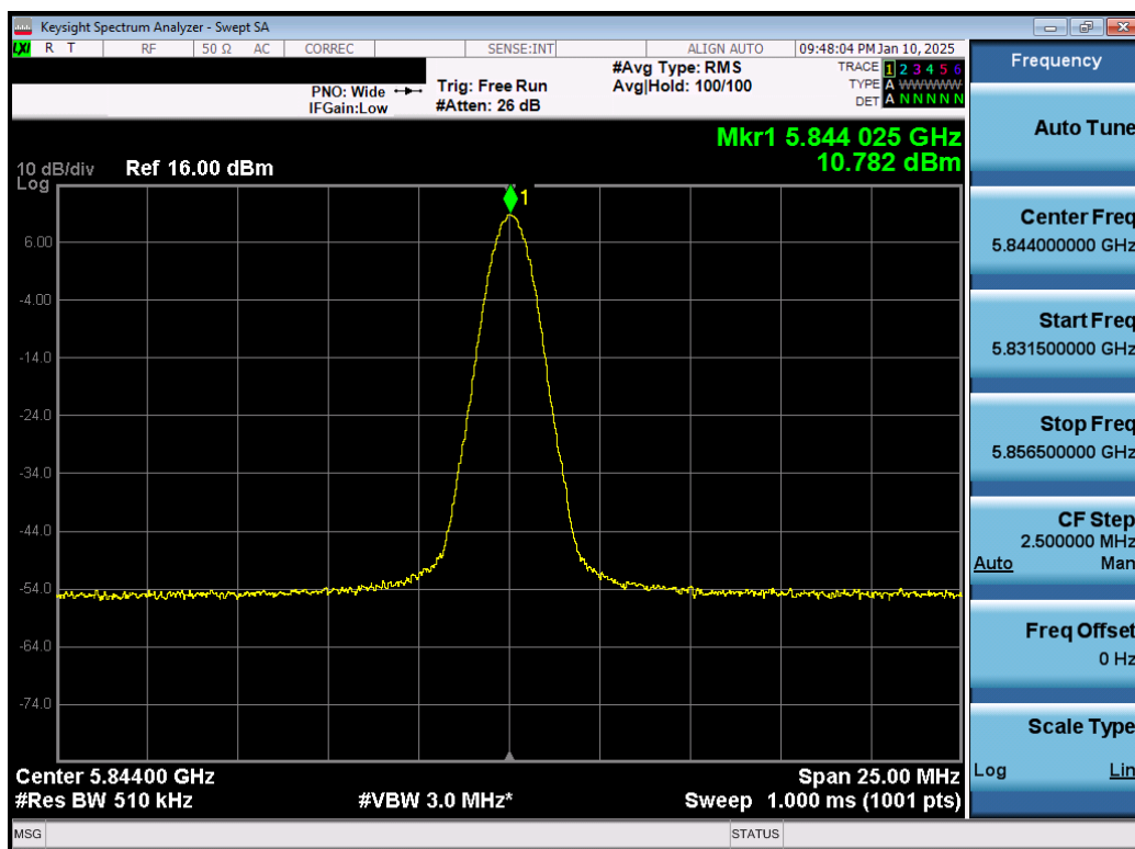
Plot 7-37. PSD Antenna 3b (NB UNII BDR, ePA – 5844MHz)
