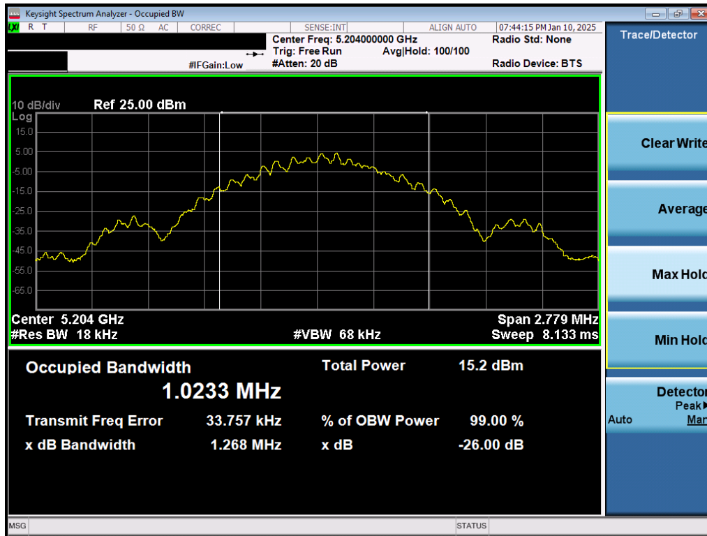
Plot 7-1. 26dB BW & 99% OBW Antenna 5T (NB UNII BDR, ePA- 5204MHz)
