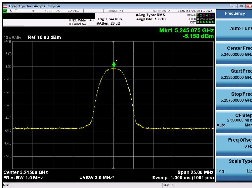
Plot 7-46. PSD Antenna 1b (NB UNII HDR4, iPA – 5245MHz)
