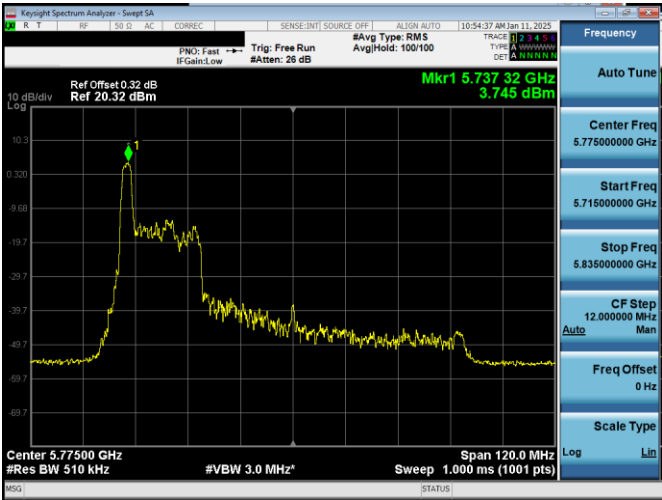
Plot 7-27. PSD Antenna 1b (20MHz BW 11ax Index 0 – RU26 – Ch.155)
