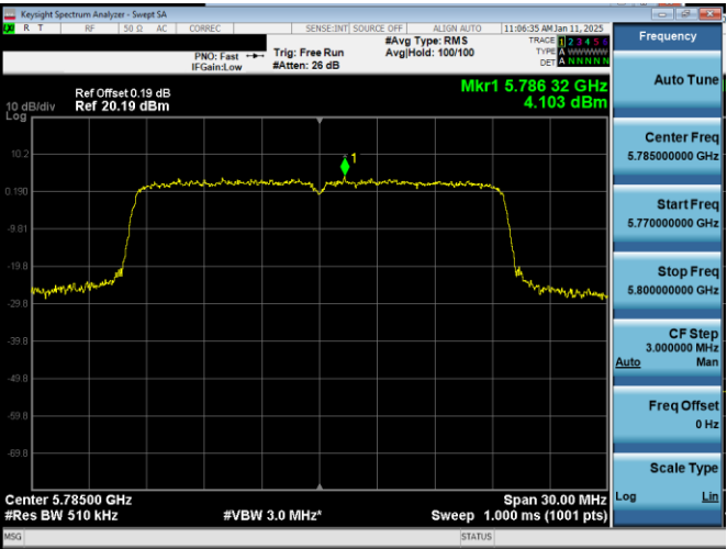
Plot 7-28. PSD Antenna 1b (20MHz BW 11ax– RU242 – Ch.157)
