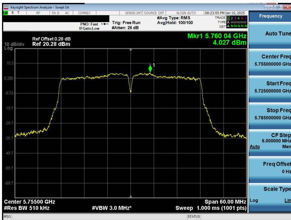
Plot 7-65. PSD CDD Primary Antenna 5T (40MHz BW 802.11n – Ch. 151)
