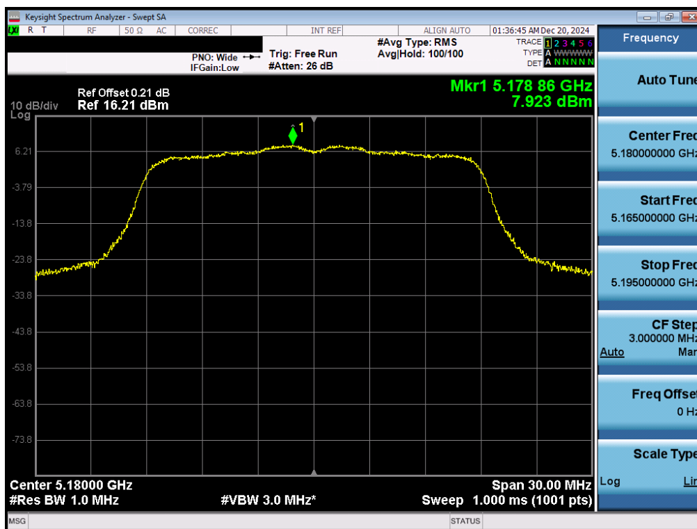
Plot 7-91. ISED PSD SDM Diversity Antenna 5T (20MHz BW 11n – Ch.36)
