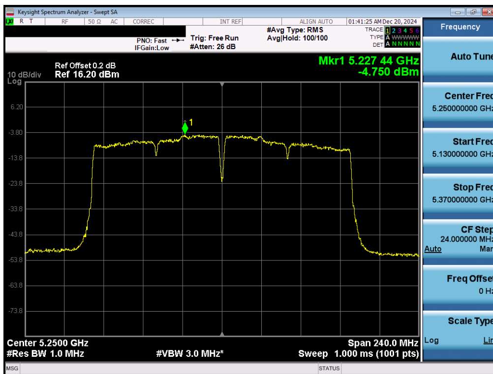
Plot 7-75. ISED PSD SDM Primary Antenna 5T (160MHz BW 11ac – Ch.50)
