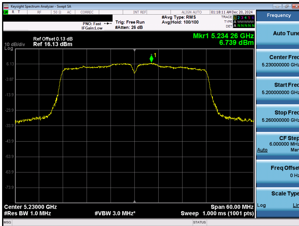
Plot 7-30. ISED PSD Antenna 5T (40MHz BW 11n – Ch.46)
