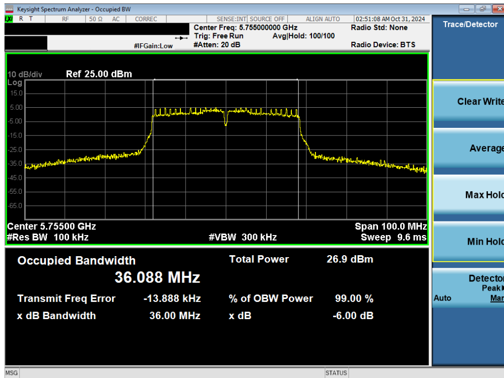
Plot 7-17. 6dB BW & 99% OBW Antenna 3b (40MHz BW 802.11n – Ch. 151)
