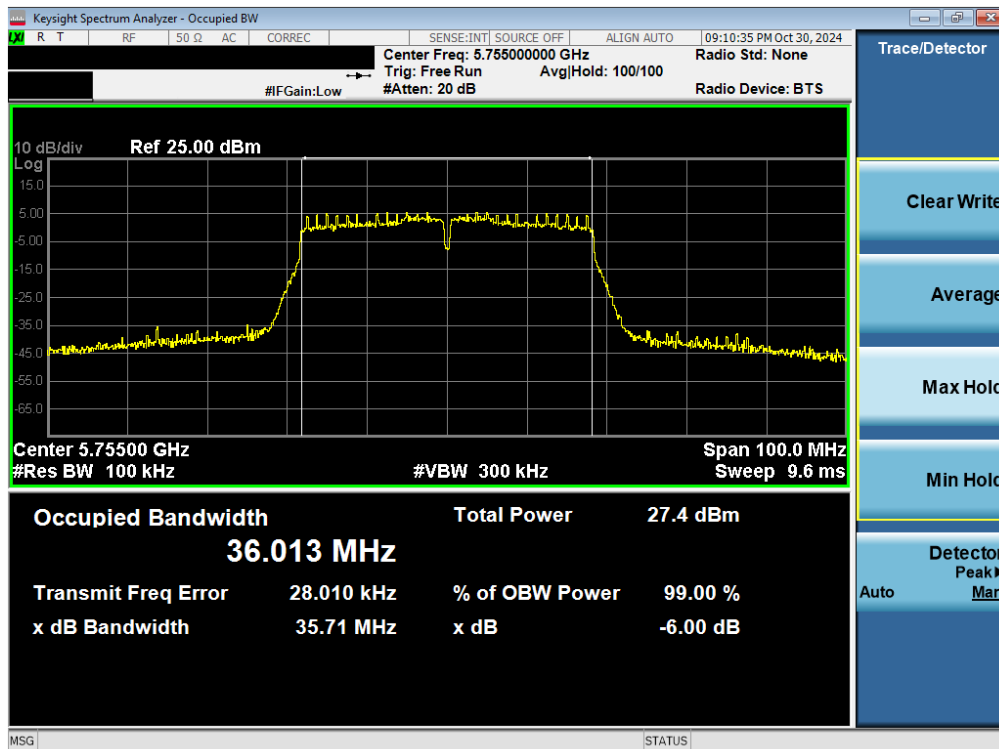
Plot 7-14. 6dB BW & 99% OBW Antenna 5T (40MHz BW 802.11n – Ch. 151)
