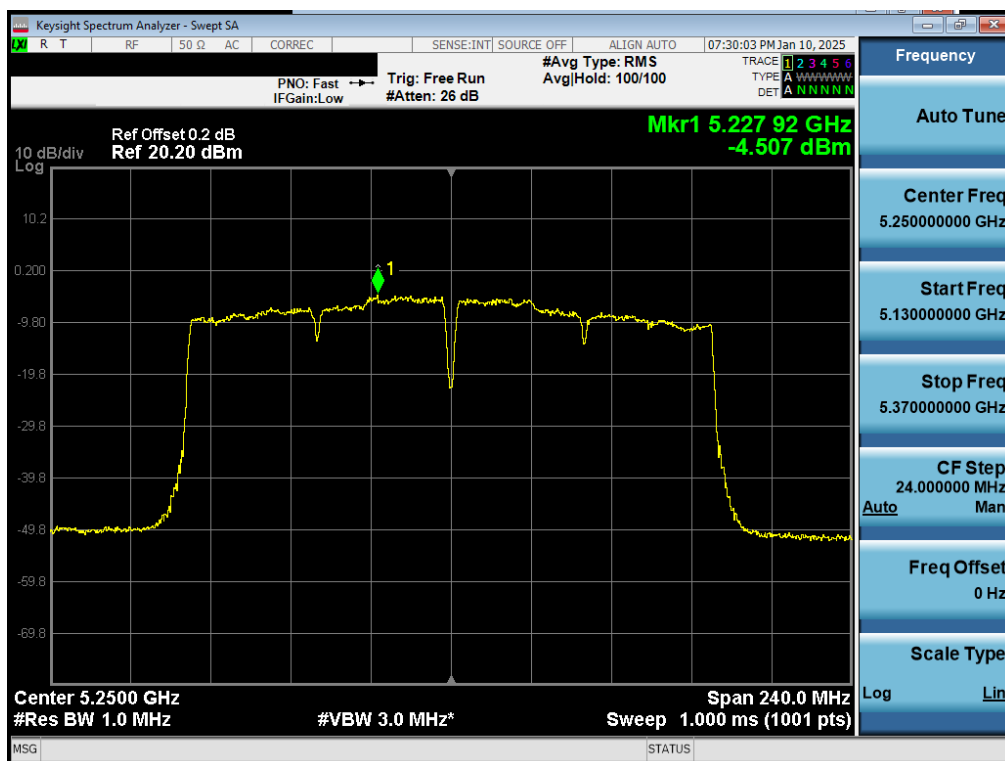
Plot 7-83. PSD CDD Diversity Antenna 5T (160MHz BW 802.11ac – Ch. 50)
