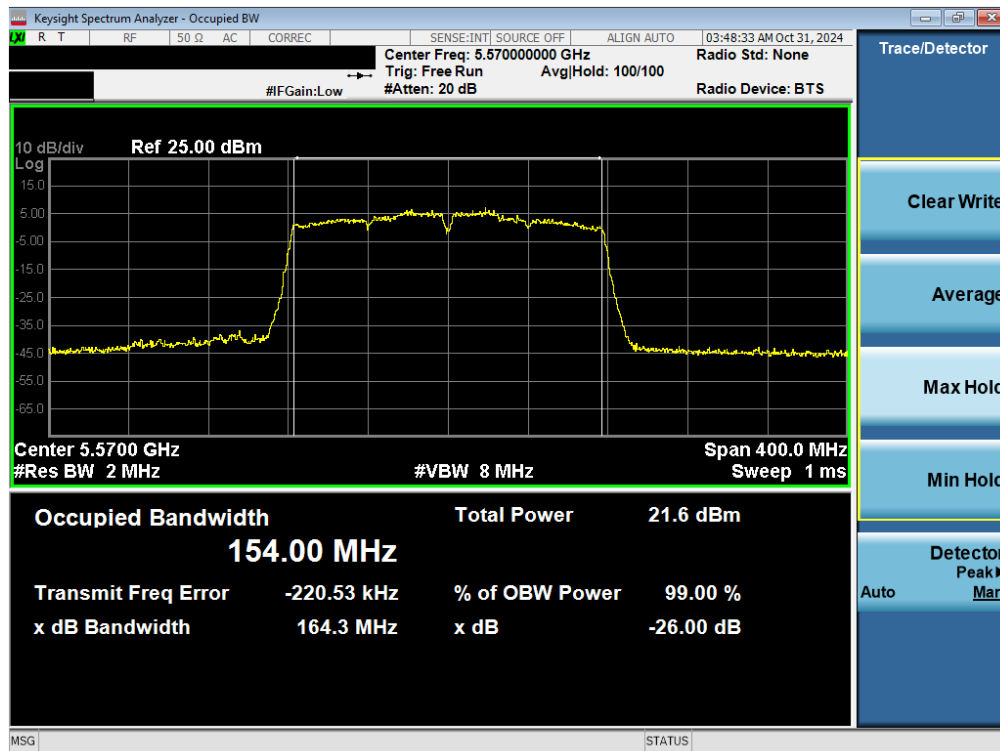
Plot 7-8. 26dB BW & 99% OBW Antenna 3b (160MHz BW 802.11ac – Ch. 114)
