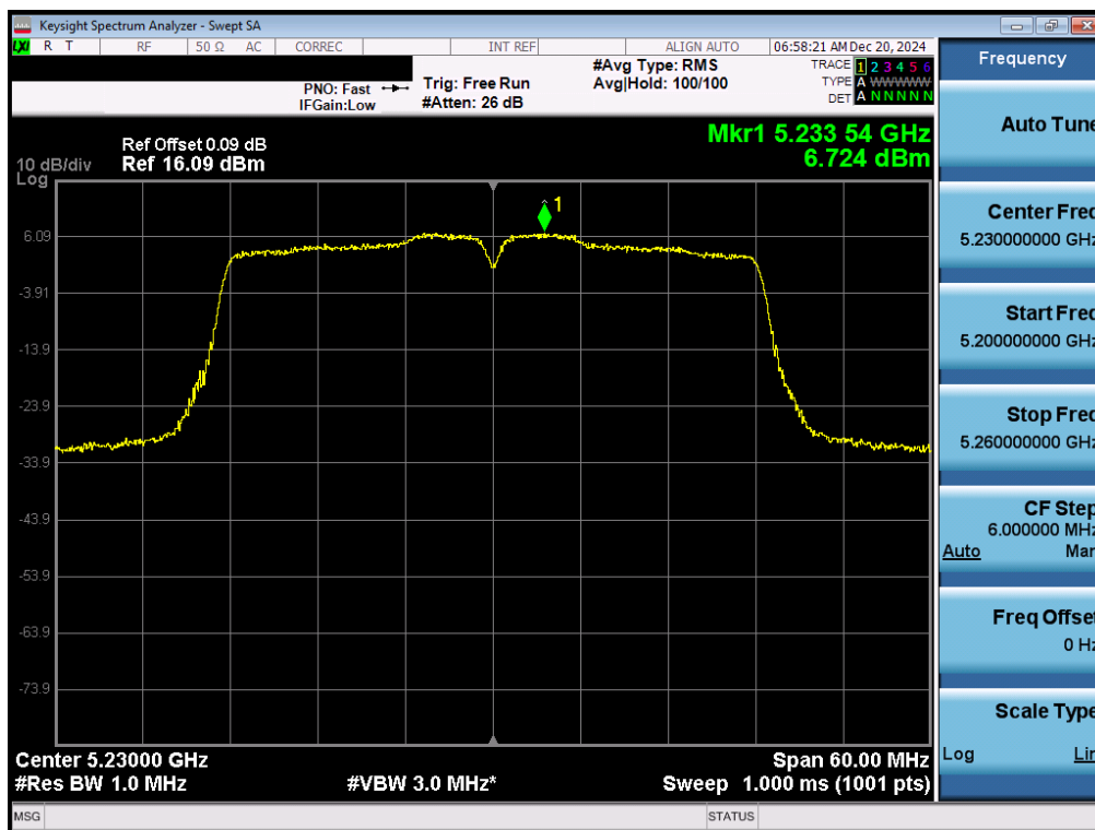
Plot 7-41. ISED PSD Antenna 3b (40MHz BW 11n – Ch.46)
