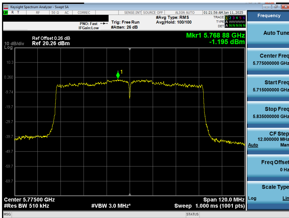
Plot 7-68. PSD CDD Primary Antenna 3b (80MHz BW 802.11ac – Ch. 155)
