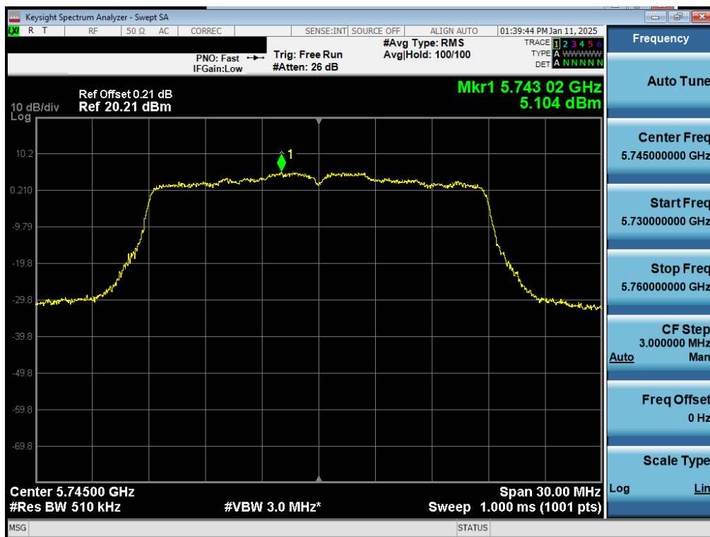
Plot 7-86. PSD CDD Diversity Antenna 1b (20MHz BW 802.11n – Ch. 149)
