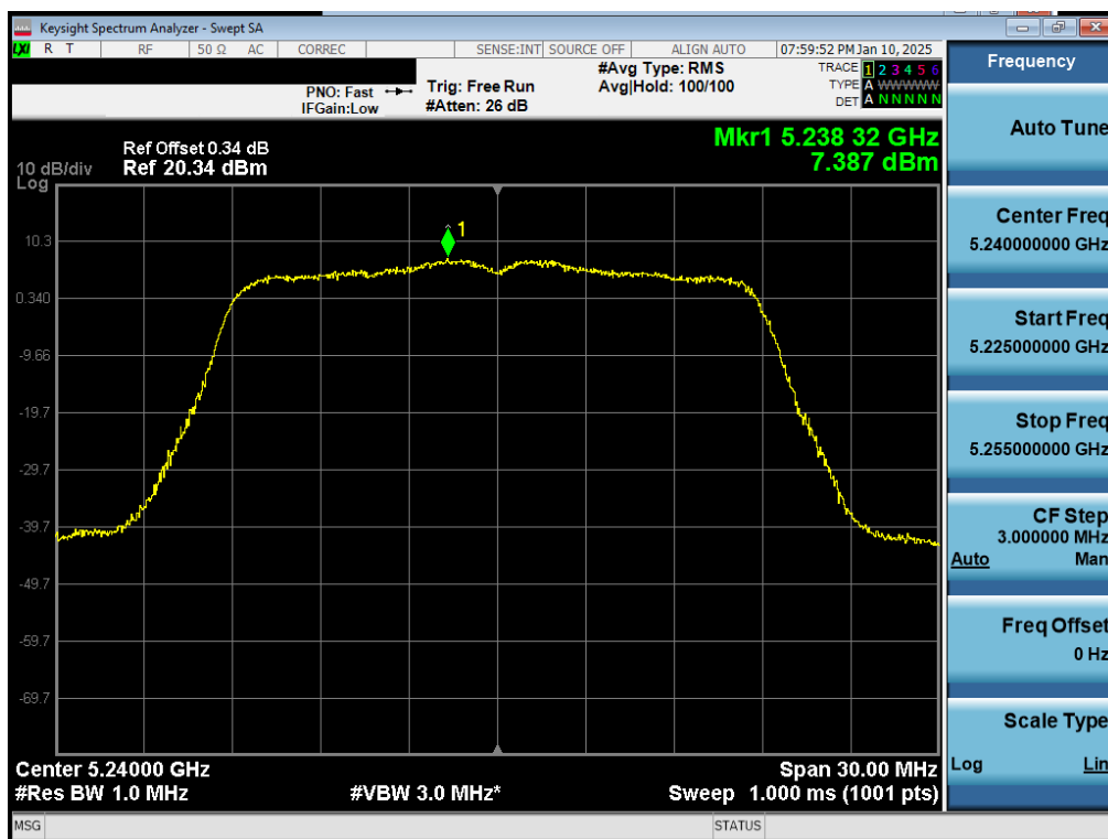
Plot 7-77. PSD CDD Diversity Antenna 5T (20MHz BW 802.11n – Ch. 48)
