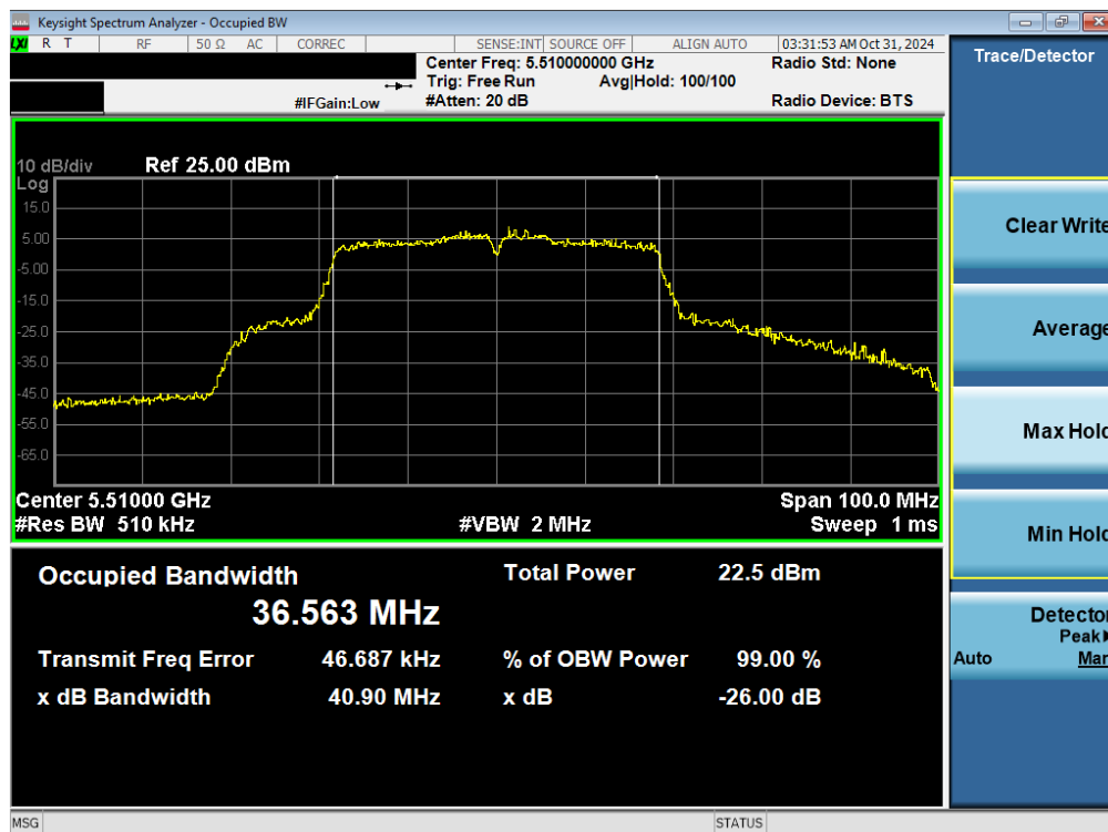
Plot 7-6. 26dB BW & 99% OBW Antenna 3b (40MHz BW 802.11n – Ch. 102)
