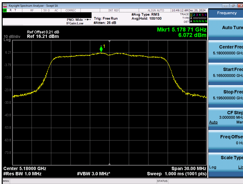
Plot 7-92. ISED PSD SDM Diversity Antenna 1b (20MHz BW 11n – Ch.36)
