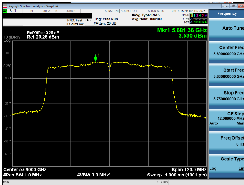
Plot 7-81. PSD CDD Diversity Antenna 5T (80MHz BW 802.11ac – Ch. 138)
