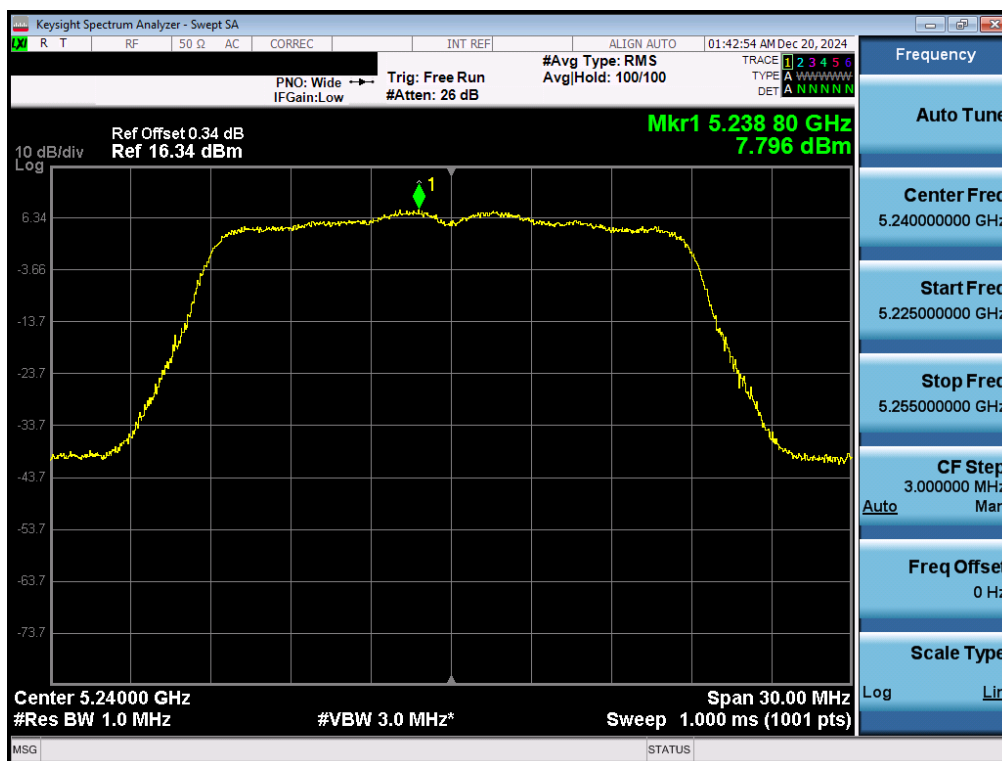
Plot 7-69. ISED PSD SDM Primary Antenna 5T (20MHz BW 11n – Ch.48)
