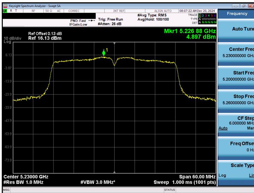
Plot 7-52. ISED PSD Antenna 1b (40MHz BW 11n – Ch.46)
