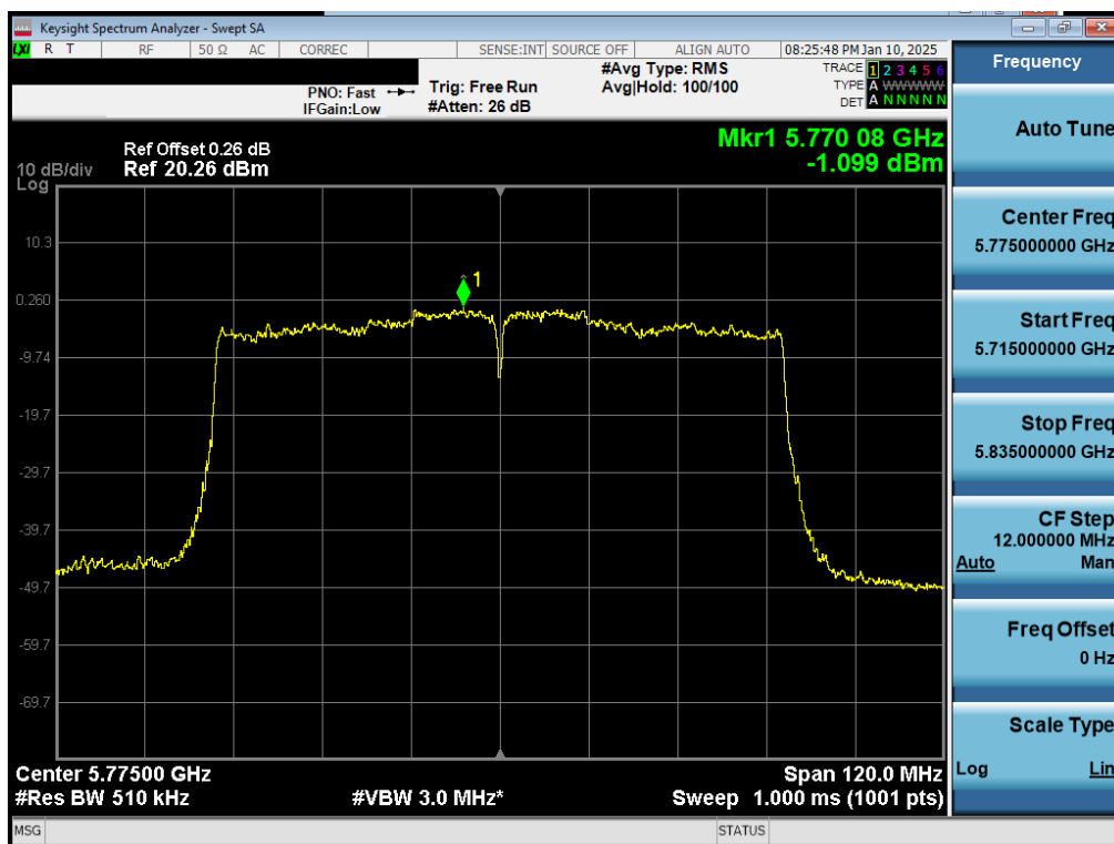
Plot 7-67. PSD CDD Primary Antenna 5T (80MHz BW 802.11ac – Ch. 155)
