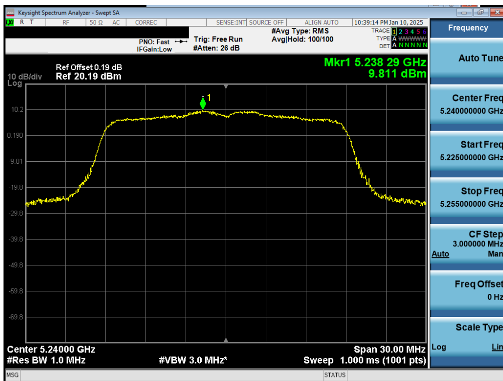
Plot 7-33. PSD Antenna 3b (20MHz BW 802.11n – Ch.48)
