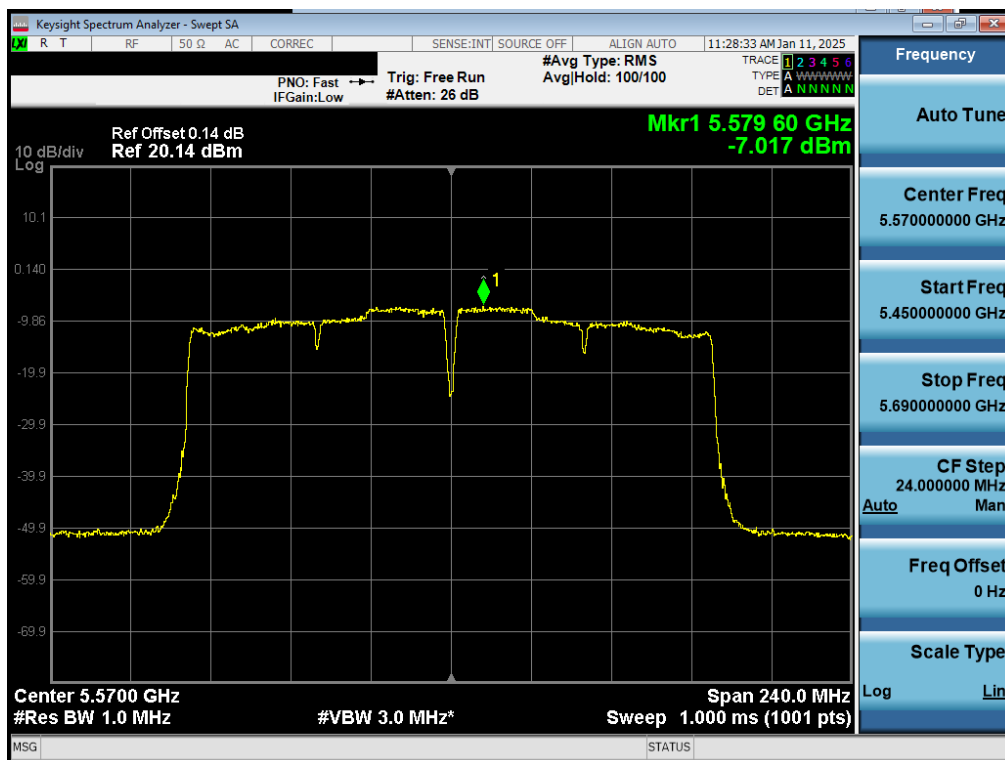
Plot 7-47. PSD Antenna 1b (160MHz BW 802.11ac – Ch. 114)
