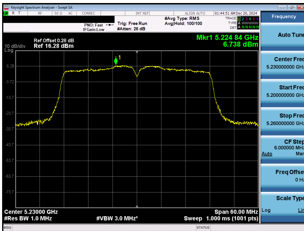
Plot 7-93. ISED PSD SDM Primary Antenna 5T (40MHz BW 11n – Ch.46)
