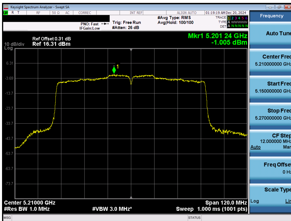
Plot 7-31. ISED PSD Antenna 5T (80MHz BW 11ac – Ch.42)
