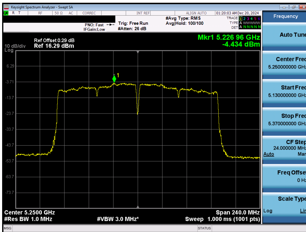
Plot 7-32. ISED PSD Antenna 5T (160MHz BW 11ac – Ch.50)
