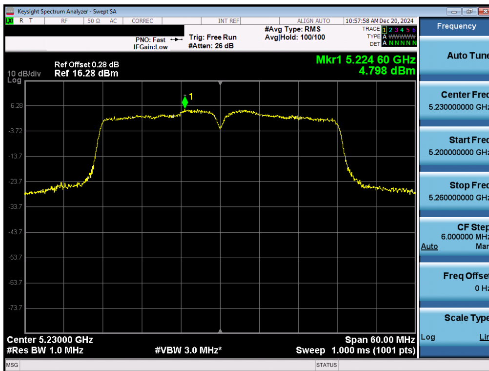
Plot 7-94. ISED PSD SDM Primary Antenna 3b (40MHz BW 11n – Ch.46)
