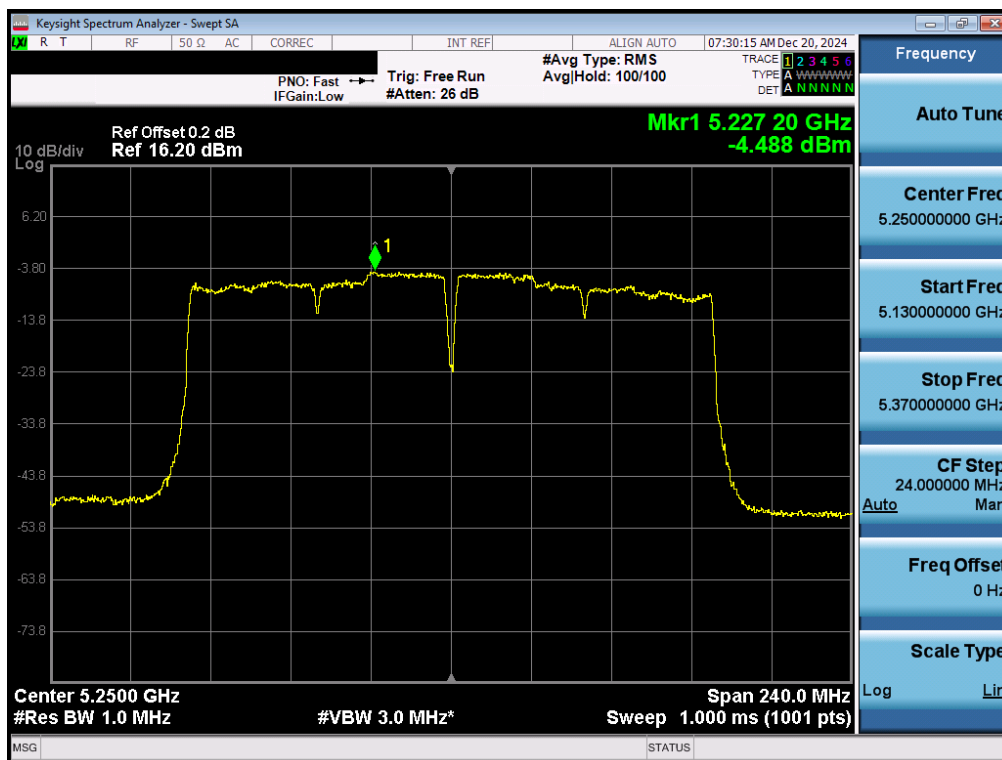
Plot 7-76. ISED PSD SDM Primary Antenna 3b (160MHz BW 11ac – Ch.50)
