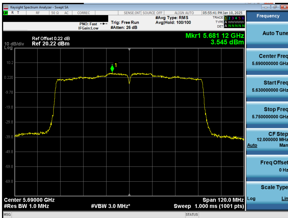
Plot 7-24. PSD Antenna 5T (80MHz BW 802.11ac – Ch. 138)
