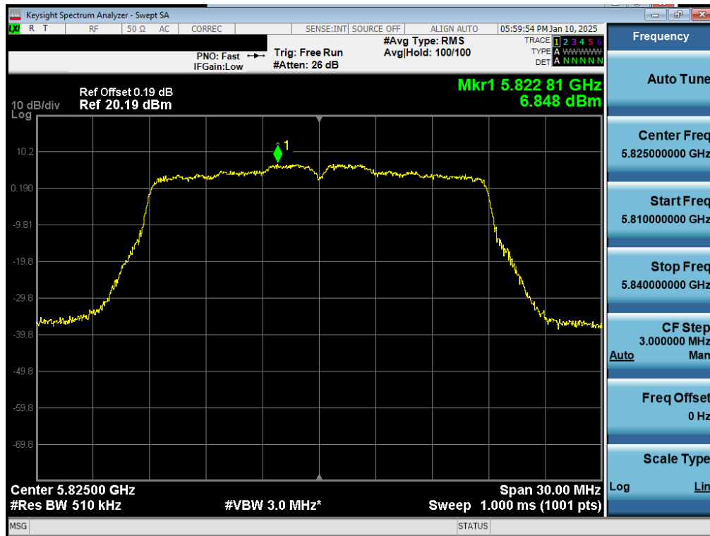
Plot 7-26. PSD Antenna 5T (20MHz BW 802.11n – Ch. 165)
