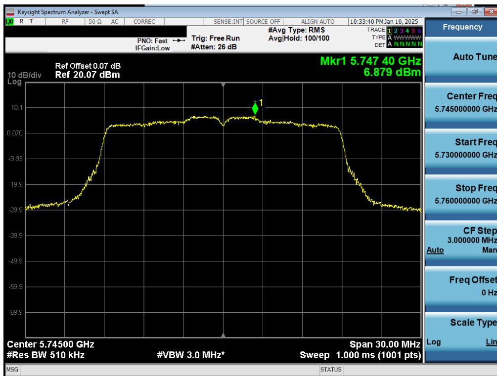
Plot 7-37. PSD Antenna 3b (20MHz BW 802.11n – Ch. 149)
