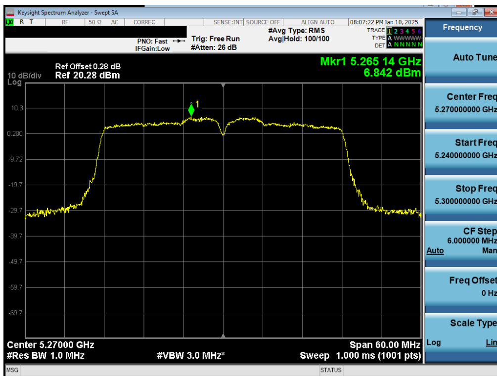
Plot 7-79. PSD CDD Diversity Antenna 5T (40MHz BW 802.11n – Ch. 54)
