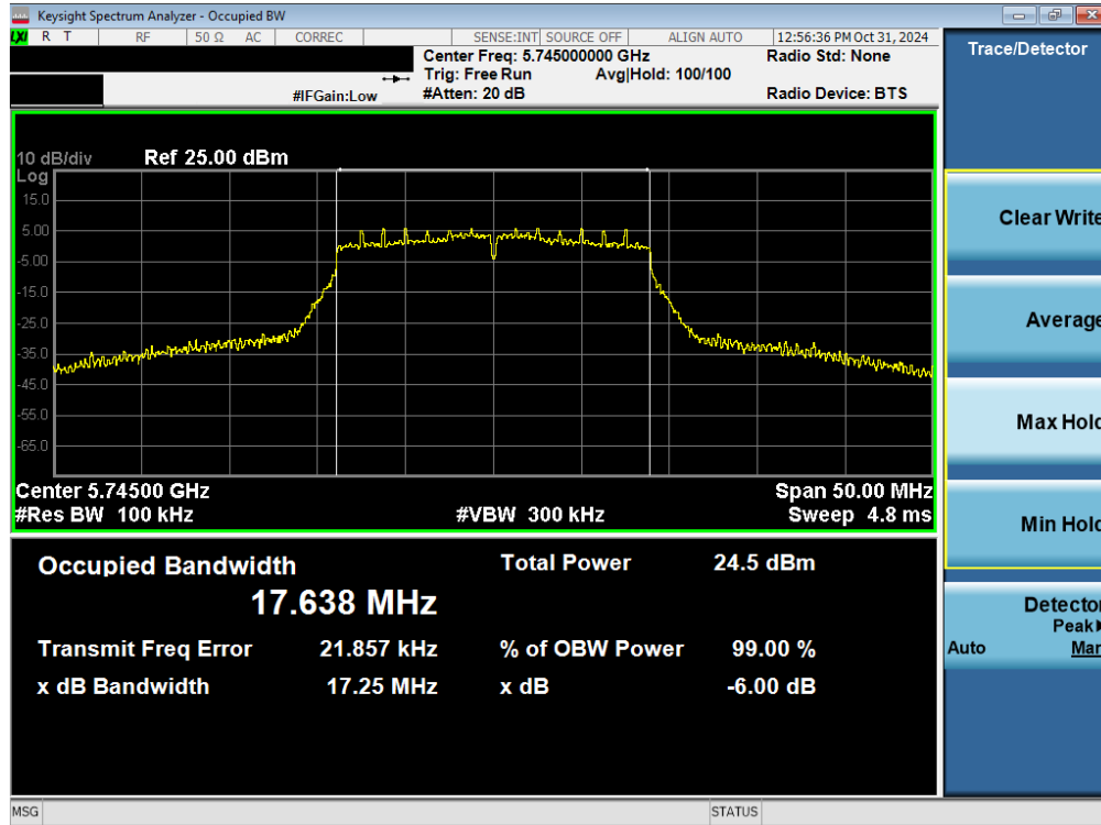
Plot 7-19. 6dB BW & 99% OBW Antenna 1b (20MHz BW 802.11n – Ch. 149)
