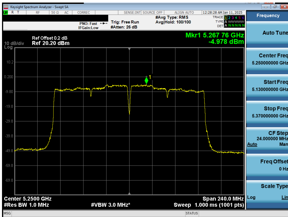
Plot 7-62. PSD CDD Primary Antenna 3b (160MHz BW 802.11ac – Ch. 50)
