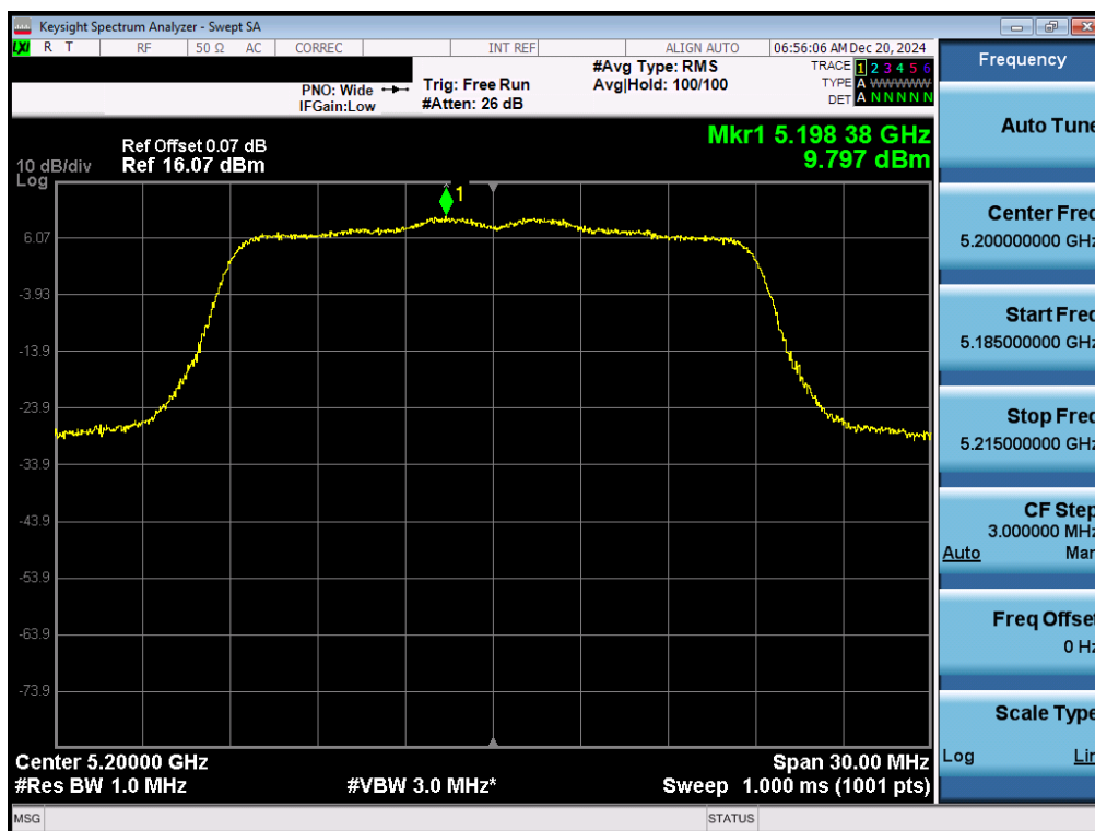
Plot 7-40. ISED PSD Antenna 3b (20MHz BW 11n – Ch.40)
