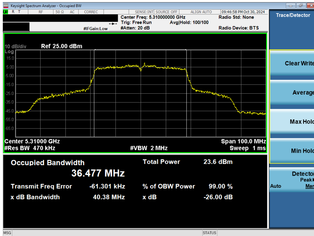
Plot 7-2. 26dB BW & 99% OBW Antenna 5T (40MHz BW 802.11n – Ch. 62)
