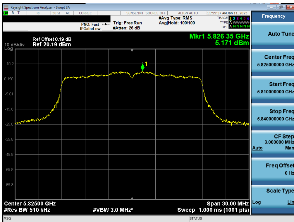
Plot 7-48. PSD Antenna 1b (20MHz BW 802.11n – Ch. 165)
