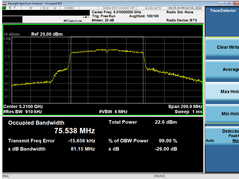
Plot 7-3. 26dB BW & 99% OBW Antenna 5T (80MHz BW 802.11ac – Ch. 42)
