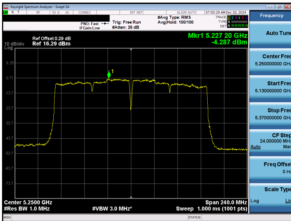
Plot 7-43. ISED PSD Antenna 3b (160MHz BW 11ac – Ch.50)
