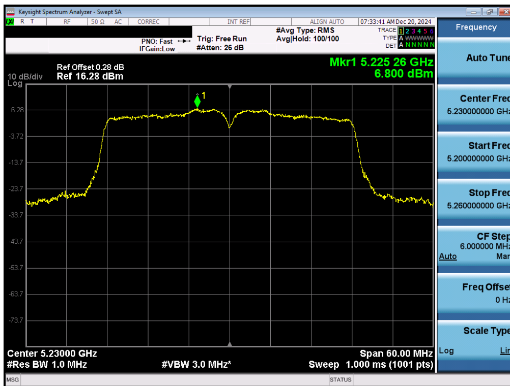
Plot 7-72. ISED PSD SDM Primary Antenna 3b (40MHz BW 11n – Ch.46)
