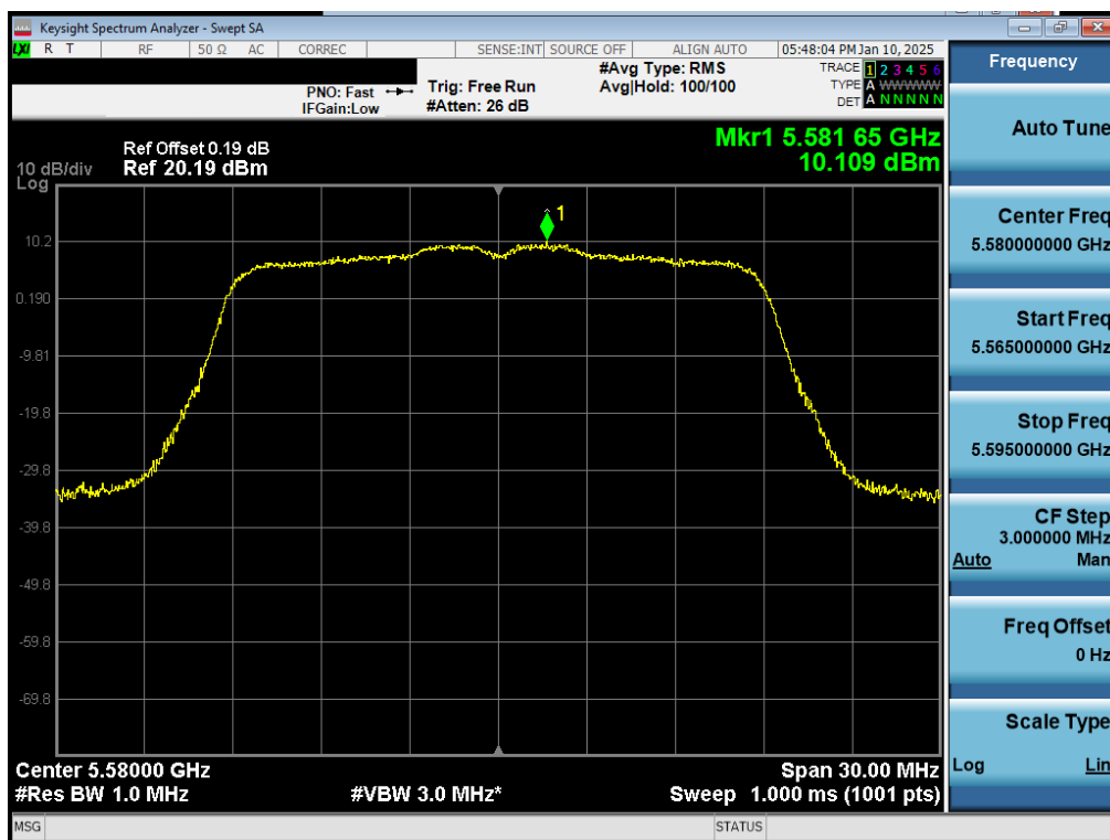
Plot 7-22. PSD Antenna 5T (20MHz BW 802.11n – Ch.116)
