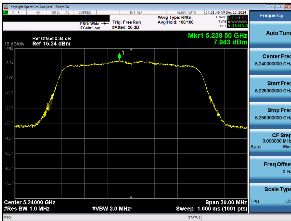
Plot 7-70. ISED PSD SDM Primary Antenna 3b (20MHz BW 11n – Ch.48)
