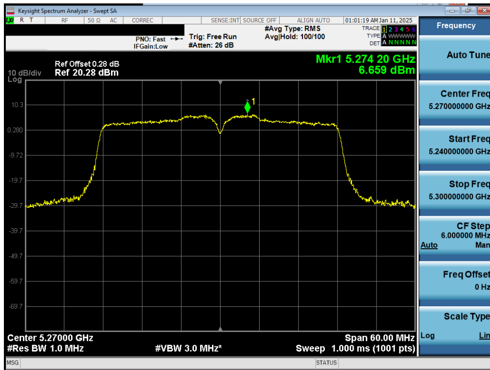
Plot 7-58. PSD CDD Primary Antenna 3b (40MHz BW 802.11n – Ch. 54)
