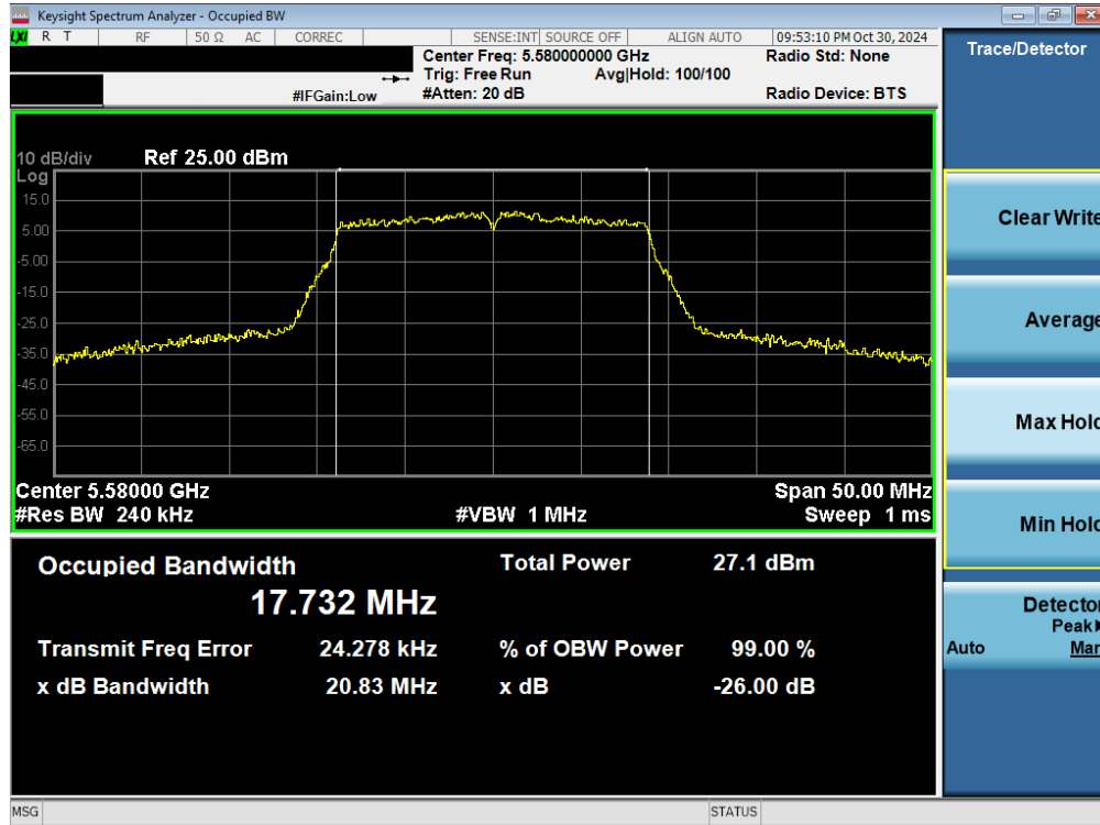
Plot 7-1. 26dB BW & 99% OBW Antenna 5T (20MHz BW 802.11n – Ch. 116)
