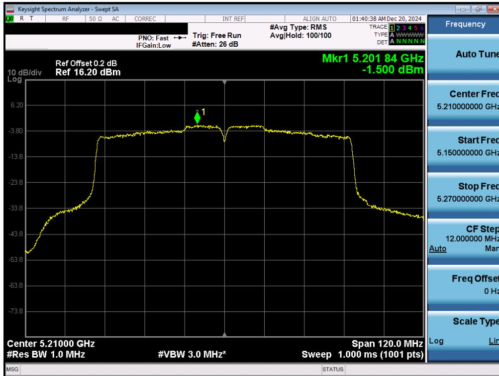
Plot 7-95. ISED PSD SDM Primary Antenna 5T (80MHz BW 11ac – Ch.42)
