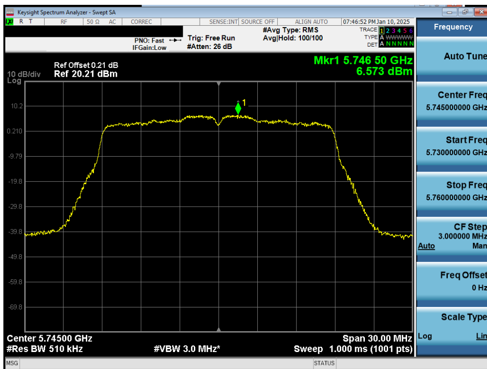
Plot 7-85. PSD CDD Diversity Antenna 5T (20MHz BW 802.11n – Ch. 149)
