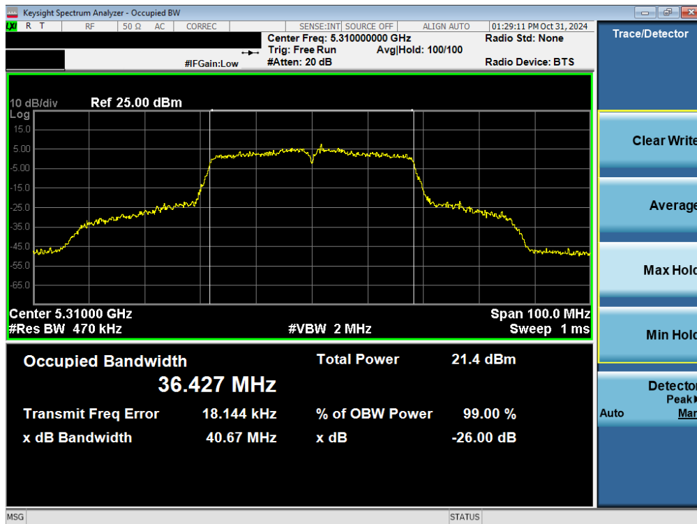
Plot 7-10. 26dB BW & 99% OBW Antenna 1b (40MHz BW 802.11n – Ch. 62)
