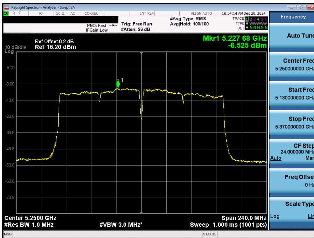
Plot 7-98. ISED PSD SDM Primary Antenna 3b (160MHz BW 11ac – Ch.50)
