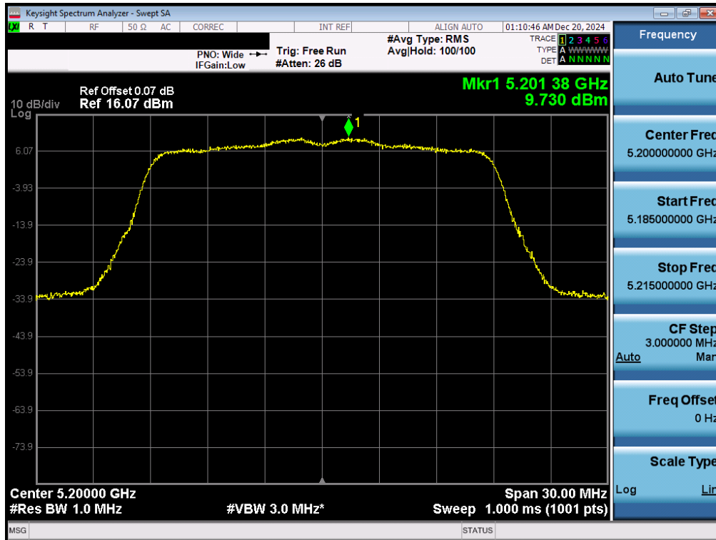
Plot 7-29. ISED PSD Antenna 5T (20MHz BW 11n – Ch.40)
