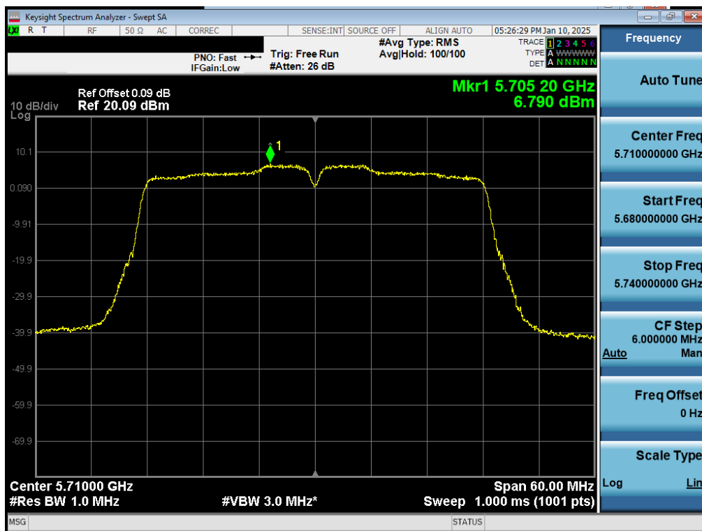
Plot 7-23. PSD Antenna 5T (40MHz BW 802.11n – Ch. 142)
