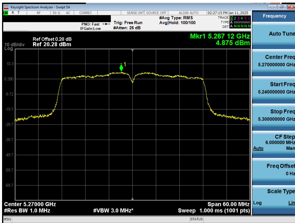
Plot 7-80. PSD CDD Diversity Antenna 1b (40MHz BW 802.11n – Ch. 54)
