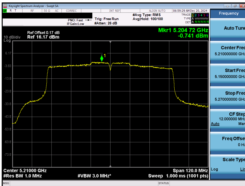
Plot 7-42. ISED PSD Antenna 3b (80MHz BW 11ac – Ch.42)
