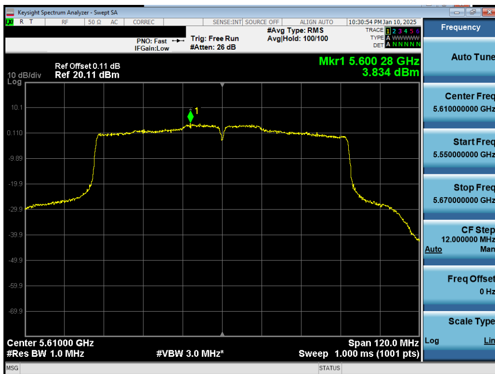
Plot 7-35. PSD Antenna 3b (80MHz BW 802.11ac – Ch. 122)
