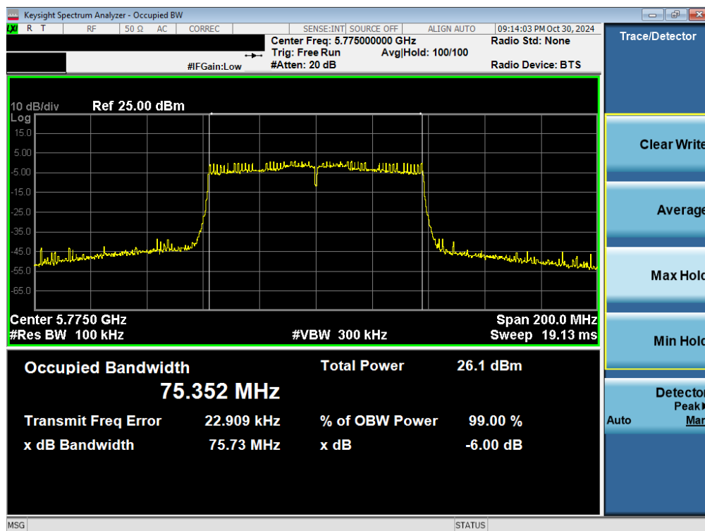
Plot 7-15. 6dB BW & 99% OBW Antenna 5T (80MHz BW 802.11ac – Ch. 155)
