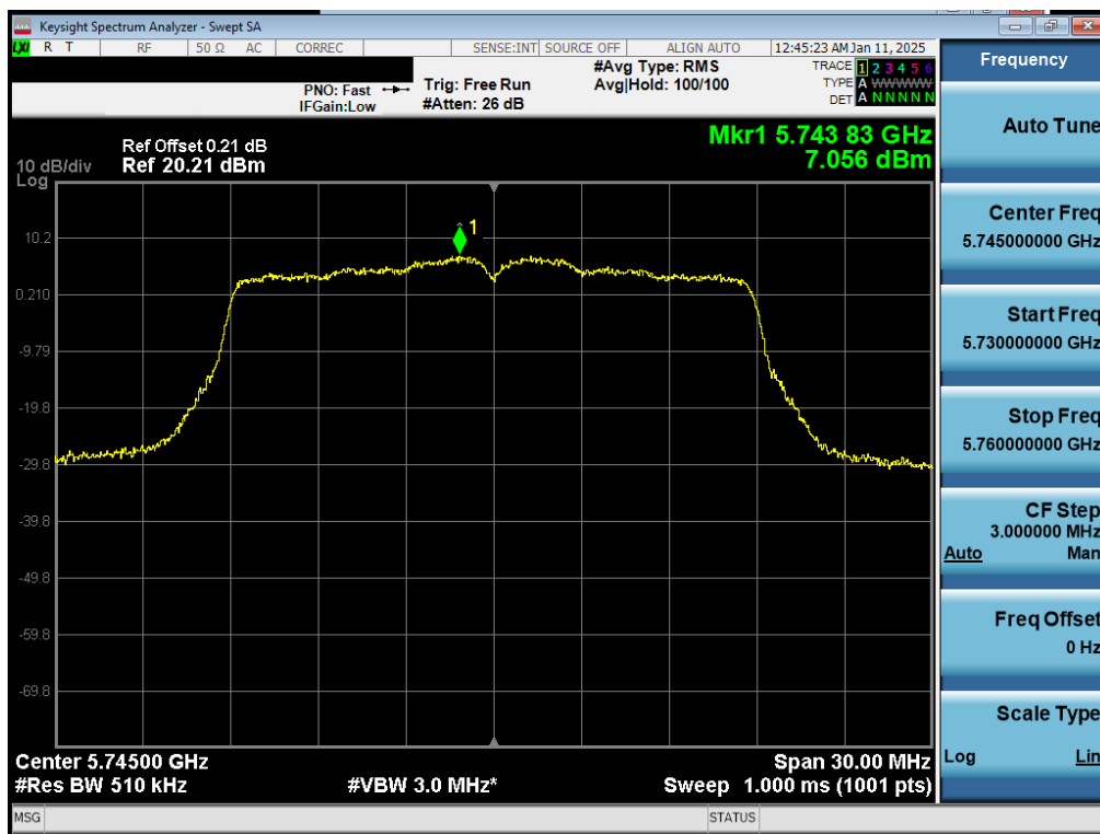
Plot 7-64. PSD CDD Primary Antenna 3b (20MHz BW 802.11n – Ch. 149)
