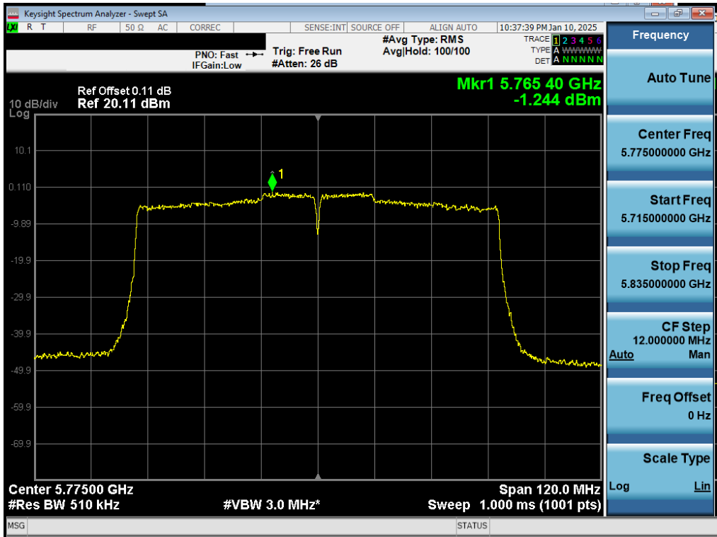
Plot 7-39. PSD Antenna 3b (80MHz BW 802.11ac – Ch. 155)
