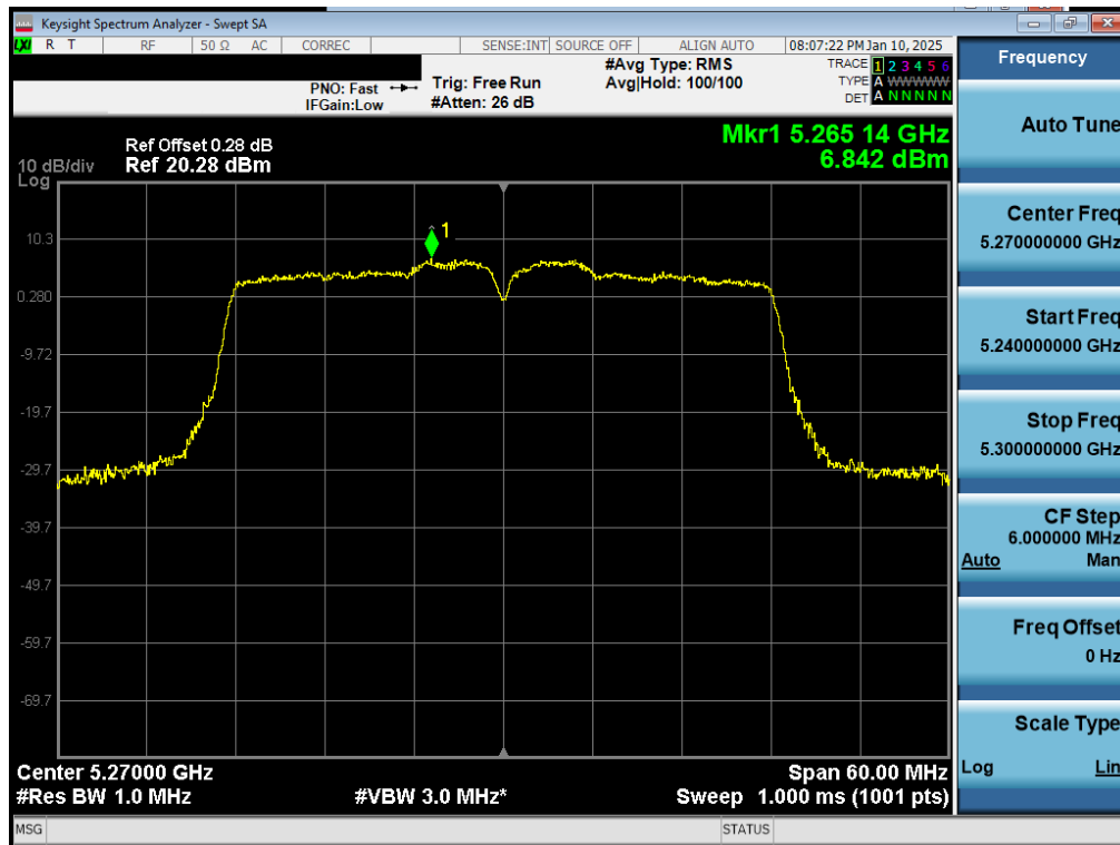
Plot 7-57. PSD CDD Primary Antenna 5T (40MHz BW 802.11n – Ch. 54)
