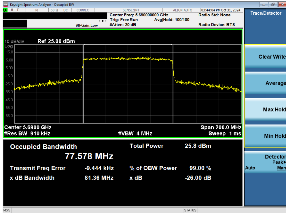
Plot 7-11. 26dB BW & 99% OBW Antenna 1b (80MHz BW 802.11ax(SU) – Ch. 138)
