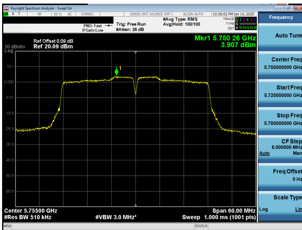
Plot 7-38. PSD Antenna 3b (40MHz BW 802.11n – Ch. 151)
