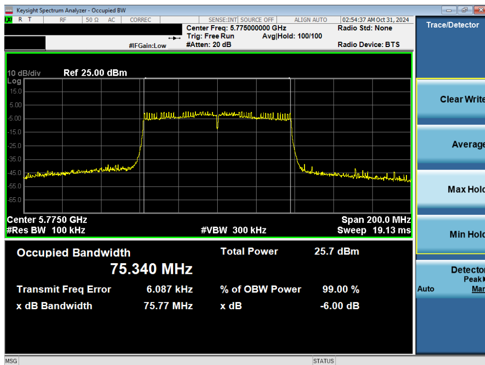
Plot 7-18. 6dB BW & 99% OBW Antenna 3b (80MHz BW 802.11ac – Ch. 155)
