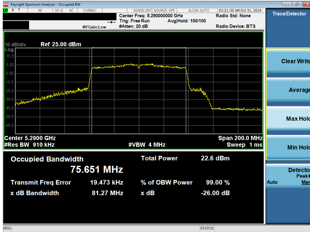
Plot 7-7. 26dB BW & 99% OBW Antenna 3b (80MHz BW 802.11ac – Ch. 58)
