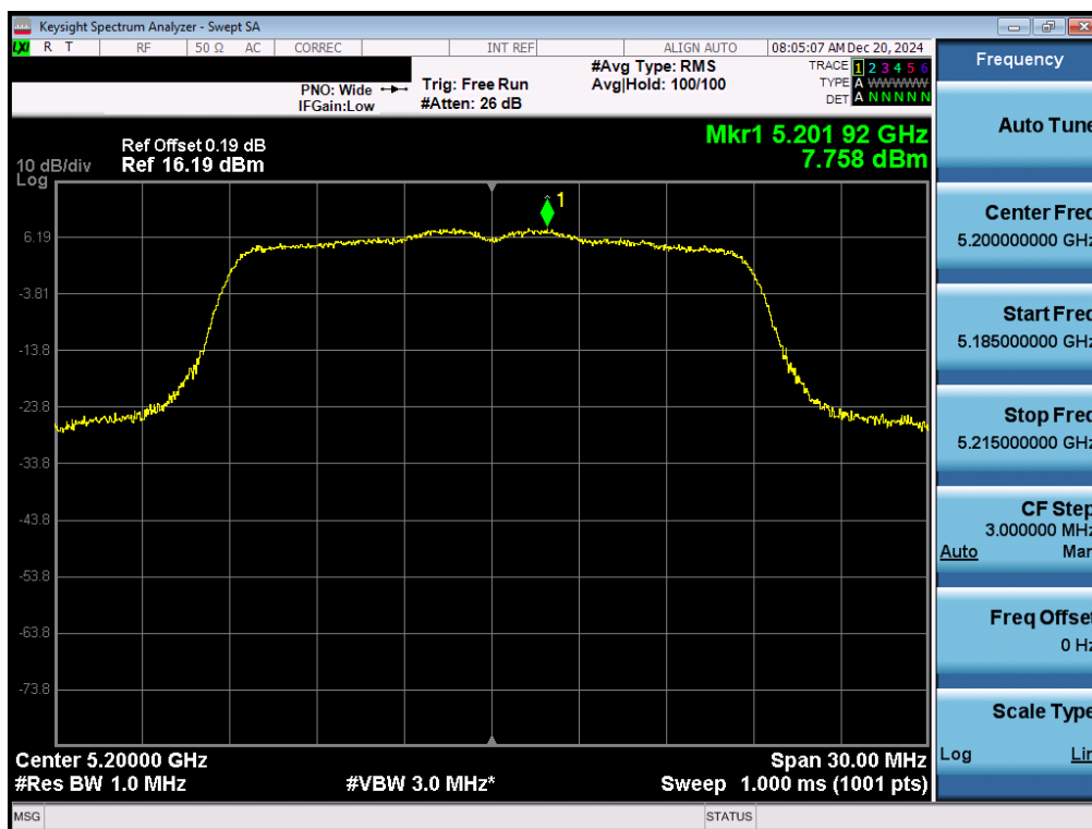
Plot 7-51. ISED PSD Antenna 1b (20MHz BW 11n – Ch.40)
