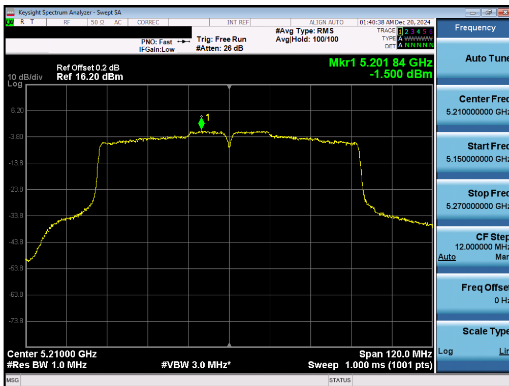
Plot 7-73. ISED PSD SDM Primary Antenna 5T (80MHz BW 11ac – Ch.42)
