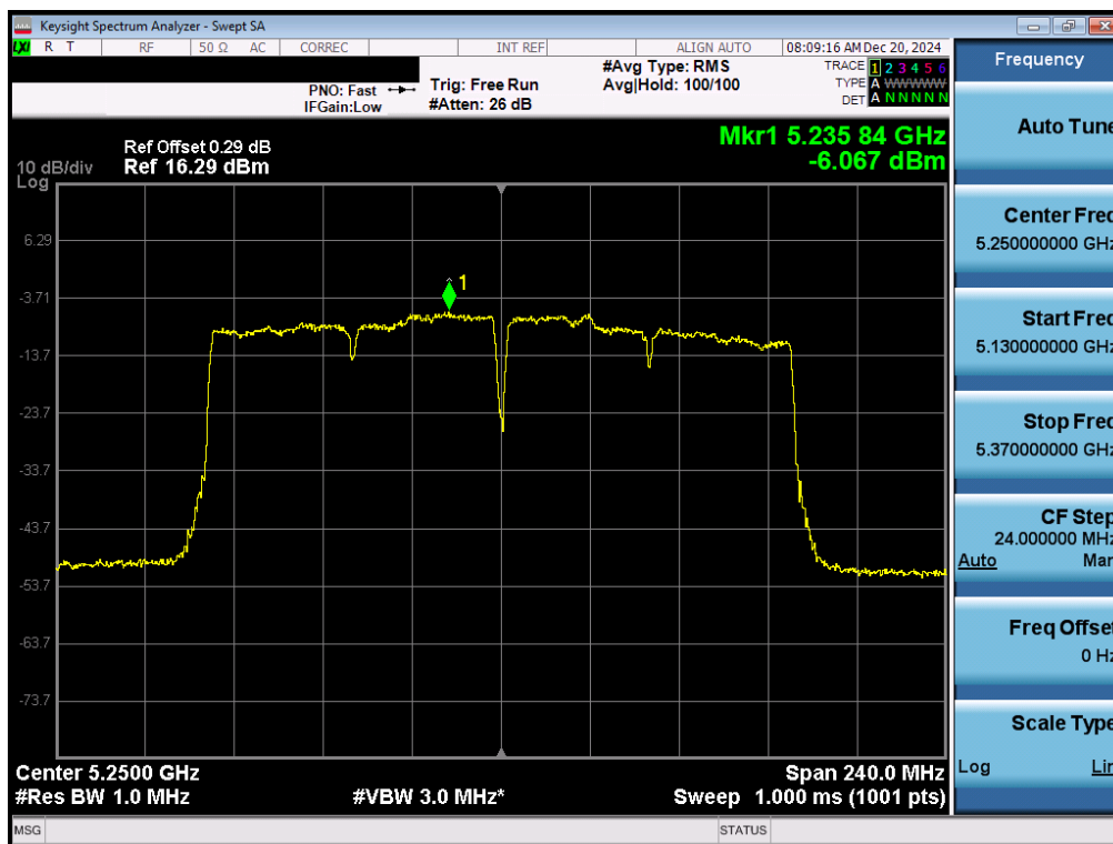
Plot 7-54. ISED PSD Antenna 1b (160MHz BW 11ac – Ch.50)
