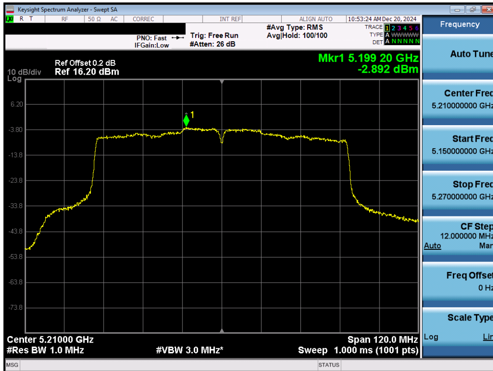
Plot 7-96. ISED PSD SDM Primary Antenna 3b (80MHz BW 11ac – Ch.42)
