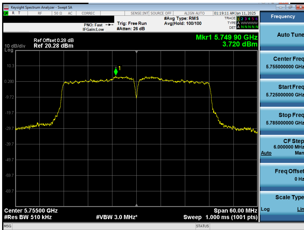
Plot 7-66. PSD CDD Primary Antenna 3b (40MHz BW 802.11n – Ch. 151)
