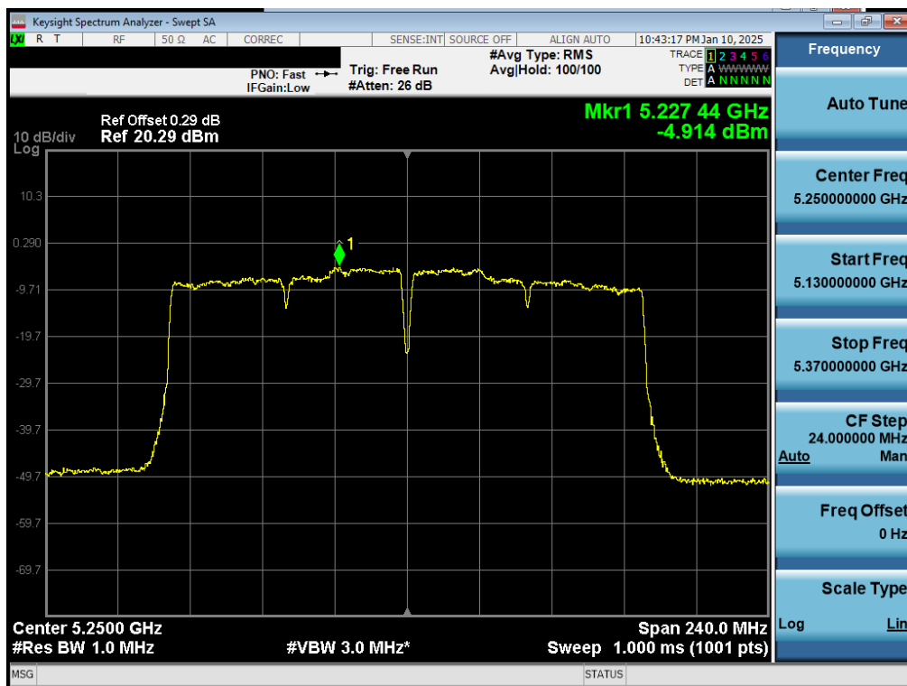
Plot 7-36. PSD Antenna 3b (160MHz BW 802.11ac – Ch. 50)
