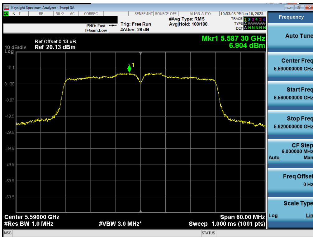
Plot 7-34. PSD Antenna 3b (40MHz BW 802.11n – Ch. 118)
