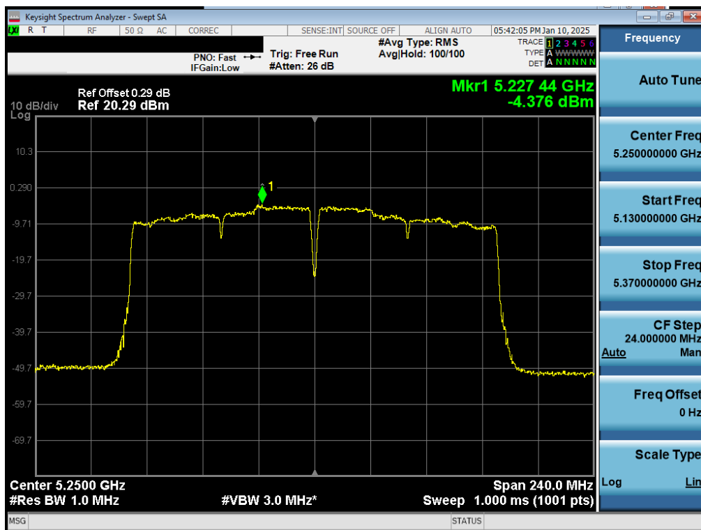
Plot 7-25. PSD Antenna 5T (160MHz BW 802.11ac – Ch. 50)
