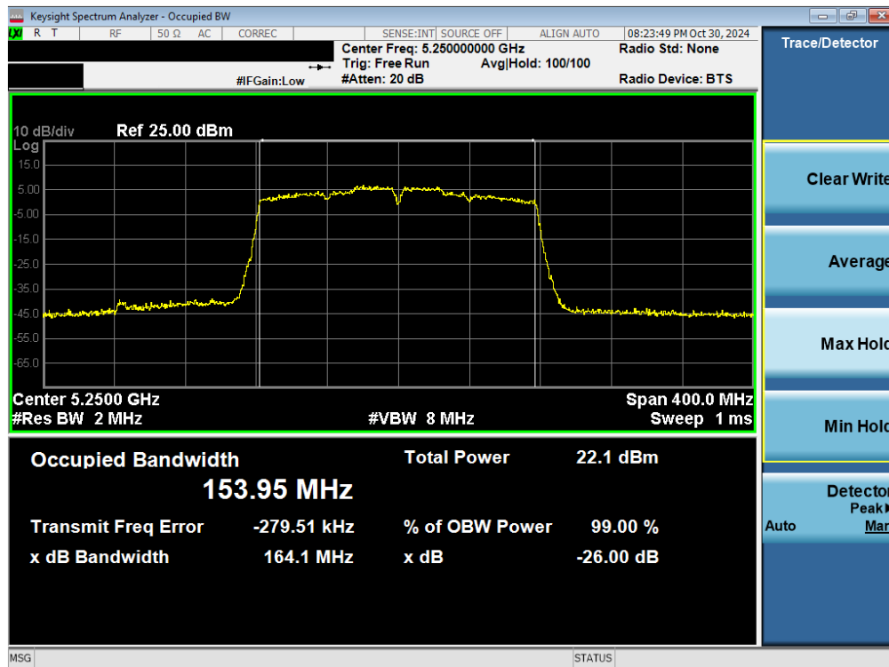
Plot 7-4. 26dB BW & 99% OBW Antenna 5T (160MHz BW 802.11ac – Ch. 50)
