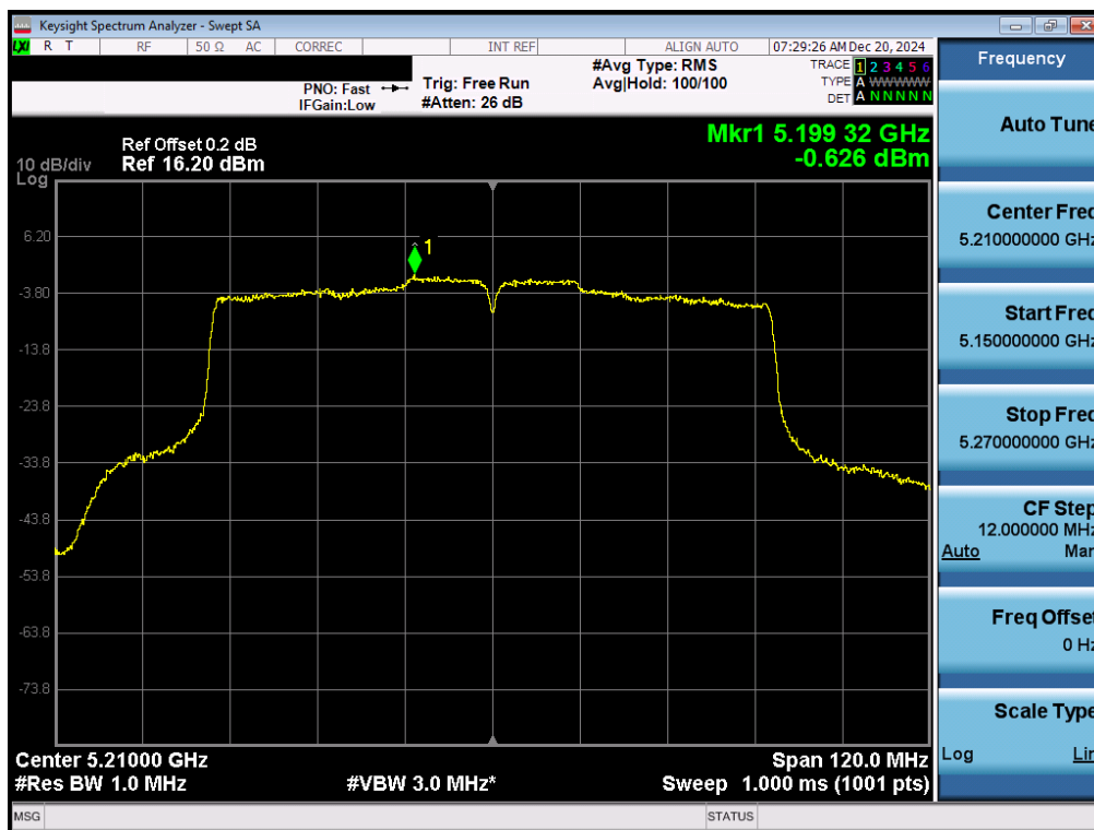
Plot 7-74. ISED PSD SDM Primary Antenna 3b (80MHz BW 11ac – Ch.42)
