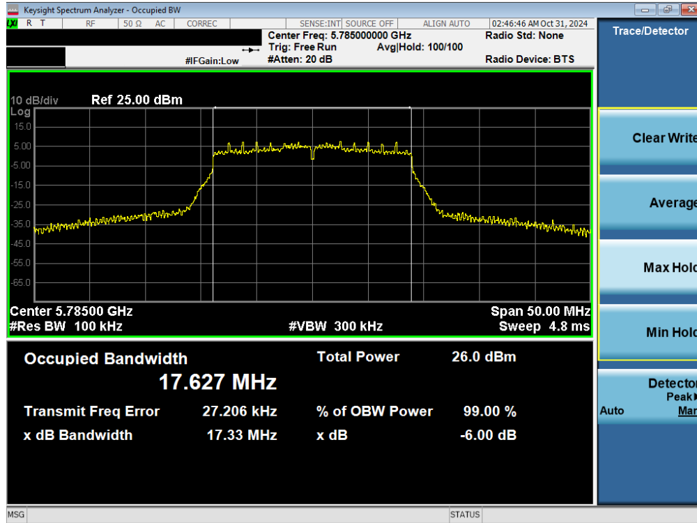
Plot 7-16. 6dB BW & 99% OBW Antenna 3b (20MHz BW 802.11n – Ch. 157)
