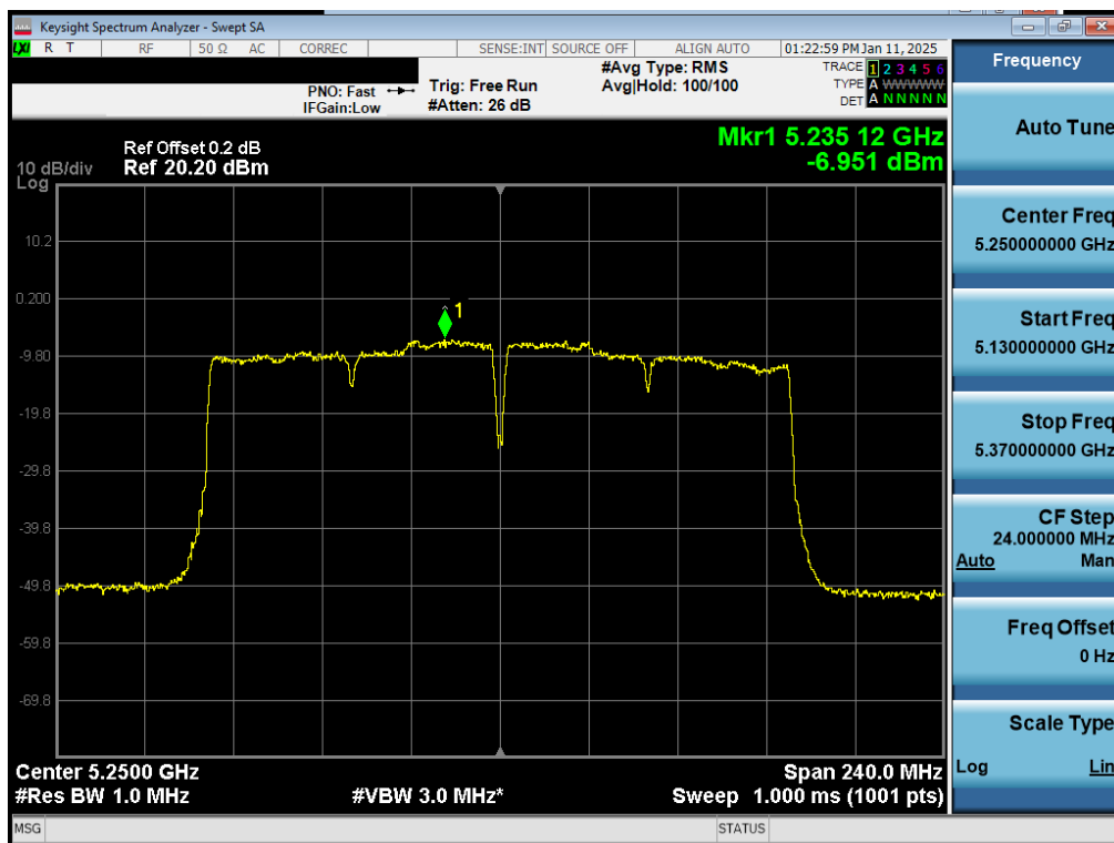
Plot 7-84. PSD CDD Diversity Antenna 3b (160MHz BW 802.11ac – Ch. 50)
