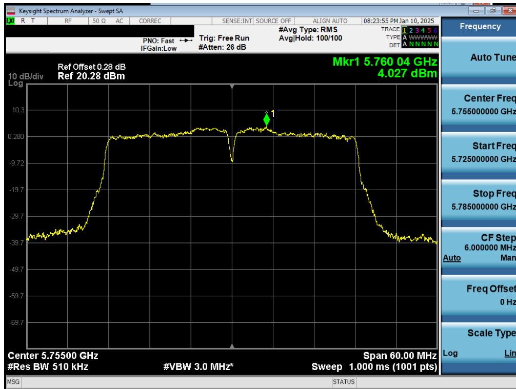
Plot 7-87. PSD CDD Diversity Antenna 5T (40MHz BW 802.11n – Ch. 151)
