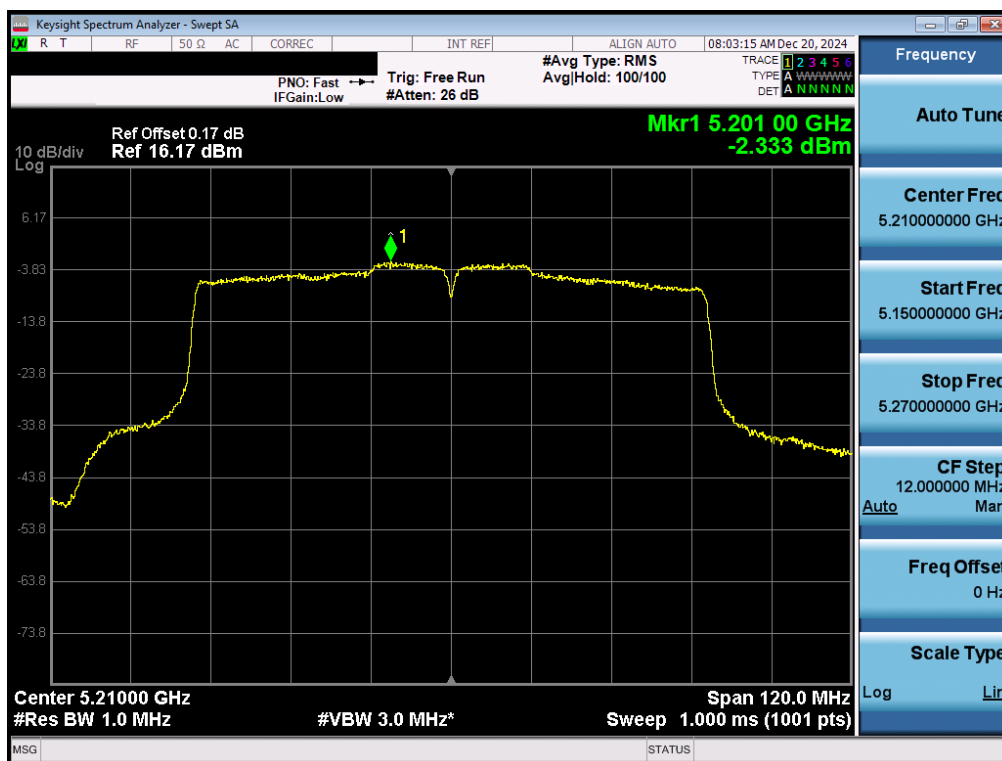
Plot 7-53. ISED PSD Antenna 1b (80MHz BW 11ac – Ch.42)
