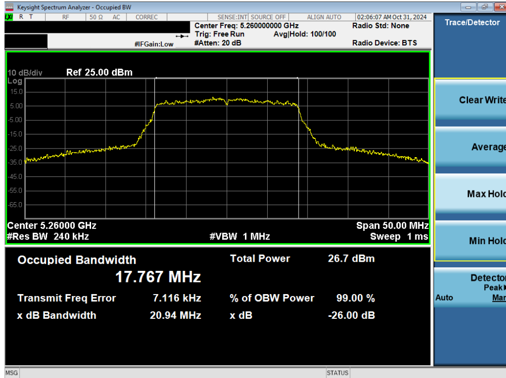
Plot 7-5. 26dB BW & 99% OBW Antenna 3b (20MHz BW 802.11n – Ch. 52)
