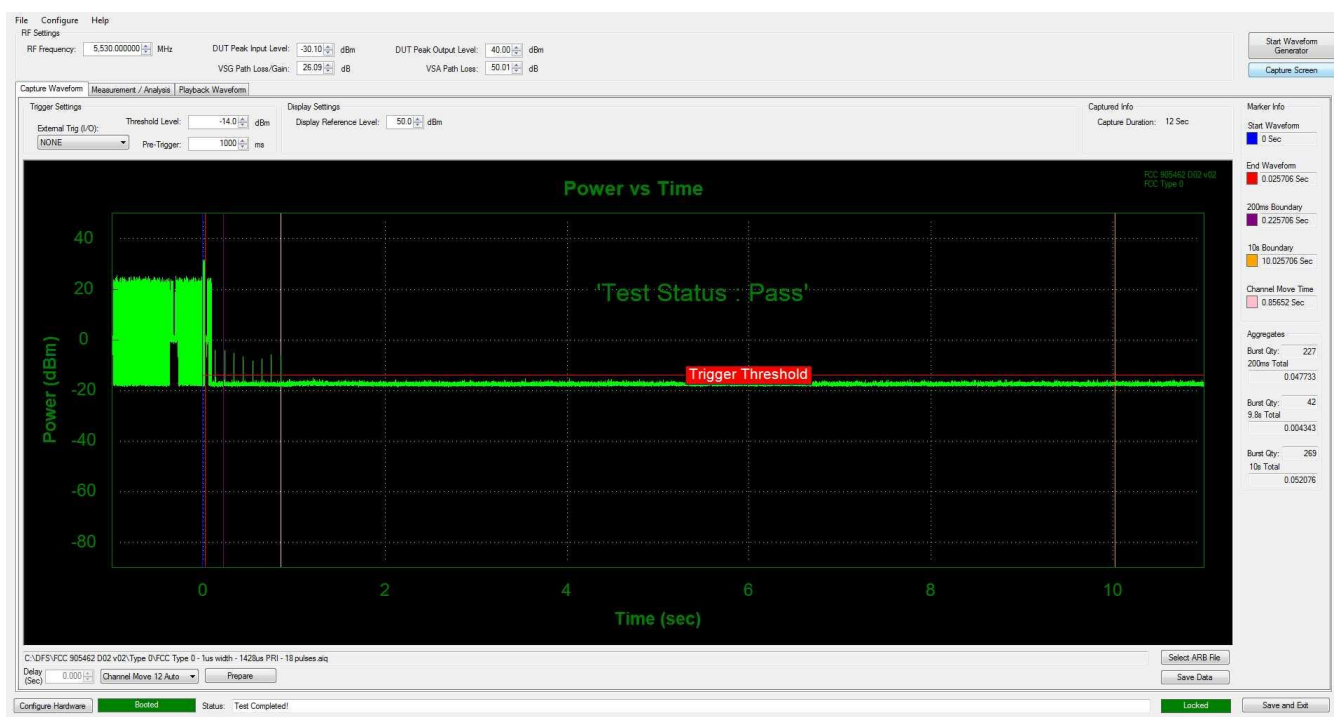
Figure 9-15. 5530MHz - Channel Move/ Closing Transmission Time - Mode 4 (80 MHz)
