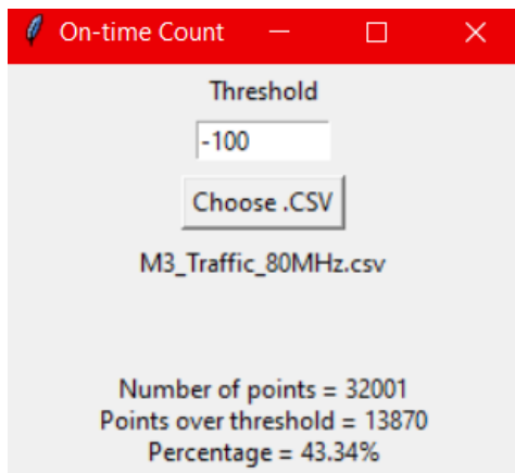
Figure 9-8. 5530MHz - Channel Loading Calculation - Mode 3 (80MHz)
