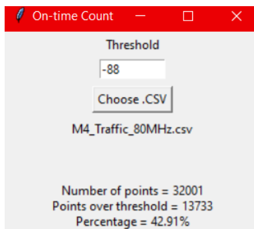
Figure 9-10. 5530MHz - Channel Loading Calculation - Mode 4 (80MHz)
