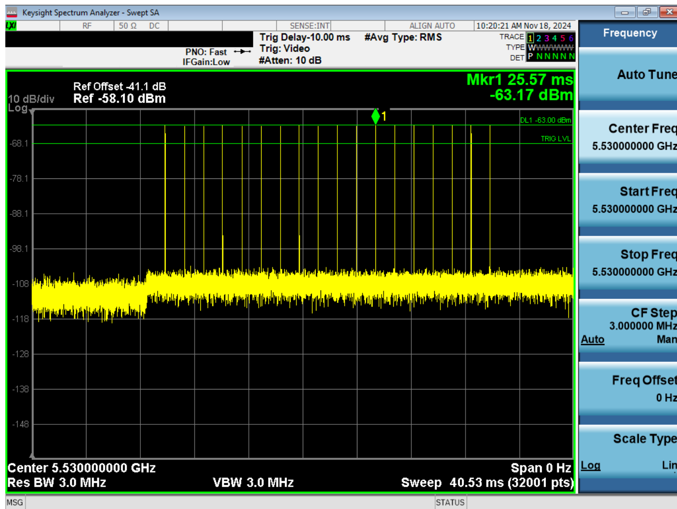
Figure 7-3. 5530MHz – Radar Pulse Type 0 (80MHz)
