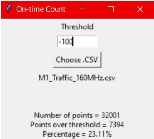
Figure 9-4. 5570MHz - Channel Loading Calculation - Mode 1 (160MHz)
