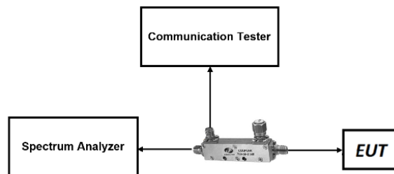
Figure 7-7. LTE Test Instrument & Measurement Setup
