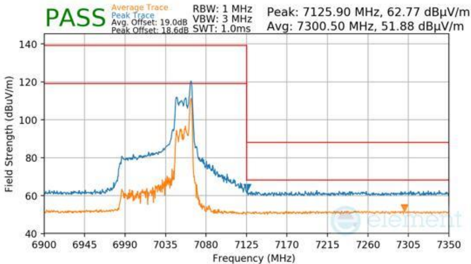
Plot 7-1166 CDD Diversity Radiated Upper Band Edge (Peak & Average – UNII Band 8)
