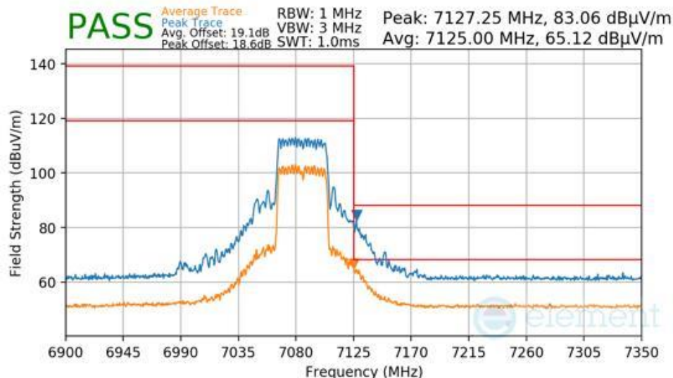
Plot 7-1138 CDD Primary Radiated Upper Band Edge (Peak & Average – UNII Band 8)
