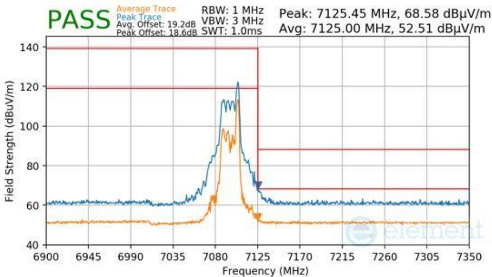
Plot 7-1130 CDD Primary Radiated Upper Band Edge (Peak & Average – UNII Band 8)
