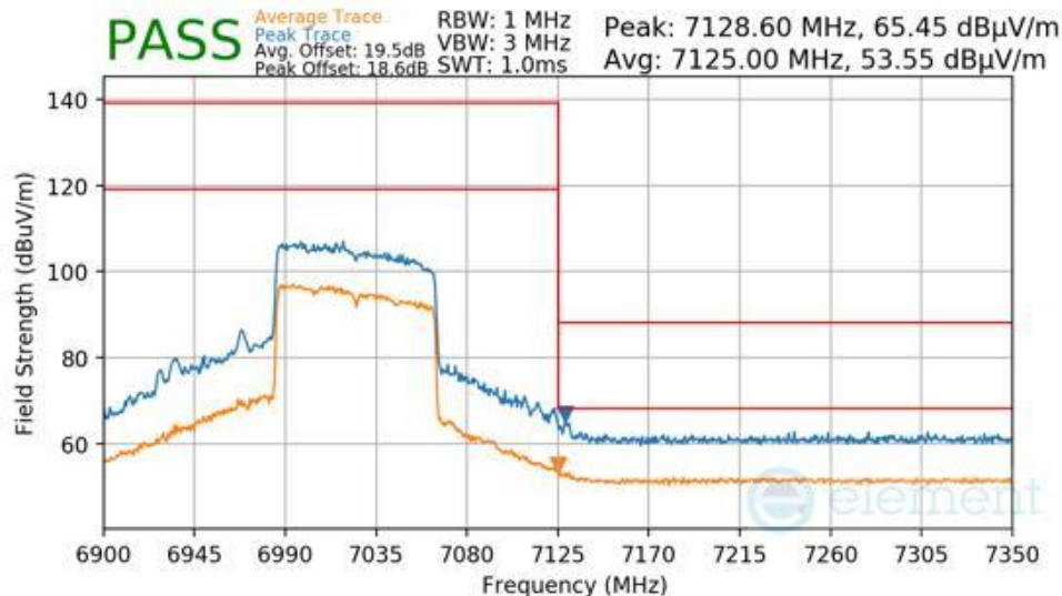
Plot 7-1120 Antenna WF7b Radiated Upper Band Edge (Peak & Average – UNII Band 8)
