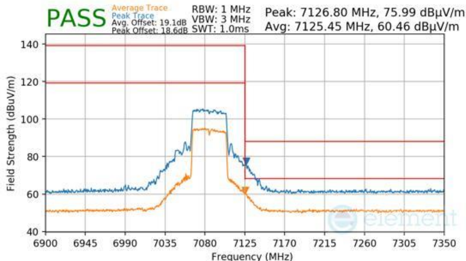
Plot 7-1114 Antenna WF7b Radiated Upper Band Edge (Peak & Average – UNII Band 8)
