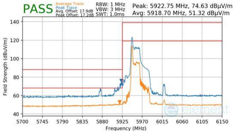
Plot 7-1109 Antenna WF7b Radiated Lower Band Edge (Peak & Average – UNII Band 5)
