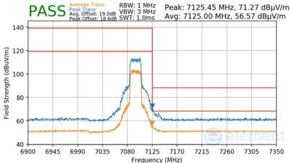
Plot 7-1156 CDD Diversity Radiated Upper Band Edge (Peak & Average – UNII Band 8)
