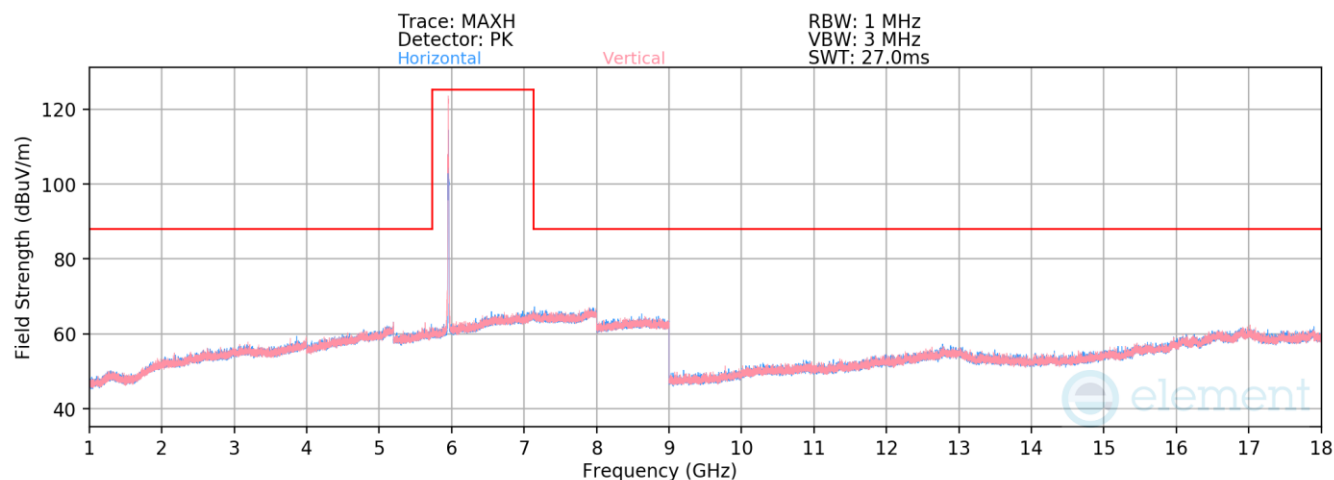
Plot 7-1021. Radiated Spurious Emissions above 1GHz SDM Diversity (802.11ax – Ch. 1 – RU26)
