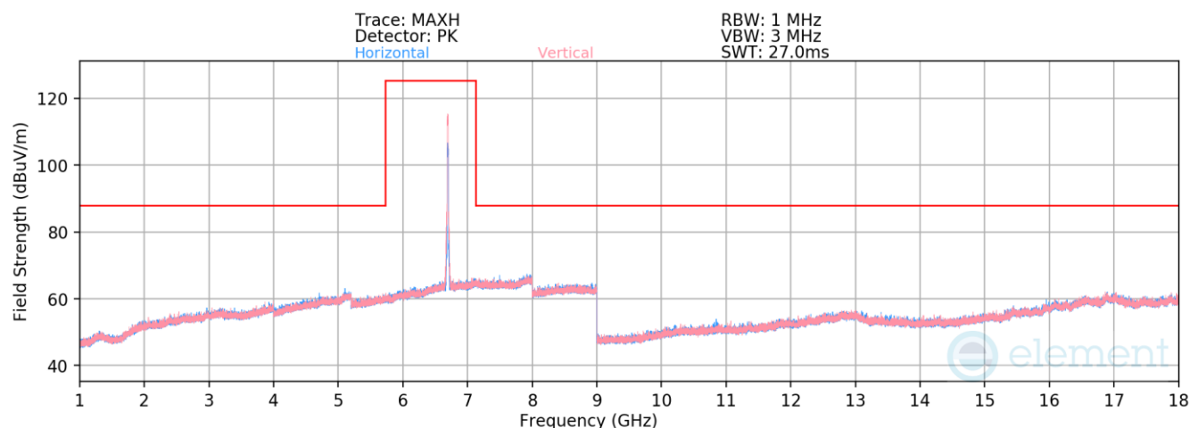
Plot 7-1014. Radiated Spurious Emissions above 1GHz SDM Primary (802.11ax – Ch. 149 – RU242)
