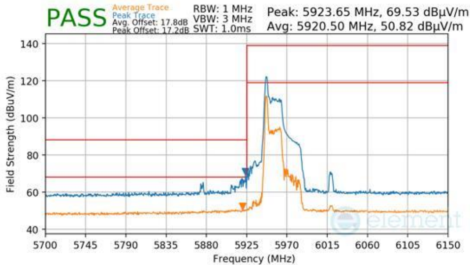
Plot 7-1085 Antenna WF2a Radiated Lower Band Edge (Peak & Average – UNII Band 5)
