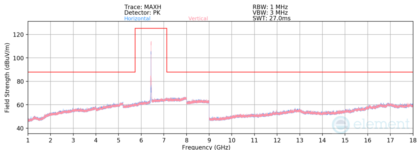
Plot 7-1041. Radiated Spurious Emissions above 1GHz SDM Diversity (802.11ax – Ch. 97 – RU242)
