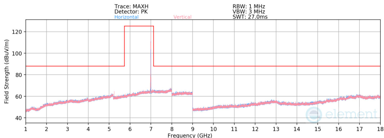
Plot 7-1034. Radiated Spurious Emissions above 1GHz SDM Diversity (802.11ax – Ch. 209 – RU26)
