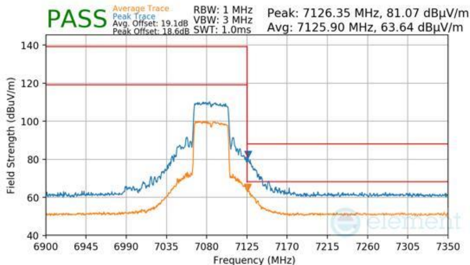
Plot 7-1090 Antenna WF2a Radiated Upper Band Edge (Peak & Average – UNII Band 8)
