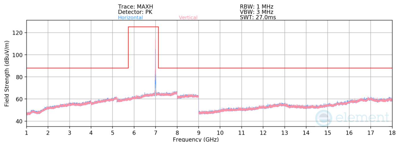
Plot 7-1050. Radiated Spurious Emissions above 1GHz SDM Diversity (802.11ax – Ch. 209 – RU242)
