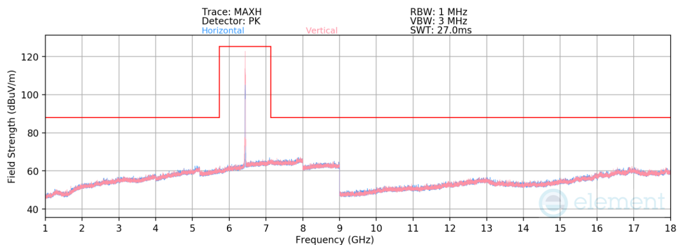
Plot 7-993. Radiated Spurious Emissions above 1GHz SDM Primary (802.11ax – Ch. 97 – RU26)
