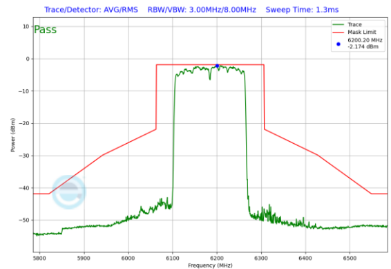
Plot 7-904. In-Band Emission Plot SDM Diversity Antenna WF7b (160MHz 802.11ax RU996x2 (UNII Band 5) – Ch. 47)
