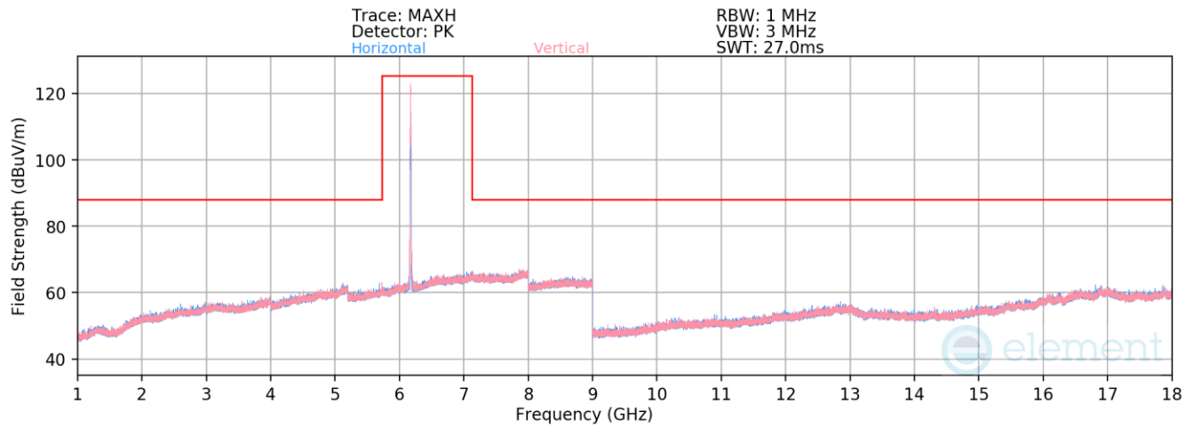
Plot 7-991. Radiated Spurious Emissions above 1GHz SDM Primary (802.11ax – Ch. 45 – RU26)
