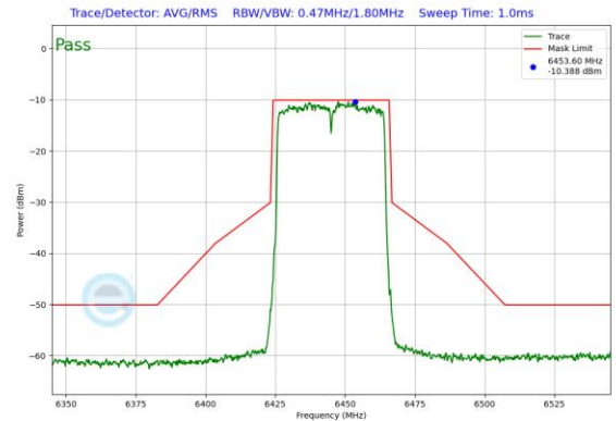
Plot 7-916. In-Band Emission Plot SDM Diversity Antenna WF7b (40MHz 802.11ax RU484 (UNII Band 6) – Ch. 99)
