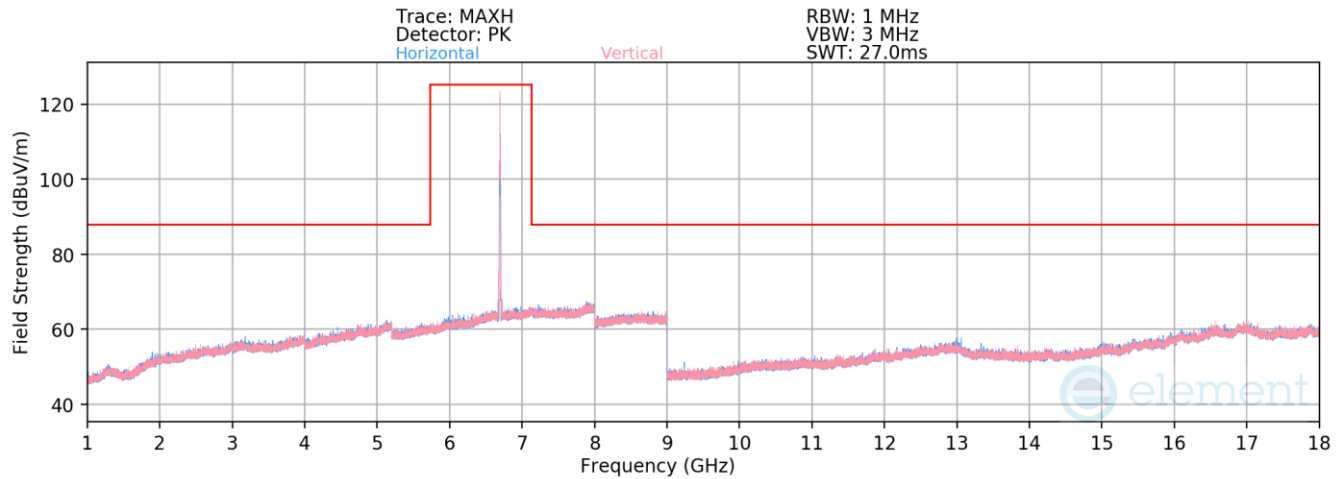
Plot 7-998. Radiated Spurious Emissions above 1GHz SDM Primary (802.11ax – Ch. 149 – RU26)
