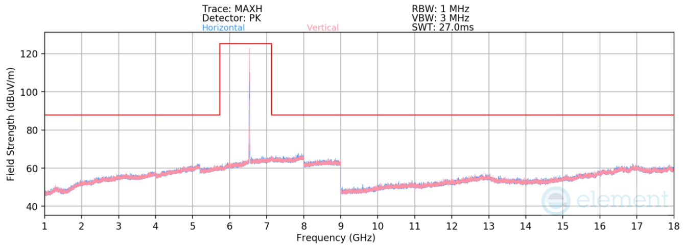
Plot 7-997. Radiated Spurious Emissions above 1GHz SDM Primary (802.11ax – Ch. 117 – RU26)
