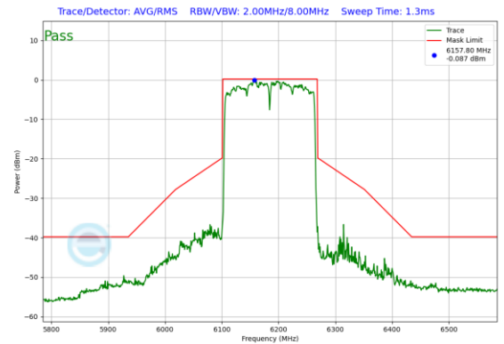
Plot 7-648. In-Band Emission Plot Antenna WF2a (160MHz 802.11ax RU26 (UNII Band 5) – Ch. 47)
