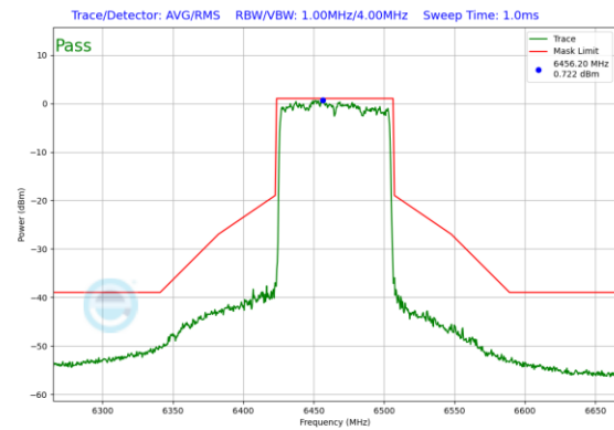
Plot 7-631. In-Band Emission Plot Antenna WF2a (80MHz 802.11ax RU996 (UNII Band 6) – Ch. 103)
