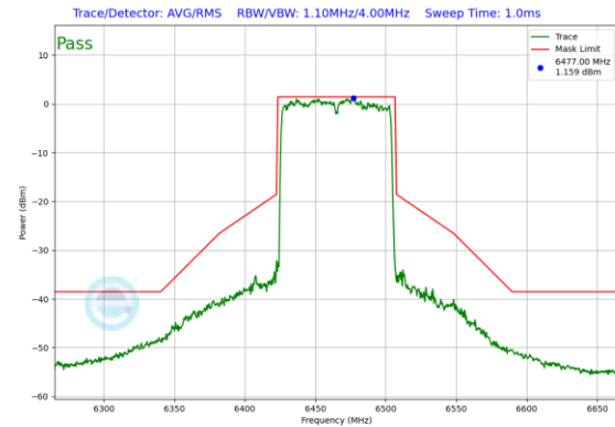
Plot 7-687. In-Band Emission Plot Antenna WF7b (80MHz 802.11ax RU996 (UNII Band 6) – Ch. 103)
