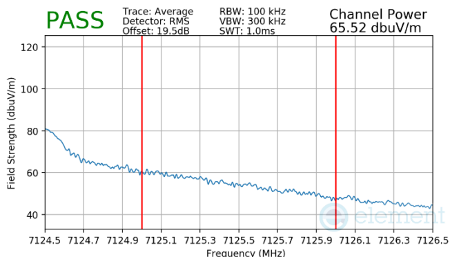
Plot 7-616. CDD/SDM Diversity Radiated Upper Band Edge (Average – UNII Band 8)
