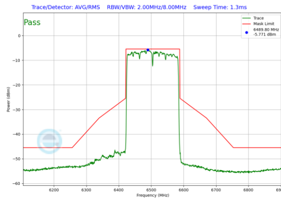
Plot 7-459. Power Spectral Density Plot SDM Diversity Antenna WF7b (160MHz 802.11ax (UNII Band 6) – Ch. 111)
