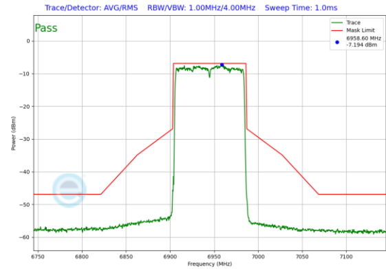
Plot 7-473. Power Spectral Density Plot SDM Diversity Antenna WF7b (80MHz 802.11ax (UNII Band 8) – Ch. 199)
