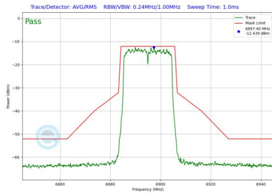
Plot 7-413. Power Spectral Density Plot SDM Primary Antenna WF7a (20MHz 802.11ax (UNII Band 8) – Ch. 189)
