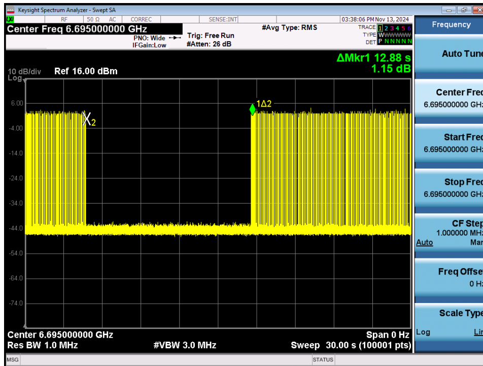
Plot 7-501. Contention Based Protocol Timing Plot – UNII 7 – 20MHz Channel 149
