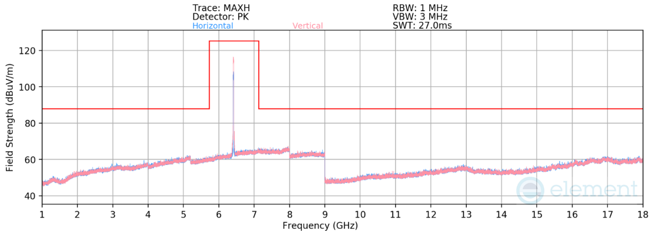
Plot 7-516. Radiated Spurious Emissions 1-18GHz CDD/SDM Primary (802.11ax – Ch. 93)
