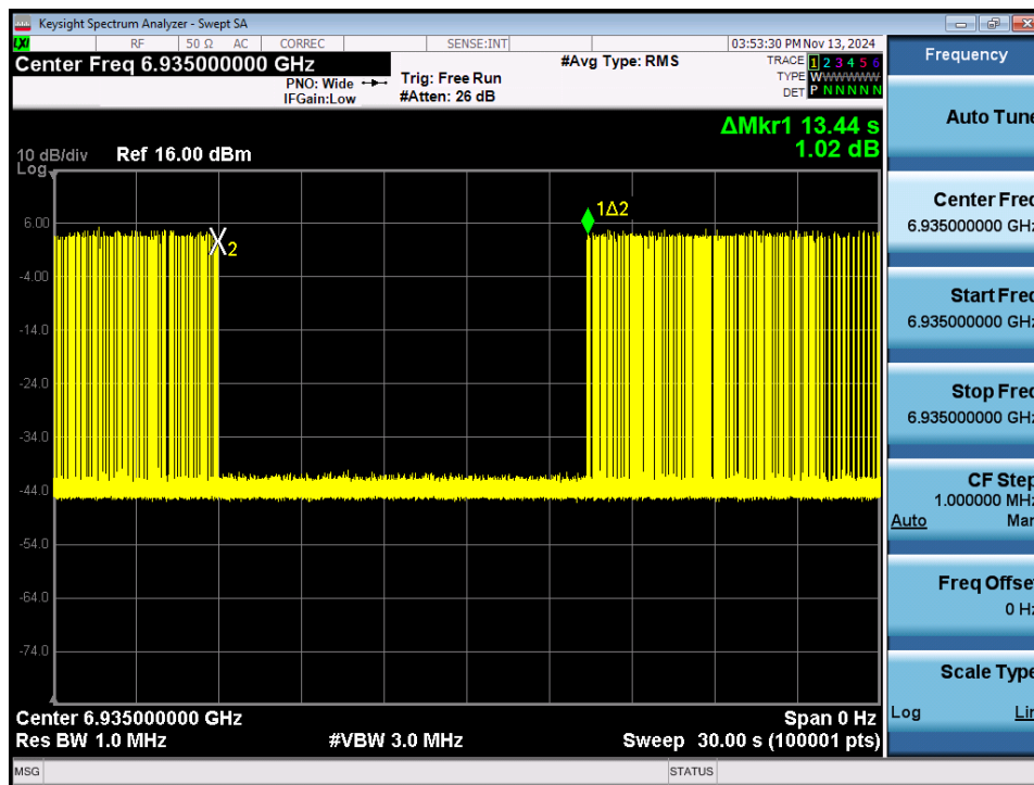
Plot 7-505. Contention Based Protocol Timing Plot – UNII 8 – 20MHz Channel 197
