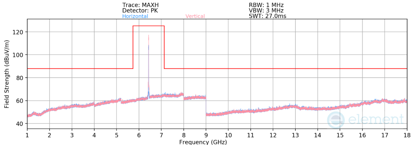
Plot 7-517. Radiated Spurious Emissions 1-18GHz CDD/SDM Primary (802.11ax – Ch. 97)
