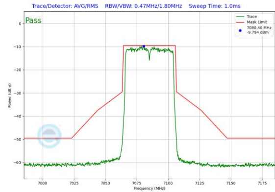
Plot 7-472. Power Spectral Density Plot SDM Diversity Antenna WF2a (40MHz 802.11ax (UNII Band 8) – Ch. 227)
