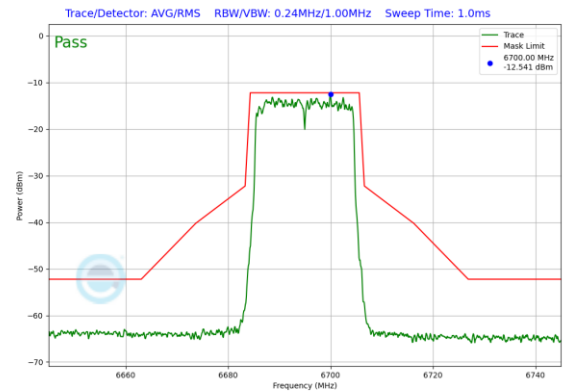
Plot 7-461. Power Spectral Density Plot SDM Diversity Antenna WF7b (20MHz 802.11ax (UNII Band 7) – Ch. 149)
