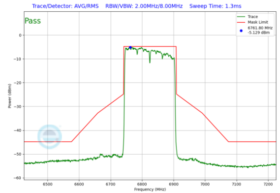
Plot 7-468. Power Spectral Density Plot SDM Diversity Antenna WF2a (160MHz 802.11ax (UNII Band 7) – Ch. 175)
