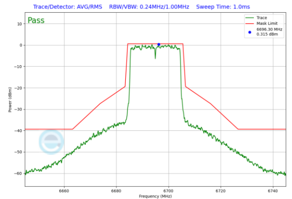
Plot 7-437. Power Spectral Density Plot CDD Diversity Antenna WF7b (20MHz 802.11ax (UNII Band 7) – Ch. 149)
