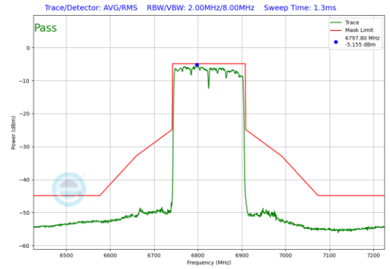
Plot 7-467. Power Spectral Density Plot SDM Diversity Antenna WF7b (160MHz 802.11ax (UNII Band 7) – Ch. 175)
