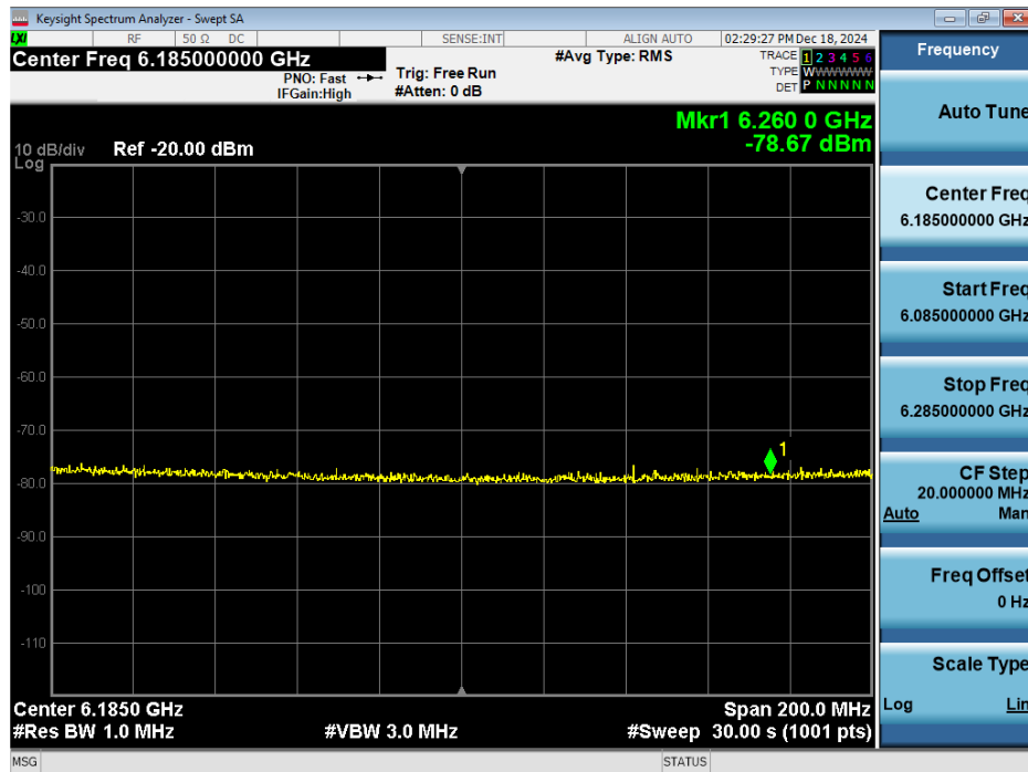
Plot 7-511. 160MHz Bandwidth, AWGN Signal Injected at Center – Channel 47
