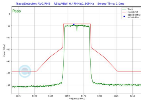
Plot 7-447. Power Spectral Density Plot SDM Diversity Antenna WF7b (40MHz 802.11ax (UNII Band 5) – Ch. 43)
