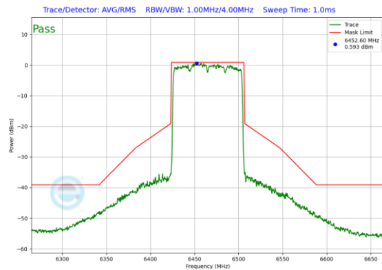
Plot 7-433. Power Spectral Density Plot CDD Diversity Antenna WF7b (80MHz 802.11ax (UNII Band 6) – Ch. 103)
