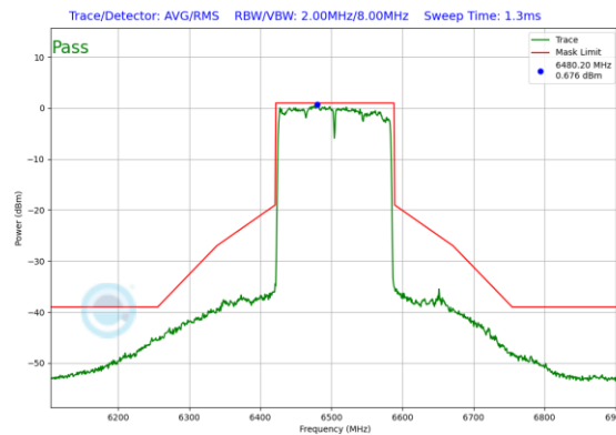
Plot 7-435. Power Spectral Density Plot CDD Diversity Antenna WF7b (160MHz 802.11ax (UNII Band 6) – Ch. 111)
