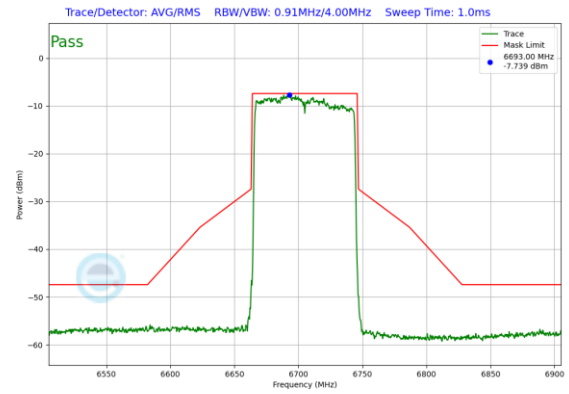
Plot 7-466. Power Spectral Density Plot SDM Diversity Antenna WF2a (80MHz 802.11ax (UNII Band 7) – Ch. 151)
