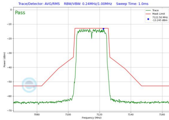
Plot 7-469. Power Spectral Density Plot SDM Diversity Antenna WF7b (20MHz 802.11ax (UNII Band 8) – Ch. 233)
