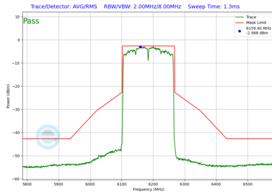
Plot 7-452. Power Spectral Density Plot SDM Diversity Antenna WF2a (160MHz 802.11ax (UNII Band 5) – Ch. 47)
