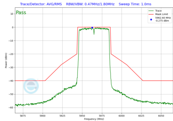
Plot 7-424. Power Spectral Density Plot CDD Diversity Antenna WF2a (40MHz 802.11ax (UNII Band 5) – Ch. 3)
