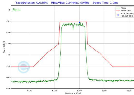
Plot 7-446. Power Spectral Density Plot SDM Diversity Antenna WF2a (20MHz 802.11ax (UNII Band 5) – Ch. 45)
