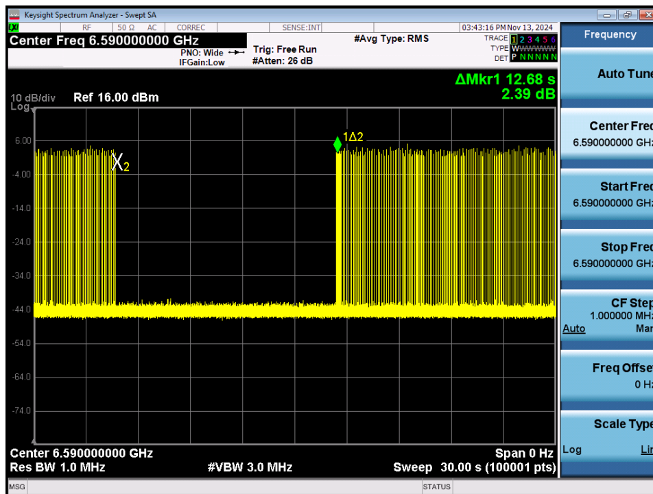
Plot 7-502. Contention Based Protocol Timing Plot – UNII 7 – 160MHz Channel 143 – Low
