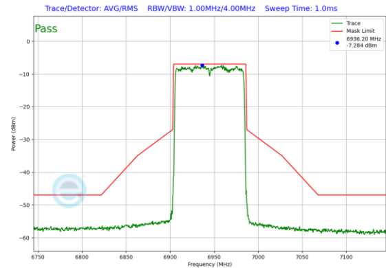
Plot 7-474. Power Spectral Density Plot SDM Diversity Antenna WF2a (80MHz 802.11ax (UNII Band 8) – Ch. 199)
