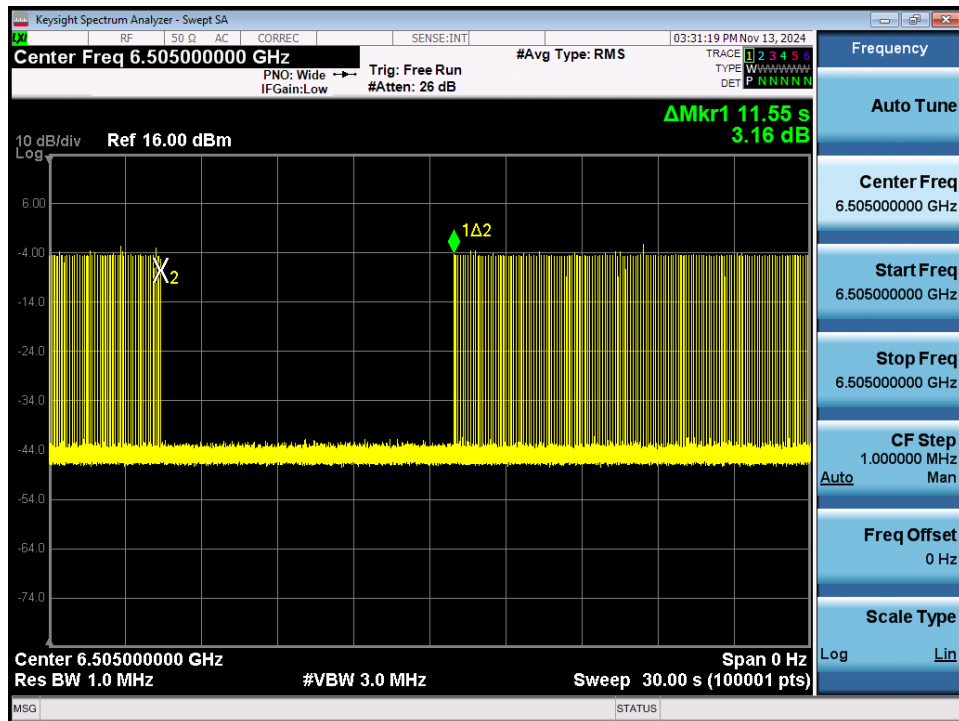
Plot 7-499. Contention Based Protocol Timing Plot – UNII 6 – 160MHz Channel 111 – Mid
