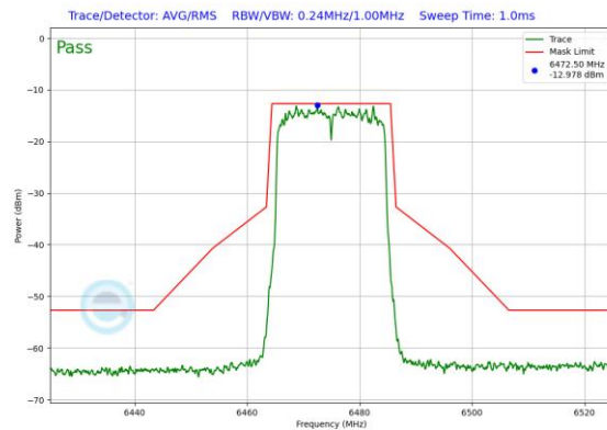
Plot 7-453. Power Spectral Density Plot SDM Diversity Antenna WF7b (20MHz 802.11ax (UNII Band 6) – Ch. 105)
