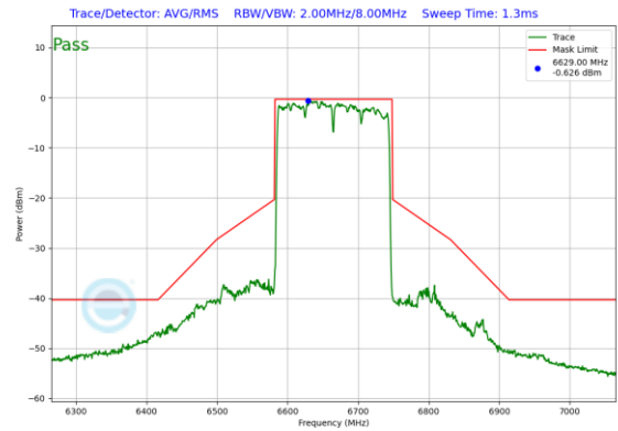
Plot 7-444. Power Spectral Density Plot CDD Diversity Antenna WF2a (160MHz 802.11ax (UNII Band 7) – Ch. 143)
