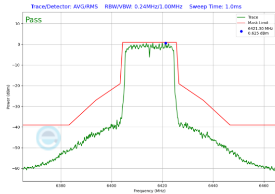
Plot 7-421. Power Spectral Density Plot CDD Diversity Antenna WF7b (20MHz 802.11ax (UNII Band 5) – Ch. 93)
