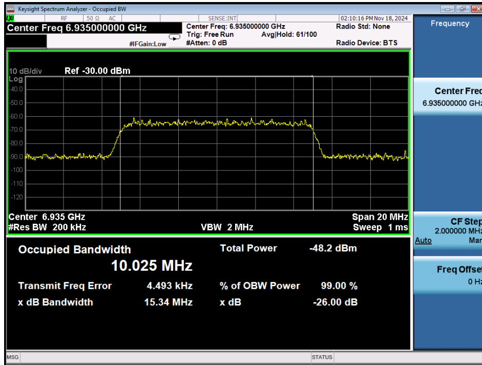
Plot 7-489. AWGN Signal – UNII 8 – 20MHz
