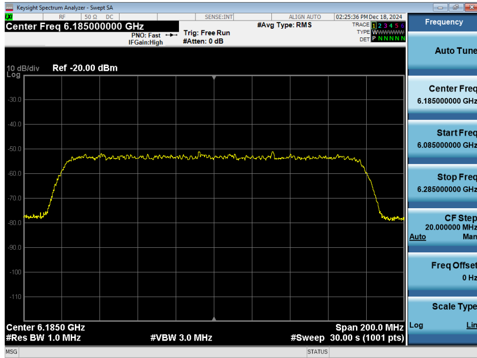
Plot 7-509. 160MHz Bandwidth, Before AWGN Signal Injected – Channel 47
