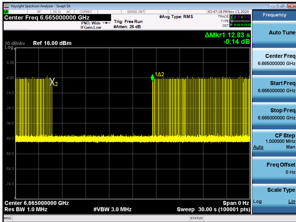
Plot 7-503. Contention Based Protocol Timing Plot – UNII 7 – 160MHz Channel 143 – Mid
