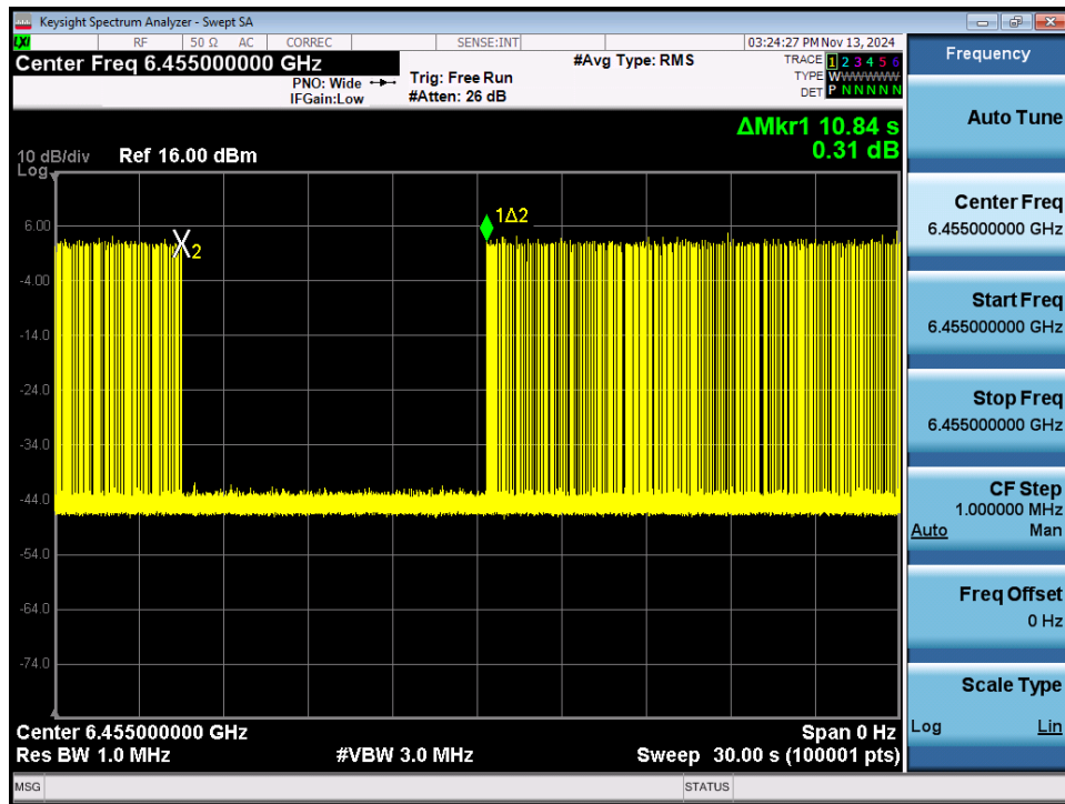
Plot 7-497. Contention Based Protocol Timing Plot – UNII 6 – 20MHz Channel 101
