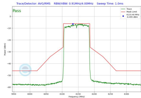
Plot 7-450. Power Spectral Density Plot SDM Diversity Antenna WF2a (80MHz 802.11ax (UNII Band 5) – Ch. 39)
