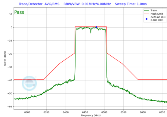
Plot 7-434. Power Spectral Density Plot CDD Diversity Antenna WF2a (80MHz 802.11ax (UNII Band 6) – Ch. 103)
