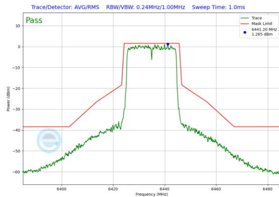
Plot 7-429. Power Spectral Density Plot CDD Diversity Antenna WF7b (20MHz 802.11ax (UNII Band 6) – Ch. 97)
