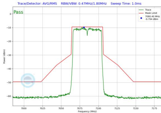
Plot 7-471. Power Spectral Density Plot SDM Diversity Antenna WF7b (40MHz 802.11ax (UNII Band 8) – Ch. 227)
