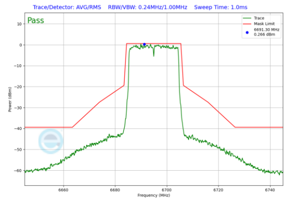
Plot 7-438. Power Spectral Density Plot CDD Diversity Antenna WF2a (20MHz 802.11ax (UNII Band 7) – Ch. 149)
