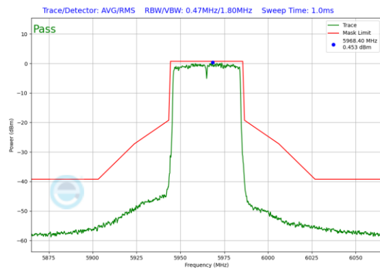
Plot 7-423. Power Spectral Density Plot CDD Diversity Antenna WF7b (40MHz 802.11ax (UNII Band 5) – Ch. 3)
