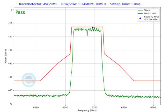
Plot 7-462. Power Spectral Density Plot SDM Diversity Antenna WF2a (20MHz 802.11ax (UNII Band 7) – Ch. 149)
