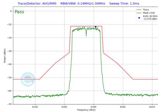
Plot 7-445. Power Spectral Density Plot SDM Diversity Antenna WF7b (20MHz 802.11ax (UNII Band 5) – Ch. 45)
