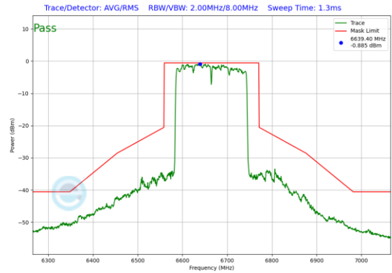
Plot 7-443. Power Spectral Density Plot CDD Diversity Antenna WF7b (160MHz 802.11ax (UNII Band 7) – Ch. 143)
