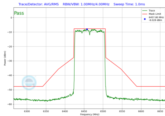
Plot 7-457. Power Spectral Density Plot SDM Diversity Antenna WF7b (80MHz 802.11ax (UNII Band 6) – Ch. 103)
