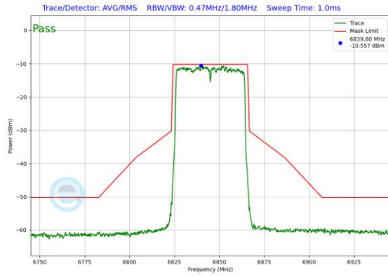
Plot 7-464. Power Spectral Density Plot SDM Diversity Antenna WF2a (40MHz 802.11ax (UNII Band 7) – Ch. 179)
