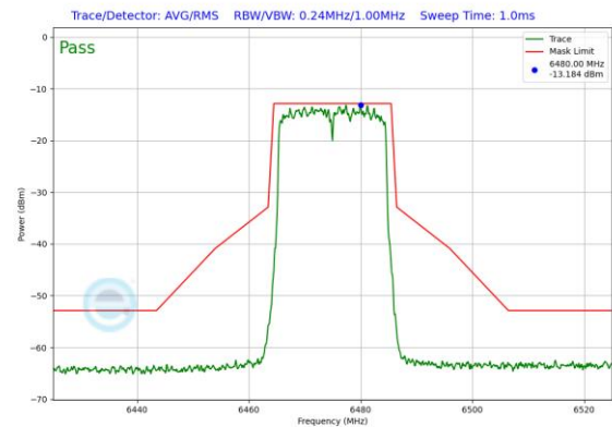
Plot 7-454. Power Spectral Density Plot SDM Diversity Antenna WF2a (20MHz 802.11ax (UNII Band 6) – Ch. 105)
