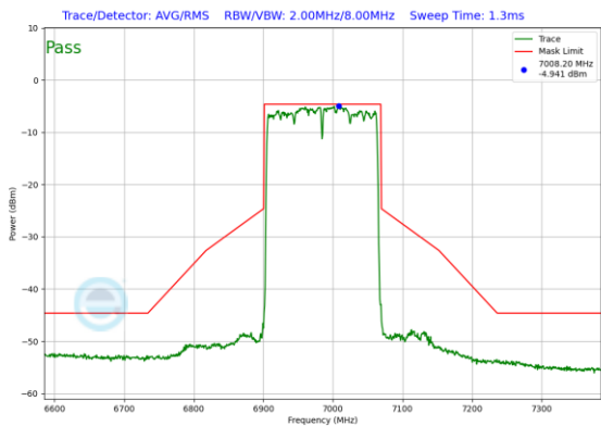
Plot 7-476. Power Spectral Density Plot SDM Diversity Antenna WF2a (160MHz 802.11ax (UNII Band 8) – Ch. 207)
