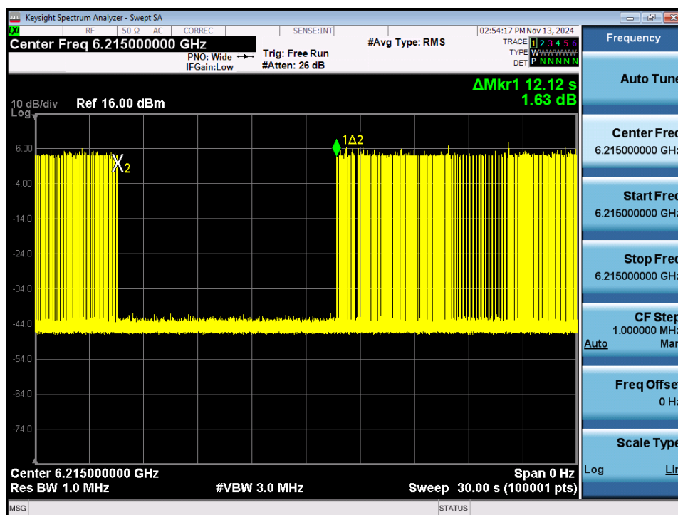
Plot 7-493. Contention Based Protocol Timing Plot – UNII 5 – 20MHz Channel 53
