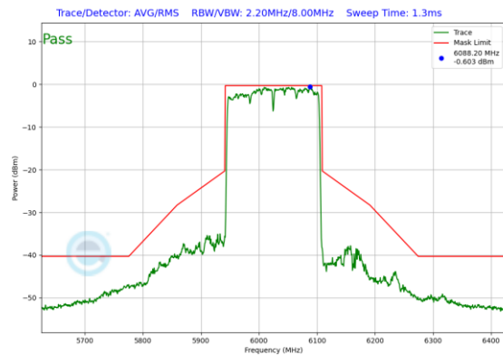
Plot 7-427. Power Spectral Density Plot CDD Diversity Antenna WF7b (160MHz 802.11ax (UNII Band 5) – Ch. 15)
