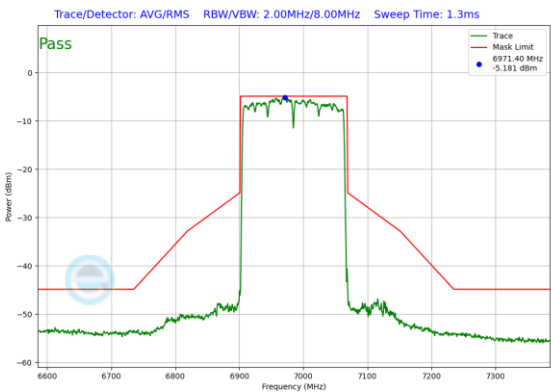
Plot 7-475. Power Spectral Density Plot SDM Diversity Antenna WF7b (160MHz 802.11ax (UNII Band 8) – Ch. 207)
