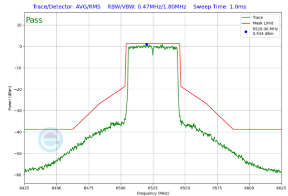
Plot 7-431. Power Spectral Density Plot CDD Diversity Antenna WF7b (40MHz 802.11ax (UNII Band 6) – Ch. 115)
