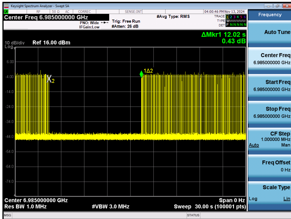
Plot 7-507. Contention Based Protocol Timing Plot – UNII 8 – 160MHz Channel 207 – Mid
