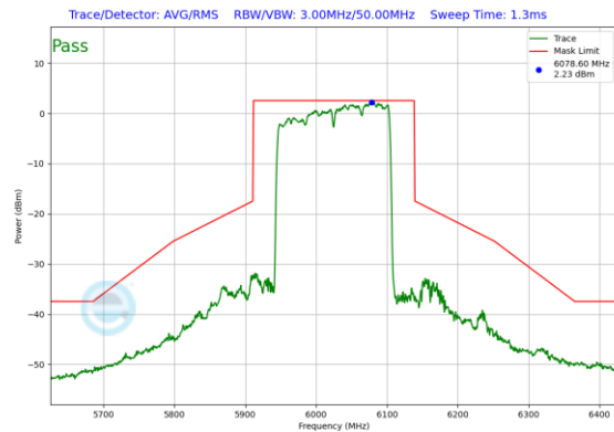
Plot 7-428. Power Spectral Density Plot CDD Diversity Antenna WF2a (160MHz 802.11ax (UNII Band 5) – Ch. 15)
