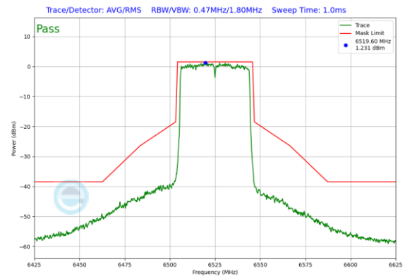
Plot 7-432. Power Spectral Density Plot CDD Diversity Antenna WF2a (40MHz 802.11ax (UNII Band 6) – Ch. 115)
