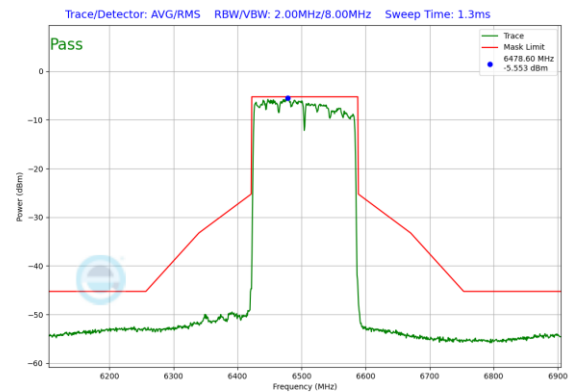
Plot 7-460. Power Spectral Density Plot SDM Diversity Antenna WF2a (160MHz 802.11ax (UNII Band 6) – Ch. 111)
