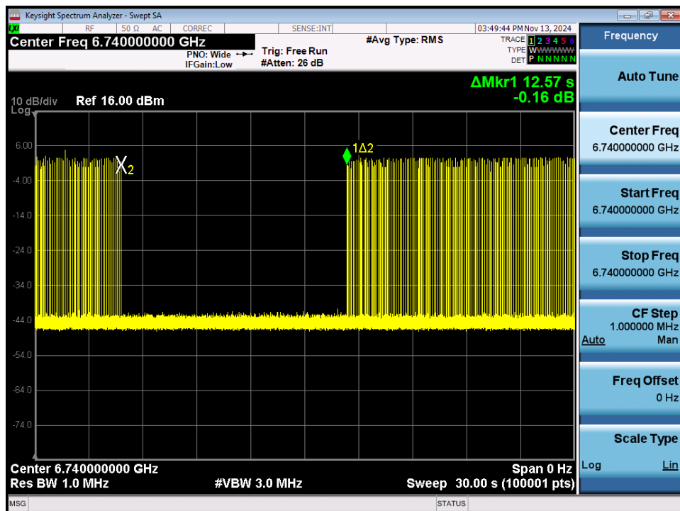
Plot 7-504. Contention Based Protocol Timing Plot – UNII 7 – 160MHz Channel 143 – High
