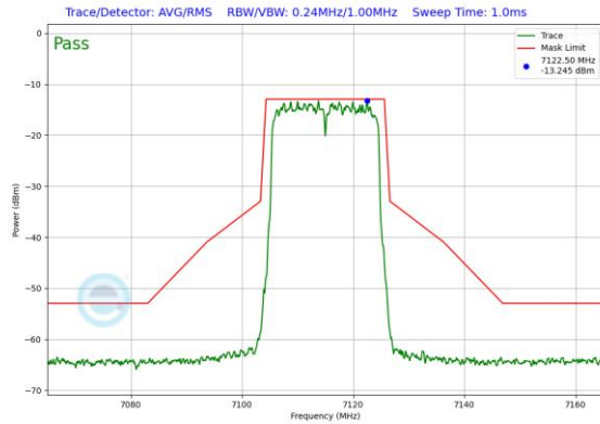
Plot 7-470. Power Spectral Density Plot SDM Diversity Antenna WF2a (20MHz 802.11ax (UNII Band 8) – Ch. 233)
