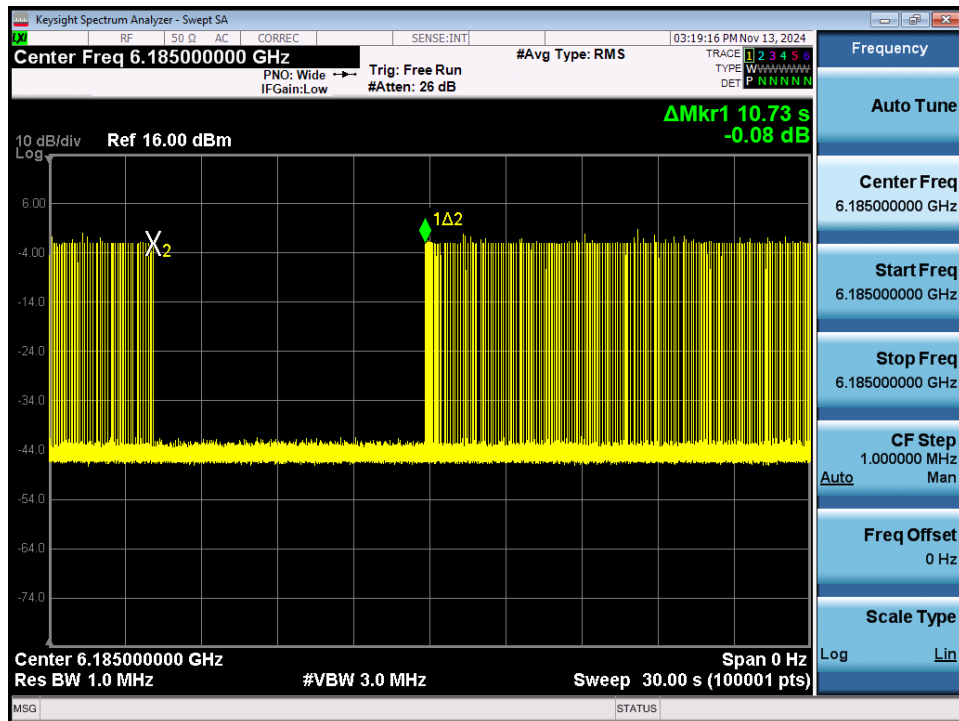
Plot 7-495. Contention Based Protocol Timing Plot –UNII 5 – 160MHz Channel 47 – Mid
