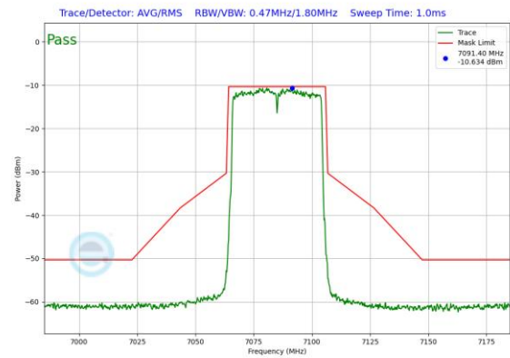
Plot 7-416. Power Spectral Density Plot SDM Primary Antenna WF2a (40MHz 802.11ax (UNII Band 8) – Ch. 227)
