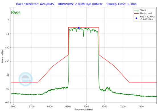
Plot 7-419. Power Spectral Density Plot SDM Primary Antenna WF7a (160MHz 802.11ax (UNII Band 8) – Ch. 207)
