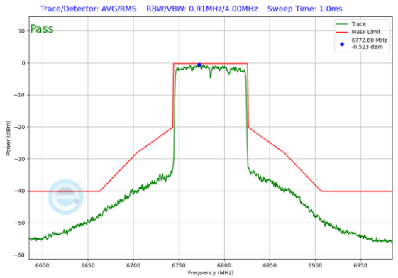
Plot 7-441. Power Spectral Density Plot CDD Diversity Antenna WF7b (80MHz 802.11ax (UNII Band 7) – Ch. 167)
