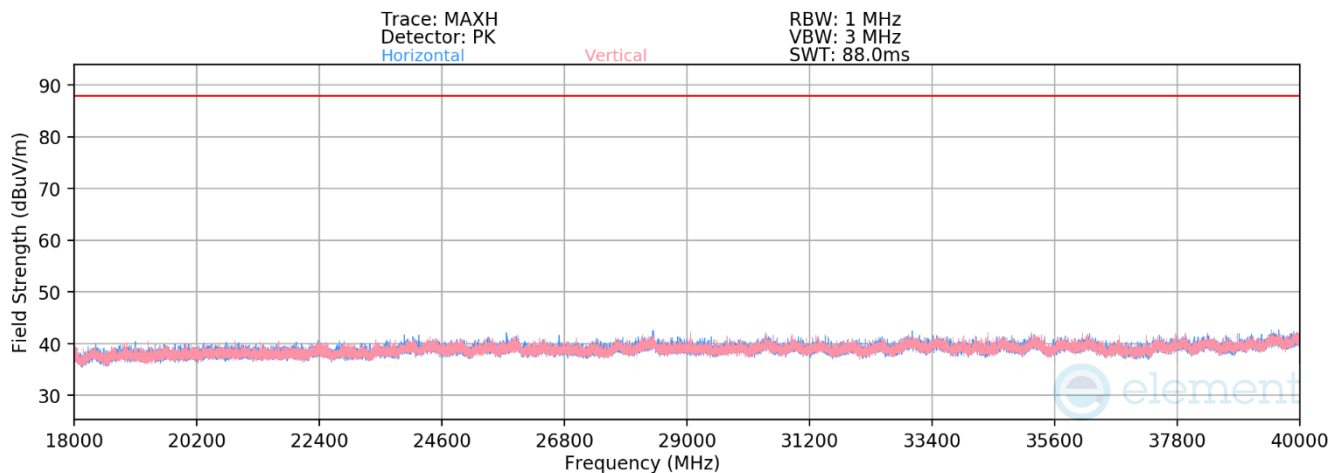
Plot 7-515. Radiated Spurious Emissions 18-40GHz CDD/SDM Primary (802.11ax – Ch. 45)
