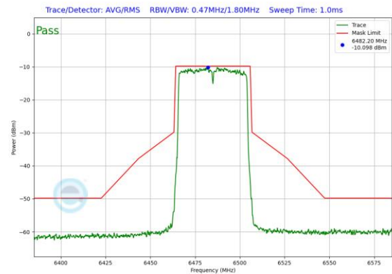
Plot 7-456. Power Spectral Density Plot SDM Diversity Antenna WF2a (40MHz 802.11ax (UNII Band 6) – Ch. 107)
