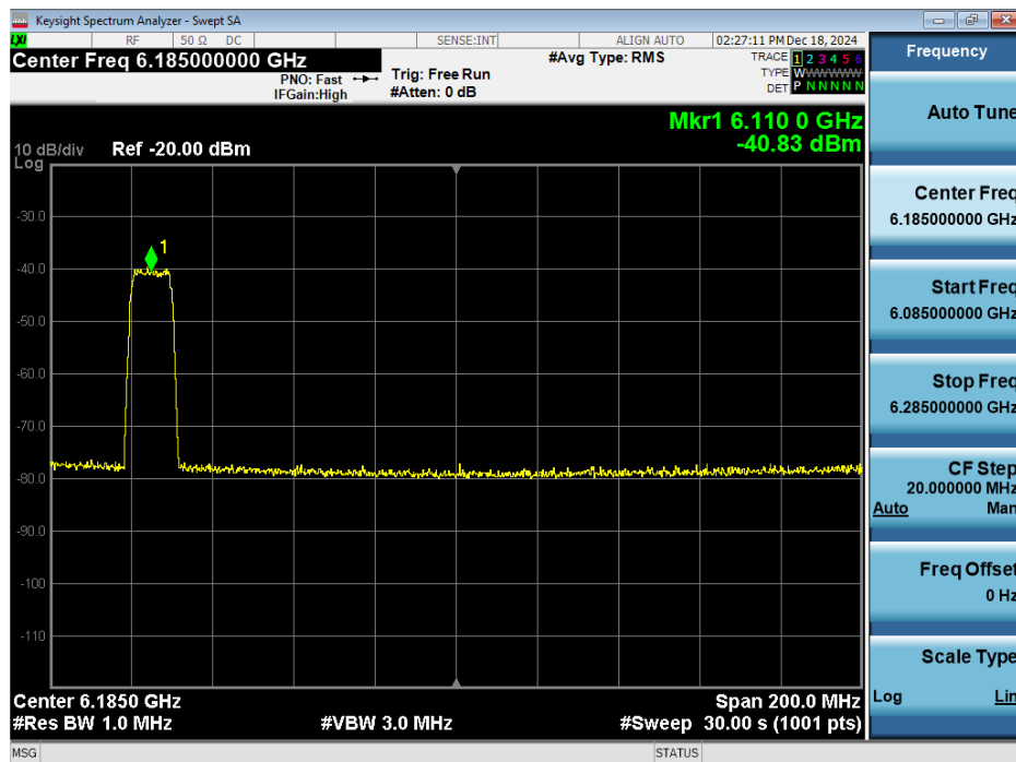
Plot 7-512. 160MHz Bandwidth, AWGN Signal Injected at High End – Channel 47
