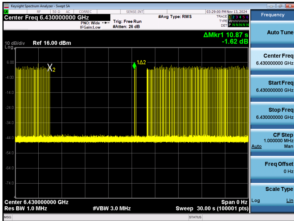
Plot 7-498. Contention Based Protocol Timing Plot – UNII 6 – 160MHz Channel 111 – Low
