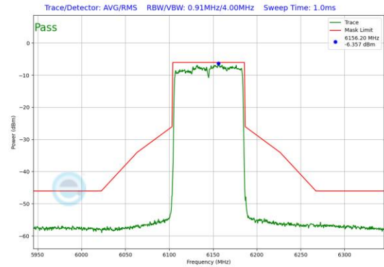
Plot 7-449. Power Spectral Density Plot SDM Diversity Antenna WF7b (80MHz 802.11ax (UNII Band 5) – Ch. 39)
