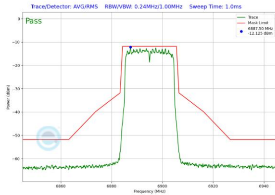
Plot 7-414. Power Spectral Density Plot SDM Primary Antenna WF2a (20MHz 802.11ax (UNII Band 8) – Ch. 189)
