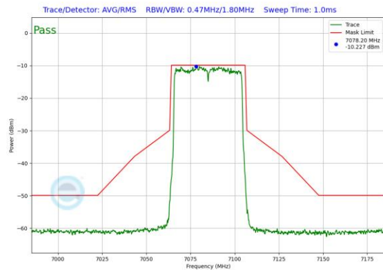
Plot 7-415. Power Spectral Density Plot SDM Primary Antenna WF7a (40MHz 802.11ax (UNII Band 8) – Ch. 227)
