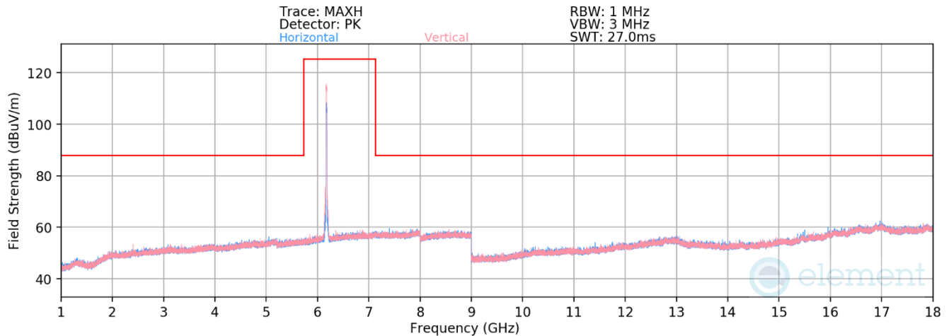
Plot 7-514. Radiated Spurious Emissions 1-18GHz CDD/SDM Primary (802.11ax – Ch. 45)
