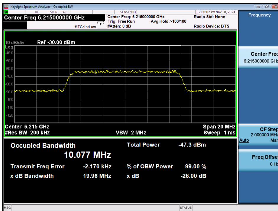
Plot 7-477. AWGN Signal – UNII 5 – 20MHz
