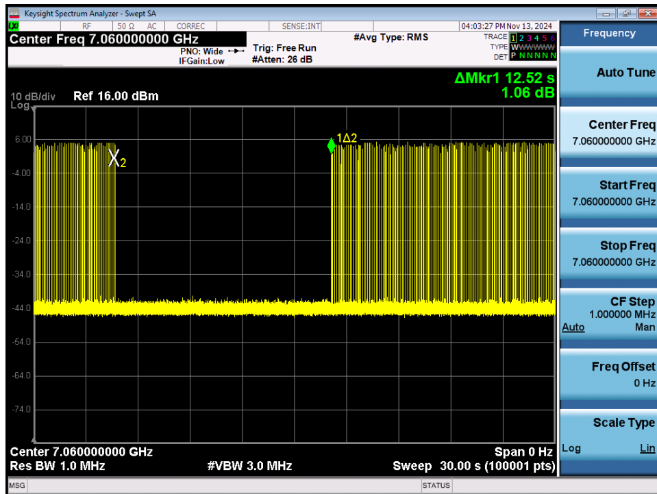
Plot 7-508. Contention Based Protocol Timing Plot – UNII 8 – 160MHz Channel 207 – High
