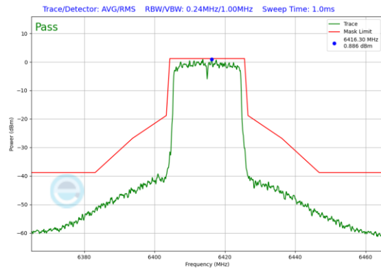
Plot 7-422. Power Spectral Density Plot CDD Diversity Antenna WF2a (20MHz 802.11ax (UNII Band 5) – Ch. 93)
