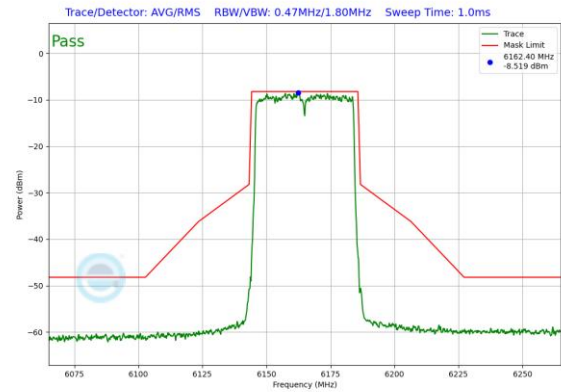
Plot 7-448. Power Spectral Density Plot SDM Diversity Antenna WF2a (40MHz 802.11ax (UNII Band 5) – Ch. 43)
