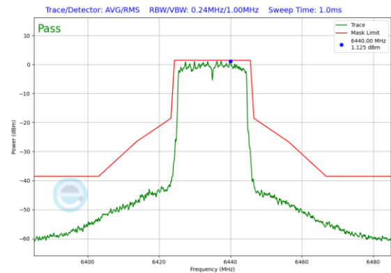
Plot 7-430. Power Spectral Density Plot CDD Diversity Antenna WF2a (20MHz 802.11ax (UNII Band 6) – Ch. 97)
