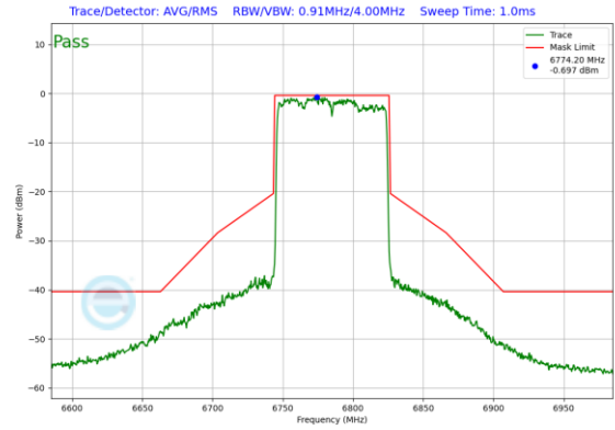
Plot 7-442. Power Spectral Density Plot CDD Diversity Antenna WF2a (80MHz 802.11ax (UNII Band 7) – Ch. 167)
