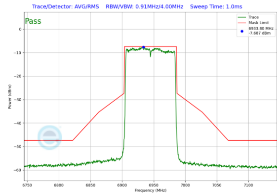
Plot 7-417. Power Spectral Density Plot SDM Primary Antenna WF7a (80MHz 802.11ax (UNII Band 8) – Ch. 199)
