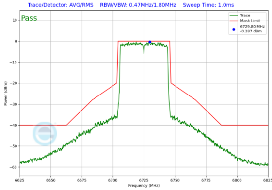
Plot 7-439. Power Spectral Density Plot CDD Diversity Antenna WF7b (40MHz 802.11ax (UNII Band 7) – Ch. 155)
