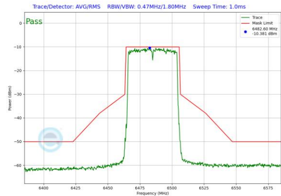
Plot 7-455. Power Spectral Density Plot SDM Diversity Antenna WF7b (40MHz 802.11ax (UNII Band 6) – Ch. 107)
