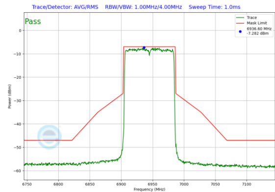
Plot 7-418. Power Spectral Density Plot SDM Primary Antenna WF2a (80MHz 802.11ax (UNII Band 8) – Ch. 199)
