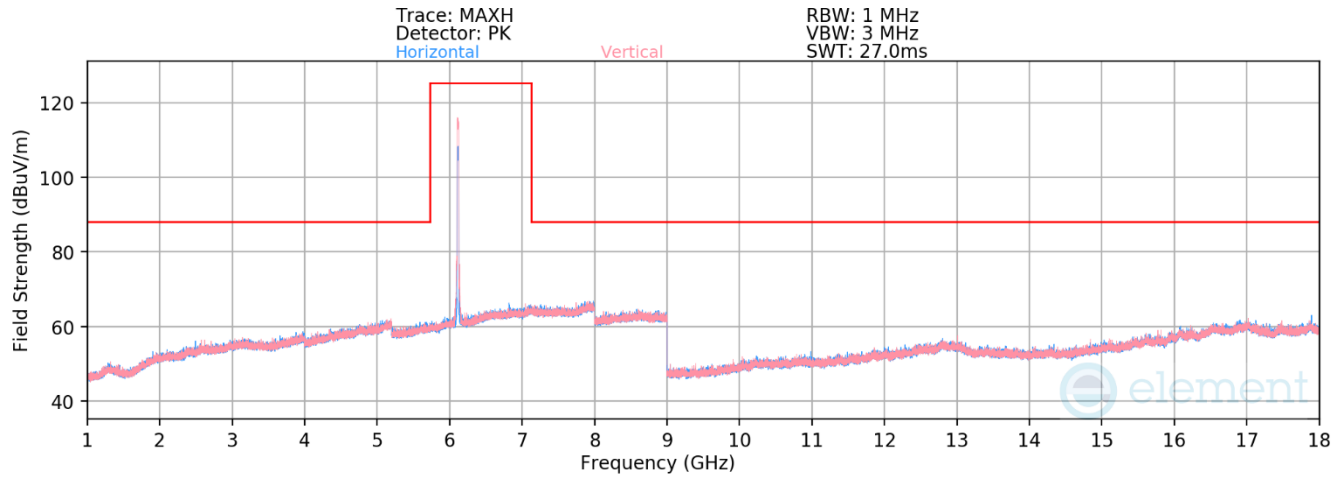
Plot 7-513. Radiated Spurious Emissions 1-18GHz CDD/SDM Primary (802.11ax – Ch. 1)
