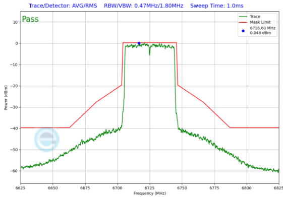
Plot 7-440. Power Spectral Density Plot CDD Diversity Antenna WF2a (40MHz 802.11ax (UNII Band 7) – Ch. 155)
