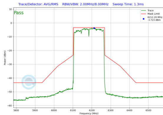
Plot 7-451. Power Spectral Density Plot SDM Diversity Antenna WF7b (160MHz 802.11ax (UNII Band 5) – Ch. 47)
