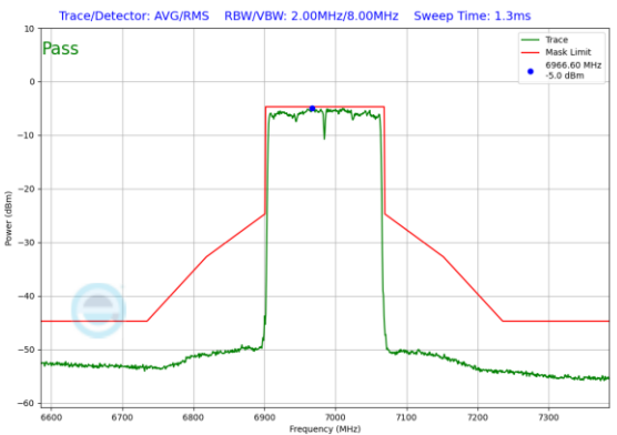
Plot 7-420. Power Spectral Density Plot SDM Primary Antenna WF2a (160MHz 802.11ax (UNII Band 8) – Ch. 207)
