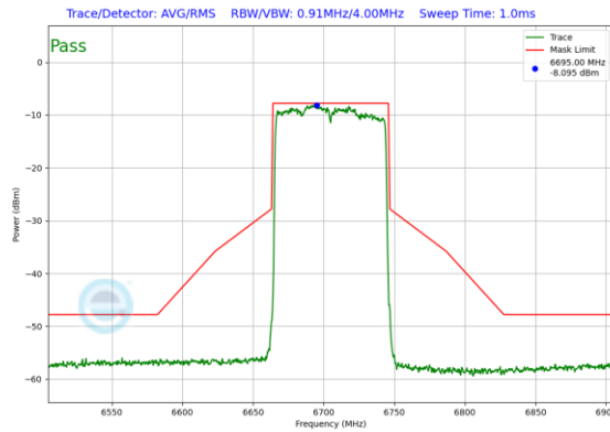
Plot 7-465. Power Spectral Density Plot SDM Diversity Antenna WF7b (80MHz 802.11ax (UNII Band 7) – Ch. 151)
