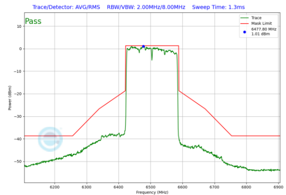
Plot 7-436. Power Spectral Density Plot CDD Diversity Antenna WF2a (160MHz 802.11ax (UNII Band 6) – Ch. 111)
