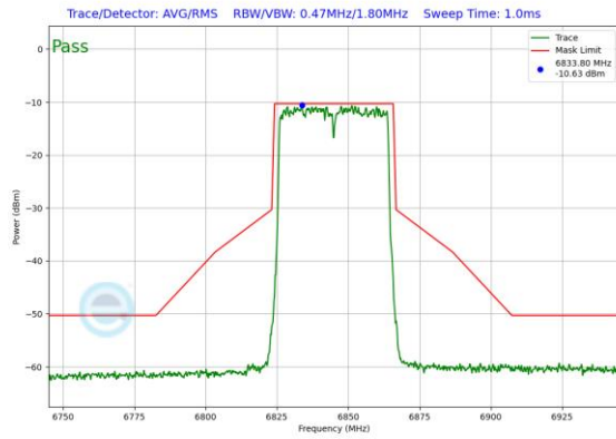
Plot 7-463. Power Spectral Density Plot SDM Diversity Antenna WF7b (40MHz 802.11ax (UNII Band 7) – Ch. 179)
