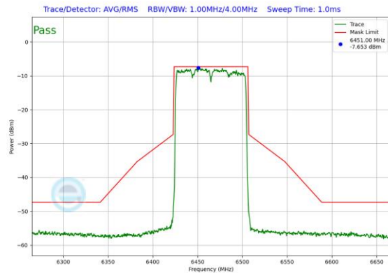
Plot 7-458. Power Spectral Density Plot SDM Diversity Antenna WF2a (80MHz 802.11ax (UNII Band 6) – Ch. 103)
