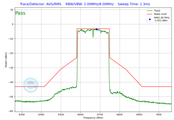
Plot 7-304. Power Spectral Density Plot Antenna WF7a (160MHz 802.11ax (UNII Band 7) – Ch. 143)
