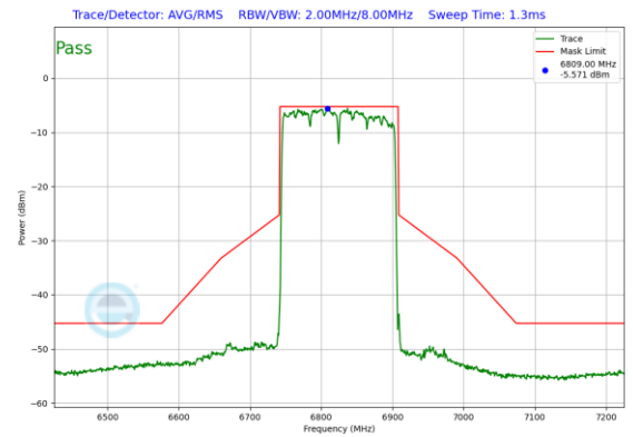
Plot 7-411. Power Spectral Density Plot SDM Primary Antenna WF7a (160MHz 802.11ax (UNII Band 7) – Ch. 175)
