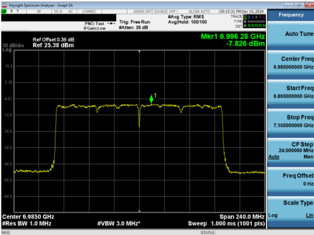
Plot 7-280. Power Spectral Density Plot SDM Diversity Antenna WF2a (160MHz 802.11ax (UNII Band 8) – Ch. 207)
