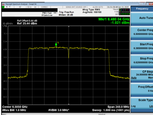
Plot 7-239. Power Spectral Density Plot CDD Diversity Antenna WF7b (160MHz 802.11ax (UNII Band 6) – Ch. 111)
