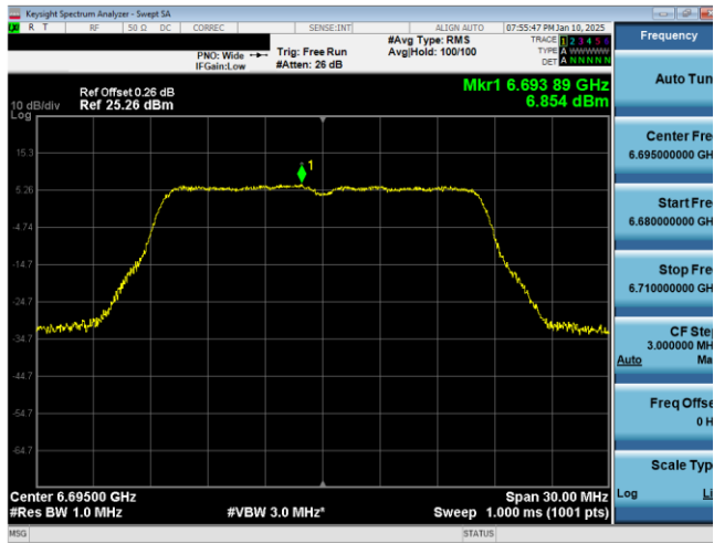
Plot 7-149. PSD Plot Antenna WF7b (20MHz 802.11a (UNII Band 7) – Ch. 149)
