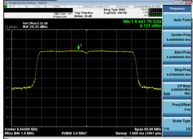
Plot 7-179. Power Spectral Density Plot CDD Primary Antenna WF7a (40MHz 802.11ax (UNII Band 6) – Ch. 99)
