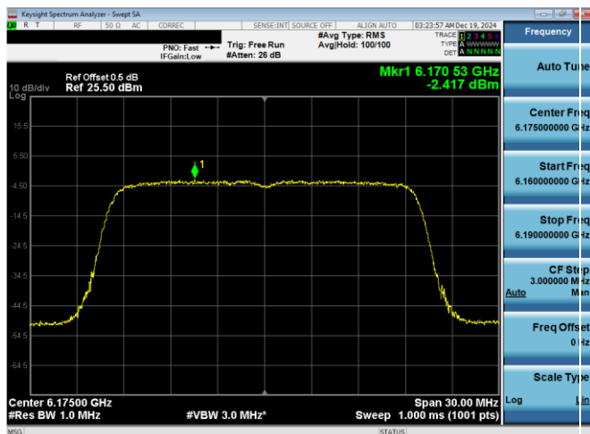
Plot 7-97. Power Spectral Density Plot Antenna WF7a (20MHz 802.11ax (UNII Band 5) – Ch. 45)
