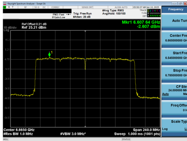
Plot 7-124. PSD Plot Antenna WF2a (160MHz 802.11ax (UNII Band 7) – Ch. 143)
