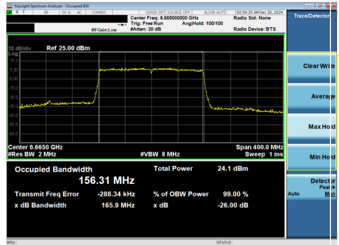
Plot 7-80. 26dB & 99% Bandwidth Plot Antenna WF7b (160MHz 802.11ax (UNII Band 7) – Ch. 143)
