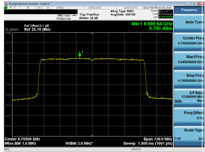
Plot 7-95. PSD Plot Antenna WF7a (80MHz 802.11ax (UNII Band 7) - Ch. 151)
