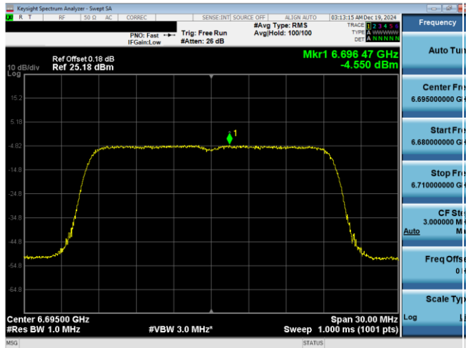
Plot 7-105. Power Spectral Density Plot Antenna WF7a (20MHz 802.11ax (UNII Band 7) – Ch. 149)
