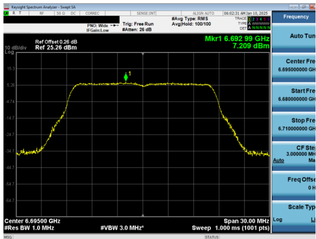
Plot 7-121. PSD Plot Antenna WF2a (20MHz 802.11a (UNII Band 7) – Ch. 149)
