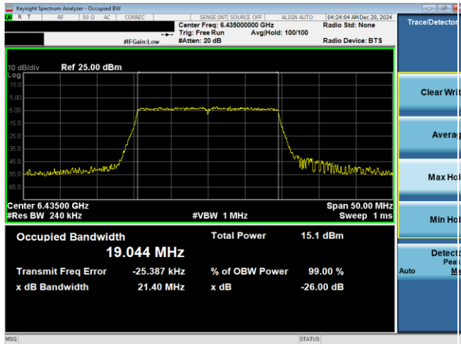
Plot 7-73. 26dB & 99% Bandwidth Plot Antenna WF7b (20MHz 802.11ax (UNII Band 6) – Ch. 97)
