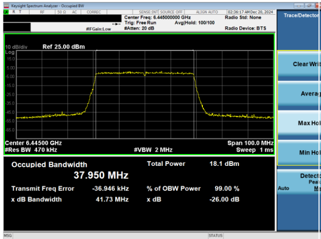
Plot 7-74. 26dB & 99% Bandwidth Plot Antenna WF7b (40MHz 802.11ax (UNII Band 6) – Ch. 99)
