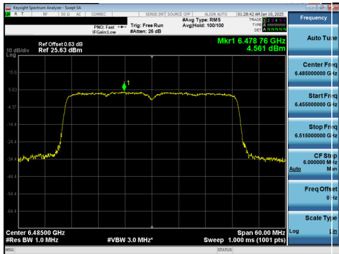
Plot 7-90. PSD Plot Antenna WF7a (40MHz 802.11ax (UNII Band 6) – Ch. 107)
