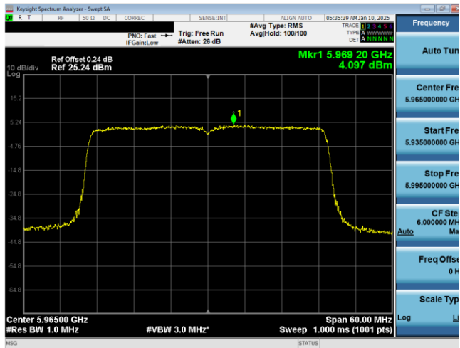
Plot 7-114. PSD Plot Antenna WF2a (40MHz 802.11ax (UNII Band 5) – Ch. 3)
