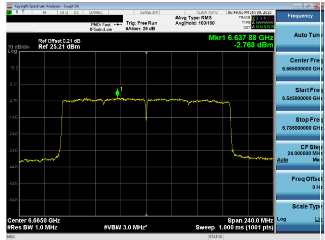
Plot 7-96. PSD Plot Antenna WF7a (160MHz 802.11ax (UNII Band 7) - Ch. 143)
