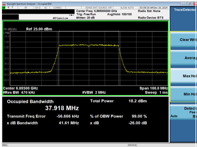
Plot 7-82. 26dB & 99% Bandwidth Plot Antenna WF7b (40MHz 802.11ax (UNII Band 8) – Ch. 187)
