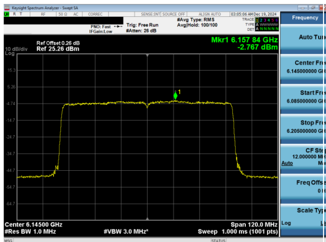
Plot 7-99. Power Spectral Density Plot Antenna WF7a (80MHz 802.11ax (UNII Band 5) – Ch. 39)
