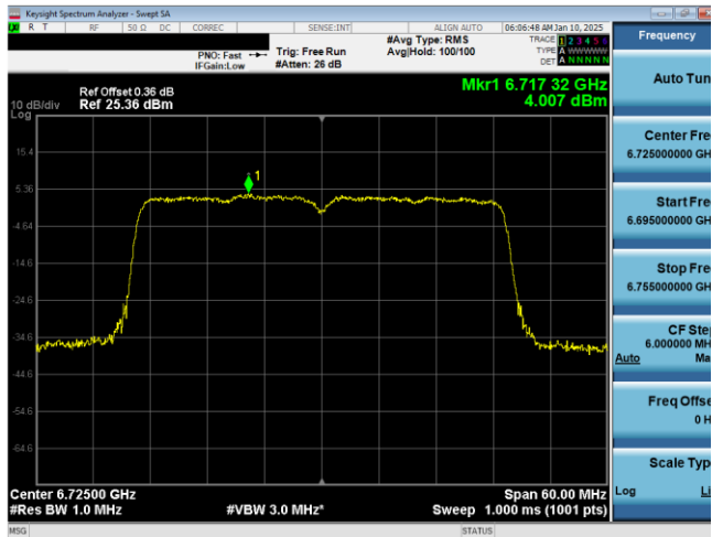
Plot 7-122. PSD Plot Antenna WF2a (40MHz 802.11ax (UNII Band 7) – Ch. 155)
