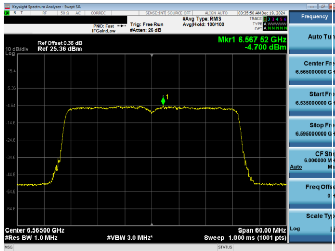
Plot 7-106. Power Spectral Density Plot Antenna WF7a (40MHz 802.11ax (UNII Band 7) – Ch. 123)
