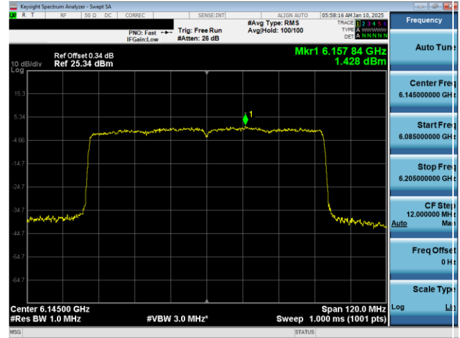
Plot 7-115. PSD Plot Antenna WF2a (80MHz 802.11ax (UNII Band 5) – Ch. 39)
