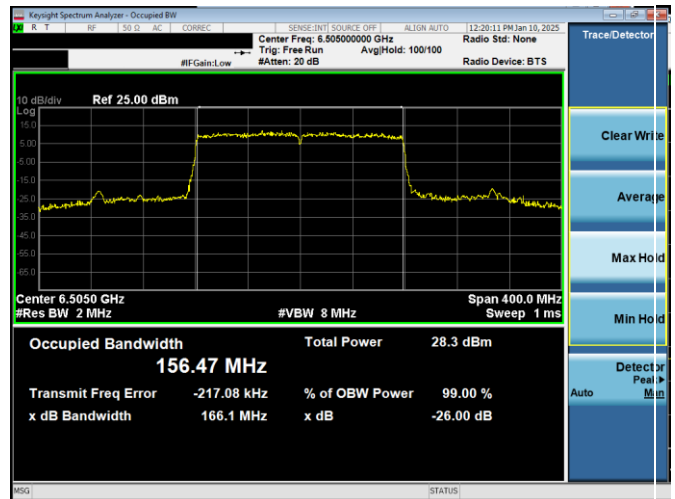
Plot 7-64. 26dB & 115% Bandwidth Plot Antenna WF7b (160MHz 802.11ax (UNII Band 7) – Ch. 111)
