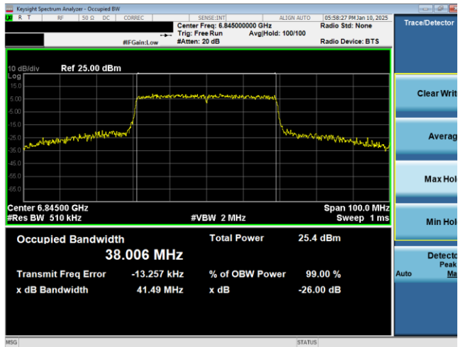
Plot 7-66. 26dB & 99% Bandwidth Plot Antenna WF7b (40MHz 802.11ax (UNII Band 7) – Ch. 179)
