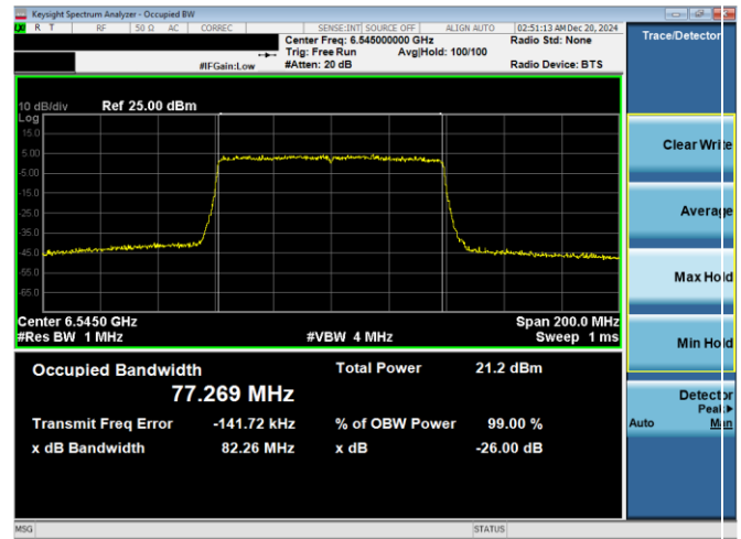
Plot 7-79. 26dB & 99% Bandwidth Plot Antenna WF7b (80MHz 802.11ax (UNII Band 7) – Ch. 119)
