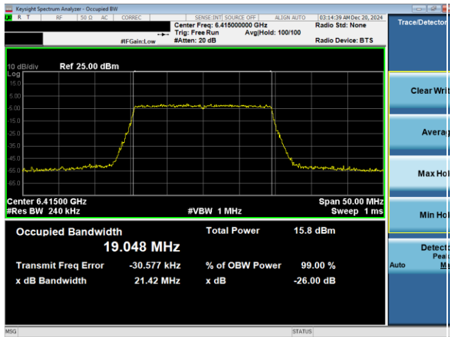
Plot 7-69. 26dB & 99% Bandwidth Plot Antenna WF7b (20MHz 802.11ax (UNII Band 5) – Ch. 93)
