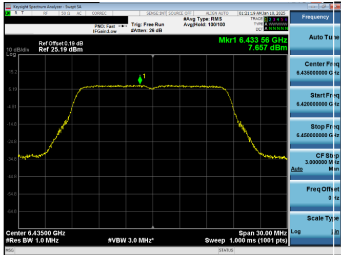
Plot 7-89. PSD Plot Antenna WF7a (20MHz 802.11a (UNII Band 6) – Ch. 97)
