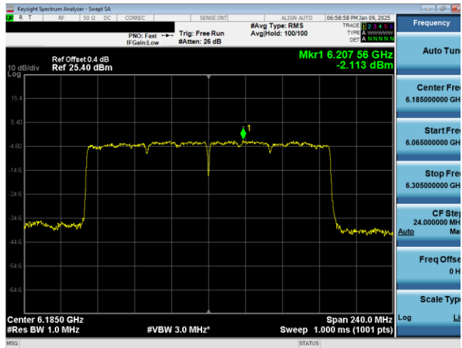
Plot 7-88. PSD Plot Antenna WF7a (160MHz 802.11ax (UNII Band 5) – Ch. 47)
