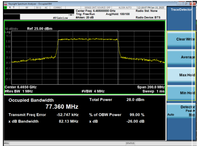
Plot 7-63. 26dB & 115% Bandwidth Plot Antenna WF7b (80MHz 802.11ax (UNII Band 6) – Ch. 103)
