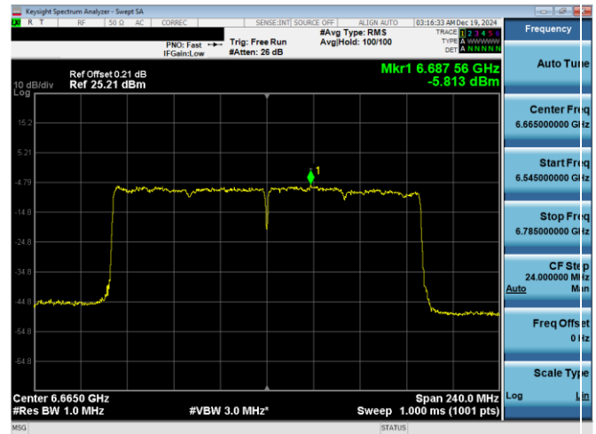
Plot 7-108. Power Spectral Density Plot Antenna WF7a (160MHz 802.11ax (UNII Band 7) – Ch. 143)
