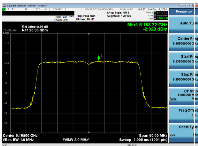
Plot 7-98. Power Spectral Density Plot Antenna WF7a (40MHz 802.11ax (UNII Band 5) – Ch. 43)
