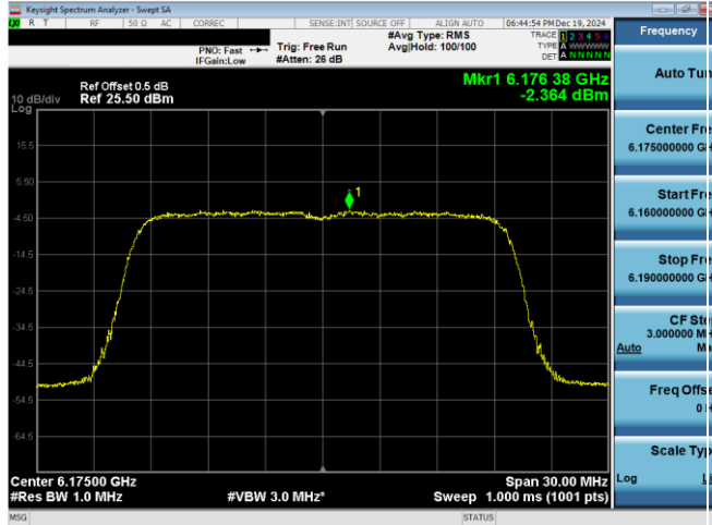
Plot 7-125. Power Spectral Density Plot Antenna WF2a (20MHz 802.11ax (UNII Band 5) – Ch. 45)
