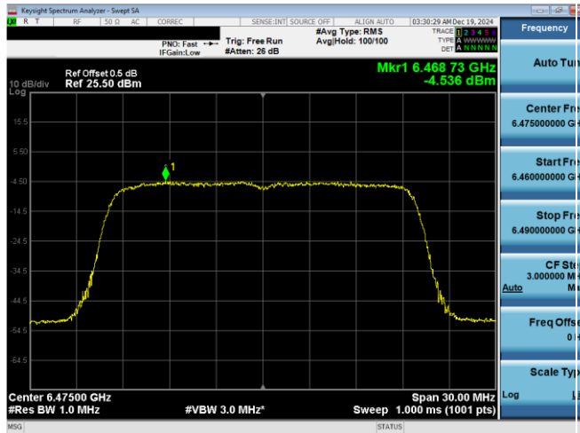
Plot 7-101. Power Spectral Density Plot Antenna WF7a (20MHz 802.11ax (UNII Band 6) – Ch. 105)
