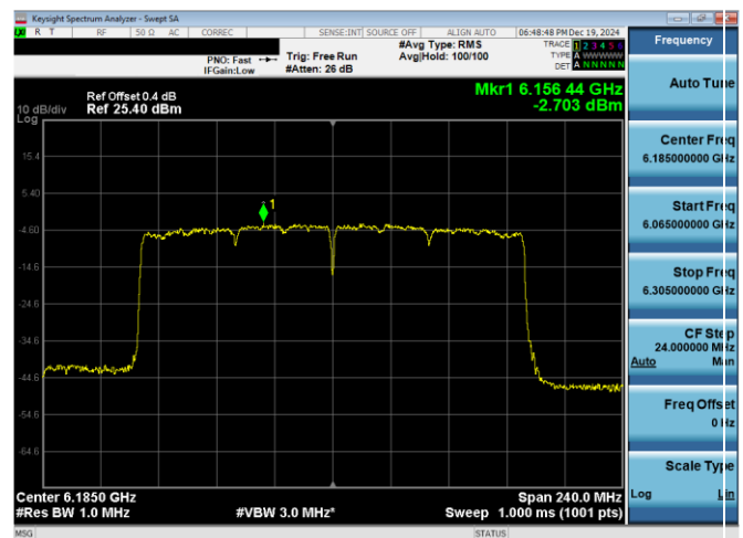
Plot 7-128. Power Spectral Density Plot Antenna WF2a (160MHz 802.11ax (UNII Band 5) – Ch. 47)
