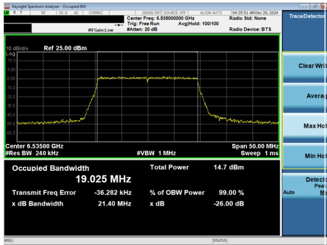
Plot 7-77. 26dB & 99% Bandwidth Plot Antenna WF7b (20MHz 802.11ax (UNII Band 7) – Ch. 117)
