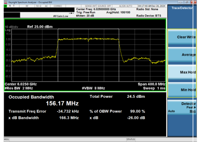
Plot 7-72. 26dB & 99% Bandwidth Plot Antenna WF7b (160MHz 802.11ax (UNII Band 5) – Ch. 15)
