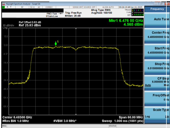
Plot 7-118. PSD Plot Antenna WF2a (40MHz 802.11ax (UNII Band 6) – Ch. 107)
