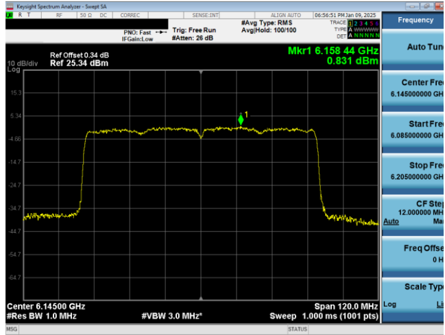
Plot 7-87. PSD Plot Antenna WF7a (80MHz 802.11ax (UNII Band 5) – Ch. 39)
