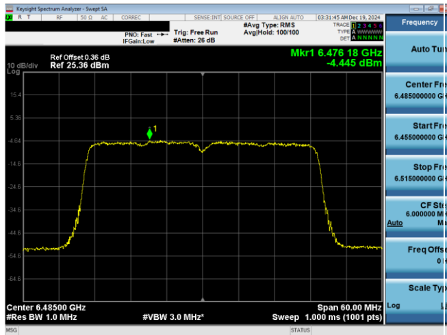
Plot 7-102. Power Spectral Density Plot Antenna WF7a (40MHz 802.11ax (UNII Band 6) – Ch. 107)
