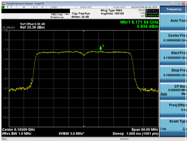
Plot 7-86. PSD Plot Antenna WF7a (40MHz 802.11ax (UNII Band 5) – Ch. 43)
