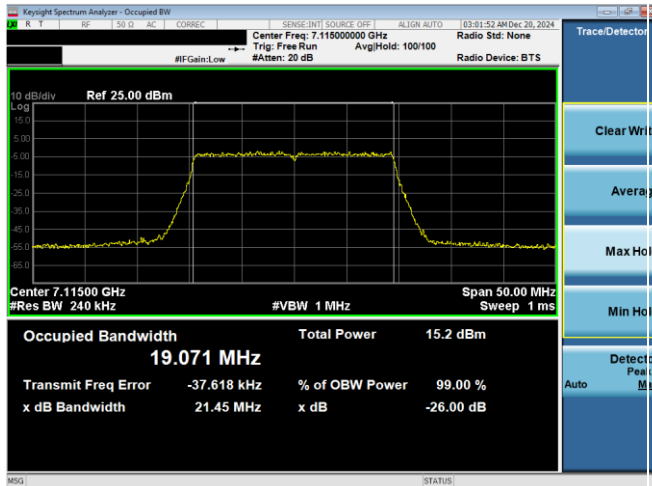
Plot 7-81. 26dB & 99% Bandwidth Plot Antenna WF7b (20MHz 802.11ax (UNII Band 8) – Ch. 233)
