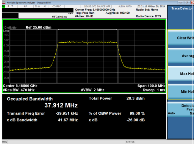
Plot 7-70. 26dB & 99% Bandwidth Plot Antenna WF7b (40MHz 802.11ax (UNII Band 5) – Ch. 43)
