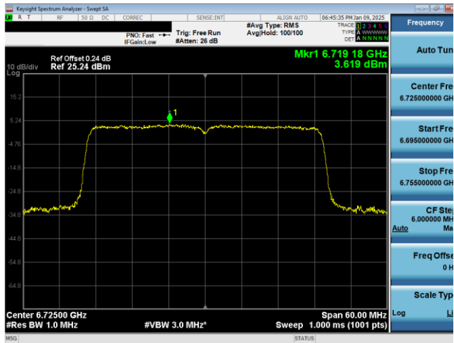
Plot 7-94. PSD Plot Antenna WF7a (40MHz 802.11ax (UNII Band 7) - Ch. 155)
