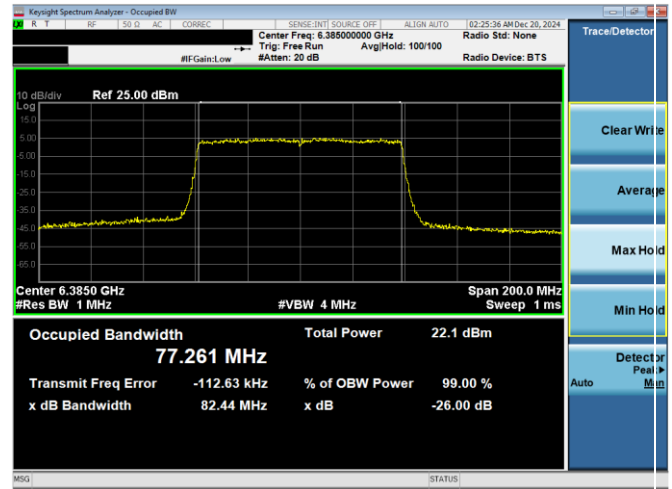
Plot 7-71. 26dB & 99% Bandwidth Plot Antenna WF7b (80MHz 802.11ax (UNII Band 5) – Ch. 87)
