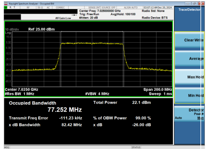
Plot 7-83. 26dB & 99% Bandwidth Plot Antenna WF7b (80MHz 802.11ax (UNII Band 8) – Ch. 215)
