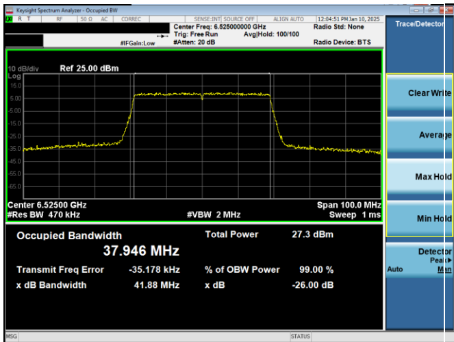
Plot 7-62. 26dB & 115% Bandwidth Plot Antenna WF7b (40MHz 802.11ax (UNII Band 6) – Ch. 115)
