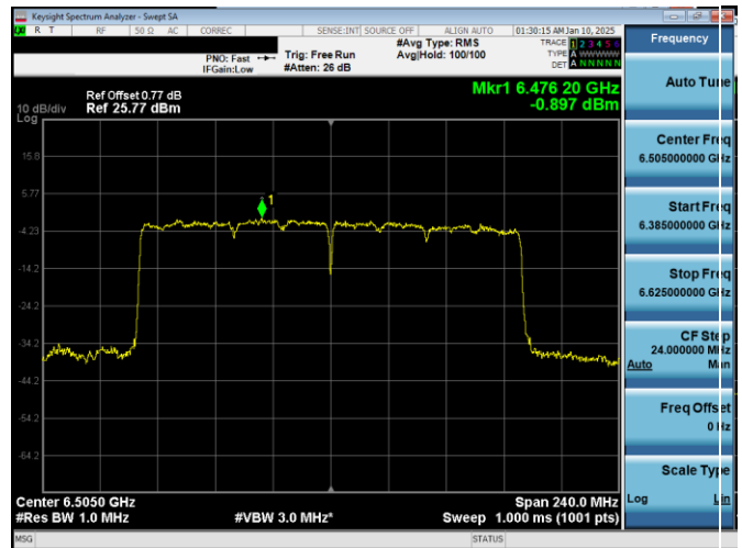
Plot 7-120. PSD Plot Antenna WF2a (160MHz 802.11ax (UNII Band 6) – Ch. 111)
