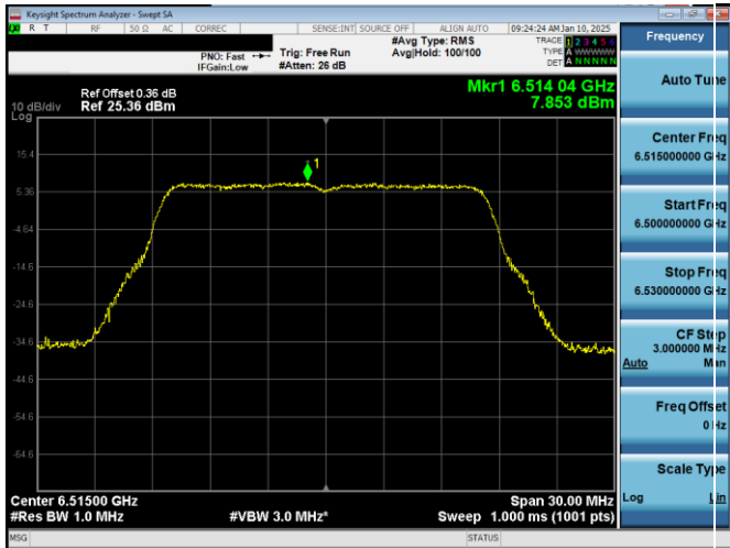
Plot 7-117. PSD Plot Antenna WF2a (20MHz 802.11a (UNII Band 6) – Ch. 113)
