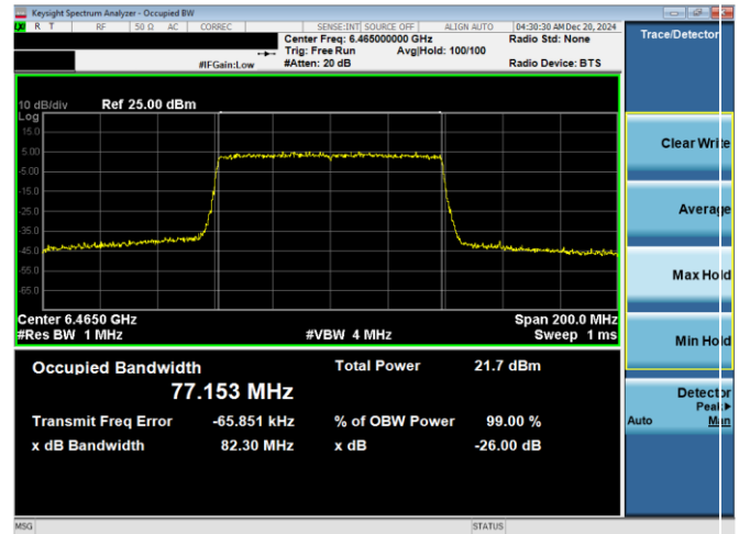
Plot 7-75. 26dB & 99% Bandwidth Plot Antenna WF7b (80MHz 802.11ax (UNII Band 6) – Ch. 103)
