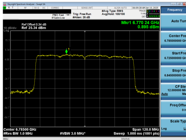
Plot 7-123. PSD Plot Antenna WF2a (80MHz 802.11ax (UNII Band 7) – Ch. 167)
