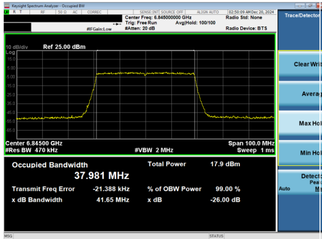
Plot 7-78. 26dB & 99% Bandwidth Plot Antenna WF7b (40MHz 802.11ax (UNII Band 7) – Ch. 179)
