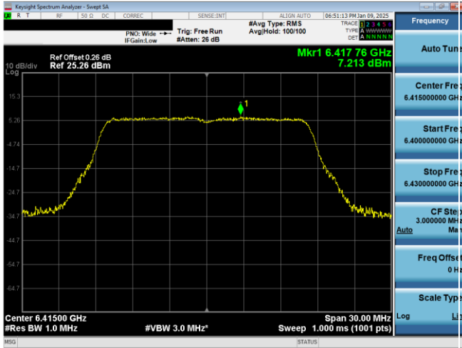
Plot 7-85. PSD Plot Antenna WF7a (20MHz 802.11a (UNII Band 5) – Ch. 93)
