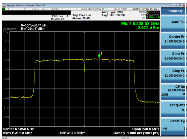
Plot 7-100. Power Spectral Density Plot Antenna WF7a (160MHz 802.11ax (UNII Band 5) – Ch. 47)
