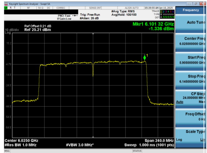
Plot 7-116. PSD Plot Antenna WF2a (160MHz 802.11ax (UNII Band 5) – Ch. 15)
