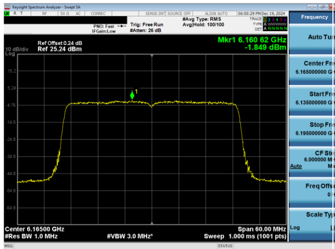
Plot 7-126. Power Spectral Density Plot Antenna WF2a (40MHz 802.11ax (UNII Band 5) – Ch. 43)
