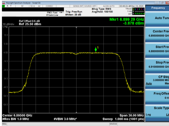
Plot 7-109. Power Spectral Density Plot Antenna WF7a (20MHz 802.11ax (UNII Band 8) – Ch. 189)
