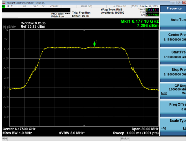
Plot 7-113. PSD Plot Antenna WF2a (20MHz 802.11a (UNII Band 5) – Ch. 45)
