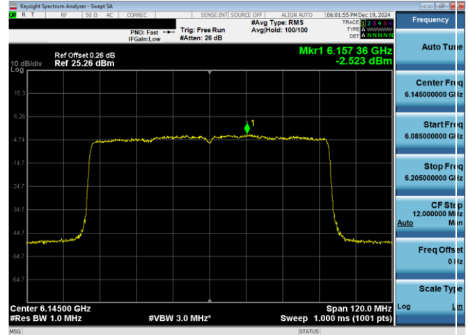
Plot 7-127. Power Spectral Density Plot Antenna WF2a (80MHz 802.11ax (UNII Band 5) – Ch. 39)
