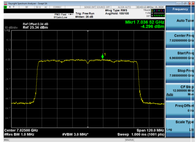
Plot 7-111. Power Spectral Density Plot Antenna WF7a (80MHz 802.11ax (UNII Band 8) – Ch. 215)
