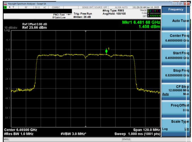
Plot 7-119. PSD Plot Antenna WF2a (80MHz 802.11ax (UNII Band 6) – Ch. 103)
