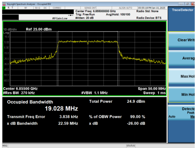
Plot 7-65. 26dB & 99% Bandwidth Plot Antenna WF7b (20MHz 802.11ax (UNII Band 7) – Ch. 181)
