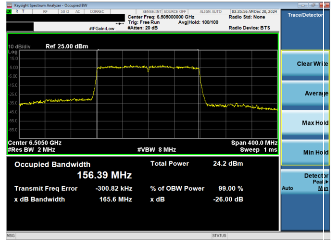
Plot 7-76. 26dB & 99% Bandwidth Plot Antenna WF7b (160MHz 802.11ax (UNII Band 6) – Ch. 111)
