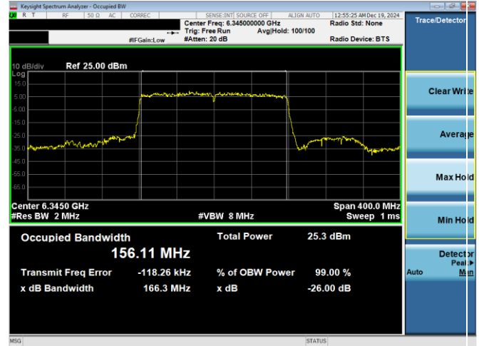
Plot 7-16. 26dB & 99% Bandwidth Plot Antenna WF7a (160MHz 802.11ax (UNII Band 5) – Ch. 79)
