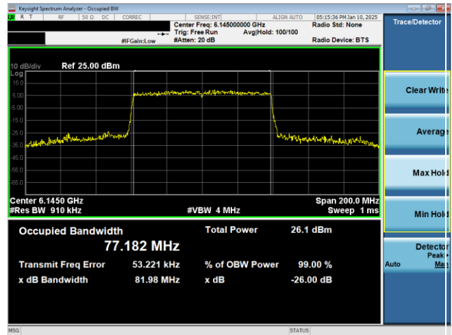
Plot 7-59. 26dB & 99% Bandwidth Plot Antenna WF7b (80MHz 802.11ax (UNII Band 5) – Ch. 39)
