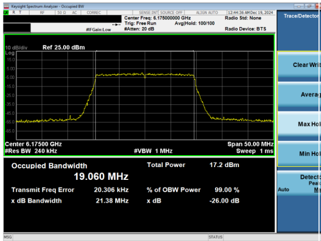
Plot 7-13. 26dB & 99% Bandwidth Plot Antenna WF7a (20MHz 802.11ax (UNII Band 5) – Ch. 45)
