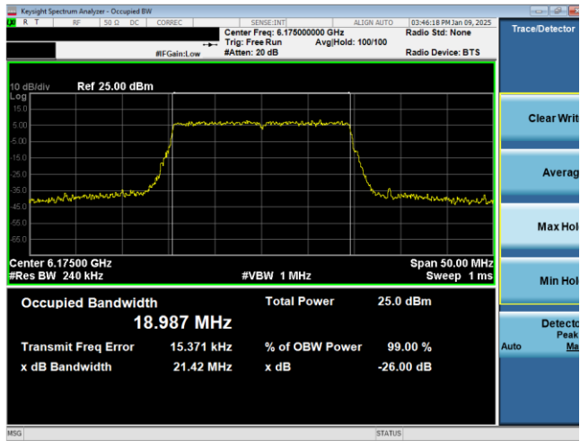
Plot 7-1. 26dB & 99% Bandwidth Plot Antenna WF7a (20MHz 802.11ax (UNII Band 5) – Ch. 45)
