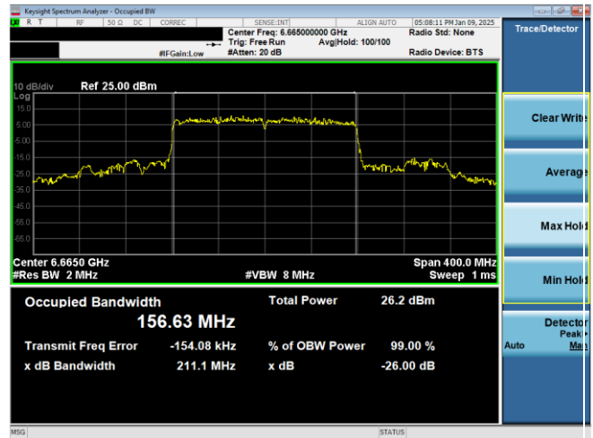
Plot 7-12. 26dB & 99% Bandwidth Plot Antenna WF7a (160MHz 802.11ax (UNII Band 7) – Ch. 143)
