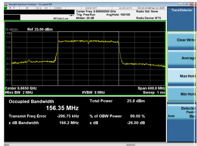
Plot 7-40. 26dB & 99% Bandwidth Plot Antenna WF2a (160MHz 802.11ax (UNII Band 7) – Ch. 143)
