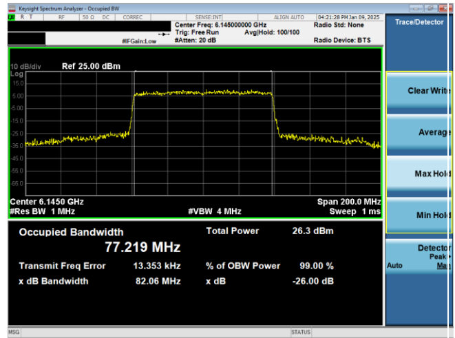
Plot 7-3. 26dB & 99% Bandwidth Plot Antenna WF7a (80MHz 802.11ax (UNII Band 5) – Ch. 39)
