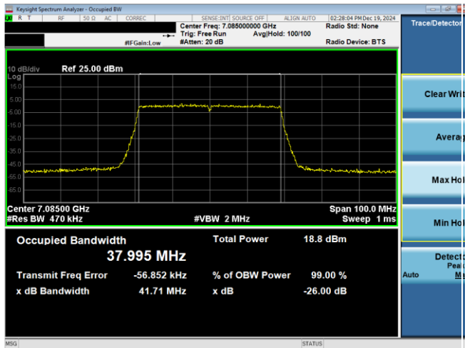
Plot 7-54. 26dB & 99% Bandwidth Plot Antenna WF2a (40MHz 802.11ax (UNII Band 8) – Ch. 227)
