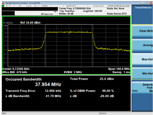
Plot 7-10. 26dB & 99% Bandwidth Plot Antenna WF7a (40MHz 802.11ax (UNII Band 7) – Ch. 155)
