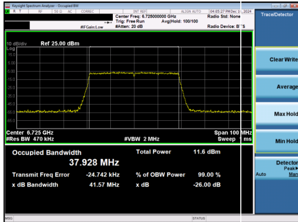
Plot 7-30. 26dB & 99% Bandwidth Plot Antenna 3a (40MHz 802.11ax RU484 (UNII Band 7) – Ch. 155)
