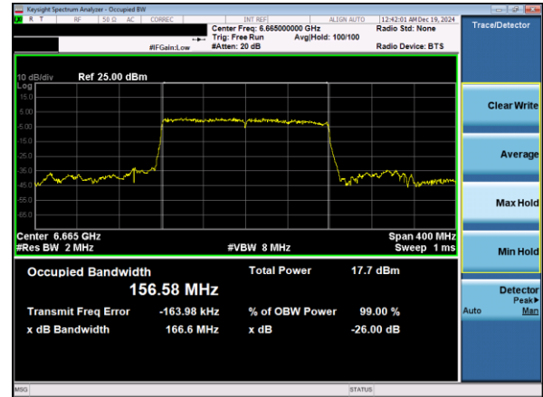
Plot 7-48. 26dB & 99% Bandwidth Plot Antenna 1b (160MHz 802.11ax RU996x2 (UNII Band 7) – Ch. 143)
