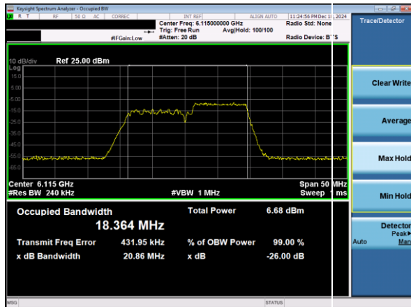
Plot 7-33. 26dB & 99% Bandwidth Plot Antenna 1b (20MHz 802.11ax RU106 (UNII Band 5) – Ch. 33)
