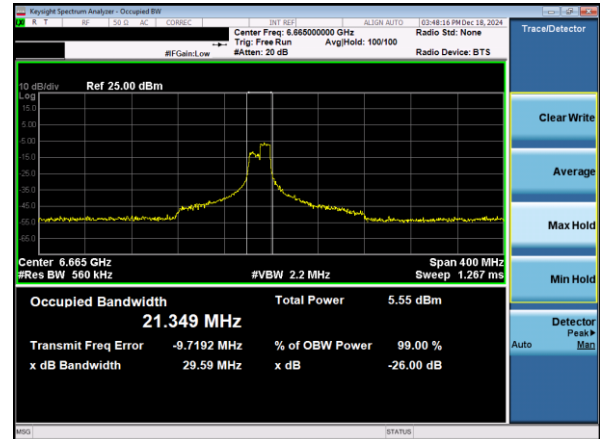
Plot 7-28. 26dB & 99% Bandwidth Plot Antenna 3a (160MHz 802.11ax RU106 (UNII Band 7) – Ch. 143)
