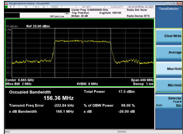
Plot 7-32. 26dB & 99% Bandwidth Plot Antenna 3a (160MHz 802.11ax RU996x2 (UNII Band 7) – Ch. 143)
