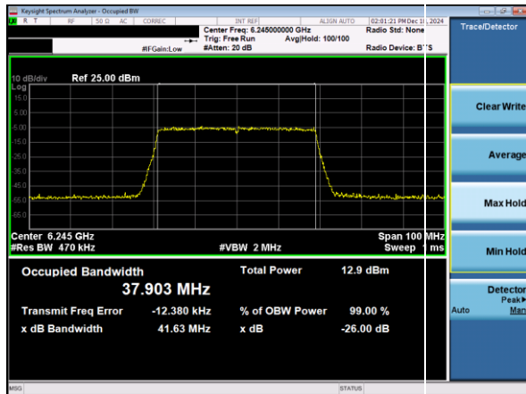
Plot 7-6. 26dB & 99% Bandwidth Plot Antenna 3c (40MHz 802.11ax RU484 (UNII Band 5) – Ch. 59)
