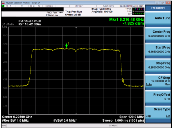
Plot 7-55. PSD Plot Antenna 3c (80MHz 802.11ax RU996 (UNII Band 5) – Ch. 55)
