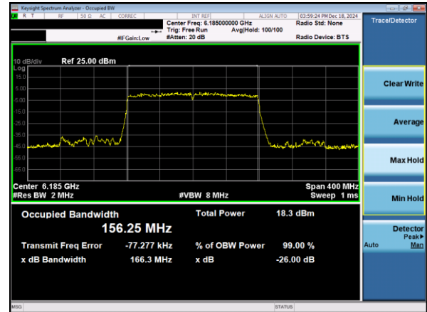
Plot 7-24. 26dB & 99% Bandwidth Plot Antenna 3a (160MHz 802.11ax RU996x2 (UNII Band 5) – Ch. 47)
