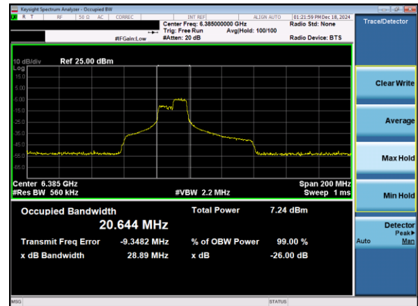
Plot 7-3. 26dB & 99% Bandwidth Plot Antenna 3c (80MHz 802.11ax RU106 (UNII Band 5) – Ch. 87)
