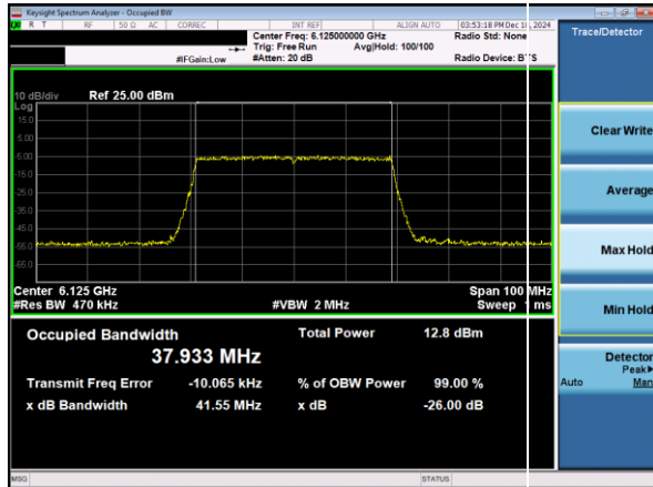
Plot 7-22. 26dB & 99% Bandwidth Plot Antenna 3a (40MHz 802.11ax RU484 (UNII Band 5) – Ch. 35)
