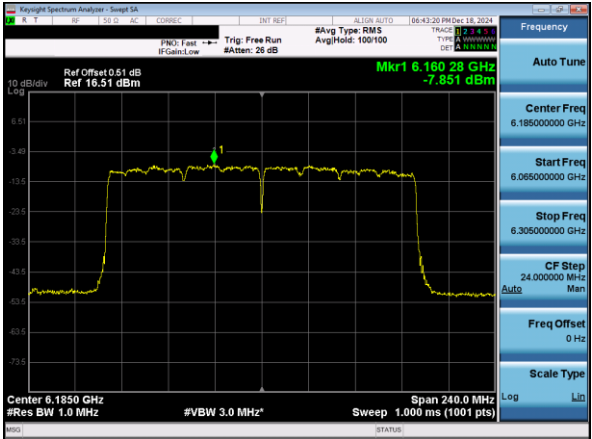
Plot 7-56. PSD Plot Antenna 3c (160MHz 802.11ax RU996x2 (UNII Band 5) – Ch. 47)
