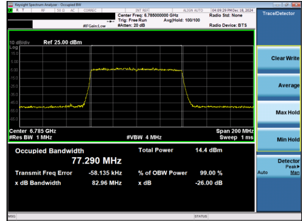
Plot 7-31. 26dB & 99% Bandwidth Plot Antenna 3a (80MHz 802.11ax RU996 (UNII Band 7) – Ch. 167)
