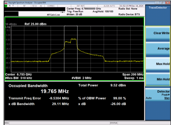
Plot 7-11. 26dB & 99% Bandwidth Plot Antenna 3c (80MHz 802.11ax RU106 (UNII Band 7) – Ch. 167)
