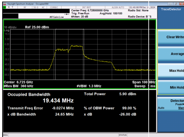
Plot 7-10. 26dB & 99% Bandwidth Plot Antenna 3c (40MHz 802.11ax RU106 (UNII Band 7) – Ch. 155)
