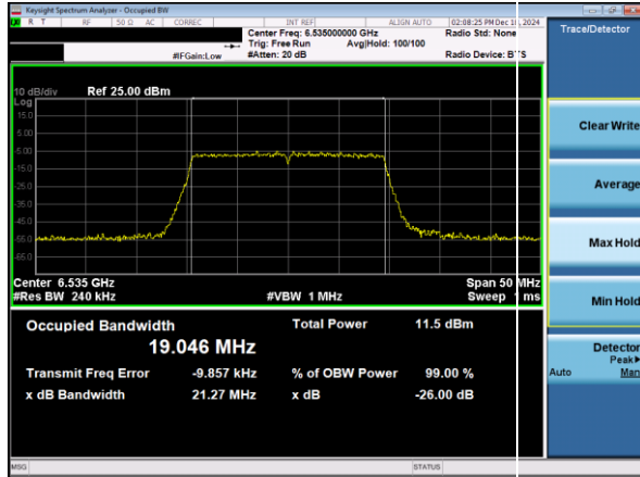
Plot 7-13. 26dB & 99% Bandwidth Plot Antenna 3c (20MHz 802.11ax RU242 (UNII Band 7) – Ch. 117)
