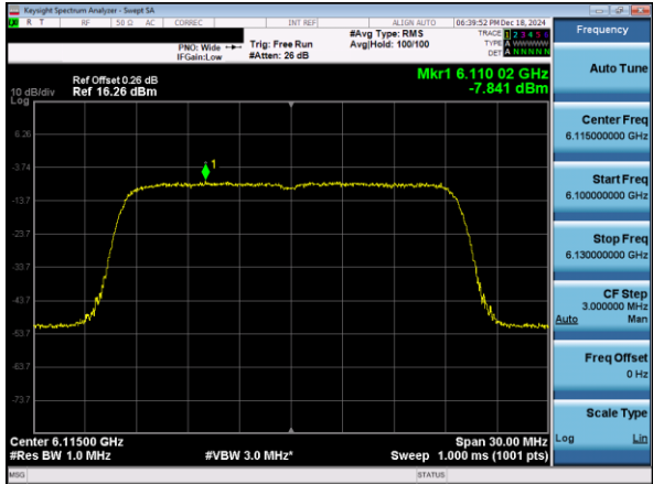
Plot 7-53. PSD Plot Antenna 3c (20MHz 802.11ax RU242 (UNII Band 5) – Ch. 33)
