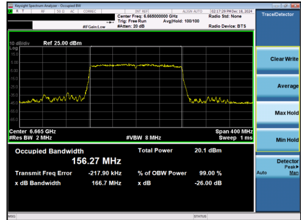
Plot 7-16. 26dB & 99% Bandwidth Plot Antenna 3c (160MHz 802.11ax RU996x2 (UNII Band 7) – Ch. 143)
