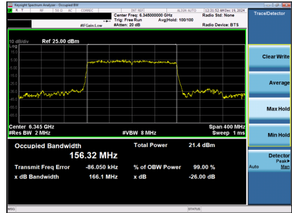
Plot 7-40. 26dB & 99% Bandwidth Plot Antenna 1b (160MHz 802.11ax RU996x2 (UNII Band 5) – Ch. 79)
