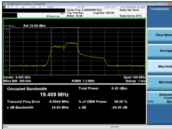
Plot 7-2. 26dB & 99% Bandwidth Plot Antenna 3c (40MHz 802.11ax RU106 (UNII Band 5) – Ch. 91)
