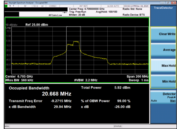
Plot 7-27. 26dB & 99% Bandwidth Plot Antenna 3a (80MHz 802.11ax RU106 (UNII Band 7) – Ch. 151)
