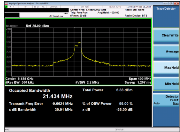
Plot 7-36. 26dB & 99% Bandwidth Plot Antenna 1b (160MHz 802.11ax RU106 (UNII Band 5) – Ch. 47)
