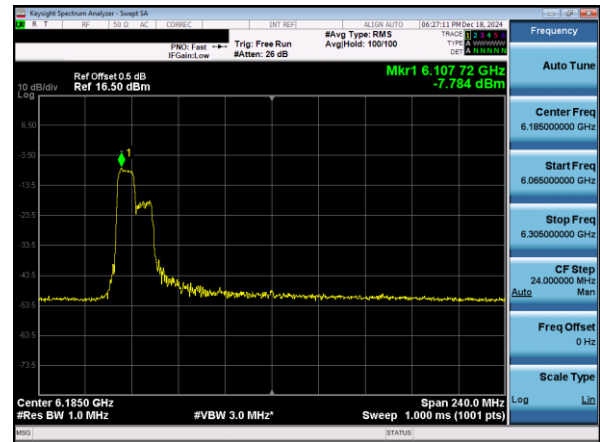
Plot 7-52. PSD Plot Antenna 3c (160MHz 802.11ax RU106 (UNII Band 5) – Ch. 47)
