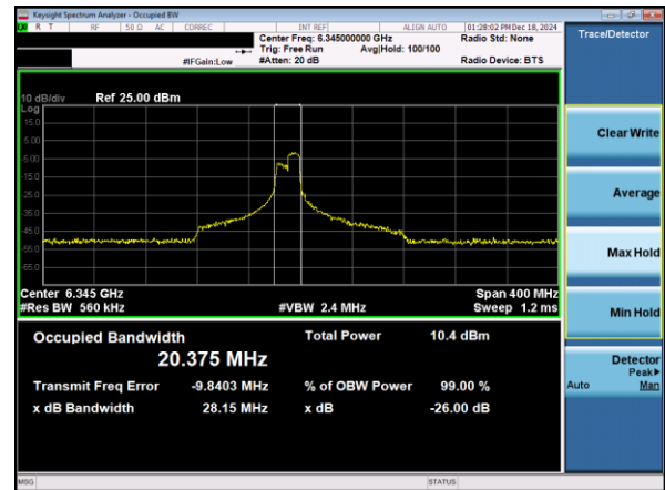
Plot 7-4. 26dB & 99% Bandwidth Plot Antenna 3c (160MHz 802.11ax RU106 (UNII Band 5) – Ch. 79)
