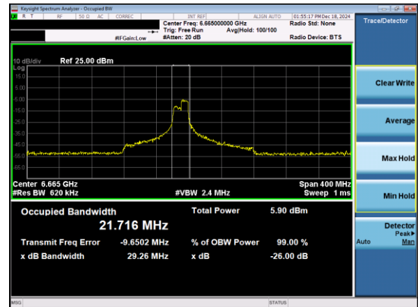
Plot 7-12. 26dB & 99% Bandwidth Plot Antenna 3c (160MHz 802.11ax RU106 (UNII Band 7) – Ch. 143)
