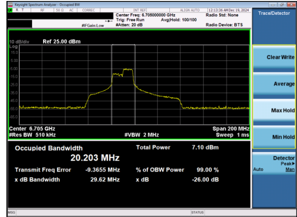
Plot 7-43. 26dB & 99% Bandwidth Plot Antenna 1b (80MHz 802.11ax RU106 (UNII Band 7) – Ch. 151)
