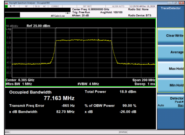
Plot 7-39. 26dB & 99% Bandwidth Plot Antenna 1b (80MHz 802.11ax RU996 (UNII Band 5) – Ch. 87)
