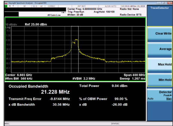
Plot 7-44. 26dB & 99% Bandwidth Plot Antenna 1b (160MHz 802.11ax RU106 (UNII Band 7) – Ch. 143)
