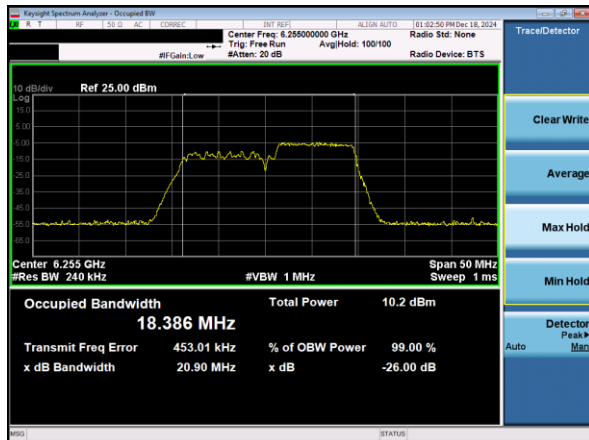
Plot 7-1. 26dB & 99% Bandwidth Plot Antenna 3c (20MHz 802.11ax RU106 (UNII Band 5) – Ch. 61)
