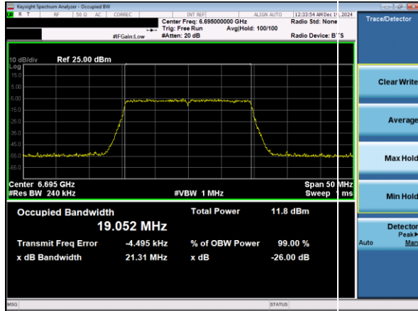
Plot 7-45. 26dB & 99% Bandwidth Plot Antenna 1b (20MHz 802.11ax RU242 (UNII Band 7) – Ch. 149)
