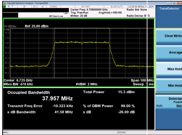
Plot 7-46. 26dB & 99% Bandwidth Plot Antenna 1b (40MHz 802.11ax RU484 (UNII Band 7) – Ch. 155)
