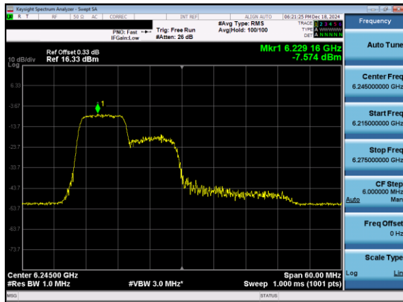
Plot 7-50. PSD Plot Antenna 3c (40MHz 802.11ax RU106 (UNII Band 5) – Ch. 59)
