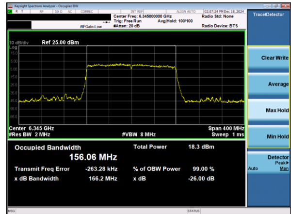
Plot 7-8. 26dB & 99% Bandwidth Plot Antenna 3c (160MHz 802.11ax RU996x2 (UNII Band 5) – Ch. 79)
