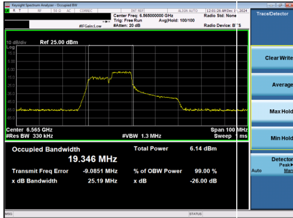
Plot 7-42. 26dB & 99% Bandwidth Plot Antenna 1b (40MHz 802.11ax RU106 (UNII Band 7) – Ch. 123)
