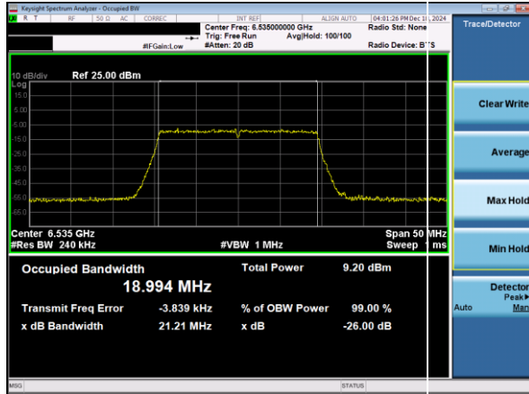
Plot 7-29. 26dB & 99% Bandwidth Plot Antenna 3a (20MHz 802.11ax RU242 (UNII Band 7) – Ch. 117)
