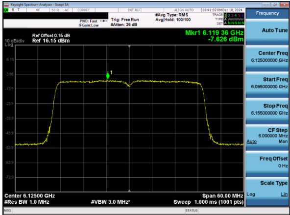
Plot 7-54. PSD Plot Antenna 3c (40MHz 802.11ax RU484 (UNII Band 5) – Ch. 35)
