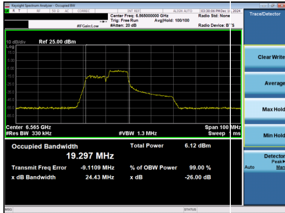
Plot 7-26. 26dB & 99% Bandwidth Plot Antenna 3a (40MHz 802.11ax RU106 (UNII Band 7) – Ch. 123)
