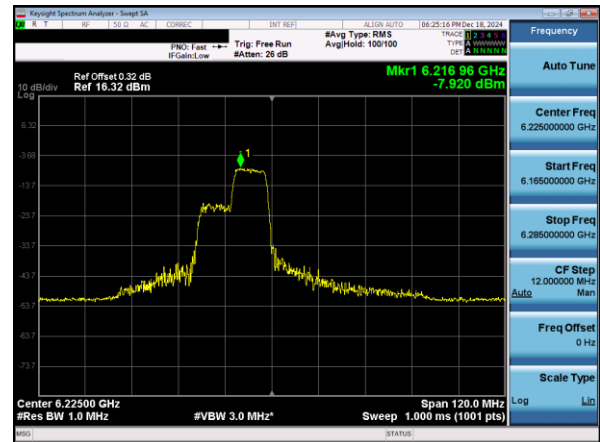
Plot 7-51. PSD Plot Antenna 3c (80MHz 802.11ax RU106 (UNII Band 5) – Ch. 55)
