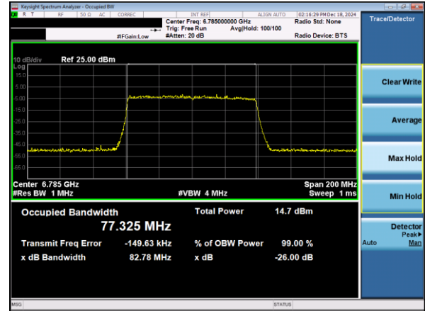
Plot 7-15. 26dB & 99% Bandwidth Plot Antenna 3c (80MHz 802.11ax RU996 (UNII Band 7) – Ch. 167)
