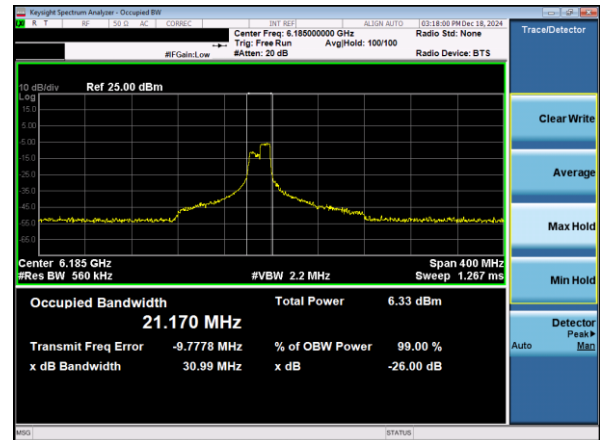
Plot 7-20. 26dB & 99% Bandwidth Plot Antenna 3a (160MHz 802.11ax RU106 (UNII Band 5) – Ch. 47)
