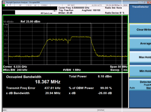
Plot 7-9. 26dB & 99% Bandwidth Plot Antenna 3c (20MHz 802.11ax RU106 (UNII Band 7) – Ch. 117)
