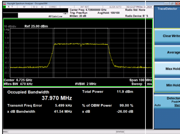
Plot 7-14. 26dB & 99% Bandwidth Plot Antenna 3c (40MHz 802.11ax RU484 (UNII Band 7) – Ch. 155)
