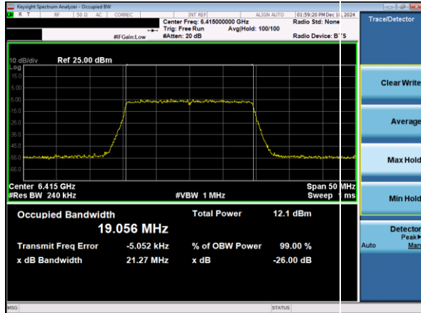
Plot 7-5. 26dB & 99% Bandwidth Plot Antenna 3c (20MHz 802.11ax RU242 (UNII Band 5) – Ch. 93)
