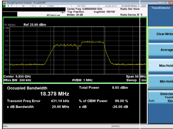
Plot 7-25. 26dB & 99% Bandwidth Plot Antenna 3a (20MHz 802.11ax RU106 (UNII Band 7) – Ch. 181)
