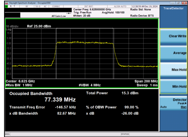
Plot 7-47. 26dB & 99% Bandwidth Plot Antenna 1b (80MHz 802.11ax RU996 (UNII Band 7) – Ch. 135)
