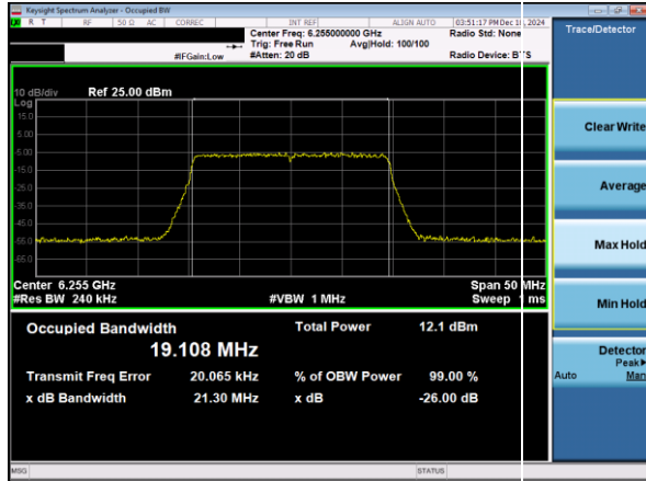
Plot 7-21. 26dB & 99% Bandwidth Plot Antenna 3a (20MHz 802.11ax RU242 (UNII Band 5) – Ch. 61)
