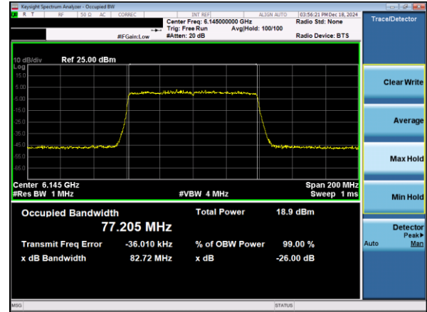
Plot 7-23. 26dB & 99% Bandwidth Plot Antenna 3a (80MHz 802.11ax RU996 (UNII Band 5) – Ch. 39)
