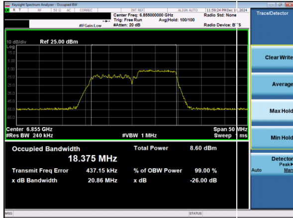
Plot 7-41. 26dB & 99% Bandwidth Plot Antenna 1b (20MHz 802.11ax RU106 (UNII Band 7) – Ch. 181)
