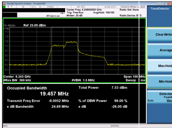
Plot 7-18. 26dB & 99% Bandwidth Plot Antenna 3a (40MHz 802.11ax RU106 (UNII Band 5) – Ch. 59)
