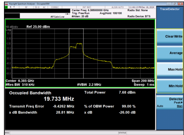
Plot 7-35. 26dB & 99% Bandwidth Plot Antenna 1b (80MHz 802.11ax RU106 (UNII Band 5) – Ch. 87)
