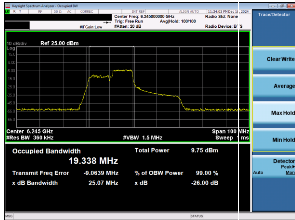
Plot 7-34. 26dB & 99% Bandwidth Plot Antenna 1b (40MHz 802.11ax RU106 (UNII Band 5) – Ch. 59)
