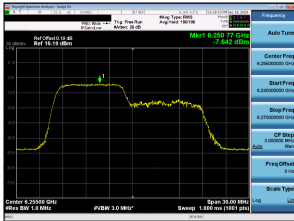
Plot 7-49. PSD Plot Antenna 3c (20MHz 802.11ax RU106 (UNII Band 5) – Ch. 61)
