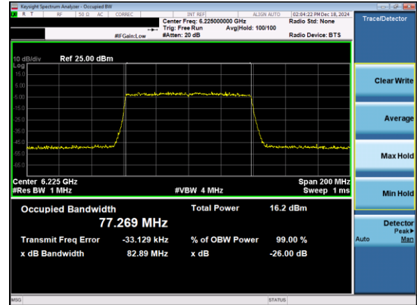
Plot 7-7. 26dB & 99% Bandwidth Plot Antenna 3c (80MHz 802.11ax RU996 (UNII Band 5) – Ch. 55)
