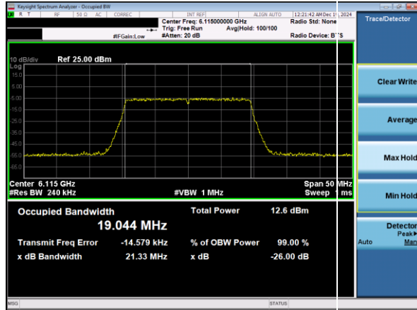
Plot 7-37. 26dB & 99% Bandwidth Plot Antenna 1b (20MHz 802.11ax RU242 (UNII Band 5) – Ch. 33)
