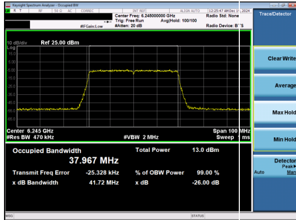
Plot 7-38. 26dB & 99% Bandwidth Plot Antenna 1b (40MHz 802.11ax RU484 (UNII Band 5) – Ch. 59)
