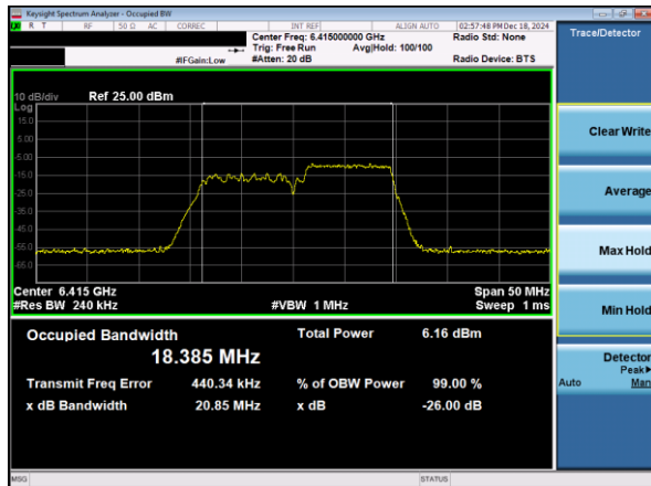
Plot 7-17. 26dB & 99% Bandwidth Plot Antenna 3a (20MHz 802.11ax RU106 (UNII Band 5) – Ch. 93)
