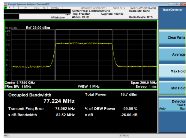
Plot 7-15. 26dB & 99% Bandwidth Plot Antenna 3a (80MHz 802.11ax (UNII Band 7) – Ch. 167)
