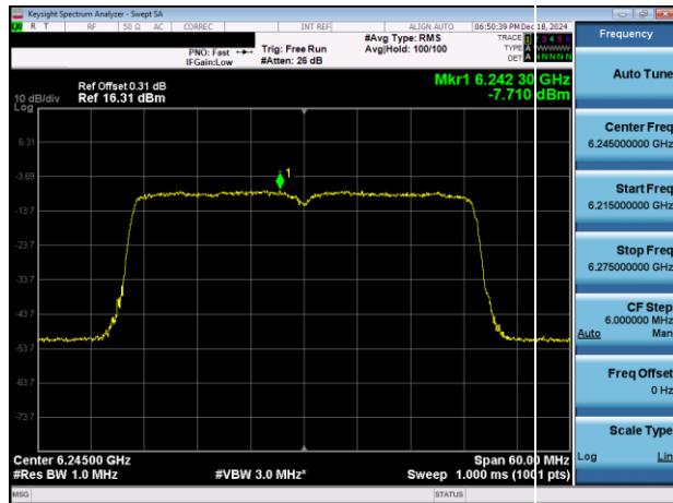
Plot 7-26. PSD Plot Antenna 3c (40MHz 802.11ax (UNII Band 5) – Ch. 59)
