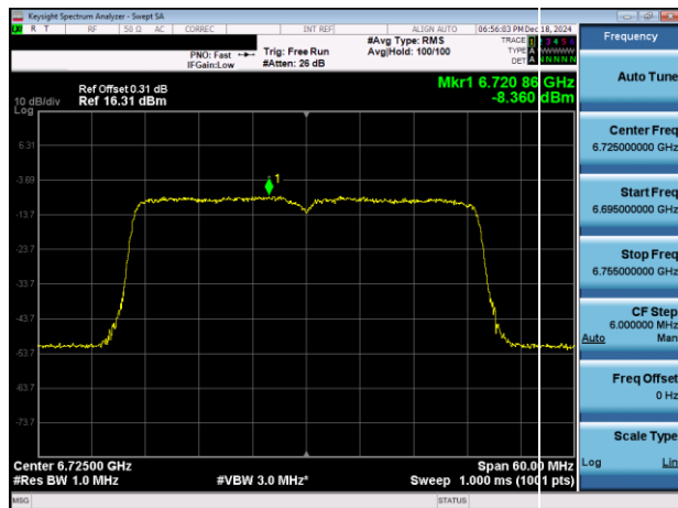
Plot 7-30. PSD Plot Antenna 3c (40MHz 802.11ax (UNII Band 7) – Ch. 155)
