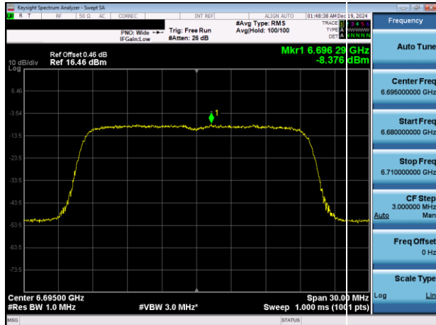
Plot 7-45. PSD Plot Antenna 1b (20MHz 802.11ax (UNII Band 7) – Ch. 149)
