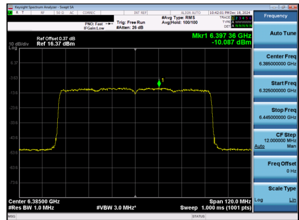
Plot 7-54. Power Spectral Density Plot SDM Primary Antenna 3a (80MHz 802.11ax (UNII Band 5) – Ch. 87)
