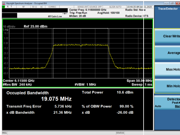
Plot 7-1. 26dB & 99% Bandwidth Plot Antenna 3c (20MHz 802.11ax (UNII Band 5) – Ch. 33)
