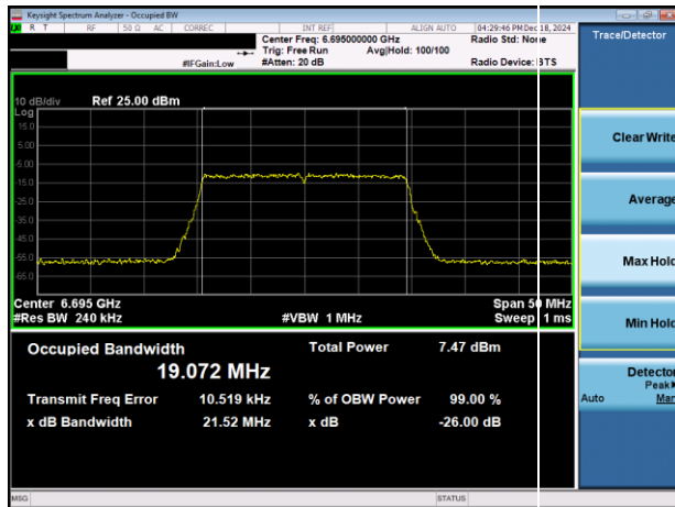
Plot 7-13. 26dB & 99% Bandwidth Plot Antenna 3a (20MHz 802.11ax (UNII Band 7) – Ch. 149)
