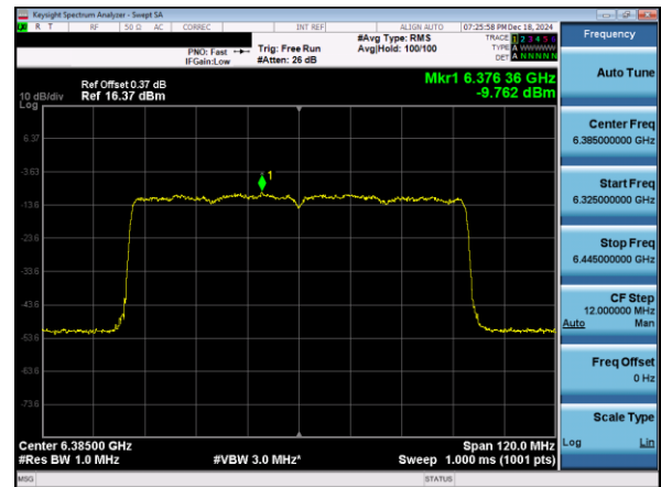
Plot 7-53. Power Spectral Density Plot SDM Primary Antenna 3c (80MHz 802.11ax (UNII Band 5) – Ch. 87)
