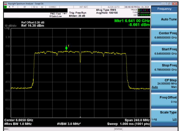
Plot 7-40. PSD Plot Antenna 3a (160MHz 802.11ax (UNII Band 7) – Ch. 143)
