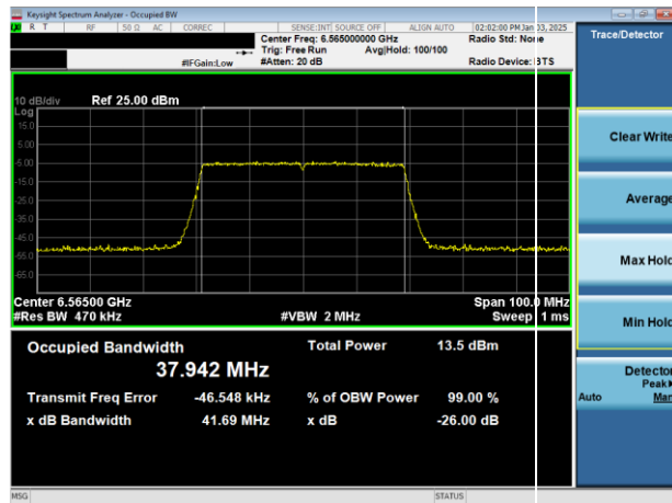
Plot 7-14. 26dB & 99% Bandwidth Plot Antenna 3a (40MHz 802.11ax (UNII Band 7) – Ch. 123)
