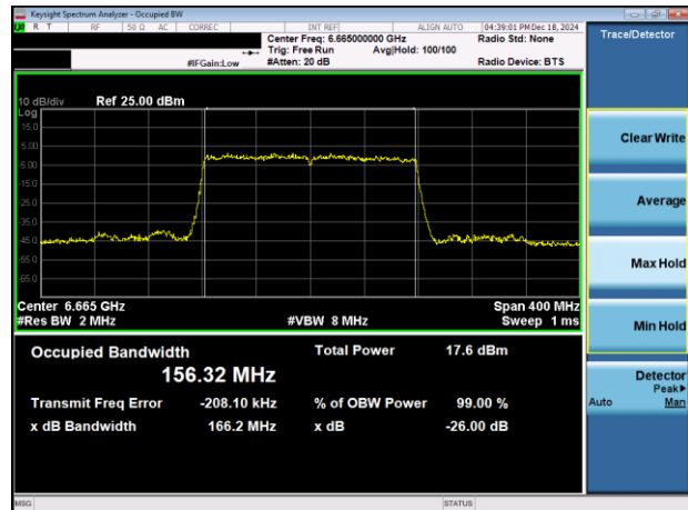
Plot 7-16. 26dB & 99% Bandwidth Plot Antenna 3a (160MHz 802.11ax (UNII Band 7) – Ch. 143)
