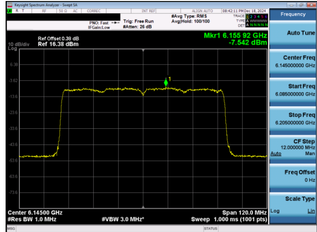
Plot 7-35. PSD Plot Antenna 3a (80MHz 802.11ax (UNII Band 5) – Ch. 39)
