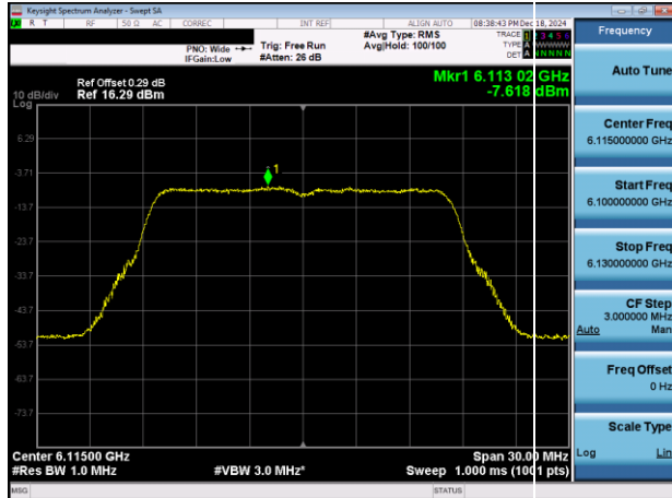
Plot 7-33. PSD Plot Antenna 3a (20MHz 802.11a (UNII Band 5) – Ch. 33)
