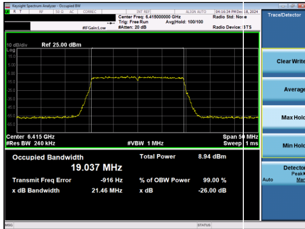
Plot 7-9. 26dB & 99% Bandwidth Plot Antenna 3a (20MHz 802.11ax (UNII Band 5) – Ch. 93)
