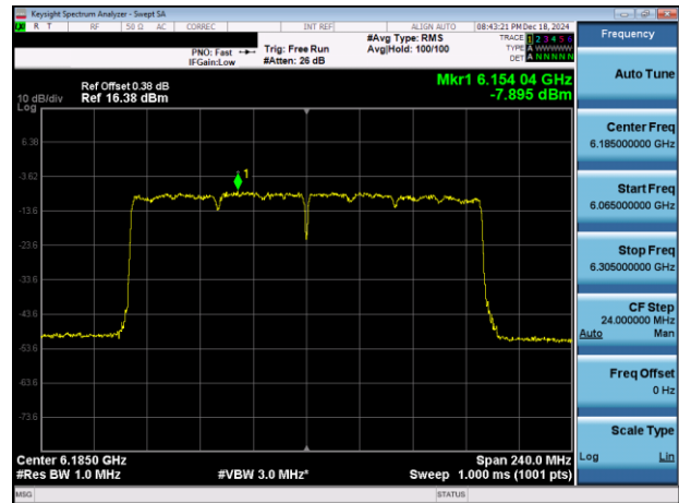
Plot 7-36. PSD Plot Antenna 3a (160MHz 802.11ax (UNII Band 5) – Ch. 47)
