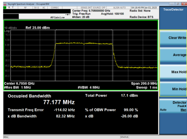
Plot 7-23. 26dB & 99% Bandwidth Plot Antenna 1b (80MHz 802.11ax (UNII Band 7) – Ch. 151)
