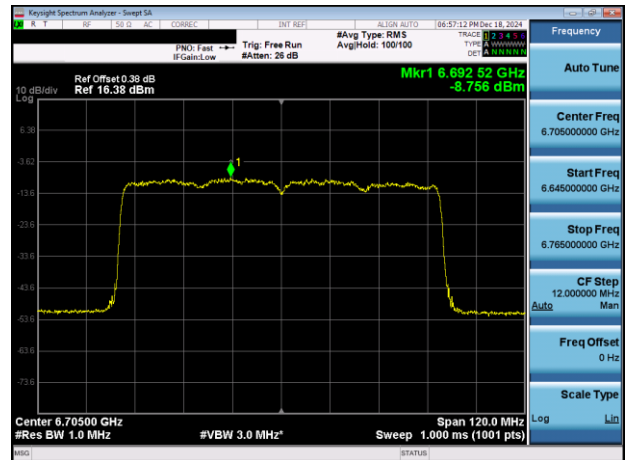
Plot 7-31. PSD Plot Antenna 3c (80MHz 802.11ax (UNII Band 7) – Ch. 151)
