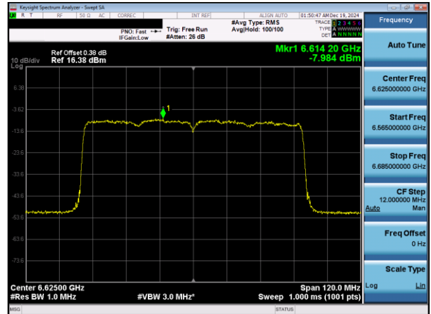
Plot 7-47. PSD Plot Antenna 1b (80MHz 802.11ax (UNII Band 7) – Ch. 135)
