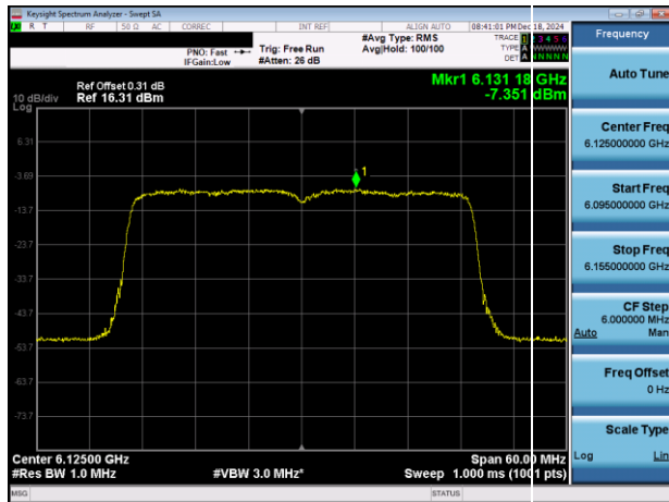
Plot 7-34. PSD Plot Antenna 3a (40MHz 802.11ax (UNII Band 5) – Ch. 35)
