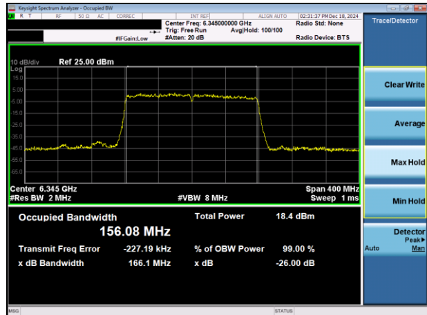
Plot 7-4. 26dB & 99% Bandwidth Plot Antenna 3c (160MHz 802.11ax (UNII Band 5) – Ch. 79)
