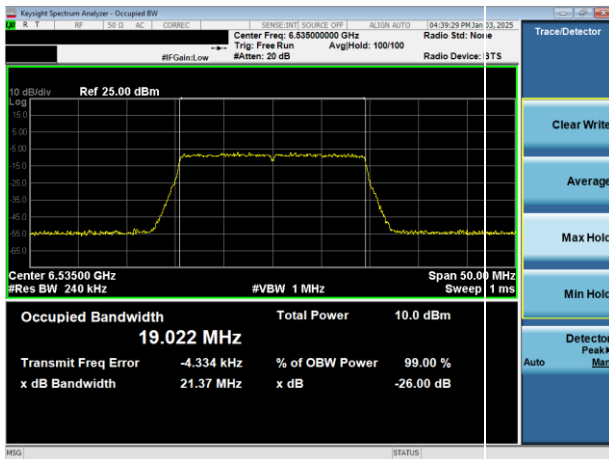
Plot 7-21. 26dB & 99% Bandwidth Plot Antenna 1b (20MHz 802.11ax (UNII Band 7) – Ch. 117)
