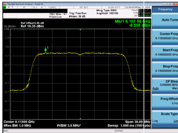
Plot 7-50. Power Spectral Density Plot SDM Primary Antenna 3a (20MHz 802.11ax (UNII Band 5) – Ch.33)
