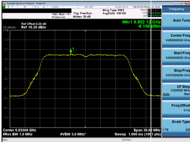
Plot 7-37. PSD Plot Antenna 3a (20MHz 802.11a (UNII Band 7) – Ch. 181)
