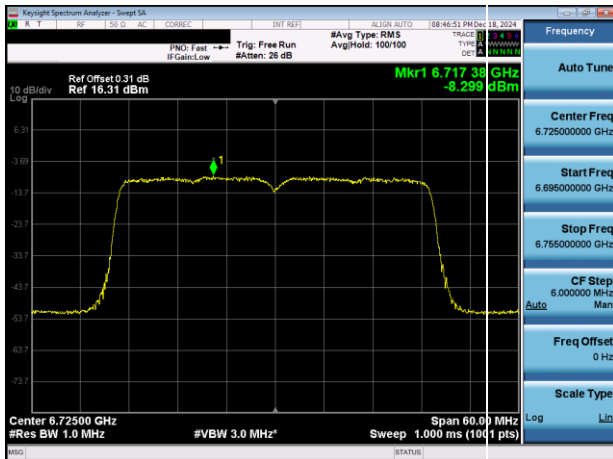
Plot 7-38. PSD Plot Antenna 3a (40MHz 802.11ax (UNII Band 7) – Ch. 155)
