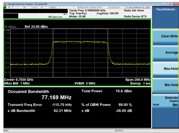
Plot 7-7. 26dB & 99% Bandwidth Plot Antenna 3c (80MHz 802.11ax (UNII Band 7) – Ch. 167)
