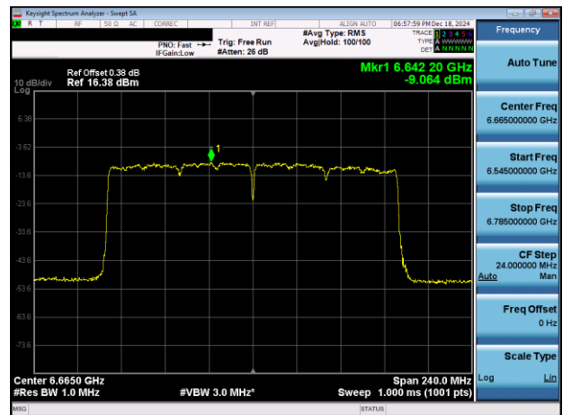
Plot 7-32. PSD Plot Antenna 3c (160MHz 802.11ax (UNII Band 7) – Ch. 143)
