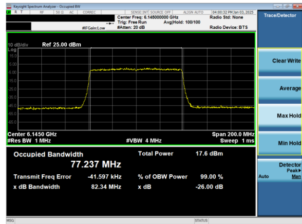
Plot 7-19. 26dB & 99% Bandwidth Plot Antenna 1b (80MHz 802.11ax (UNII Band 5) – Ch. 39)
