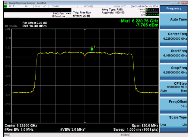
Plot 7-27. PSD Plot Antenna 3c (80MHz 802.11ax (UNII Band 5) – Ch. 55)
