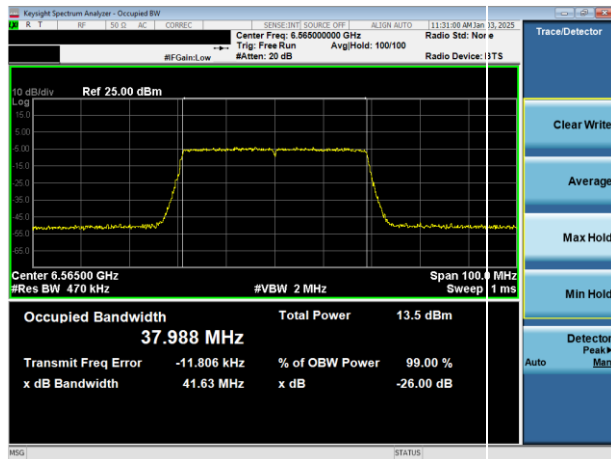
Plot 7-6. 26dB & 99% Bandwidth Plot Antenna 3c (40MHz 802.11ax (UNII Band 7) – Ch. 123)
