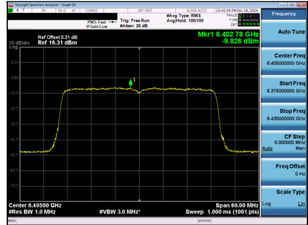
Plot 7-52. Power Spectral Density Plot SDM Primary Antenna 3a (40MHz 802.11ax (UNII Band 5) – Ch. 91)
