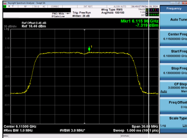
Plot 7-25. PSD Plot Antenna 3c (20MHz 802.11ax (UNII Band 5) – Ch. 33)
