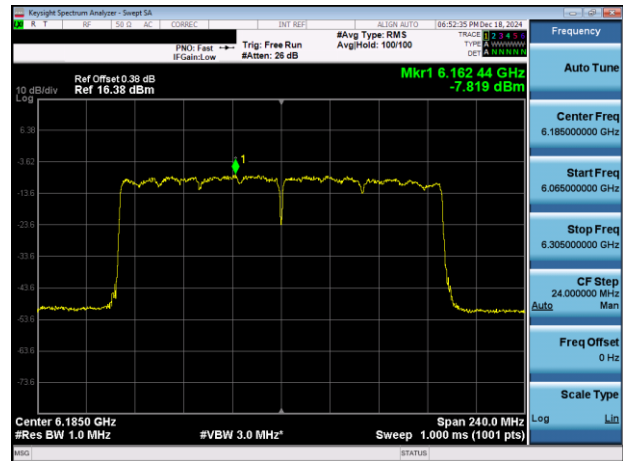
Plot 7-28. PSD Plot Antenna 3c (160MHz 802.11ax (UNII Band 5) – Ch. 47)
