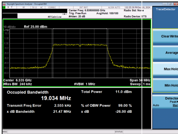
Plot 7-5. 26dB & 99% Bandwidth Plot Antenna 3c (20MHz 802.11ax (UNII Band 7) – Ch. 117)
