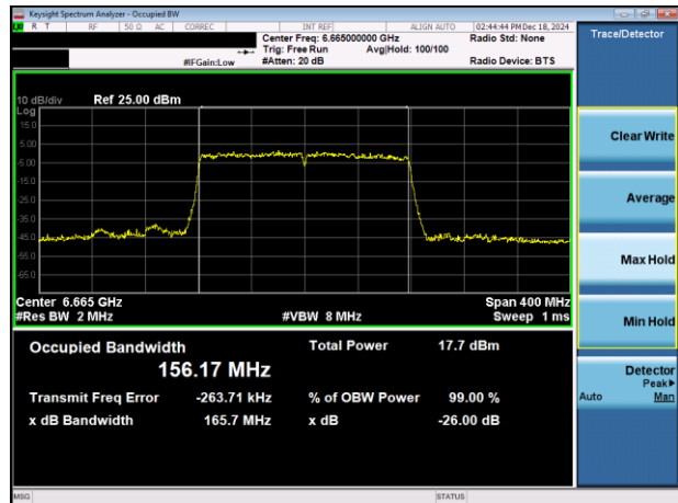
Plot 7-8. 26dB & 99% Bandwidth Plot Antenna 3c (160MHz 802.11ax (UNII Band 7) – Ch. 143)
