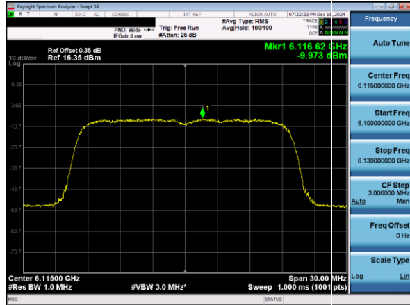
Plot 7-49. Power Spectral Density Plot SDM Primary Antenna 3c (20MHz 802.11ax (UNII Band 5) – Ch.33)
