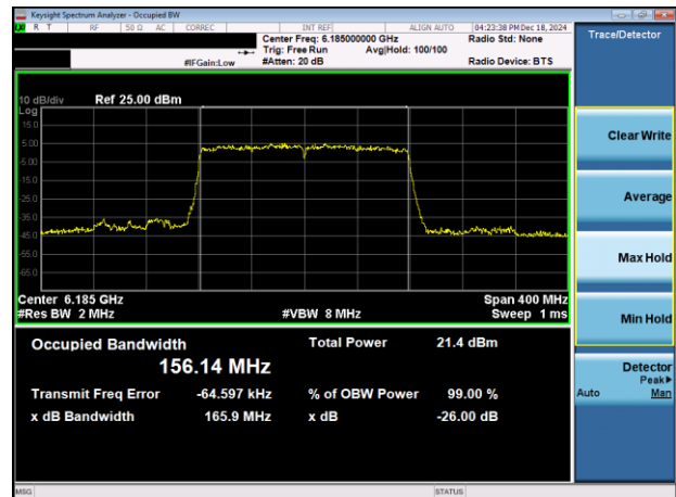
Plot 7-12. 26dB & 99% Bandwidth Plot Antenna 3a (160MHz 802.11ax (UNII Band 5) – Ch. 47)
