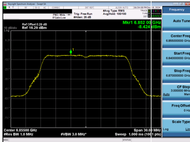
Plot 7-29. PSD Plot Antenna 3c (20MHz 802.11a (UNII Band 7) – Ch. 181)– Ch. 181)
