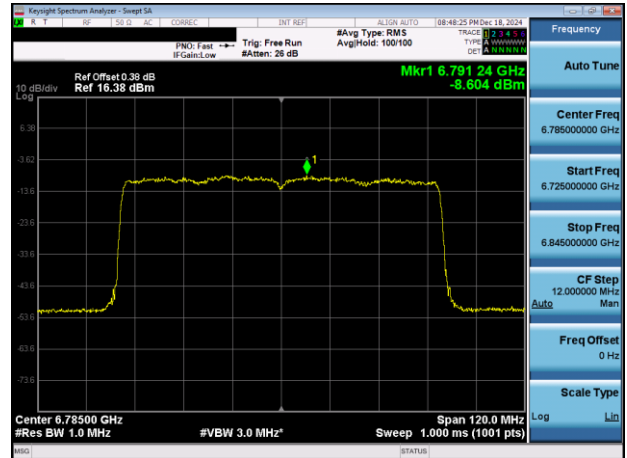
Plot 7-39. PSD Plot Antenna 3a (80MHz 802.11ax (UNII Band 7) – Ch. 167)
