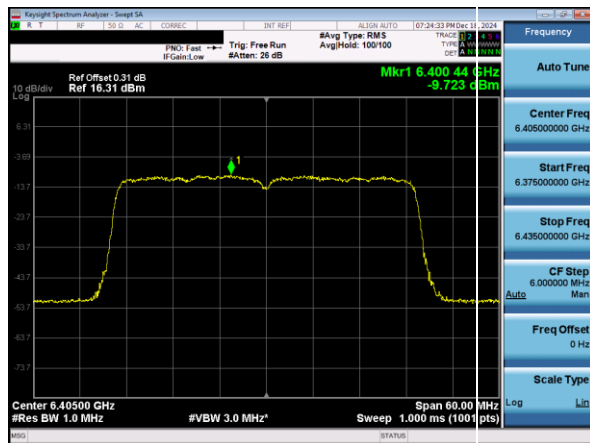
Plot 7-51. Power Spectral Density Plot SDM Primary Antenna 3c (40MHz 802.11ax (UNII Band 5) – Ch. 91)
