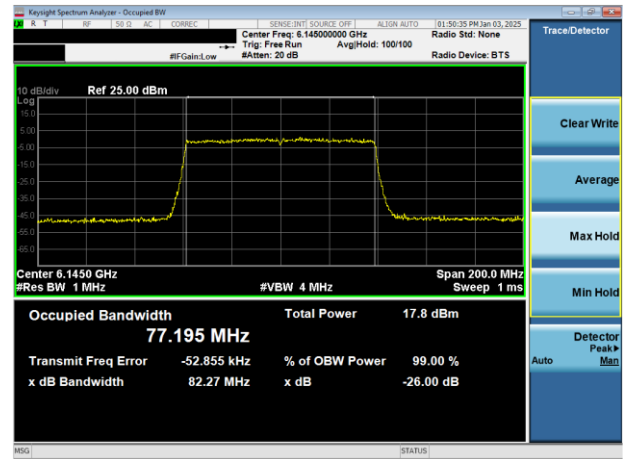
Plot 7-11. 26dB & 99% Bandwidth Plot Antenna 3a (80MHz 802.11ax (UNII Band 5) – Ch. 39)
