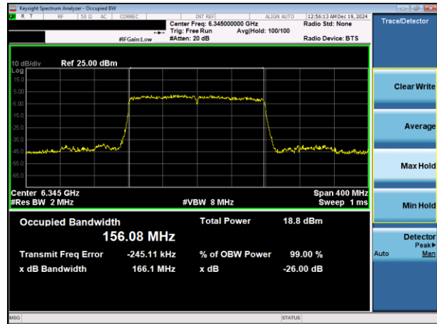
Plot 7-20. 26dB & 99% Bandwidth Plot Antenna 1b (160MHz 802.11ax (UNII Band 5) – Ch. 79)
