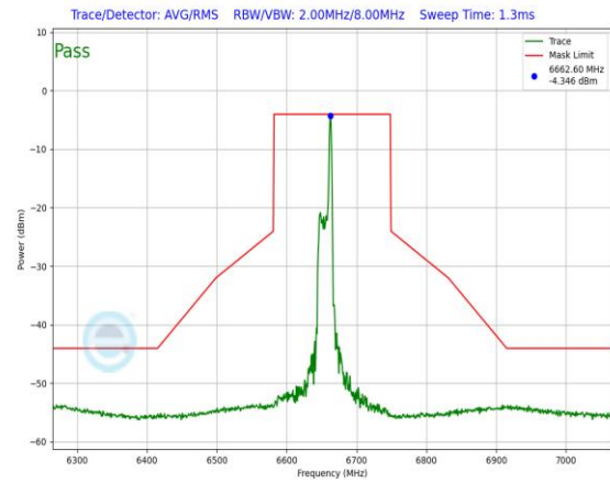
Plot 7-660. In-Band Emission Plot Antenna 3a (160MHz 802.11ax RU26 (UNII Band 7) – Ch. 143)
