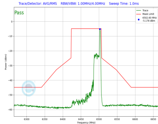
Plot 7-651. In-Band Emission Plot Antenna 3a (80MHz 802.11ax RU26 (UNII Band 6) – Ch. 103)
