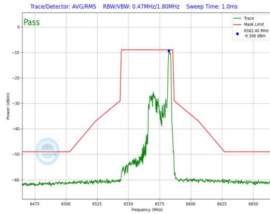
Plot 7-658. In-Band Emission Plot Antenna 3a (40MHz 802.11ax RU26 (UNII Band 7) – Ch. 123)
