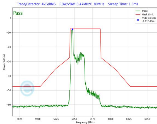
Plot 7-642. In-Band Emission Plot Antenna 3a (40MHz 802.11ax RU26 (UNII Band 5) – Ch. 3)
