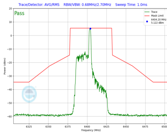
Plot 7-731. In-Band Emission Plot CDD Primary Antenna 3c (40MHz 802.11ax RU26 (UNII Band 5) – Ch. 91)
