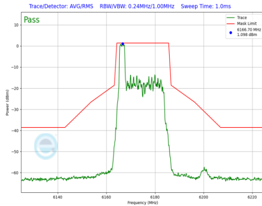
Plot 7-729. In-Band Emission Plot CDD Primary Antenna 3c (20MHz 802.11ax RU26 (UNII Band 5) – Ch. 45)
