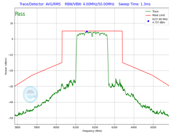
Plot 7-624. In-Band Emission Plot Antenna 3a (160MHz 802.11ax RU996x2 (UNII Band 5) – Ch. 47)
