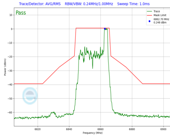
Plot 7-633. In-Band Emission Plot Antenna 3a (20MHz 802.11ax RU26 (UNII Band 7) – Ch. 181)
