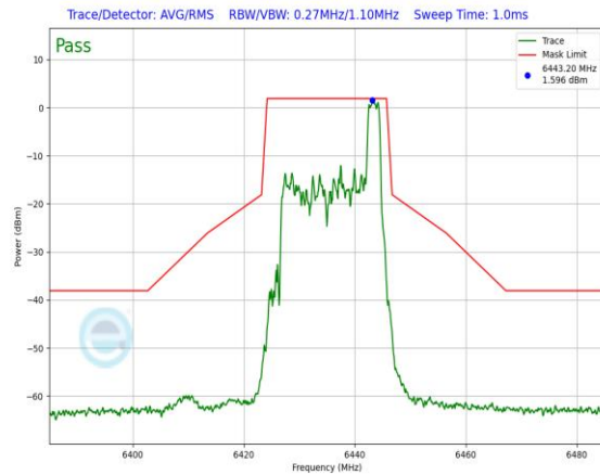
Plot 7-625. In-Band Emission Plot Antenna 3a (20MHz 802.11ax RU26 (UNII Band 6) – Ch. 97)
