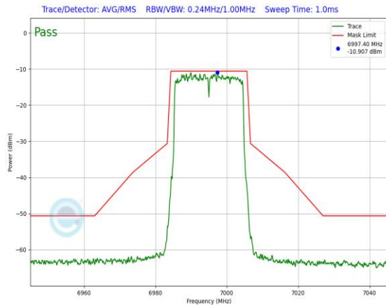
Plot 7-669. In-Band Emission Plot Antenna 3a (20MHz 802.11ax RU242 (UNII Band 8) – Ch. 209)
