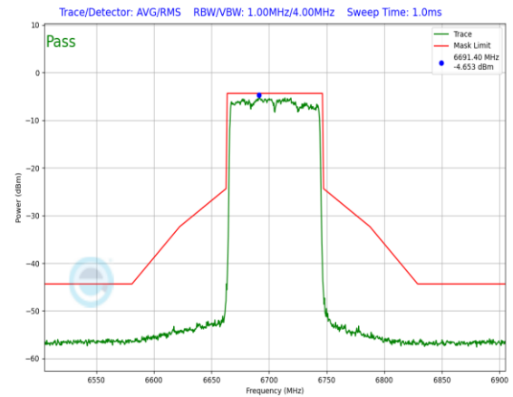
Plot 7-663. In-Band Emission Plot Antenna 3a (80MHz 802.11ax RU996 (UNII Band 7) – Ch. 151)
