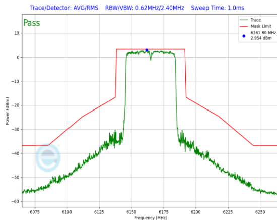
Plot 7-739. In-Band Emission Plot CDD Primary Antenna 3c (40MHz) 802.11ax RU484 (UNII Band 5) – Ch. 43)
