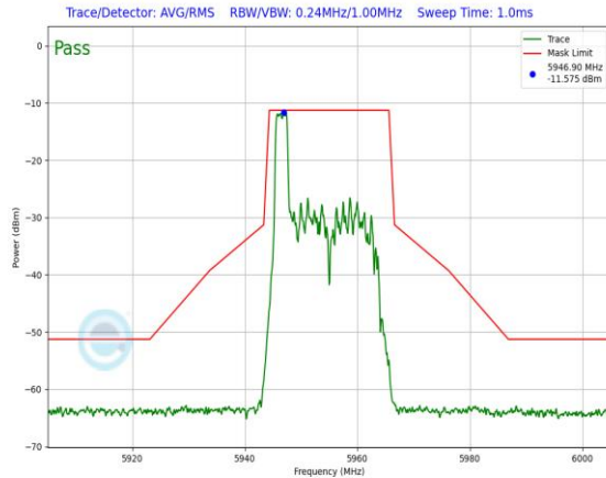
Plot 7-641. In-Band Emission Plot Antenna 3a (20MHz 802.11ax RU26 (UNII Band 5) – Ch. 1)
