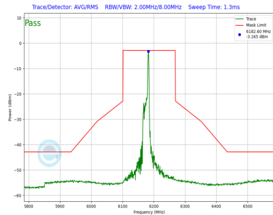
Plot 7-644. In-Band Emission Plot Antenna 3a (160MHz 802.11ax RU26 (UNII Band 5) – Ch. 47)
