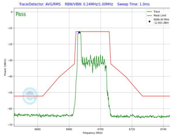
Plot 7-713. In-Band Emission Plot Antenna 1b (20MHz 802.11ax RU26 (UNII Band 7) – Ch. 149)
