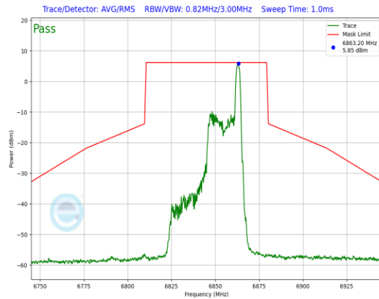
Plot 7-634. In-Band Emission Plot Antenna 3a (40MHz 802.11ax RU26 (UNII Band 7) – Ch. 179)
