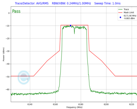
Plot 7-701. In-Band Emission Plot Antenna 1b (20MHz 802.11ax RU242 (UNII Band 5) – Ch. 45)
