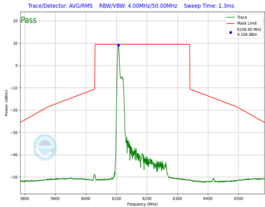
Plot 7-736. In-Band Emission Plot CDD Primary Antenna 3a (160MHz 802.11ax RU26 (UNII Band 5) – Ch. 47)
