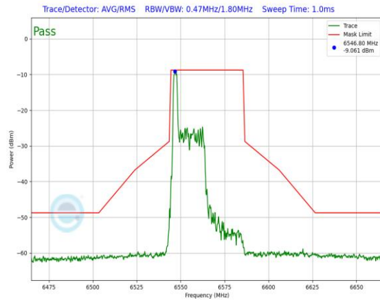
Plot 7-714. In-Band Emission Plot Antenna 1b (40MHz 802.11ax RU26 (UNII Band 7) – Ch. 123)
