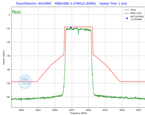
Plot 7-670. In-Band Emission Plot Antenna 3a (40MHz 802.11ax RU484 (UNII Band 8) – Ch. 187)
