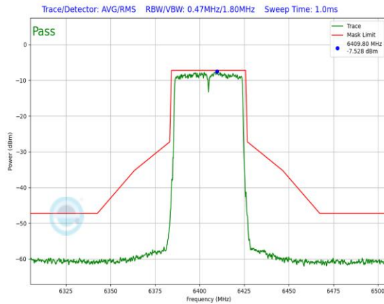
Plot 7-646. In-Band Emission Plot Antenna 3a (40MHz 802.11ax RU484 (UNII Band 5) – Ch. 91)
