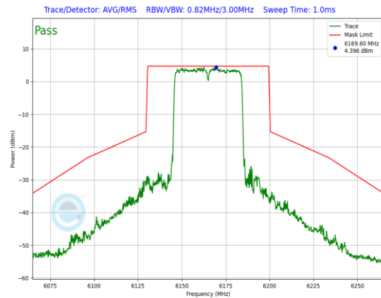
Plot 7-740. In-Band Emission Plot CDD Primary Antenna 3a (40MHz) 802.11ax RU484 (UNII Band 5) – Ch. 43)
