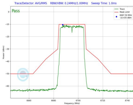
Plot 7-717. In-Band Emission Plot Antenna 1b (20MHz 802.11ax RU242 (UNII Band 7) – Ch. 149)
