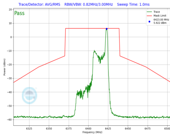
Plot 7-674. In-Band Emission Plot Antenna 1b (40MHz 802.11ax RU26 (UNII Band 5) – Ch. 91)
