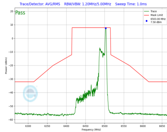
Plot 7-683. In-Band Emission Plot Antenna 1b (80MHz 802.11ax RU26 (UNII Band 6) – Ch. 103)
