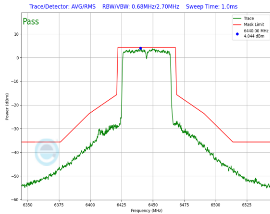
Plot 7-630. In-Band Emission Plot Antenna 3a (40MHz 802.11ax RU484 (UNII Band 6) – Ch. 99)
