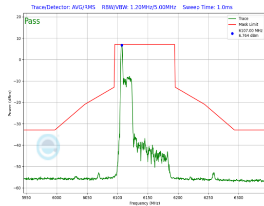
Plot 7-734. In-Band Emission Plot CDD Primary Antenna 3a (80MHz 802.11ax RU26 (UNII Band 5) – Ch. 39)
