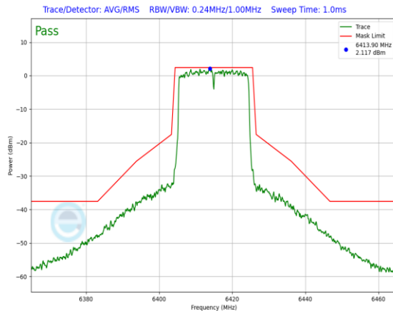
Plot 7-738. In-Band Emission Plot CDD Primary Antenna 3a (20MHz) 802.11ax RU242 (UNII Band 5) – Ch. 93)
