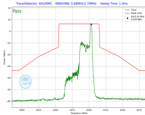
Plot 7-682. In-Band Emission Plot Antenna 1b (40MHz 802.11ax RU26 (UNII Band 6) – Ch. 107)
