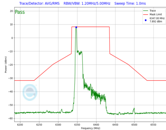
Plot 7-675. In-Band Emission Plot Antenna 1b (80MHz 802.11ax RU26 (UNII Band 5) – Ch. 87)
