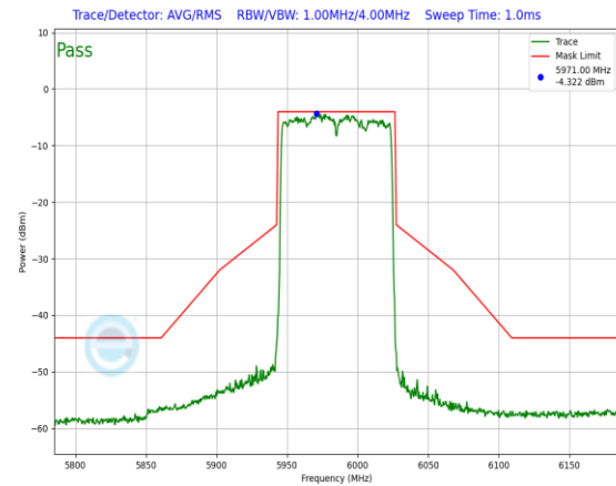
Plot 7-647. In-Band Emission Plot Antenna 3a (80MHz 802.11ax RU996 (UNII Band 5) – Ch. 7)
