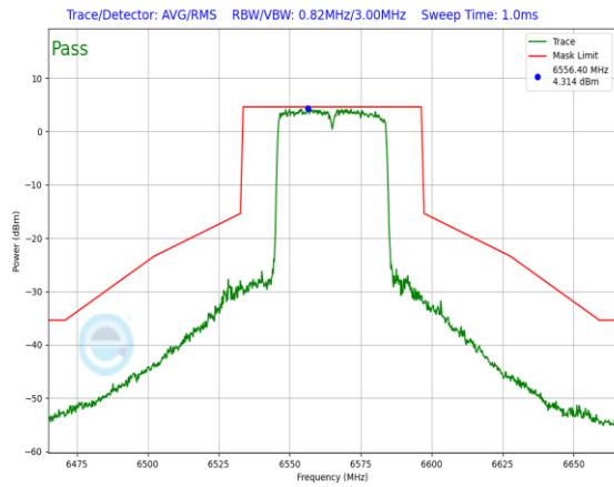
Plot 7-638. In-Band Emission Plot Antenna 3a (40MHz 802.11ax RU484 (UNII Band 7) – Ch. 123)
