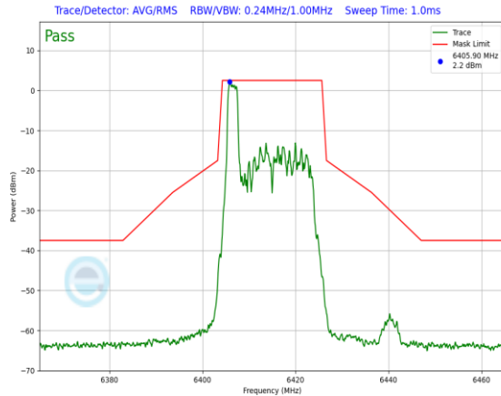
Plot 7-673. In-Band Emission Plot Antenna 1b (20MHz 802.11ax RU26 (UNII Band 5) – Ch. 93)
