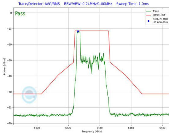
Plot 7-705. In-Band Emission Plot Antenna 1b (20MHz 802.11ax RU26 (UNII Band 6) – Ch. 97)
