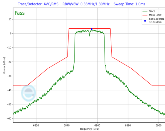
Plot 7-693. In-Band Emission Plot Antenna 1b (20MHz 802.11ax RU242 (UNII Band 7) – Ch. 181)
