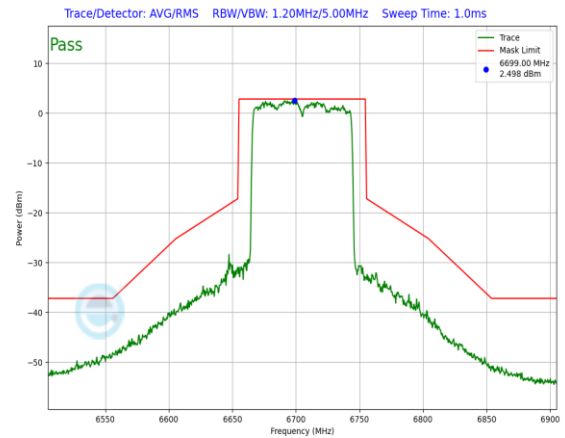
Plot 7-639. In-Band Emission Plot Antenna 3a (80MHz 802.11ax RU996 (UNII Band 7) – Ch. 151)
