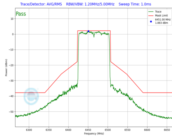
Plot 7-631. In-Band Emission Plot Antenna 3a (80MHz 802.11ax RU996 (UNII Band 6) – Ch. 103)
