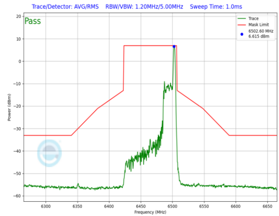
Plot 7-627. In-Band Emission Plot Antenna 3a (80MHz 802.11ax RU26 (UNII Band 6) – Ch. 103)
