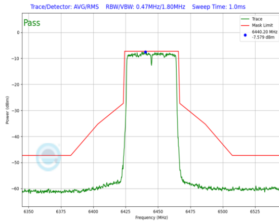
Plot 7-710. In-Band Emission Plot Antenna 1b (40MHz 802.11ax RU484 (UNII Band 6) – Ch. 99)
