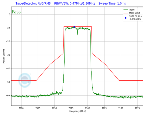
Plot 7-726. In-Band Emission Plot Antenna 1b (40MHz 802.11ax RU484 (UNII Band 8) – Ch. 227)
