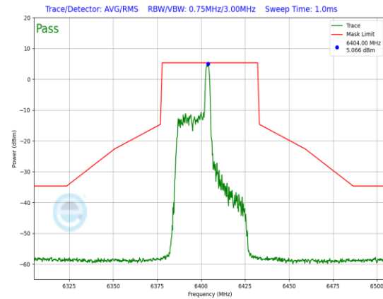
Plot 7-732. In-Band Emission Plot CDD Primary Antenna 3a (40MHz 802.11ax RU26 (UNII Band 5) – Ch. 91)
