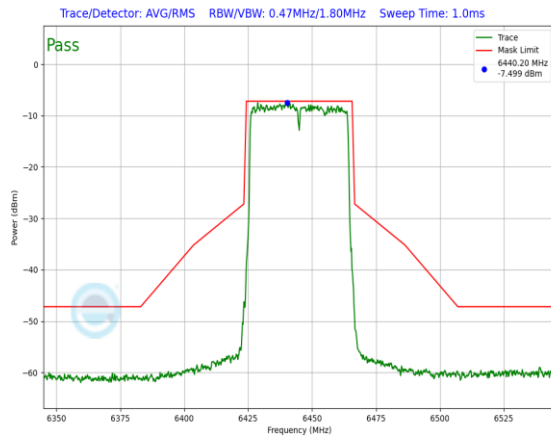
Plot 7-654. In-Band Emission Plot Antenna 3a (40MHz 802.11ax RU484 (UNII Band 6) – Ch. 99)
