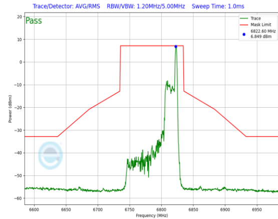
Plot 7-635. In-Band Emission Plot Antenna 3a (80MHz 802.11ax RU26 (UNII Band 7) – Ch. 167)
