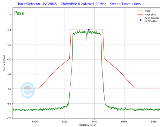
Plot 7-709. In-Band Emission Plot Antenna 1b (20MHz 802.11ax RU242 (UNII Band 6) – Ch. 97)
