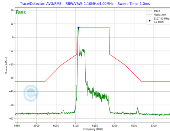
Plot 7-733. In-Band Emission Plot CDD Primary Antenna 3c (80MHz 802.11ax RU26 (UNII Band 5) – Ch. 39)
