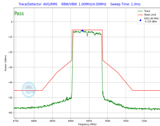
Plot 7-727. In-Band Emission Plot Antenna 1b (80MHz 802.11ax RU996 (UNII Band 8) – Ch. 199)
