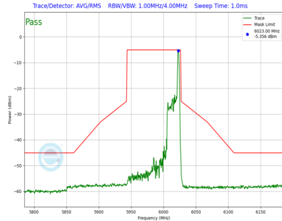
Plot 7-699. In-Band Emission Plot Antenna 1b (80MHz 802.11ax RU26 (UNII Band 5) – Ch. 7)
