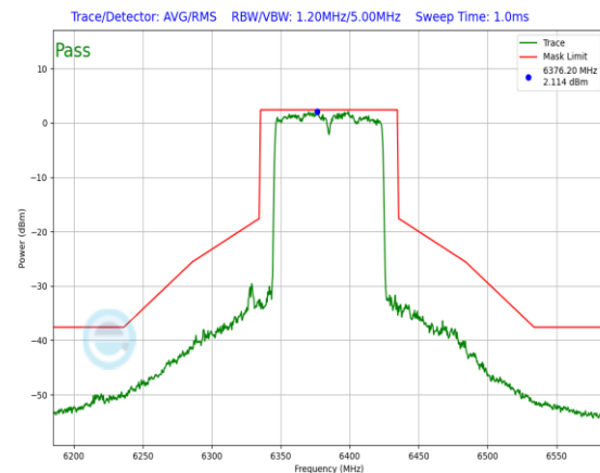
Plot 7-742. In-Band Emission Plot CDD Primary Antenna 3a (80MHz) 802.11ax RU996 (UNII Band 5) – Ch. 87)
