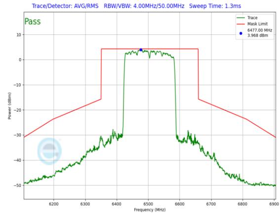
Plot 7-632. In-Band Emission Plot Antenna 3a (160MHz 802.11ax RU996x2 (UNII Band 6) – Ch. 111)
