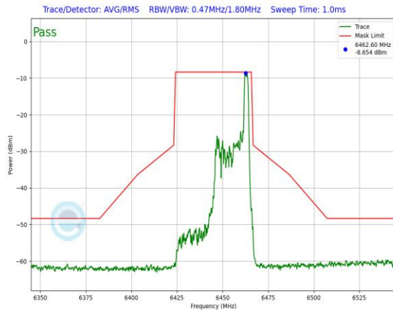
Plot 7-706. In-Band Emission Plot Antenna 1b (40MHz 802.11ax RU26 (UNII Band 6) – Ch. 99)
