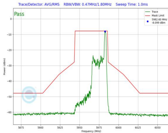
Plot 7-698. In-Band Emission Plot Antenna 1b (40MHz 802.11ax RU26 (UNII Band 5) – Ch. 3)
