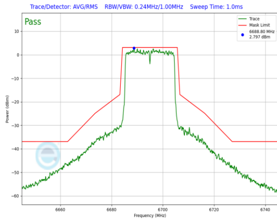
Plot 7-637. In-Band Emission Plot Antenna 3a (20MHz 802.11ax RU242 (UNII Band 7) – Ch. 149)
