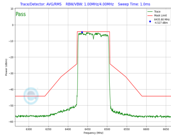
Plot 7-655. In-Band Emission Plot Antenna 3a (80MHz 802.11ax RU996 (UNII Band 6) – Ch. 103)
