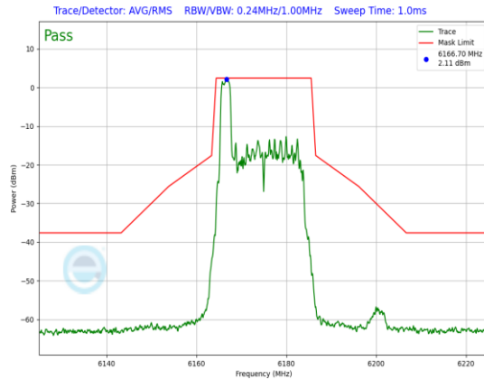
Plot 7-730. In-Band Emission Plot CDD Primary Antenna 3a (20MHz 802.11ax RU26 (UNII Band 5) – Ch. 45)
