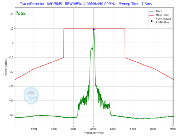
Plot 7-628. In-Band Emission Plot Antenna 3a (160MHz 802.11ax RU26 (UNII Band 6) – Ch. 111)
