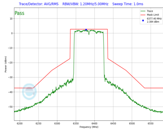
Plot 7-623. In-Band Emission Plot Antenna 3a (80MHz 802.11ax RU996 (UNII Band 5) – Ch. 87)
