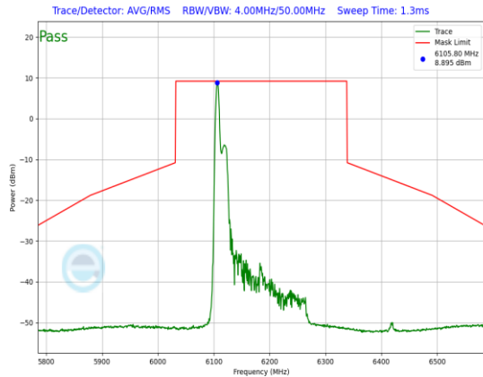
Plot 7-735. In-Band Emission Plot CDD Primary Antenna 3c (160MHz 802.11ax RU26 (UNII Band 5) – Ch. 47)
