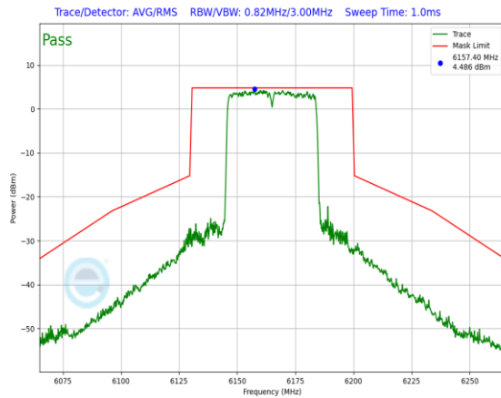
Plot 7-678. In-Band Emission Plot Antenna 1b (40MHz 802.11ax RU484 (UNII Band 5) – Ch. 43)
