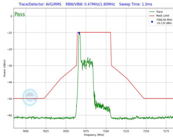
Plot 7-666. In-Band Emission Plot Antenna 3a (40MHz 802.11ax RU26 (UNII Band 8) – Ch. 227)
