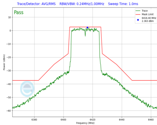
Plot 7-677. In-Band Emission Plot Antenna 1b (20MHz 802.11ax RU242 (UNII Band 5) – Ch. 93)
