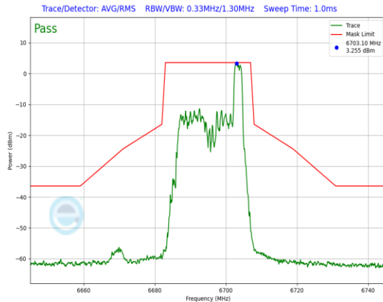
Plot 7-689. In-Band Emission Plot Antenna 1b (20MHz 802.11ax RU26 (UNII Band 7) – Ch. 149)
