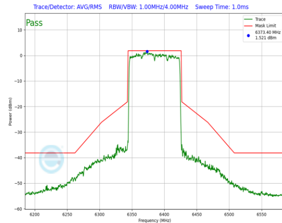
Plot 7-741. In-Band Emission Plot CDD Primary Antenna 3c (80MHz) 802.11ax RU996 (UNII Band 5) – Ch. 87)
