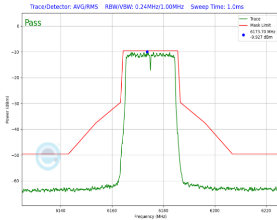
Plot 7-645. In-Band Emission Plot Antenna 3a (20MHz 802.11ax RU242 (UNII Band 5) – Ch. 45)
