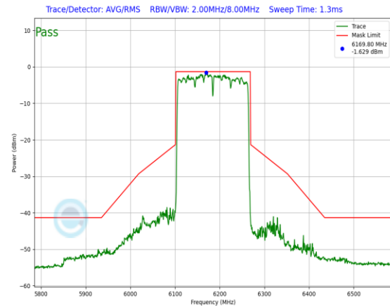
Plot 7-648. In-Band Emission Plot Antenna 3a (160MHz 802.11ax RU26 (UNII Band 5) – Ch. 47)
