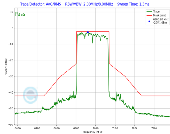
Plot 7-672. In-Band Emission Plot Antenna 3a (160MHz 802.11ax RU26 (UNII Band 8) – Ch. 207)
