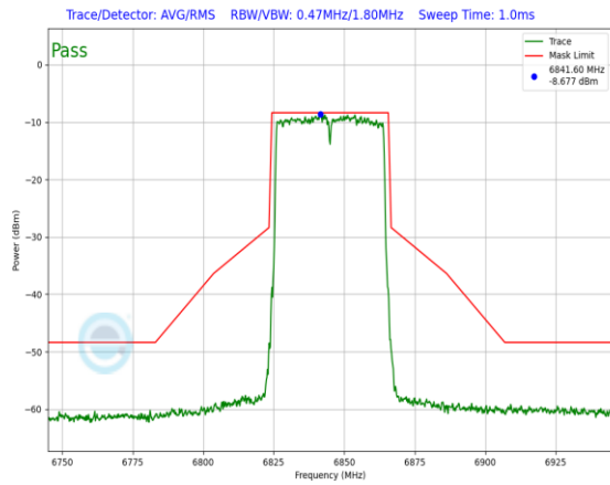
Plot 7-718. In-Band Emission Plot Antenna 1b (40MHz 802.11ax RU484 (UNII Band 7) – Ch. 179)
