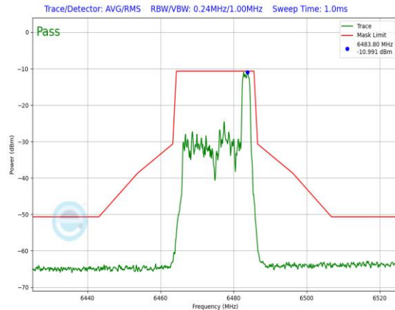
Plot 7-649. In-Band Emission Plot Antenna 3a (20MHz 802.11ax RU26 (UNII Band 6) – Ch. 105)
