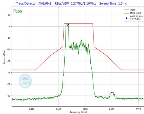
Plot 7-681. In-Band Emission Plot Antenna 1b (20MHz 802.11ax RU26 (UNII Band 6) – Ch. 105)
