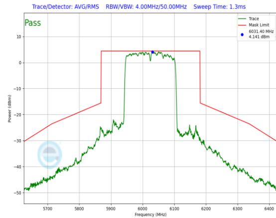
Plot 7-680. In-Band Emission Plot Antenna 1b (160MHz 802.11ax RU996x2 (UNII Band 5) – Ch. 15)
