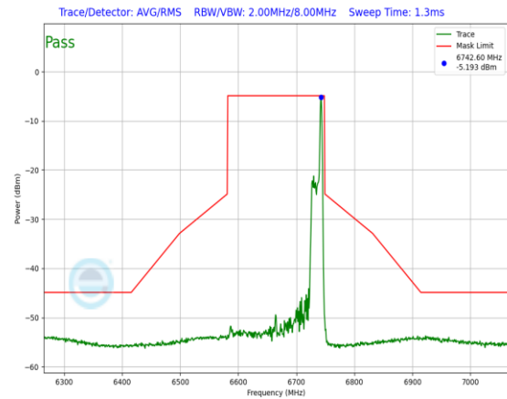
Plot 7-716. In-Band Emission Plot Antenna 1b (160MHz 802.11ax RU26 (UNII Band 7) – Ch. 143)
