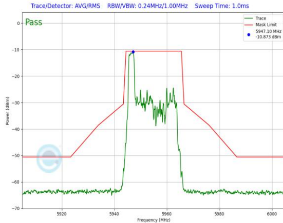
Plot 7-697. In-Band Emission Plot Antenna 1b (20MHz 802.11ax RU26 (UNII Band 5) – Ch. 1)
