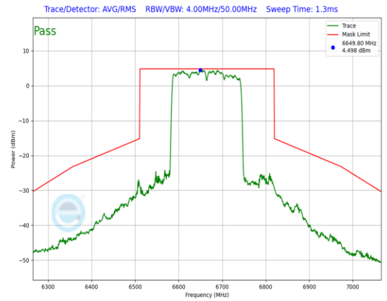
Plot 7-640. In-Band Emission Plot Antenna 3a (160MHz 802.11ax RU996x2 (UNII Band 7) – Ch. 143)
