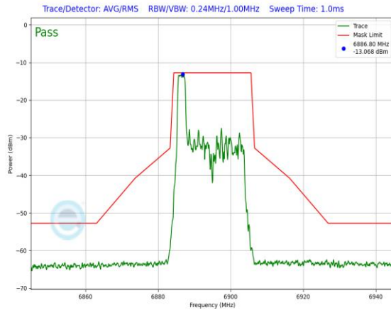
Plot 7-721. In-Band Emission Plot Antenna 1b (20MHz 802.11ax RU26 (UNII Band 8) – Ch. 189)
