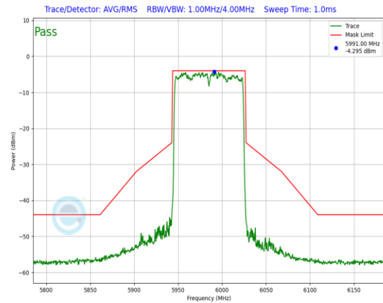
Plot 7-703. In-Band Emission Plot Antenna 1b (80MHz 802.11ax RU996 (UNII Band 5) – Ch. 7)
