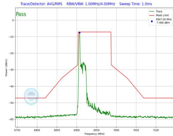
Plot 7-667. In-Band Emission Plot Antenna 3a (80MHz 802.11ax RU26 (UNII Band 8) – Ch.199)
