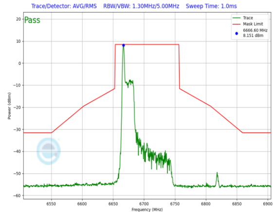
Plot 7-691. In-Band Emission Plot Antenna 1b (80MHz 802.11ax RU26 (UNII Band 7) – Ch. 151)
