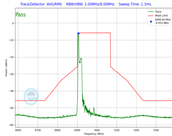
Plot 7-668. In-Band Emission Plot Antenna 3a (160MHz 802.11ax RU26 (UNII Band 8) – Ch. 207)
