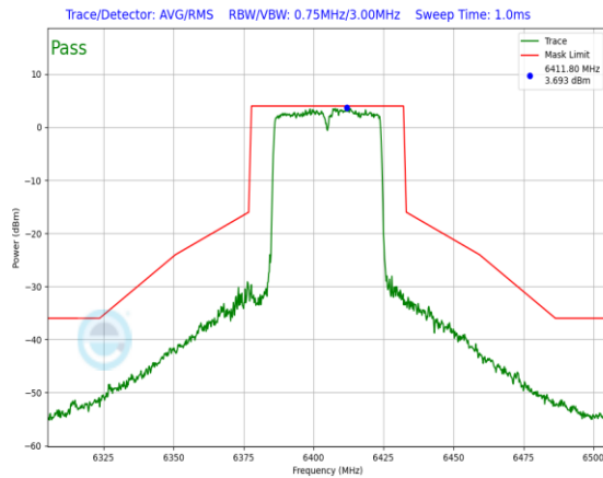
Plot 7-622. In-Band Emission Plot Antenna 3a (40MHz 802.11ax RU484 (UNII Band 5) – Ch. 91)
