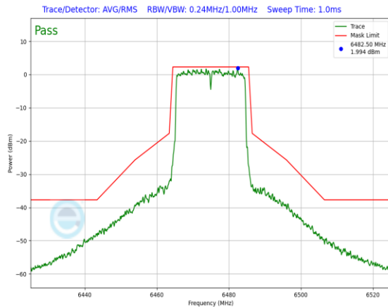
Plot 7-629. In-Band Emission Plot Antenna 3a (20MHz 802.11ax RU242 (UNII Band 6) – Ch. 105
