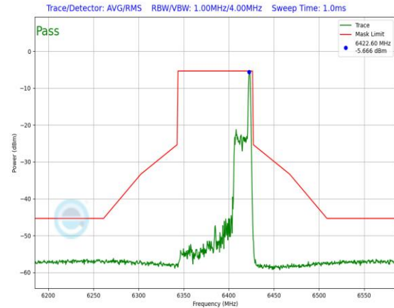
Plot 7-643. In-Band Emission Plot Antenna 3a (80MHz 802.11ax RU26 (UNII Band 5) – Ch. 87)
