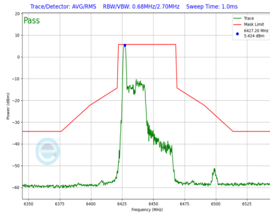
Plot 7-626. In-Band Emission Plot Antenna 3a (40MHz 802.11ax RU26 (UNII Band 6) – Ch. 99)
