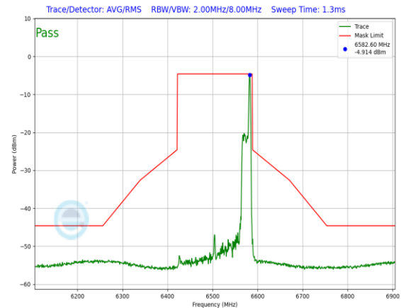
Plot 7-652. In-Band Emission Plot Antenna 3a (160MHz 802.11ax RU26 (UNII Band 6) – Ch. 111)
