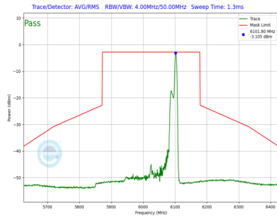
Plot 7-700. In-Band Emission Plot Antenna 1b (160MHz 802.11ax RU26 (UNII Band 5) – Ch. 15)
