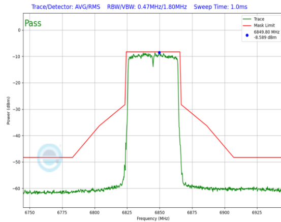
Plot 7-662. In-Band Emission Plot Antenna 3a (40MHz 802.11ax RU484 (UNII Band 7) – Ch. 179)
