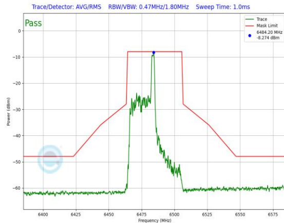
Plot 7-650. In-Band Emission Plot Antenna 3a (40MHz 802.11ax RU26 (UNII Band 6) – Ch. 107)
