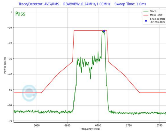
Plot 7-657. In-Band Emission Plot Antenna 3a (20MHz 802.11ax RU26 (UNII Band 7) – Ch. 149)
