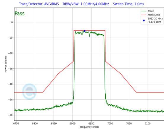
Plot 7-671. In-Band Emission Plot Antenna 3a (80MHz 802.11ax RU996 (UNII Band 8) – Ch. 199)
