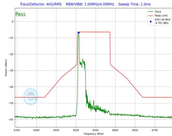
Plot 7-659. In-Band Emission Plot Antenna 3a (80MHz 802.11ax RU26 (UNII Band 7) – Ch. 119)
