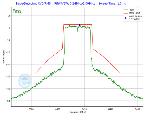
Plot 7-621. In-Band Emission Plot Antenna 3a (20MHz 802.11ax RU242 (UNII Band 5) – Ch. 93)
