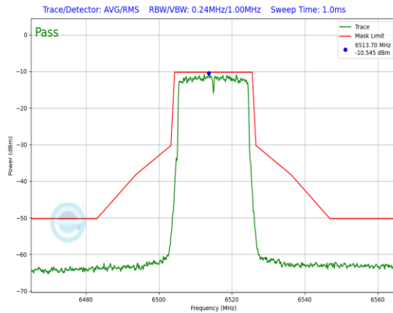
Plot 7-653. In-Band Emission Plot Antenna 3a (20MHz 802.11ax RU242 (UNII Band 6) – Ch. 113)
