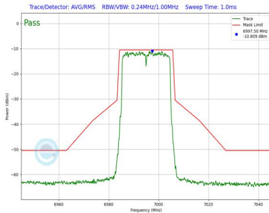
Plot 7-725. In-Band Emission Plot Antenna 1b (20MHz 802.11ax RU242 (UNII Band 8) – Ch. 209)
