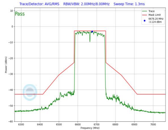
Plot 7-664. In-Band Emission Plot Antenna 3a (160MHz 802.11ax RU26 (UNII Band 7) – Ch. 143)
