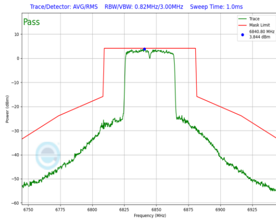
Plot 7-694. In-Band Emission Plot Antenna 1b (40MHz 802.11ax RU484 (UNII Band 7) – Ch. 179)
