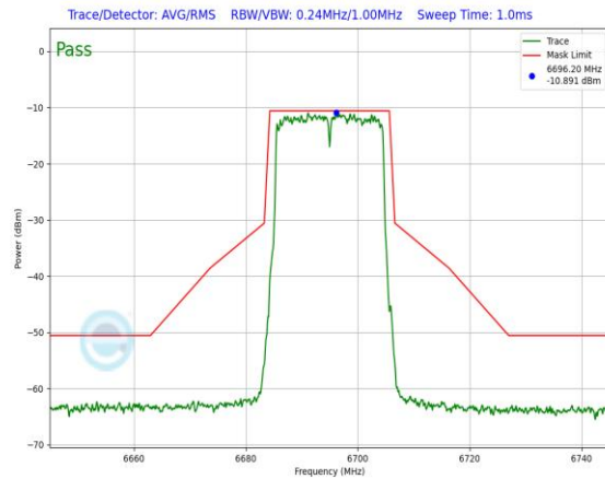
Plot 7-661. In-Band Emission Plot Antenna 3a (20MHz 802.11ax RU242 (UNII Band 7) – Ch. 149)
