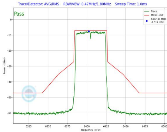
Plot 7-702. In-Band Emission Plot Antenna 1b (40MHz 802.11ax RU484 (UNII Band 5) – Ch. 91)
