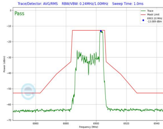
Plot 7-665. In-Band Emission Plot Antenna 3a (20MHz 802.11ax RU26 (UNII Band 8) – Ch. 189)
