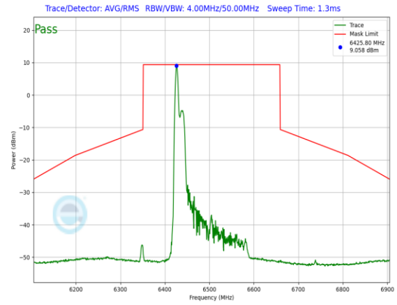
Plot 7-684. In-Band Emission Plot Antenna 1b (160MHz 802.11ax RU26 (UNII Band 6) – Ch. 111)
