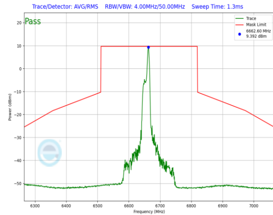
Plot 7-636. In-Band Emission Plot Antenna 3a (160MHz 802.11ax RU26 (UNII Band 7) – Ch. 143)
