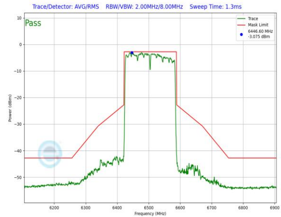
Plot 7-656. In-Band Emission Plot Antenna 3a (160MHz 802.11ax RU26 (UNII Band 6) – Ch. 111)
