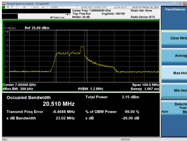
Plot 7-50. 26dB & 99% Bandwidth Plot Antenna 3c (40MHz 802.11ax RU26 (UNII Band 8) – Ch. 211)
