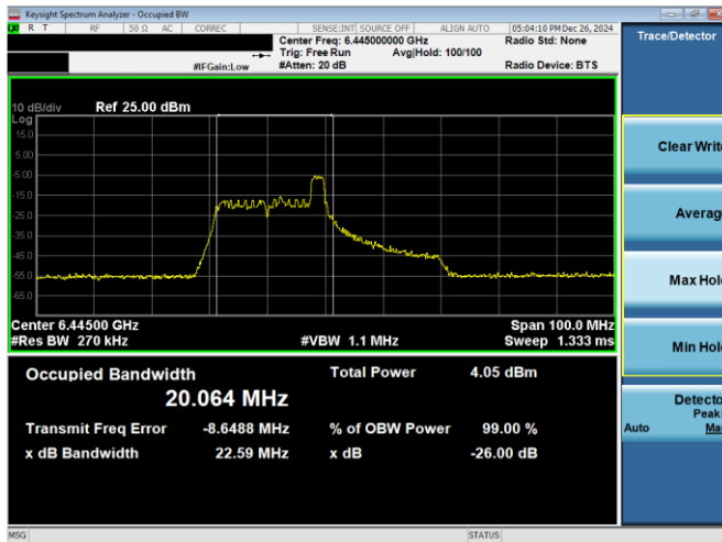
Plot 7-34. 26dB & 99% Bandwidth Plot Antenna 3c (40MHz 802.11ax RU26 (UNII Band 6) – Ch. 99)
