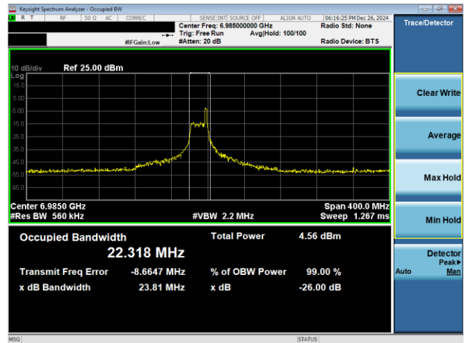
Plot 7-52. 26dB & 99% Bandwidth Plot Antenna 3c (160MHz 802.11ax RU26 (UNII Band 8) – Ch. 207)
