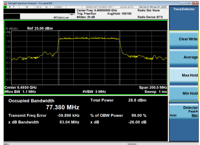
Plot 7-15. 26dB & 99% Bandwidth Plot Antenna 3c (80MHz 802.11ax RU996 (UNII Band 6) – Ch. 103)
