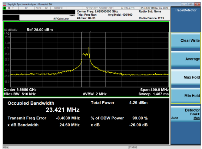
Plot 7-44. 26dB & 99% Bandwidth Plot Antenna 3c (160MHz 802.11ax RU26 (UNII Band 7) – Ch. 143)
