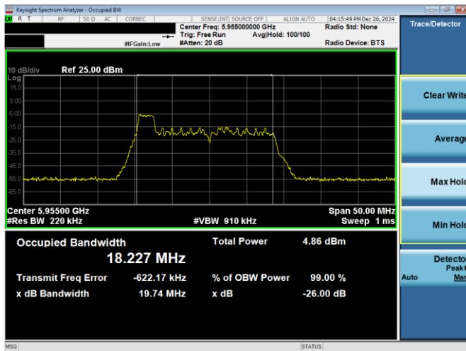
Plot 7-25. 26dB & 99% Bandwidth Plot Antenna 3c (20MHz 802.11ax RU26 (UNII Band 5) – Ch. 1)
