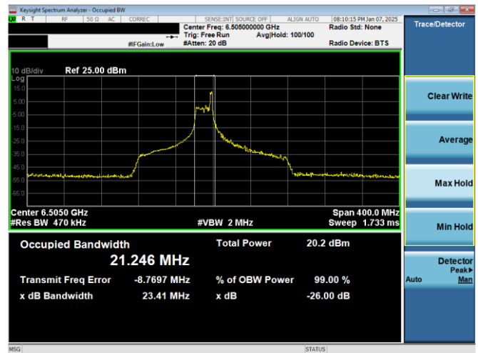
Plot 7-12. 26dB & 99% Bandwidth Plot Antenna 3c (160MHz 802.11ax RU26 (UNII Band 6) – Ch. 111)
