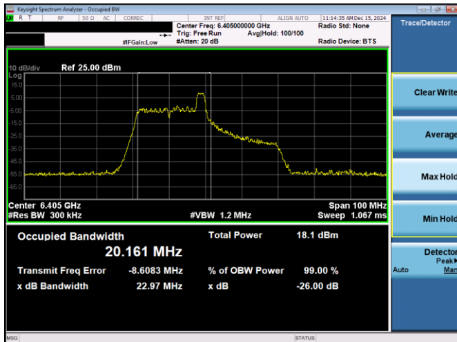
Plot 7-2. 26dB & 99% Bandwidth Plot Antenna 3c (40MHz 802.11ax RU26 (UNII Band 5) – Ch. 91)
