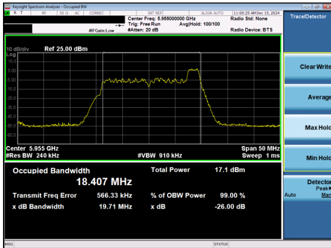
Plot 7-1. 26dB & 99% Bandwidth Plot Antenna 3c (20MHz 802.11ax RU26 (UNII Band 5) – Ch. 1)
