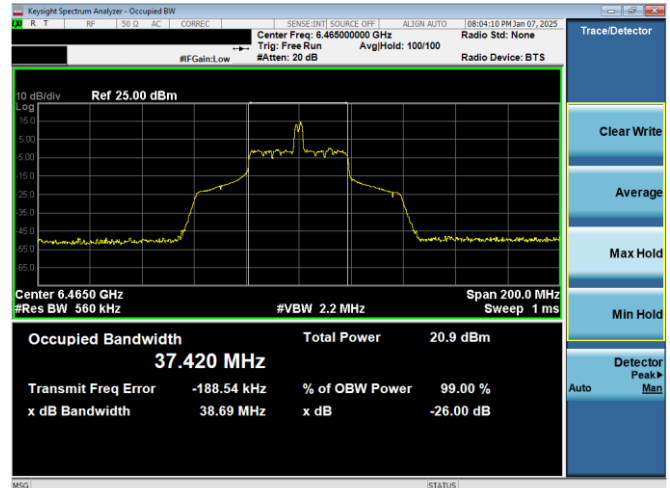
Plot 7-11. 26dB & 99% Bandwidth Plot Antenna 3c (80MHz 802.11ax RU26 (UNII Band 6) – Ch. 103)
