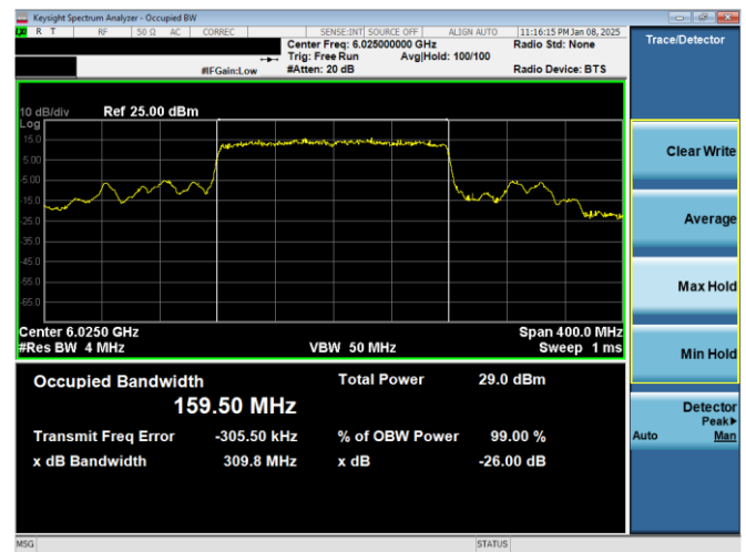
Plot 7-8. 26dB & 99% Bandwidth Plot Antenna 3c (160MHz 802.11ax RU996x2 (UNII Band 5) – Ch. 15)
