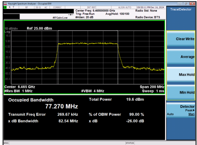
Plot 7-39. 26dB & 99% Bandwidth Plot Antenna 3c (80MHz 802.11ax RU996 (UNII Band 6) – Ch. 103)
