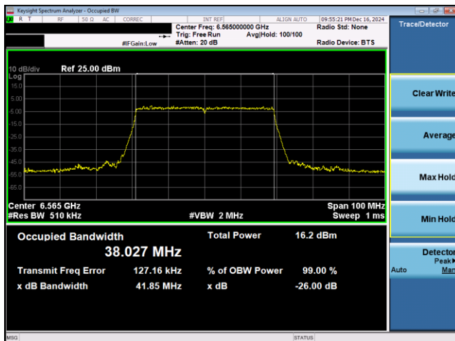
Plot 7-46. 26dB & 99% Bandwidth Plot Antenna 3c (40MHz 802.11ax RU484 (UNII Band 7) – Ch. 123)
