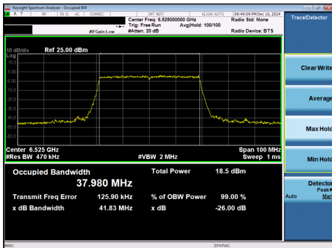
Plot 7-38. 26dB & 99% Bandwidth Plot Antenna 3c (40MHz 802.11ax RU484 (UNII Band 6) – Ch. 115)
