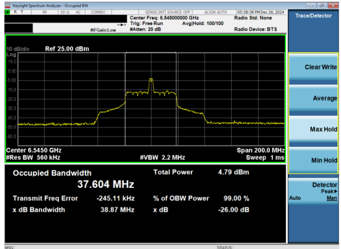
Plot 7-43. 26dB & 99% Bandwidth Plot Antenna 3c (80MHz 802.11ax RU26 (UNII Band 7) – Ch. 119)
