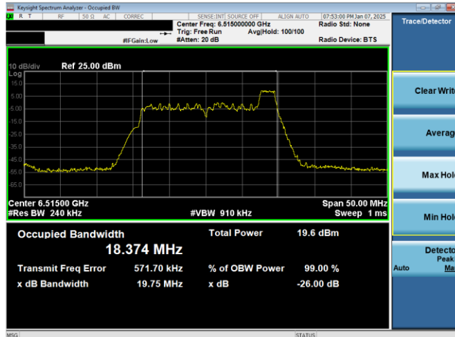
Plot 7-9. 26dB & 99% Bandwidth Plot Antenna 3c (20MHz 802.11ax RU26 (UNII Band 6) – Ch. 113)
