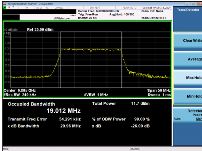
Plot 7-53. 26dB & 99% Bandwidth Plot Antenna 3c (20MHz 802.11ax RU242 (UNII Band 8) – Ch. 189)
