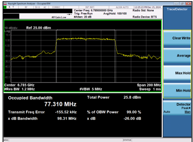
Plot 7-23. 26dB & 99% Bandwidth Plot Antenna 3c (80MHz 802.11ax RU996 (UNII Band 7) – Ch. 167)
