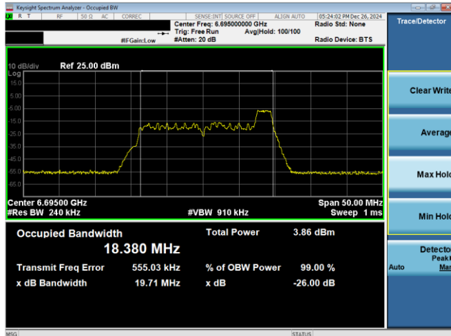
Plot 7-41. 26dB & 99% Bandwidth Plot Antenna 3c (20MHz 802.11ax RU26 (UNII Band 7) – Ch. 149)
