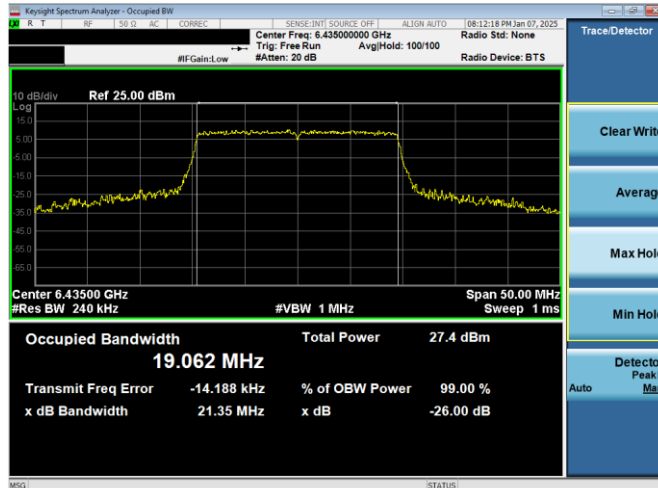
Plot 7-13. 26dB & 99% Bandwidth Plot Antenna 3c (20MHz 802.11ax RU242 (UNII Band 6) – Ch. 97)
