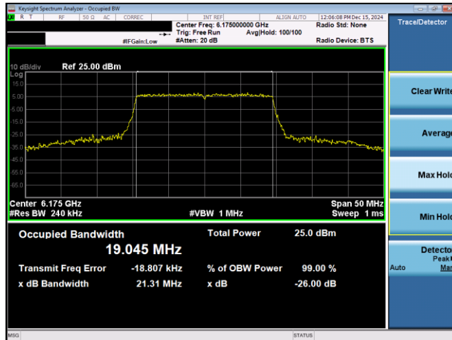
Plot 7-5. 26dB & 99% Bandwidth Plot Antenna 3c (20MHz 802.11ax RU242 (UNII Band 5) – Ch. 45)
