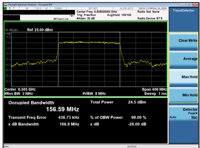
Plot 7-40. 26dB & 99% Bandwidth Plot Antenna 3c (160MHz 802.11ax RU996x2 (UNII Band 6) – Ch. 111)
