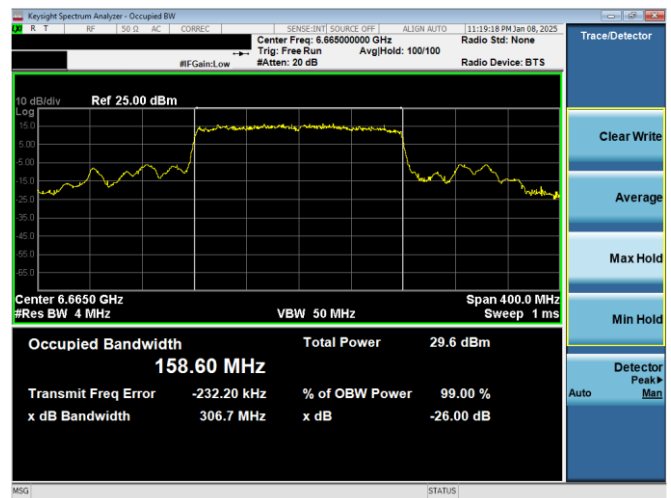
Plot 7-24. 26dB & 99% Bandwidth Plot Antenna 3c (160MHz 802.11ax RU996x2 (UNII Band 7) – Ch. 143)
