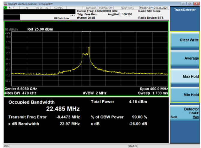
Plot 7-36. 26dB & 99% Bandwidth Plot Antenna 3c (160MHz 802.11ax RU26 (UNII Band 6) – Ch. 111)
