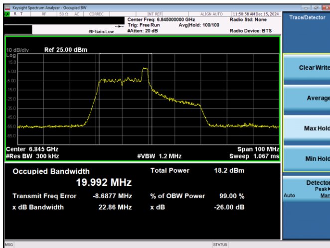
Plot 7-18. 26dB & 99% Bandwidth Plot Antenna 3c (40MHz 802.11ax RU26 (UNII Band 7) – Ch. 179)
