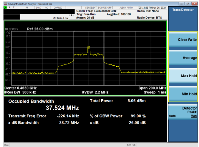
Plot 7-35. 26dB & 99% Bandwidth Plot Antenna 3c (80MHz 802.11ax RU26 (UNII Band 6) – Ch. 103)
