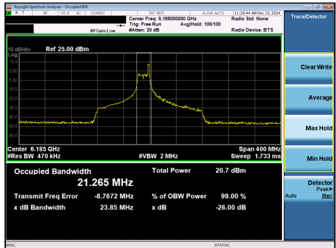
Plot 7-4. 26dB & 99% Bandwidth Plot Antenna 3c (160MHz 802.11ax RU26 (UNII Band 5) – Ch. 47)
