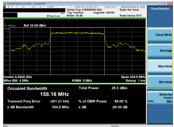
Plot 7-16. 26dB & 99% Bandwidth Plot Antenna 3c (160MHz 802.11ax RU996x2 (UNII Band 6) – Ch. 111)
