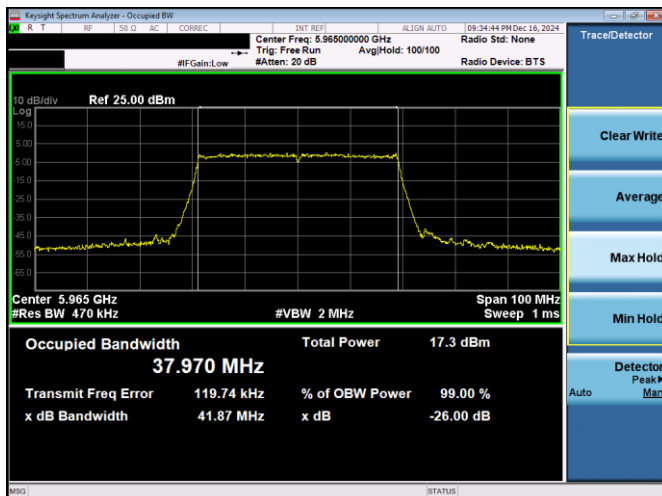
Plot 7-30. 26dB & 99% Bandwidth Plot Antenna 3c (40MHz 802.11ax RU484 (UNII Band 5) – Ch. 3)
