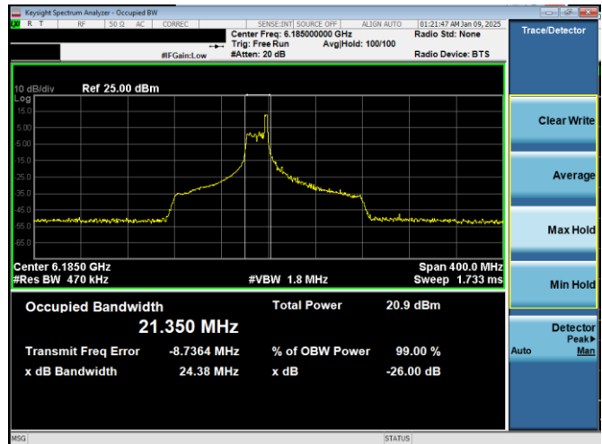
Plot 7-60. 26dB & 99% Bandwidth Plot Antenna 3a (160MHz 802.11ax RU26 (UNII Band 5) – Ch. 47)
