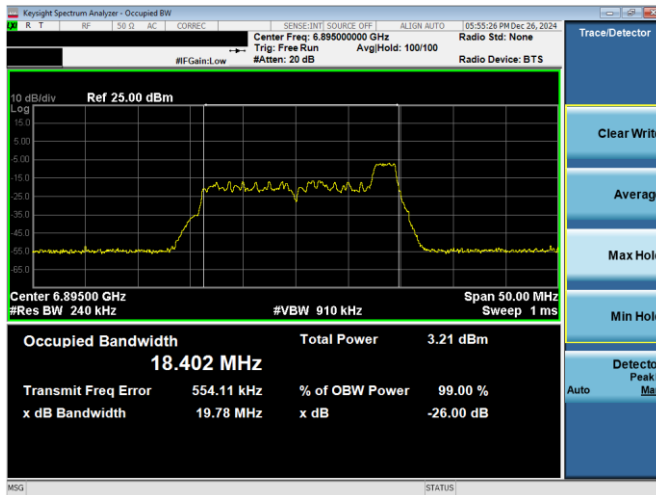
Plot 7-49. 26dB & 99% Bandwidth Plot Antenna 3c (20MHz 802.11ax RU26 (UNII Band 8) – Ch. 189)
