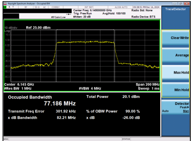
Plot 7-31. 26dB & 99% Bandwidth Plot Antenna 3c (80MHz 802.11ax RU996 (UNII Band 5) – Ch. 39)
