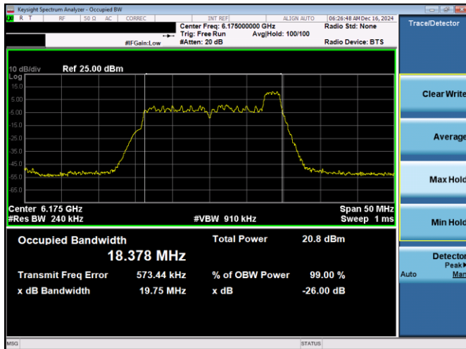
Plot 7-57. 26dB & 99% Bandwidth Plot Antenna 3a (20MHz 802.11ax RU26 (UNII Band 5) – Ch. 45)
