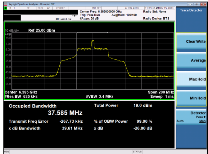
Plot 7-3. 26dB & 99% Bandwidth Plot Antenna 3c (80MHz 802.11ax RU26 (UNII Band 5) – Ch. 87)
