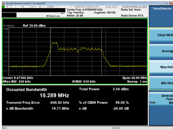
Plot 7-33. 26dB & 99% Bandwidth Plot Antenna 3c (20MHz 802.11ax RU26 (UNII Band 6) – Ch. 105)
