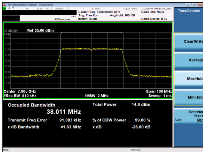
Plot 7-54. 26dB & 99% Bandwidth Plot Antenna 3c (40MHz 802.11ax RU484 (UNII Band 8) – Ch. 211)
