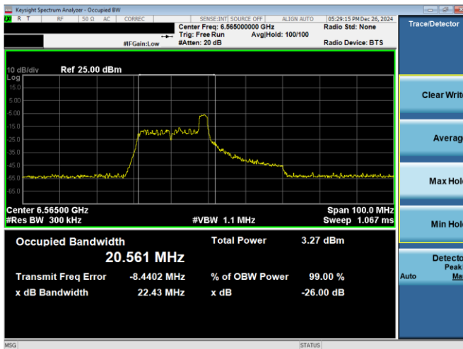
Plot 7-42. 26dB & 99% Bandwidth Plot Antenna 3c (40MHz 802.11ax RU26 (UNII Band 7) – Ch. 123)
