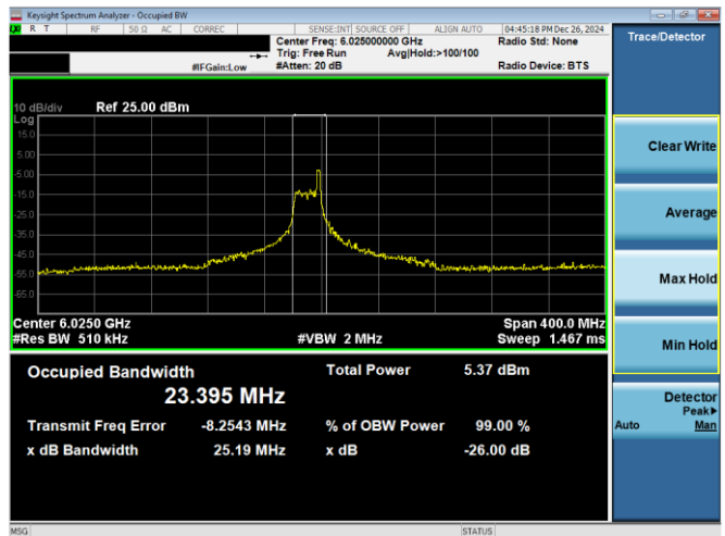
Plot 7-28. 26dB & 99% Bandwidth Plot Antenna 3c (160MHz 802.11ax RU26 (UNII Band 5) – Ch. 15)
