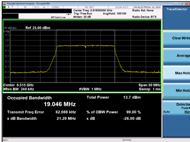
Plot 7-37. 26dB & 99% Bandwidth Plot Antenna 3c (20MHz 802.11ax RU242 (UNII Band 6) – Ch. 113)
