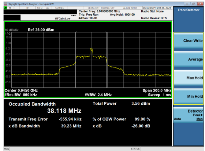
Plot 7-51. 26dB & 99% Bandwidth Plot Antenna 3c (80MHz 802.11ax RU26 (UNII Band 8) – Ch. 199)
