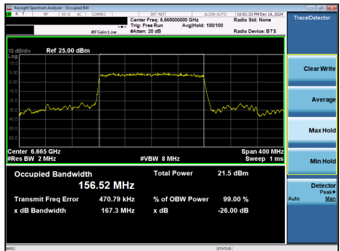
Plot 7-48. 26dB & 99% Bandwidth Plot Antenna 3c (160MHz 802.11ax RU996x2 (UNII Band 7) – Ch. 143)
