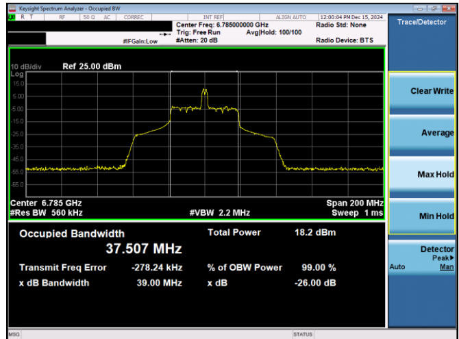
Plot 7-19. 26dB & 99% Bandwidth Plot Antenna 3c (80MHz 802.11ax RU26 (UNII Band 7) – Ch. 167)
