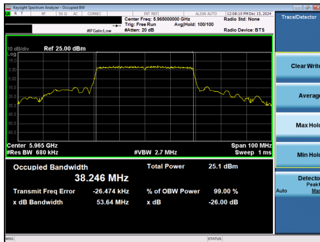
Plot 7-6. 26dB & 99% Bandwidth Plot Antenna 3c (40MHz 802.11ax RU484 (UNII Band 5) – Ch. 3)
