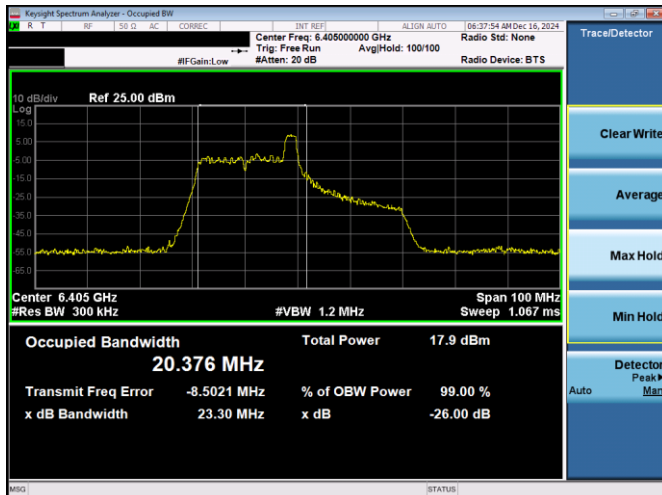
Plot 7-58. 26dB & 99% Bandwidth Plot Antenna 3a (40MHz 802.11ax RU26 (UNII Band 5) – Ch. 91)
