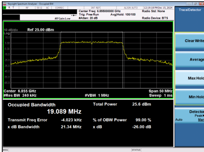
Plot 7-21. 26dB & 99% Bandwidth Plot Antenna 3c (20MHz 802.11ax RU242 (UNII Band 7) – Ch. 181)
