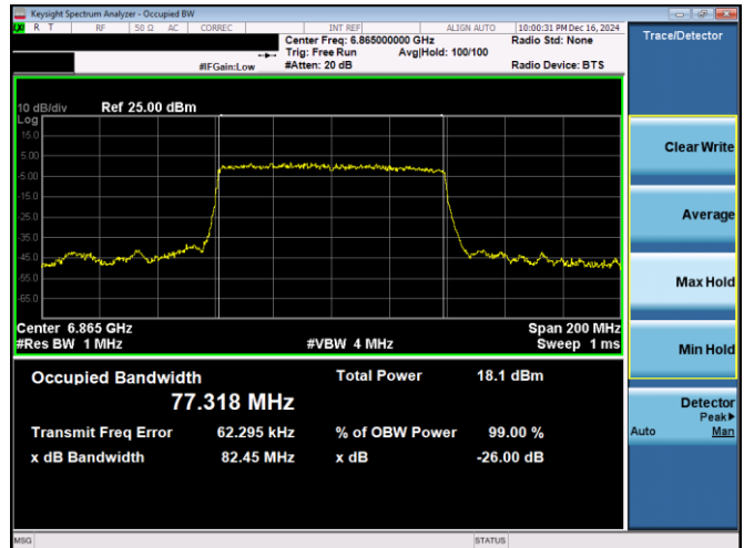
Plot 7-47. 26dB & 99% Bandwidth Plot Antenna 3c (80MHz 802.11ax RU996 (UNII Band 7) – Ch. 183)
