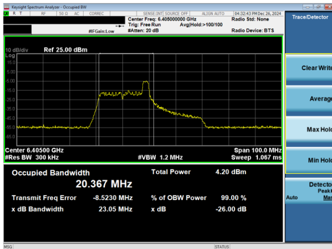
Plot 7-26. 26dB & 99% Bandwidth Plot Antenna 3c (40MHz 802.11ax RU26 (UNII Band 5) – Ch. 91)
