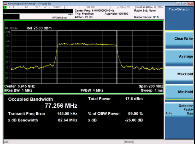
Plot 7-55. 26dB & 99% Bandwidth Plot Antenna 3c (80MHz 802.11ax RU996 (UNII Band 8) – Ch. 199)
