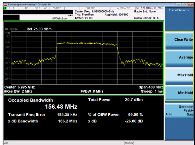
Plot 7-56. 26dB & 99% Bandwidth Plot Antenna 3c (160MHz 802.11ax RU996x2 (UNII Band 8) – Ch. 207)
