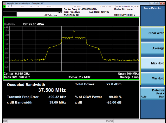
Plot 7-59. 26dB & 99% Bandwidth Plot Antenna 3a (80MHz 802.11ax RU26 (UNII Band 5) – Ch. 39)
