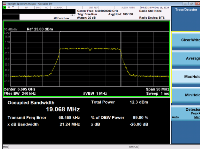
Plot 7-45. 26dB & 99% Bandwidth Plot Antenna 3c (20MHz 802.11ax RU242 (UNII Band 7) – Ch. 149)
