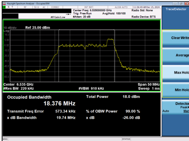
Plot 7-17. 26dB & 99% Bandwidth Plot Antenna 3c (20MHz 802.11ax RU26 (UNII Band 7) – Ch. 117)
