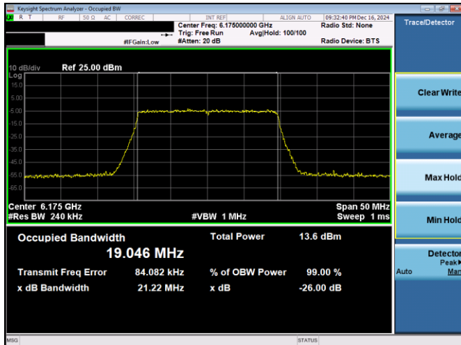
Plot 7-29. 26dB & 99% Bandwidth Plot Antenna 3c (20MHz 802.11ax RU242 (UNII Band 5) – Ch. 45)
