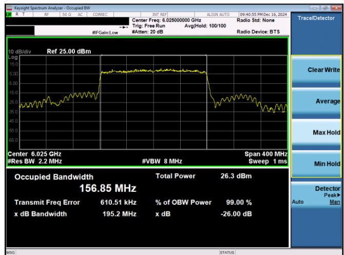
Plot 7-32. 26dB & 99% Bandwidth Plot Antenna 3c (160MHz 802.11ax RU996x2 (UNII Band 5) – Ch. 15)
