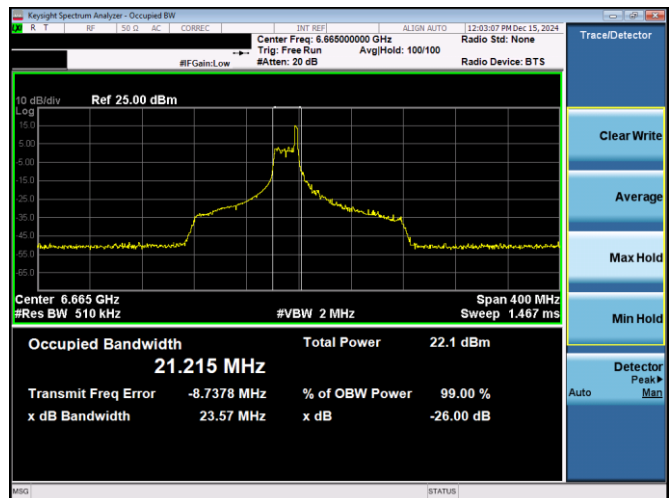
Plot 7-20. 26dB & 99% Bandwidth Plot Antenna 3c (160MHz 802.11ax RU26 (UNII Band 7) – Ch. 143)
