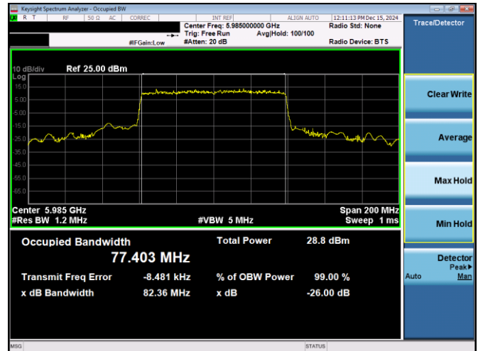
Plot 7-7. 26dB & 99% Bandwidth Plot Antenna 3c (80MHz 802.11ax RU996 (UNII Band 5) – Ch. 7)
