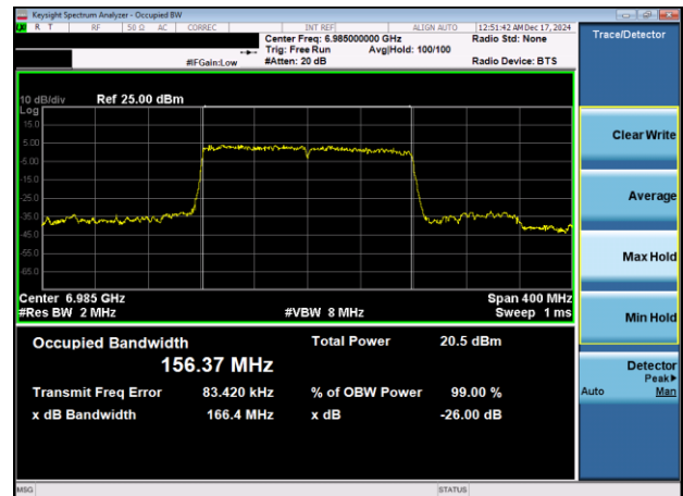
Plot 7-28. 26dB & 99% Bandwidth Plot Antenna 3c (160MHz 802.11ax (UNII Band 8) – Ch. 207)
