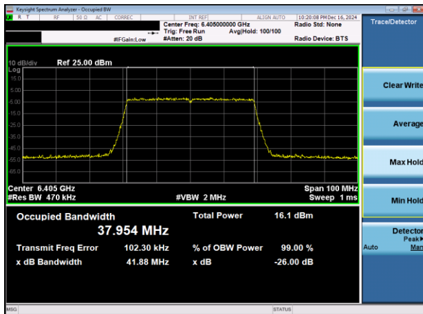
Plot 7-14. 26dB & 99% Bandwidth Plot Antenna 3c (40MHz 802.11ax (UNII Band 5) – Ch. 91)
