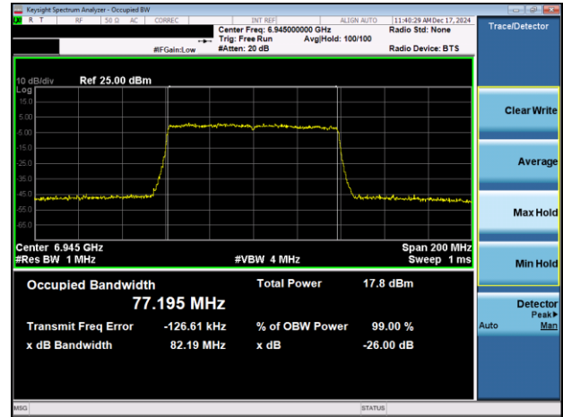
Plot 7-55. 26dB & 99% Bandwidth Plot Antenna 3a (80MHz 802.11ax (UNII Band 8) – Ch. 199)
