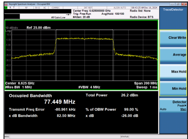
Plot 7-39. 26dB & 99% Bandwidth Plot Antenna 3a (80MHz 802.11ax (UNII Band 7) – Ch. 135)
