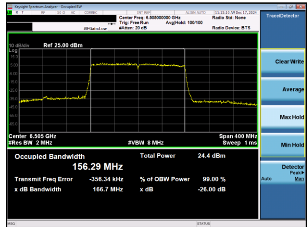
Plot 7-48. 26dB & 99% Bandwidth Plot Antenna 3a (160MHz 802.11ax (UNII Band 6) – Ch. 111)
