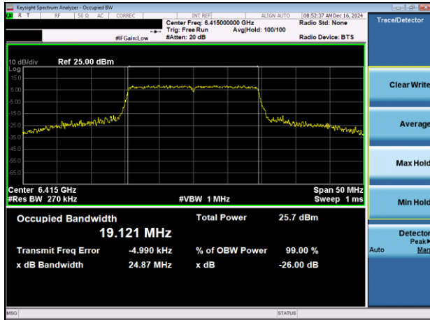
Plot 7-29. 26dB & 99% Bandwidth Plot Antenna 3a (20MHz 802.11ax (UNII Band 5) – Ch. 93)
