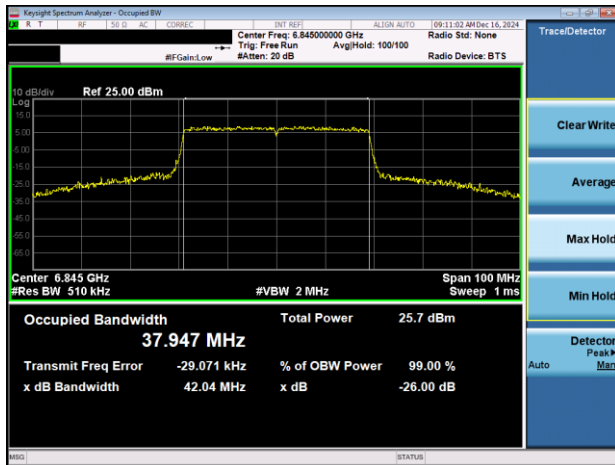
Plot 7-38. 26dB & 99% Bandwidth Plot Antenna 3a (40MHz 802.11ax (UNII Band 7) – Ch. 179)
