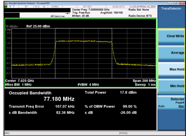
Plot 7-27. 26dB & 99% Bandwidth Plot Antenna 3c (80MHz 802.11ax (UNII Band 8) – Ch. 215)
