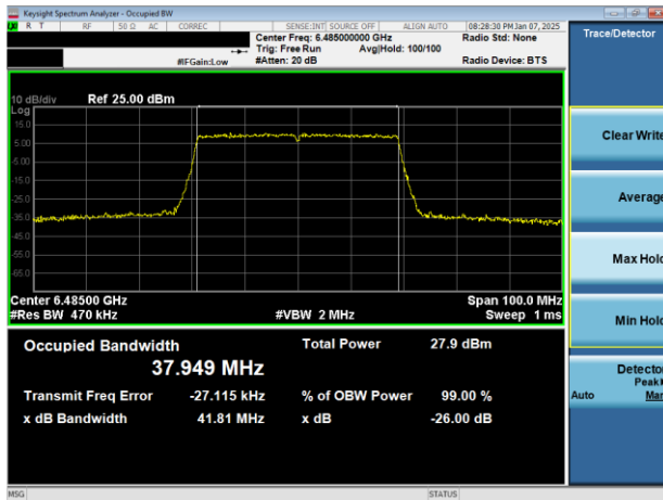
Plot 7-6. 26dB & 99% Bandwidth Plot Antenna 3c (40MHz 802.11ax (UNII Band 6) – Ch. 107)
