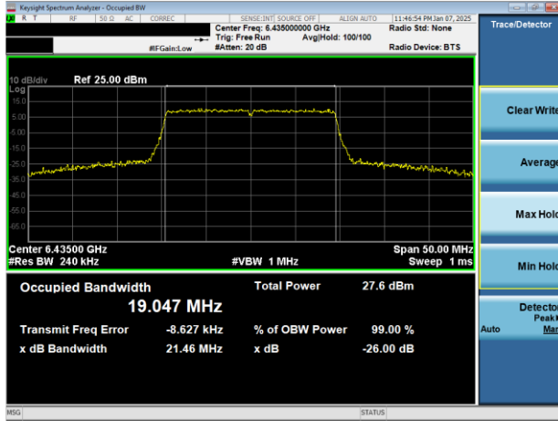
Plot 7-33. 26dB & 99% Bandwidth Plot Antenna 3a (20MHz 802.11ax (UNII Band 6) – Ch. 97)
