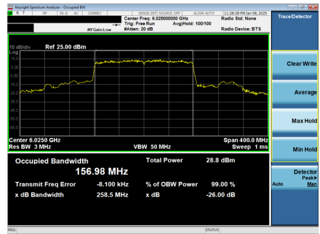
Plot 7-4. 26dB & 99% Bandwidth Plot Antenna 3c (160MHz 802.11ax (UNII Band 5) – Ch. 15)
