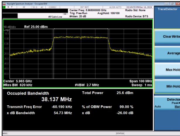
Plot 7-58. 26dB & 99% Bandwidth Plot Antenna 1b (40MHz 802.11ax (UNII Band 5) – Ch. 3)
