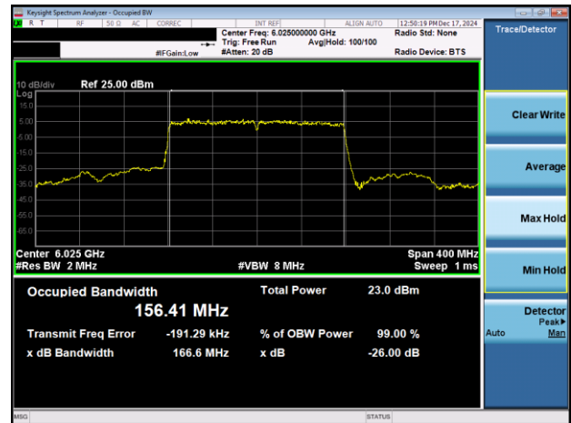
Plot 7-44. 26dB & 99% Bandwidth Plot Antenna 3a (160MHz 802.11ax (UNII Band 5) – Ch. 15)
