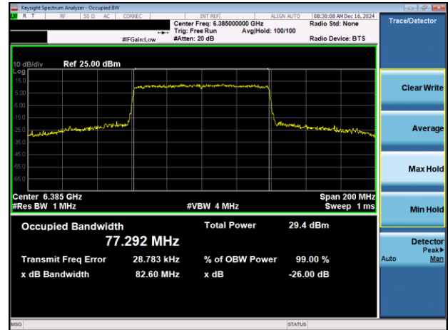
Plot 7-31. 26dB & 99% Bandwidth Plot Antenna 3a (80MHz 802.11ax (UNII Band 5) – Ch. 87)
