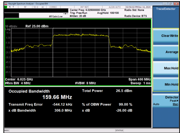
Plot 7-60. 26dB & 99% Bandwidth Plot Antenna 1b (160MHz 802.11ax (UNII Band 5) – Ch. 15)
