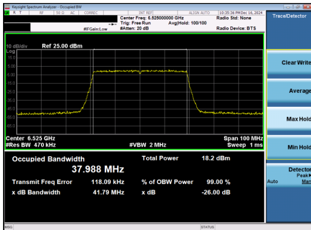
Plot 7-18. 26dB & 99% Bandwidth Plot Antenna 3c (40MHz 802.11ax (UNII Band 6) – Ch. 115)
