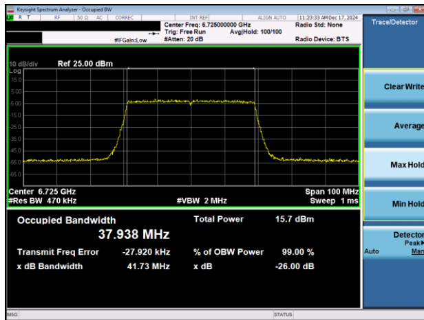
Plot 7-50. 26dB & 99% Bandwidth Plot Antenna 3a (40MHz 802.11ax (UNII Band 7) – Ch. 155)
