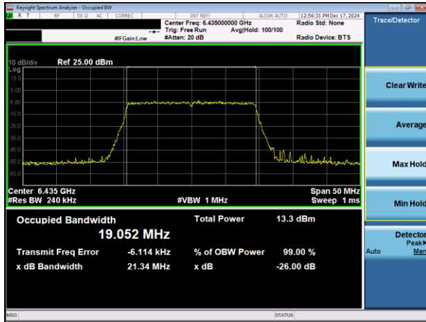
Plot 7-45. 26dB & 99% Bandwidth Plot Antenna 3a (20MHz 802.11ax (UNII Band 6) – Ch. 97)
