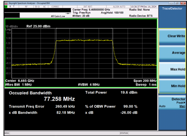
Plot 7-19. 26dB & 99% Bandwidth Plot Antenna 3c (80MHz 802.11ax (UNII Band 6) – Ch. 103)
