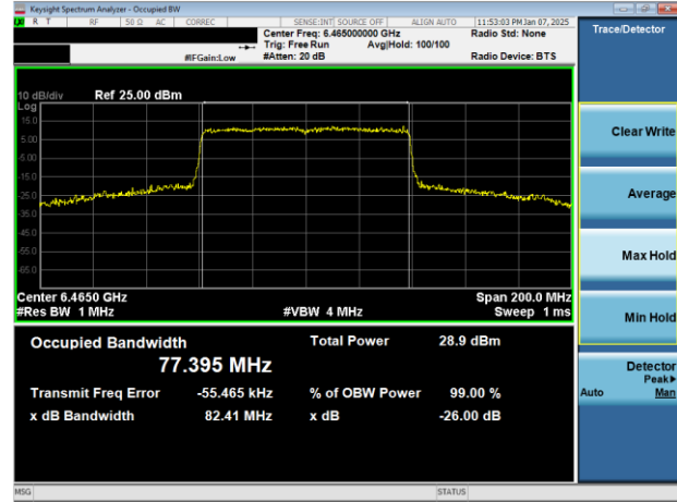
Plot 7-35. 26dB & 99% Bandwidth Plot Antenna 3a (80MHz 802.11ax (UNII Band 6) – Ch. 103)
