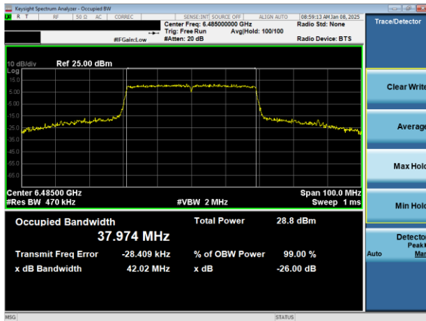
Plot 7-62. 26dB & 99% Bandwidth Plot Antenna 1b (40MHz 802.11ax (UNII Band 6) – Ch. 107)
