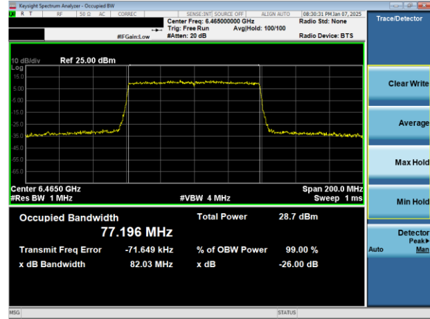
Plot 7-7. 26dB & 99% Bandwidth Plot Antenna 3c (80MHz 802.11ax (UNII Band 6) – Ch. 103)
