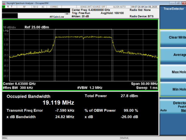
Plot 7-61. 26dB & 99% Bandwidth Plot Antenna 1b (20MHz 802.11ax (UNII Band 6) – Ch. 97)
