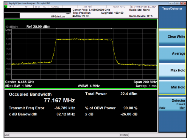
Plot 7-47. 26dB & 99% Bandwidth Plot Antenna 3a (80MHz 802.11ax (UNII Band 6) – Ch. 103)
