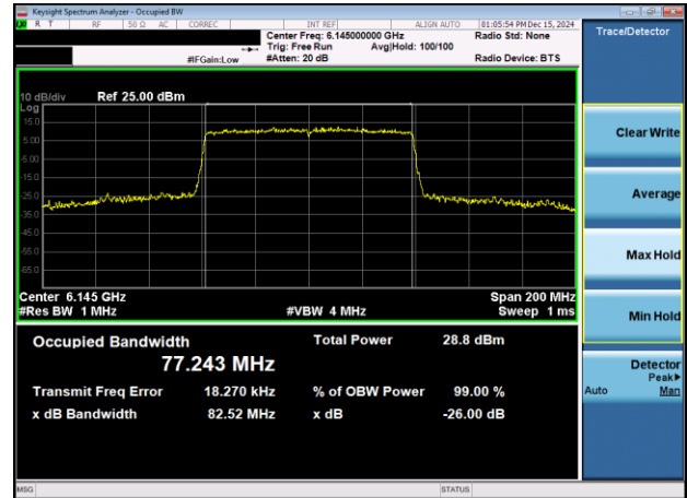
Plot 7-3. 26dB & 99% Bandwidth Plot Antenna 3c (80MHz 802.11ax (UNII Band 5) – Ch. 39)
