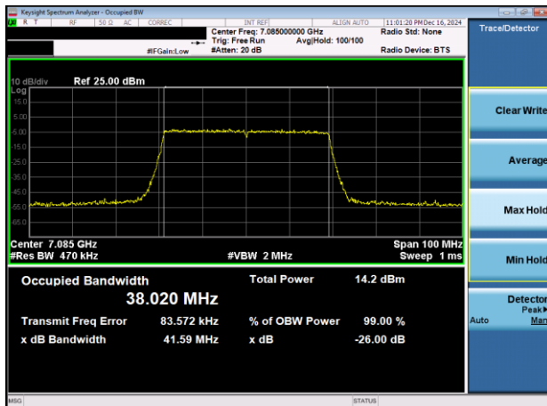
Plot 7-26. 26dB & 99% Bandwidth Plot Antenna 3c (40MHz 802.11ax (UNII Band 8) – Ch. 227)
