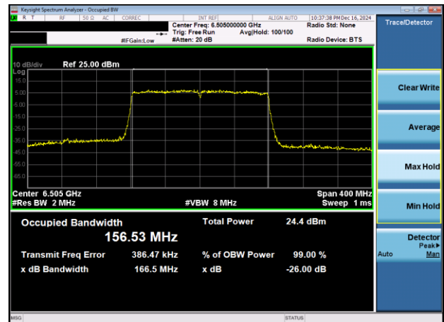
Plot 7-20. 26dB & 99% Bandwidth Plot Antenna 3c (160MHz 802.11ax (UNII Band 6) – Ch. 111)
