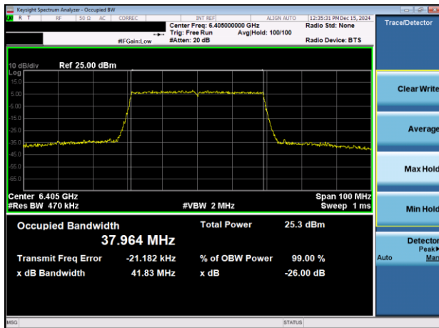
Plot 7-2. 26dB & 99% Bandwidth Plot Antenna 3c (40MHz 802.11ax (UNII Band 5) – Ch. 91)
