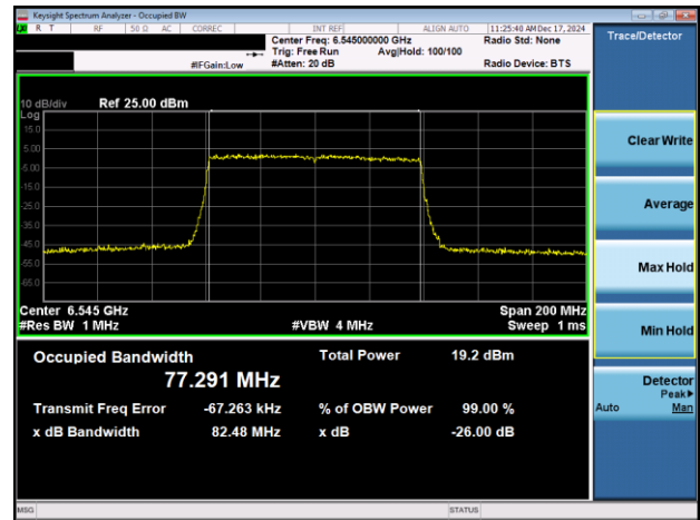
Plot 7-51. 26dB & 99% Bandwidth Plot Antenna 3a (80MHz 802.11ax (UNII Band 7) – Ch. 119)
