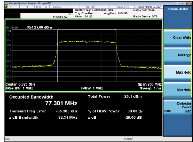
Plot 7-43. 26dB & 99% Bandwidth Plot Antenna 3a (80MHz 802.11ax (UNII Band 5) – Ch. 87)
