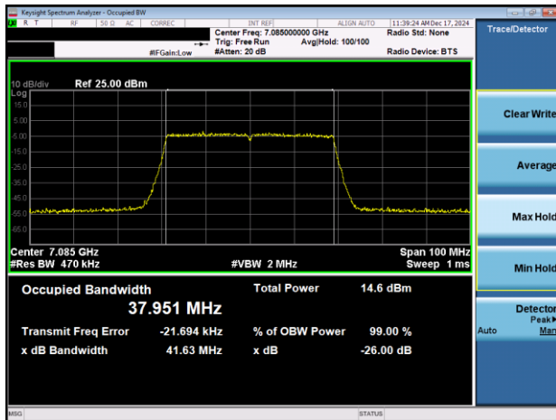
Plot 7-54. 26dB & 99% Bandwidth Plot Antenna 3a (40MHz 802.11ax (UNII Band 8) – Ch. 227)
