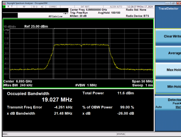
Plot 7-53. 26dB & 99% Bandwidth Plot Antenna 3a (20MHz 802.11ax (UNII Band 8) – Ch. 189)
