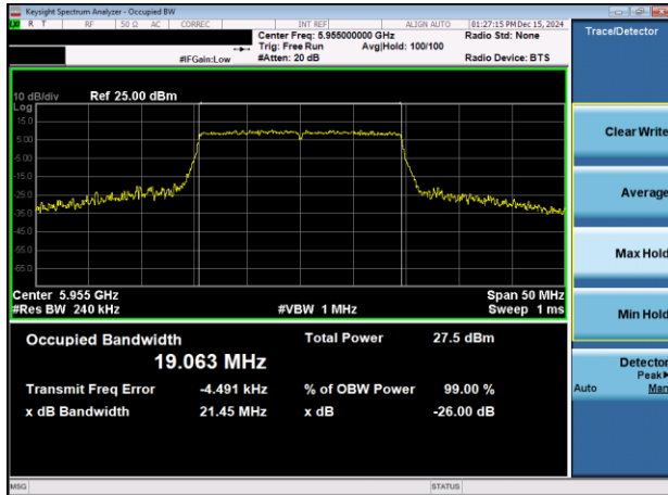
Plot 7-1. 26dB & 99% Bandwidth Plot Antenna 3c (20MHz 802.11ax (UNII Band 5) – Ch. 1)
