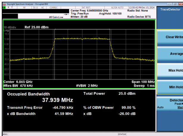
Plot 7-10. 26dB & 99% Bandwidth Plot Antenna 3c (40MHz 802.11ax (UNII Band 7) – Ch. 179)
