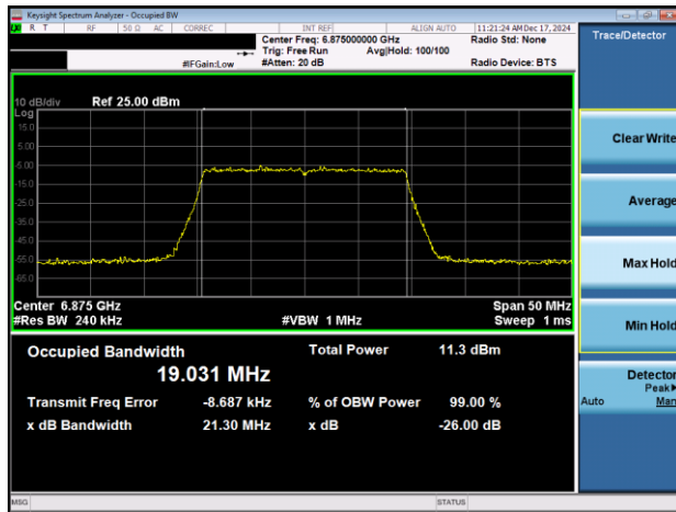
Plot 7-49. 26dB & 99% Bandwidth Plot Antenna 3a (20MHz 802.11ax (UNII Band 7) – Ch. 185)
