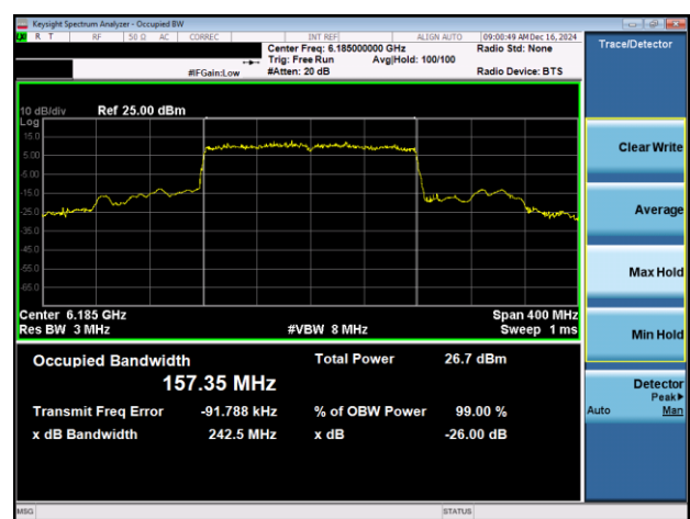
Plot 7-32. 26dB & 99% Bandwidth Plot Antenna 3a (160MHz 802.11ax (UNII Band 5) – Ch. 47)
