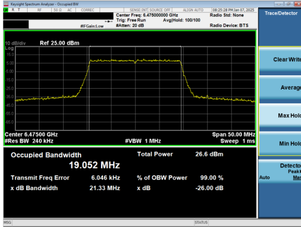
Plot 7-5. 26dB & 99% Bandwidth Plot Antenna 3c (20MHz 802.11ax (UNII Band 6) – Ch. 105)
