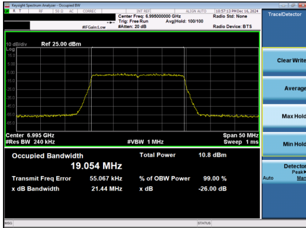
Plot 7-25. 26dB & 99% Bandwidth Plot Antenna 3c (20MHz 802.11ax (UNII Band 8) – Ch. 209)
