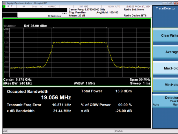
Plot 7-41. 26dB & 99% Bandwidth Plot Antenna 3a (20MHz 802.11ax (UNII Band 5) – Ch. 45)
