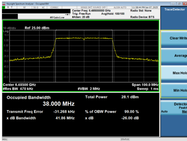
Plot 7-34. 26dB & 99% Bandwidth Plot Antenna 3a (40MHz 802.11ax (UNII Band 6) – Ch. 107)
