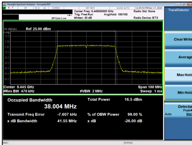
Plot 7-46. 26dB & 99% Bandwidth Plot Antenna 3a (40MHz 802.11ax (UNII Band 6) – Ch. 99)
