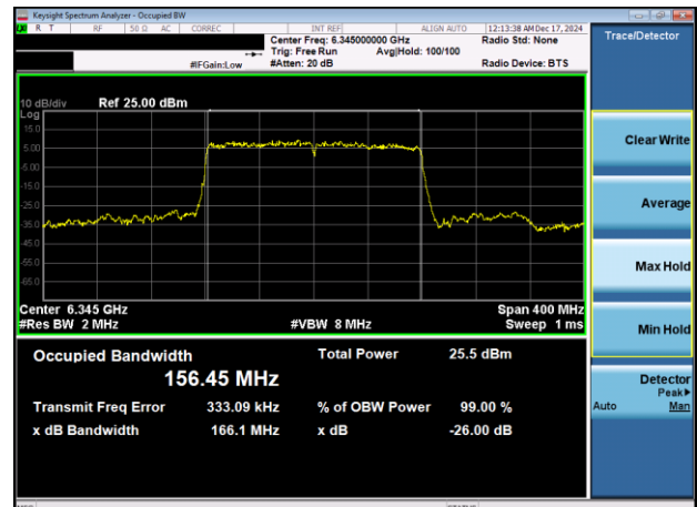
Plot 7-16. 26dB & 99% Bandwidth Plot Antenna 3c (160MHz 802.11ax (UNII Band 5) – Ch. 79)
