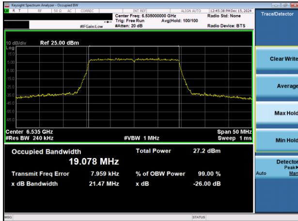
Plot 7-9. 26dB & 99% Bandwidth Plot Antenna 3c (20MHz 802.11ax (UNII Band 7) – Ch. 117)
