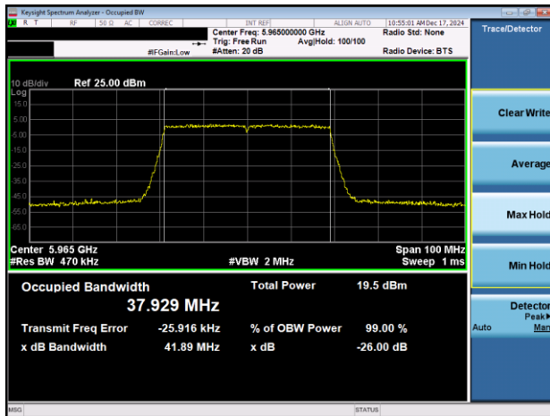
Plot 7-42. 26dB & 99% Bandwidth Plot Antenna 3a (40MHz 802.11ax (UNII Band 5) – Ch. 3)
