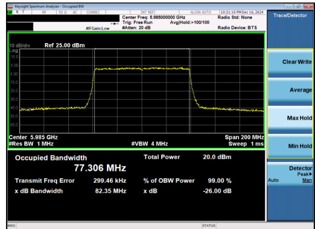
Plot 7-15. 26dB & 99% Bandwidth Plot Antenna 3c (80MHz 802.11ax (UNII Band 5) – Ch. 7)
