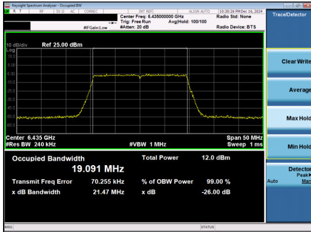
Plot 7-17. 26dB & 99% Bandwidth Plot Antenna 3c (20MHz 802.11ax (UNII Band 6) – Ch. 97)
