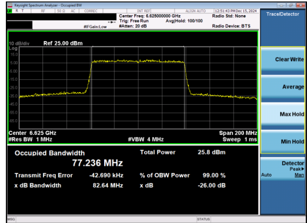
Plot 7-11. 26dB & 99% Bandwidth Plot Antenna 3c (80MHz 802.11ax (UNII Band 7) – Ch. 135)
