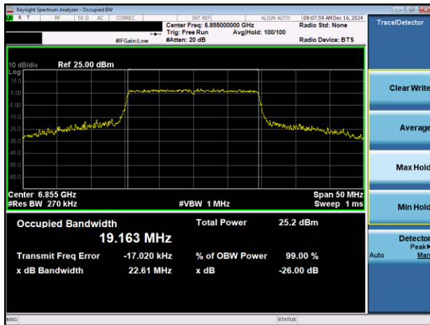
Plot 7-37. 26dB & 99% Bandwidth Plot Antenna 3a (20MHz 802.11ax (UNII Band 7) – Ch. 181)
