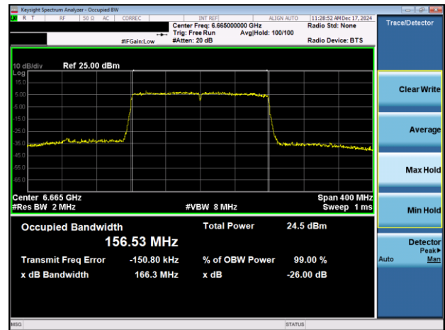
Plot 7-52. 26dB & 99% Bandwidth Plot Antenna 3a (160MHz 802.11ax (UNII Band 7) – Ch. 143)
