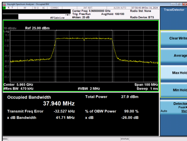
Plot 7-30. 26dB & 99% Bandwidth Plot Antenna 3a (40MHz 802.11ax (UNII Band 5) – Ch. 3)
