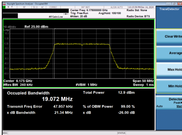
Plot 7-13. 26dB & 99% Bandwidth Plot Antenna 3c (20MHz 802.11ax (UNII Band 5) – Ch. 45)
