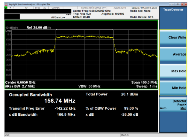
Plot 7-12. 26dB & 99% Bandwidth Plot Antenna 3c (160MHz 802.11ax (UNII Band 7) – Ch. 143)
