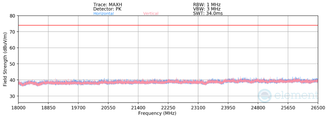
Plot 7-38. Radiated Spurious Emissions Above 18GHz Antenna 3a (802.15.4 ePA – Ch. 25)
