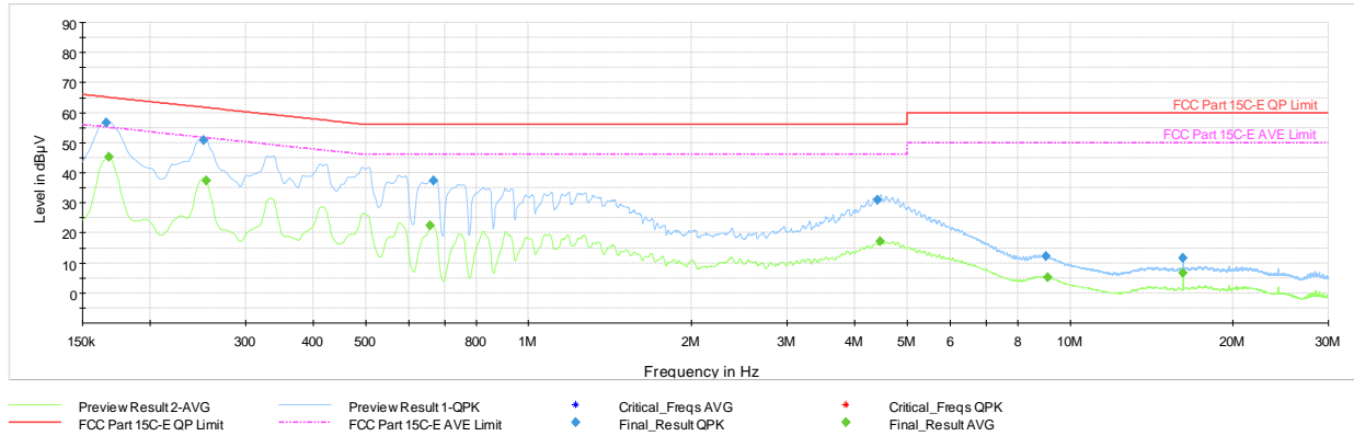
Plot 7-48. AC Line Conducted Emission with 802.15.4 Antenna 3a (N, Ch.25 - ePA, with AC/DC Adapter via USB-C cable with wire charger)
