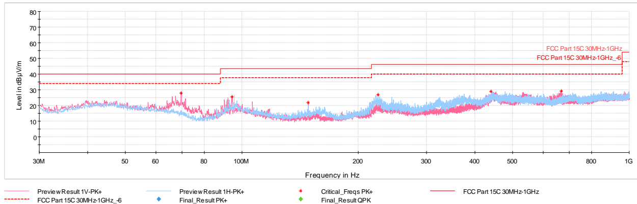
Plot 7-46. Radiated Spurious Emissions 30MHz-1GHz Antenna 3a (ePA - Ch.25, with AC/DC Adapter via USB-C cable with wire charger)
