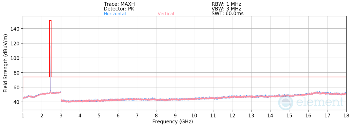
Plot 7-40. Radiated Spurious Emissions 1-18GHz Antenna 1a (802.15.4 ePA – Ch. 18)
