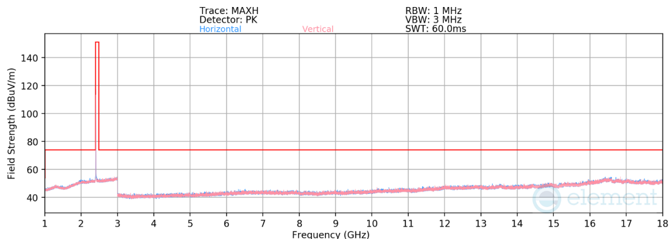
Plot 7-39. Radiated Spurious Emissions 1-18GHz Antenna 1a (802.15.4 ePA – Ch. 11)
