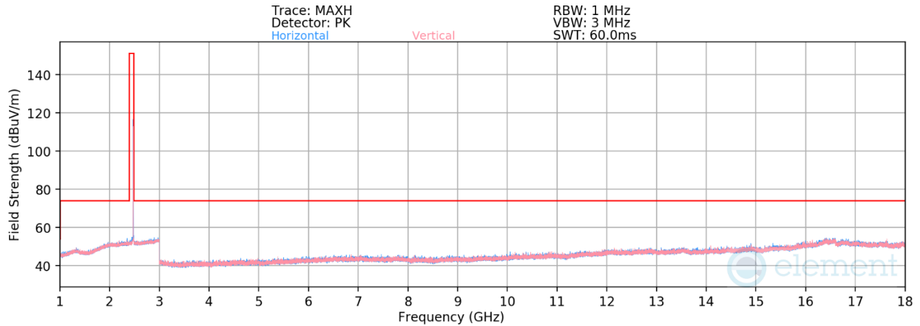
Plot 7-41. Radiated Spurious Emissions 1-18GHz Antenna 1a (802.15.4 ePA – Ch. 25)
