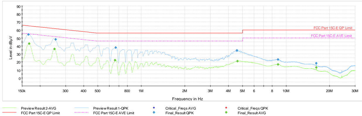
Plot 7-47. AC Line Conducted Emission with 802.15.4 Antenna 3a (L1, Ch.25 - ePA, with AC/DC Adapter via USB-C cable with wire charger)
