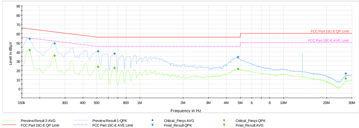
Plot 7-5. AC Line-Conducted Plot (N, Charging Rate 2.6C, with AC/DC Adapter)
