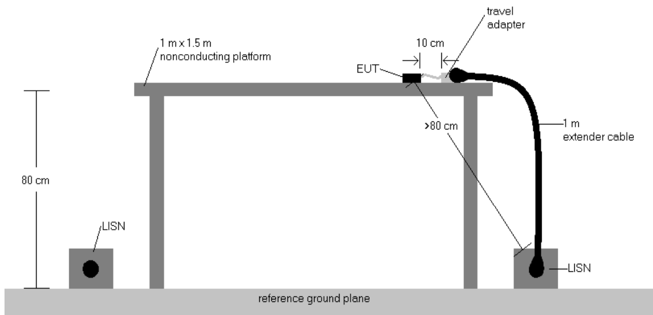
Figure 7-9. Test Instrument & Measurement Setup
