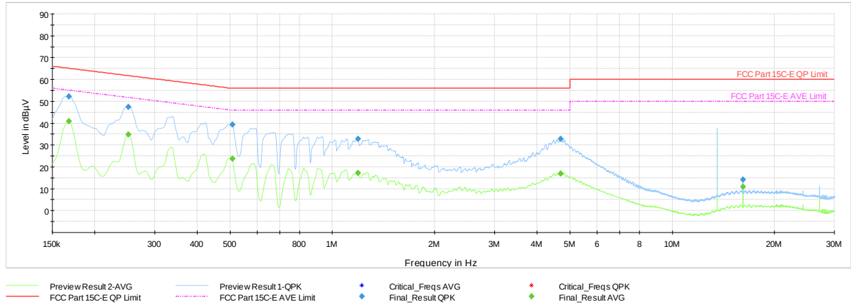
Plot 7-4. AC Line-Conducted Plot (L1, Charging Rate 2.6C, with AC/DC Adapter)
