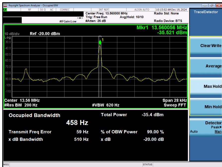
Figure 7-3. 20dB and 99% Bandwidth Communication Mode Plot
