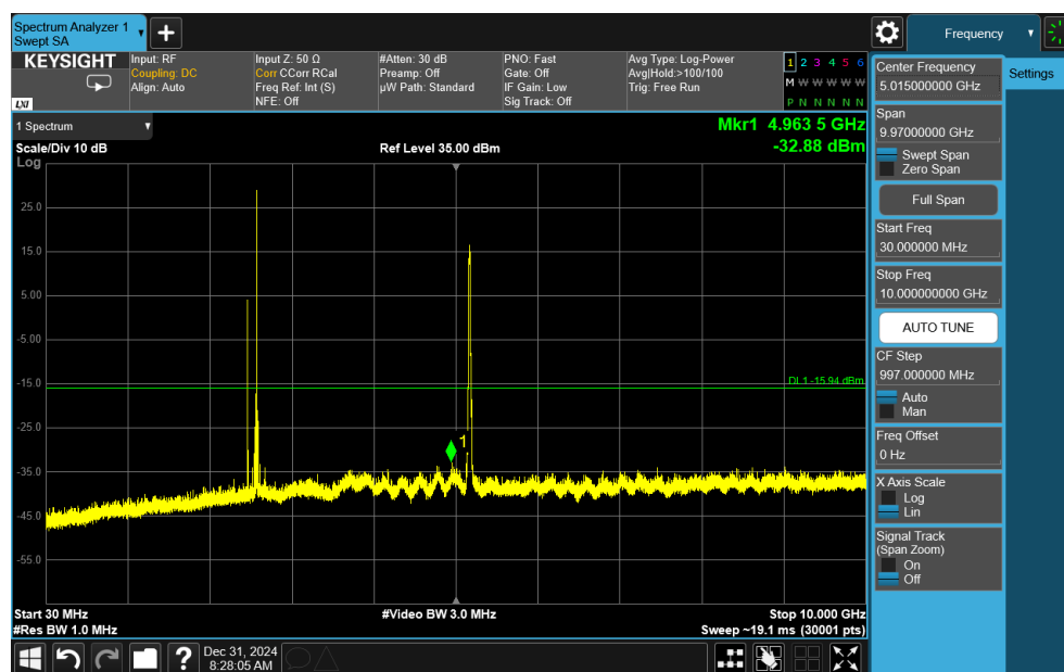
Plot 7-57. Conducted Simultaneous Tx Spurious Plots Antenna3a (Bluetooth + LTE B41 + UNII)
