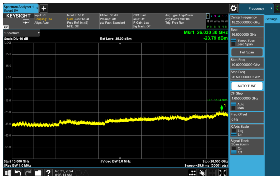
Plot 7-58. Conducted Simultaneous Tx Spurious Plots Antenna3a (Bluetooth + LTE B41 + UNII)
