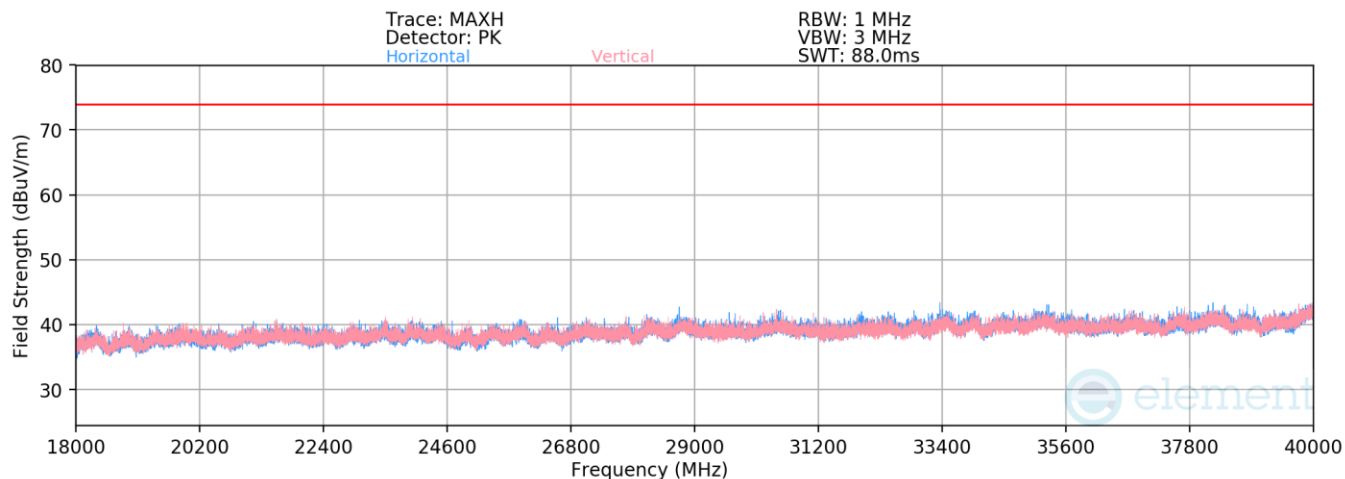
Plot 7-64. Radiated Spurious Emissions – Simultaneous Transmission Above 18GHz
