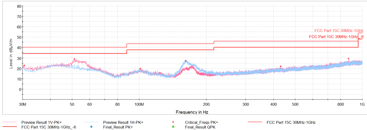
Plot 7-78. Radiated Spurious Emissions – Simultaneous Transmission Below 1GHz (with AC/DC Adapter)
