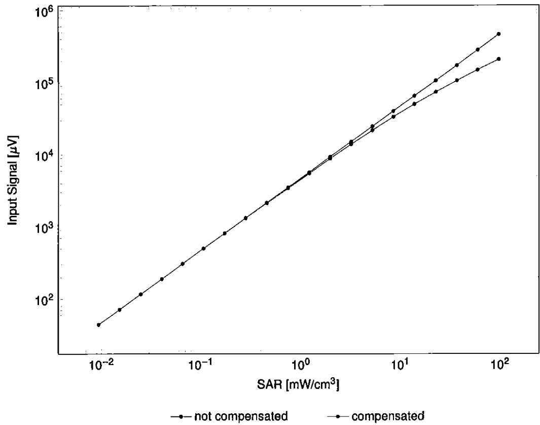
Dynamic Range f(SAR head ) (TEM cell, f aval = 1900MHz)
