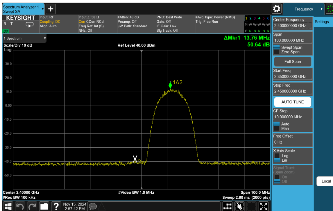
Plot 7-68. Band Edge Plot Antenna 1a (802.11b – Ch. 1)
