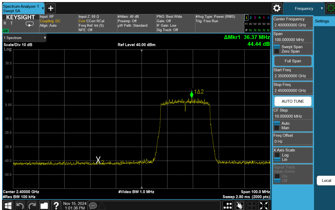
Plot 7-56. Band Edge Plot Antenna 3a (802.11ax (SU - 2.4GHz) – Ch. 2)
