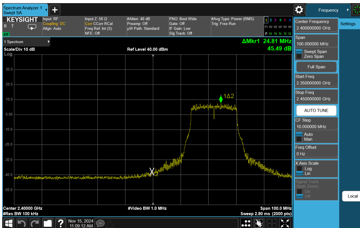
Plot 7-29. Band Edge Plot Antenna 3a (802.11g – Ch. 3)
