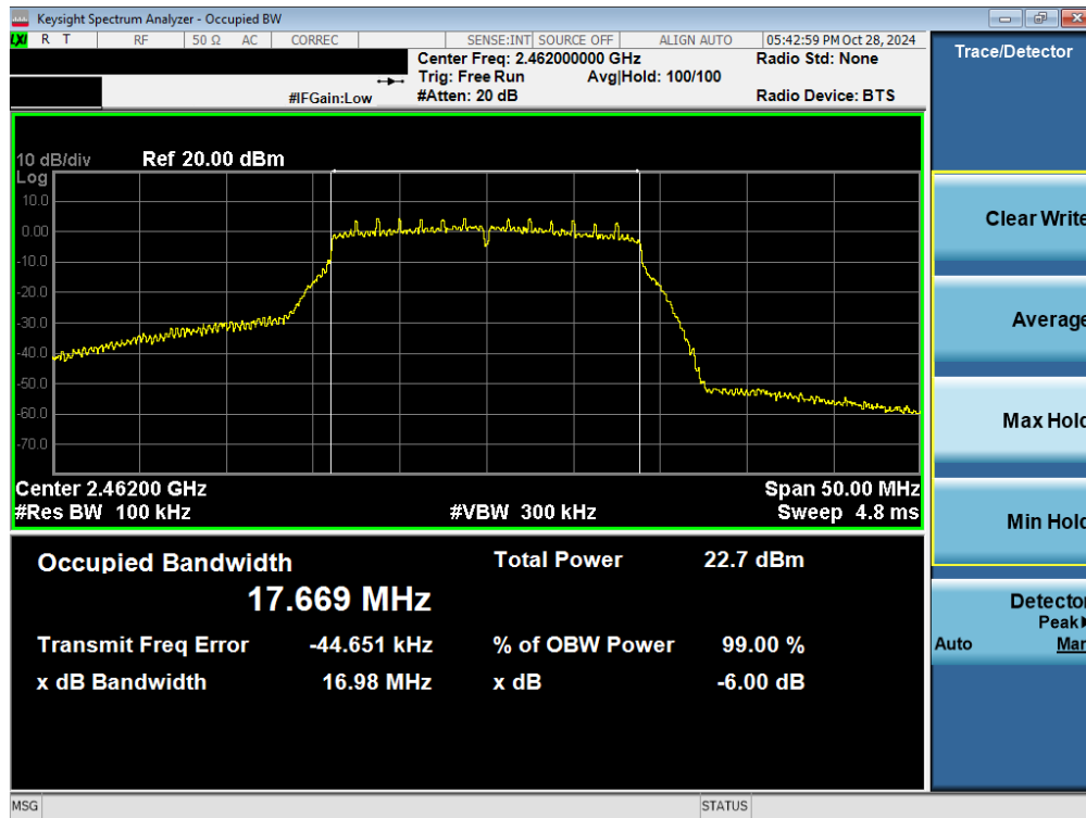
Plot 7-3. 6 dB BW and 99% OBW Plot Antenna 3a (802.11n – Ch. 11)
