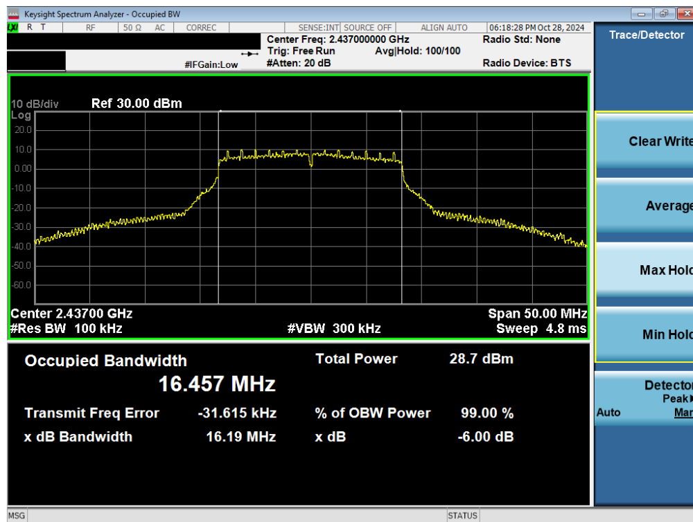
Plot 7-6. 6 dB BW and 99% OBW Plot Antenna 1a (802.11g – Ch. 6)
