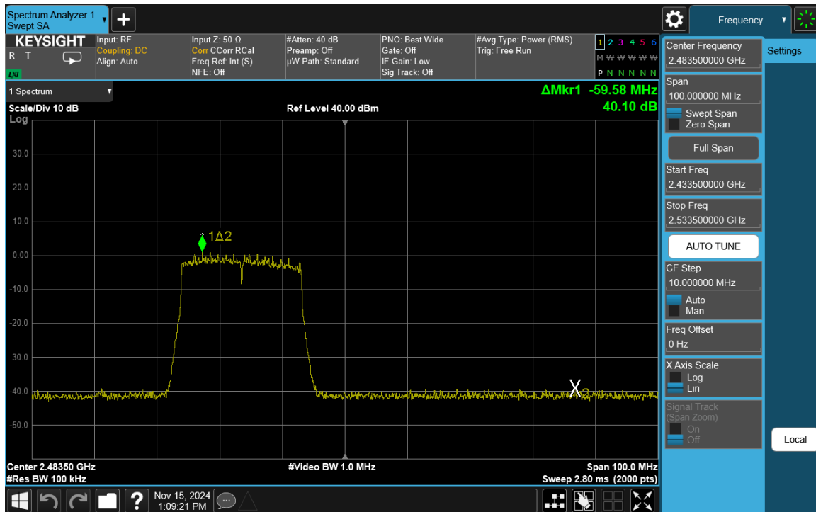
Plot 7-67. Band Edge Plot Antenna 3a (802.11ax (SU - 2.4GHz) – Ch. 12)
