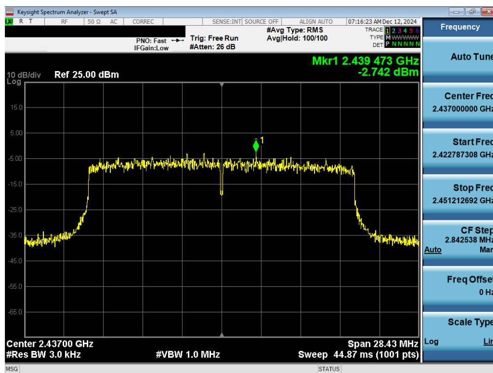
Plot 7-22. Power Spectral Density Plot CDD Antenna 1a (802.11axSU – Ch. 6)
