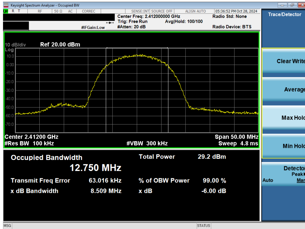
Plot 7-1. 6 dB BW and 99% OBW Plot Antenna 3a (802.11b – Ch. 1)
