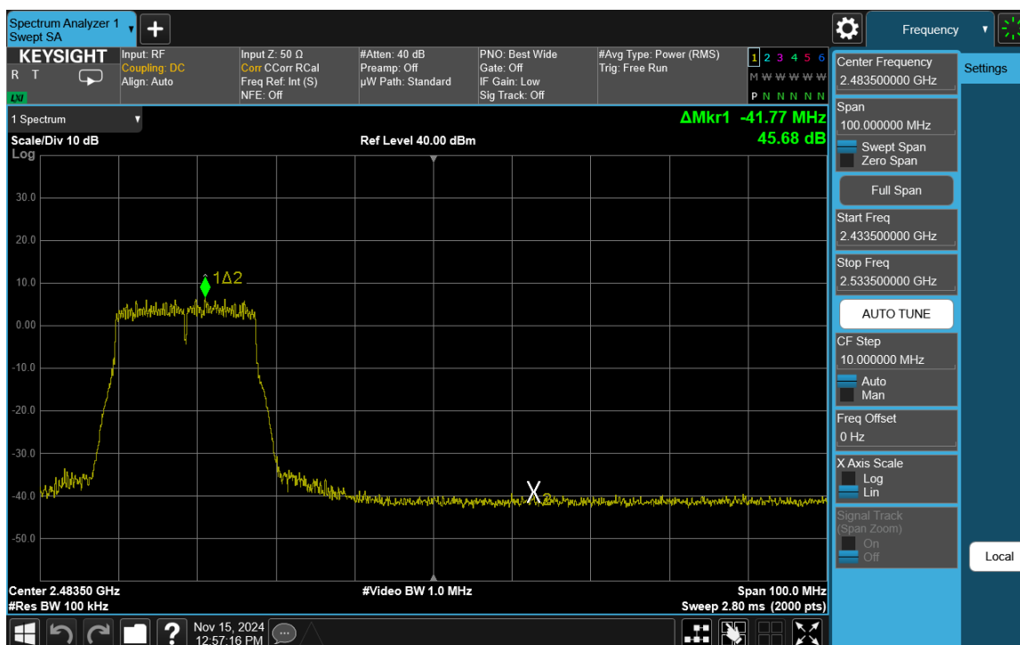
Plot 7-50. Band Edge Plot Antenna 3a (802.11n (2.4GHz) – Ch. 9)
