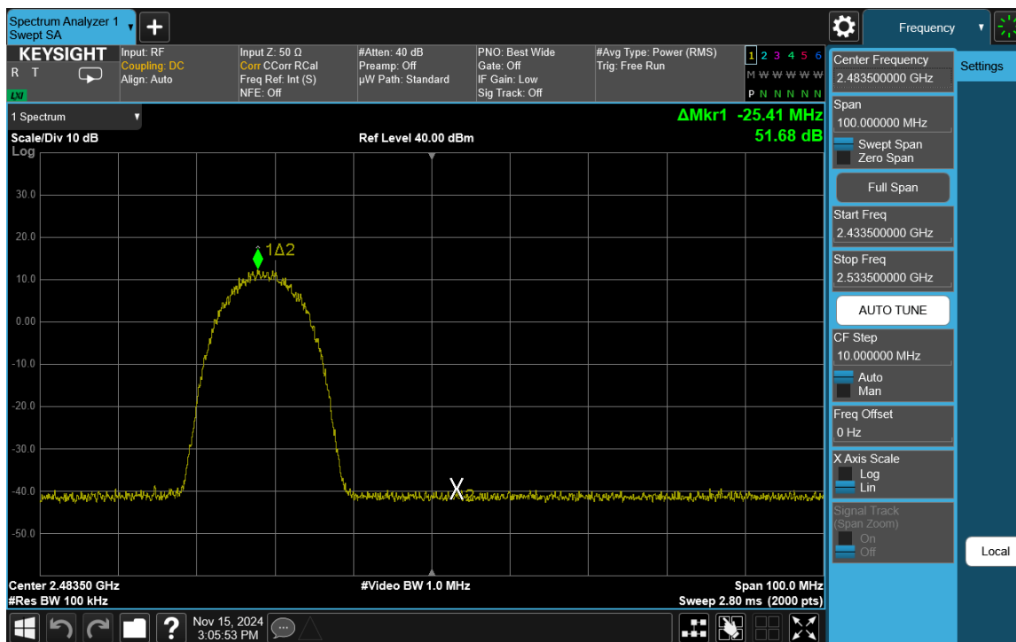
Plot 7-69. Band Edge Plot Antenna 1a (802.11b – Ch. 11)
