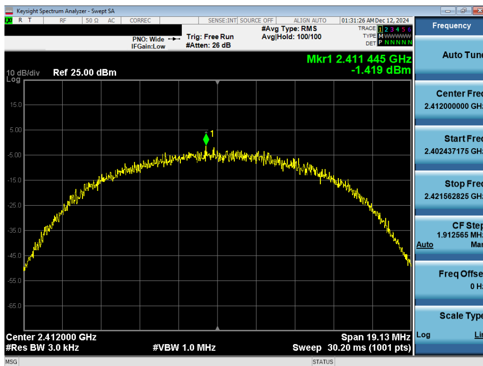
Plot 7-9. Power Spectral Density Plot Antenna 3a (802.11b – Ch. 1)
