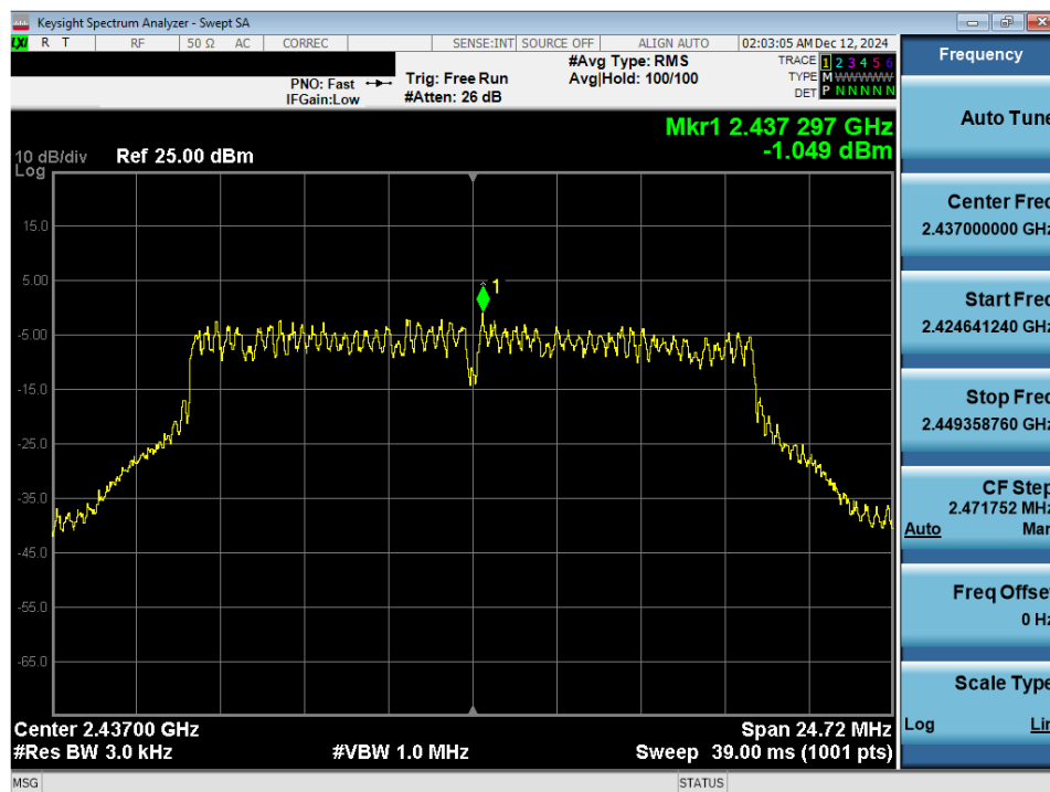
Plot 7-17. Power Spectral Density Plot CDD Antenna 3a (802.11g – Ch. 6)
