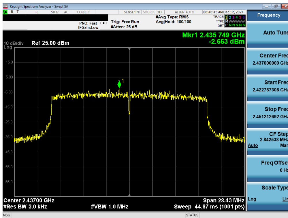
Plot 7-16. Power Spectral Density Plot Antenna 1a (802.11axSU – Ch. 6)
