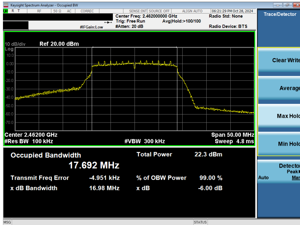
Plot 7-7. 6 dB BW and 99% OBW Plot Antenna 1a (802.11n – Ch. 11)
