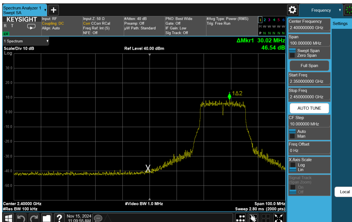
Plot 7-30. Band Edge Plot Antenna 3a (802.11g – Ch. 4)
