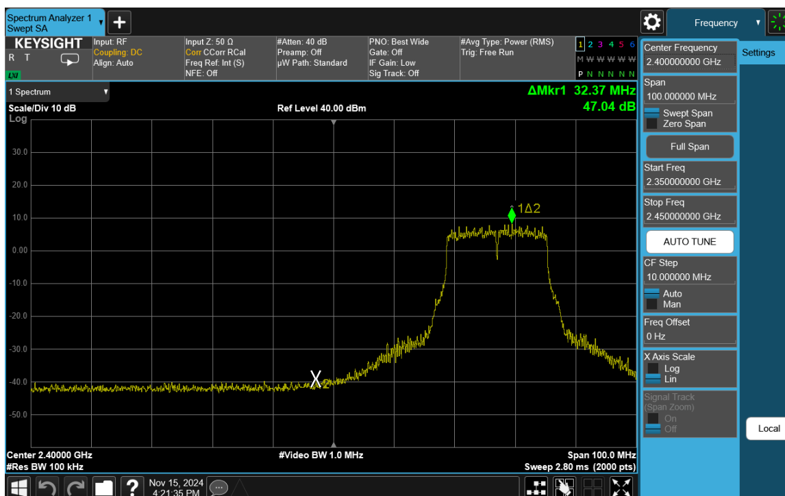
Plot 7-75. Band Edge Plot Antenna 1a (802.11g – Ch. 4)
