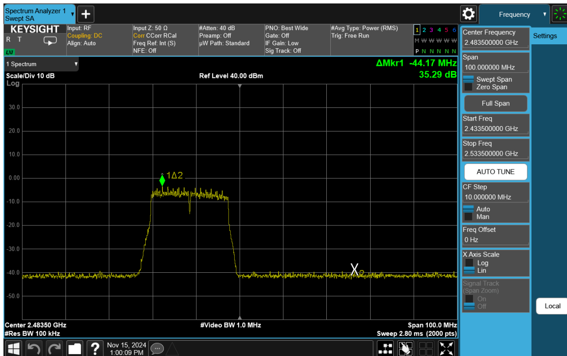
Plot 7-54. Band Edge Plot Antenna 3a (802.11n (2.4GHz) – Ch. 13)
