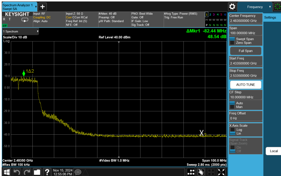
Plot 7-47. Band Edge Plot Antenna 3a (802.11n (2.4GHz) – Ch. 6-High)
