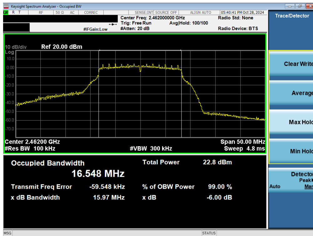
Plot 7-2. 6 dB BW and 99% OBW Plot Antenna 3a (802.11g – Ch. 11)
