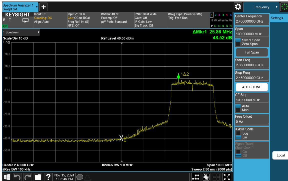
Plot 7-59. Band Edge Plot Antenna 3a (802.11ax (SU - 2.4GHz) – Ch. 5)
