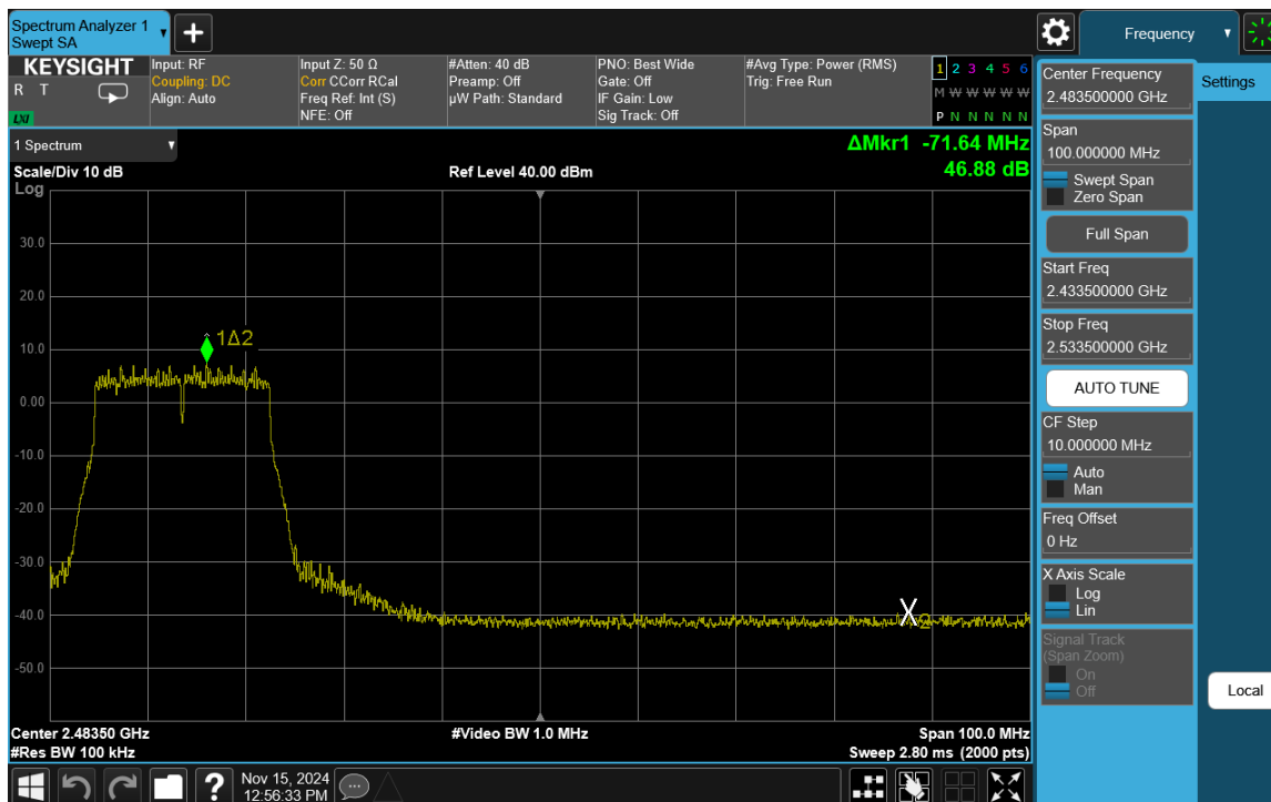
Plot 7-49. Band Edge Plot Antenna 3a (802.11n (2.4GHz) – Ch. 8)
