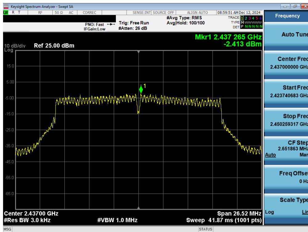
Plot 7-11. Power Spectral Density Plot Antenna 3a (802.11n – Ch. 6)
