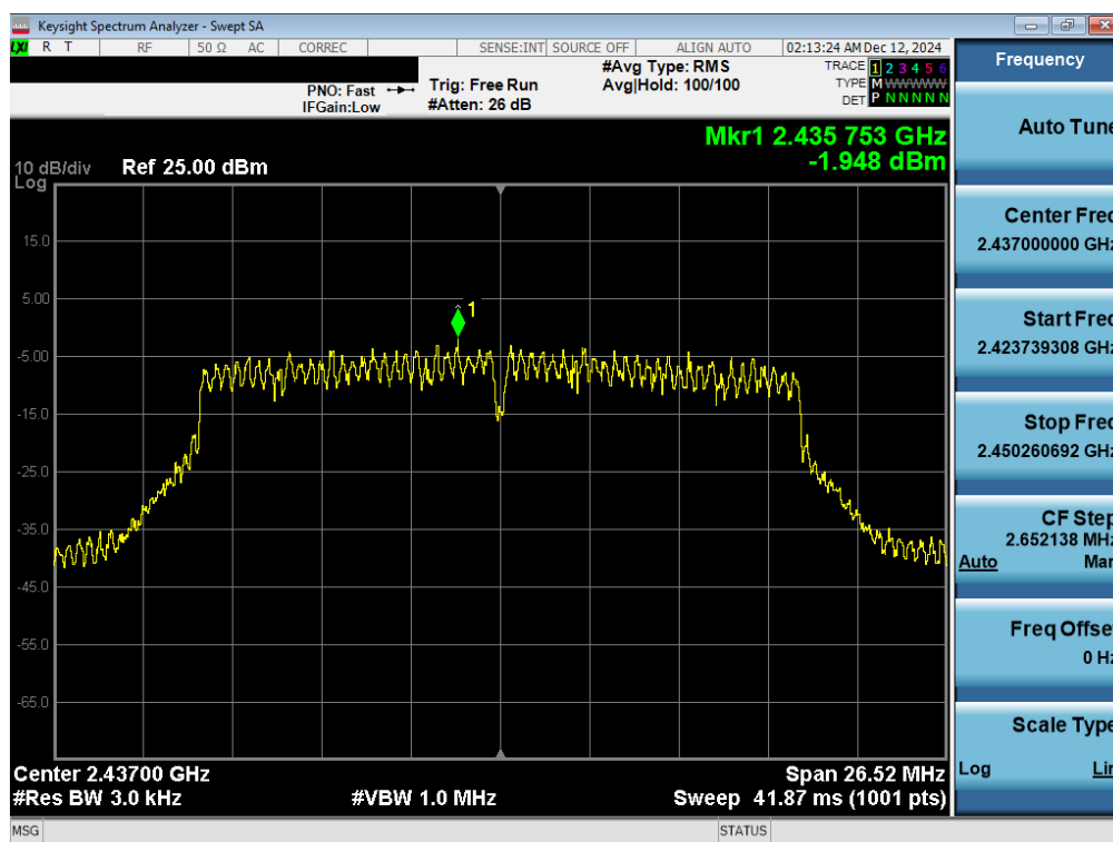
Plot 7-19. Power Spectral Density Plot CDD Antenna 3a (802.11n – Ch. 6)
