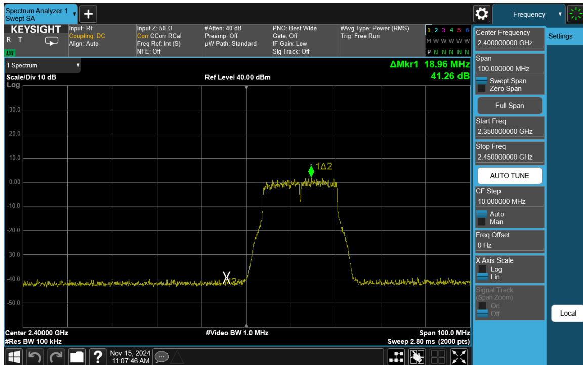
Plot 7-27. Band Edge Plot Antenna 3a (802.11g – Ch. 1)
