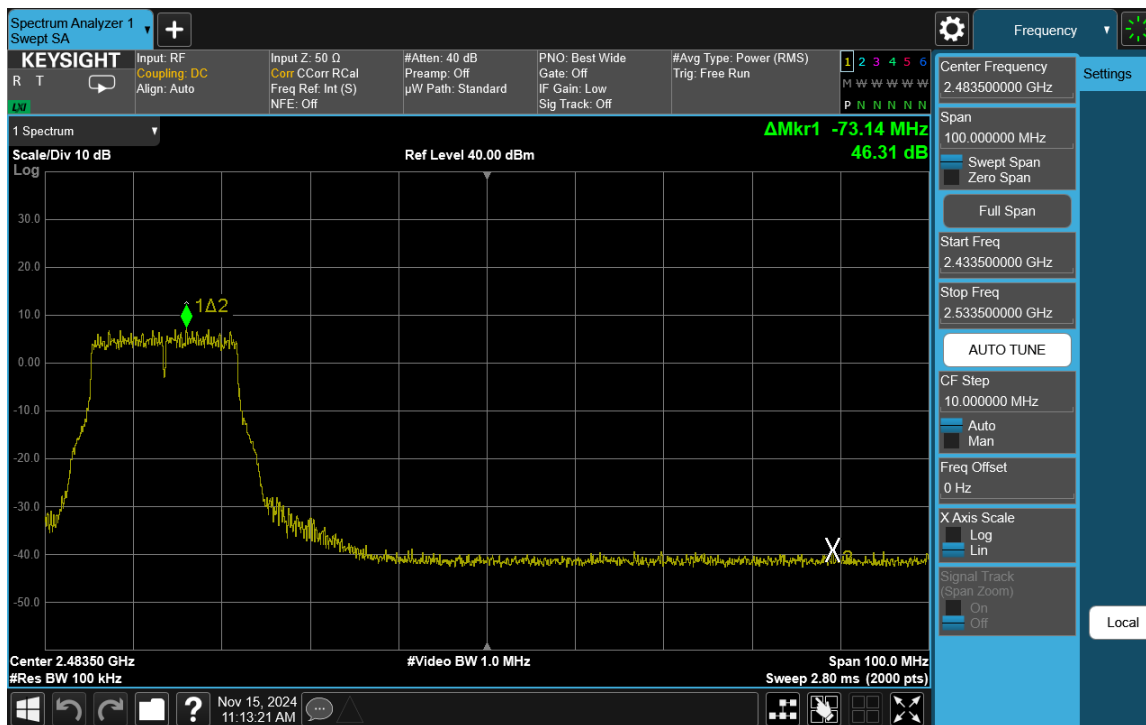
Plot 7-35. Band Edge Plot Antenna 3a (802.11g – Ch. 8)
