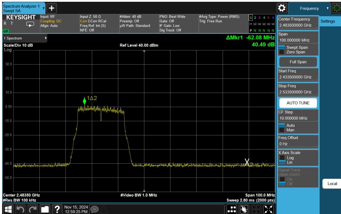
Plot 7-53. Band Edge Plot Antenna 3a (802.11n (2.4GHz) – Ch. 12)
