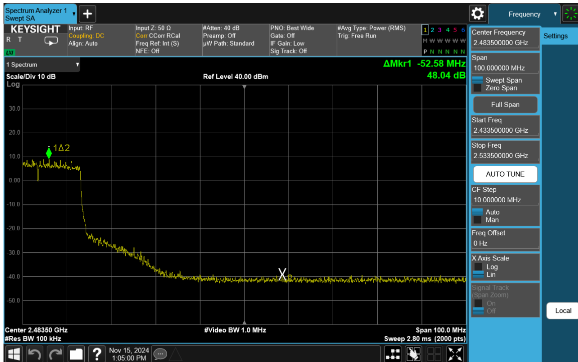
Plot 7-61. Band Edge Plot Antenna 3a (802.11ax (SU - 2.4GHz) – Ch. 6-High)
