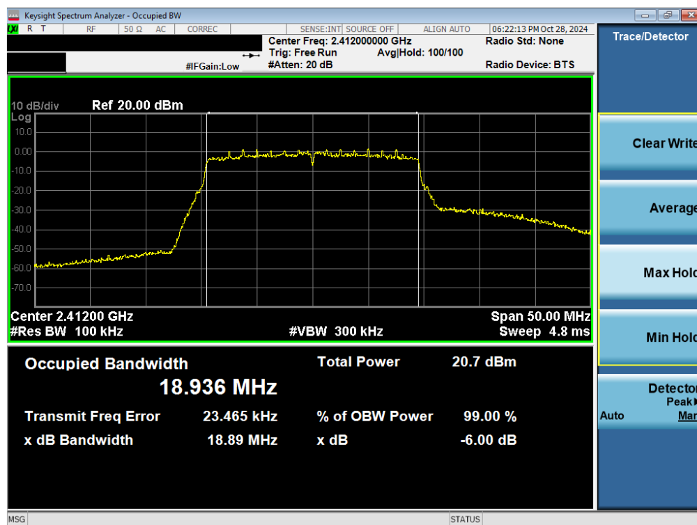
Plot 7-8. 6 dB BW and 99% OBW Plot Antenna 1a (802.11axSU – Ch. 1)
