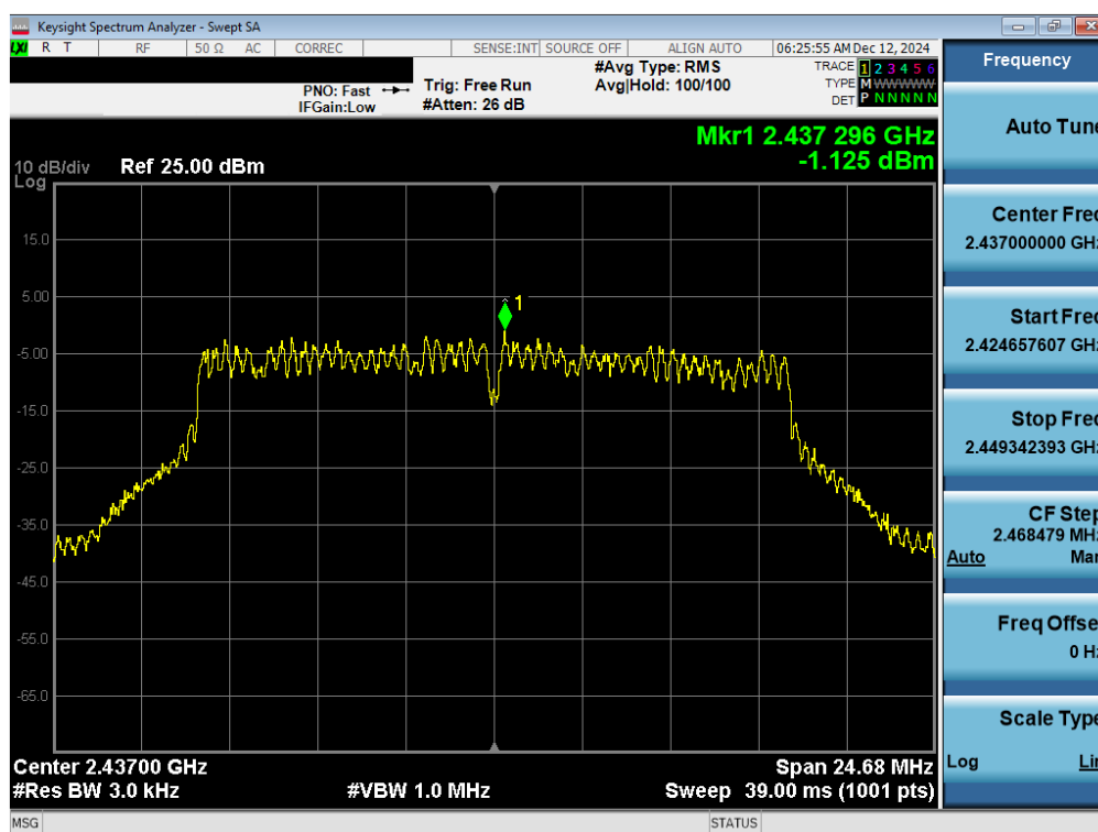
Plot 7-14. Power Spectral Density Plot Antenna 1a (802.11g – Ch. 6)
