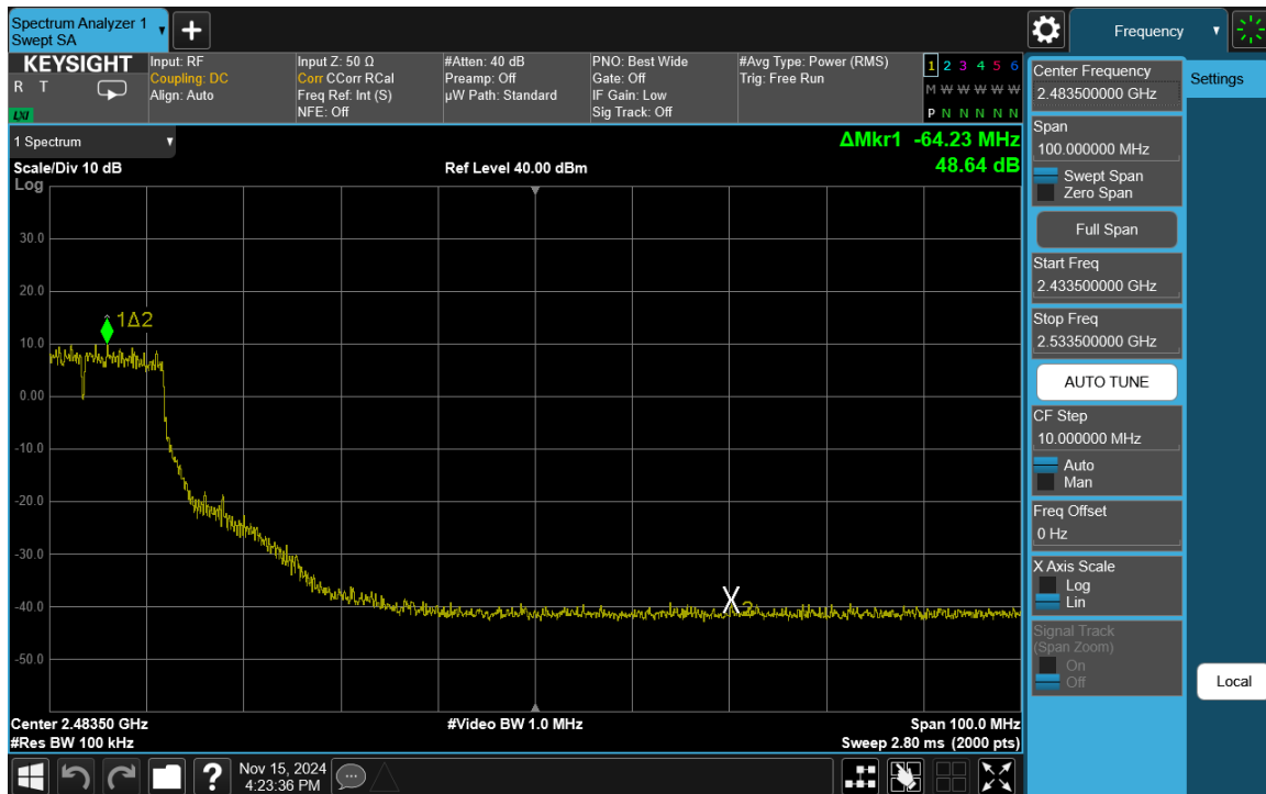
Plot 7-78. Band Edge Plot Antenna 1a (802.11g – Ch. 6-High)
