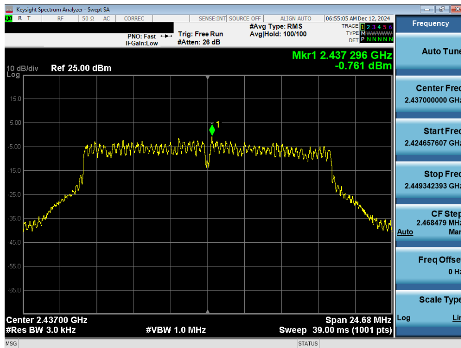
Plot 7-18. Power Spectral Density Plot CDD Antenna 1a (802.11g – Ch. 6)
