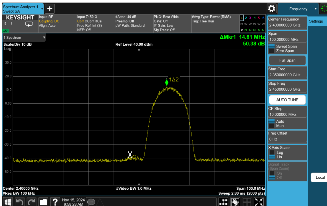
Plot 7-23. Band Edge Plot Antenna 3a (802.11b – Ch. 1)
