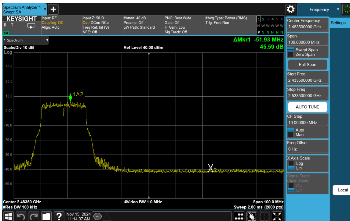
Plot 7-36. Band Edge Plot Antenna 3a (802.11g – Ch. 9)
