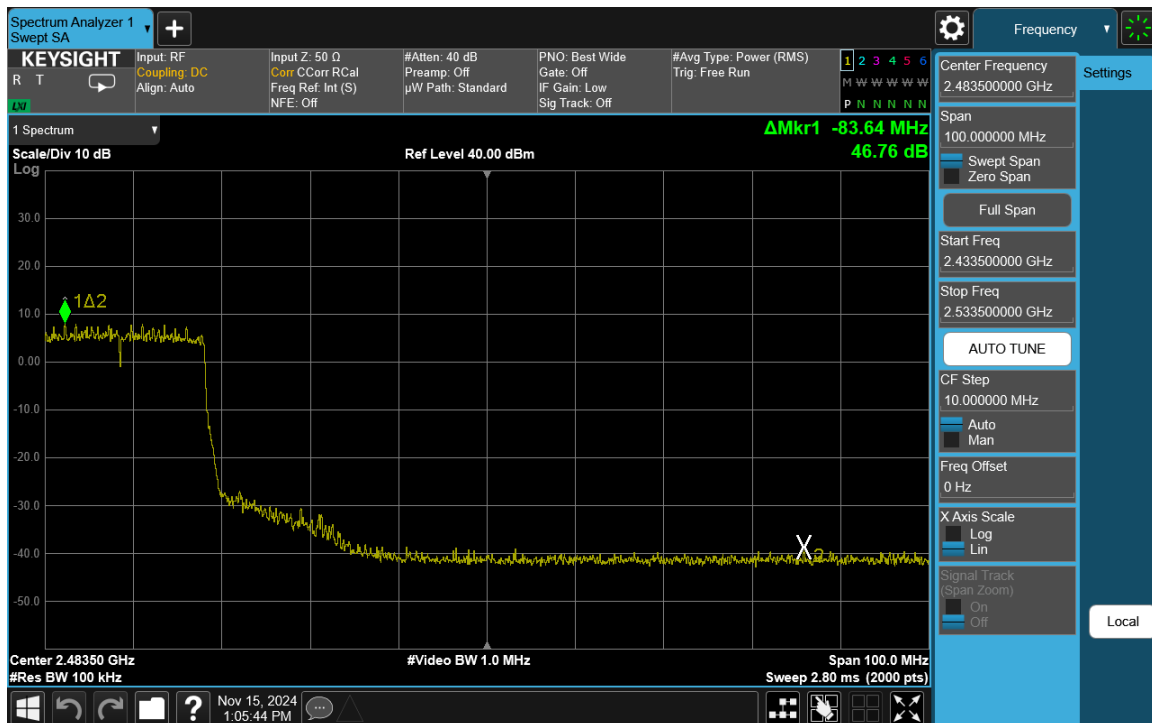
Plot 7-62. Band Edge Plot Antenna 3a (802.11ax (SU - 2.4GHz) – Ch. 7)
