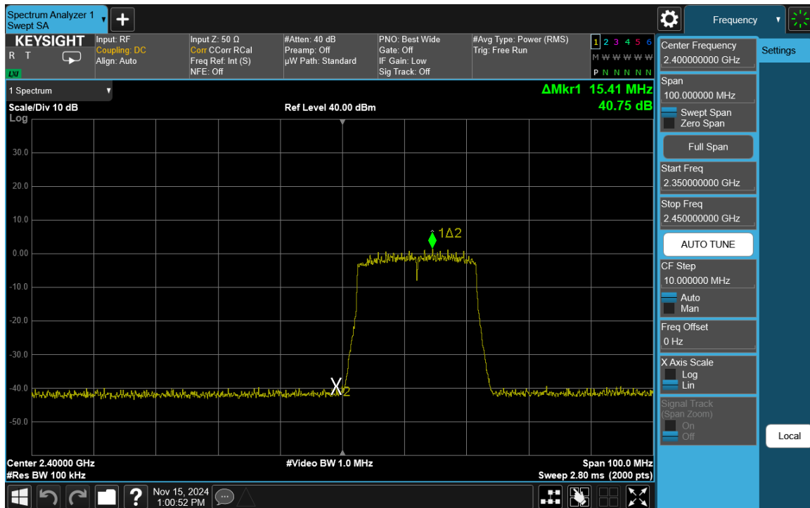
Plot 7-55. Band Edge Plot Antenna 3a (802.11ax (SU - 2.4GHz) – Ch. 1)
