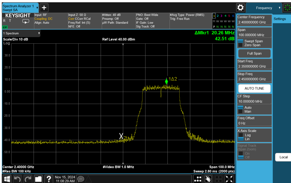
Plot 7-28. Band Edge Plot Antenna 3a (802.11g – Ch. 2)
