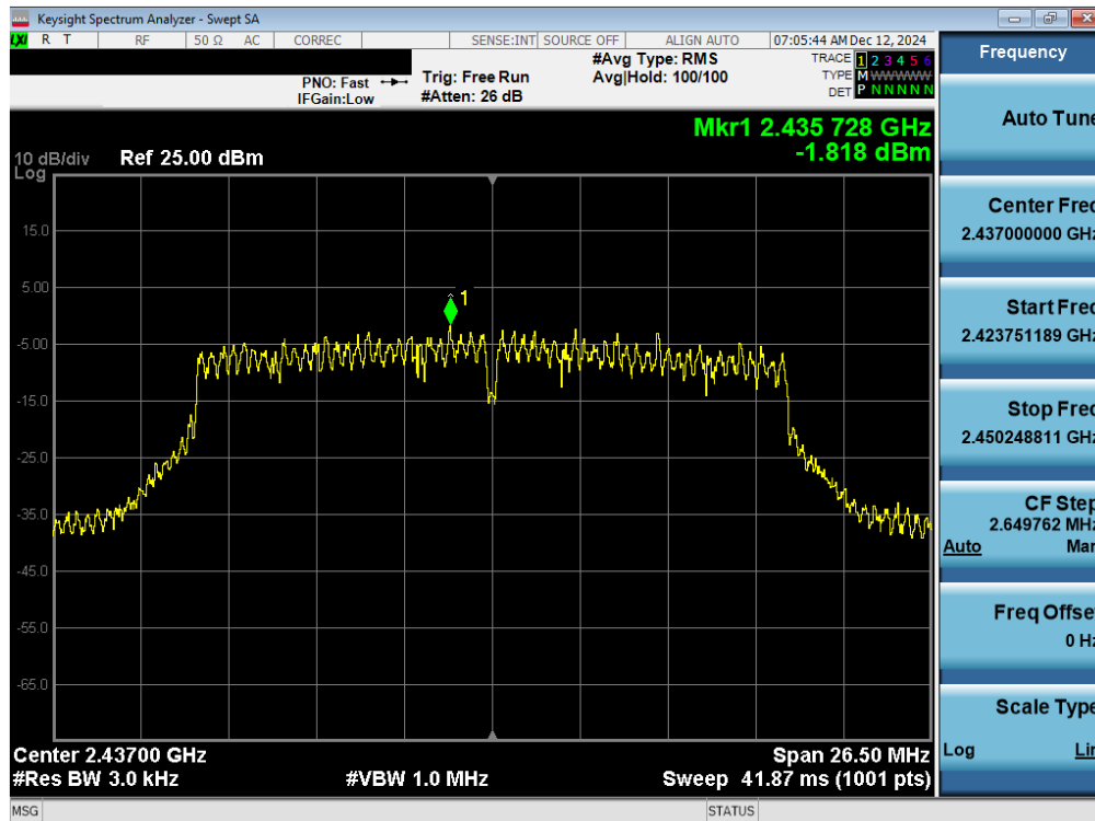
Plot 7-20. Power Spectral Density Plot CDD Antenna 1a (802.11n – Ch. 6)
