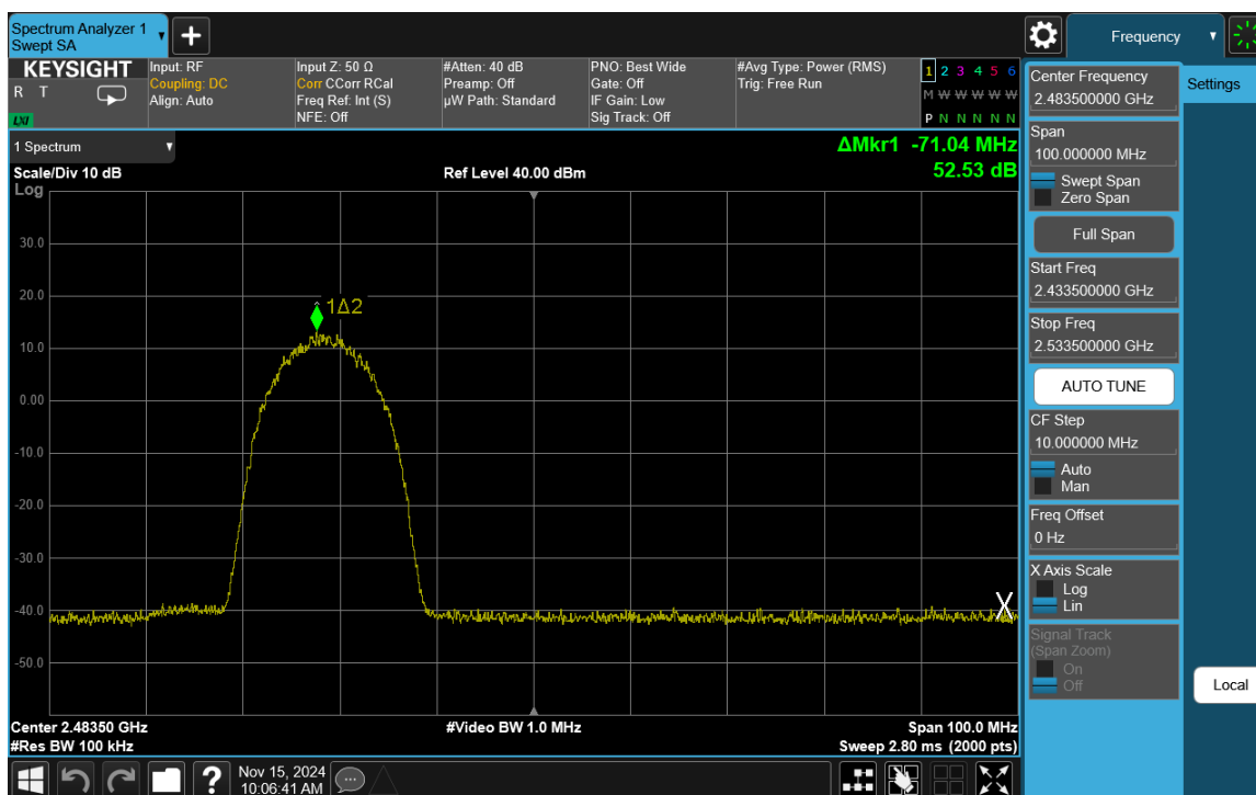
Plot 7-24. Band Edge Plot Antenna 3a (802.11b – Ch. 11)
