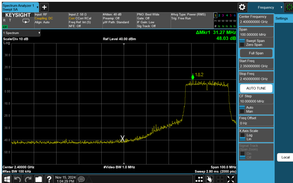
Plot 7-60. Band Edge Plot Antenna 3a (802.11ax (SU - 2.4GHz) – Ch. 6-Low)
