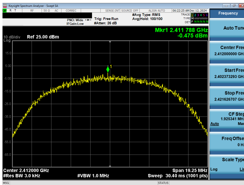
Plot 7-13. Power Spectral Density Plot Antenna 1a (802.11b – Ch. 1)
