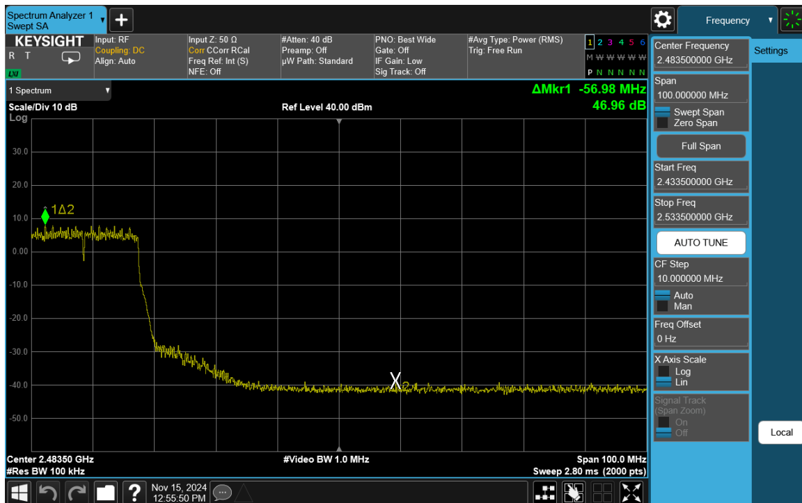
Plot 7-48. Band Edge Plot Antenna 3a (802.11n (2.4GHz) – Ch. 7)
