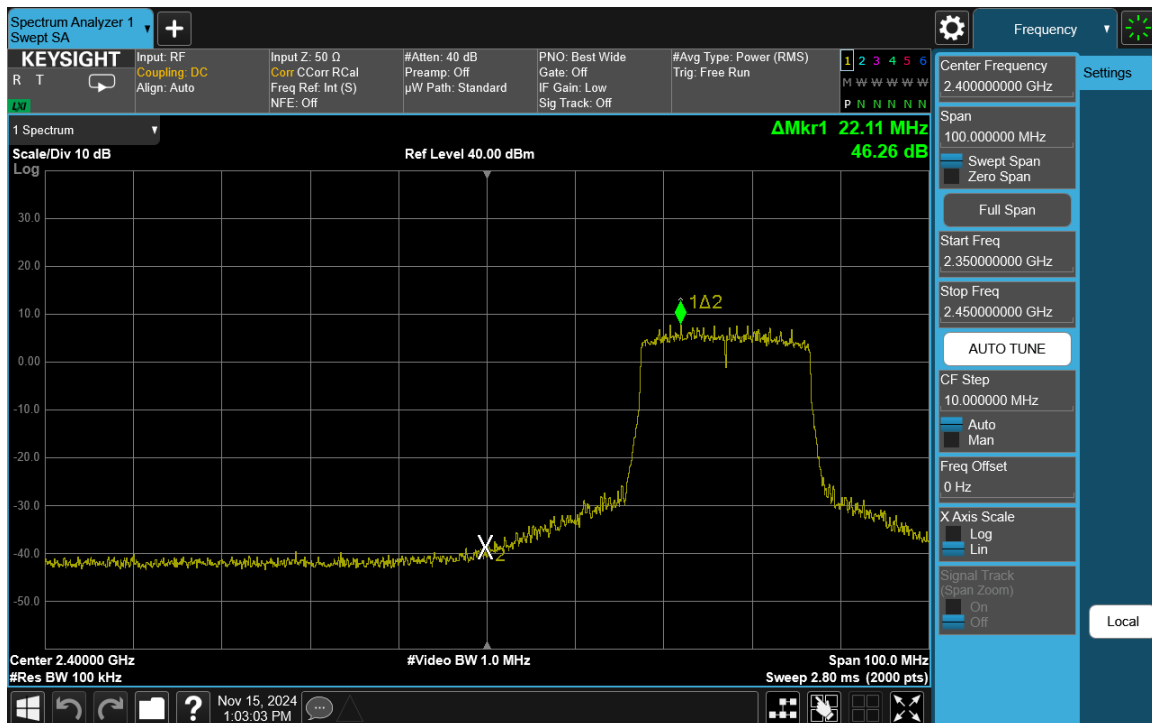
Plot 7-58. Band Edge Plot Antenna 3a (802.11ax (SU - 2.4GHz) – Ch. 4)
