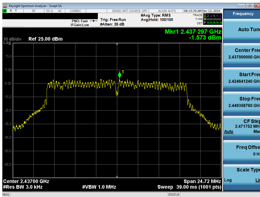
Plot 7-10. Power Spectral Density Plot Antenna 3a (802.11g – Ch. 6)
