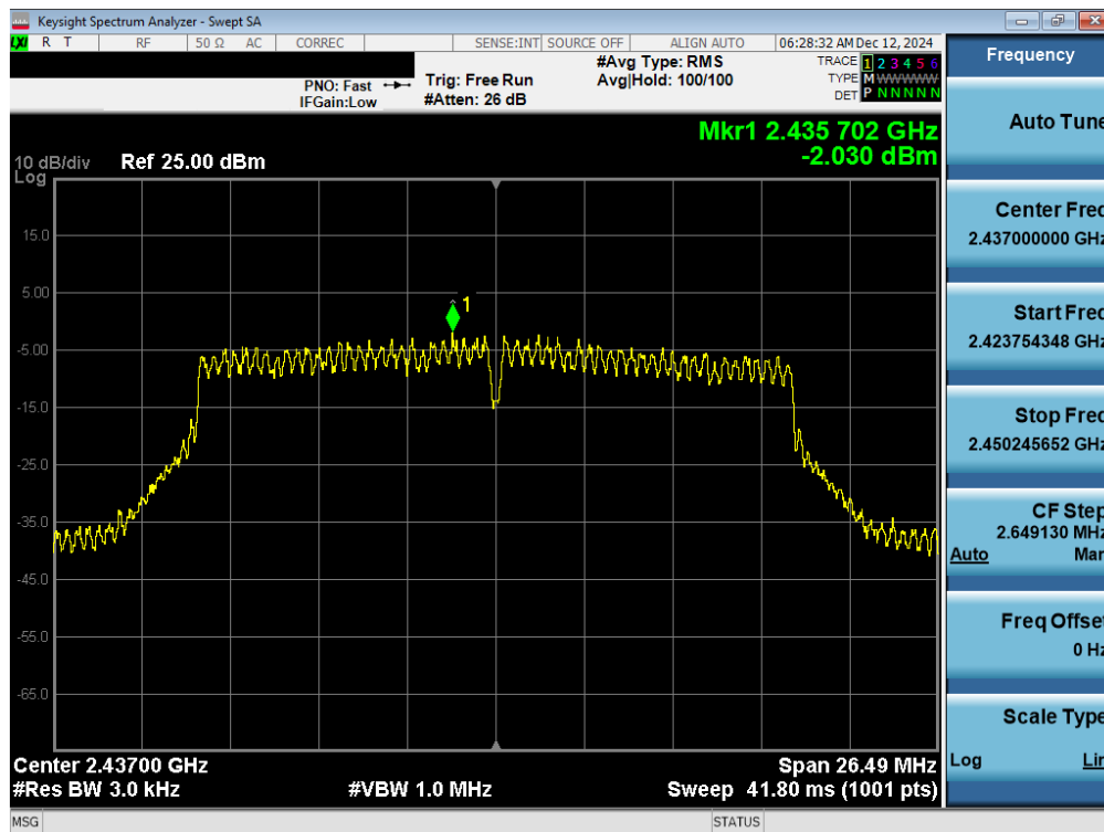
Plot 7-15. Power Spectral Density Plot Antenna 1a (802.11n – Ch. 6)
