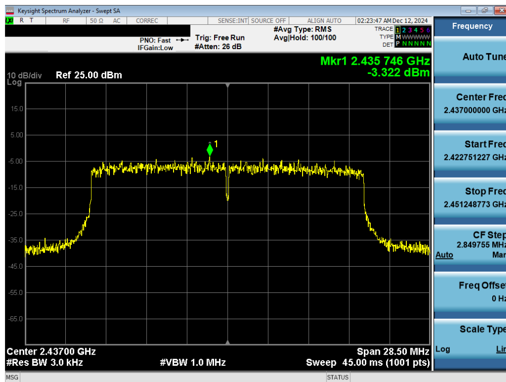
Plot 7-21. Power Spectral Density Plot CDD Antenna 3a (802.11axSU – Ch. 6)
