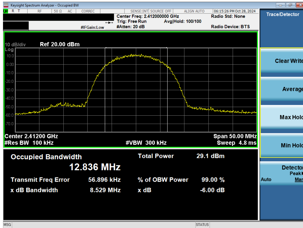
Plot 7-5. 6 dB BW and 99% OBW Plot Antenna 1a (802.11b – Ch. 1)
