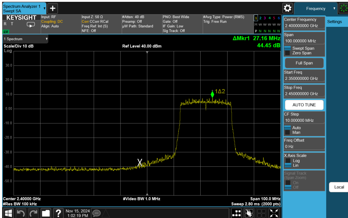
Plot 7-57. Band Edge Plot Antenna 3a (802.11ax (SU - 2.4GHz) – Ch. 3)
