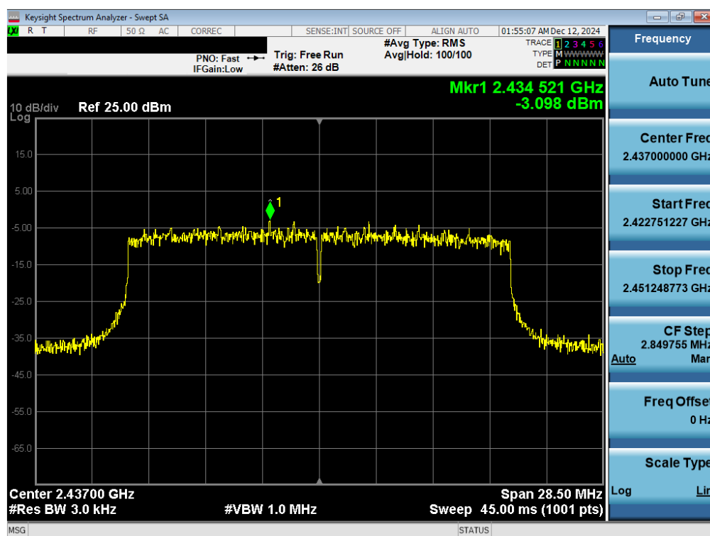
Plot 7-12. Power Spectral Density Plot Antenna 3a (802.11axSU – Ch. 6)
