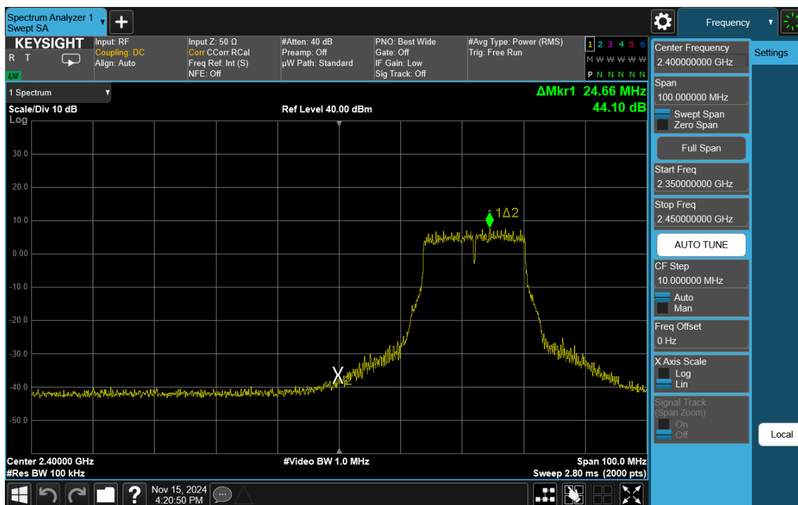
Plot 7-74. Band Edge Plot Antenna 1a (802.11g – Ch. 3)
